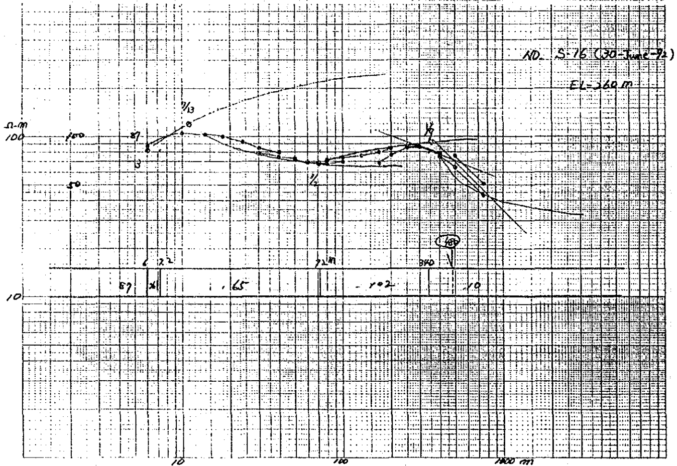
Fig. Result of Electrical Prospecting (ρ-a curve)
