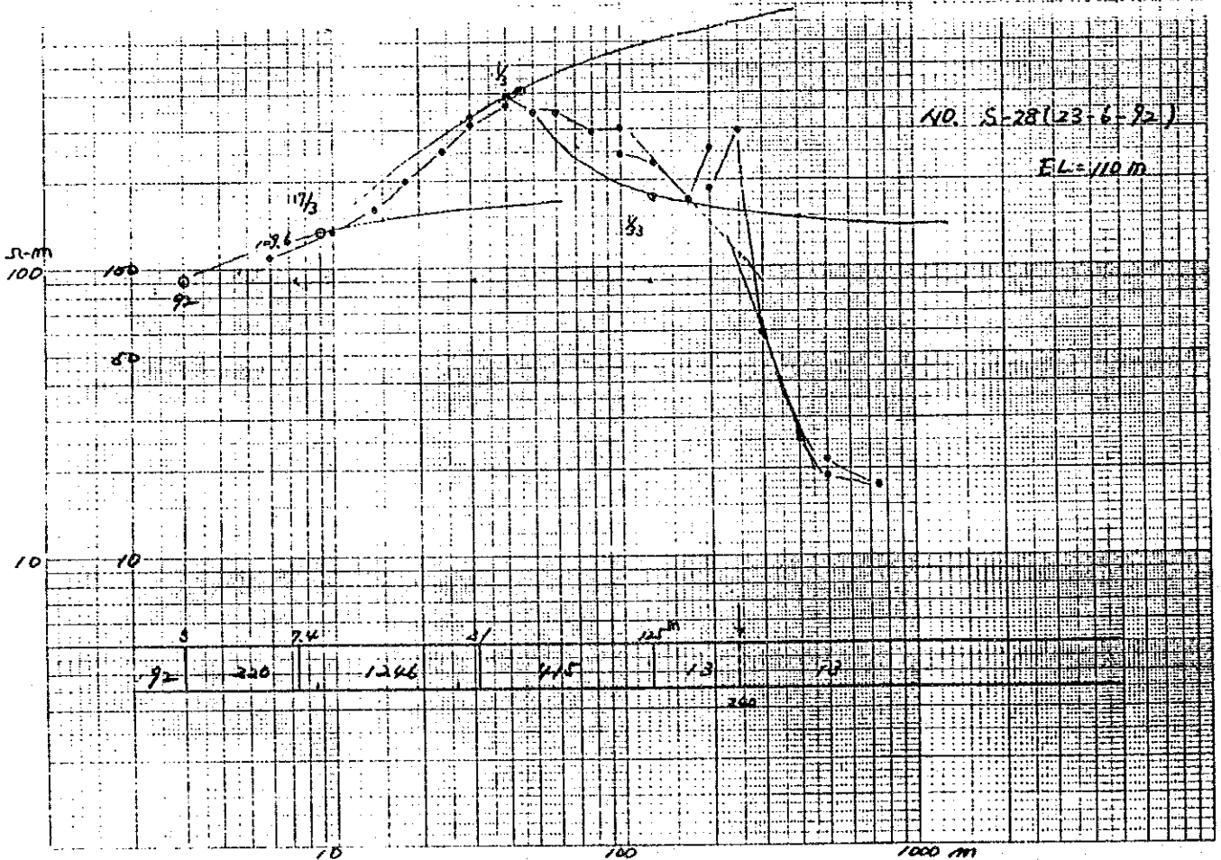
Fig. Result of Electrical Prospecting (p-a curve)
