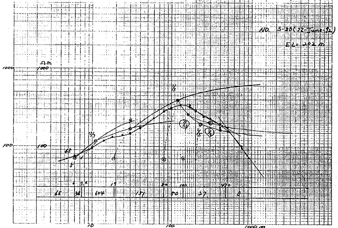
Fig. Result of Electrical Prospecting ( \rho -a curve)
