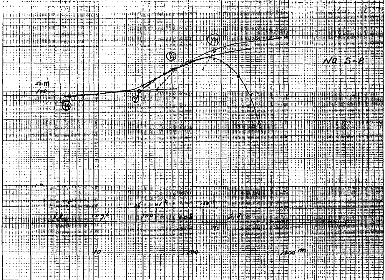
Fig. Result of Electrical Prospecting (ρ-a curve)
