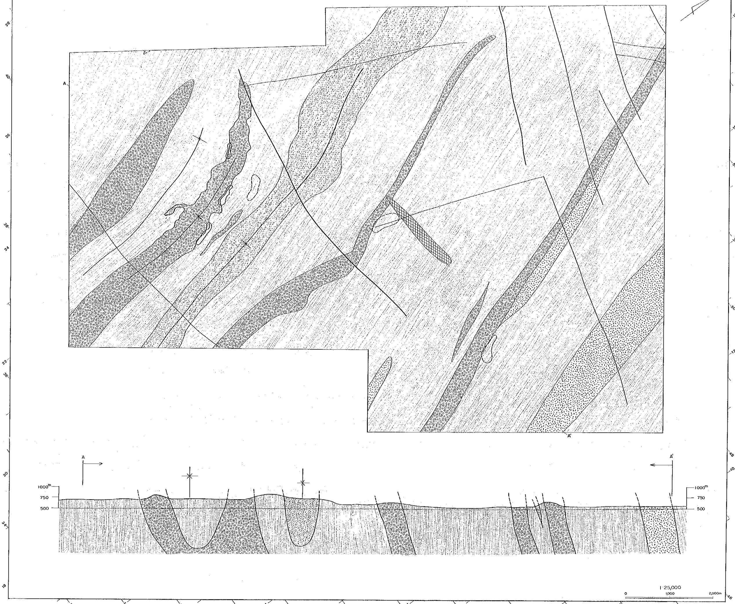
PLATE 12 Geological Map and Geological Section of Chipfunde Area 1 : 25,000
