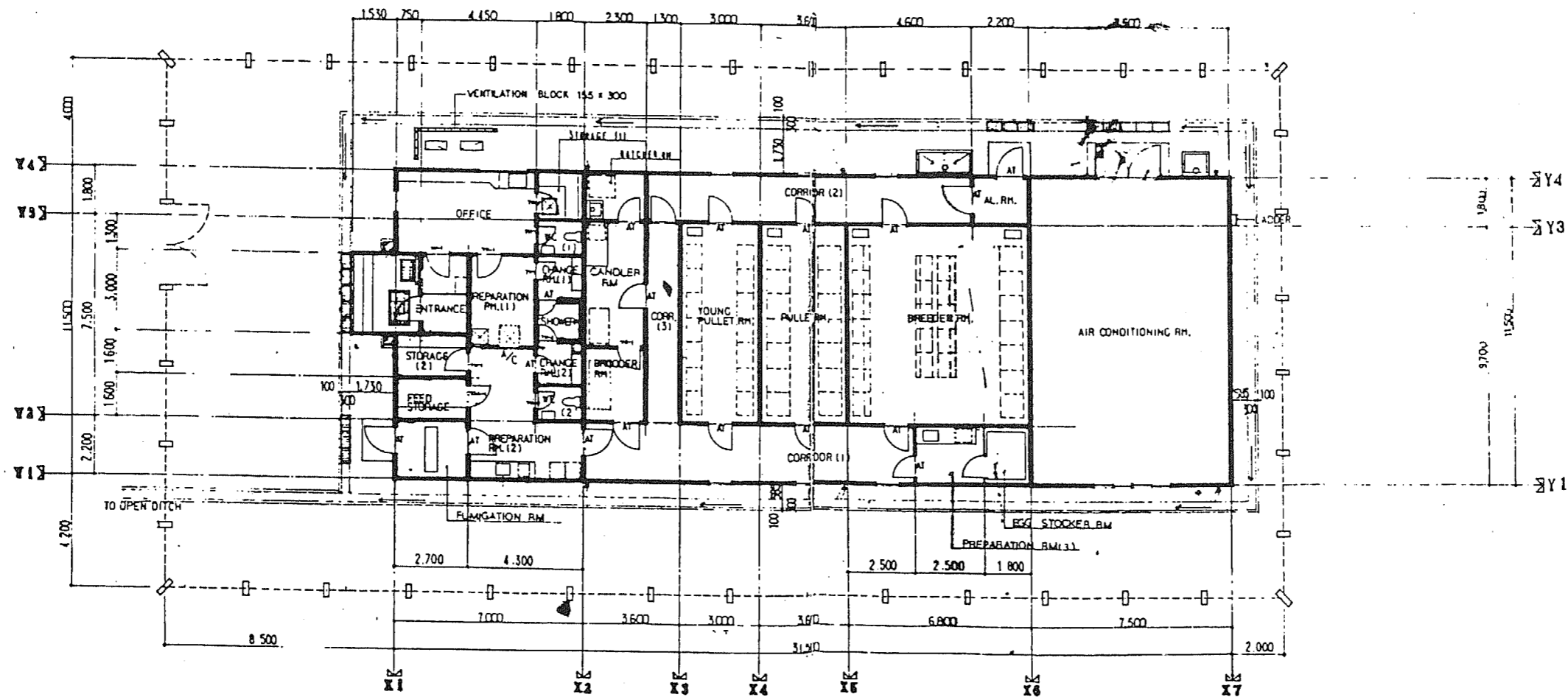
FLOOR PLAN 1:100
