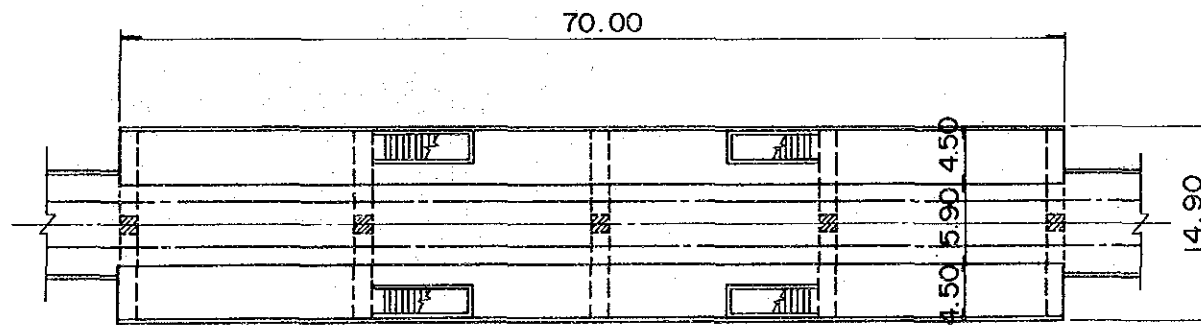
PLAN OF PLATFORM
