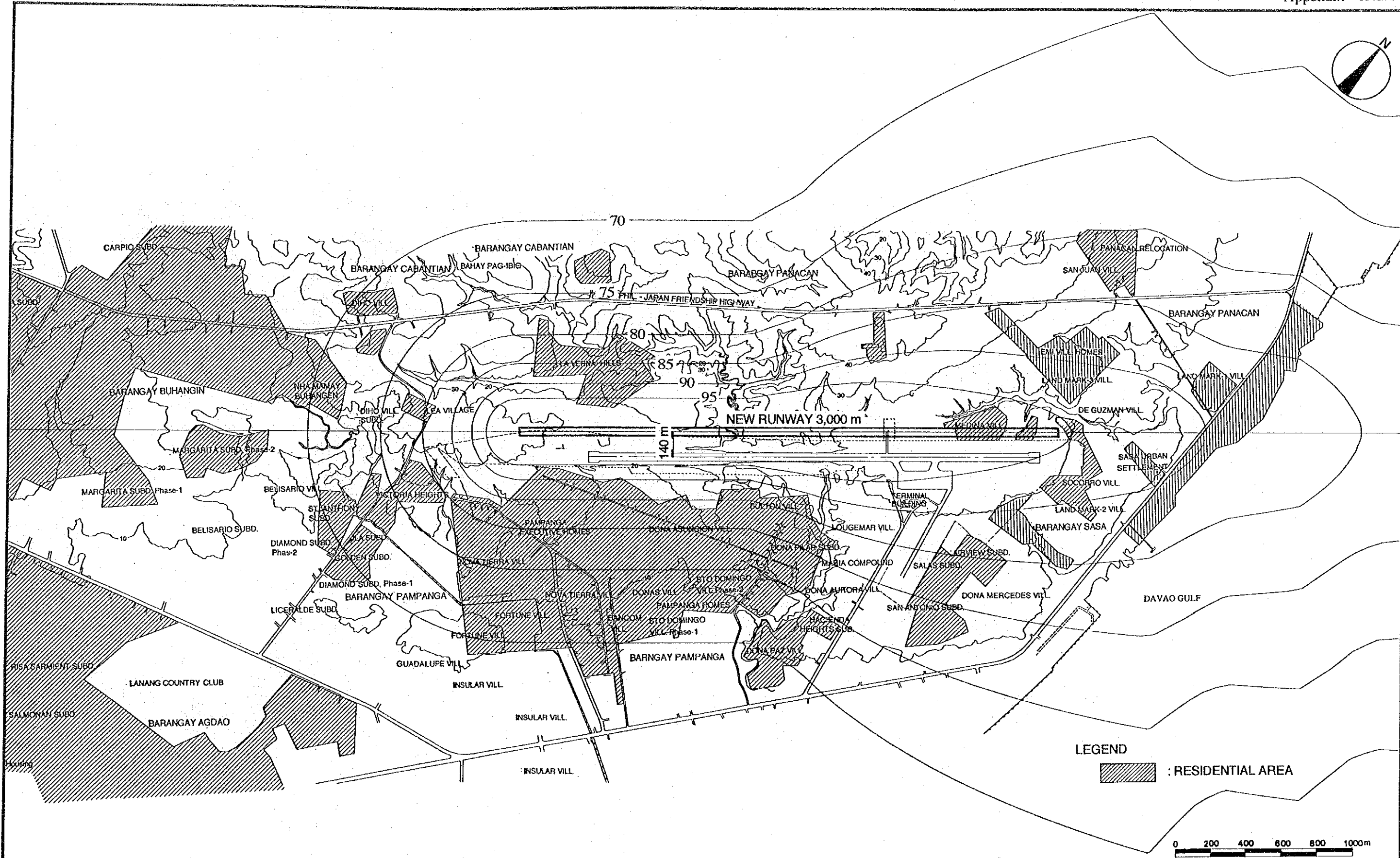
Aircraft Noise Contours at dB(A) of Taking off DC-10
