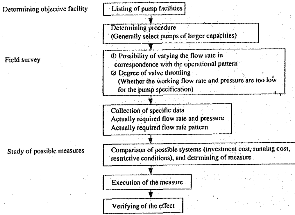
Figure 11.47 Electric power saving flow of pumps
