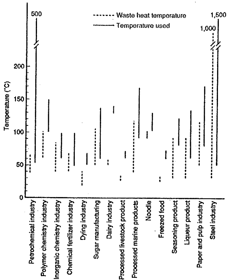
Figure 11.54 Heat utilization temperature distribution by sector
