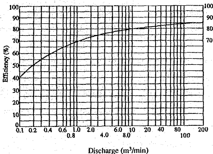
Figure 11.37 Standard efficiency of general purpose pumps
