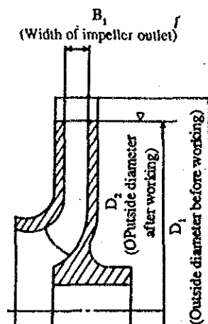
Figure 11.41 Working the impeller of its outside diameter
