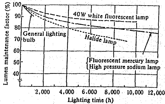
Figure 11.48 Lumen maintenance characteristic of various light sources
