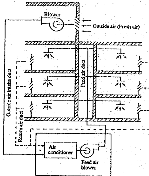
Figure 11.60 Air conditioning system when return air is available
