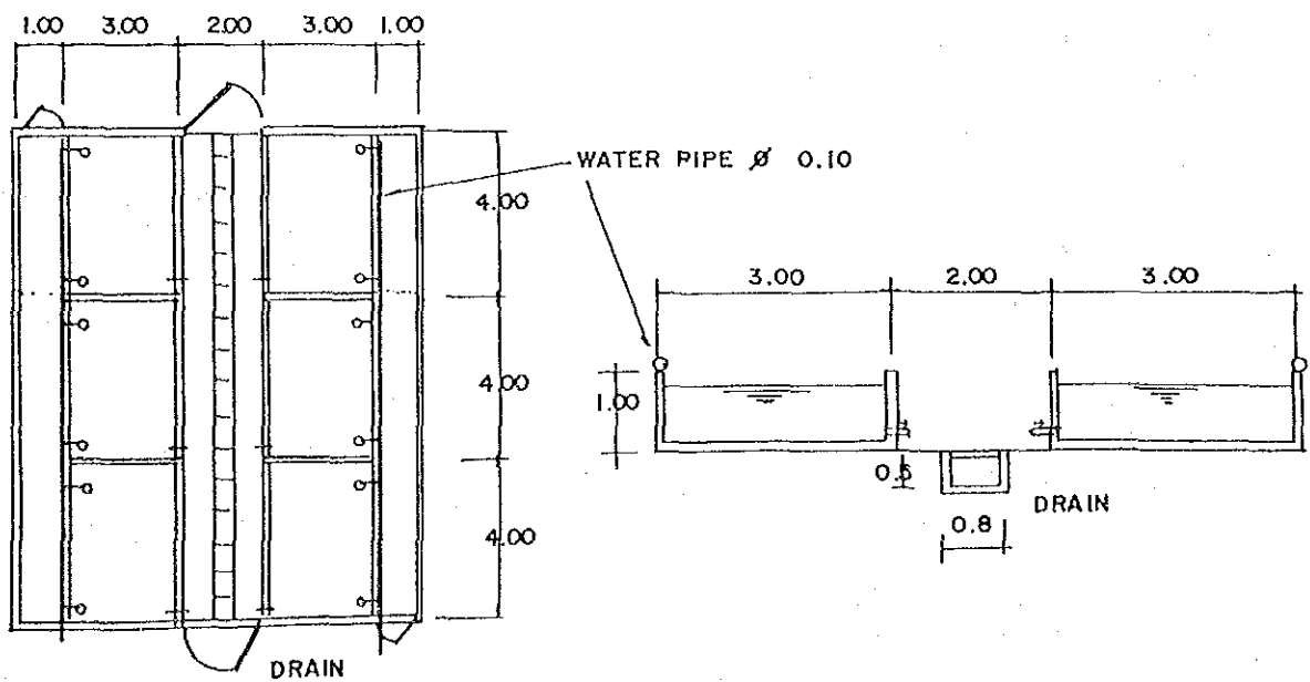
FISH BREEDING FARM S = 1:200
