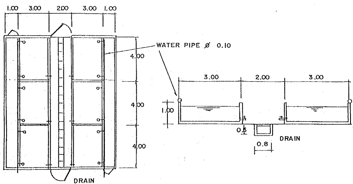
FISH BREEDING FARM S = 1:200
