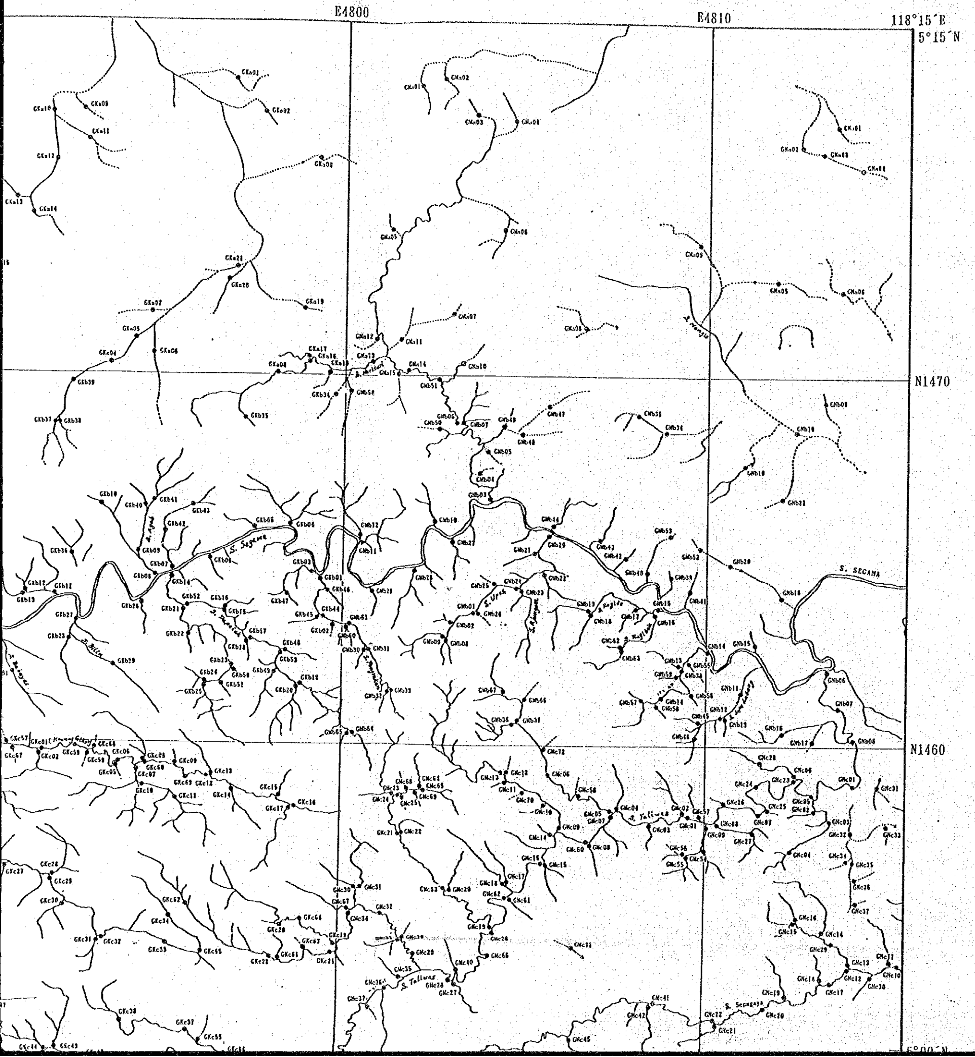
Plate II-1-1 MINERAL EXPLORATION: SUPRA-REGIONAL SURVEY IN CENTRAL SABAH, MALAYSIA PHASE II LOCATION MAP OF STREAM SEDIMENT GEOCHEMICAL SAMPLES IN THE SEGAMA AREA Scale 1:100,000 JAPAN INTERNATIONAL COOPERATION AGENCY METAL MINING AGENCY OF JAPAN FEBRUARY, 1992
