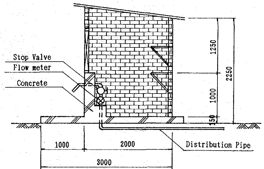
Section B-B
