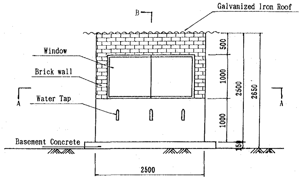
Front View
