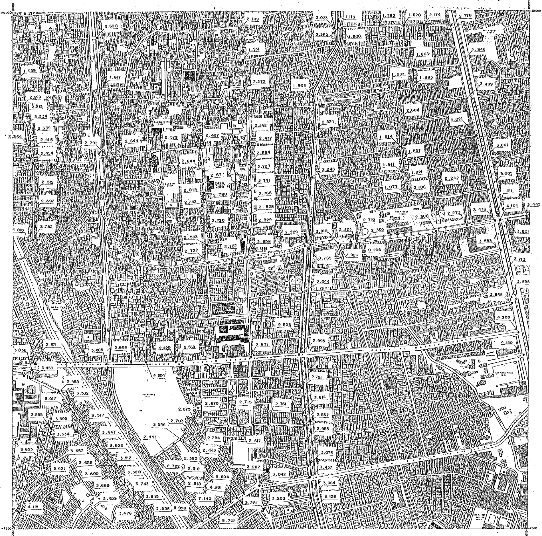
RESULT OF SPOT ELEVATION SURVEY (MAP NO. 806)
