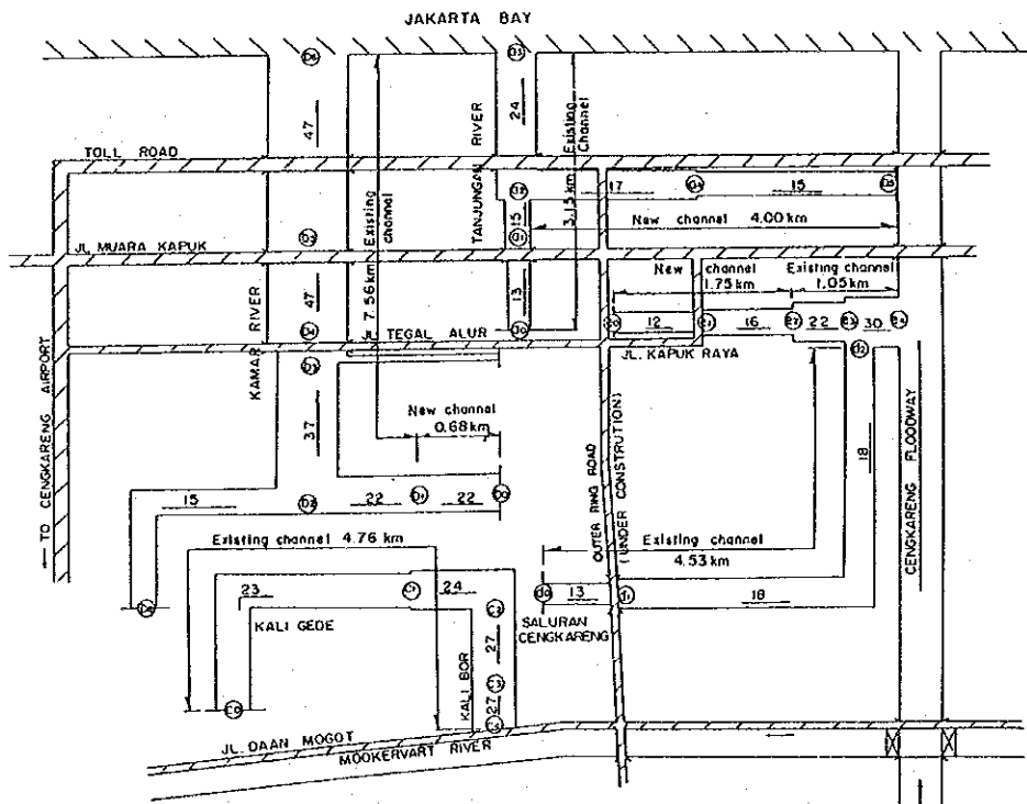
LOCATION OF PROPOSED CHANNEL IMPROVEMENT
