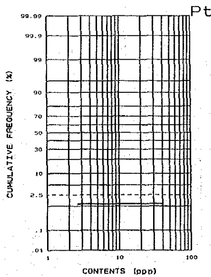
Bidu Bidu Hill stream sediments (A)
