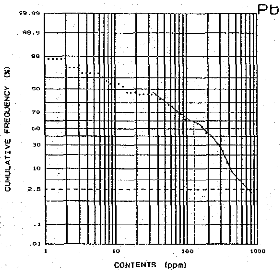
Mantri stream sediments (A)
