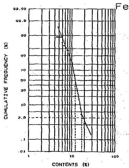
Bidu Bidu Hill Soil (B)
