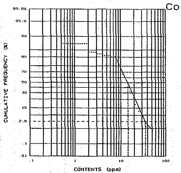
Mantri stream sediments (C)
