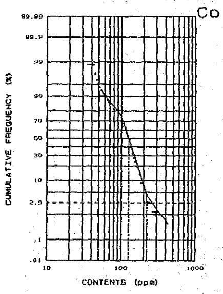
Bidu Bidu Hill stream sediments (C)
