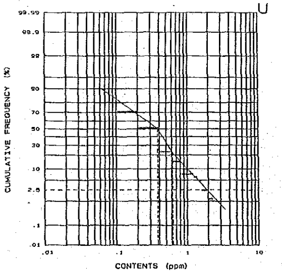
Bidu Bidu Hill Soil (C)
