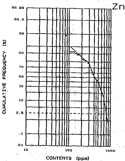
Bidu Bidu Hill stream sediments (B)
