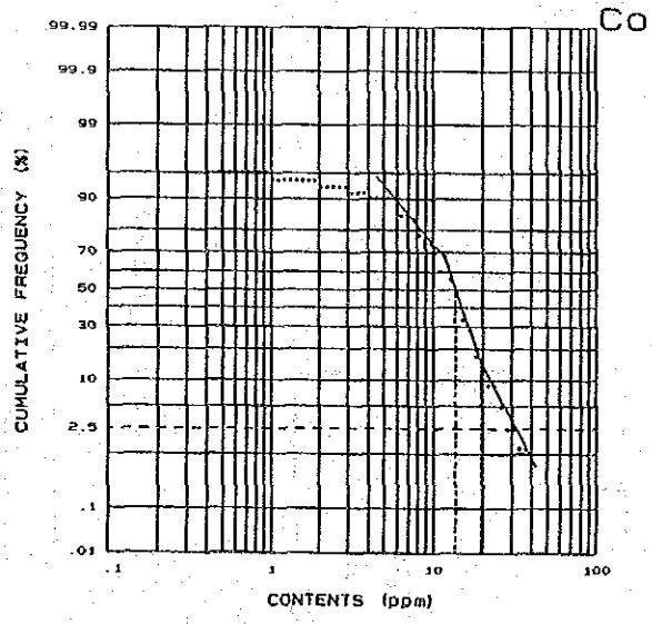
Mantri stream sediments (A)
