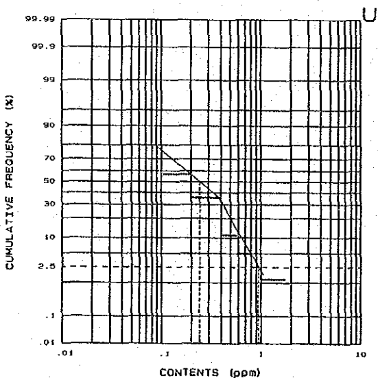
Bidu Bidu Hill stream sediments (C)
