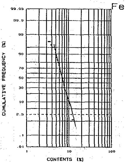
Mantri stream sediments (B)
