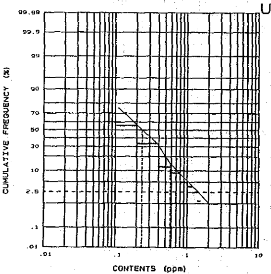
Bidu Bidu Hill stream sediments (A)
