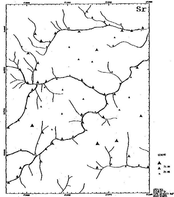
Bidu Bidu Hill Soil (B)
