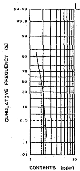
Mantri stream sediments (B)
