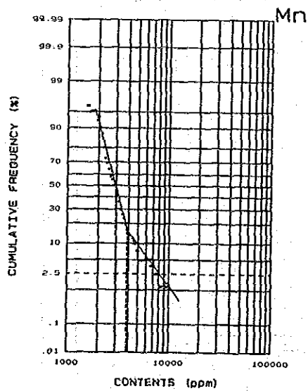
Bidu Bidu Hill stream sediments. (A)
