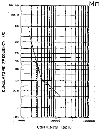
Bidu Bidu Hill stream sediments (B)
