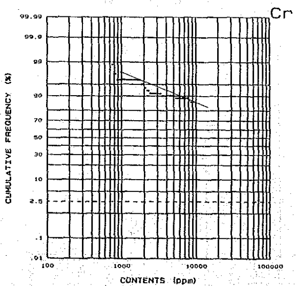
Bidu Bidu Hill stream sediments (A)
