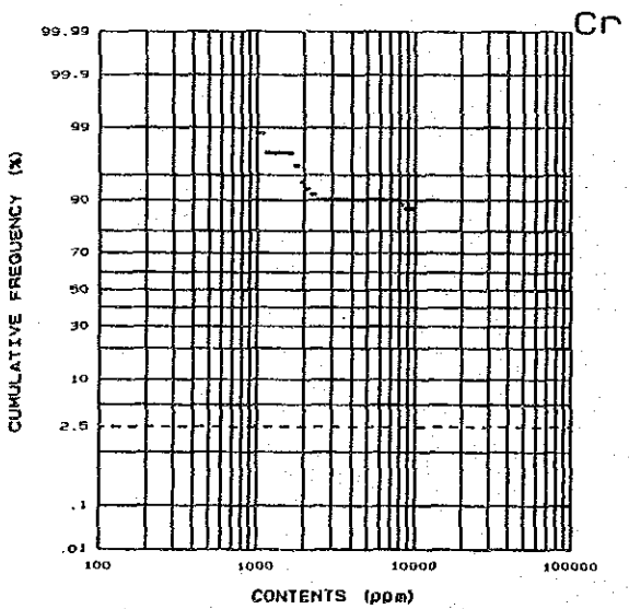
Bidu Bidu Hill stream sediments (B)
