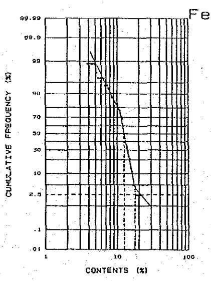
Bidu Bidu Hill Soil (C)
