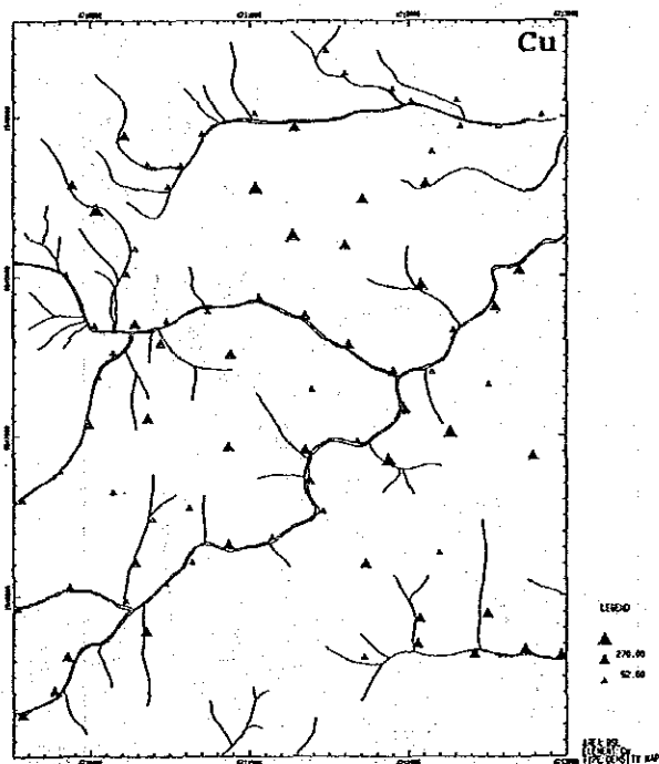
Bidu Bidu Hill Soil (B)
