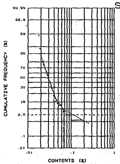
Bidu Bidu Hill stream sediments (B)
