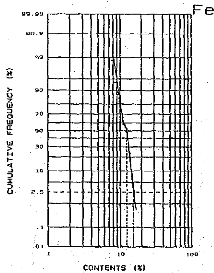
Bidu Bidu Hill stream sediments (C)
