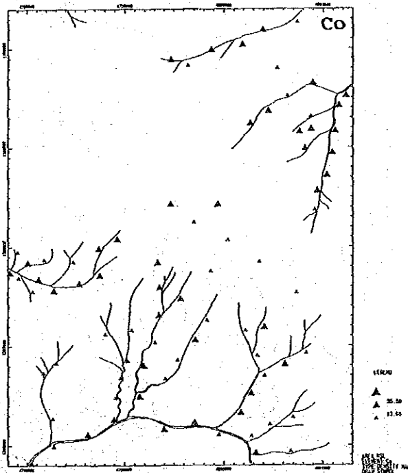
Mantri soil (B)
