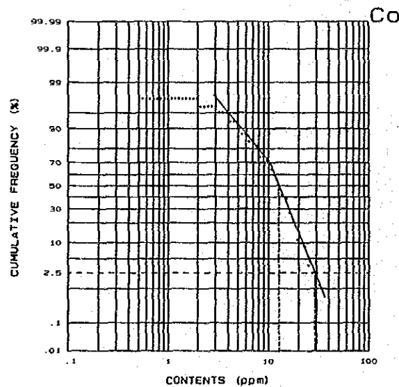
Mantri stream sediments (B)
