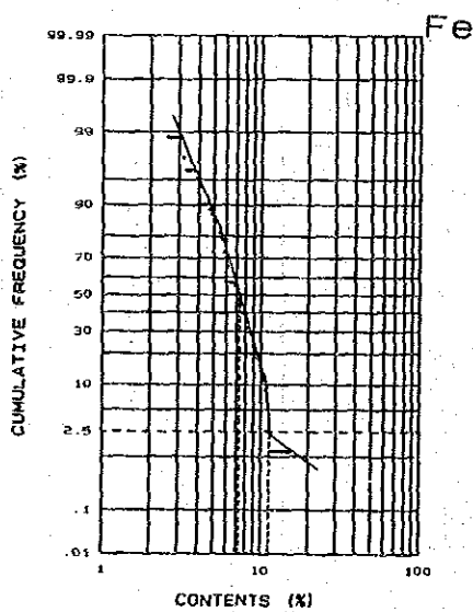
Mantri stream sediments (A)
