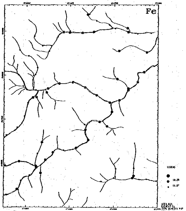
Bidu Bidu Hill stream sediments (B)
