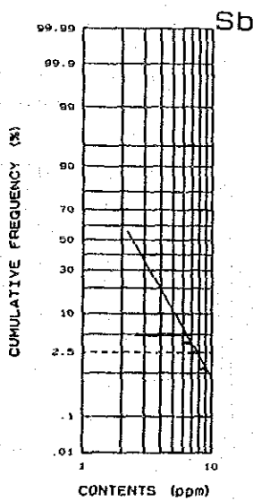
Mantri stream sediments (A)
