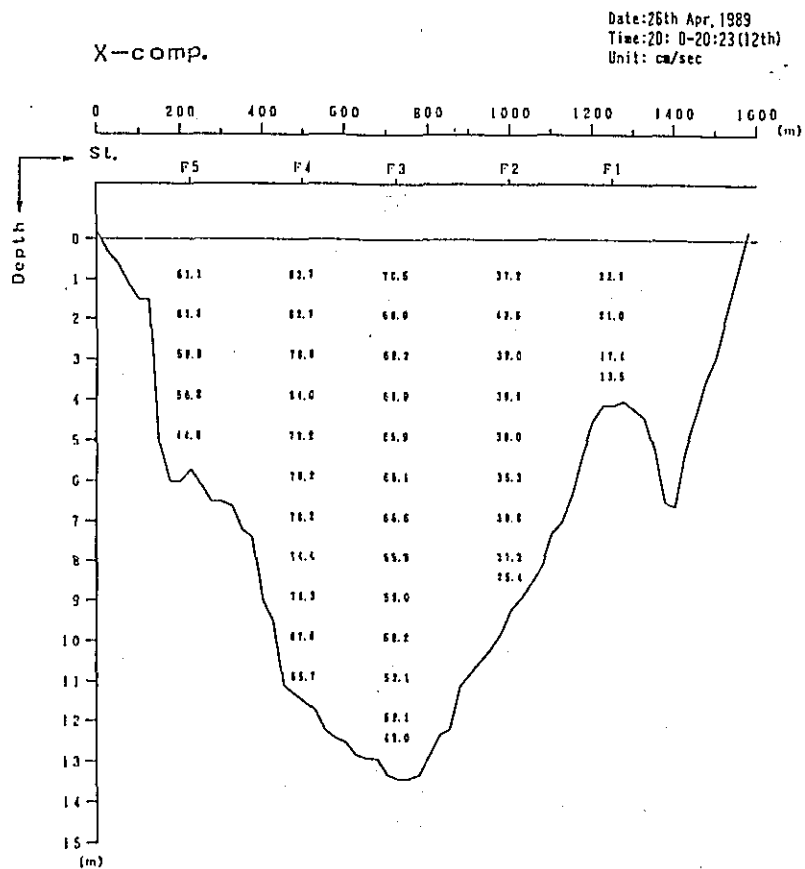
Fig. 2. 1-2(162) Profile in Distribution of Discharge Survey Results (7th Stage)
