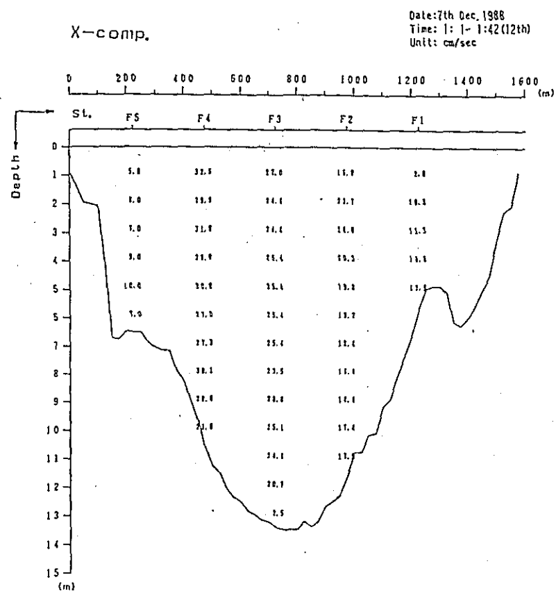
Fig. 2. 1-2 (62) Profile in Distribution of Discharge Survey Results (3rd Stage)
