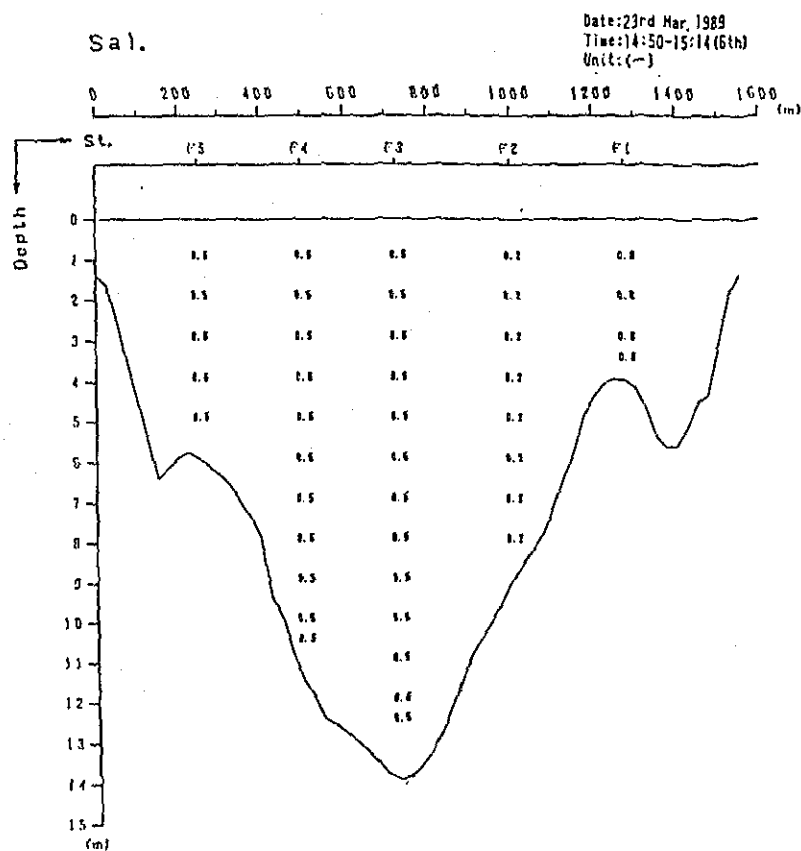
Fig. 2. 1-1(131) Profile in Distribution of Discharge Survey Results (6th Stage)
