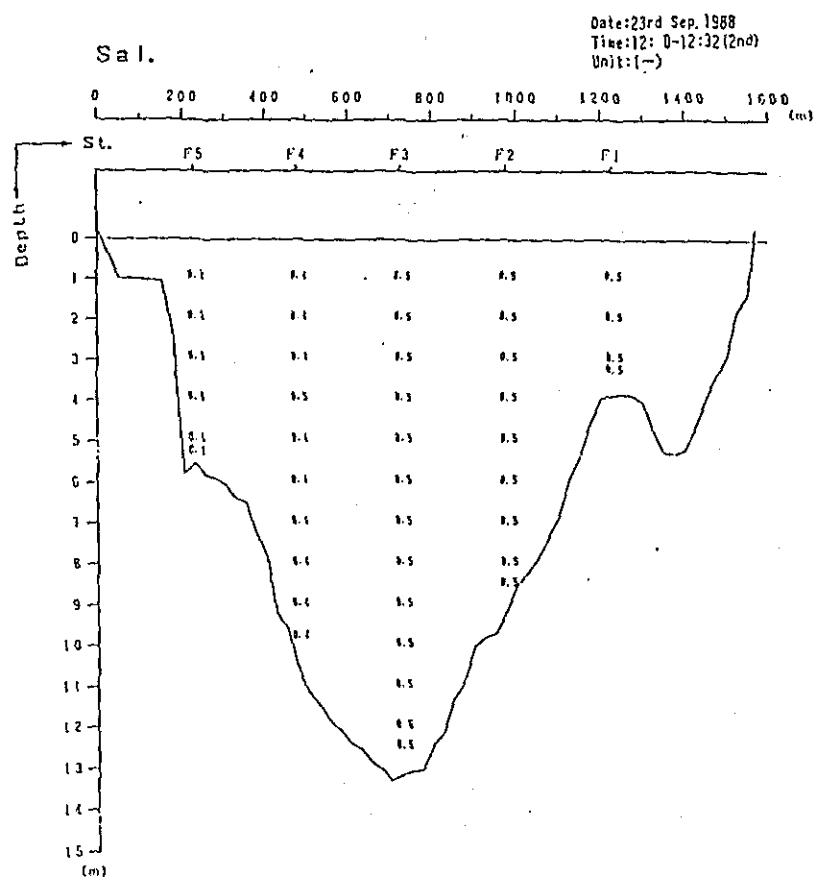
Fig. 2. 1-10) Profile in Distribution of Discharge Survey Results (1st Stage)
