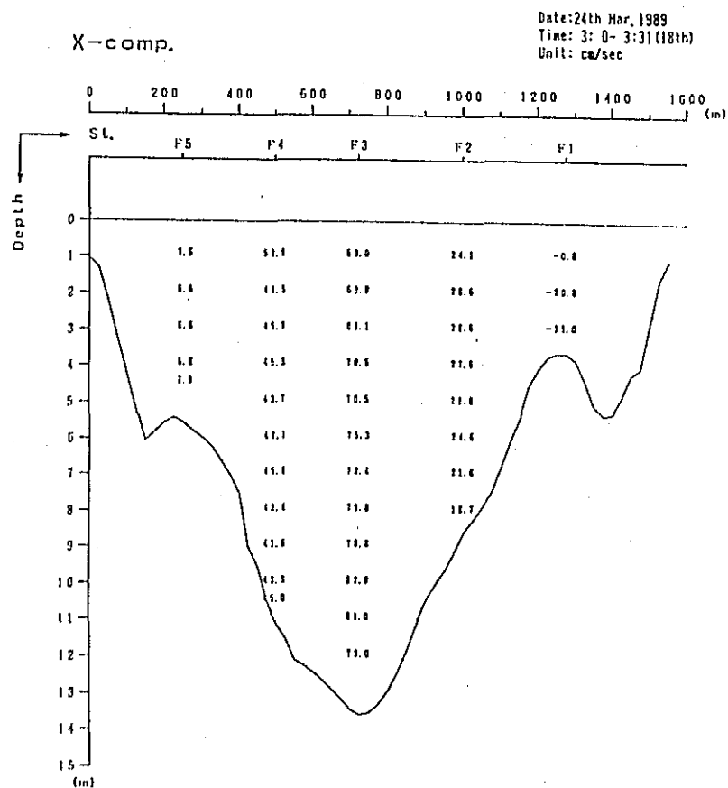
Fig. 2. 1-2(143) Profile in Distribution of Discharge Survey Results (6th Stage)
