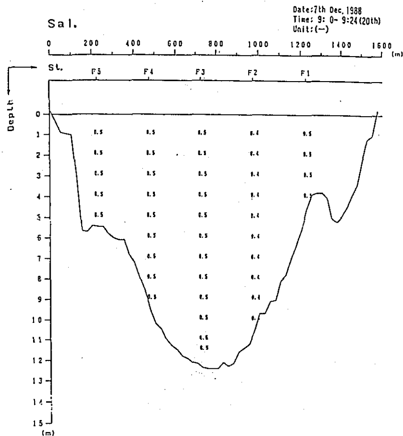
Fig. 2. 1-1(70) Profile in Distribution of Discharge Survey Results (3rd Stage)
