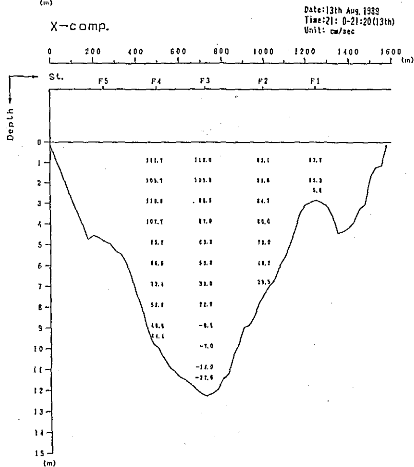
Fig. 2. 1-2(223) Profile in Distribution of Discharge Survey Results (12th Stage)
