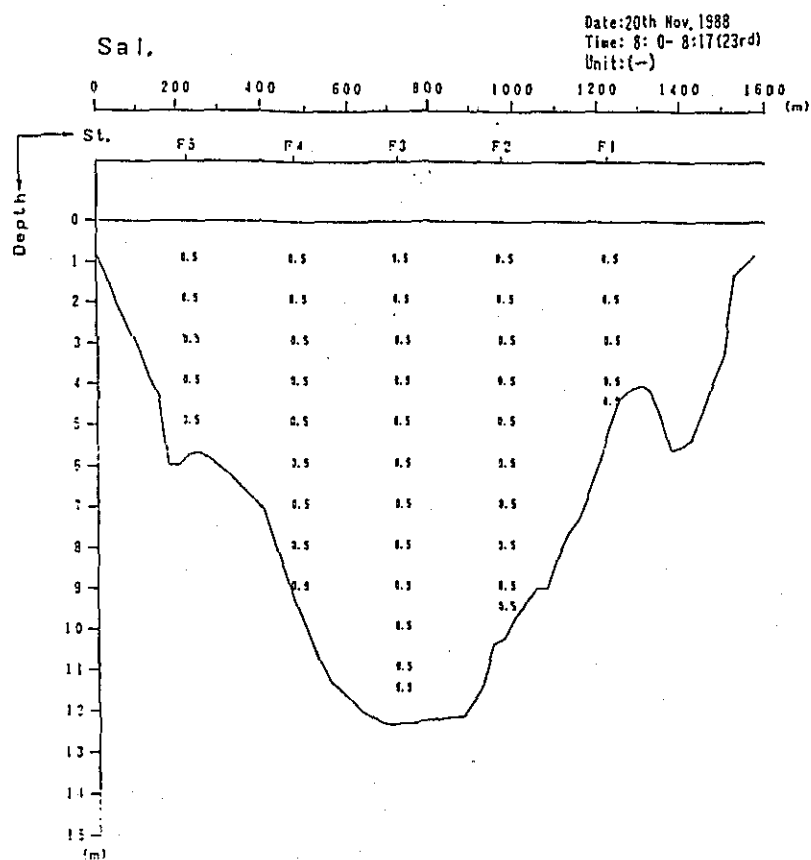
Fig. 2. 1-1(48) Profile in Distribution of Discharge Survey Results (2nd Stage)
