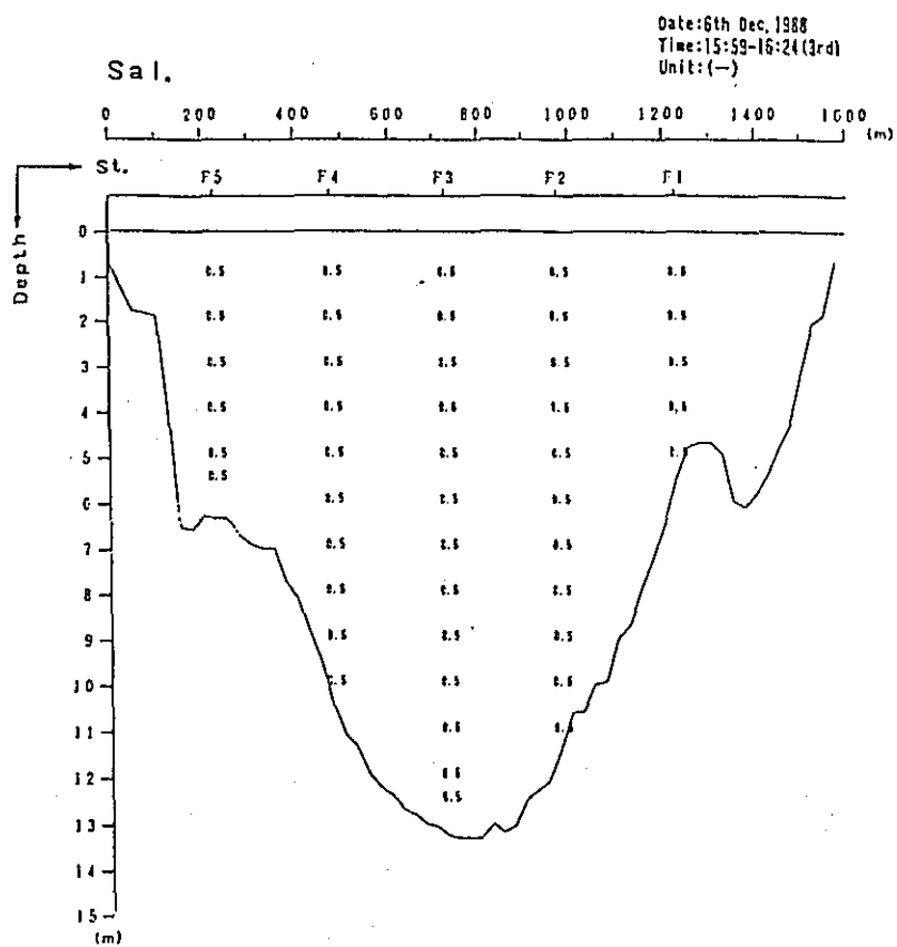
Fig. 2. 1-1(53) Profile in Distribution of Discharge Survey Results (3rd Stage)
