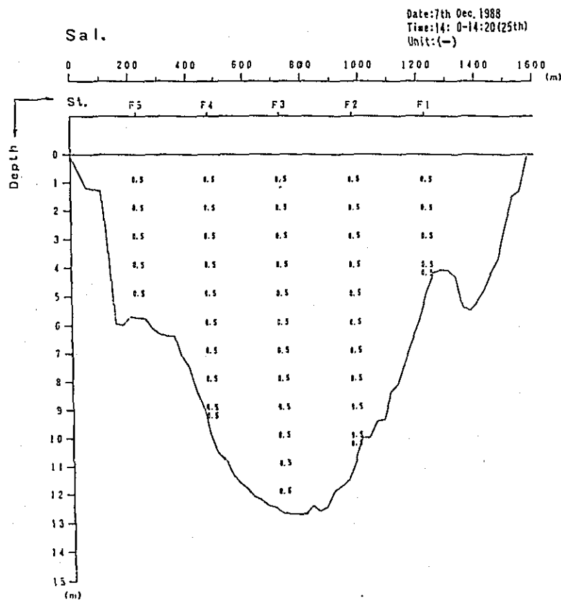
Fig. 2. 1-1(75) Profile in Distribution of Discharge Survey Results (3rd Stage)
