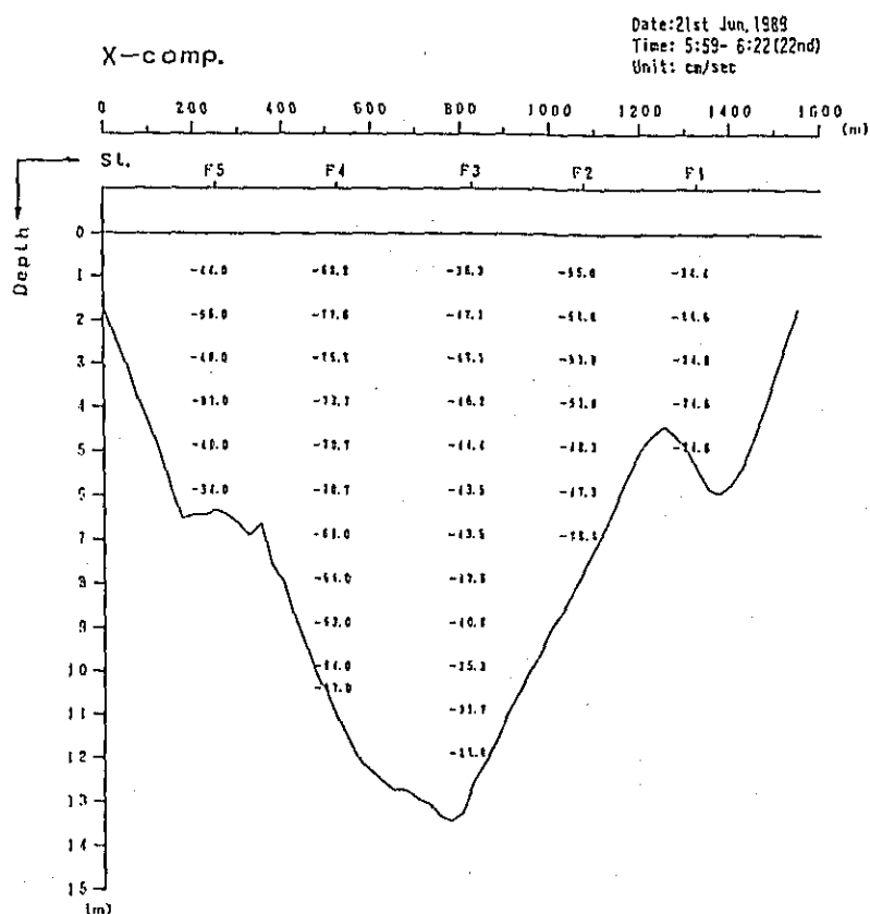
Fig. 2. 1-2(22) Profile in Distribution of Discharge Survey Results (9th Stage)
