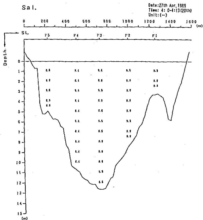
Fig. 2. 1-1(170) Profile in Distribution of Discharge Survey Results (7th Stage)
