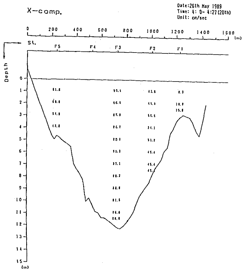
Fig. 2. 1-2(195) Profile in Distribution of Discharge Survey Results (8th Stage)
