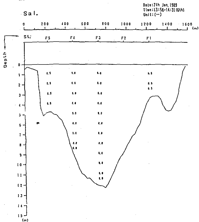
Fig. 2. 1-1(81) Profile in Distribution of Discharge Survey Results (4th Stage)
