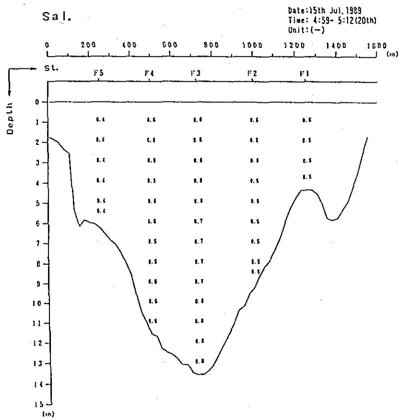
Fig. 2. 1-1(245) Profile in Distribution of Discharge Survey Results (00th Stage)
