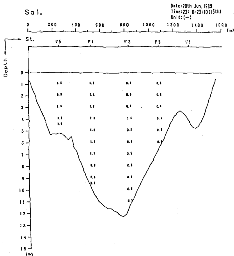
Fig. 2. 1-1015 Profile in Distribution of Discharge Survey Results (9th Stage)
