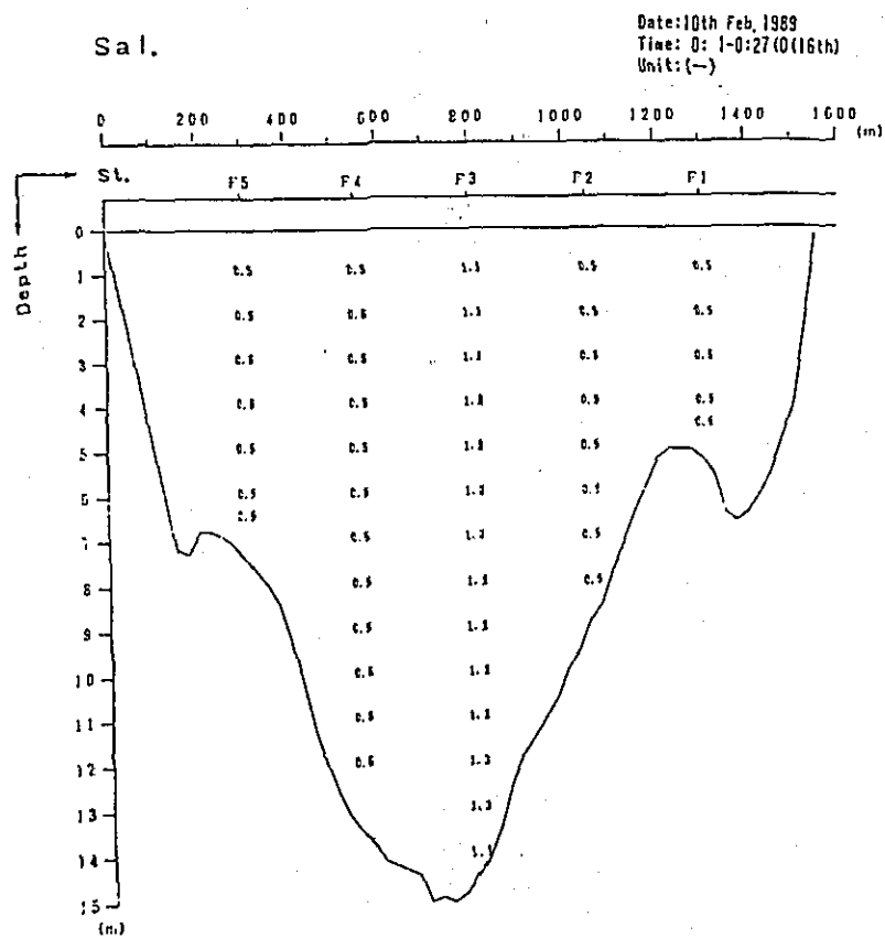
Fig. 2. 1-1(16) Profile in Distribution of Discharge Survey Results (5th Stage)
