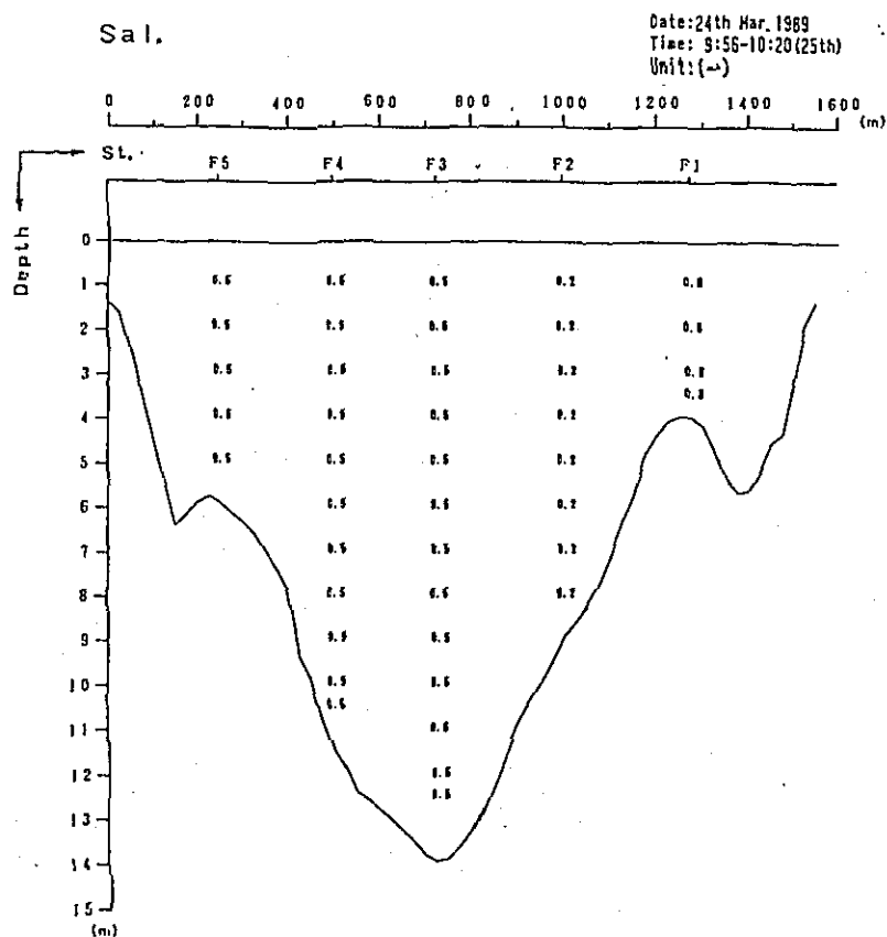
Fig. 2. 1-1(150) Profile in Distribution of Discharge Survey Results (6th Stage)
