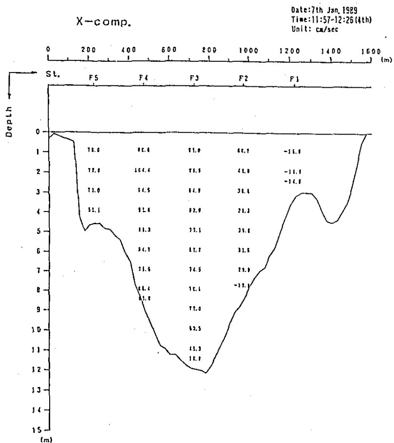
Fig. 2. 1-2(79) Profile in Distribution of Discharge Survey Results (4th Stage)
