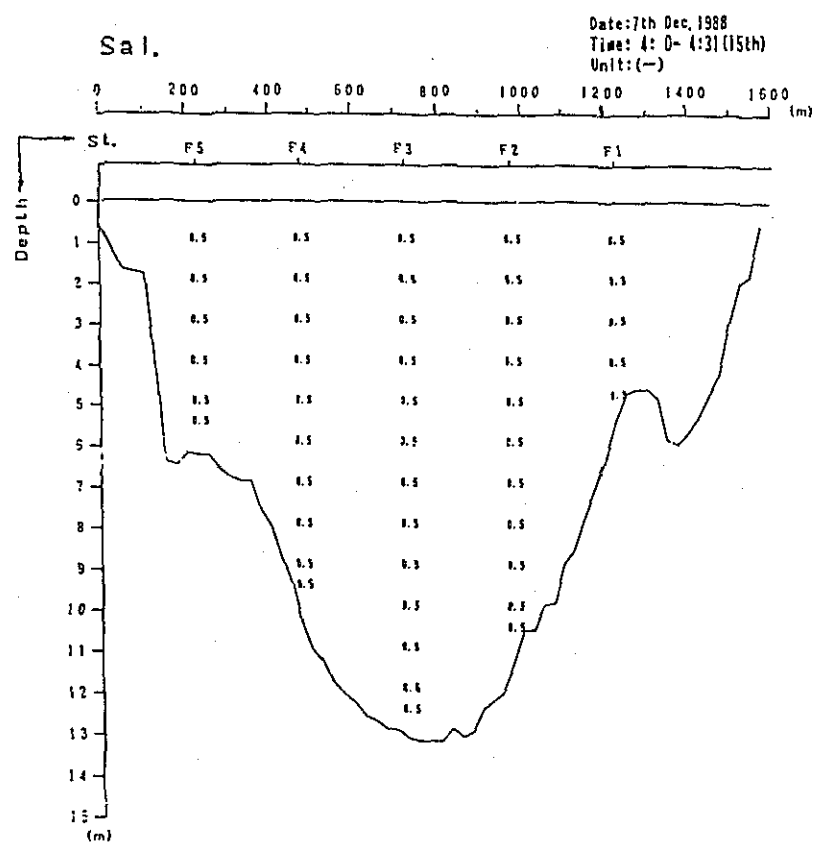
Fig. 2. 1-1(65) Profile in Distribution of Discharge Survey Results (3rd Stage)
