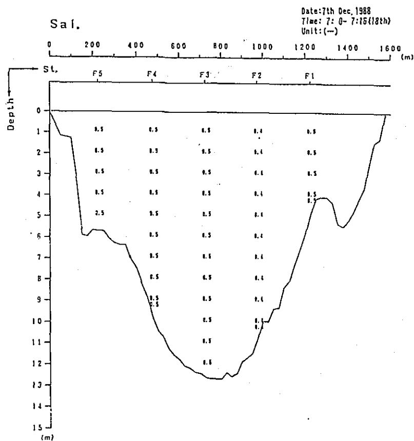
Fig. 2. 1-1(63) Profile in Distribution of Discharge Survey Results (3rd Stage)
