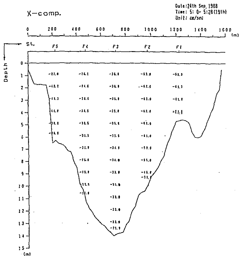
Fig. 2. 1-2(19) Profile in Distribution of Discharge Survey Results (1st Stage)
