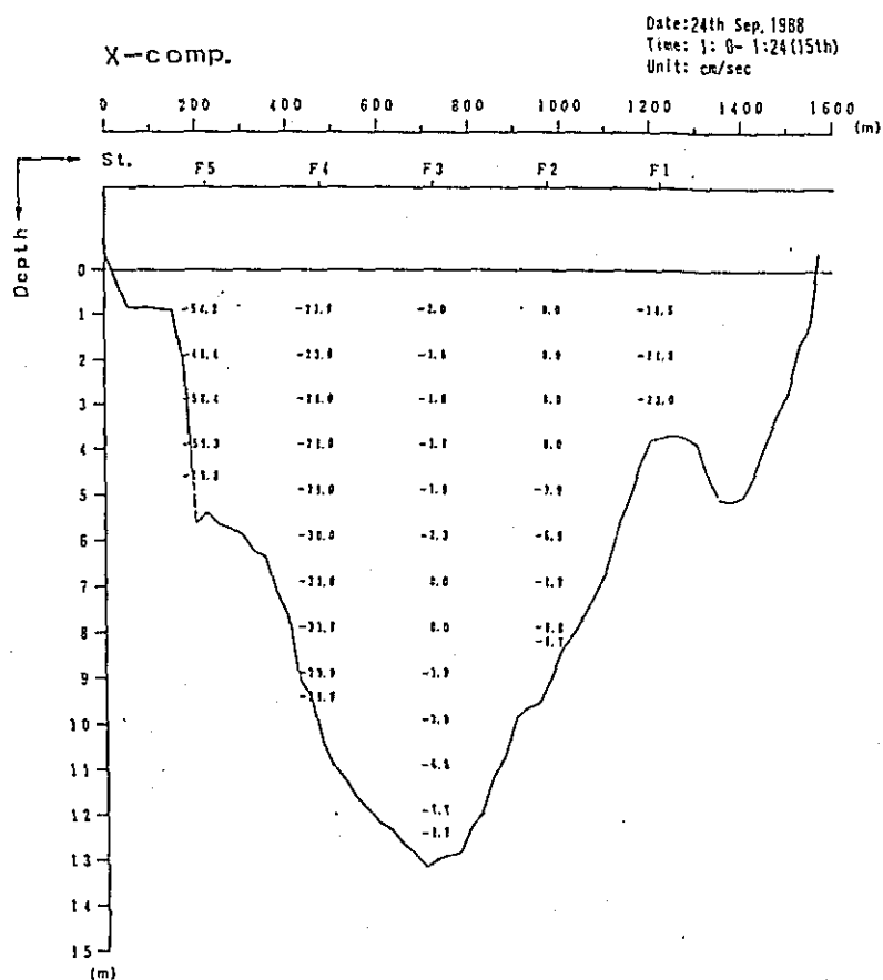
Fig. 2. 1-2(15) Profile in Distribution of Discharge Survey Results (1st Stage)
