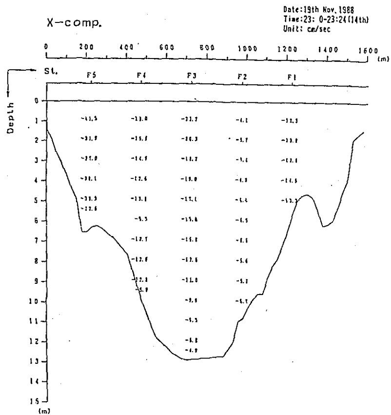
Fig. 2. 1-2 (3) Profile in Distribution of Discharge Survey Results (2nd Stage)
