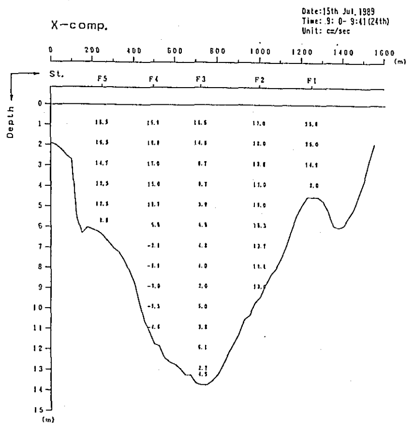
Fig. 2. 1-2(249) Profile in Distribution of Discharge Survey Results (10th Stage)
