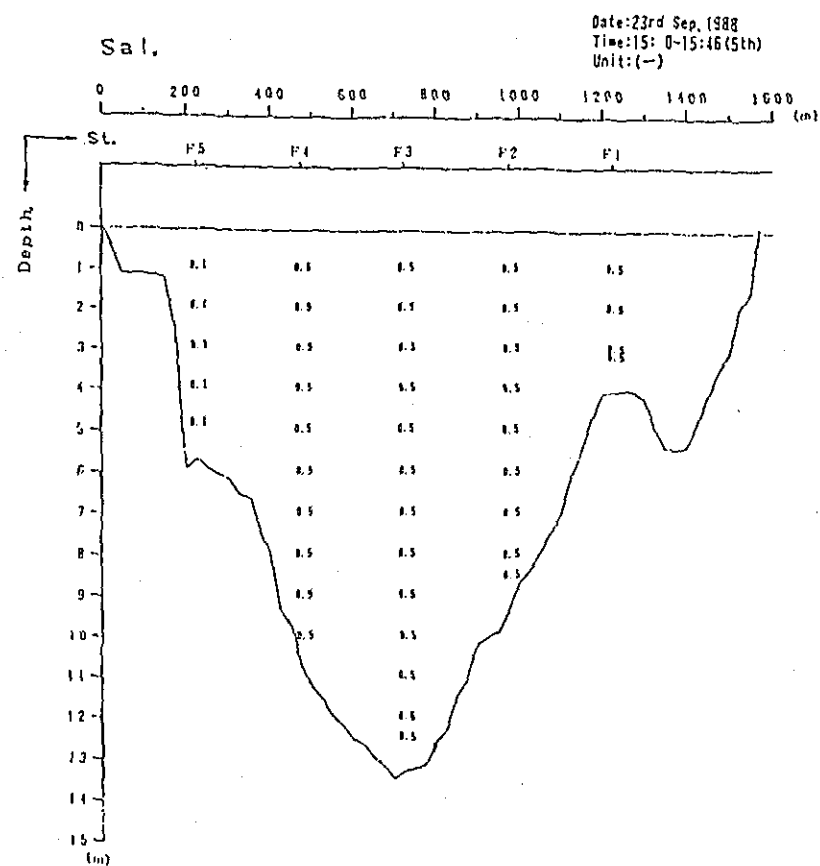
Fig. 2. 1-15 Profile in Distribution of Discharge Survey Results (1st Stage)
