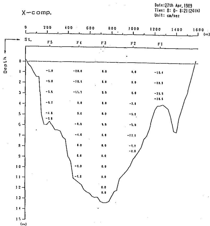
Fig. 2. 1-2(174) Profile in Distribution of Discharge Survey Results (7th Stage)
