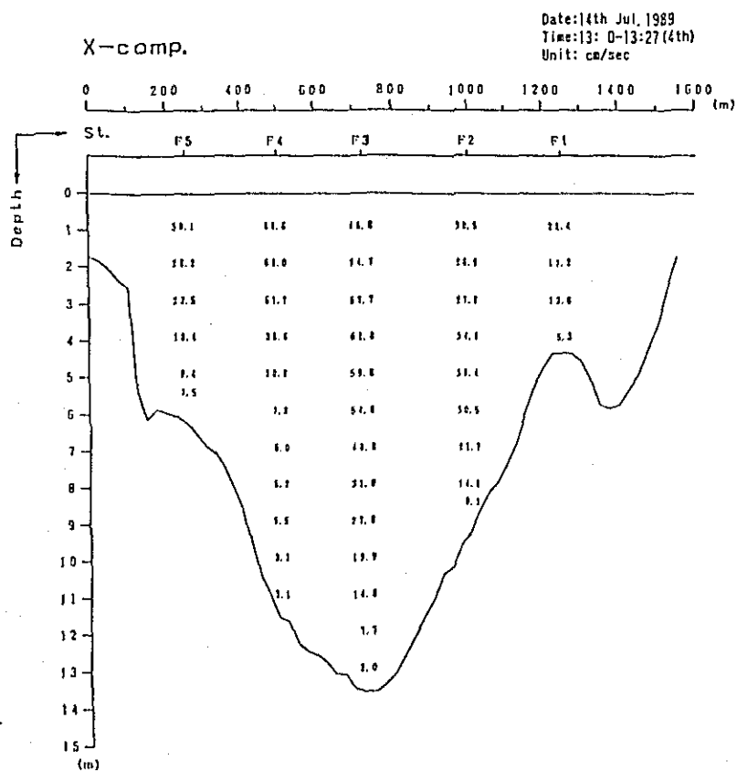
Fig. 2. 1-2(229) Profile in Distribution of Discharge Survey Results (0th Stage)
