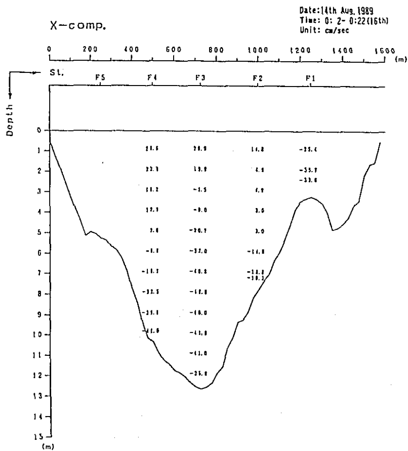
Fig. 2. 1-2(2) Profile in Distribution of Discharge Survey Results (2th Stage)
