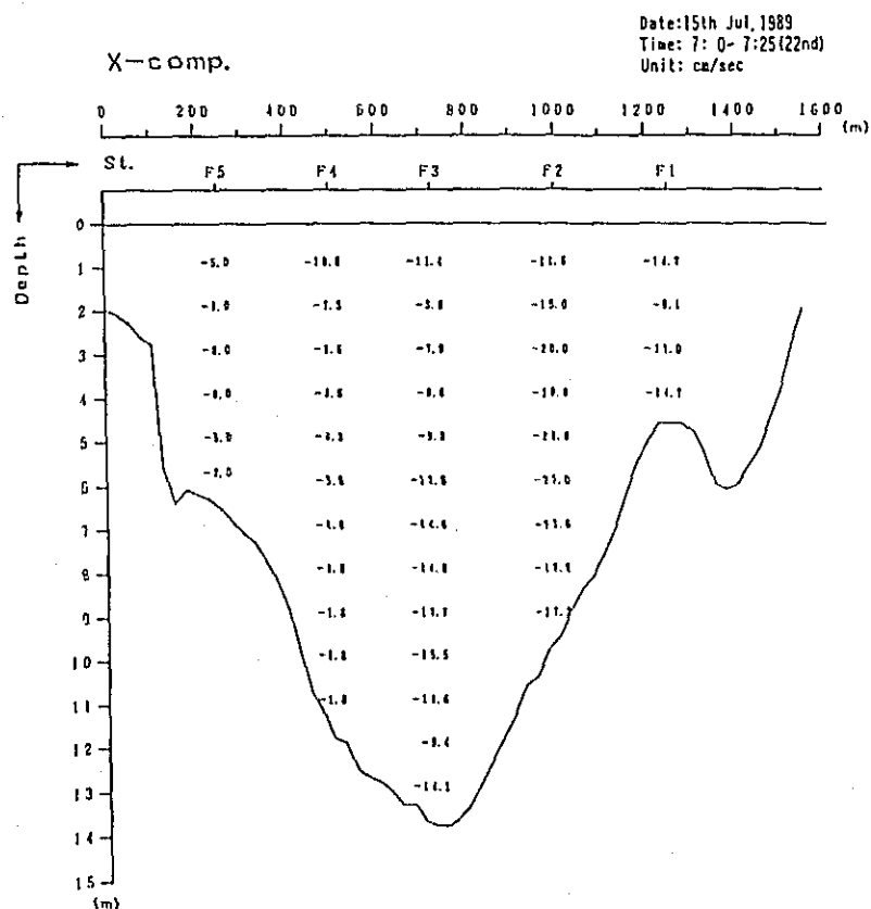
Fig. 2. 1-2(247) Profile in Distribution of Discharge Survey Results (00th Stage)
