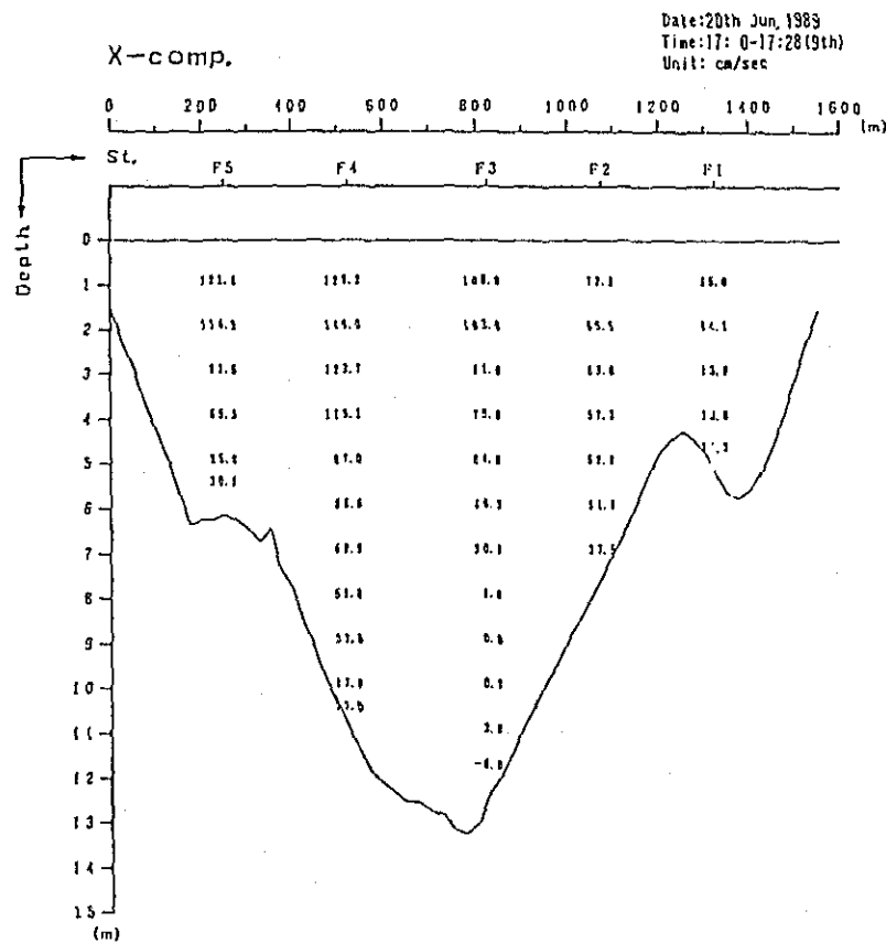
Fig. 2. 1-2(200) Profile in Distribution of Discharge Survey Results (9th Stage)
