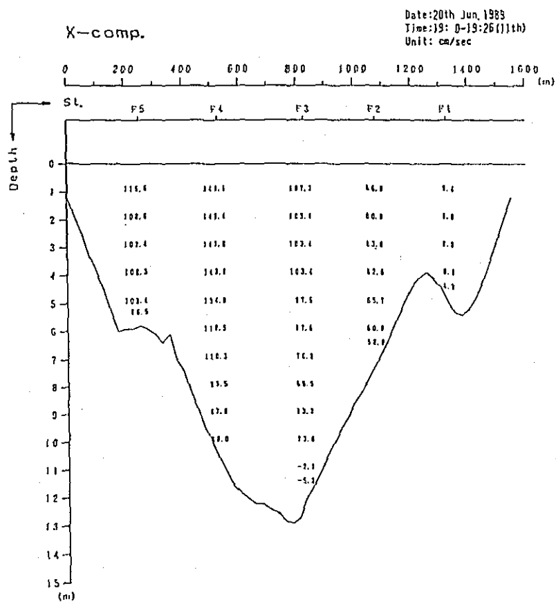
Fig. 2. 1-2(211) Profile in Distribution of Discharge Survey Results (9th Stage)
