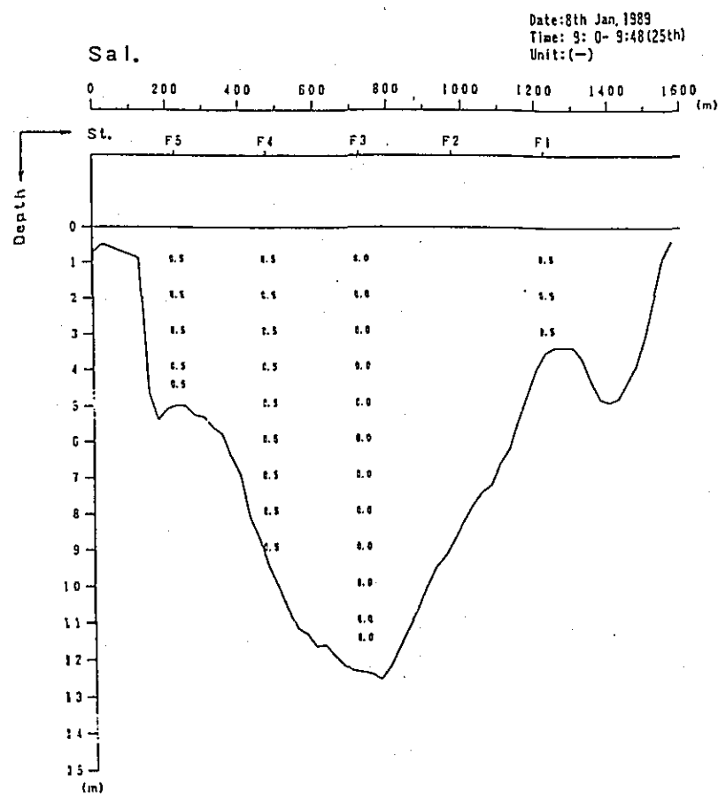
Fig. 2. 1-1(100) Profile in Distribution of Discharge Survey Results (4th Stage)
