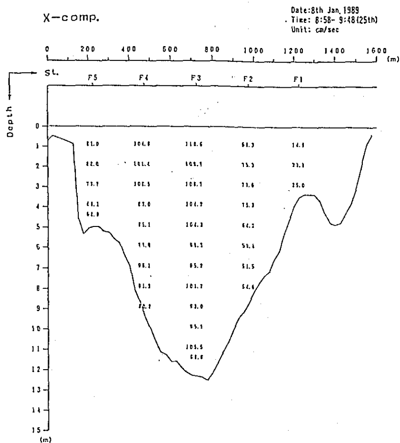
Fig. 2. 1-2(100) Profile in Distribution of Discharge Survey Results (4th Stage)
