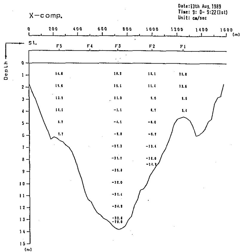
Fig. 2. 1-2(276) Profile in Distribution of Discharge Survey Results (12th Stage)
