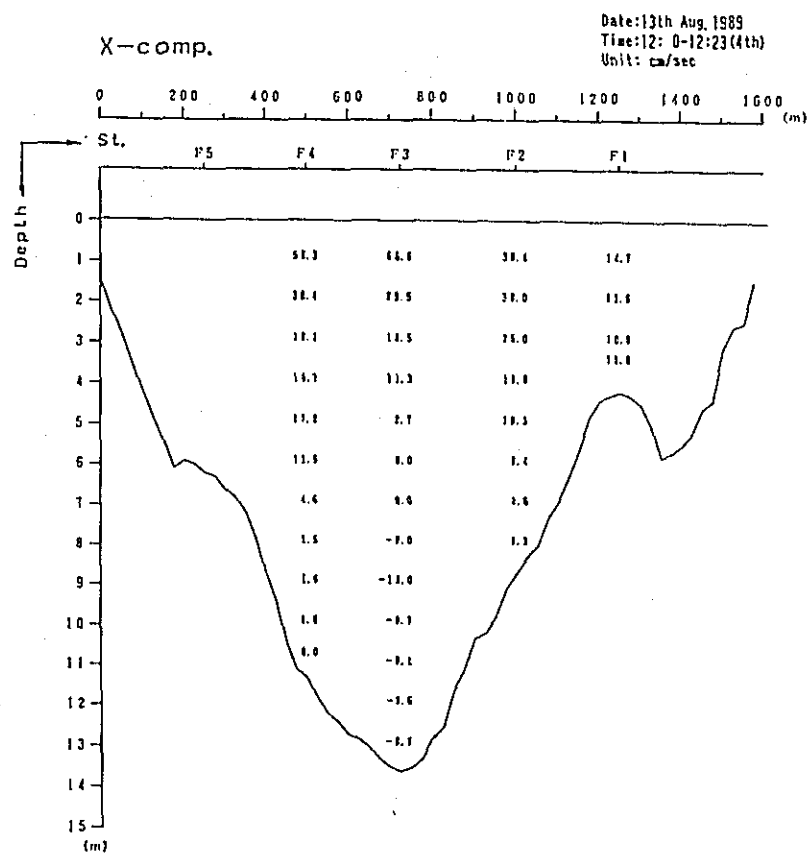
Fig. 2. 1-2(29) Profile in Distribution of Discharge Survey Results (12th Stage)
