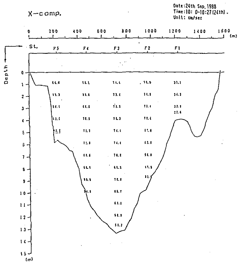
Fig. 2. 1-204) Profile in Distribution of Discharge Survey Results (1st Stage)
