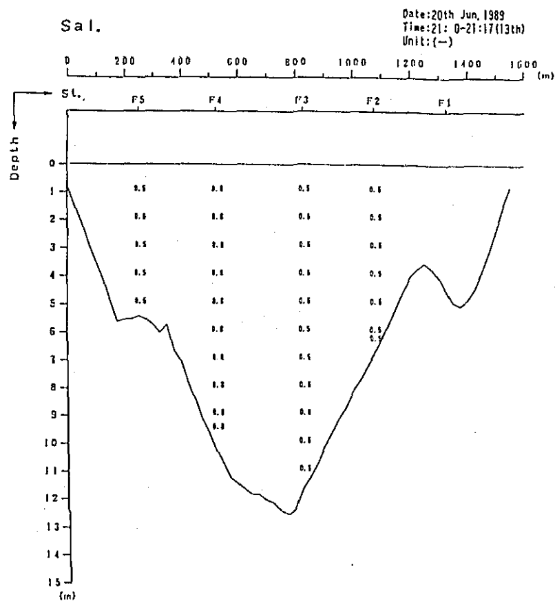
Fig. 2. 1-1(213) Profile in Distribution of Discharge Survey Results (9th Stage)
