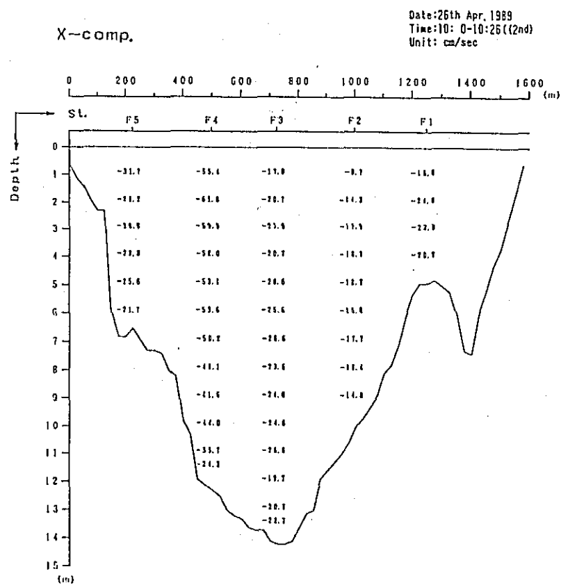
Fig. 2. 1-2(152) Profile in Distribution of Discharge Survey Results (7th Stage)
