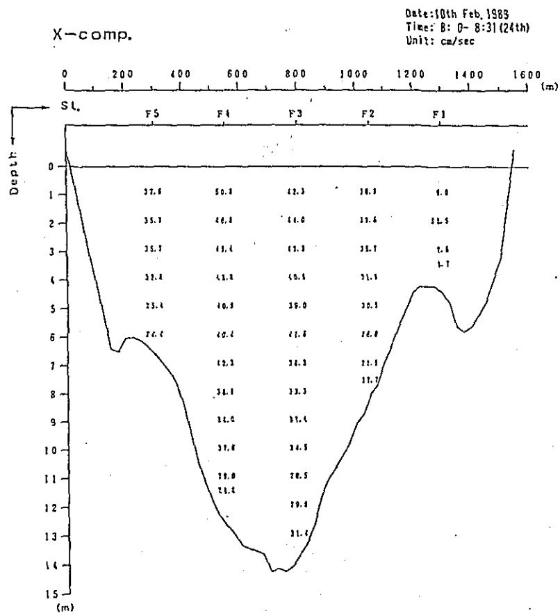
Fig. 2. 1-2(24) Profile in Distribution of Discharge Survey Results (5th Stage)
