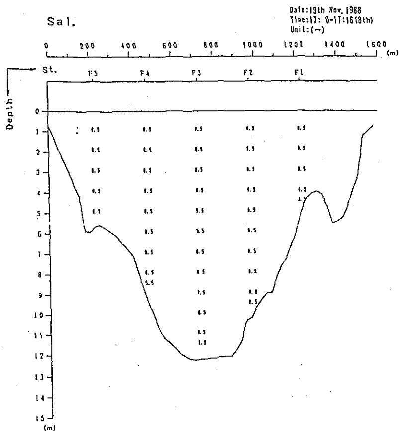
Fig. 2. 1-1(3) Profile in Distribution of Discharge Survey Results (2nd Stage)
