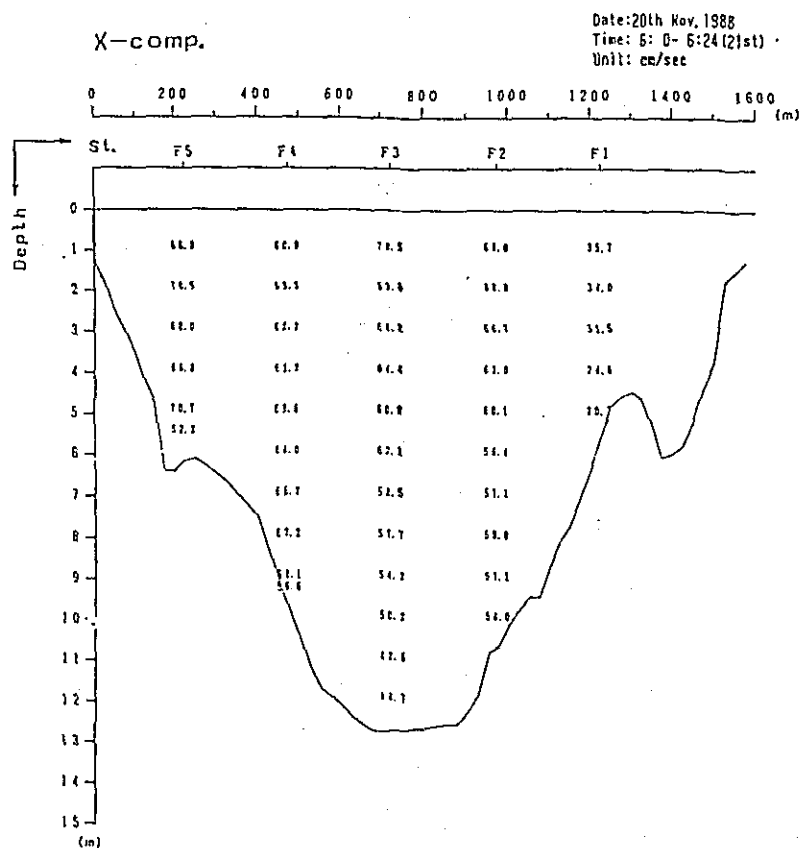
Fig. 2. 1-2(46) Profile in Distribution of Discharge Survey Results (2nd Stage)
