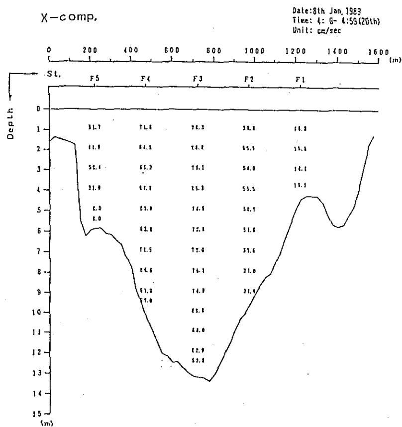
Fig. 2. 1-2(5) Profile in Distribution of Discharge Survey Results (4th Stage)
