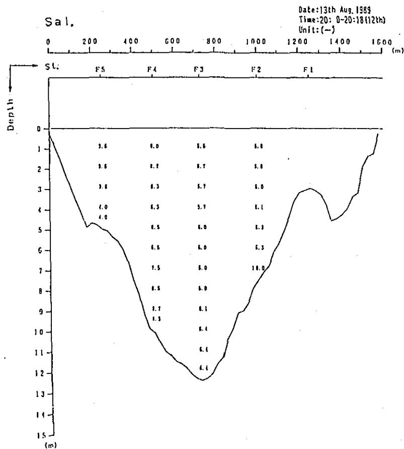
Fig. 2. 1-1(237) Profile in Distribution of Discharge Survey Results (12th Stage)
