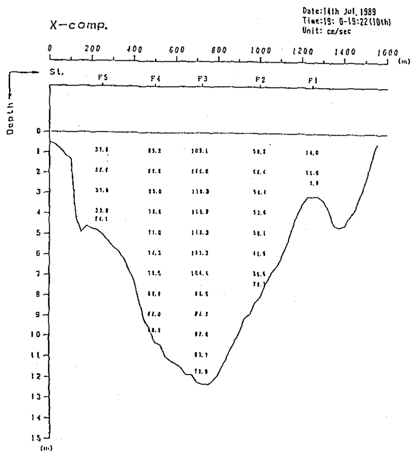
Fig. 2. 1-2(33) Profile in Distribution of Discharge Survey Results (10th Stage)
