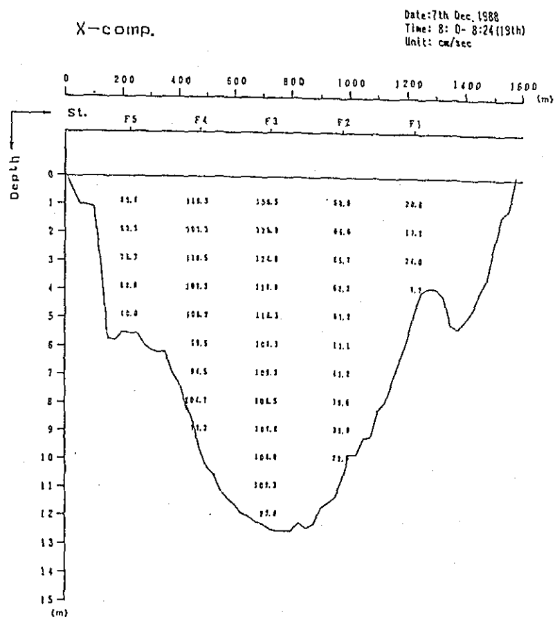
Fig. 2. 1-2 (99) Profile in Distribution of Discharge Survey Results (3rd Stage)
