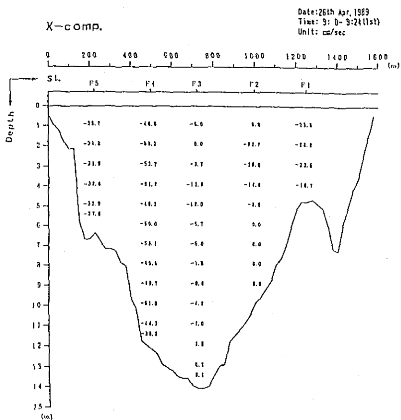
Fig. 2. 1-2(15) Profile in Distribution of Discharge Survey Results
