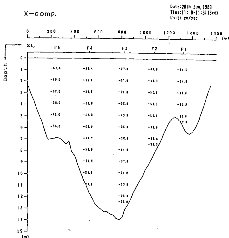
Fig. 2. 1-2(20) Profile in Distribution of Discharge Survey Results
