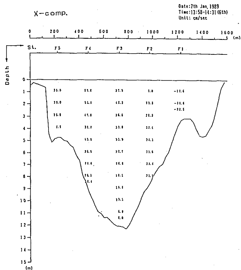
Fig. 2. 1-2(8) Profile in Distribution of Discharge Survey Results
