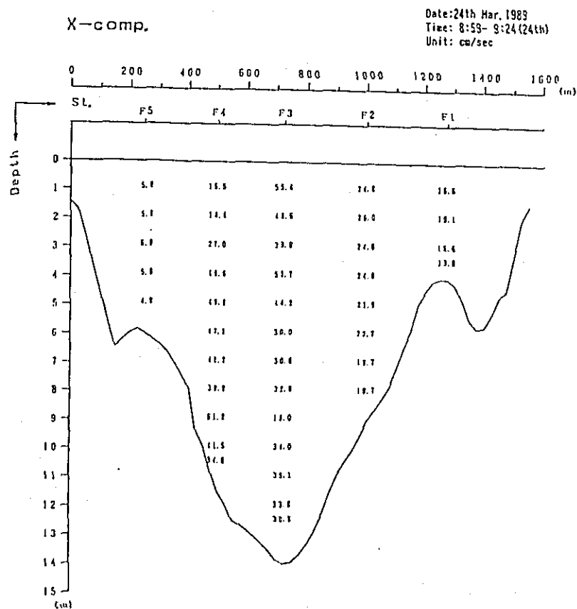
Fig. 2. 1-2(149) Profile in Distribution of Discharge Survey Results (6th Stage)
