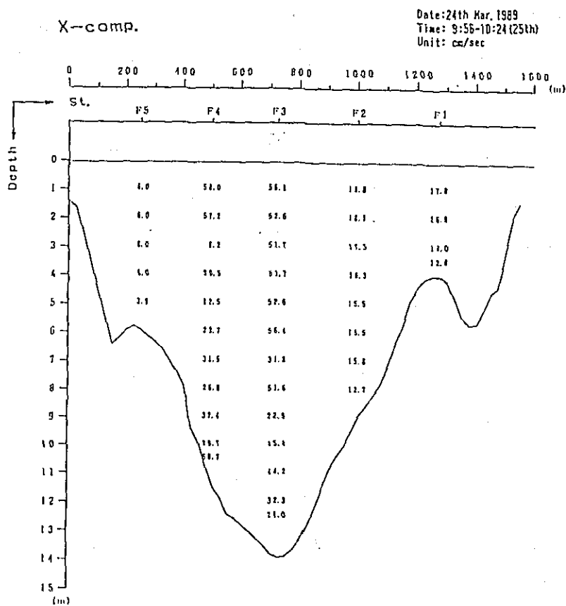
Fig. 2. 1-2(50) Profile in Distribution of Discharge Survey Results (6th Stage)
