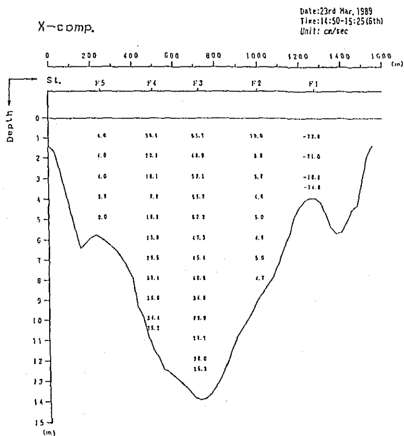
Fig. 2. 1-2(13) Profile in Distribution of Discharge Survey Results
