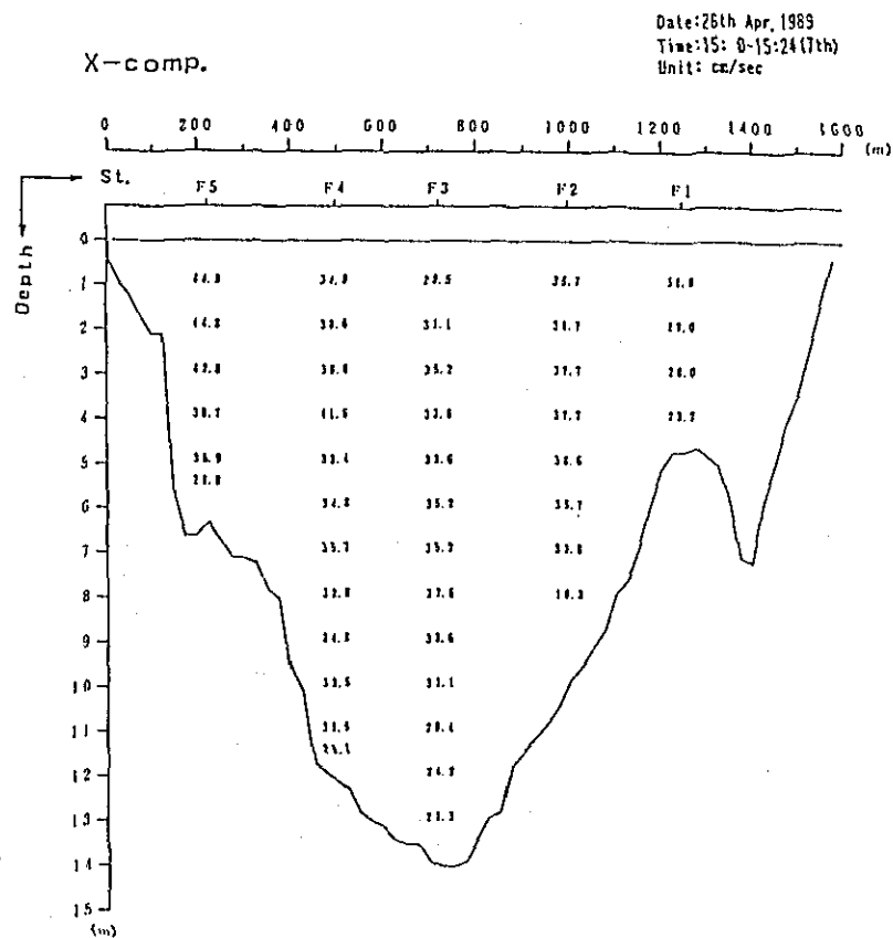
Fig. 2. 1-2(157) Profile in Distribution of Discharge Survey Results (7th Stage)
