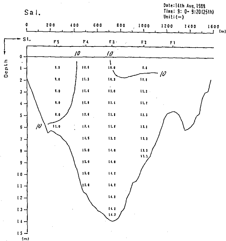
Fig. 2. 1-1(300) Profile in Distribution of Discharge Survey Results (2th Stage)
