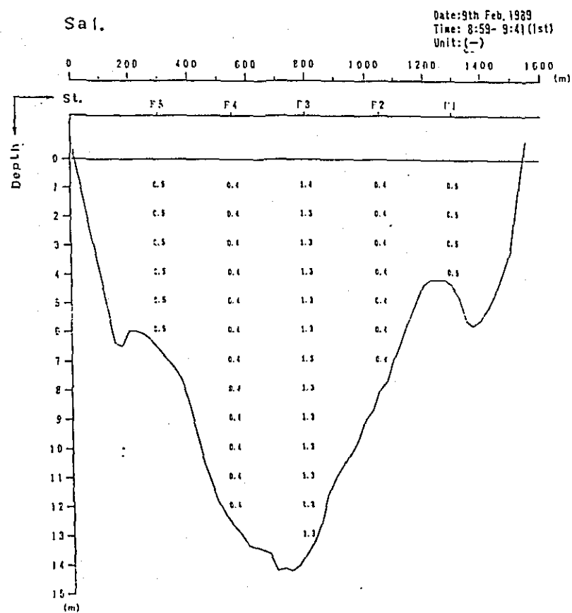
Fig. 2. 1-1(10) Profile in Distribution of Discharge Survey Results (5th Stage)
