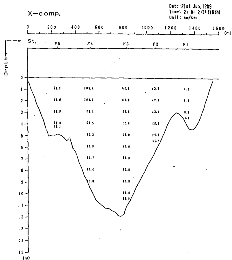
Fig. 2. 1-2(20) Profile in Distribution of Discharge Survey Results. (9th Stage)
