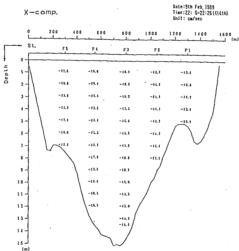
Fig. 2. 1-2(14) Profile in Distribution of Discharge Survey Results (5th Stage)
