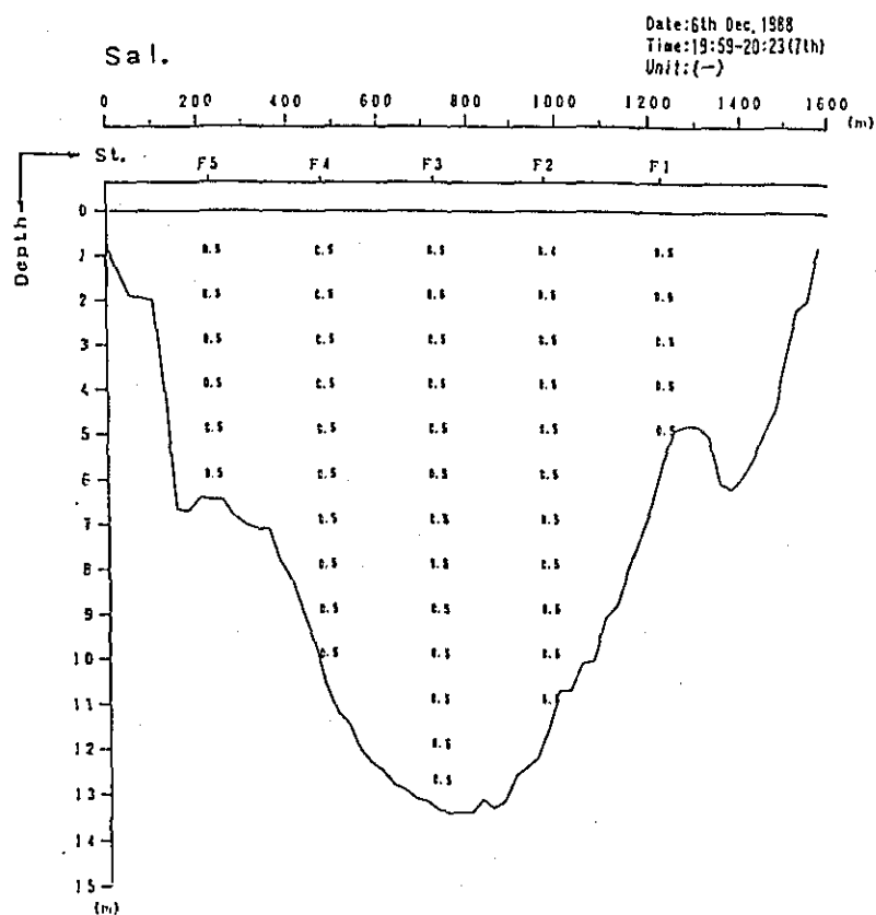
Fig. 2. 1-1(57) Profile in Distribution of Discharge Survey Results (3rd Stage)
