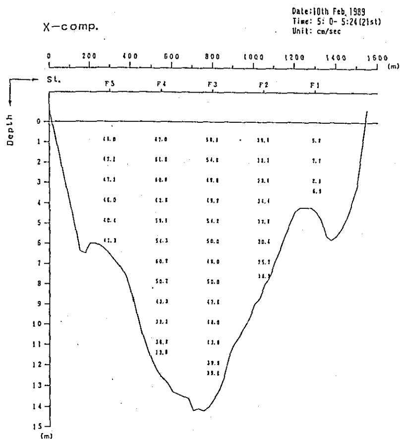
Fig. 2. 1-2(21) Profile in Distribution of Discharge Survey Results
