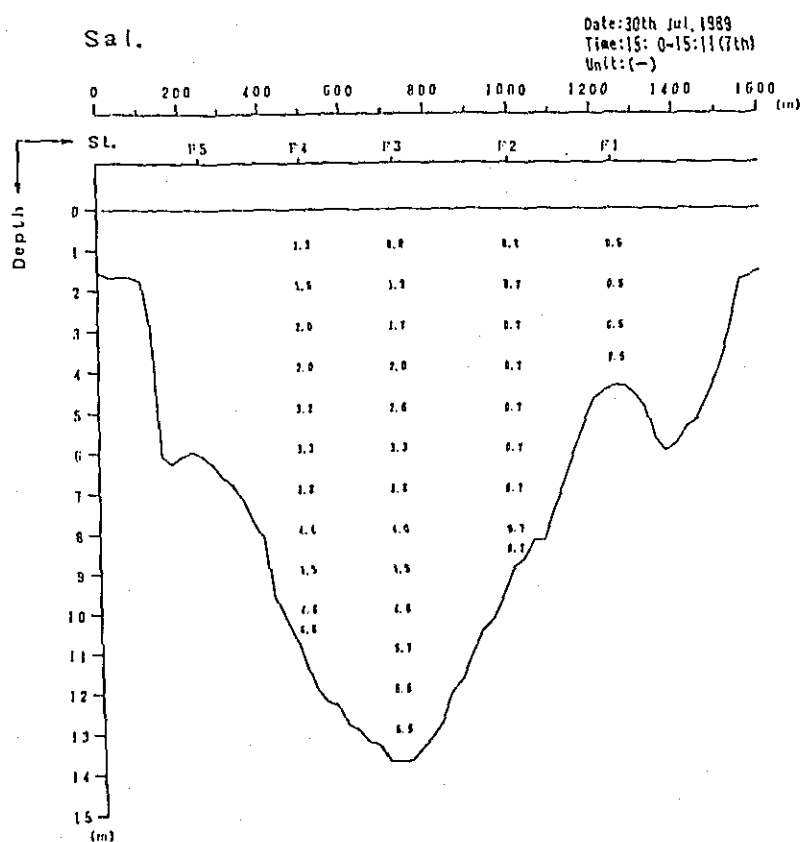
Fig. 2. 1-1(257) Profile in Distribution of Discharge Survey Results (11th Stage)
