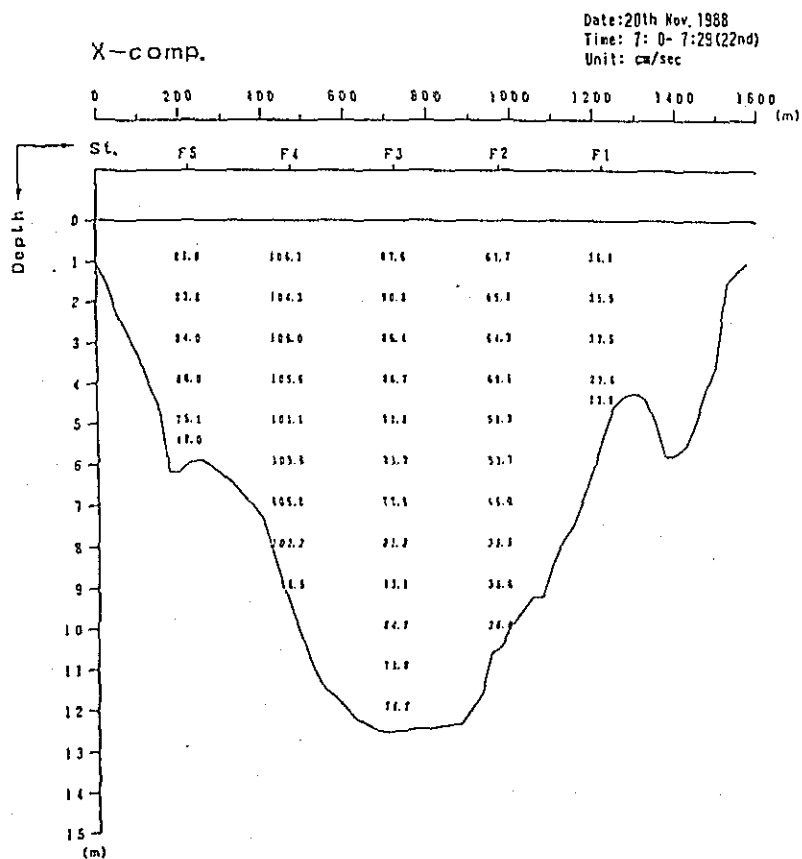
Fig. 2.1-2(47) Profile in Distribution of Discharge Survey Results (2nd Stage)
