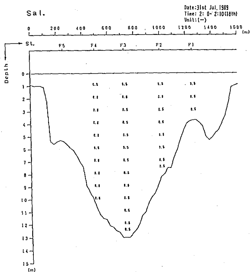
Fig. 2. 1-1 (268) Profile in Distribution of Discharge Survey Results (11th Stage)
