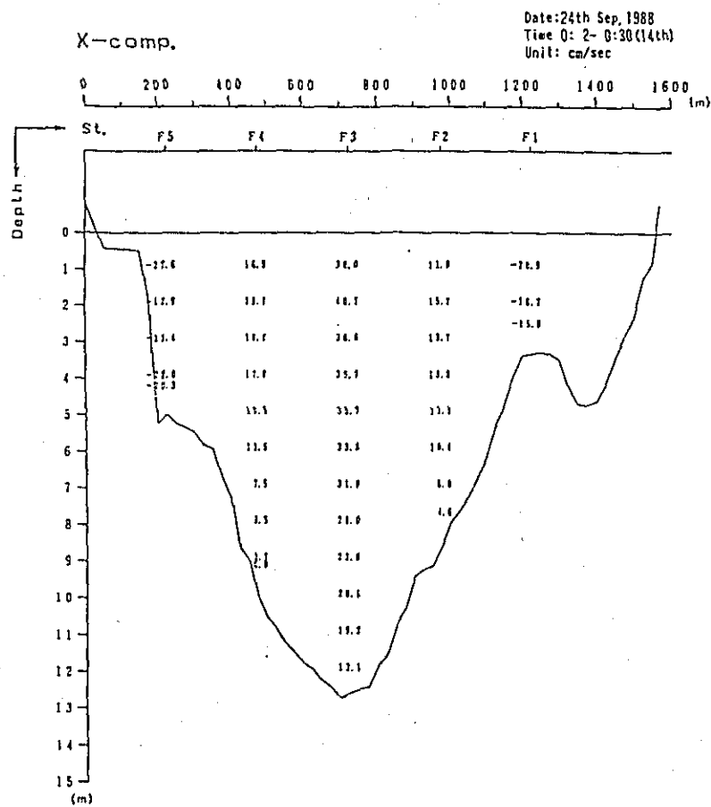
Fig. 2. 1-2(14) Profile in Distribution of Discharge Survey Results (1st Stage)
