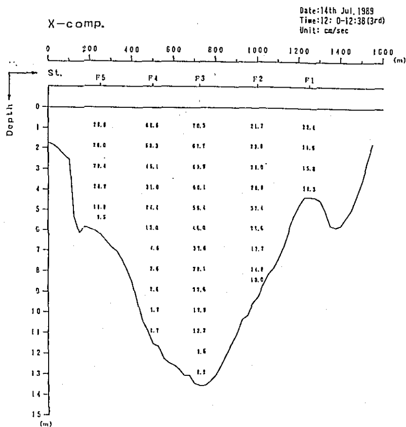
Fig. 2. 1-2(28) Profile in Distribution of Discharge Survey Results (10th Stage)
