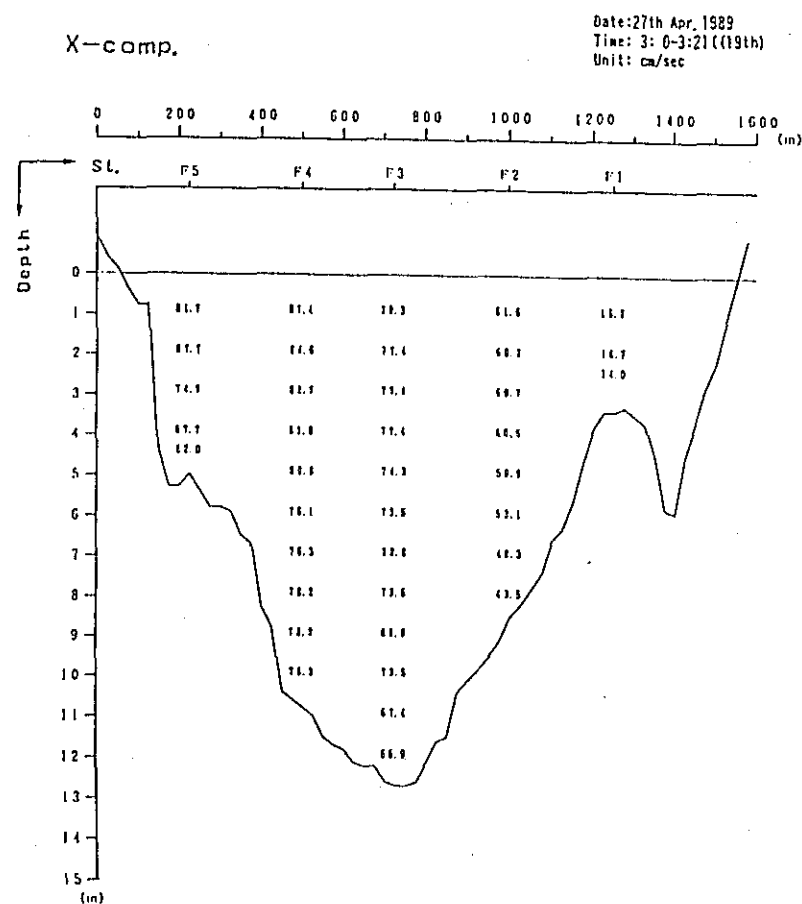
Fig. 2. 1-2(169) Profile in Distribution of Discharge Survey Results (7th Stage)
