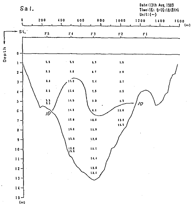
Fig. 2. 1-1(223) Profile in Distribution of Discharge Survey Results (12th Stage)
