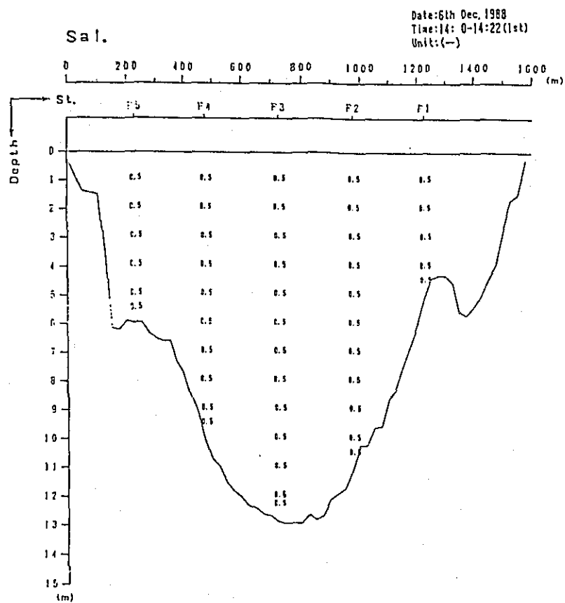
Fig. 2. 1-151) Profile in Distribution of Discharge Survey Results (3rd Stage)
