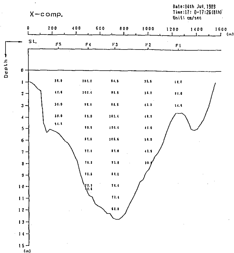
Fig. 2. 1-2(23) Profile in Distribution of Discharge Survey Results (10th Stage)
