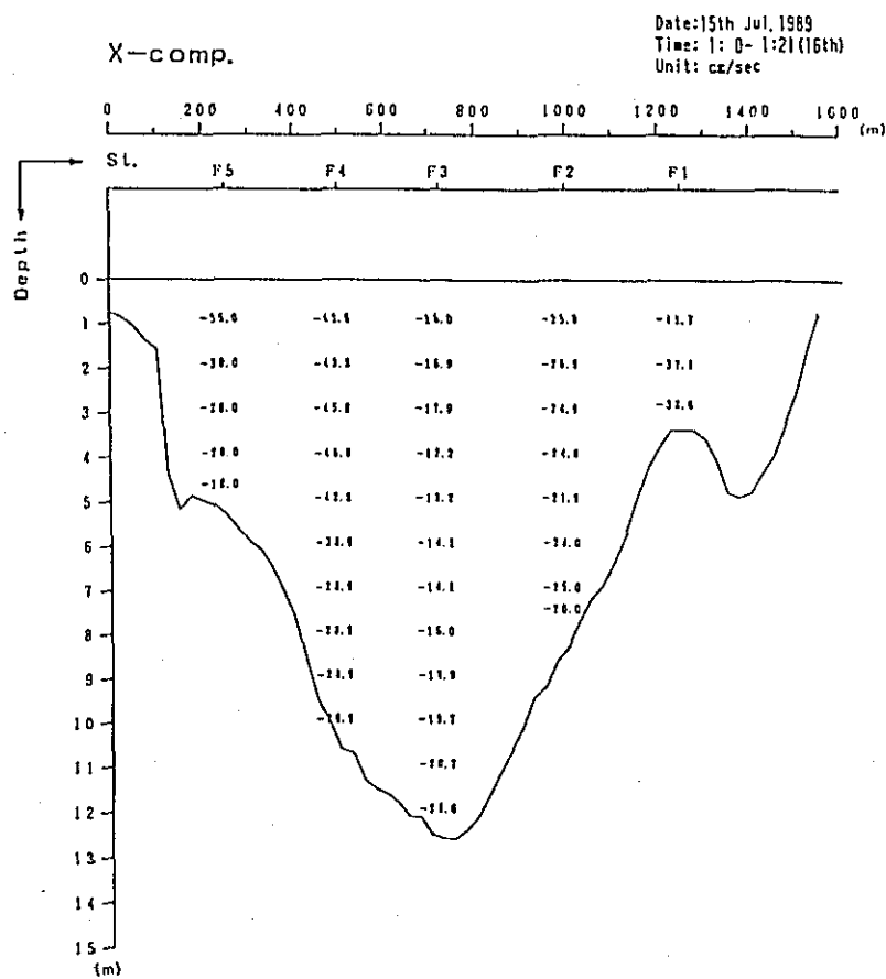
Fig. 2. 1-2(24) Profile in Distribution of Discharge Survey Results (00th Stage)
