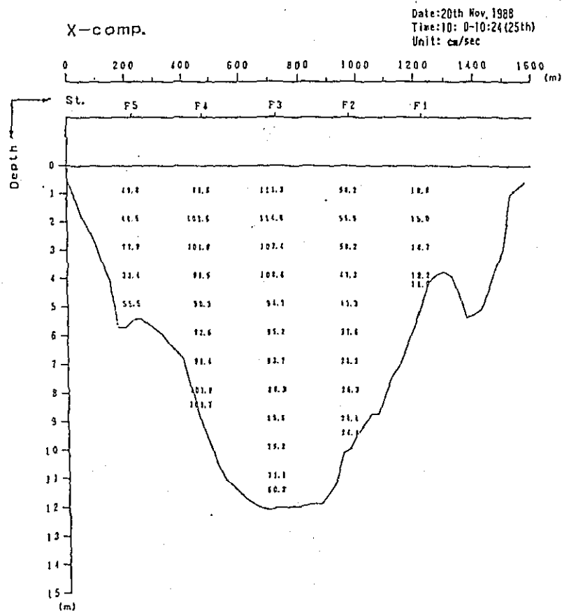
Fig. 2. 1-2(50) Profile in Distribution of Discharge Survey Results
