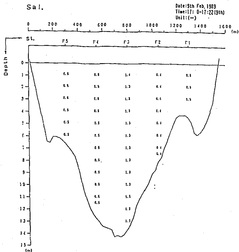
Fig. 2. 1-1(109) Profile in Distribution of Discharge Survey Results (5th Stage)
