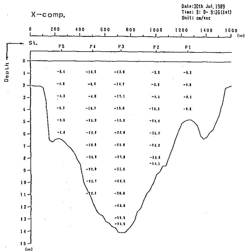
Fig. 2. 1-2(251) Profile in Distribution of Discharge Survey Results (11th Stage)
