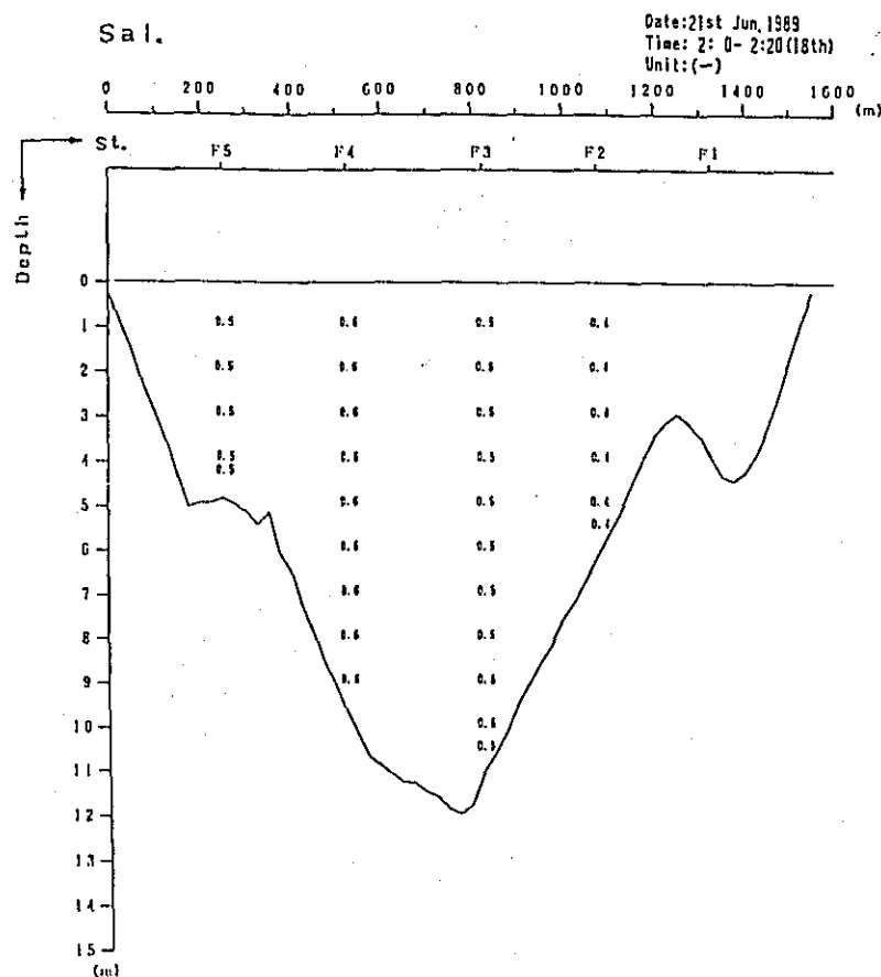
Fig. 2. 1-1(218) Profile in Distribution of Discharge Survey Results (9th Stage)
