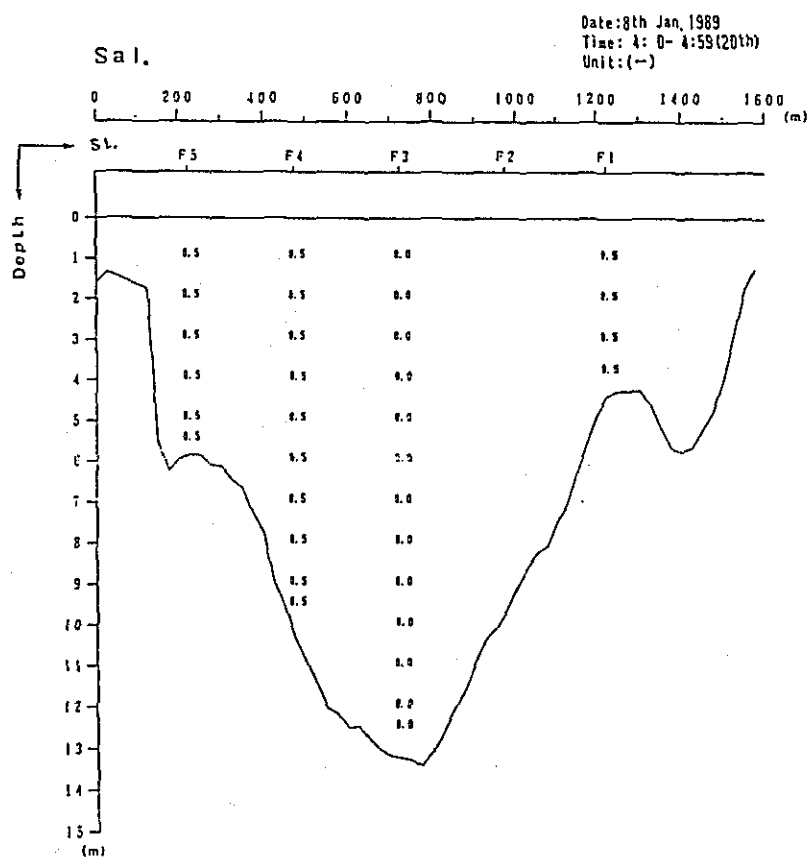
Fig. 2. 1-1(95) Profile in Distribution of Discharge Survey Results (4th Stage)
