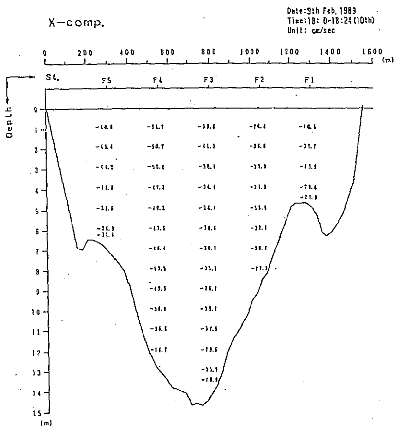
Fig. 2. 1-2(110) Profile in Distribution of Discharge Survey Results (5th Stage)
