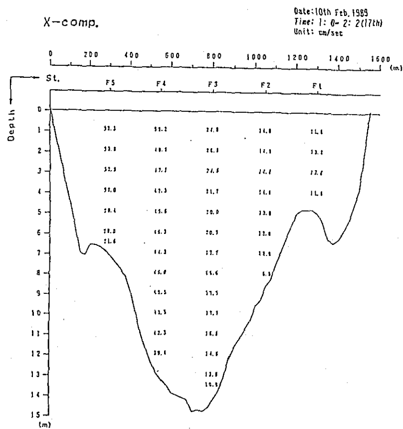
Fig. 2. 1-2(117) Profile in Distribution of Discharge Survey Results (5th Stage)
