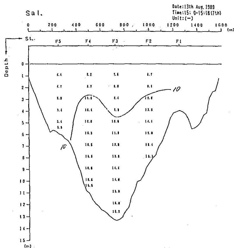
Fig. 2. 1-1(232) Profile in Distribution of Discharge Survey Results (12th Stage).
