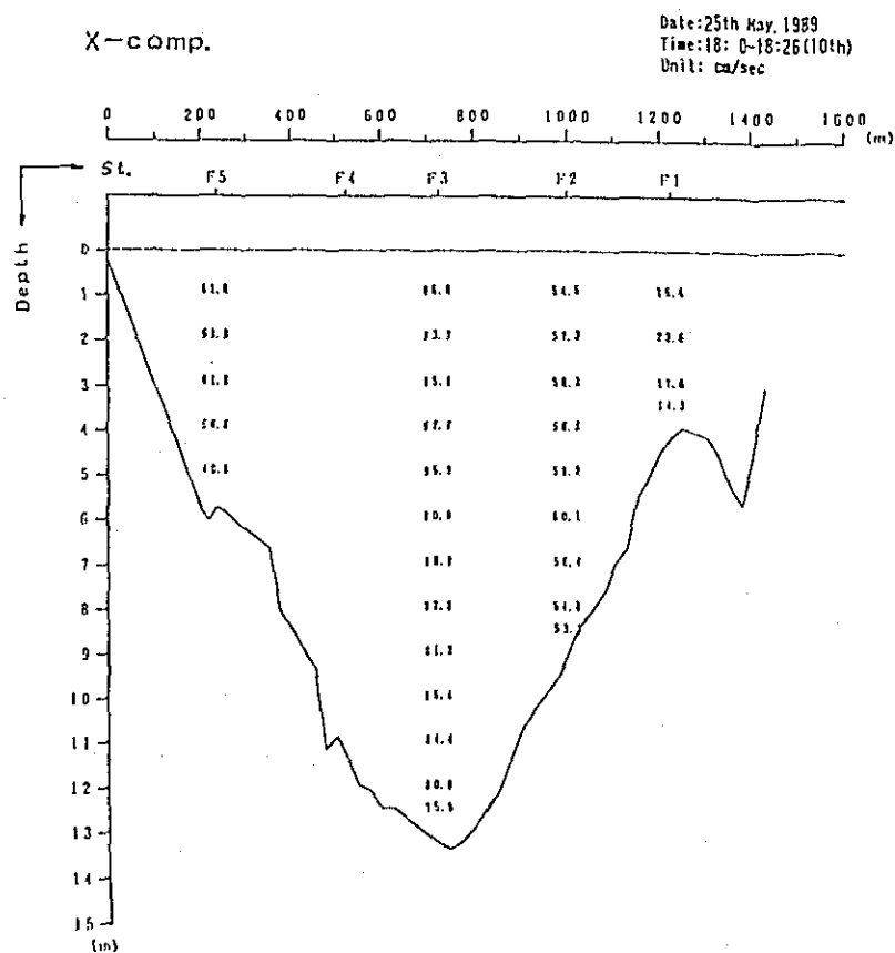
Fig. 2. 1-2(185) Profile in Distribution of Discharge Survey Results (8th Stage)
