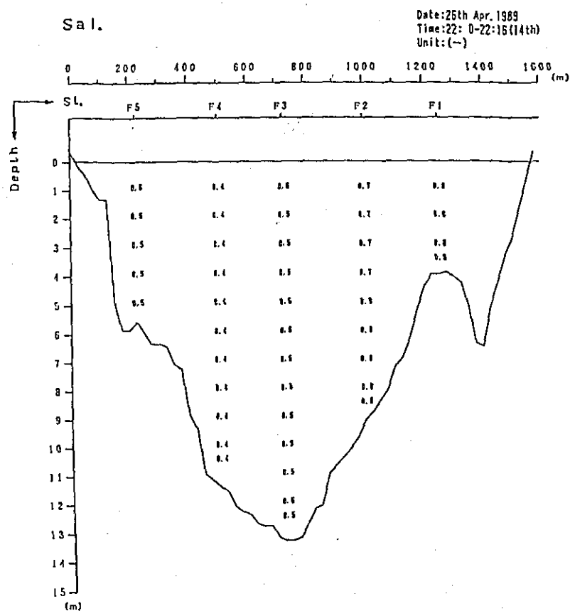
Fig. 2. 1-1(164) Profile in Distribution of Discharge Survey Results (7th Stage)
