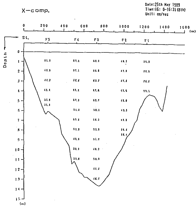
Fig. 2. 1-2(183) Profile in Distribution of Discharge Survey Results (8th Stage)
