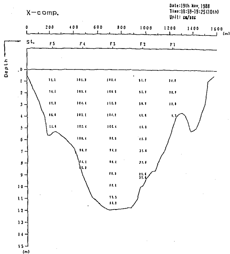
Fig. 2. 1-2(35) Profile in Distribution of Discharge Survey Results
