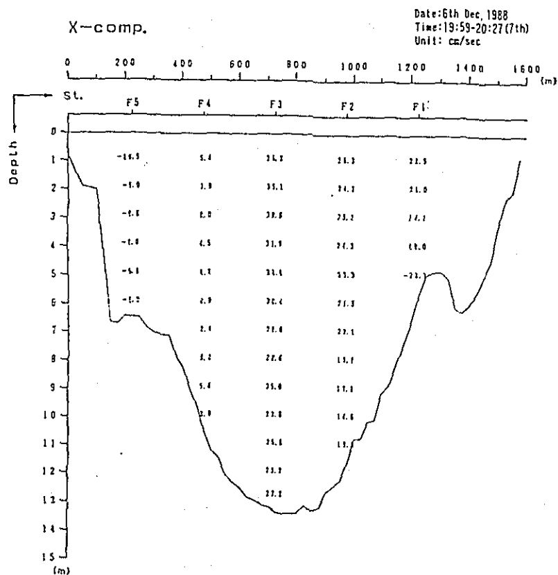
Fig. 2. 1-2(57) Profile in Distribution of Discharge Survey Results (3rd Stage)
