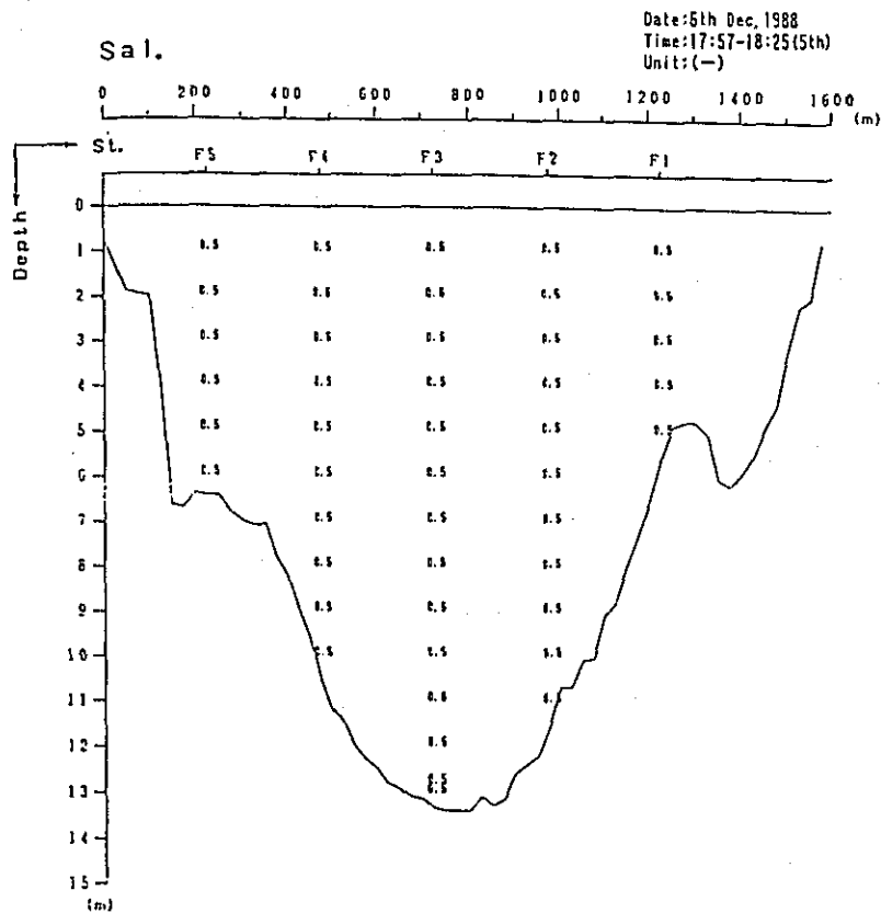
Fig. 2. 1-1(55) Profile in Distribution of Discharge Survey Results (3rd Stage)
