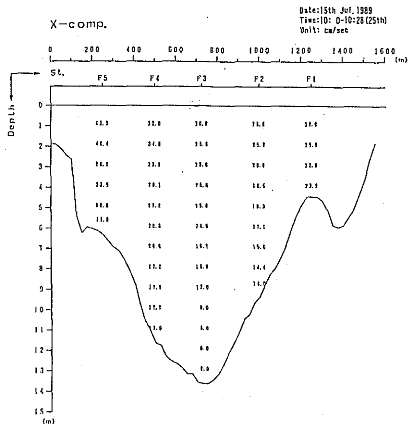
Fig. 2. 1-2 (250) Profile in Distribution of Discharge Survey Results (10th Stage)
