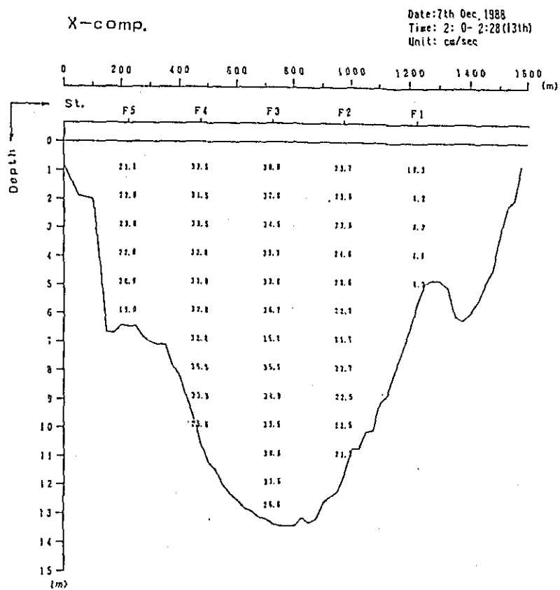
Fig. 2. 1-2(63) Profile in Distribution of Discharge Survey Results (3rd Stage)
