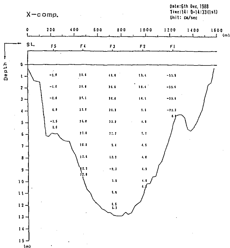
Fig. 2. 1-2(5) Profile in Distribution of Discharge Survey Results (3rd Stage)
