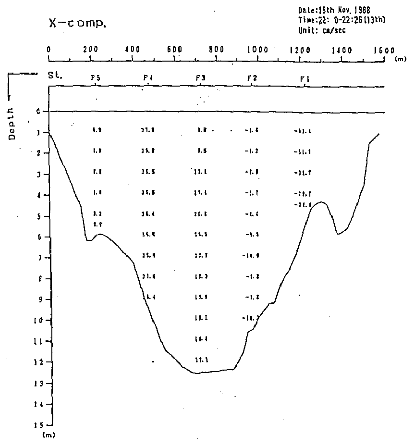
Fig. 2. 1-2(39) Profile in Distribution of Discharge Survey Results (2nd Stage)
