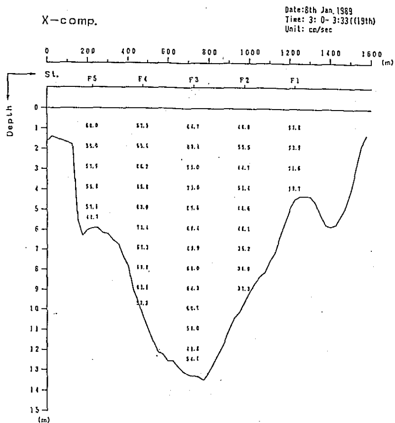
Fig. 2. 1-2(9) Profile in Distribution of Discharge Survey Results
