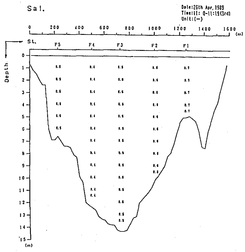
Fig. 2. 1-1(153) Profile in Distribution of Discharge Survey Results (7th Stage)
