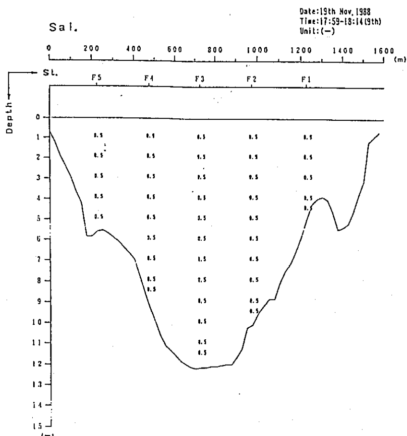
Fig. 2. 1-1(34) Profile in Distribution of Discharge Survey Results (2nd Stage)
