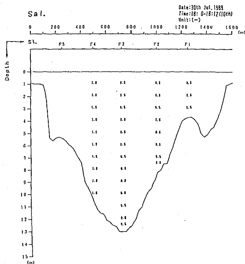
Fig. 2. 1-1(260) Profile in Distribution of Discharge Survey Results (11th Stage)
