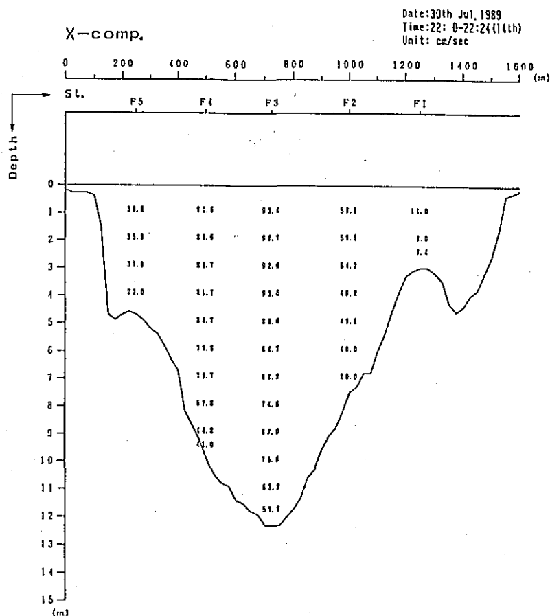
Fig. 2. 1-2(264) Profile in Distribution of Discharge Survey Results (11th Stage)
