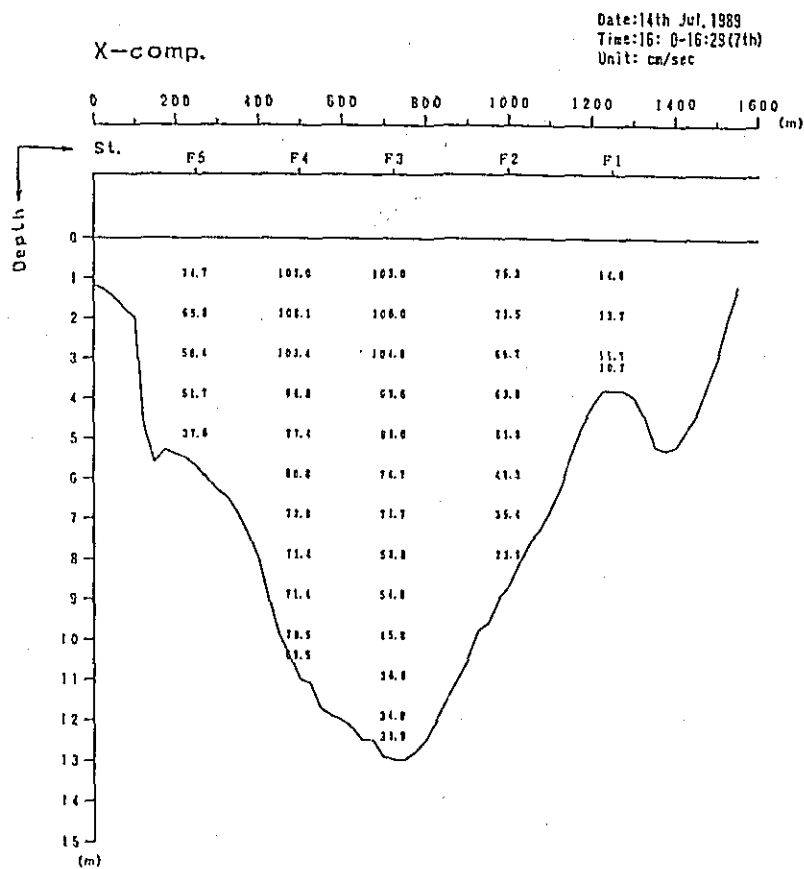
Fig. 2. 1-2(32) Profile in Distribution of Discharge Survey Results (10th Stage)
