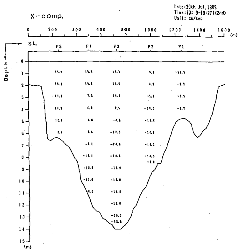
Fig. 2. 1-2(252) Profile in Distribution of Discharge Survey Results (11th Stage)
