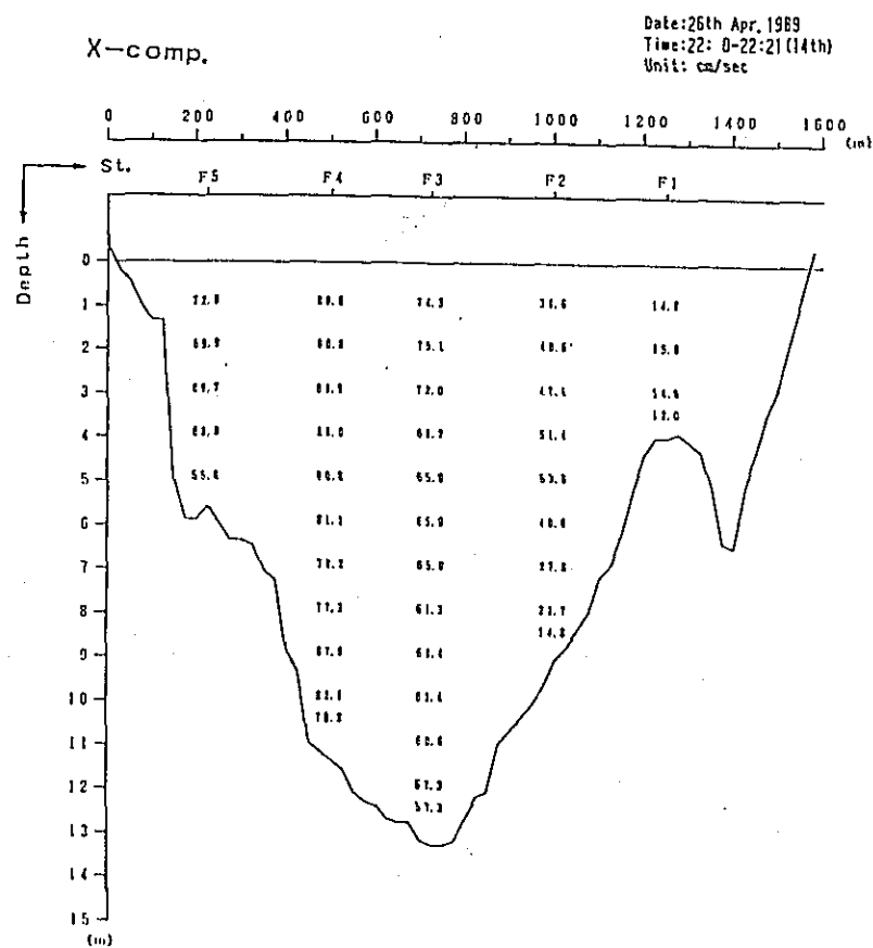
Fig. 2. 1-2(164) Profile in Distribution of Discharge Survey Results (7th Stage)
