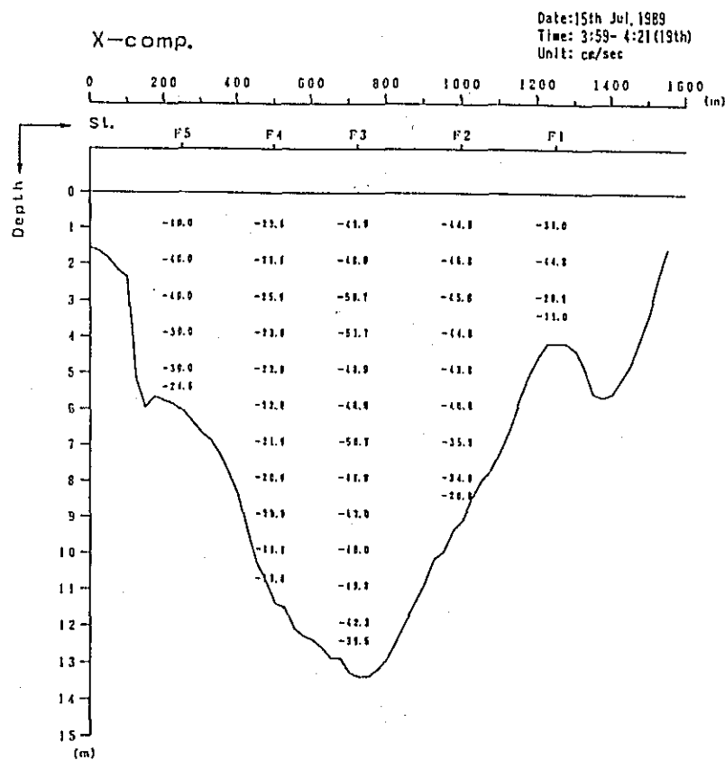
Fig. 2. 1-2(24) Profile in Distribution of Discharge Survey Results (10th Stage)
