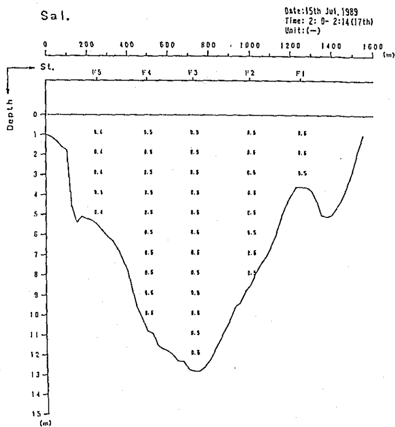
Fig. 2. 1-1(242) Profile in Distribution of Discharge Survey Results (00th Stage)
