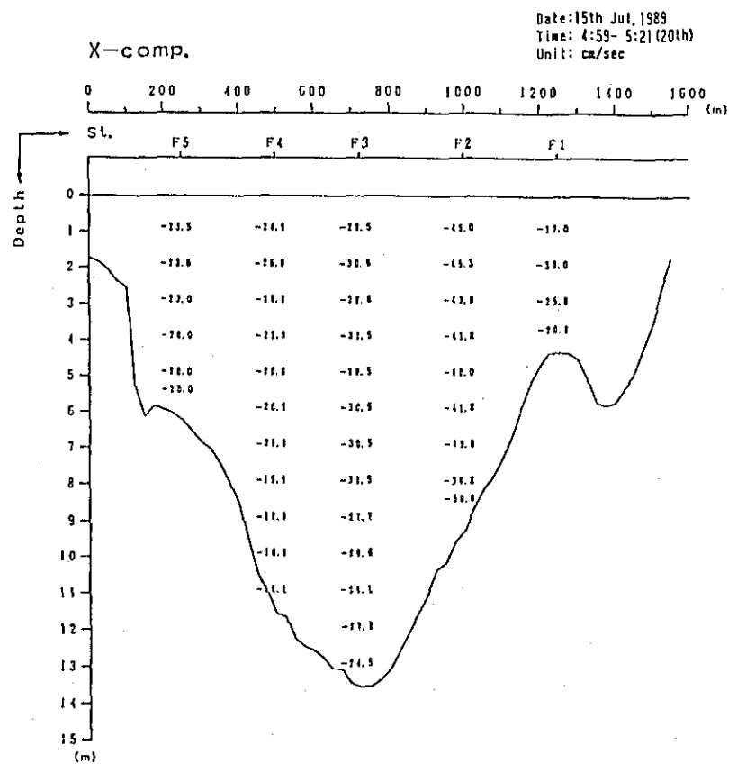
Fig. 2. 1-2(45) Profile in Distribution of Discharge Survey Results (00th Stage)
