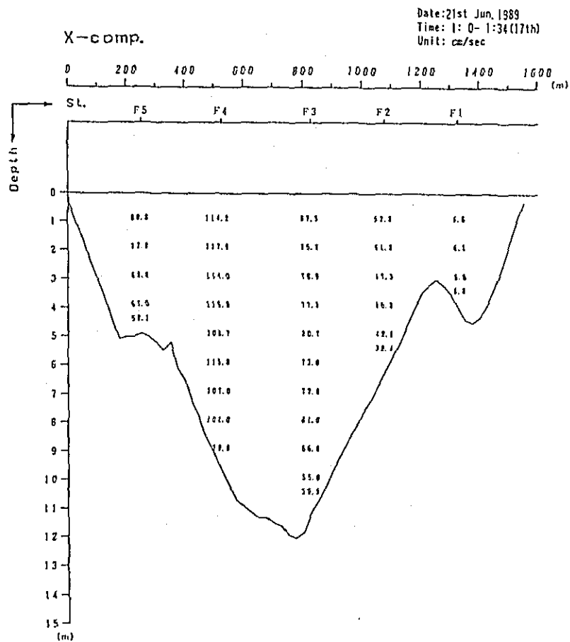
Fig. 2. 1-2(17) Profile in Distribution of Discharge Survey Results (9th Stage)
