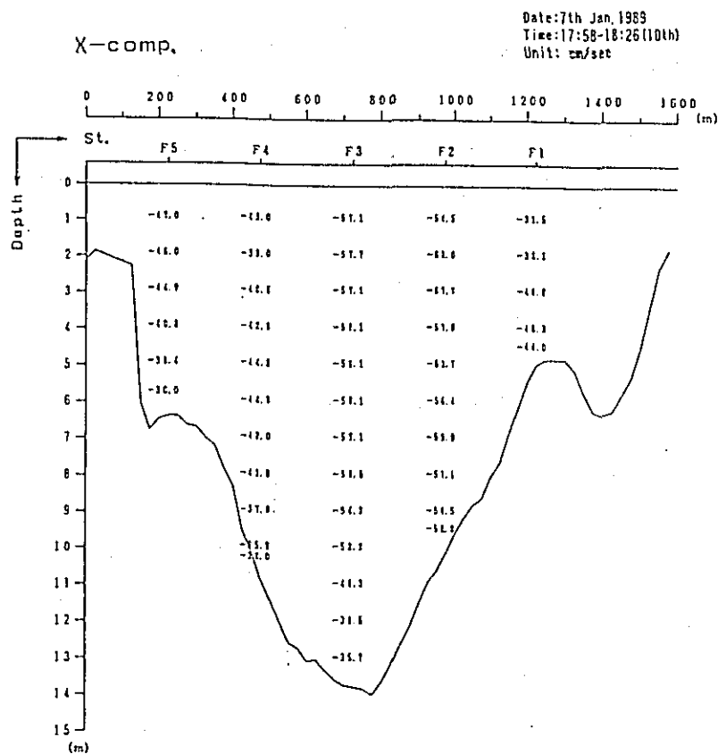
Fig. 2. 1-2(85) Profile in Distribution of Discharge Survey Results (4th Stage)
