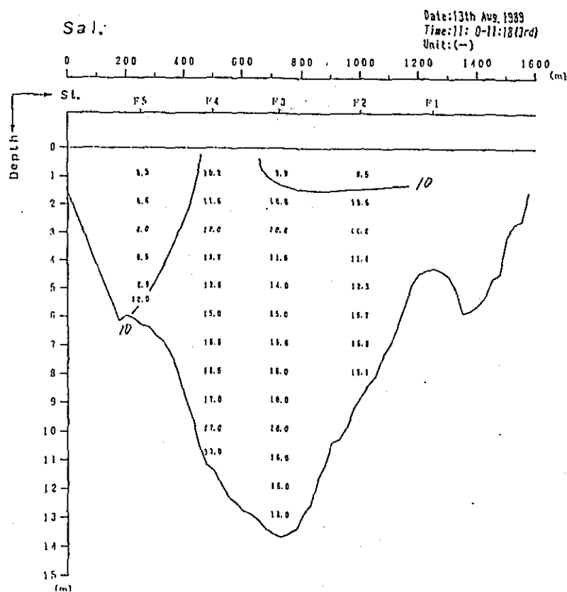
Fig. 2. 1-1(273) Profile in Distribution of Discharge Survey Results (2th Stage)
