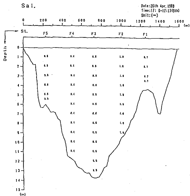
Fig. 2. 1-1(159) Profile in Distribution of Discharge Survey Results (7th Stage)
