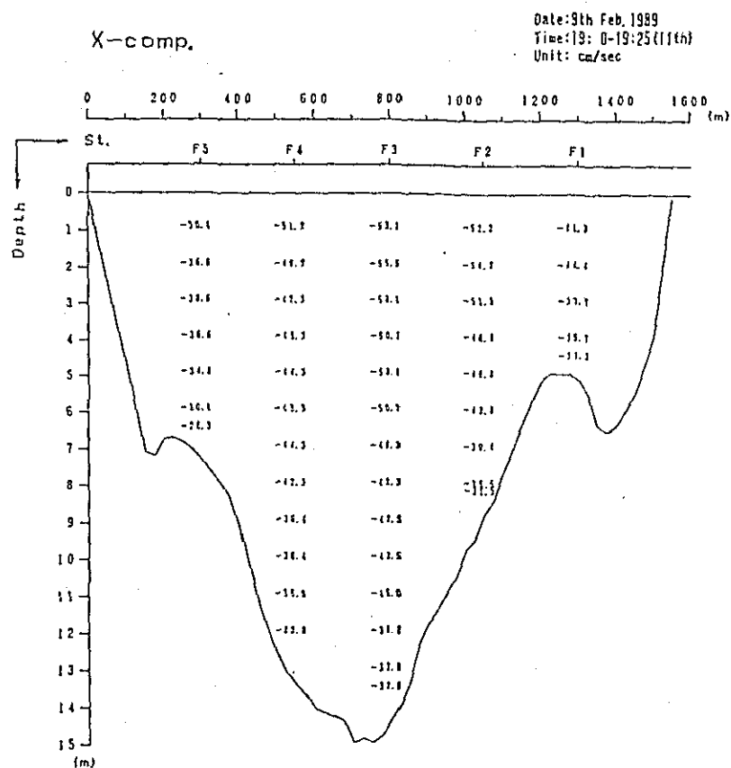
Fig. 2. 1-2(11) Profile in Distribution of Discharge Survey Results (5th Stage)
