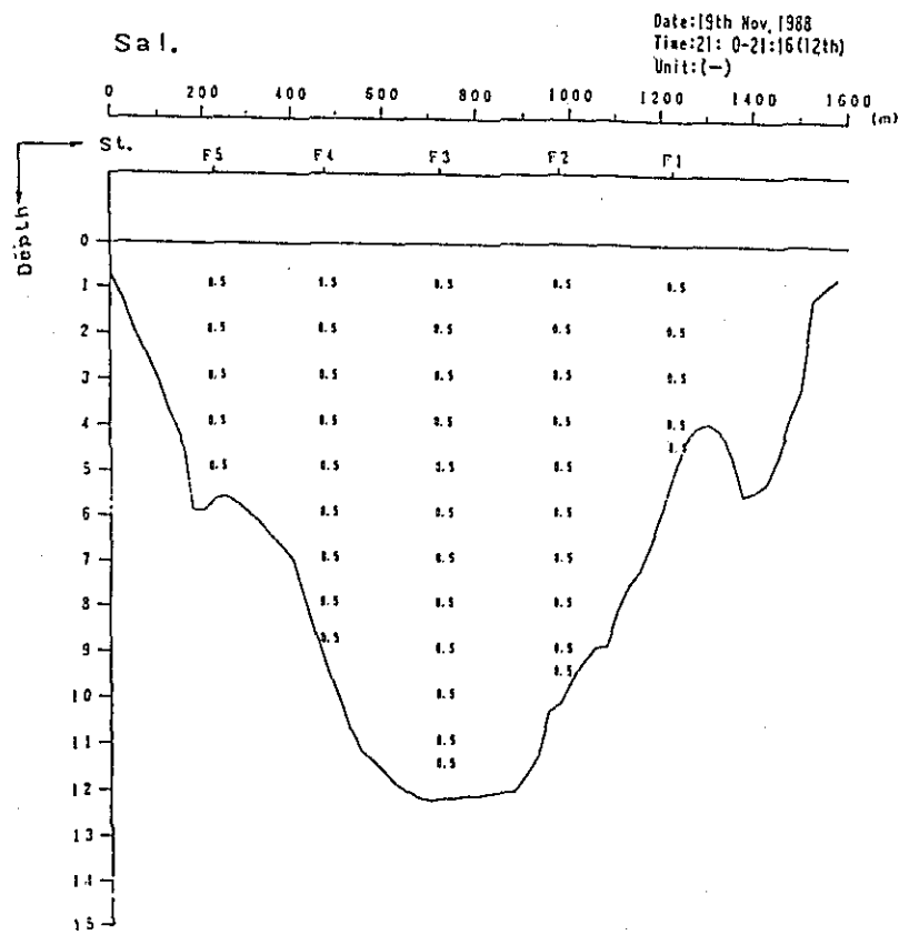
Fig. 2. 1-137 Profile in Distribution of Discharge Survey Results (2nd Stage)
