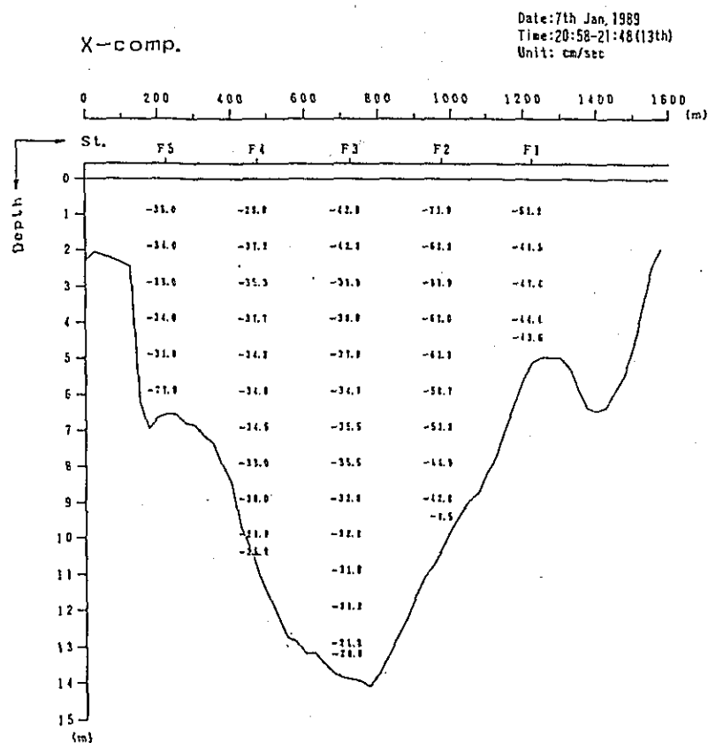
Fig. 2. 1-2(88) Profile in Distribution of Discharge Survey Results (4th Stage)
