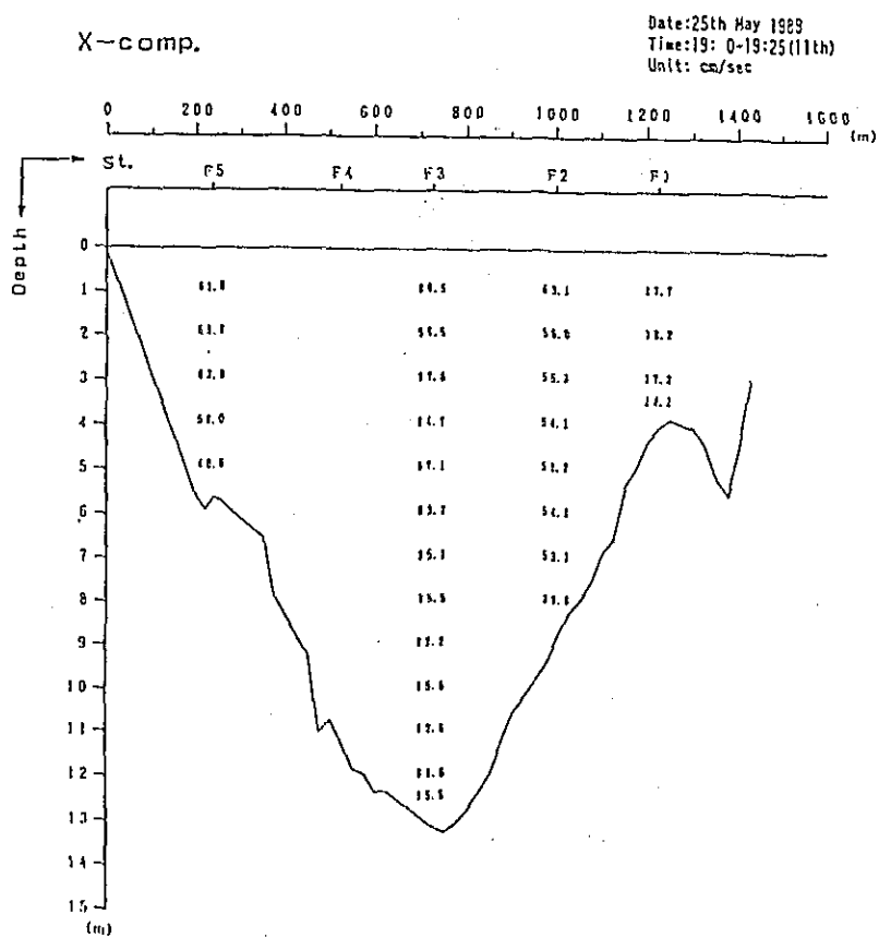
Fig. 2. 1-2(186) Profile in Distribution of Discharge Survey Results (8th Stage)
