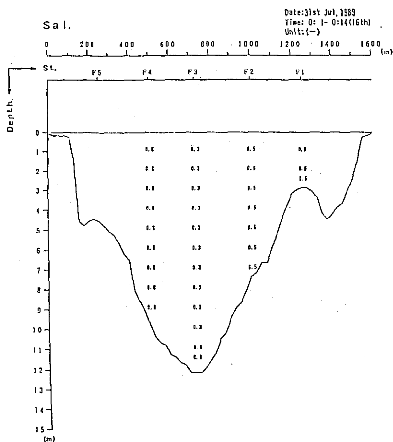
Fig. 2. 1-1(266) Profile in Distribution of Discharge Survey Results (11th Stage)
