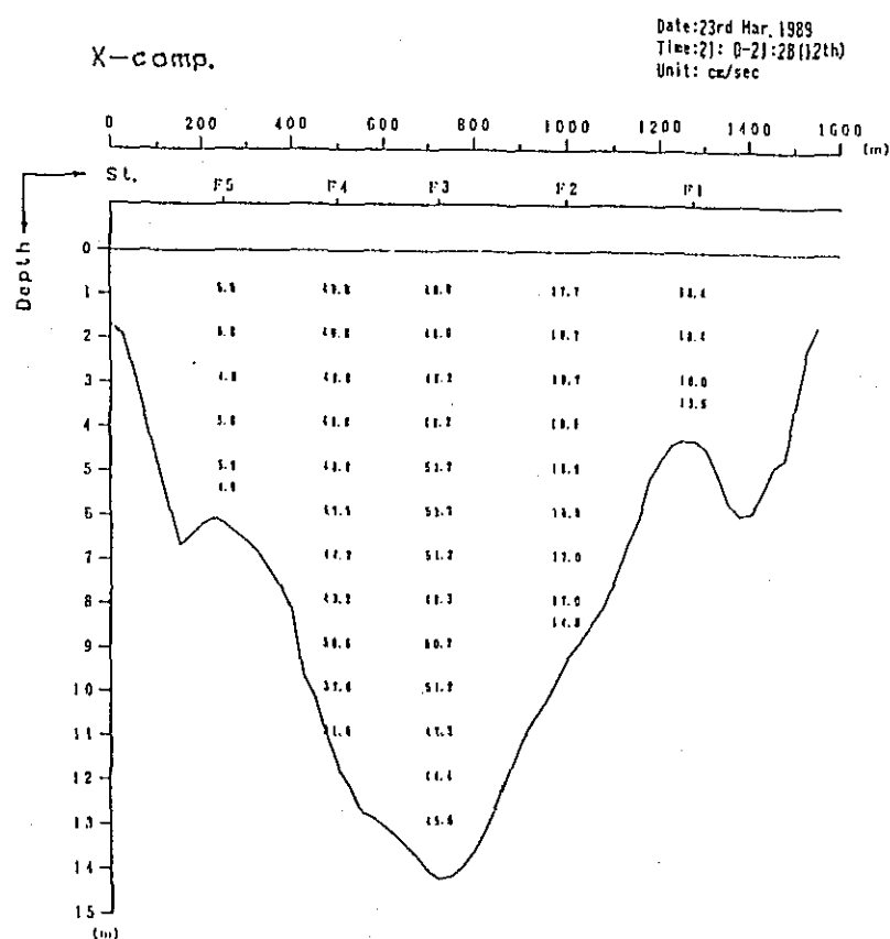
Fig. 2. 1-2(137) Profile in Distribution of Discharge Survey Results (6th Stage)
