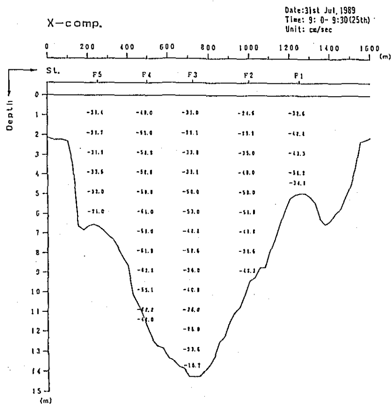
Fig. 2. 1-2(275) Profile in Distribution of Discharge Survey Results (11th Stage)
