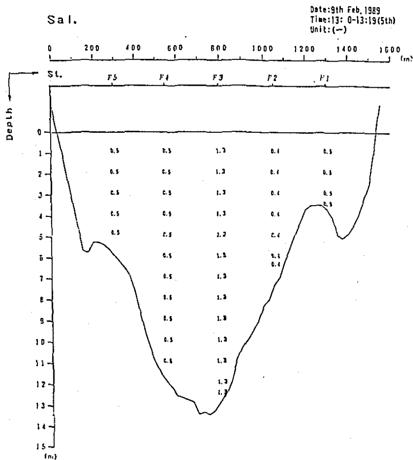
Fig. 2. 1-1(105) Profile in Distribution of Discharge Survey Results (5th Stage)
