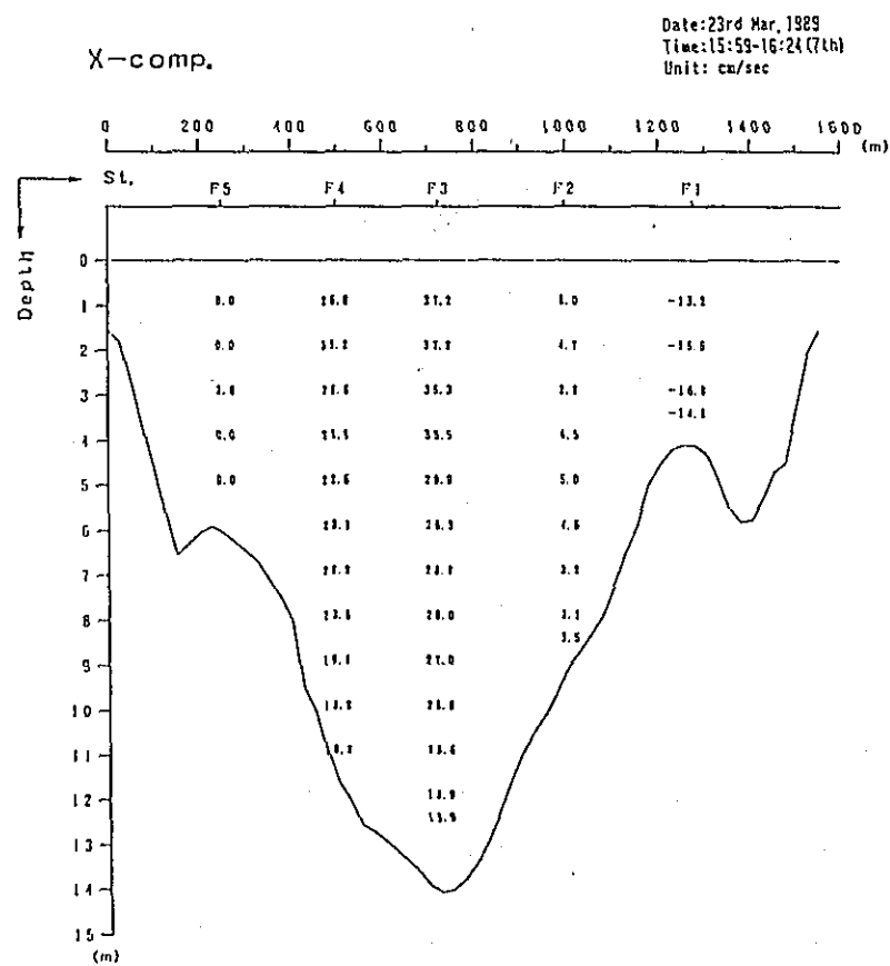
Fig. 2. 1-2(132) Profile in Distribution of Discharge Survey Results (6th Stage)
