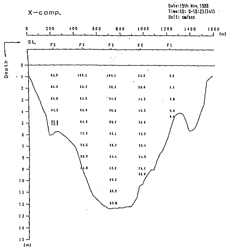
Fig. 2. 1-2(26) Profile in Distribution of Discharge Survey Results (2nd Stage)
