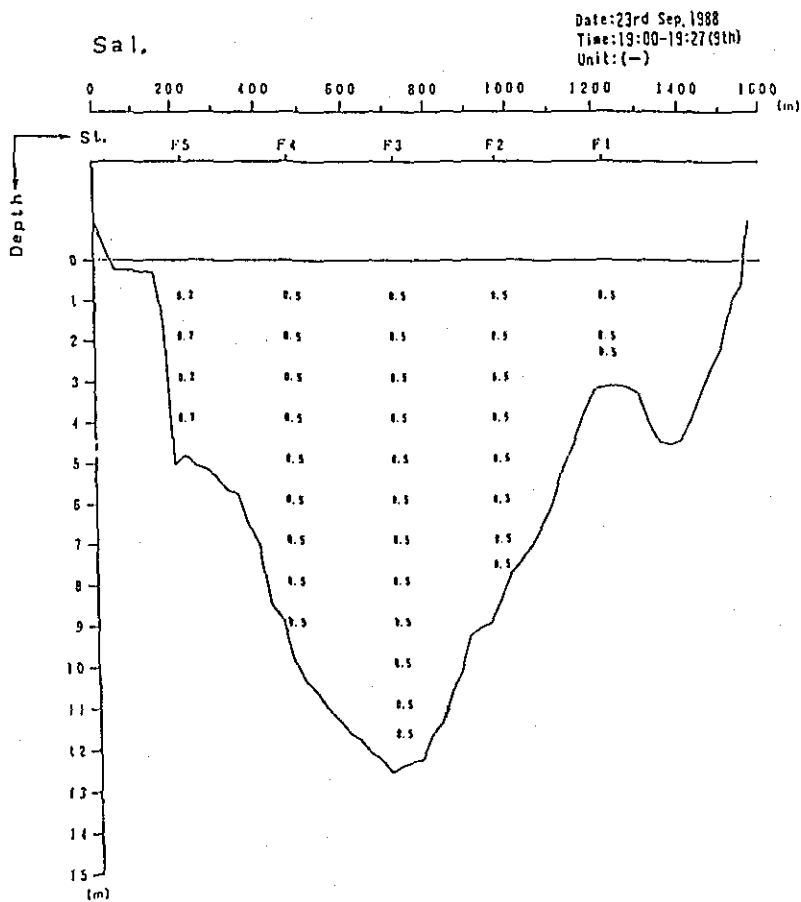
Fig. 2. 1-1(9) Profile in Distribution of Discharge Survey Results (1st Stage)
