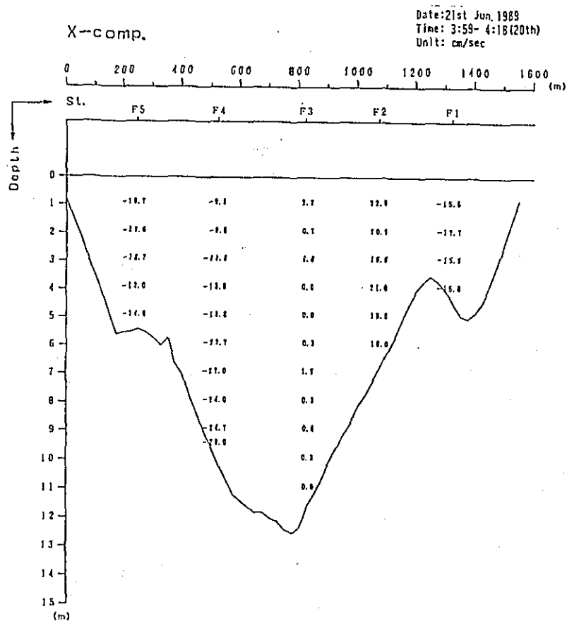
Fig. 2. 1-2(220) Profile in Distribution of Discharge Survey Results (9th Stage)
