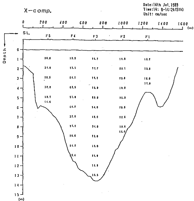
Fig. 2. 1-2(230) Profile in Distribution of Discharge Survey Results (10th Stage)
