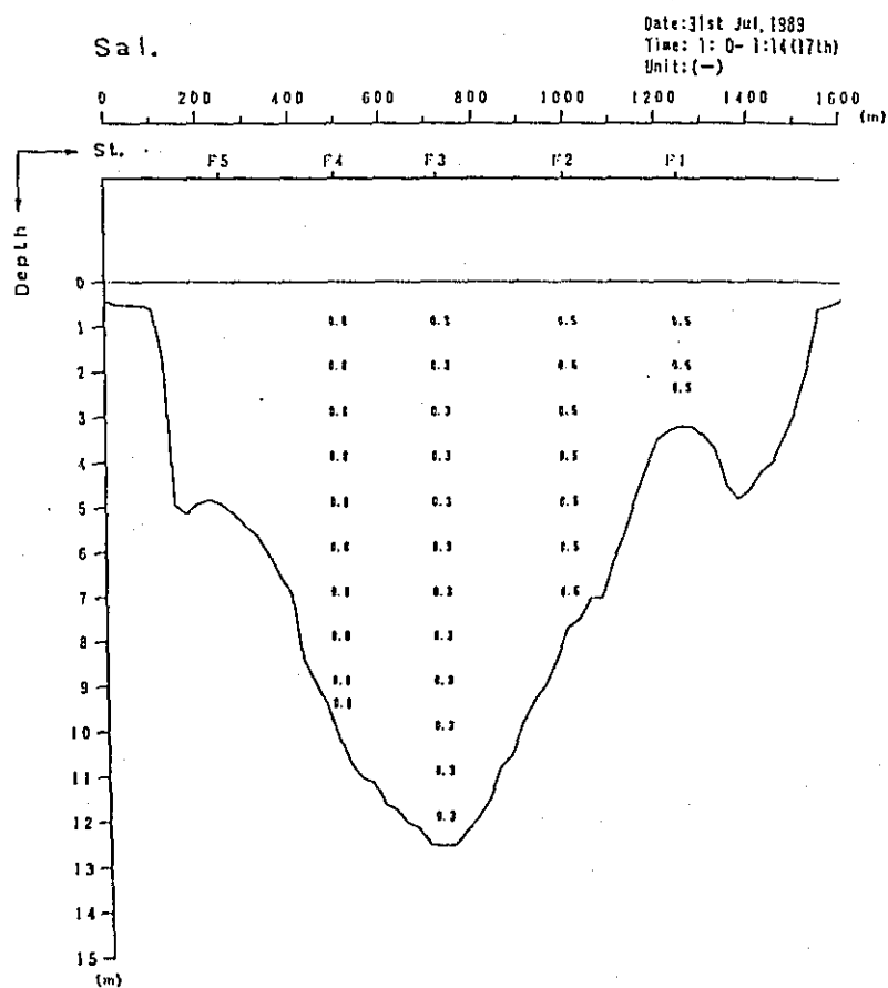
Fig. 2. 1-1267 Profile in Distribution of Discharge Survey Results (11th Stage)
