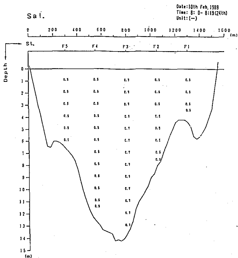
Fig. 2. 1-1(124) Profile in Distribution of Discharge Survey Results (5th Stage)
