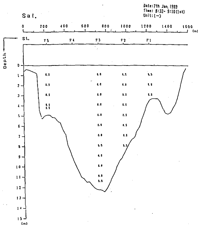
Fig. 2. 1-1(76) Profile in Distribution of Discharge Survey Results (4th Stage)
