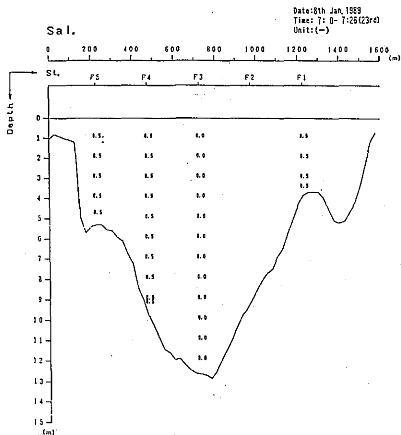
Fig. 2. 1-1(2) Profile in Distribution of Discharge Survey Results (4th Stage)
