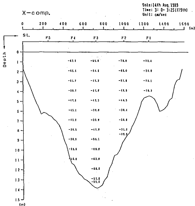
Fig. 2. 1-2(24) Profile in Distribution of Discharge Survey Results (12th Stage)
