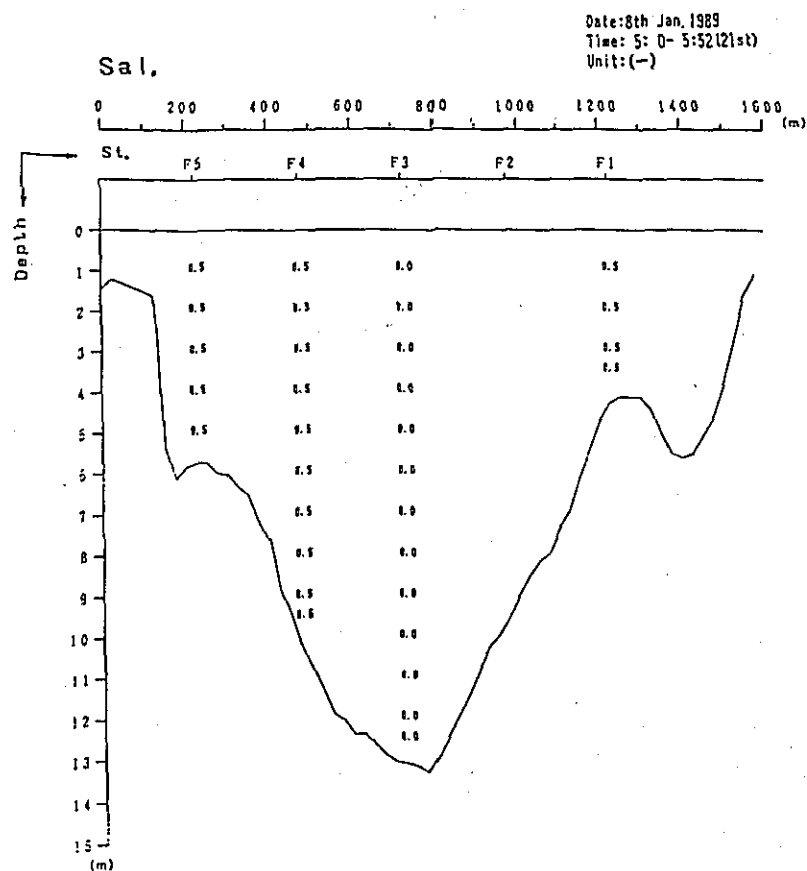
Fig. 2. 1-100 Profile in Distribution of Discharge Survey Results (4th Stage)
