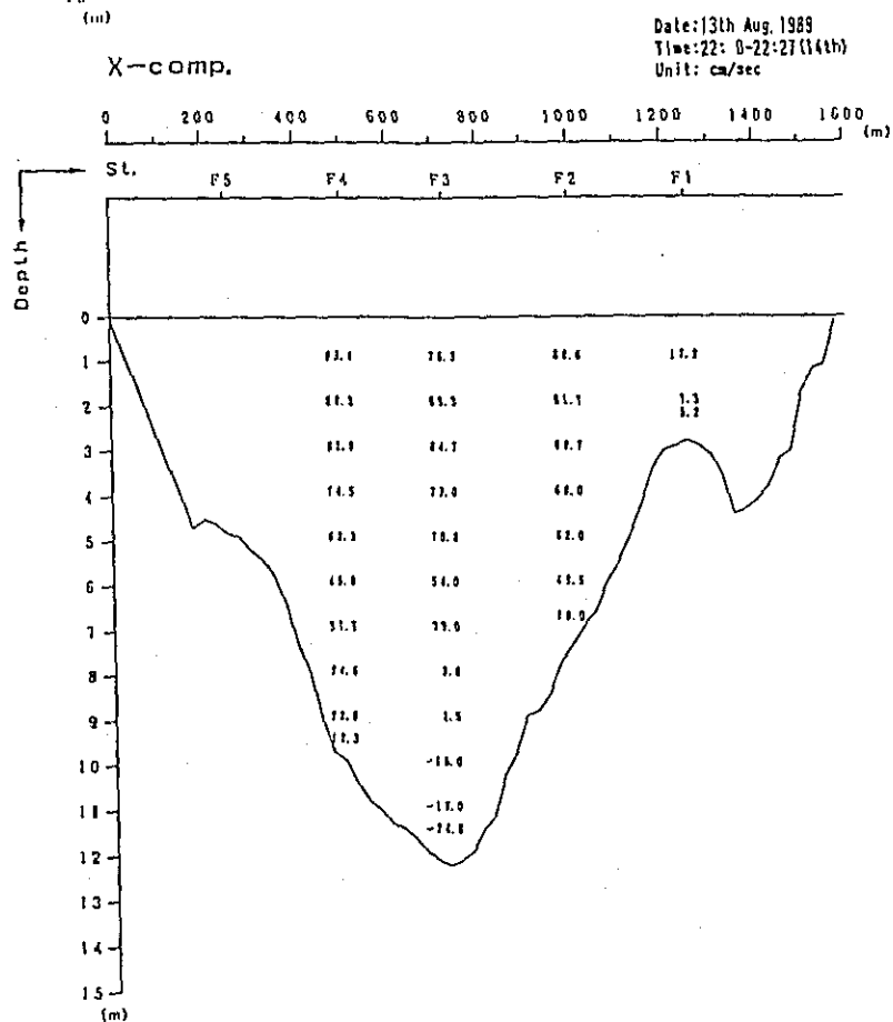
Fig. 2. 1-2(239) Profile in Distribution of Discharge Survey Results (12th Stage)
