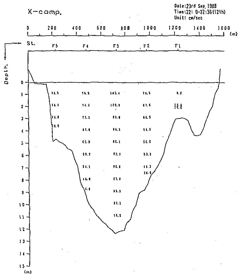
Fig. 2. 1-2(12) Profile in Distribution of Discharge Survey Results (1st Stage)
