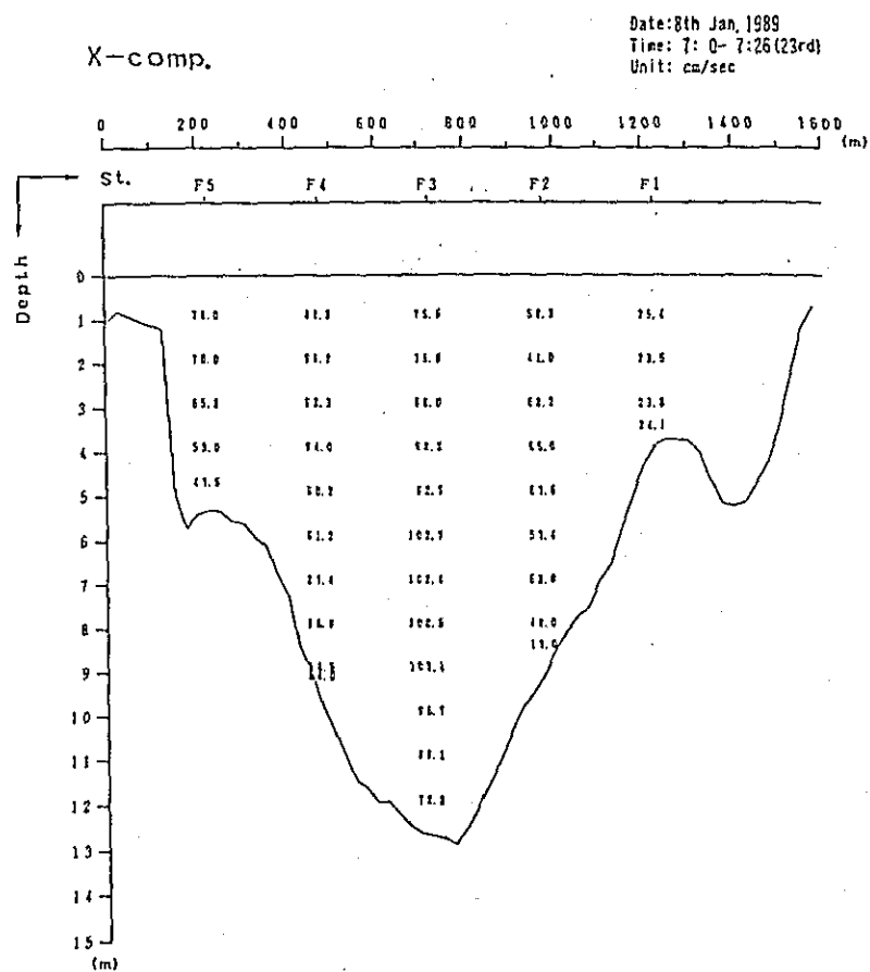
Fig. 2. 1-2(93) Profile in Distribution of Discharge Survey Results (4th Stage)
