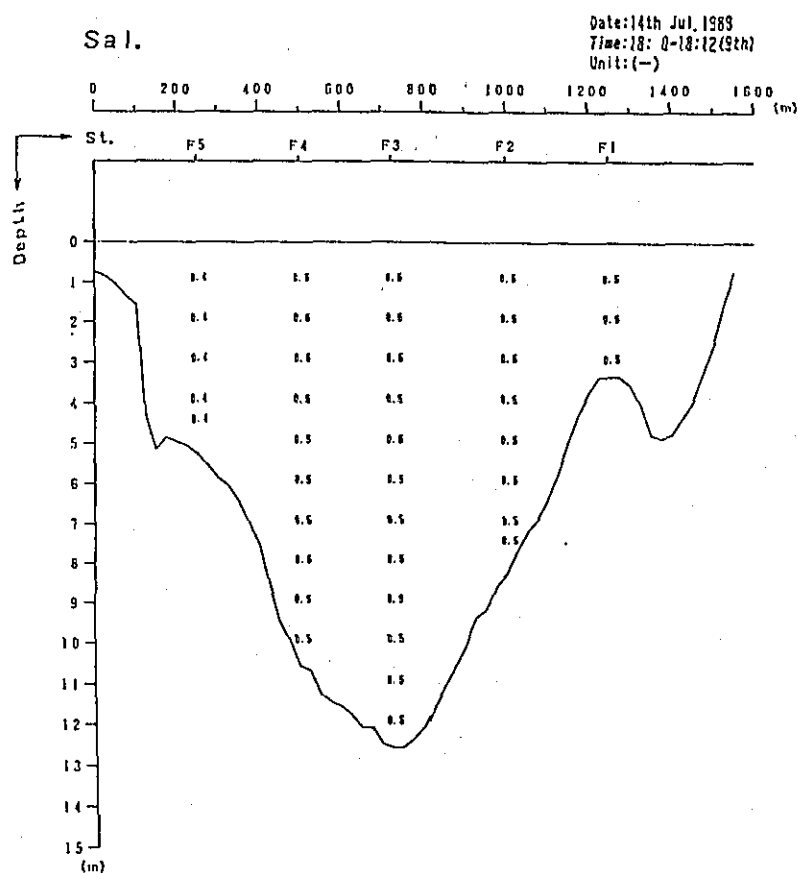
Fig. 2. 1-1(234) Profile in Distribution of Discharge Survey Results (10th Stage)
