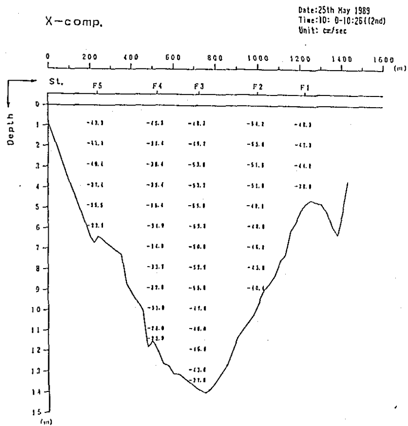
Fig. 2. 1-2(177) Profile in Distribution of Discharge Survey Results (8th Stage)
