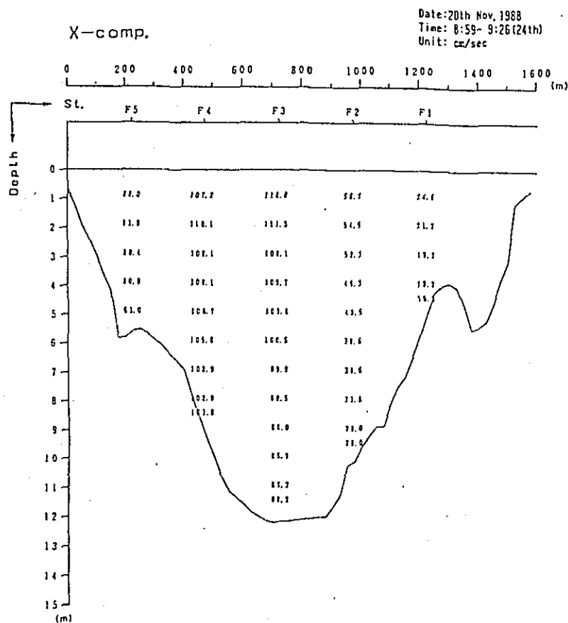
Fig. 2. 1-2(49) Profile in Distribution of Discharge Survey Results (2nd Stage)
