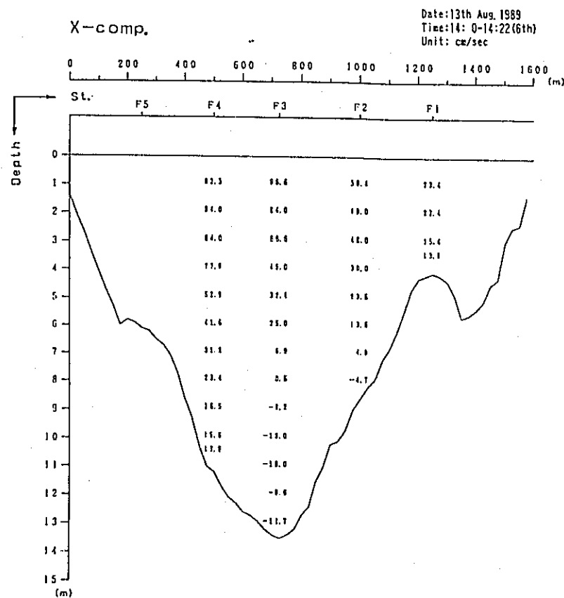
Fig. 2. 1-2(28) Profile in Distribution of Discharge Survey Results (12th Stage)
