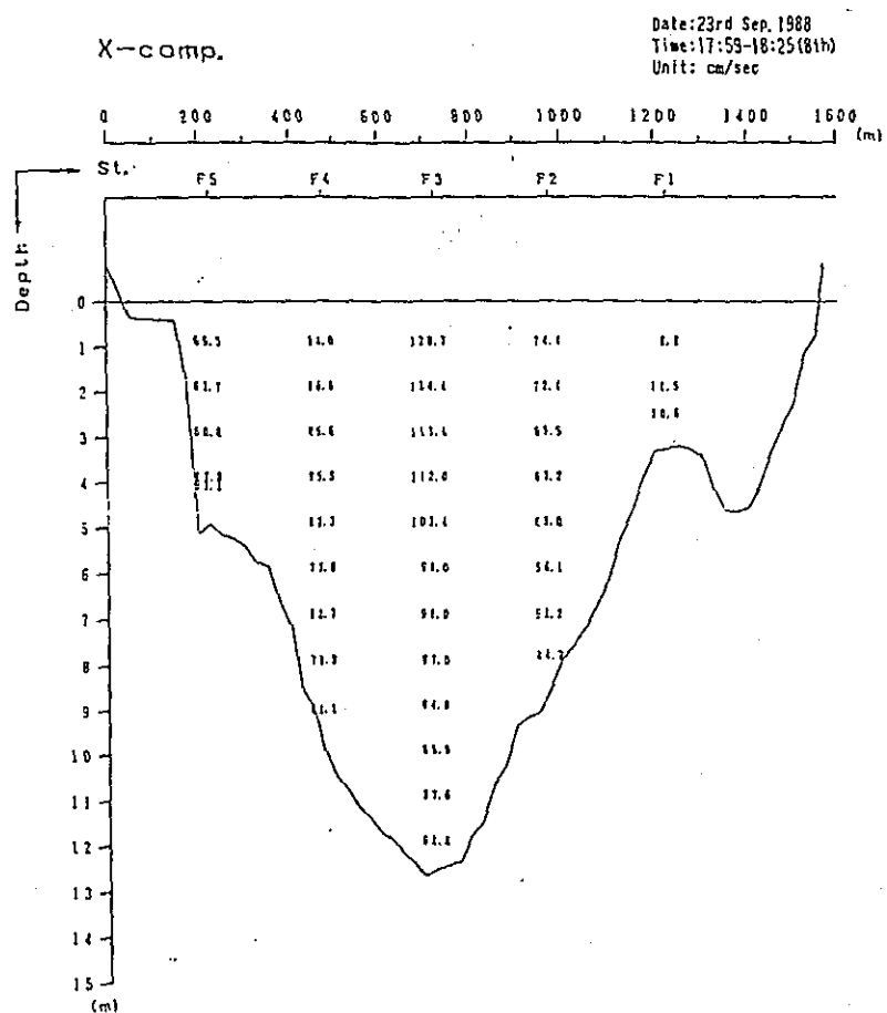
Fig. 2. 1-2(3) Profile in Distribution of Discharge Survey Results (1st Stage)
