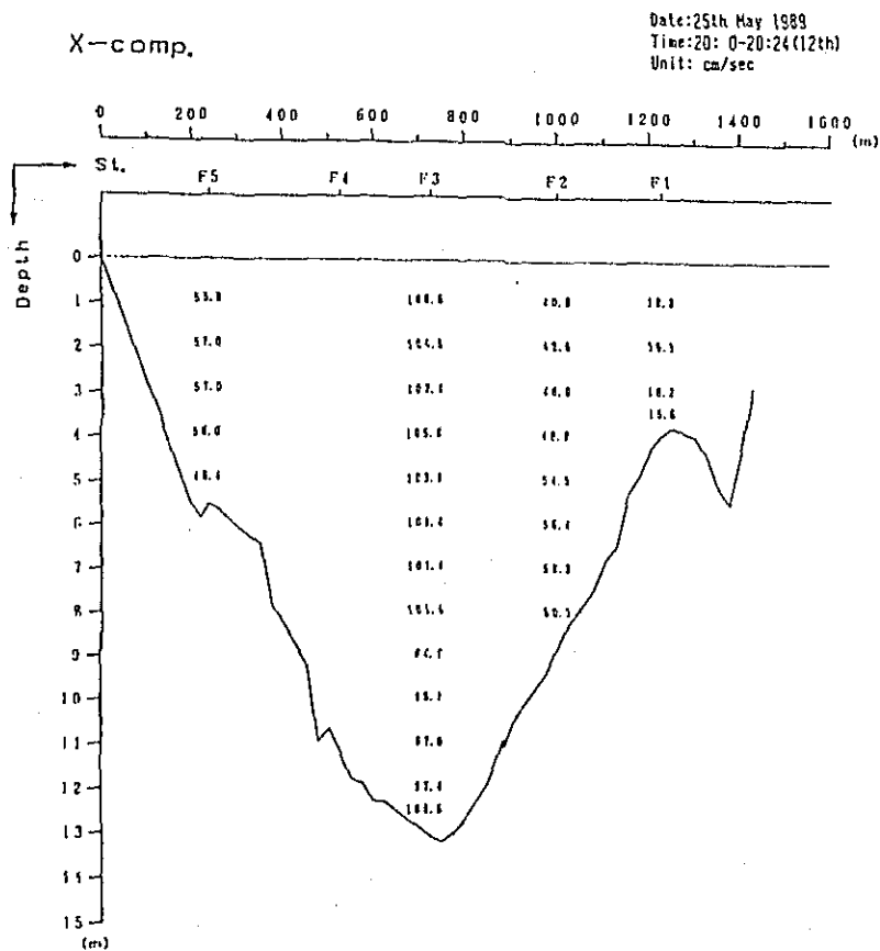
Fig. 2. 1-2(187) Profile in Distribution of Discharge Survey Results (8th Stage)
