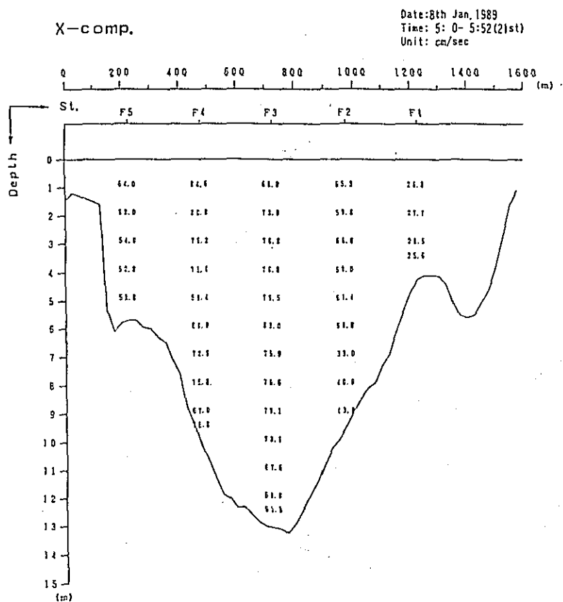
Fig. 2. 1-200 Profile in Distribution of Discharge Survey Results (4th Stage)
