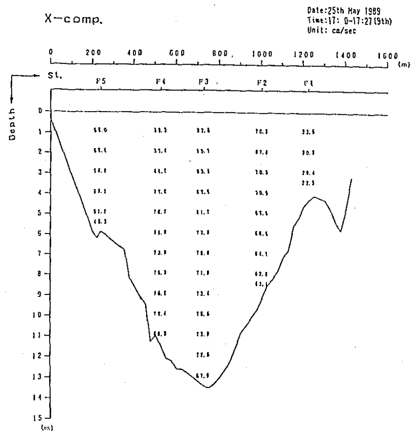
Fig. 2. 1-2(124) Profile in Distribution of Discharge Survey Results (8th Stage)
