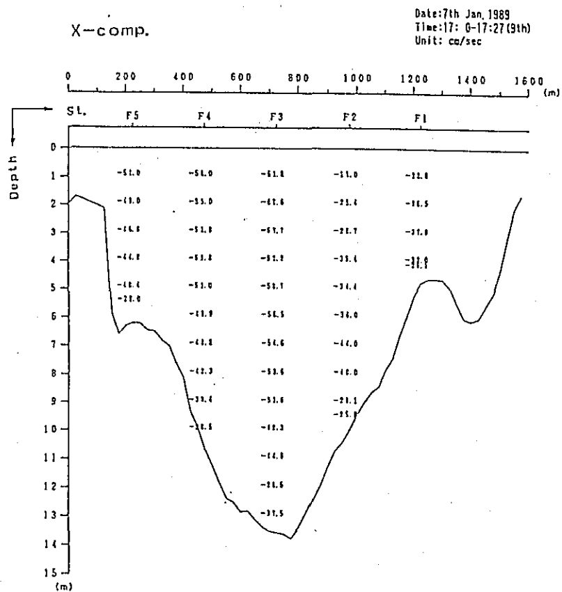
Fig. 2. 1-2(84) Profile in Distribution of Discharge Survey Results (4th Stage)
