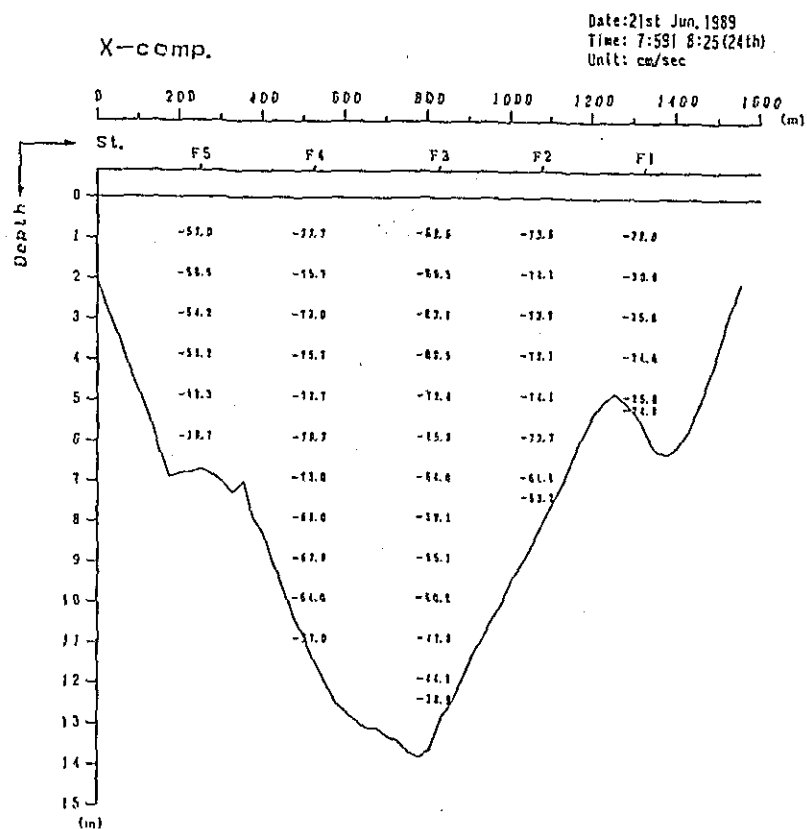
Fig. 2. 1-2(24) Profile in Distribution of Discharge Survey Results (9th Stage)
