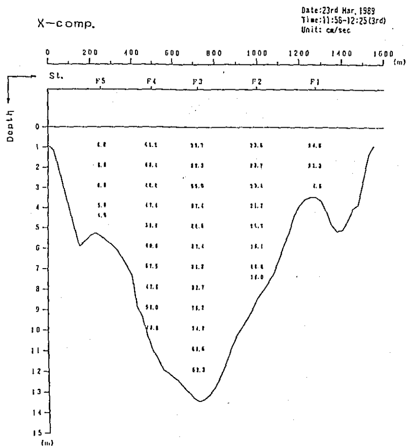
Fig. 2. 1-2(128) Profile in Distribution of Discharge Survey Results
