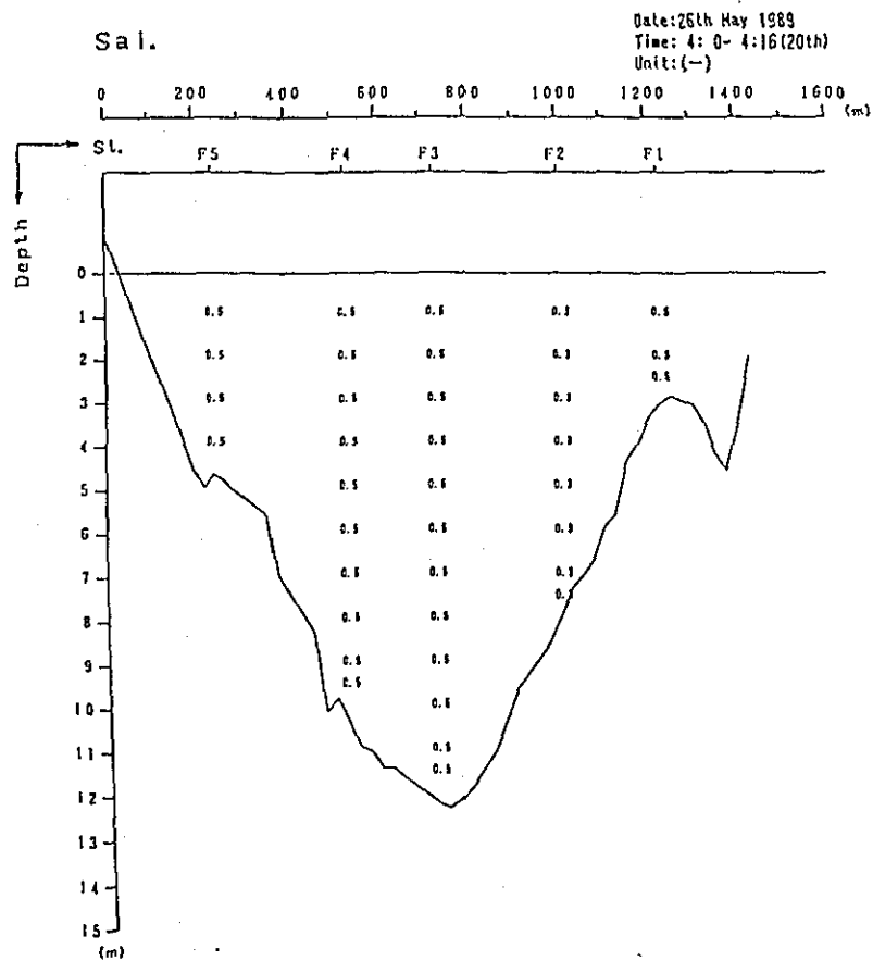
Fig. 2. 1-1(195) Profile in Distribution of Discharge Survey Results (8th Stage)
