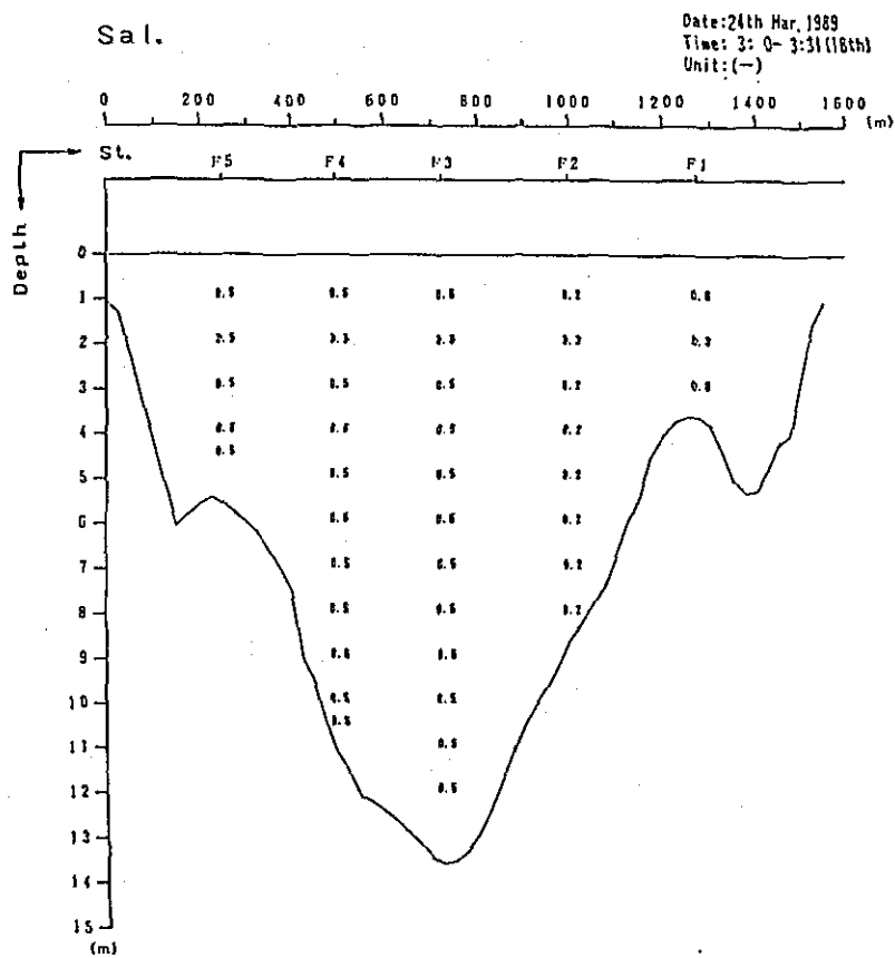
Fig. 2. 1-1(143) Profile in Distribution of Discharge Survey Results (6th Stage)
