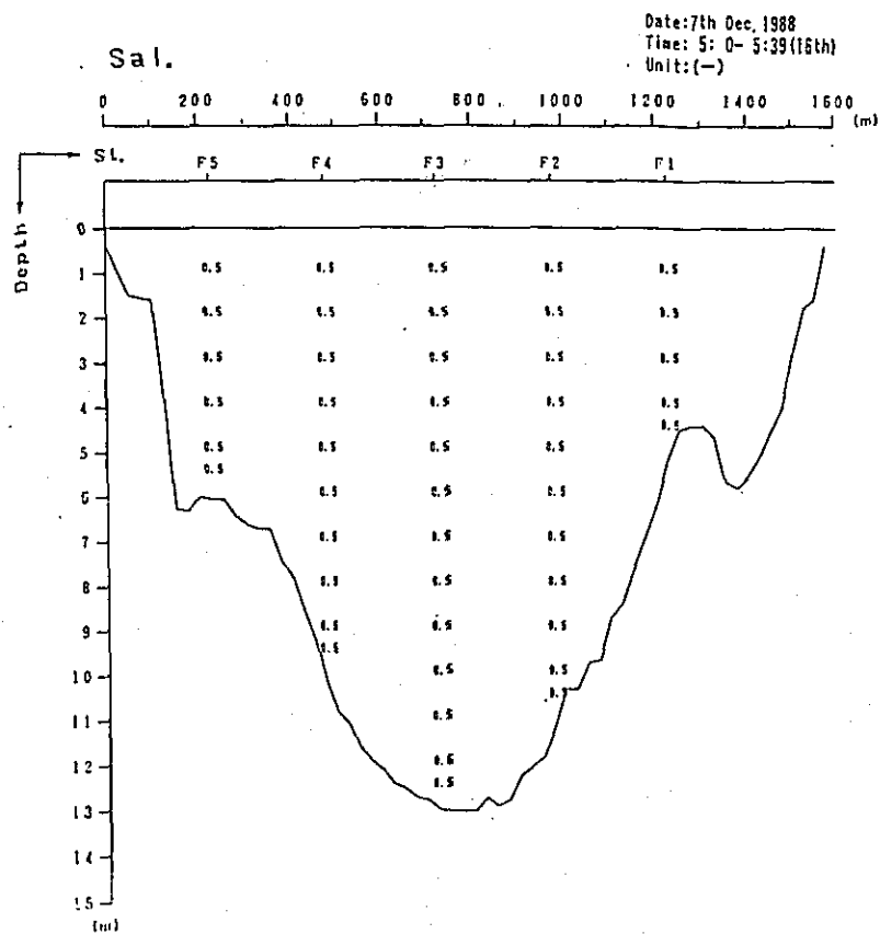
Fig. 2. 1-1(66) Profile in Distribution of Discharge Survey Results (3rd Stage)
