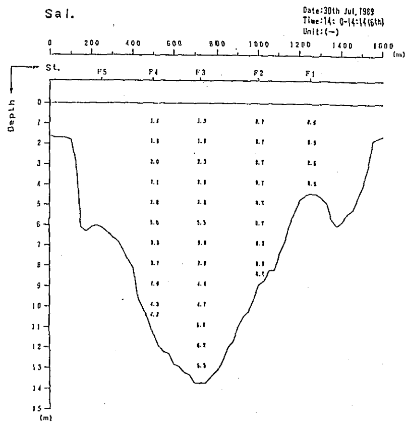
Fig. 2. 1-1(256) Profile in Distribution of Discharge Survey Results (11th Stage)
