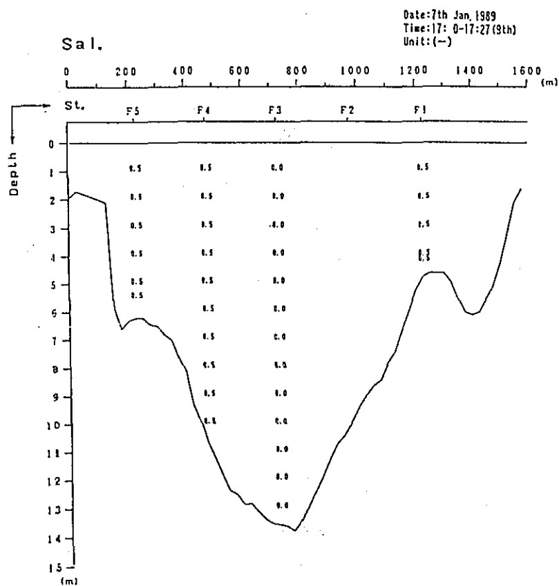
Fig. 2. 1-1(84) Profile in Distribution of Discharge Survey Results (4th Stage)
