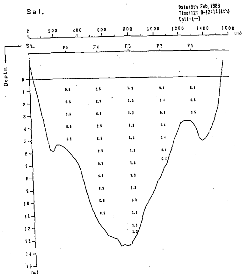
Fig. 2. 1-1(104) Profile in Distribution of Discharge Survey Results (5th Stage)
