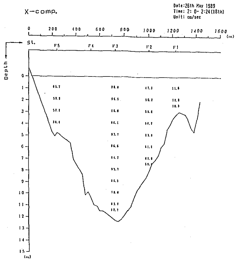
Fig. 2. 1-2(193) Profile in Distribution of Discharge Survey Results (3th Stage)
