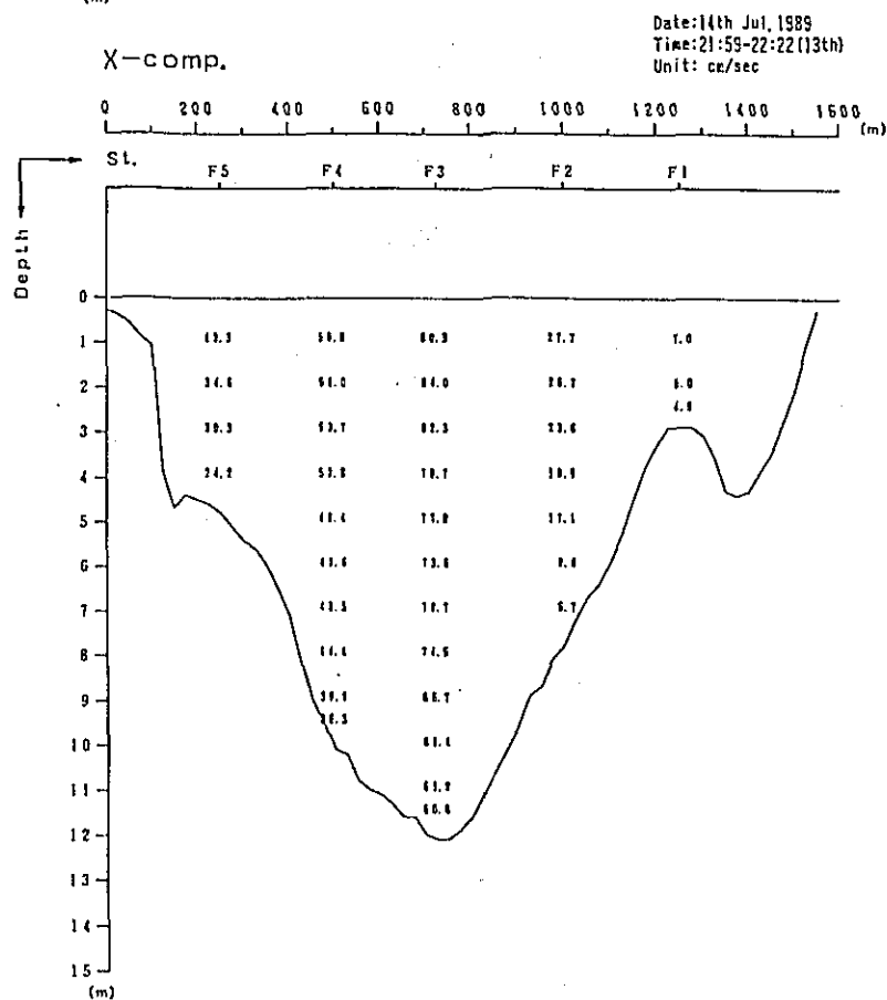
Fig. 2. 1-2(233) Profile in Distribution of Discharge Survey Results (10th Stage)
