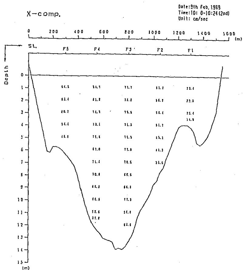
Fig. 2. 1-2002 Profile in Distribution of Discharge Survey Results (5th Stage)
