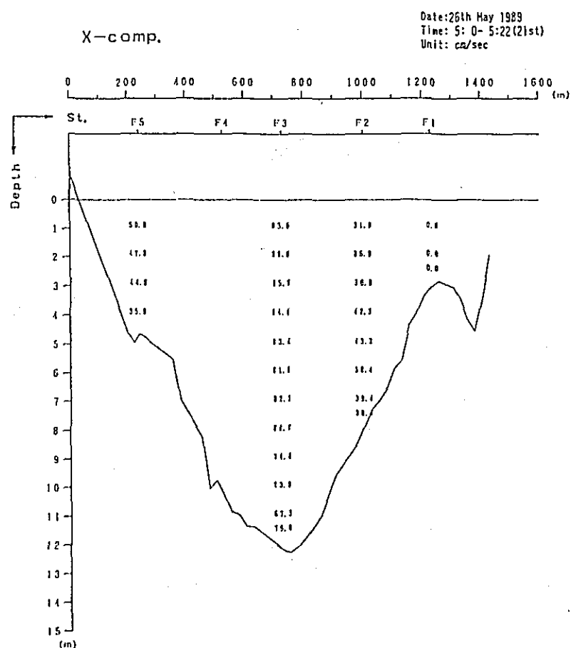
Fig. 2. 1-2(95) Profile in Distribution of Discharge Survey Results
