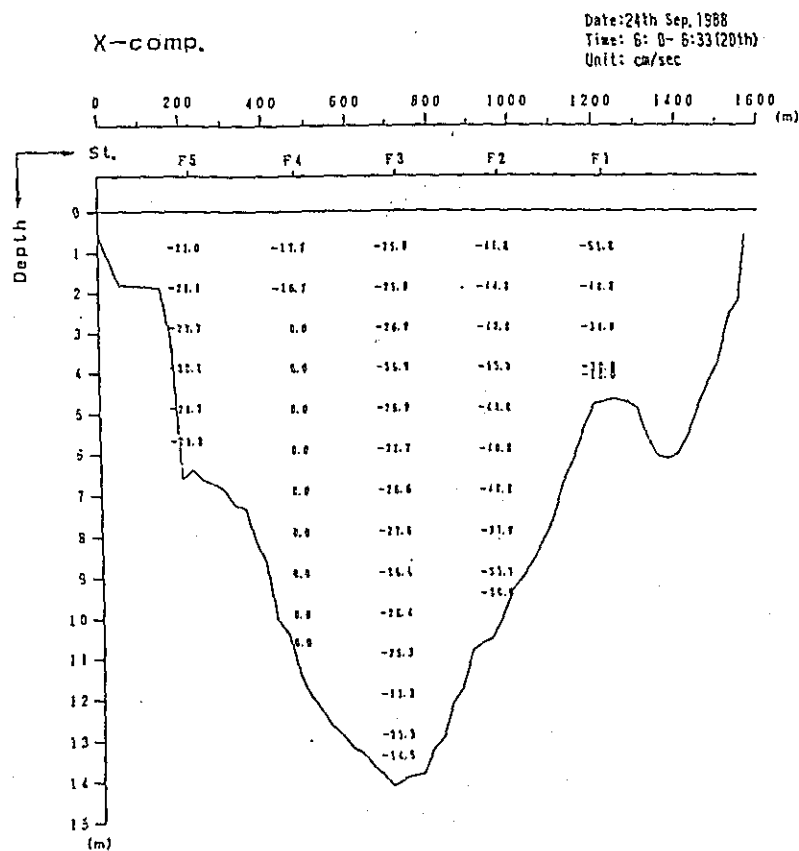
Fig. 2. 1-2(20) Profile in Distribution of Discharge Survey Results (1st Stage)
