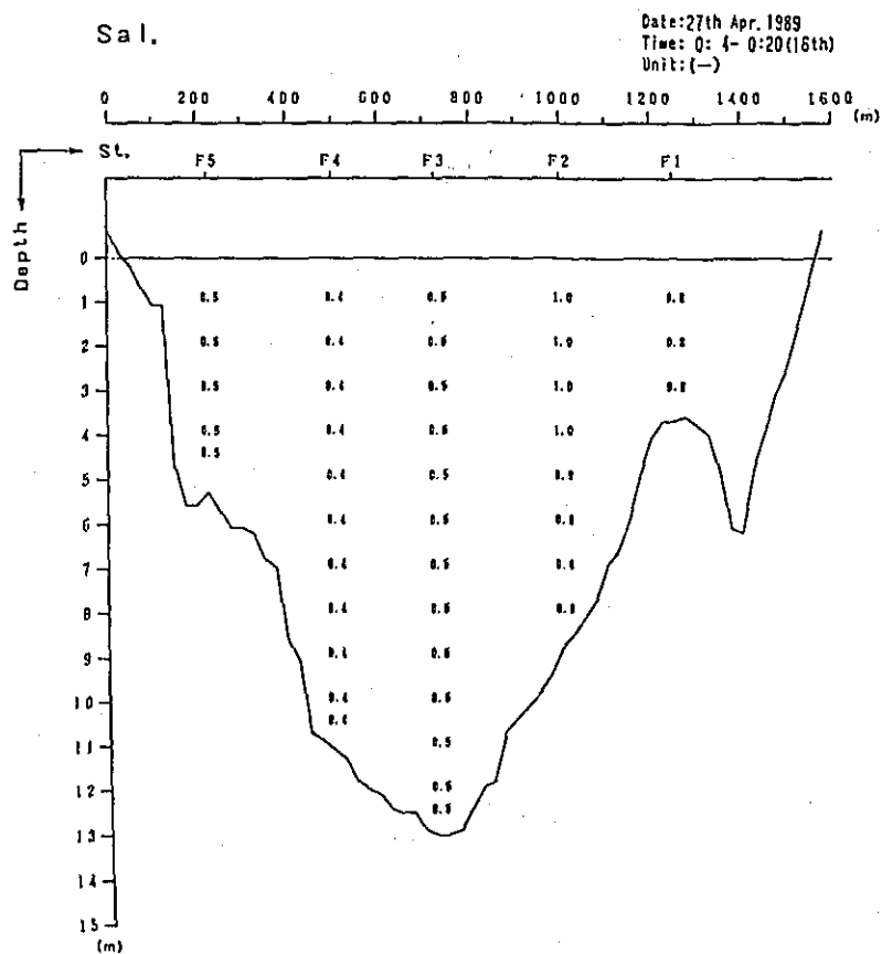
Fig. 2. 1-1(166) Profile in Distribution of Discharge Survey Results (7th Stage)
