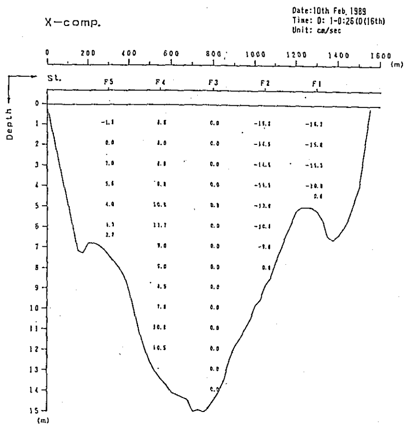
Fig. 2. 1-2(116) Profile in Distribution of Discharge Survey Results
