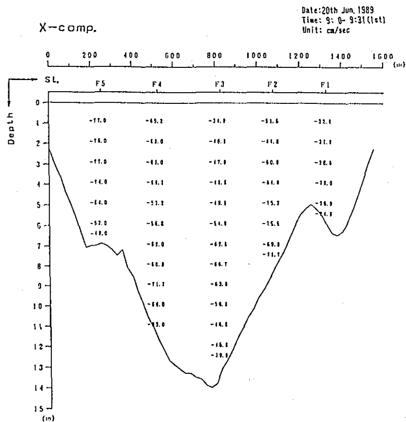
Fig. 2. 1-2(20) Profile in Distribution of Discharge Survey Results (9th Stage)
