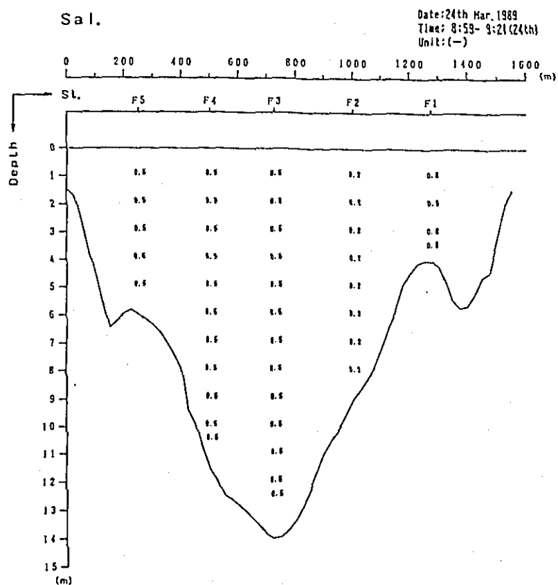
Fig. 2. 1-1(149) Profile in Distribution of Discharge Survey Results (6th Stage)
