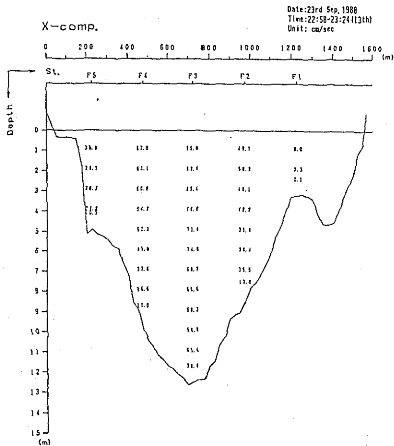
Fig. 2. 1-2(13) Profile in Distribution of Discharge: Survey Results (1st Stage)
