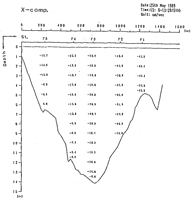
Fig. 2. 1-2(130) Profile in Distribution of Discharge Survey Results
