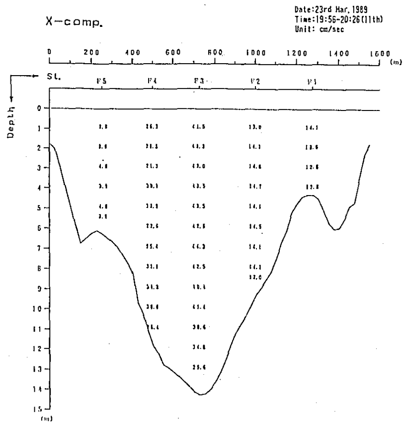
Fig. 2. 1-2(13) Profile in Distribution of Discharge Survey Results (6th Stage)
