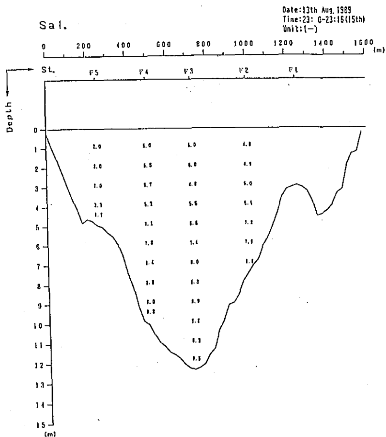
Fig. 2. 1-1(230) Profile in Distribution of Discharge Survey Results (2th Stage)
