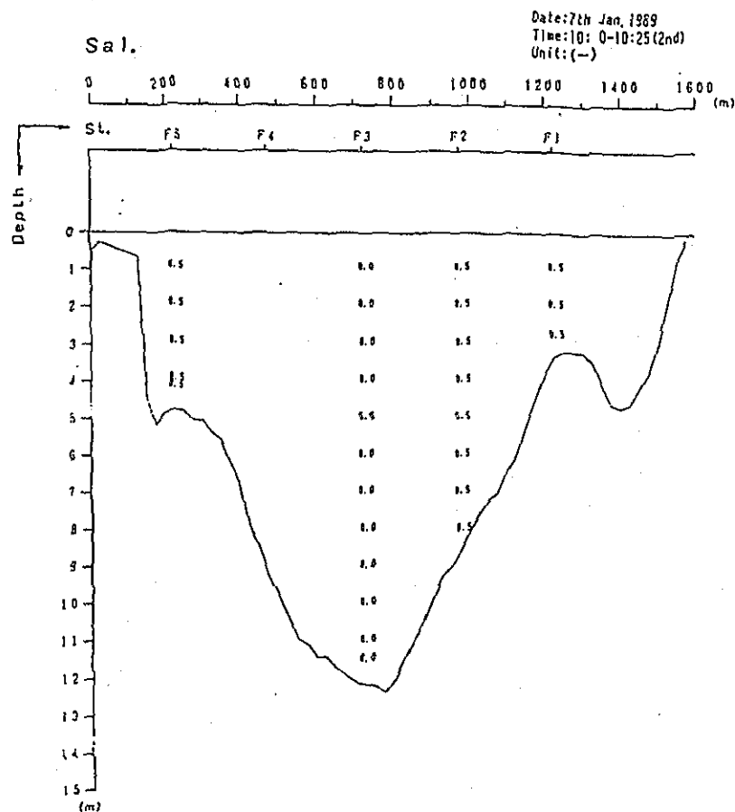
Fig. 2. 1-177 Profile in Distribution of Discharge Survey Results (4th Stage)
