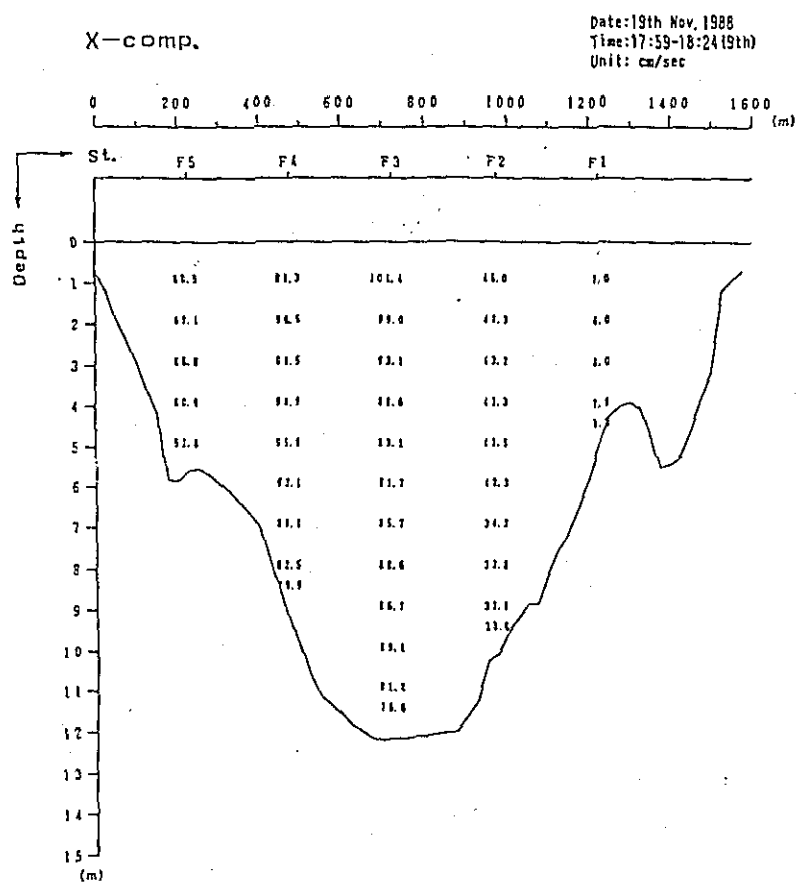
Fig. 2. 1-2(3) Profile in Distribution of Discharge Survey Results (2nd Stage)
