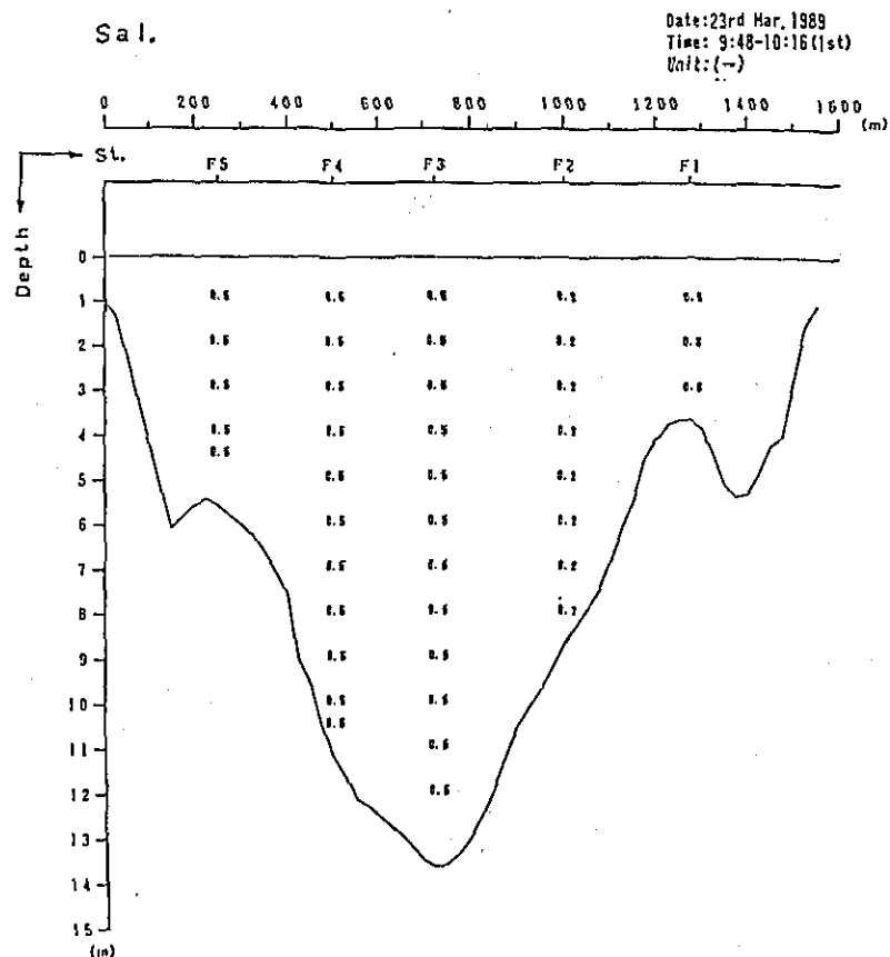
Fig. 2. 1-1(126) Profile in Distribution of Discharge Survey Results (6th Stage)
