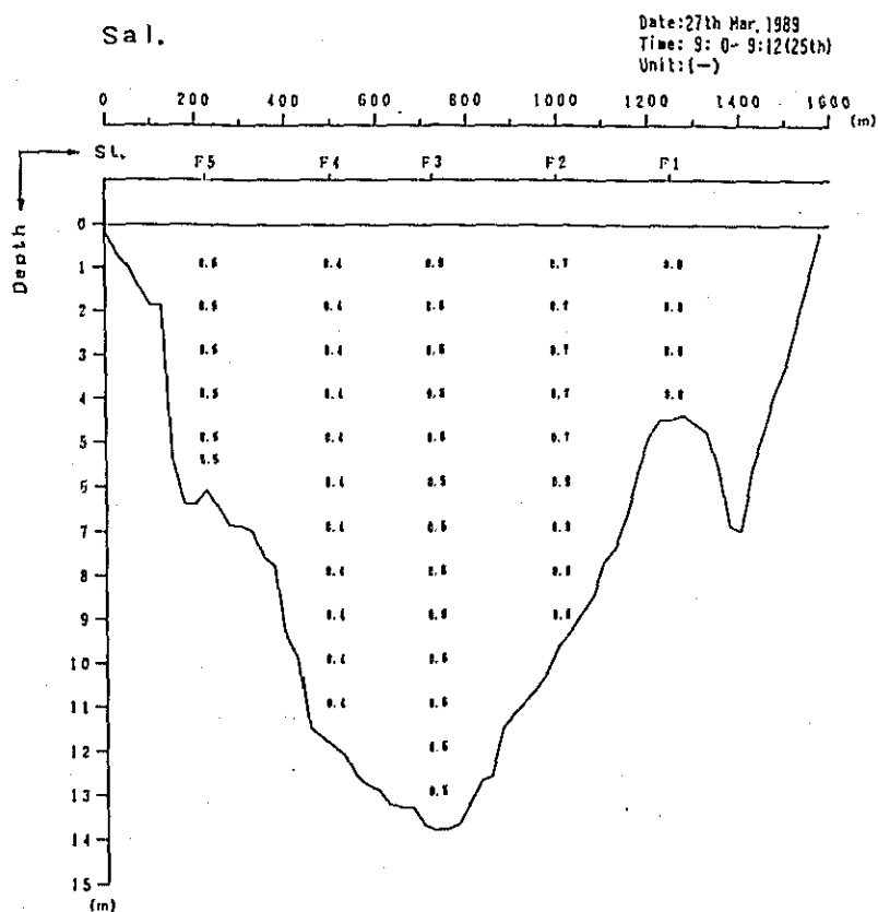
Fig. 2. 1-1(175) Profile in Distribution of Discharge Survey Results (7th Stage)
