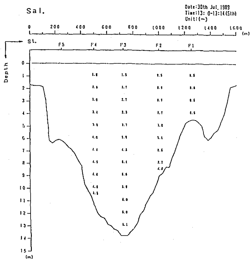
Fig. 2. 1-1(255) Profile in Distribution of Discharge Survey Results (11th Stage)
