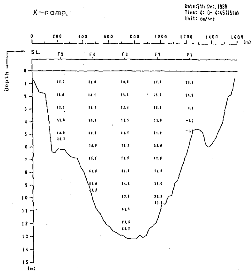
Fig. 2. 1-2(55) Profile in Distribution of Discharge Survey Results (3rd Stage)
