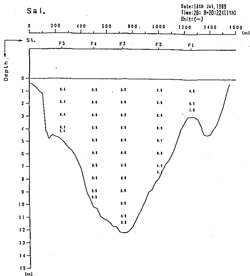
Fig. 2. 1-1(235) Profile in Distribution of Discharge Survey Results (00th Stage)
