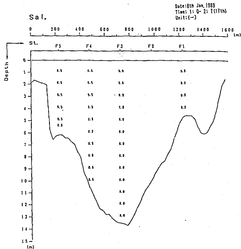
Fig. 2. 1-1(2) Profile in Distribution of Discharge Survey Results (4th Stage)
