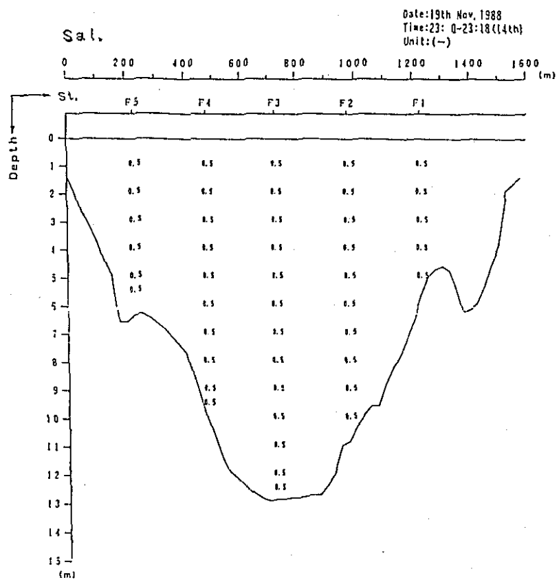
Fig. 2. 1-1(39) Profile in Distribution of Discharge Survey Results (2nd Stage)
