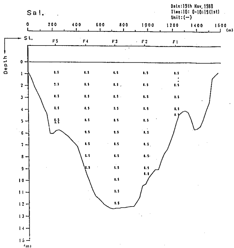
Fig. 2. 1-1(26) Profile in Distribution of Discharge Survey Results (2nd Stage)
