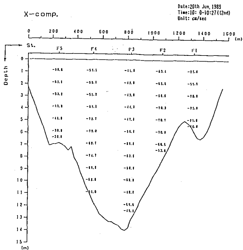
Fig. 2. 1-2002 Profile in Distribution of Discharge Survey Results (9th Stage)
