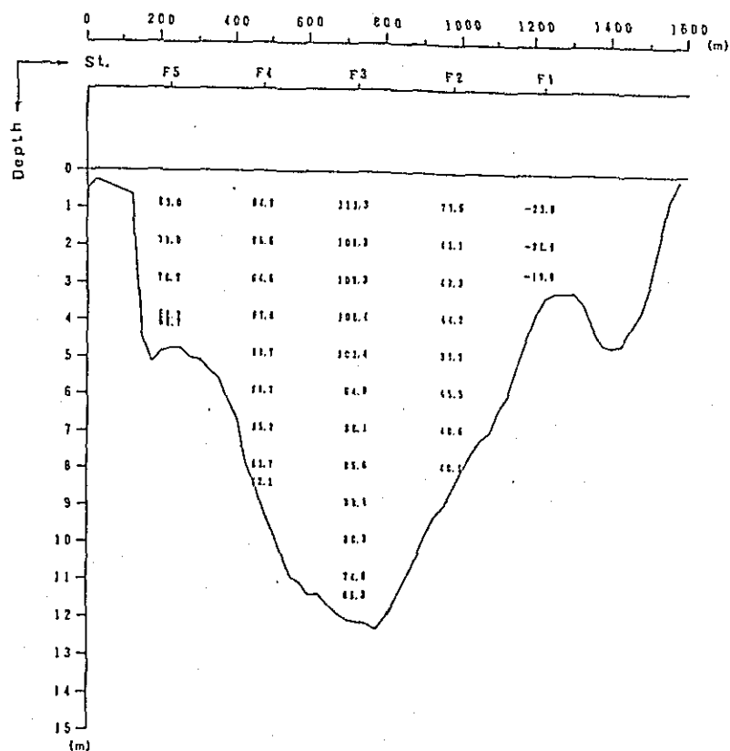
Fig. 2. 1-2(77) Profile in Distribution of Discharge Survey Results
