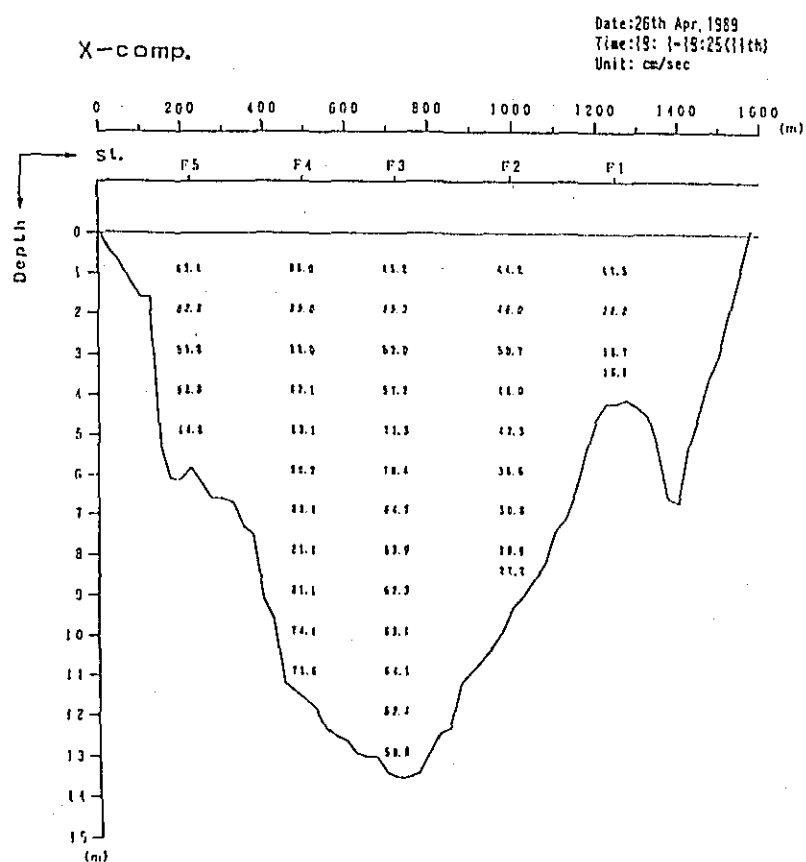
Fig. 2. 1-2(16) Profile in Distribution of Discharge Survey Results (7th Stage)
