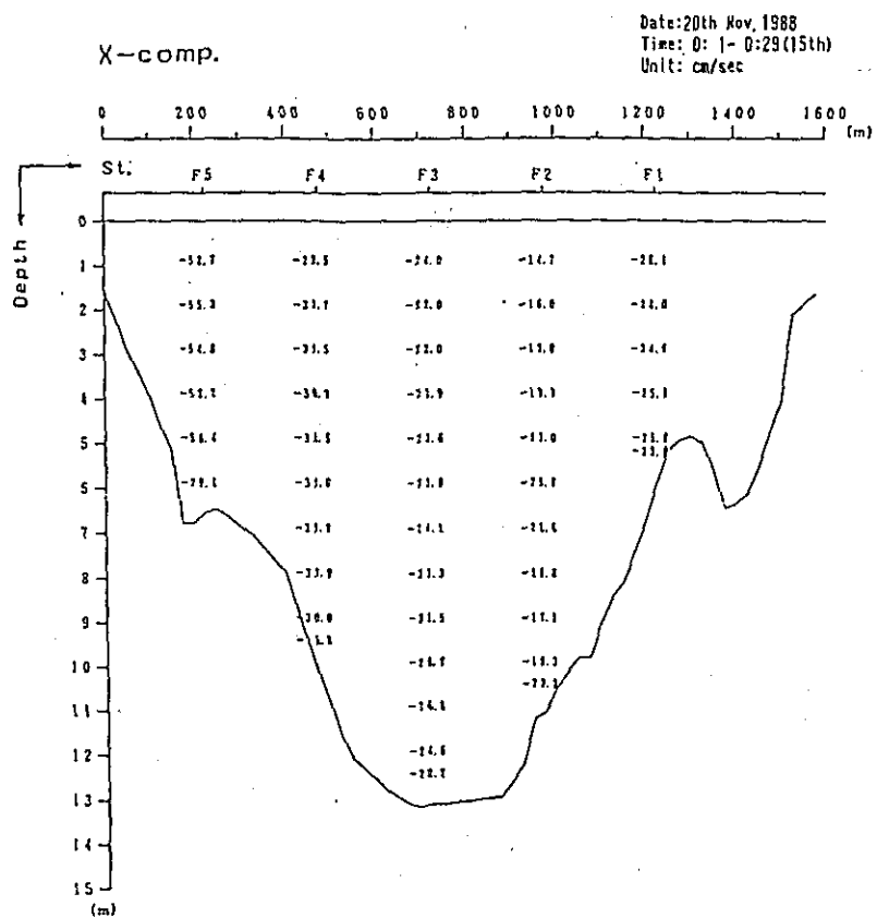
Fig. 2. 1-2(40) Profile in Distribution of Discharge Survey Results (2nd Stage)
