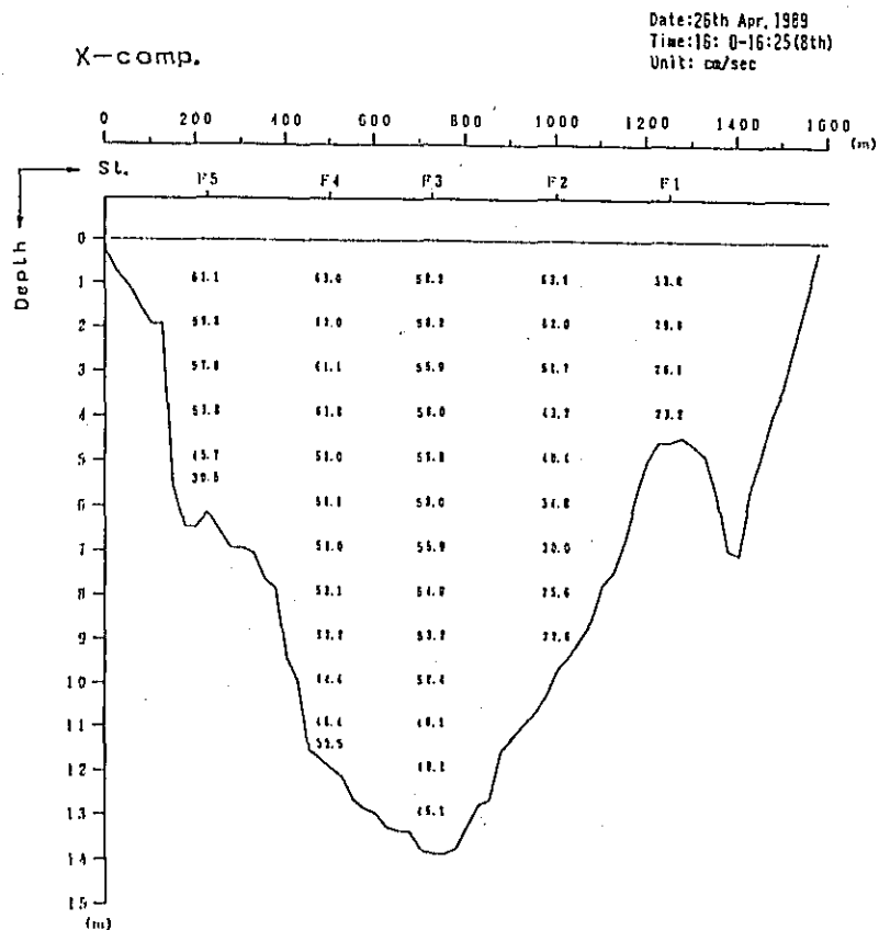
Fig. 2. 1-2(153) Profile in Distribution of Discharge Survey Results (7th Stage).
