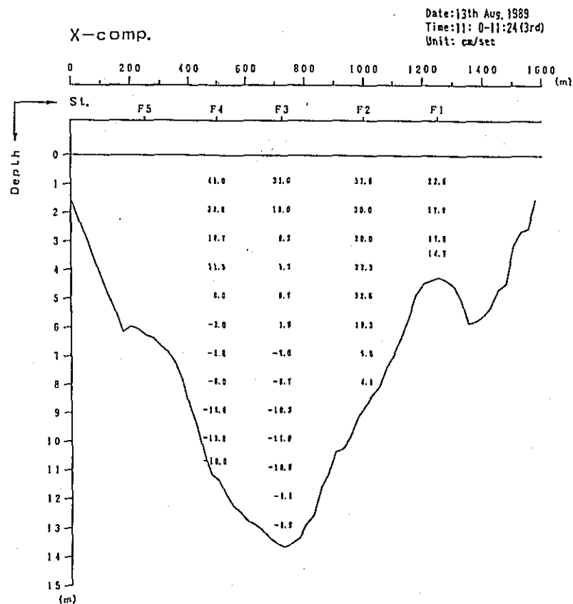
Fig. 2. 1-2(278) Profile in Distribution of Discharge Survey Results (2th Stage)
