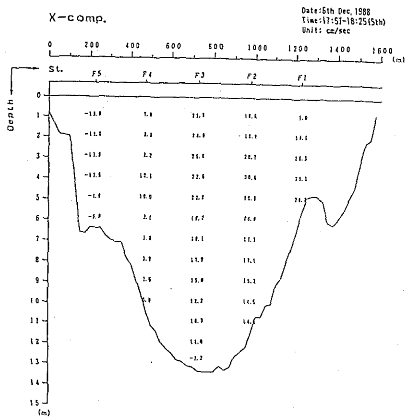
Fig. 2. 1-2(55) Profile in Distribution of Discharge Survey Results (3rd Stage)
