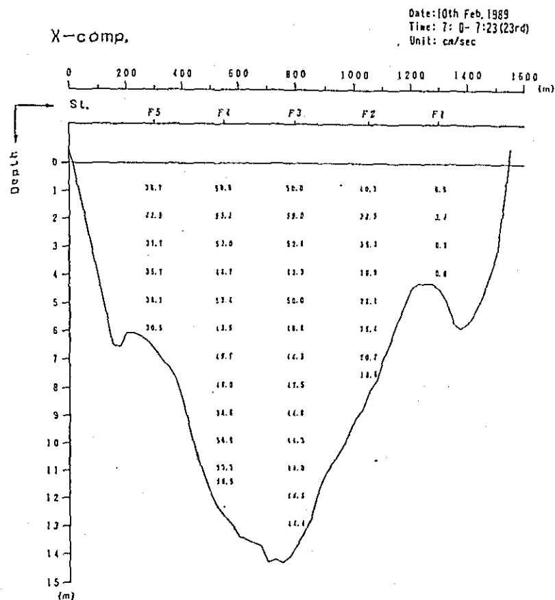
Fig. 2. 1-2(23) Profile in Distribution of Discharge Survey Results (5th Stage)
