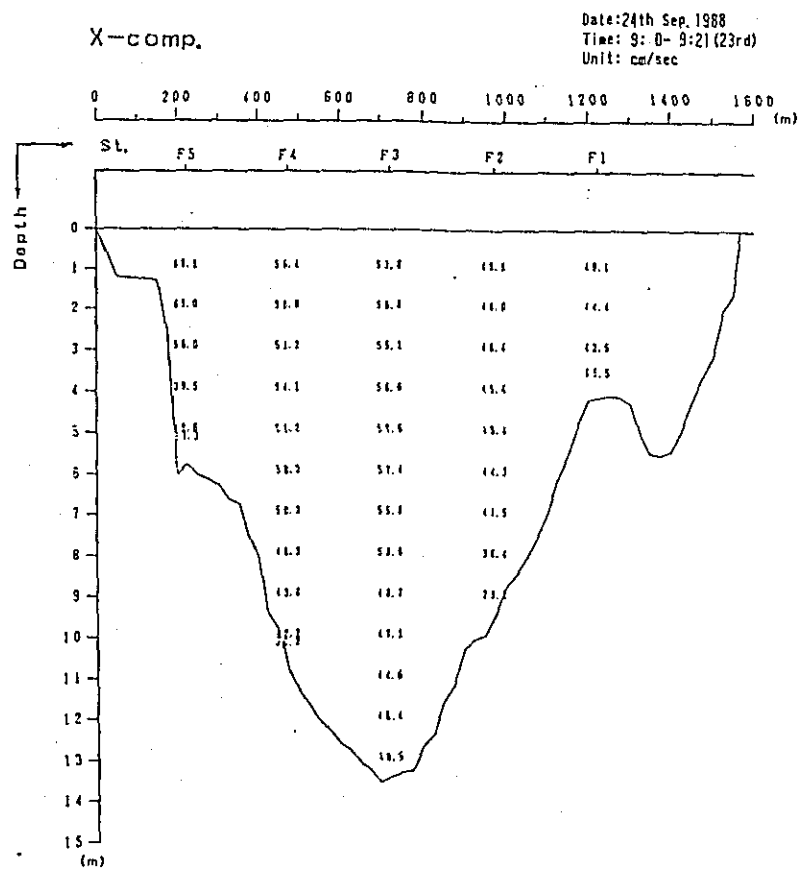
Fig. 2. 1-2(3) Profile in Distribution of Discharge Survey Results (1st Stage)
