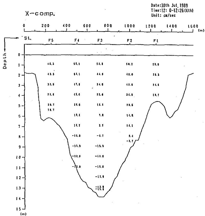
Fig. 2. 1-2(54) Profile in Distribution of Discharge Survey Results (11th Stage)
