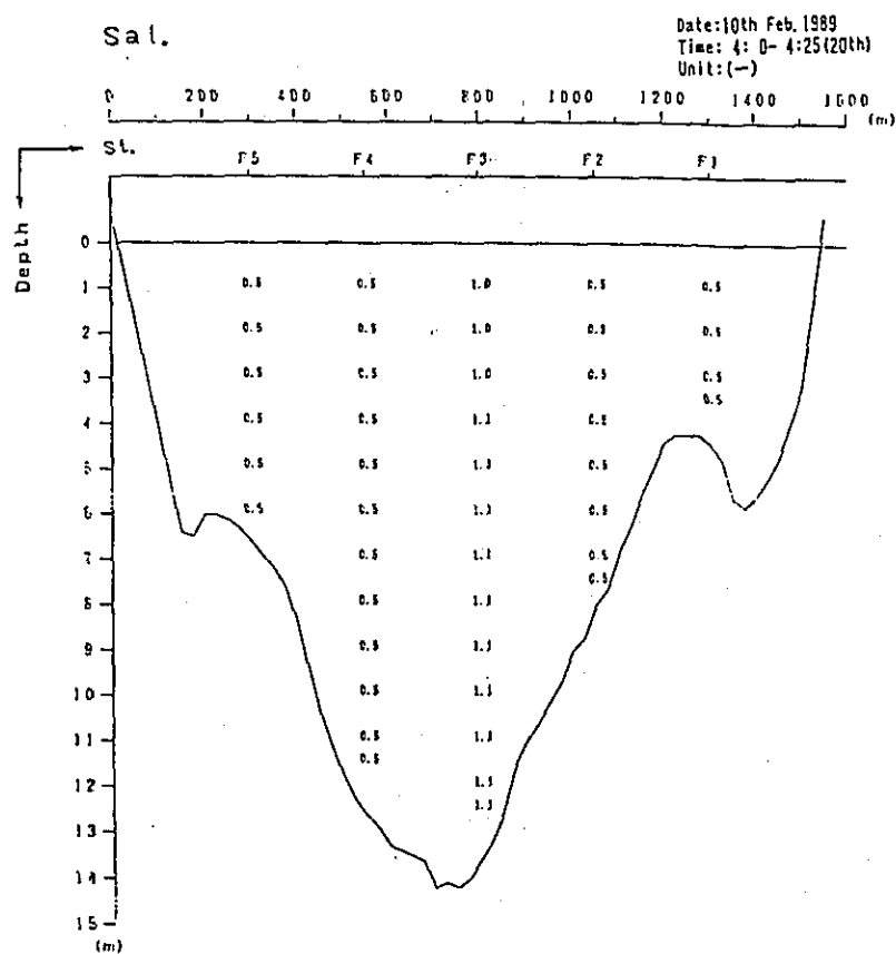
Fig. 2. 1-1(120) Profile in Distribution of Discharge Survey Results (5th Stage)
