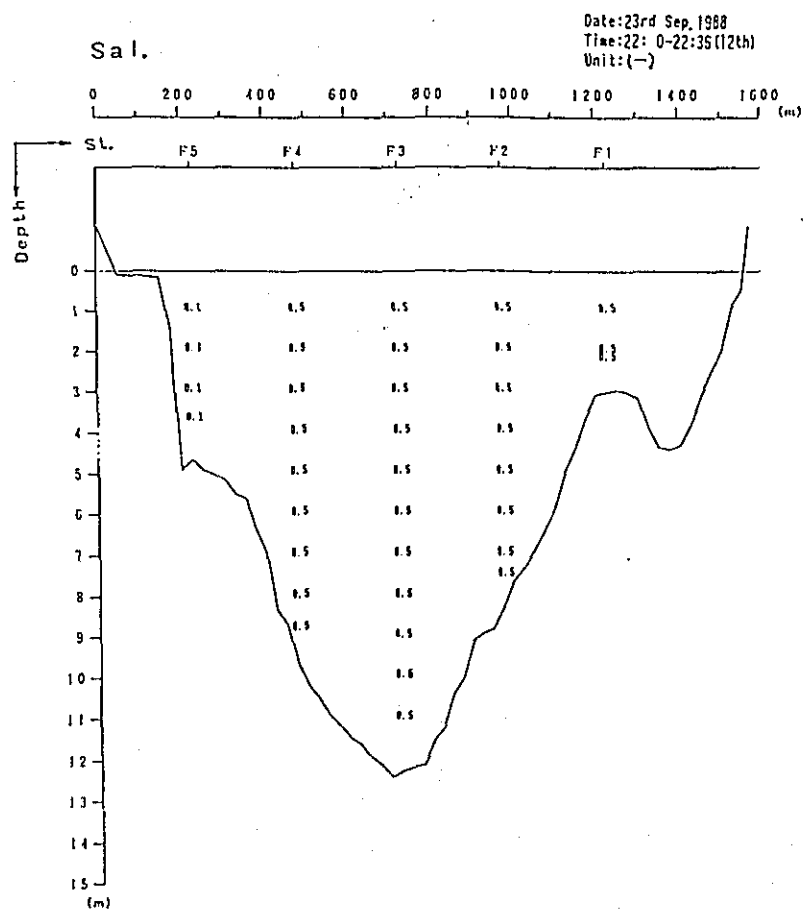
Fig. 2. 1-1(12) Profile in Distribution of Discharge Survey Results (1st Stage)
