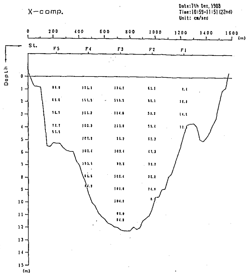
Fig. 2. 1-2(72) Profile in Distribution of Discharge Survey Results (3rd Stage)
