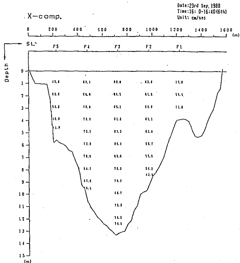
Fig. 2. 1-2(6) Profile in Distribution of Discharge Survey Results (1st Stage)
