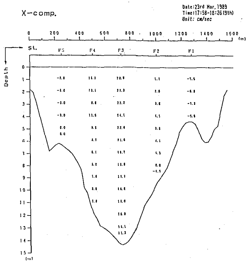
Fig. 2. 1-2(134) Profile in Distribution of Discharge Survey Results (6th Stage)
