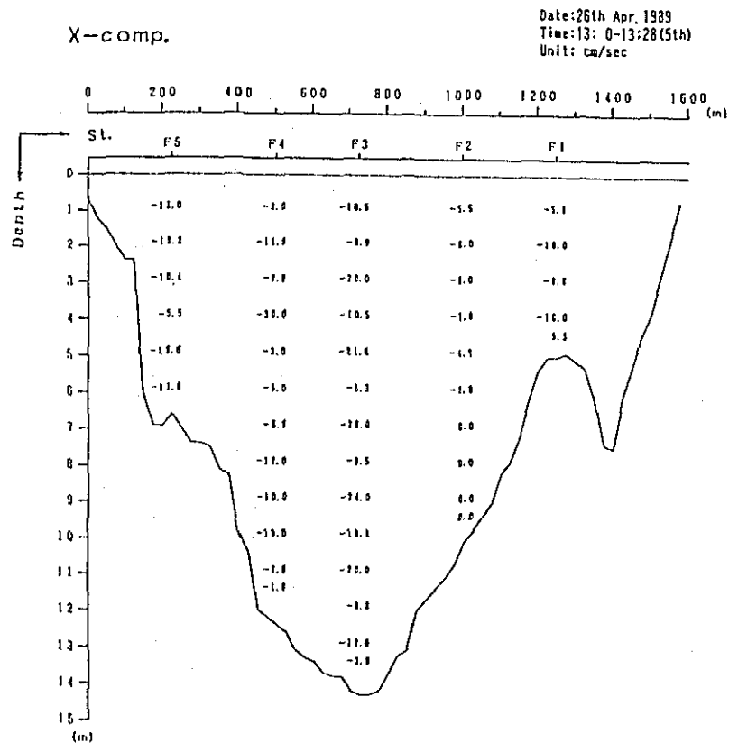
Fig. 2. 1-2(155) Profile in Distribution of Discharge Survey Results (7th Stage)
