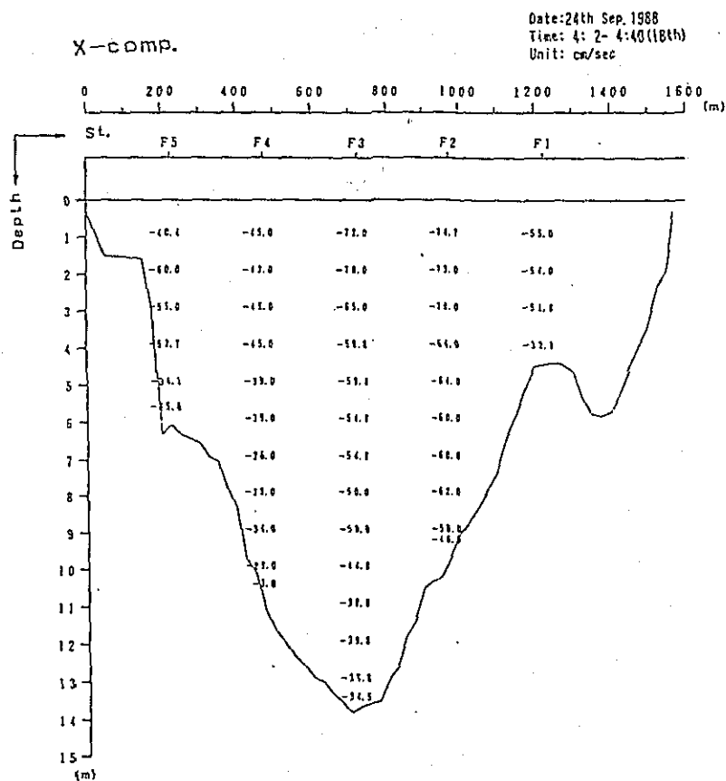
Fig. 2. 1-2(18) Profile in Distribution of Discharge Survey Results (1st Stage)
