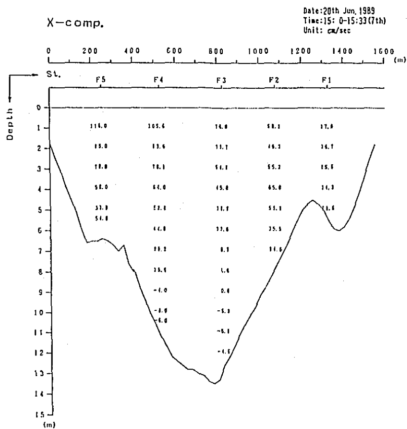
Fig. 2. 1-2(207) Profile in Distribution of Discharge Survey Results (9th Stage)
