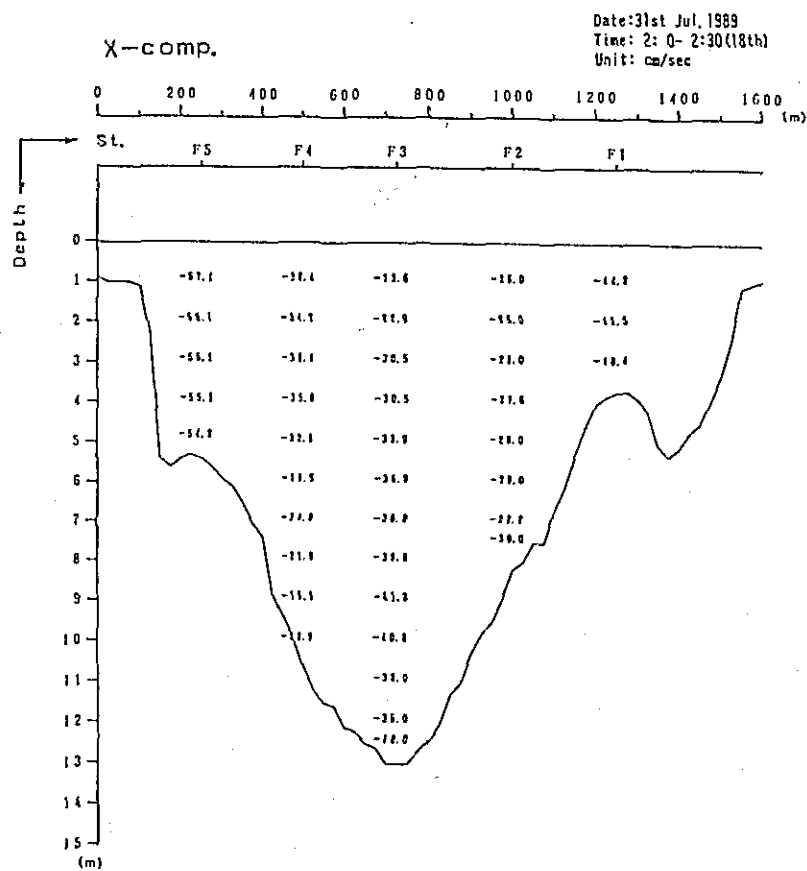
Fig. 2. 1-2(263) Profile in Distribution of Discharge Survey Results (11th Stage)
