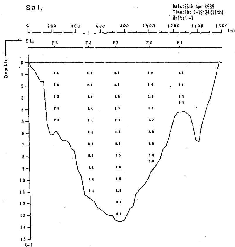
Fig. 2. 1-1(16) Profile in Distribution of Discharge Survey Results (7th Stage)
