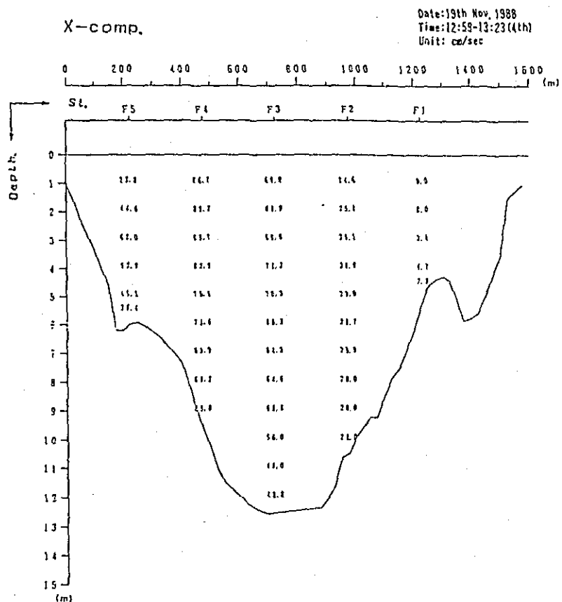
Fig. 2. 1-2(2) Profile in Distribution of Discharge Survey Results (2nd Stage)
