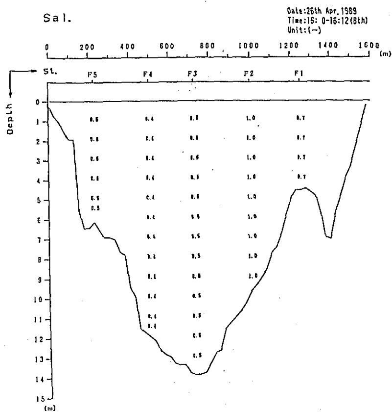
Fig. 2. 1-1(158) Profile in Distribution of Discharge Survey Results (7th Stage)
