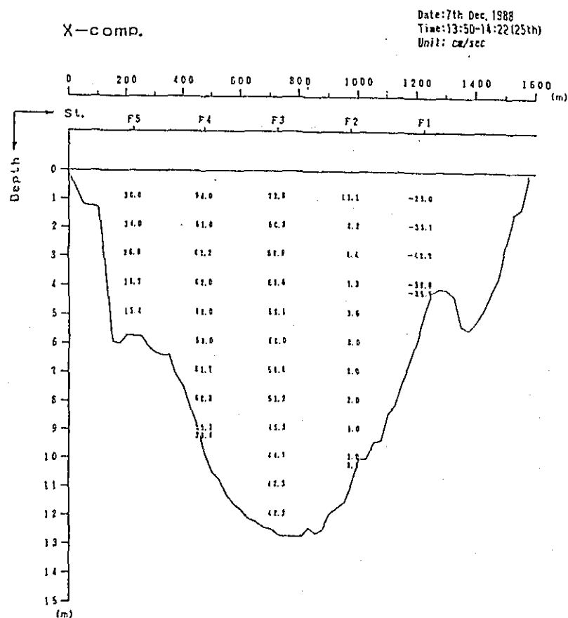
Fig. 2. 1-2(7) Profile in Distribution of Discharge Survey Results (3rd Stage)
