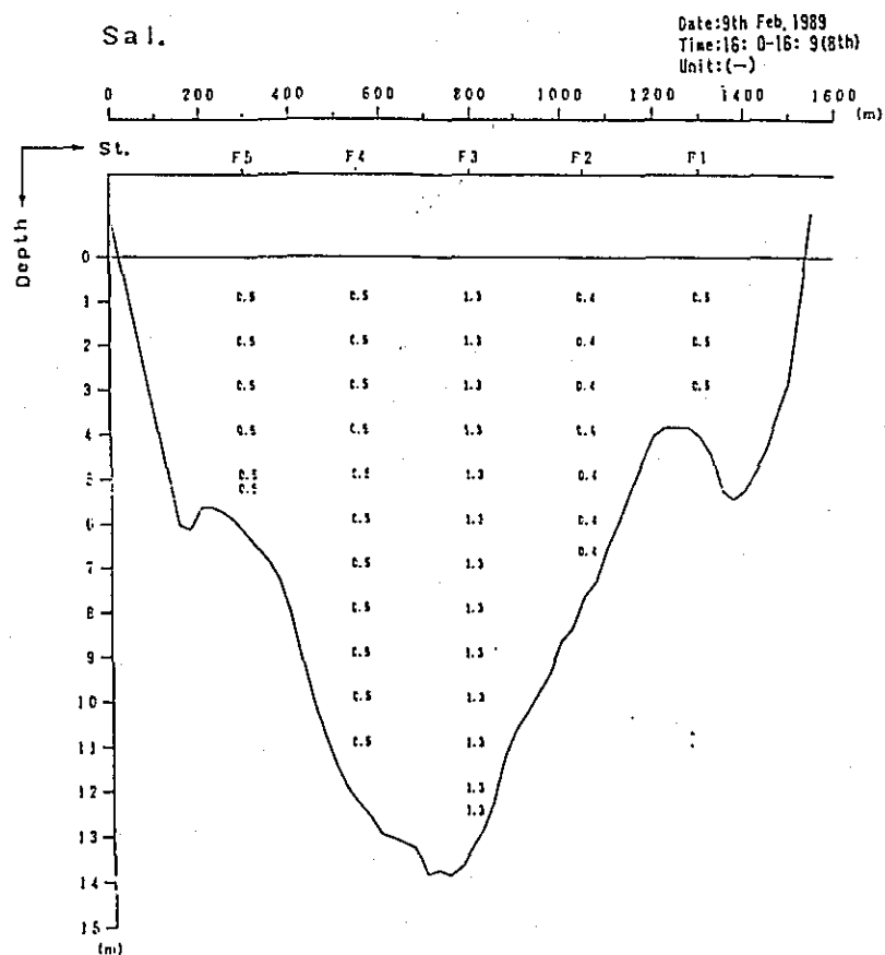
Fig. 2. 1-1(108) Profile in Distribution of Discharge Survey Results (5th Stage)
