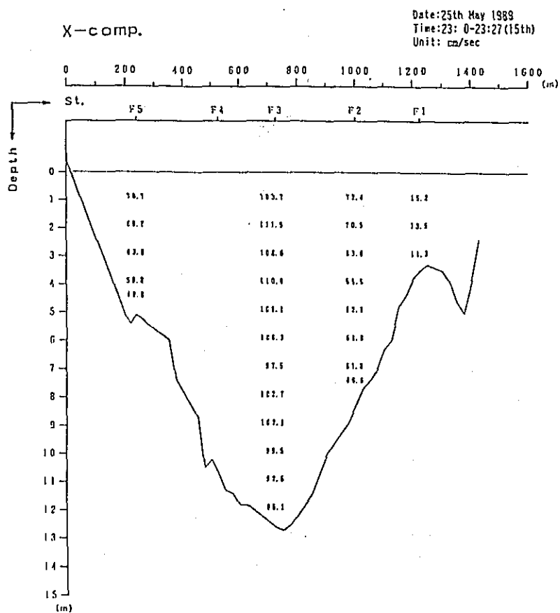
Fig. 2. 1-2(190) Profile in Distribution of Discharge Survey Results (8th Stage)
