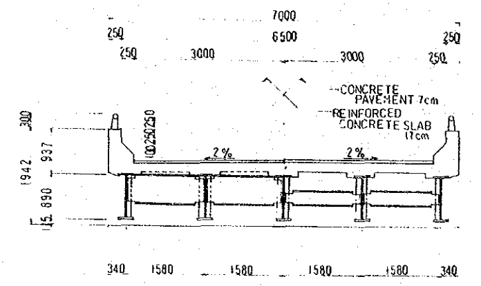
SUPERSTRUCTURE CROSS SECTION SCALE 1:50
