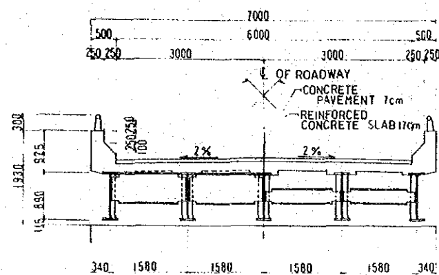
SUPERSTRUCTURE CROSS SECTION SCALE 1:50
