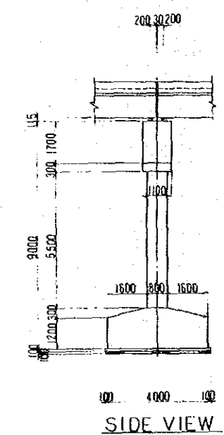
PIER (P1) SCALE 1:100
