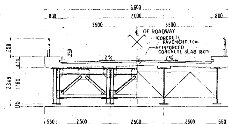
SUPERSTRUCTURE CROSS SECTION SCALE 1:50
