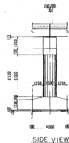
PIER (P1) SCALE 1:100
