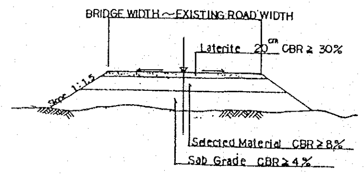
CROSS SECTION OF APPROACH
