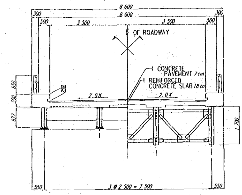
SUPERSTRUCTURE CROSS SECTION SCALE 1 : 50
