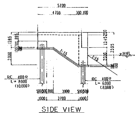
ABOUT MENT (A12) SCALE 1:100
