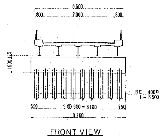
PIER (P1) SCALE 1:100
