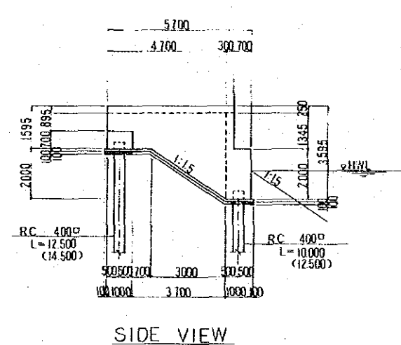
ABOUT MENT (A12) SCAEL 1:100
