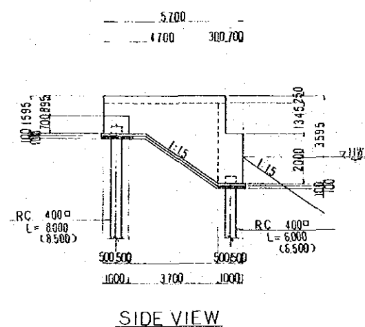
ABOUT MENT (A12) SCALE 1:100
