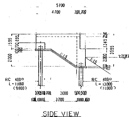
ABOUT MENT (A12) SCALE: 1:100
