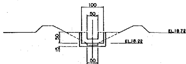
Outlet of drainage
