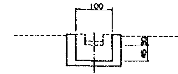
C - C Section
