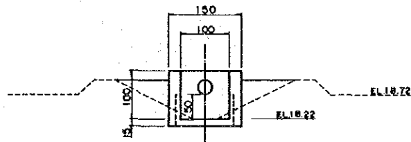
D - D Section
