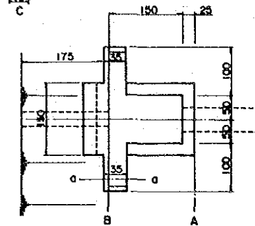
B - B Section
