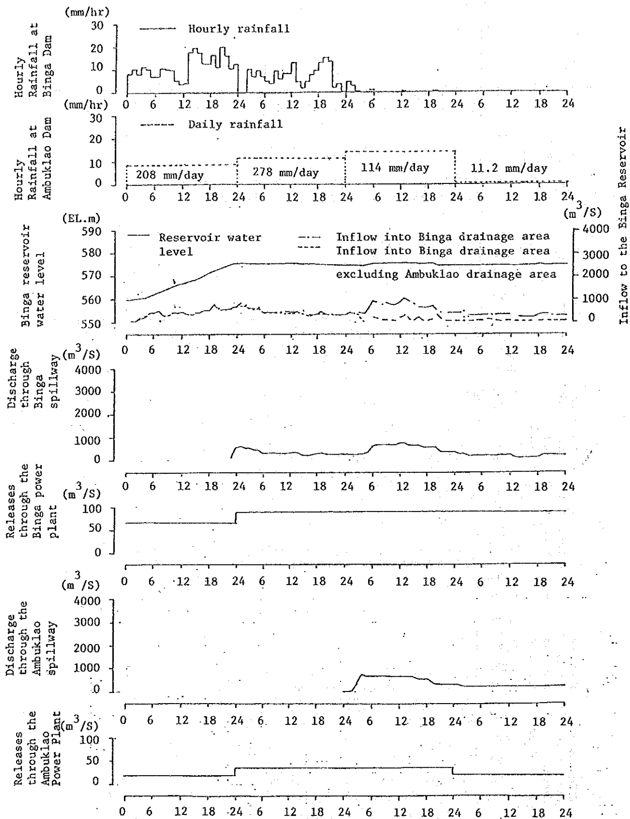
☒ - 9.10(7) Hourly Inflow to the Binga Reservoir During Typical Flood Period (July 9 - 12, 1986)
