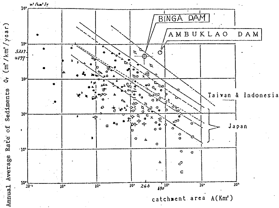
☒ - 10.8 Comparison of the Binga Sediment Yields with Those of Other River Basins
