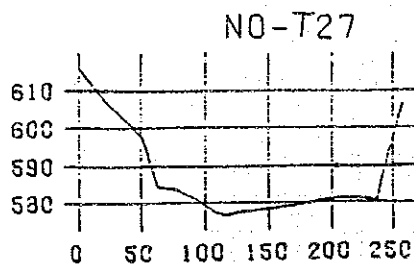
☒ - 10.19(6) Cross Sections of the Upstream Reaches of the Binga Reservoir (1987 Survey)
