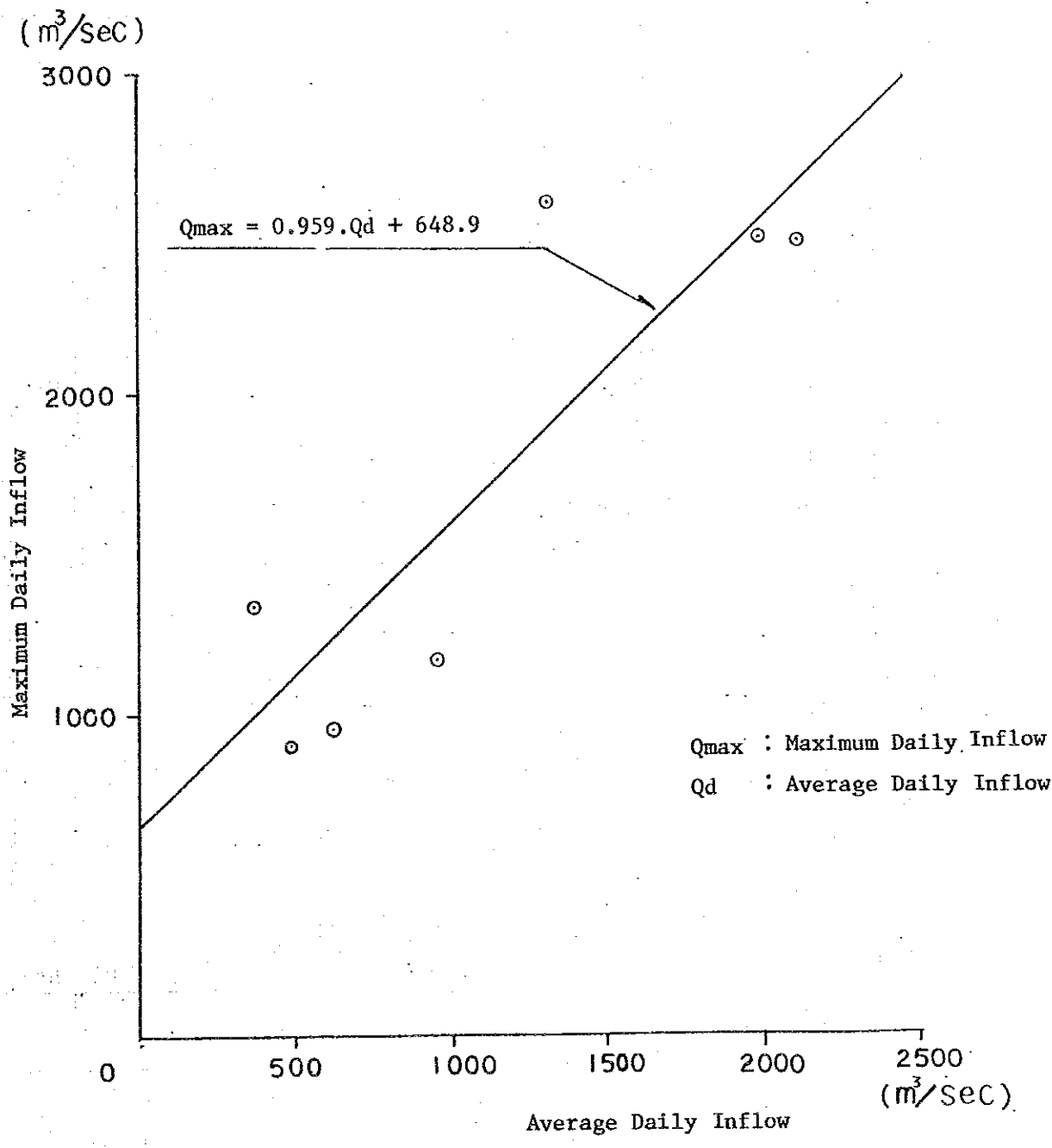
☒ - 10.10 Relation between Average Daily Inflow and Maximum Daily Inflow to the Binga Reservoir
