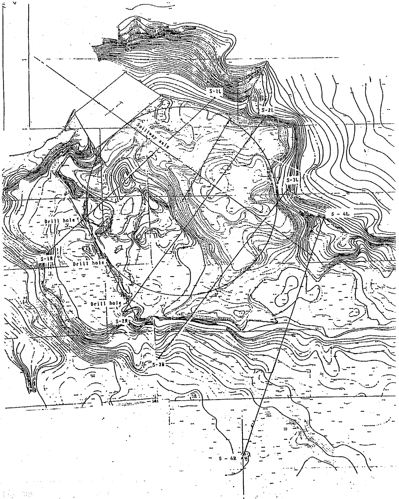
9.21 Plan of the Plunge Pool
