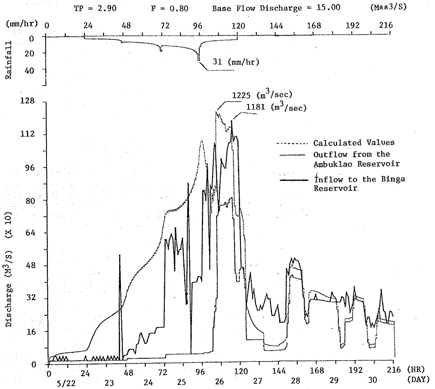
☒ - 9.11(1) Inflow to the Binga Reservoir During Typical Flood Period (May 22 - 30, 1976)
