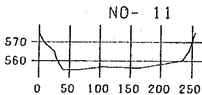
☒ - 10.2(4) Cross Sections of the Binga Reservoir (1986 Survey)
