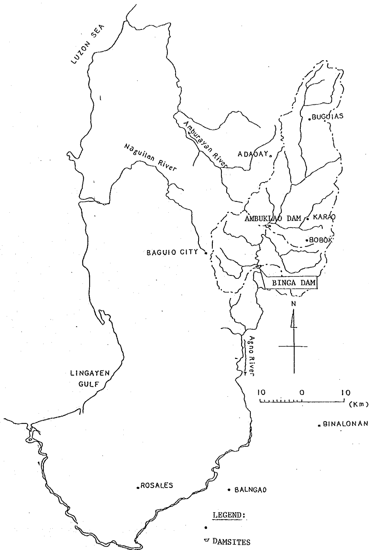
☒ - 9.3 Hydrologic Observation Stations
