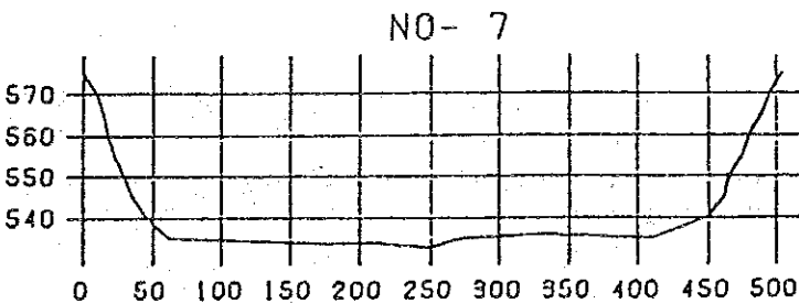
☒ - 10.2(3) Cross Sections of the Binga Reservoir (1986 Survey)
