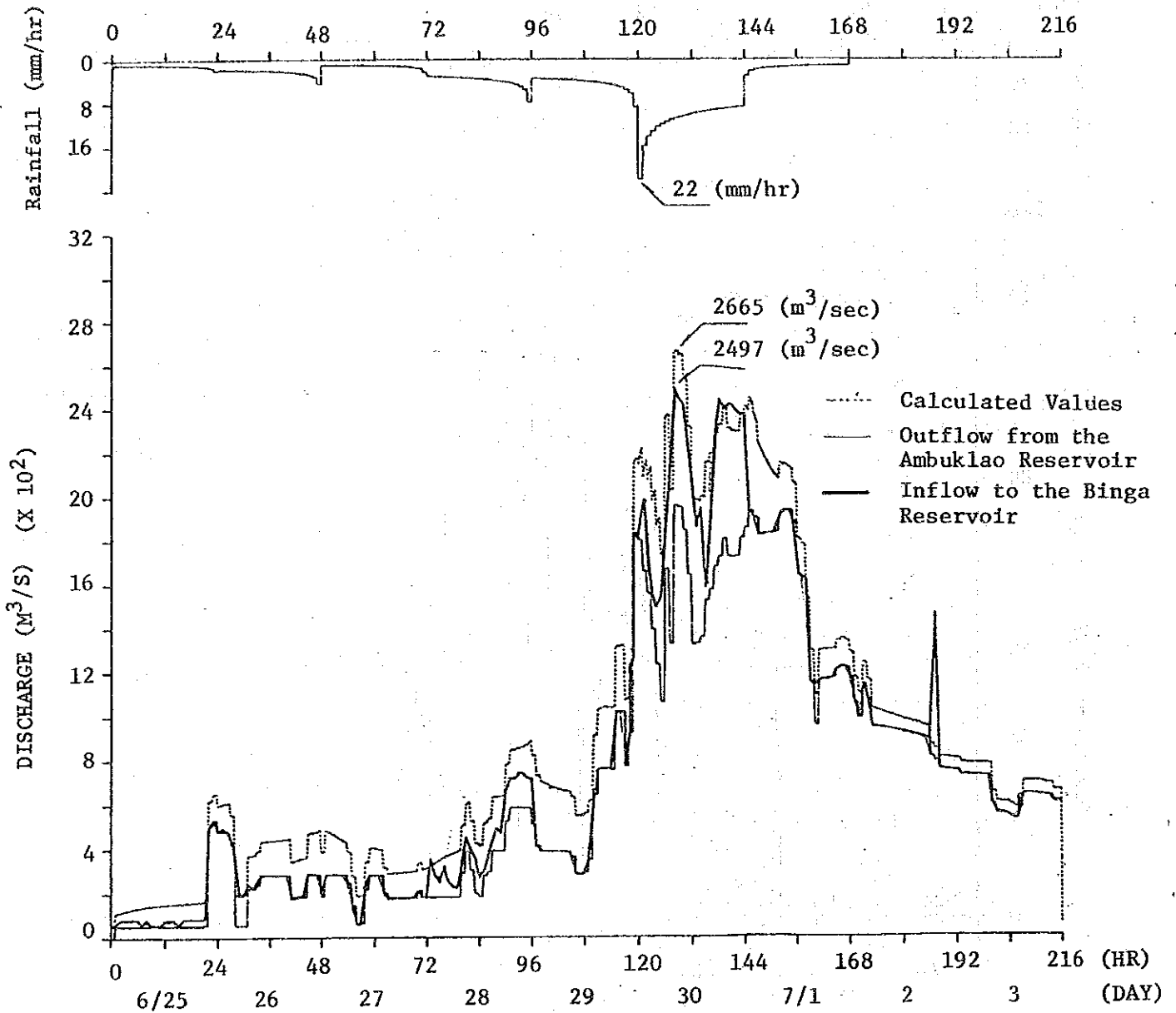
☒ - 9.11(2) Inflow to the Binga Reservoir During Typical Flood Period (June 25 - July 3, 1976)
