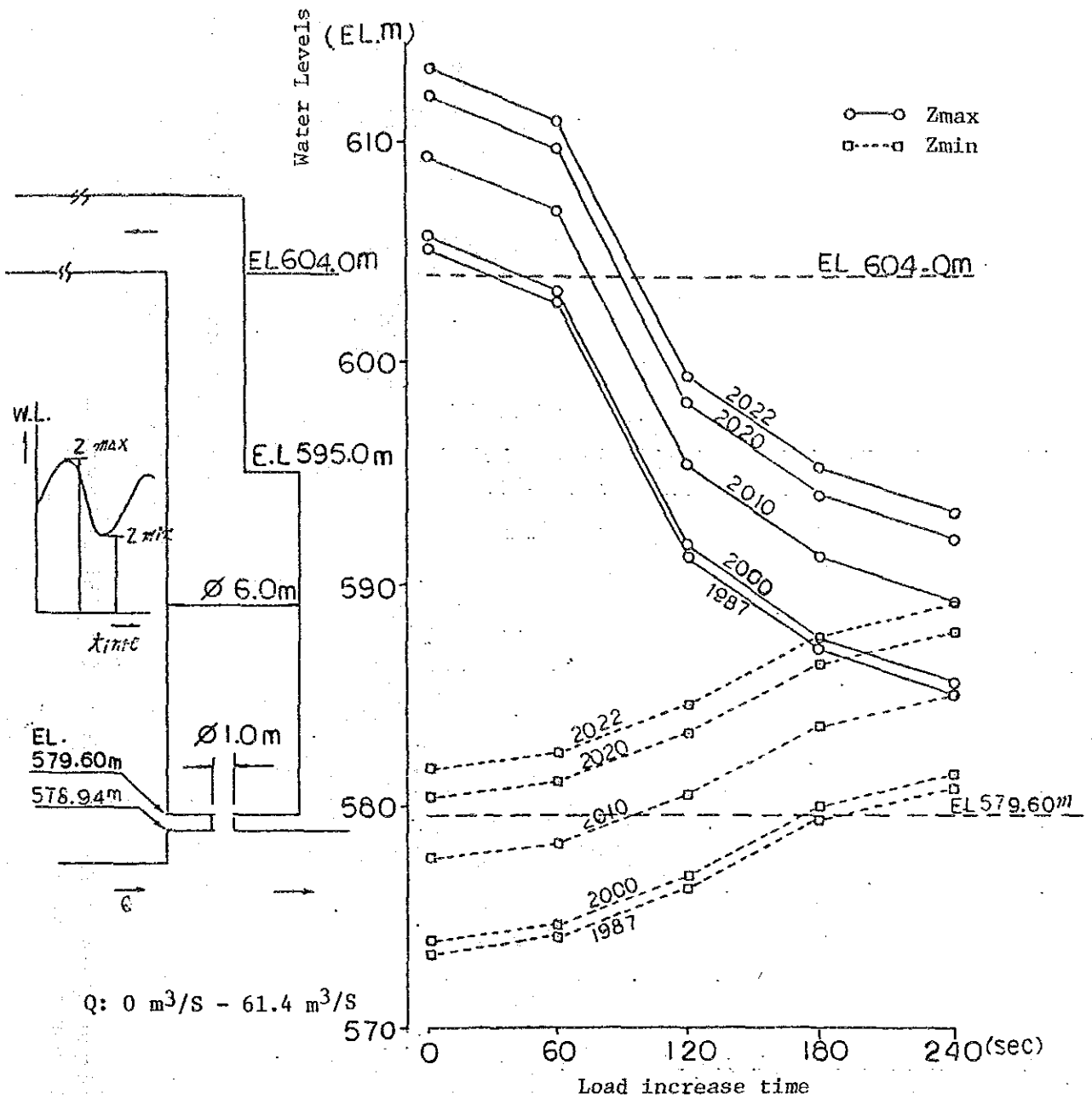
Fig. 10.16 Effects on the Water Levels in the Ambuklao Surge Tank by Further Accumulation of Sedimentation in the Area Around the Ambuklao Tailrace Outlet in Case of Sudden Load Increase
