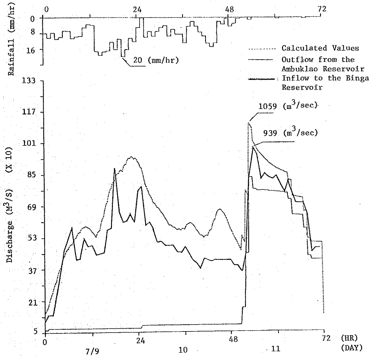
9.11(3) Inflow to the Binga Reservoir During Typical Flood Period (July 9 - 11, 1986)
