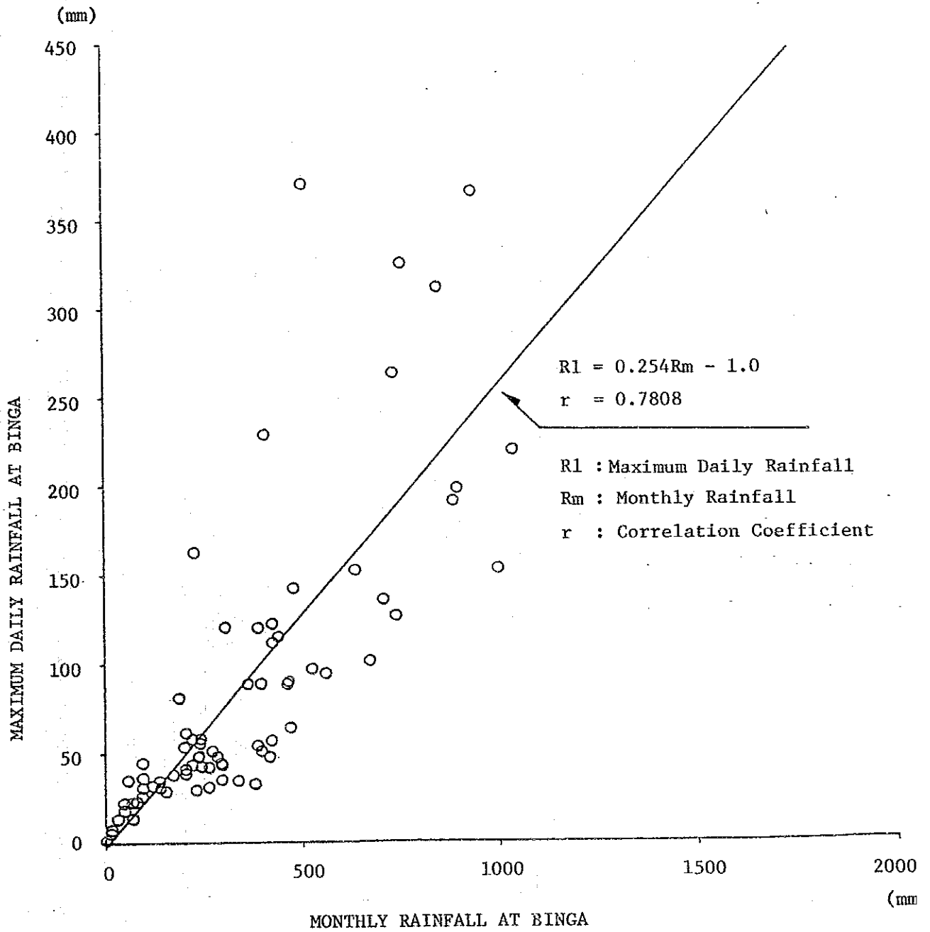
☒ - 9.7 Relation between Monthly Rainfall and Maximum Daily Rainfall at Binga
