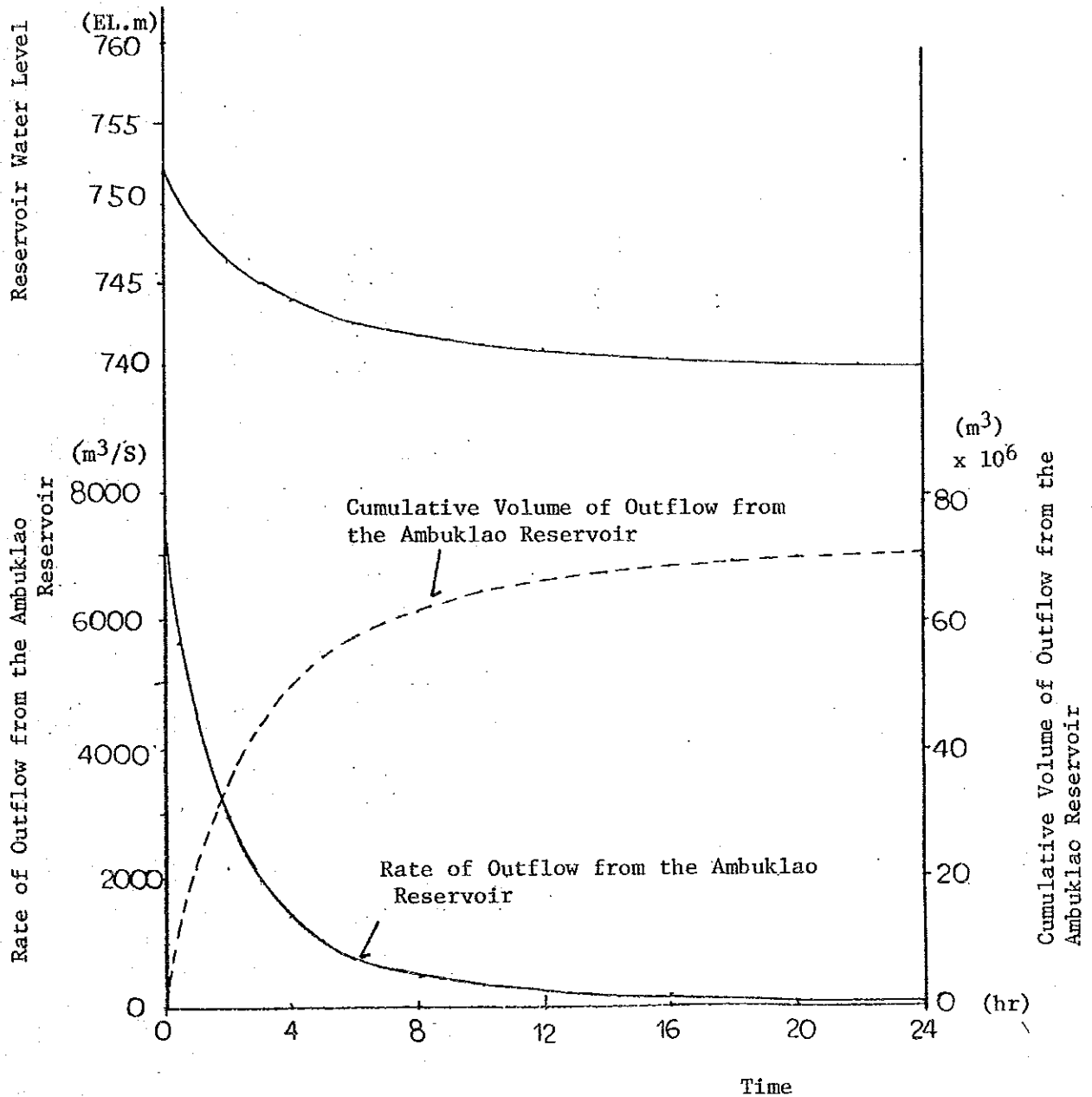
☒ - 10.23 Change with Time in the Outflow from the Ambuklao Reservoir and its Water Level.
