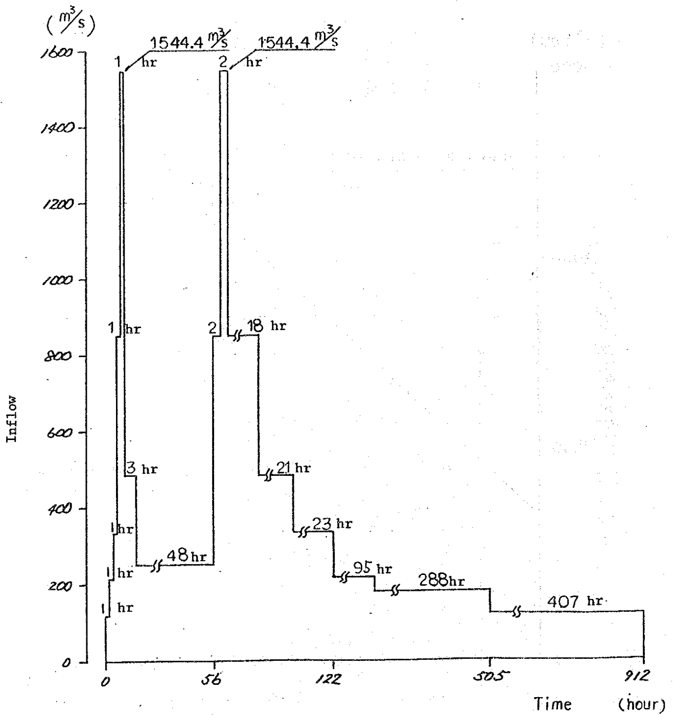
☒ - 10.11 Model Flood Inflow of the Average Year (Including the Inflow from Sadyo River)
