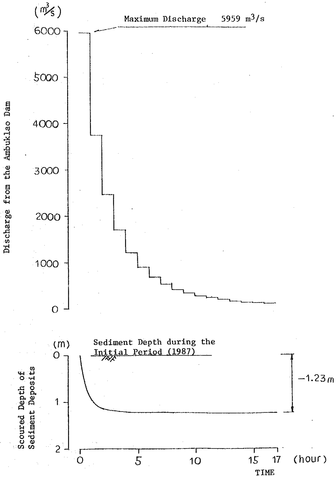
10.21 Changes with Time of Discharges by the Ambuklao Reservoir Operation and Scoured Depth of the Sediment Deposits in the Area Around the Tailrace Outlet
