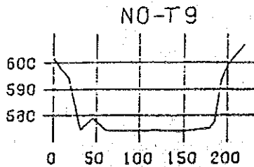
☒ - 10.19(2) Cross Sections of the Upstream Reaches of the Binga Reservoir (1987 Survey)
