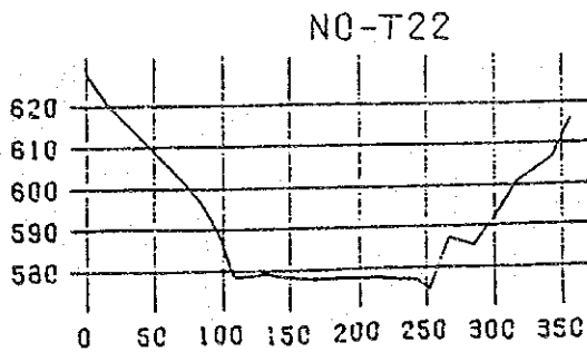
☒ - 10.19(5) Cross Sections of the Upstream Reaches of the Binga Reservoir (1987 Survey)
