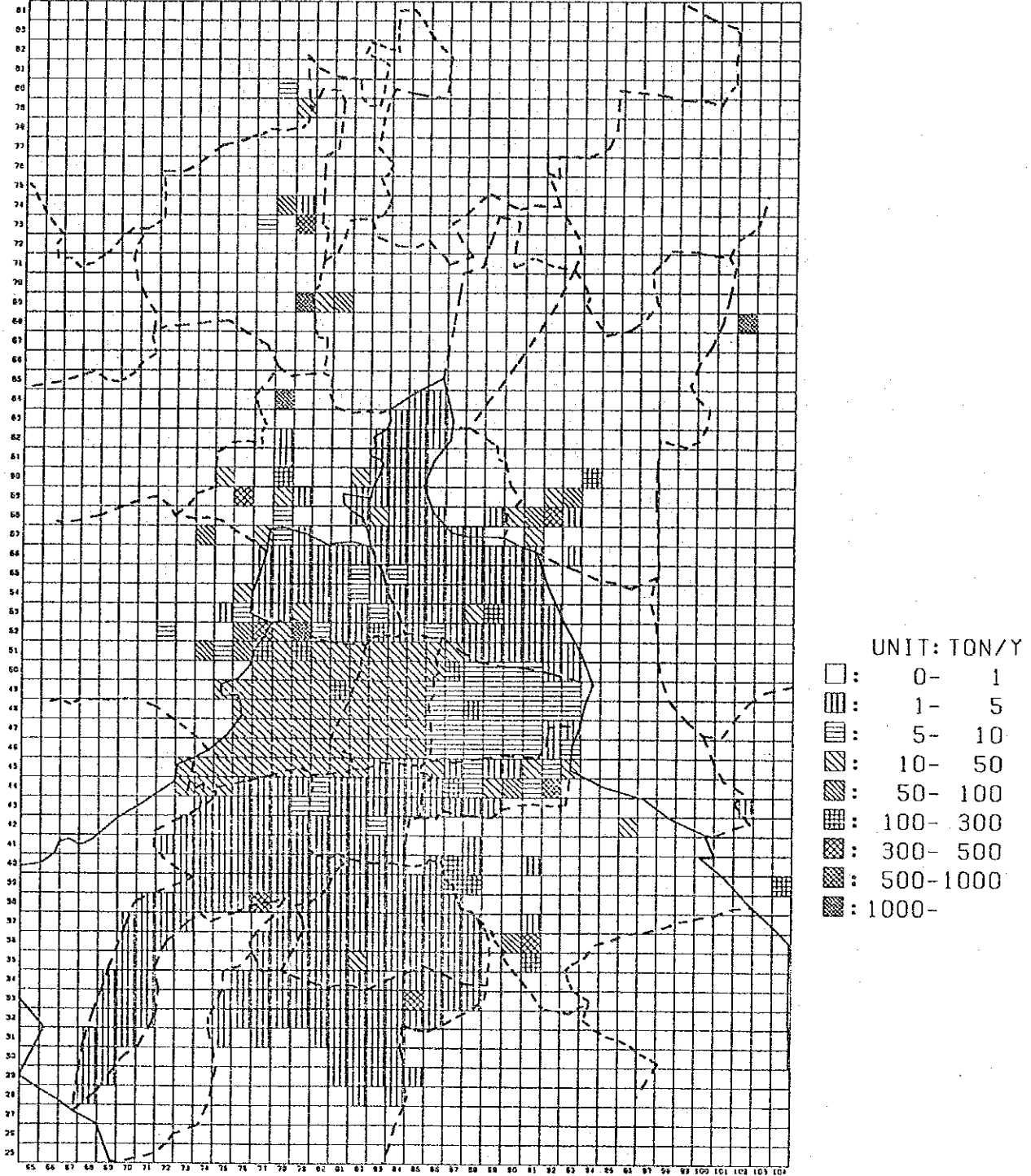
Figure 5.3.1 Distribution of SO 2 Emission From Stationary Sources (1993, With short-term control measures)
