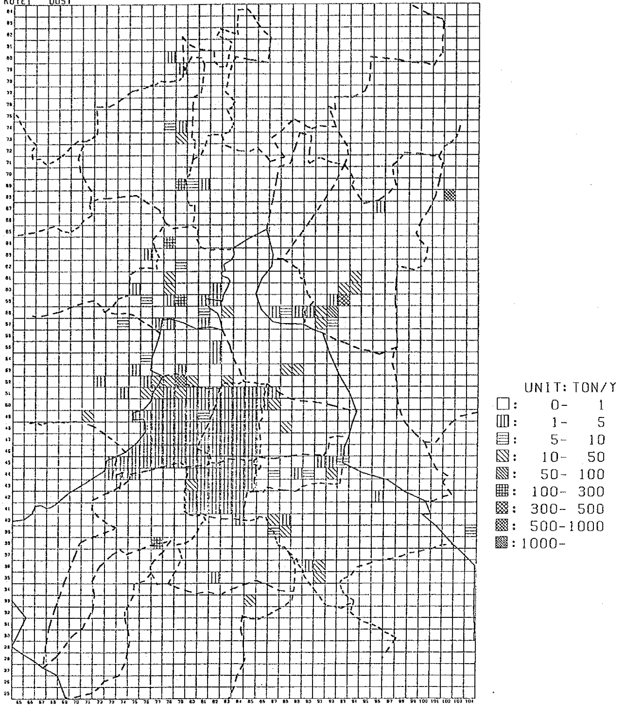
Figure 5.3.8 Distribution of Dust Emission From Stationary Sources (1993, With short-term control measures)
