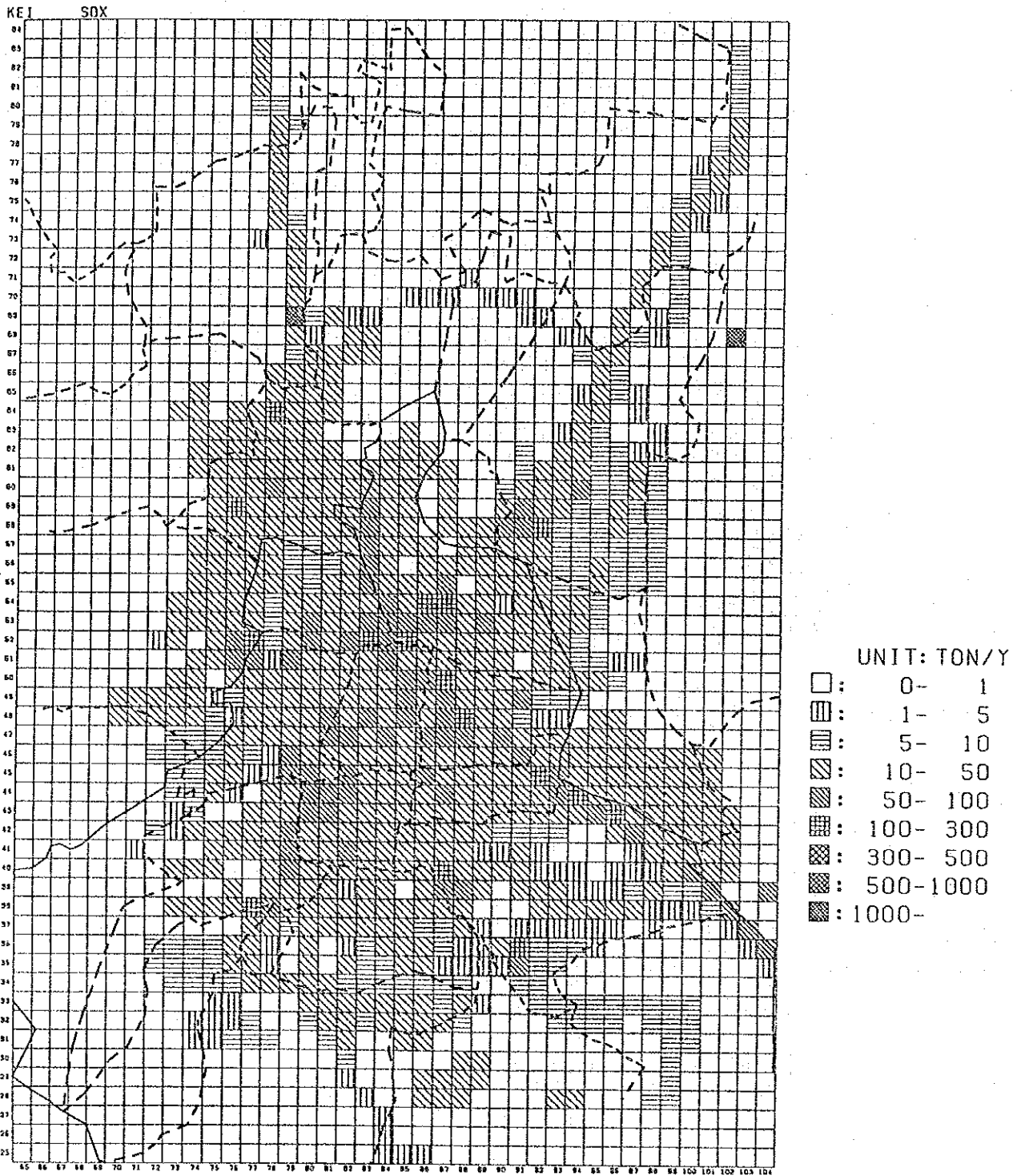
Figure 5.3.11 Distribution of SOx Emission From All Sources (2001, With long-term control measures)
