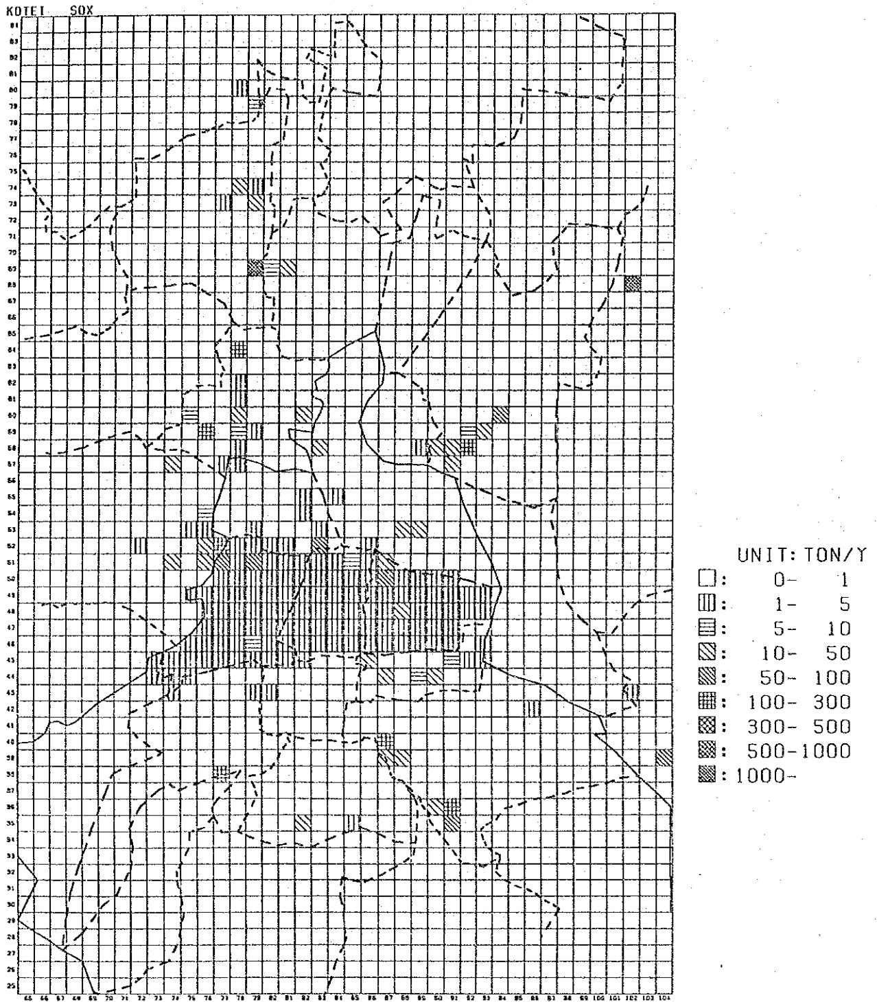
Figure 5.3.9 Distribution of SOx Emission From Stationary Sources (2001, With long-term control measures)
