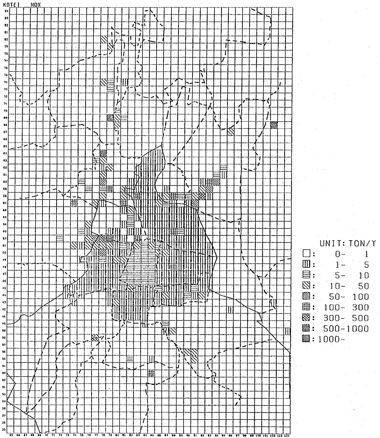
Figure 5.3.5 Distribution of NOx Emission From Stationary Sources (1993, With short-term control measures)
