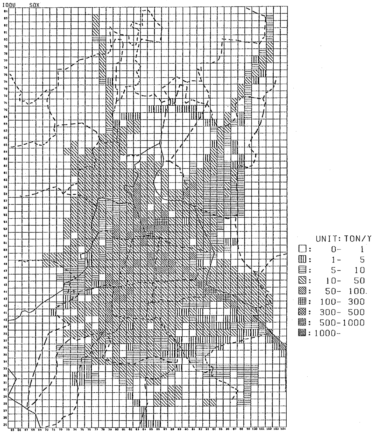
Figure 5.3.2 Distribution of SOx Emission From Mobile Sources (1993, With short-term control measures)
