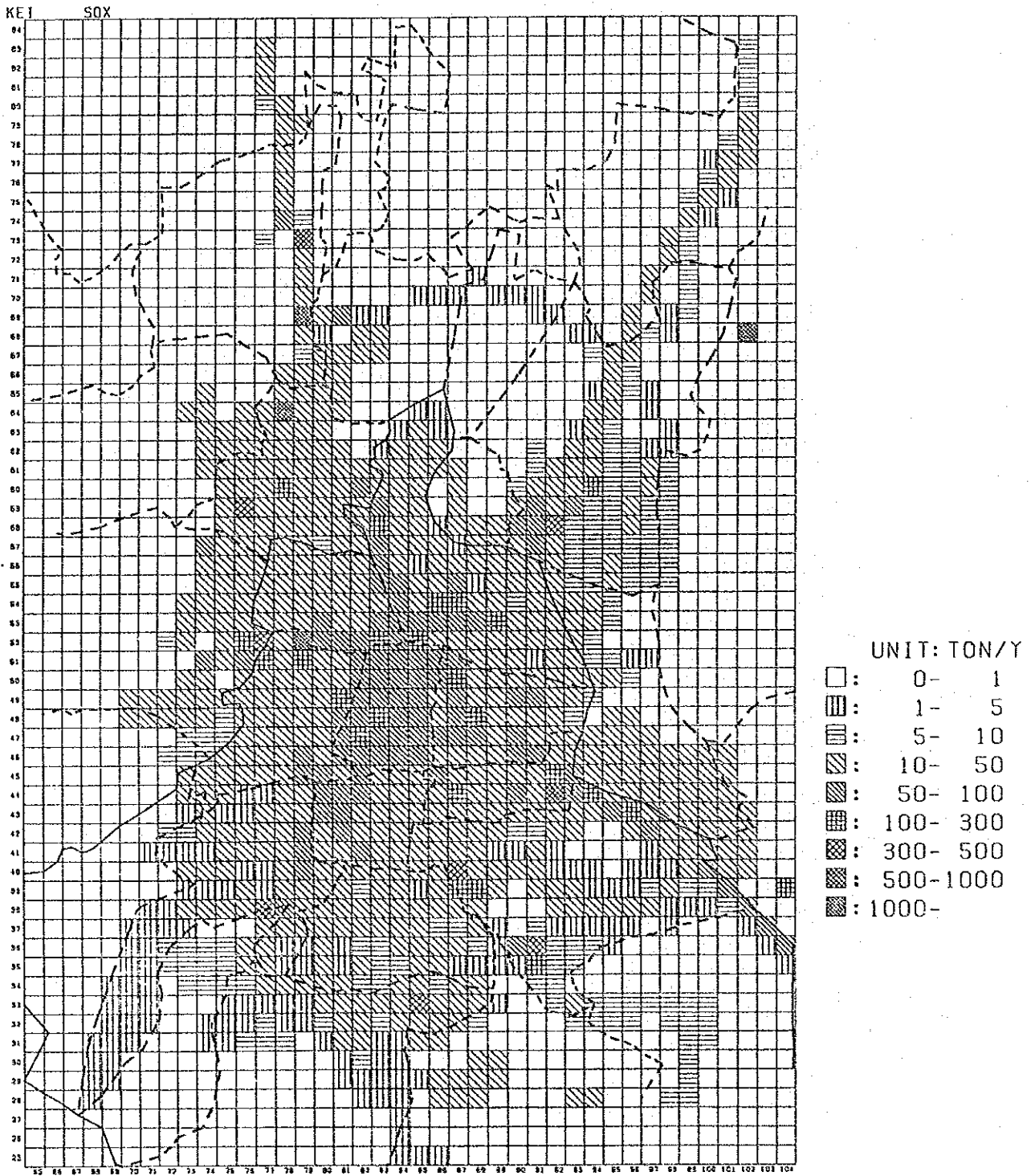
Figure 5.3.3 Distribution of SOx Emission From All Sources (1993, With short-term control measures)
