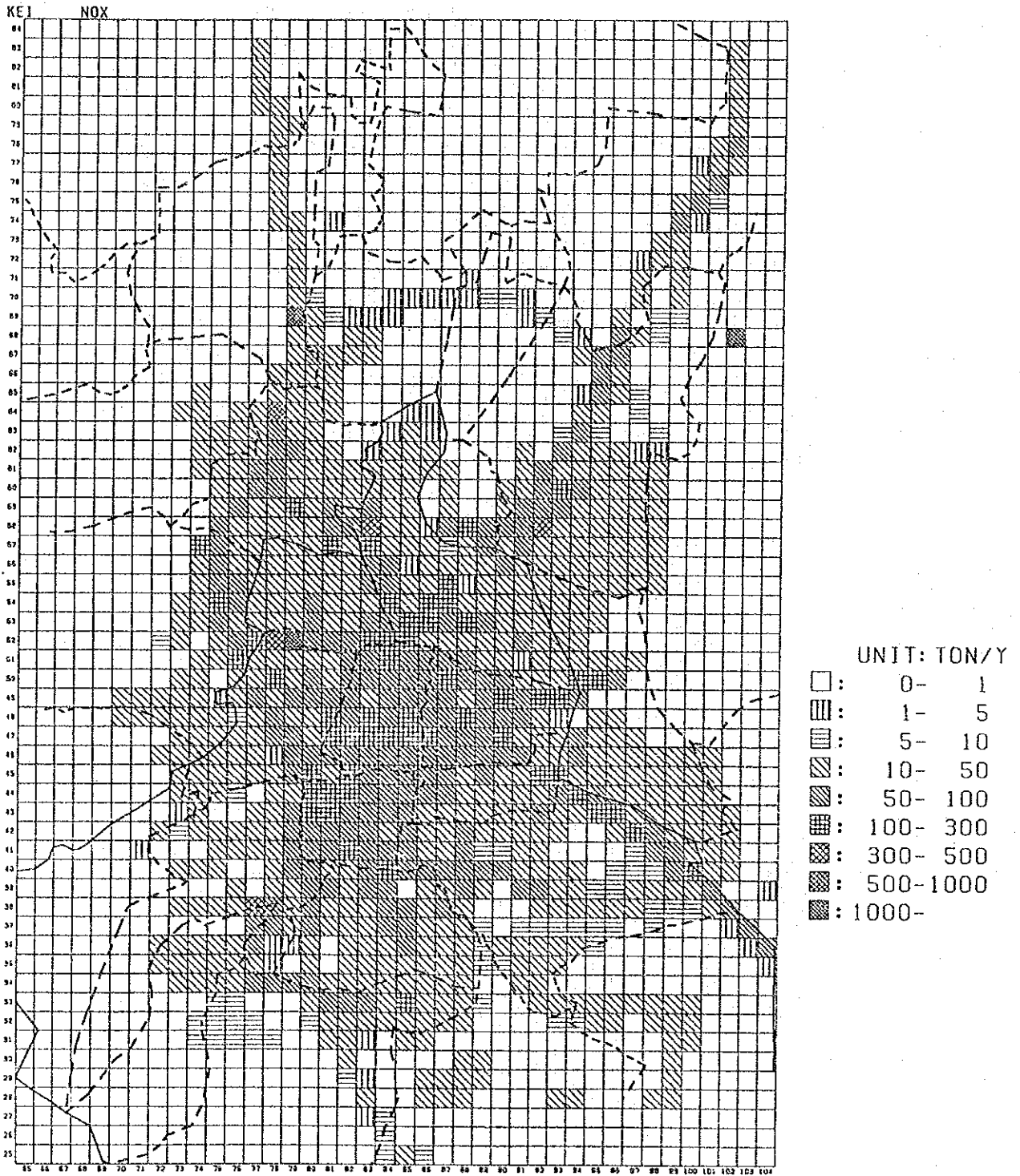
Figure 5.3.15 Distribution of NOx Emission From All Sources (2001, With long-term control measures)
