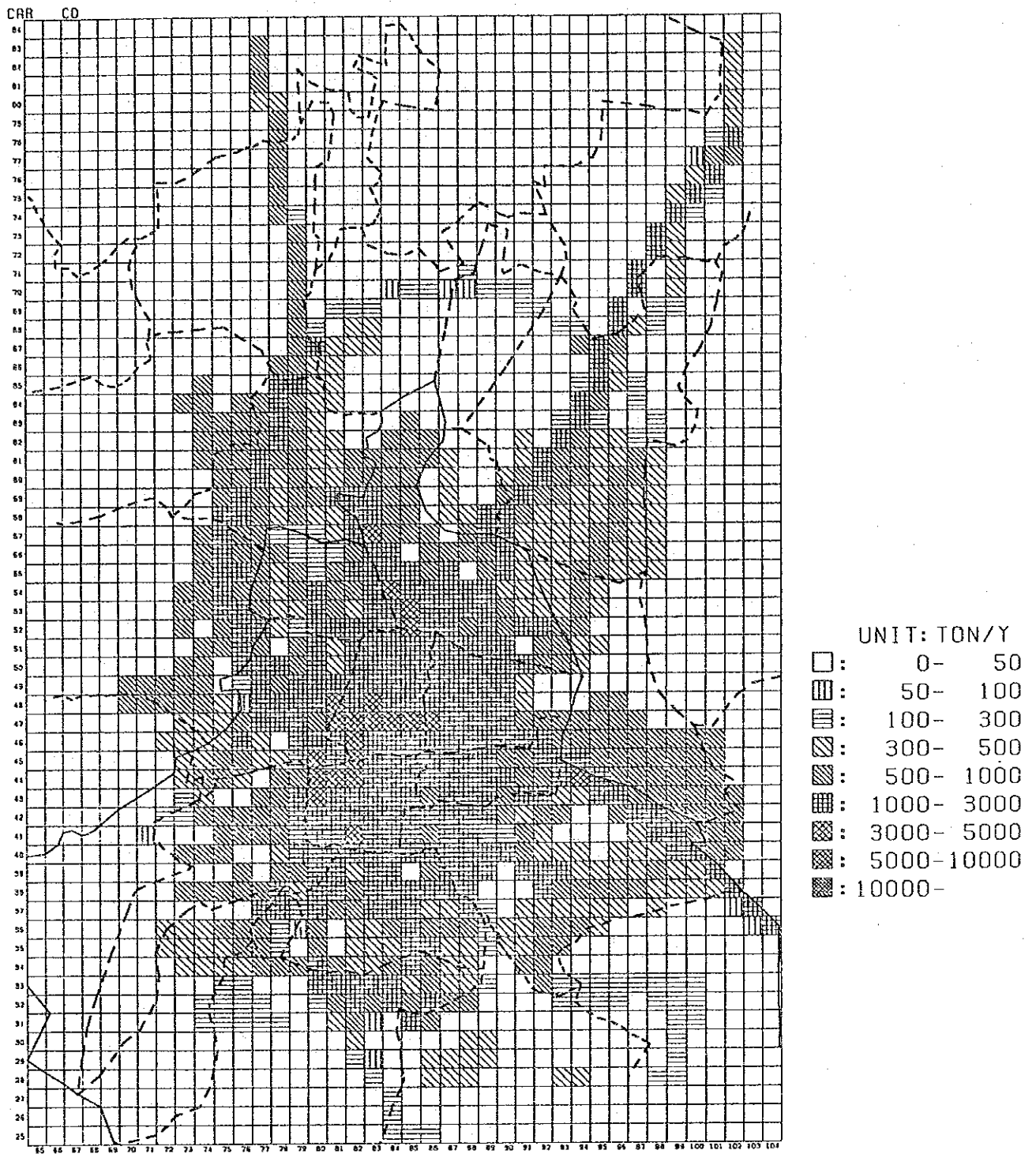
Figure 5.3.6 Distribution of NOx Emission From Mobile Sources (1993, With short-term control measures)
