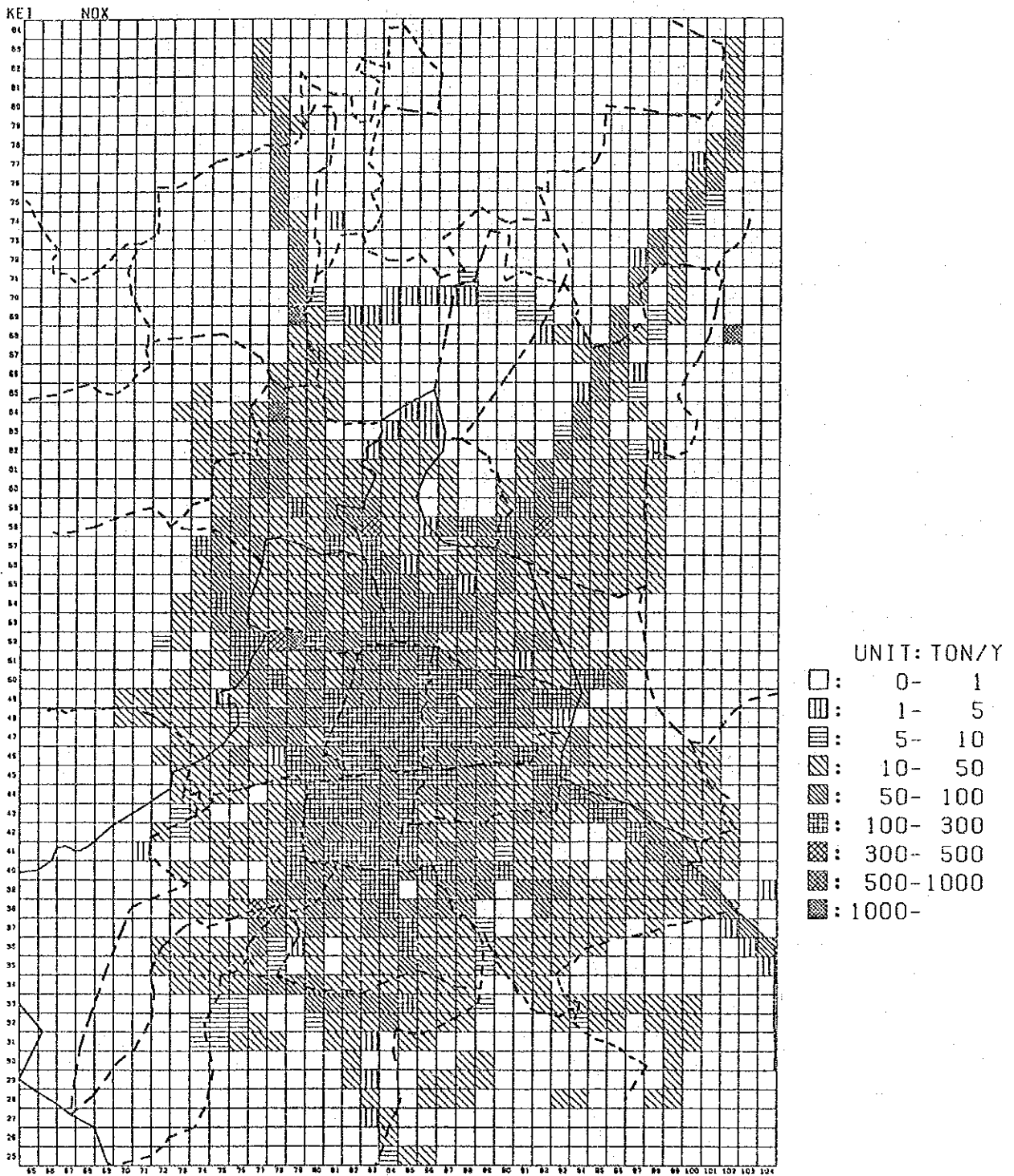
Figure 5.3.7 Distribution of NOx Emission From Mobile Sources (1993, With short-term control measures)
