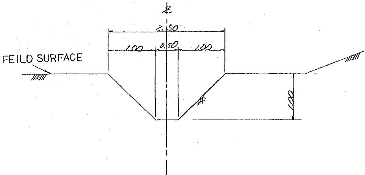
FIG 20 DRAINAGE CANAL STANDARD CROSS SECTION
