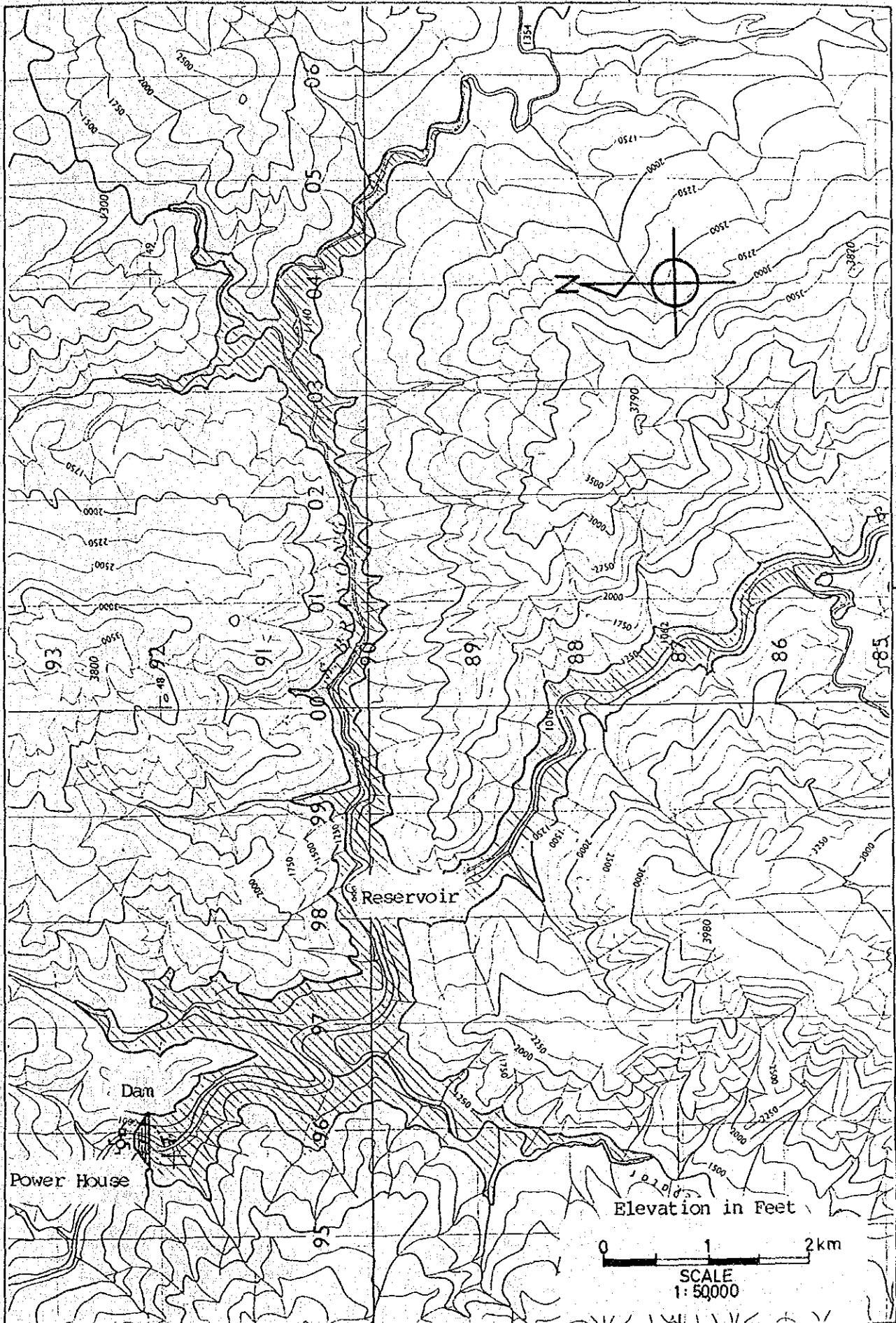
Fig. I. 3 Preliminary Layout Plan for Trusan
