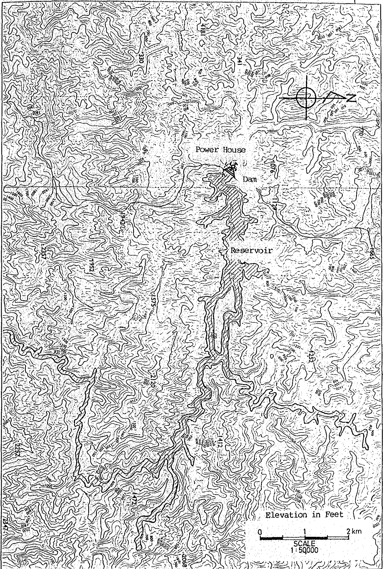
Fig.1. 9 Preliminary Layout Plan for Kapit-2
