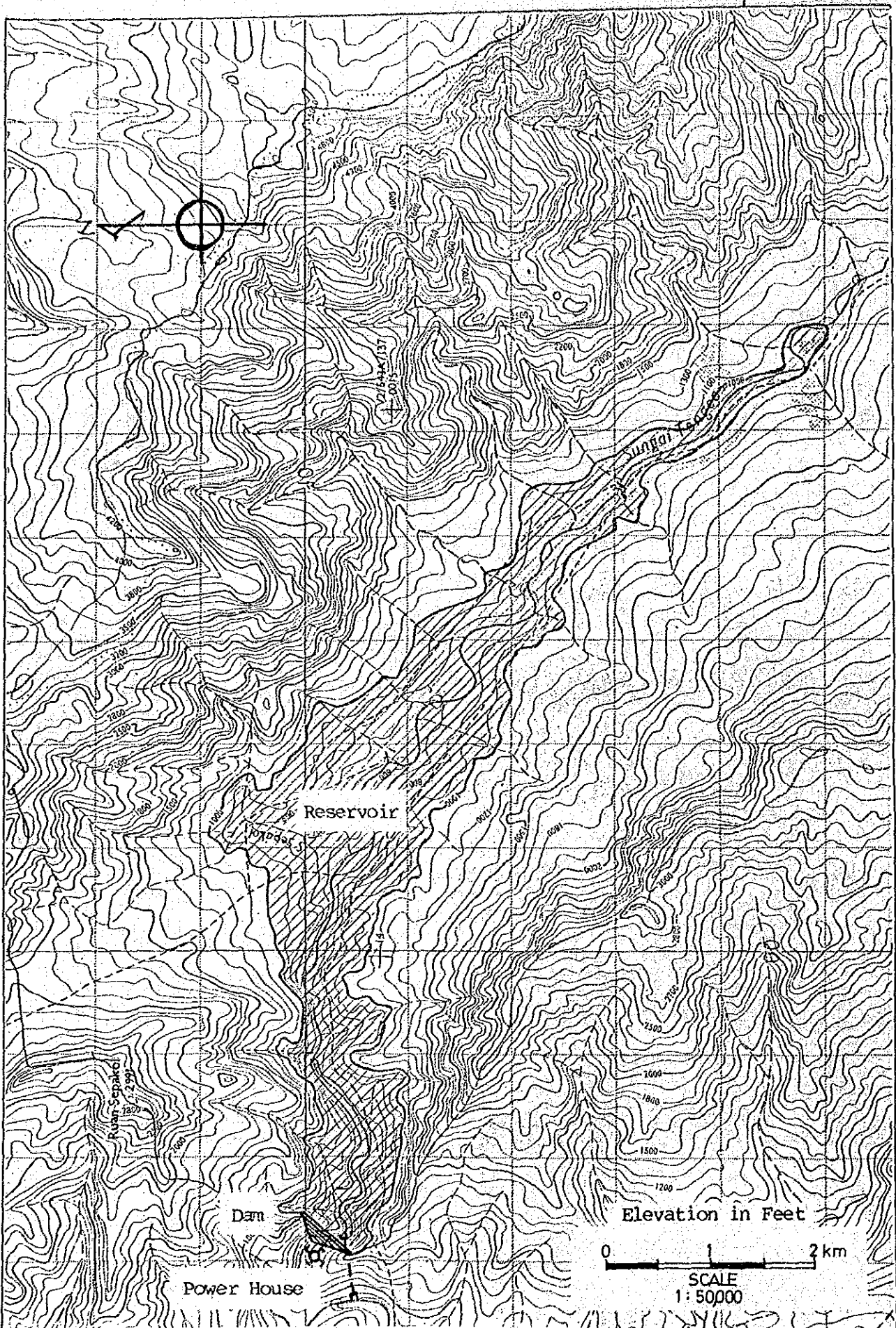
Fig. I. 2 Preliminary Layout Plan for Tengoa
