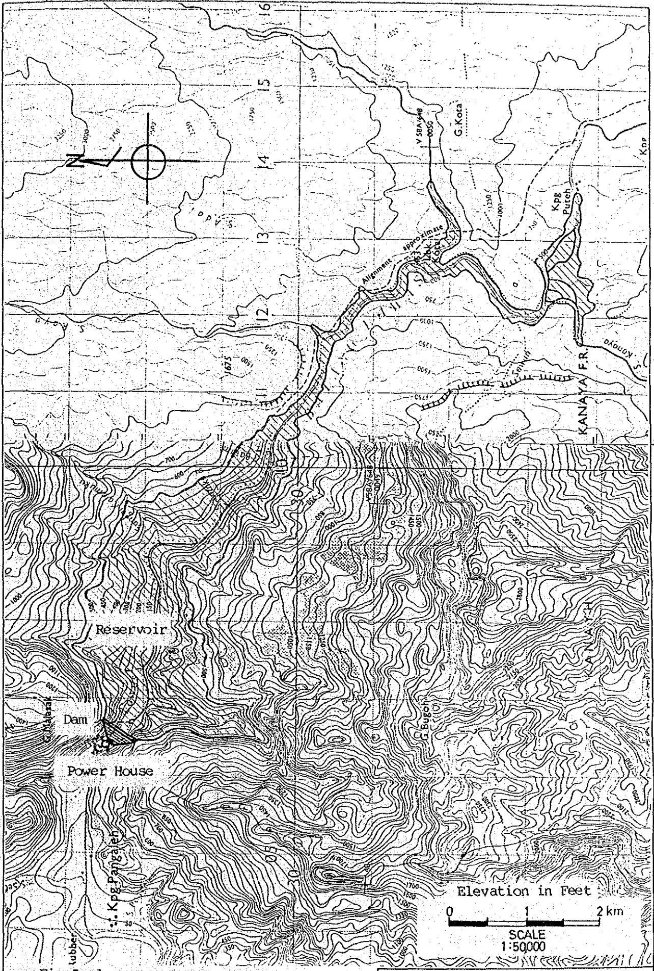
Fig.1. 1 Preliminary Layout Plan for Lawas
