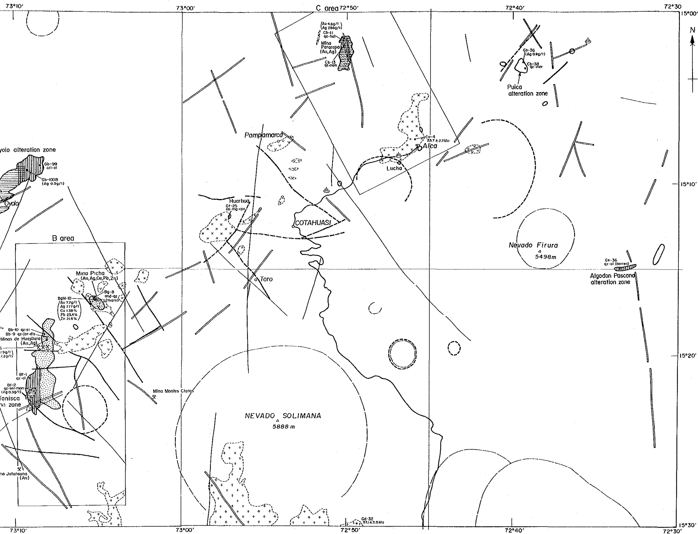
Fig. II-7 Location Map of Alteration and Mineralized Zones
