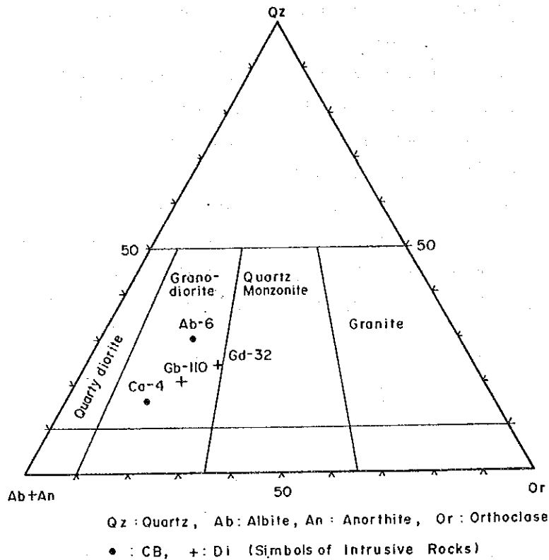
Fig. II-6 Normative Quartz - Orthoclase - (Albite + Anorthite) Triangular Digram of Some Igneous Rocks
