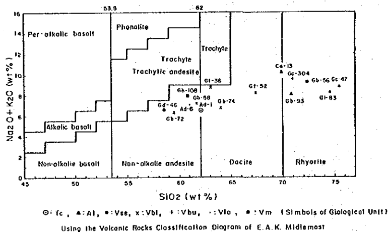
Fig. II-4 SiO_2 - (Na_2O + K_2O) Variation Diagram of Volcanic Rocks
