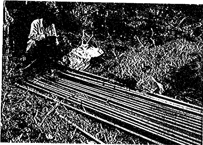
Steel rigs for Standard Penetration Test
