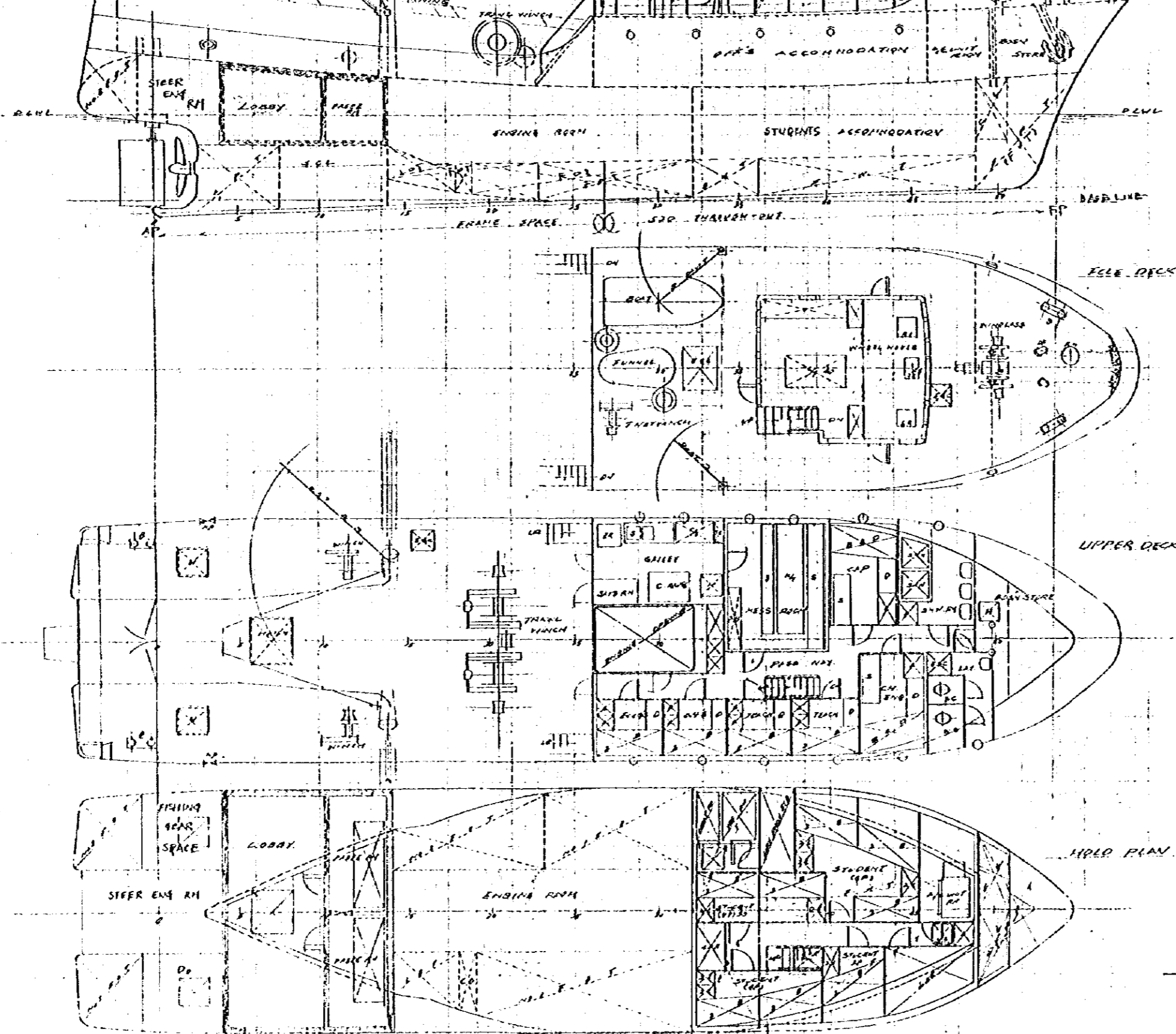
TRAINING BOAT GENERAL ARRANGEMENT
