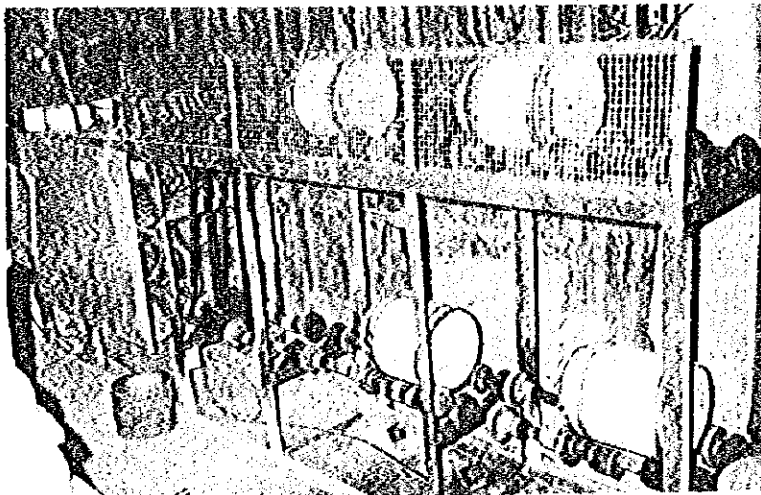
Photo 3-3 Pot mill
