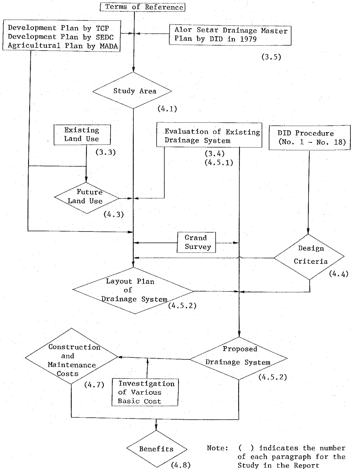
Figure 1.1 Working Flow Sheet for Drainage Master Plan
