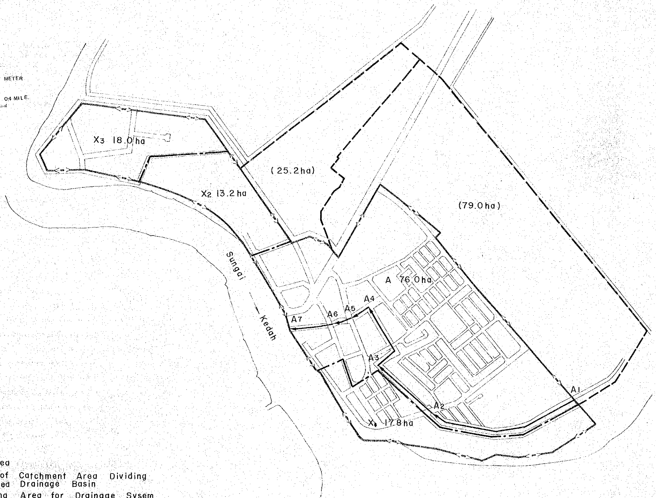
MASTER PLAN AND FEASIBILITY STUDY FOR SEWERAGE AND DRAINAGE SYSTEM PROJECT IN ALOR SETAR AND ITS URBAN ENVIRONS RECOMMENDED LAYOUT PLANNING FOR DRAINAGE SYSTEM FIGURE 4.4
