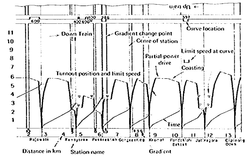
Explanation of Figures of Train Operation Curve
