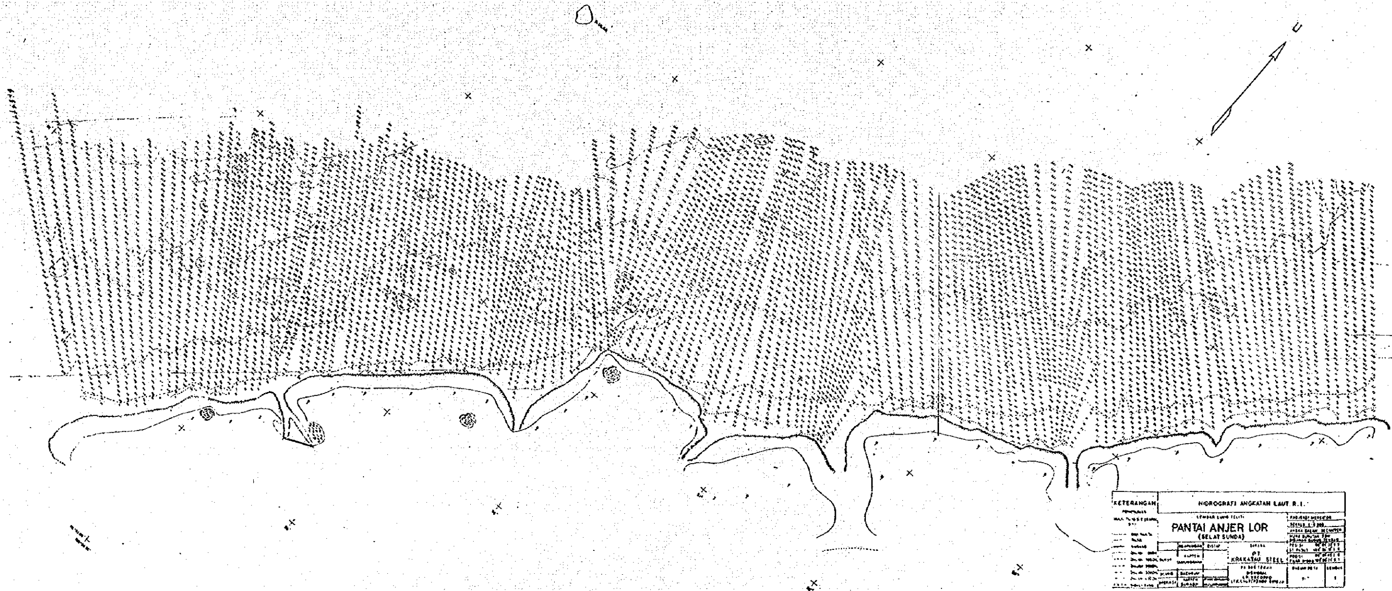
Map - 4 Sea Chart off Anjer-Lor
