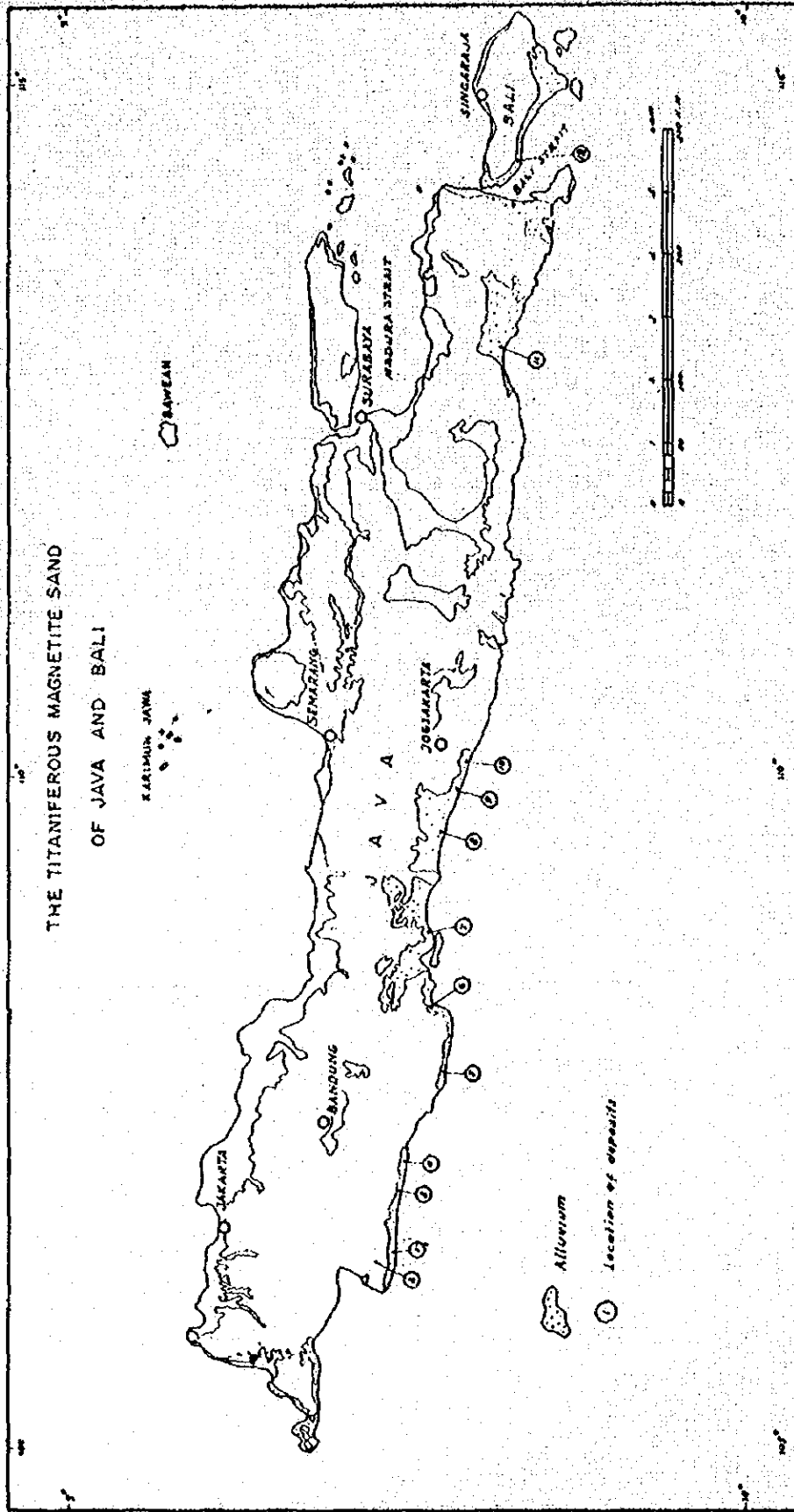
MAP - 1 The Titaniferous Magnetite Sand of Java and Bali
