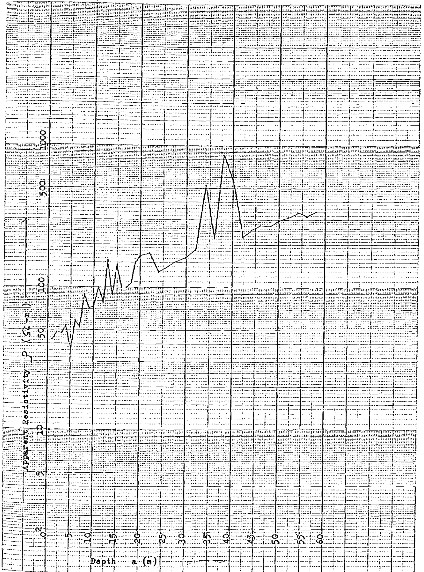
\rho - a Curve ( E - 23 )
