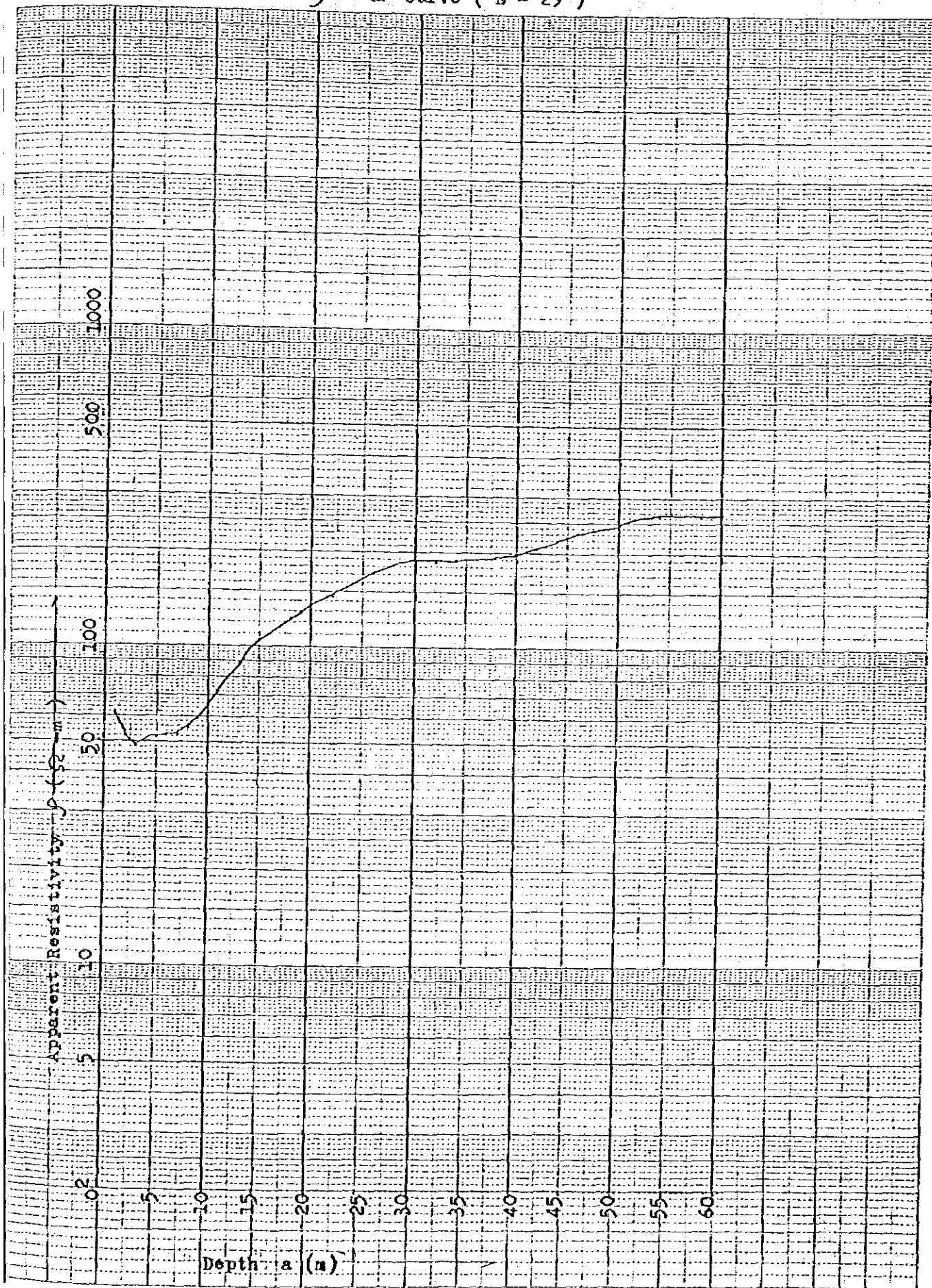
\rho - a Curve ( F - 29 )
