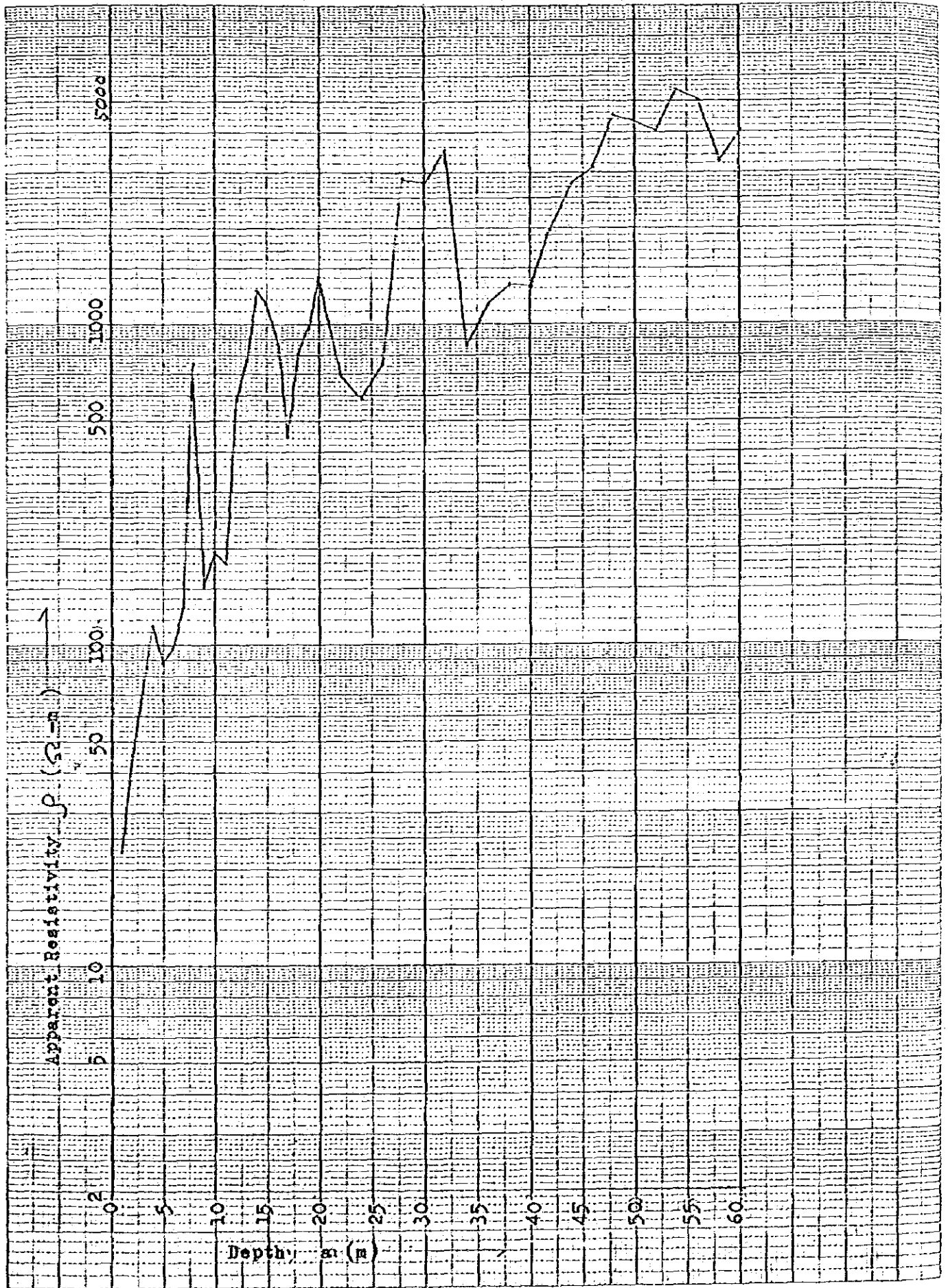
\rho - \alpha Curve ( E - 20 )
