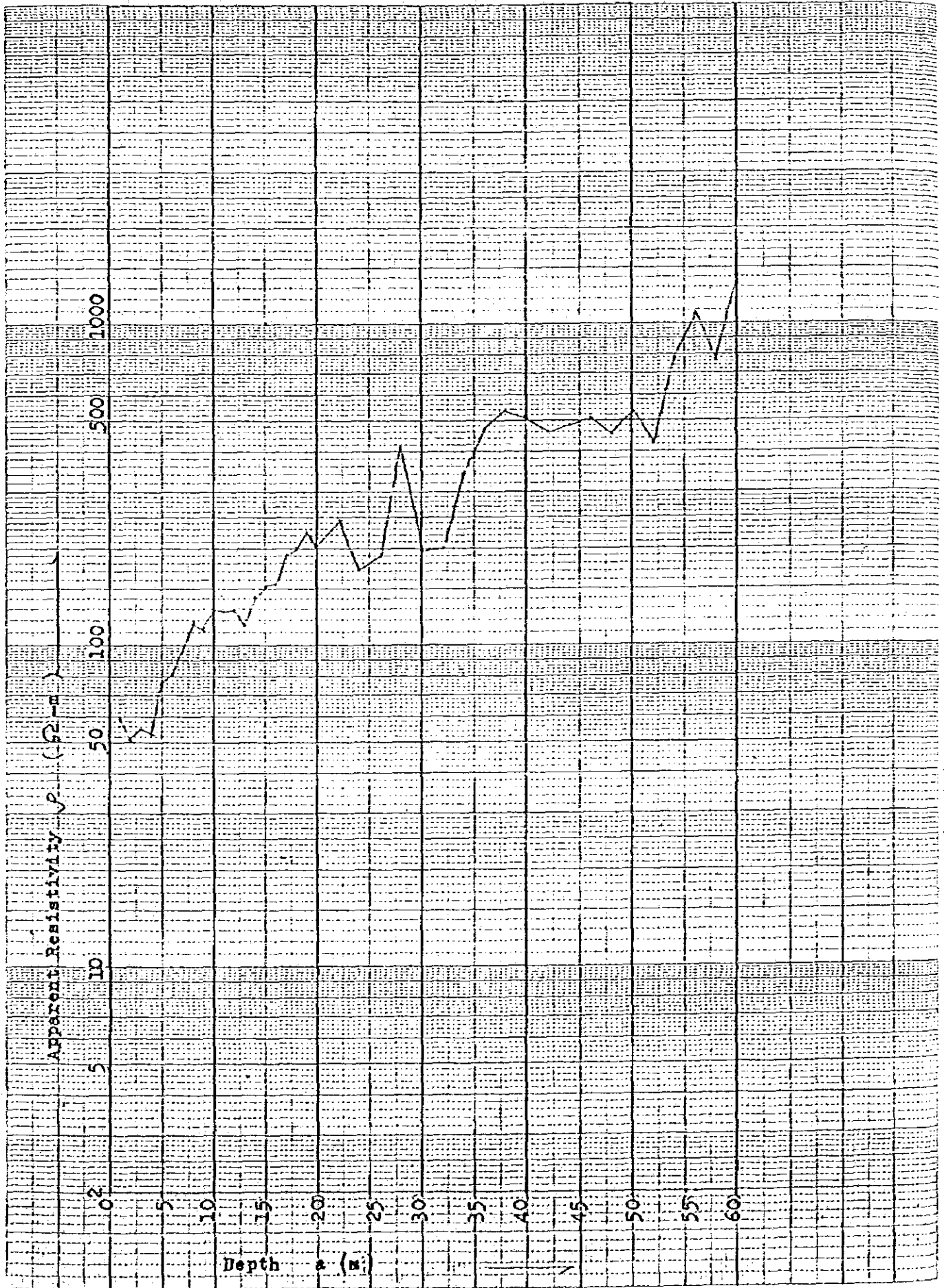
\rho - a Curve ( E - 24 )
