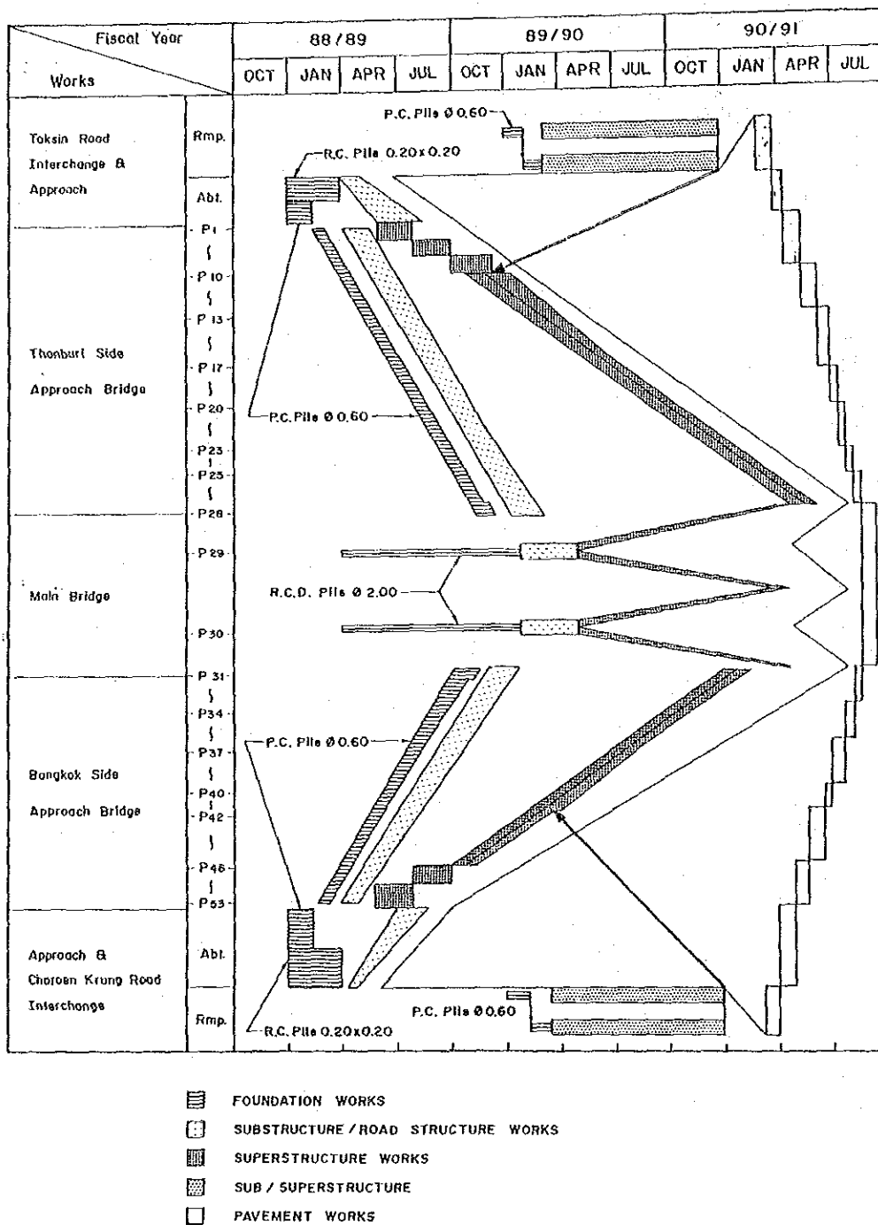
Fig. S-3 Construction Schedule of New Krungthep Bridge
