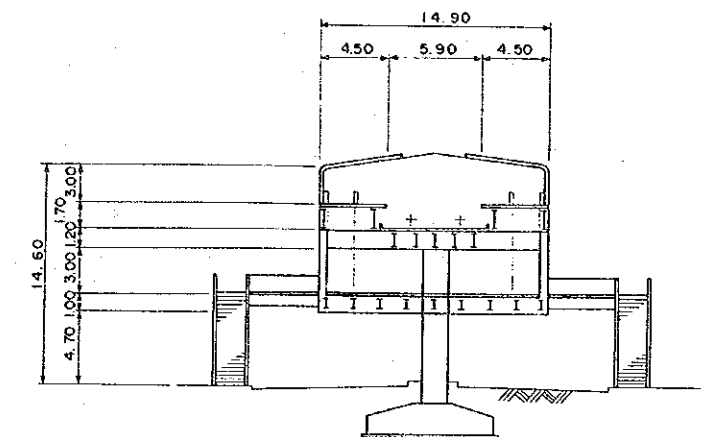
sectional view
