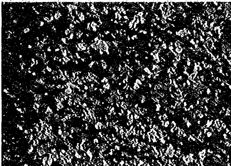
E92203 Locality: 2G Permian-Triassic igneous rock Meta-andesite
