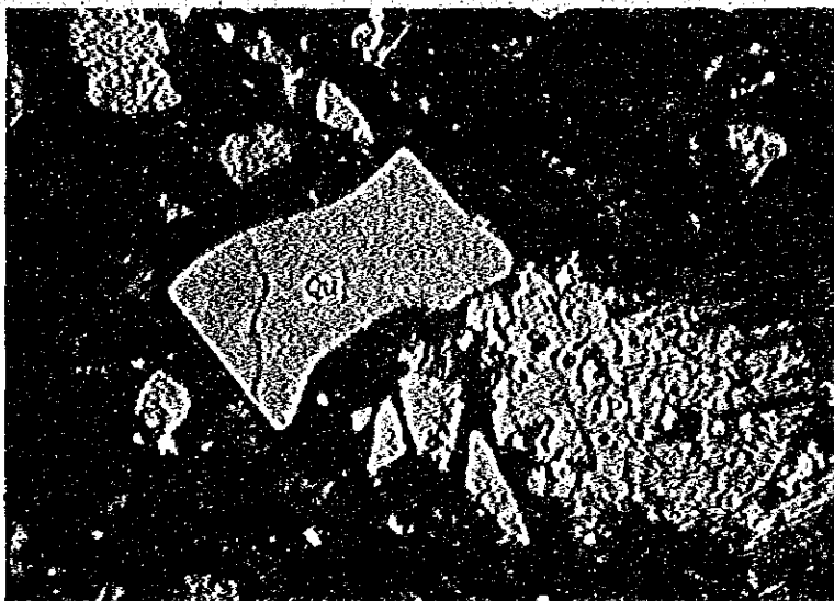
F101102 Locality: 6E Palaeogene igneous rock Rhyolite Qu: Quartz Pl: Plagioclase
