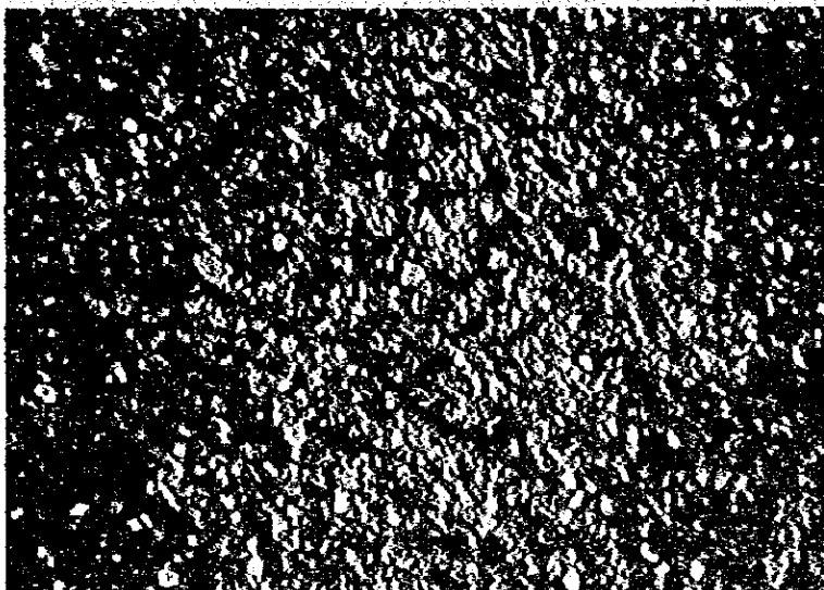
H102814 Locality: 30 Pucara group Calcareous sandstone
