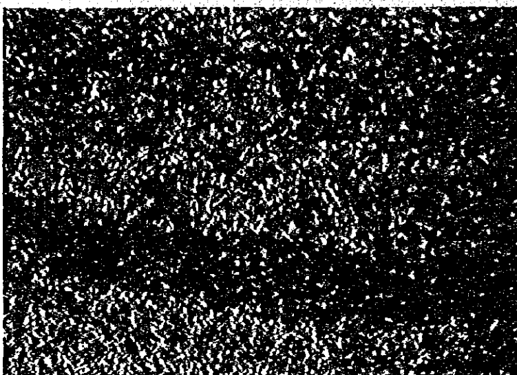
T91306 Locality: 2D Copacabana-Tarma group Muscovite-chlorite phyllite
