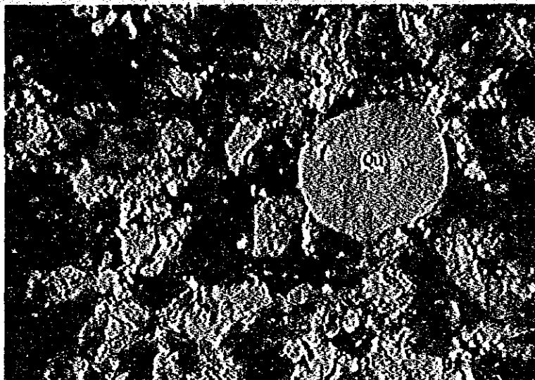
T90906 Locality: 2E Permian-Triassic igneous rock Quartz porphyry Qu: Quartz
