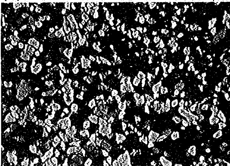
H10207 Locality: 26 Mitu group Sandstone
