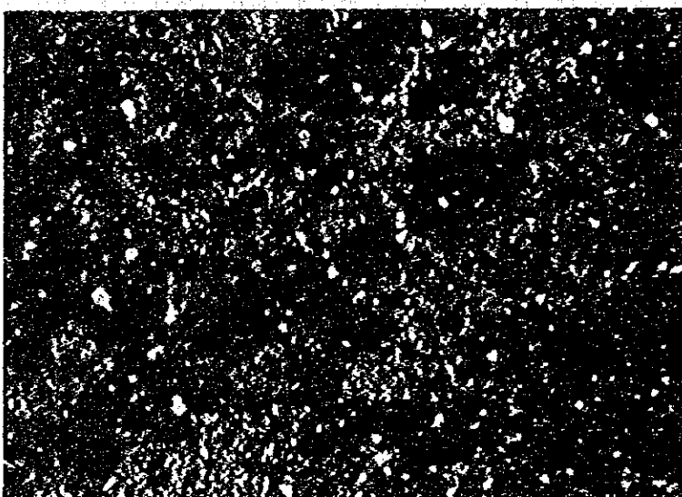
H102819 Locality: 30 Mitu group Red mudstone
