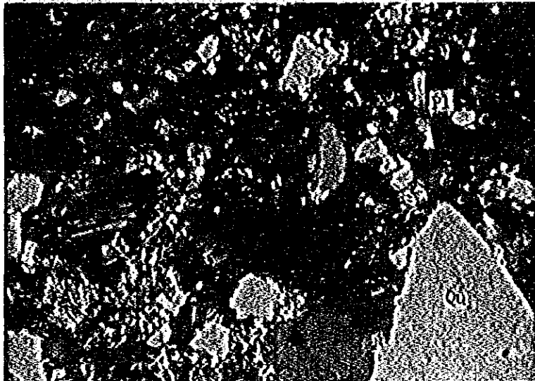
T92202 Locality: 2D Palaeogene igneous rock Rhyolitic tuff breccia Qu: Quartz Pl: Plagioclase
