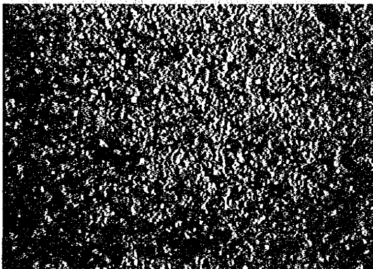
S19602 Locality: 6P Pucara group Mudstone
