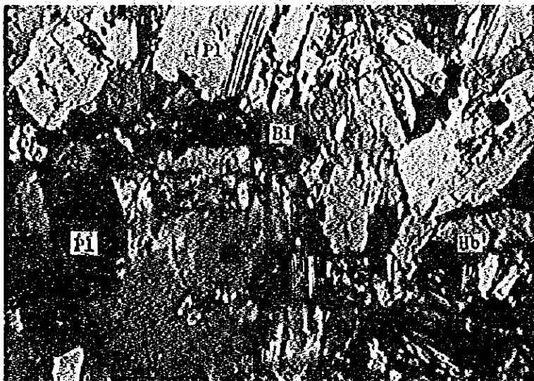
F101301 Locality: 6D Permian-Triassic igneous Rock Hornblende diorite Pl: Plagioclase Hb: Hornblende Bi: Biotite
