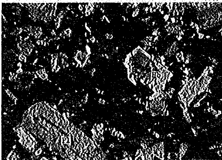
S92104 Locality: 7G Palaeogene igneous rock Clinopyroxene bearing hornblende porphyrite Pl: Plagioclase Hb: Hornblende
