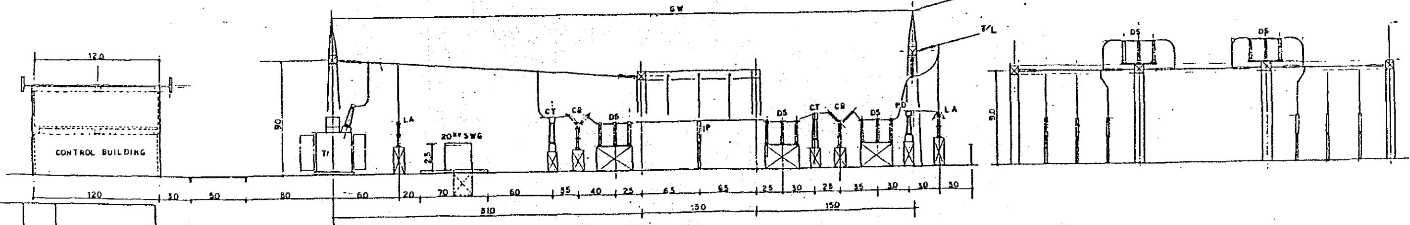
Annex 6-1 (B) Arrangement and Connection Diagram for Simpang baru S/S-2
