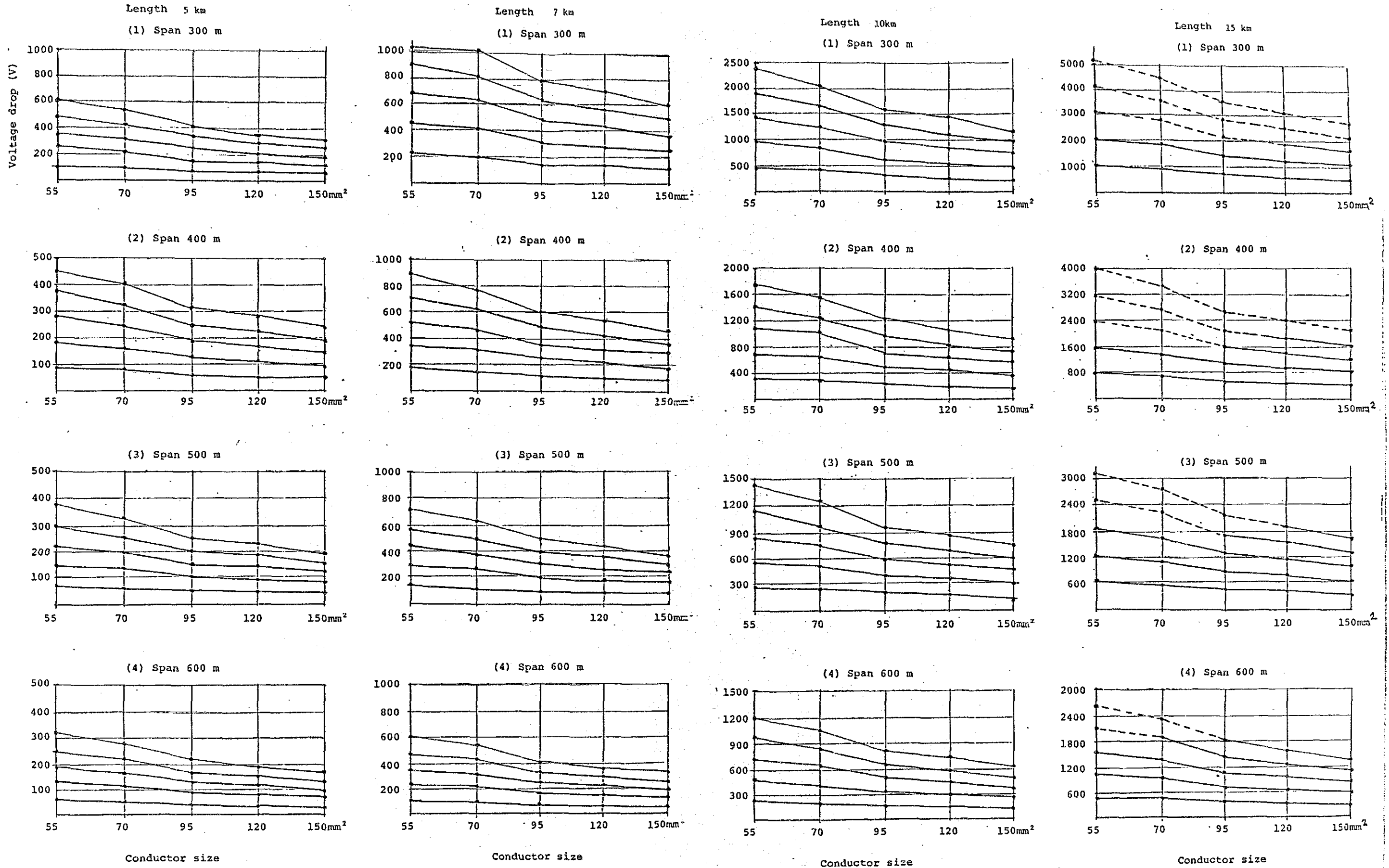
Fig. 2 Maximum Voltage Drop (V) at the end of Distribution Line
