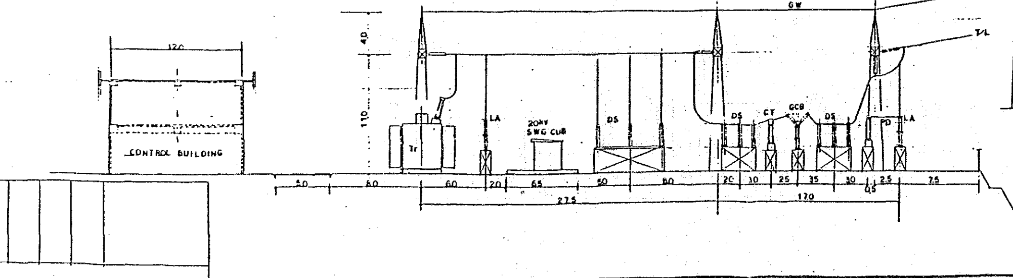
Annex 6-1 (a) Arrangement and Connection Diagram for Simpang baru S/S-1
