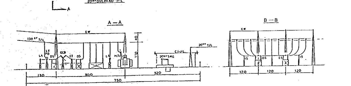
Annex 6-4 Typical Layout for 150/20 kV, 30 MVA x3 Substation
