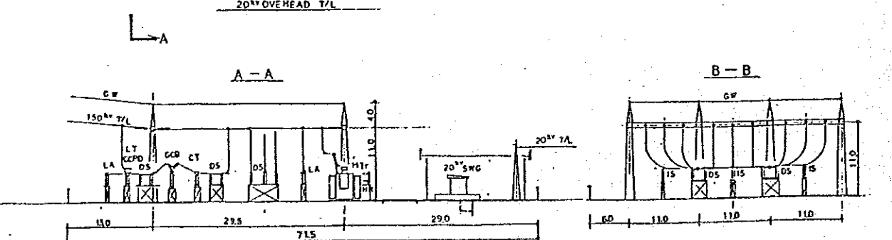
Annex 6-3 Typical Layout for 150/20 kV, 10 MVA x3 Substation
