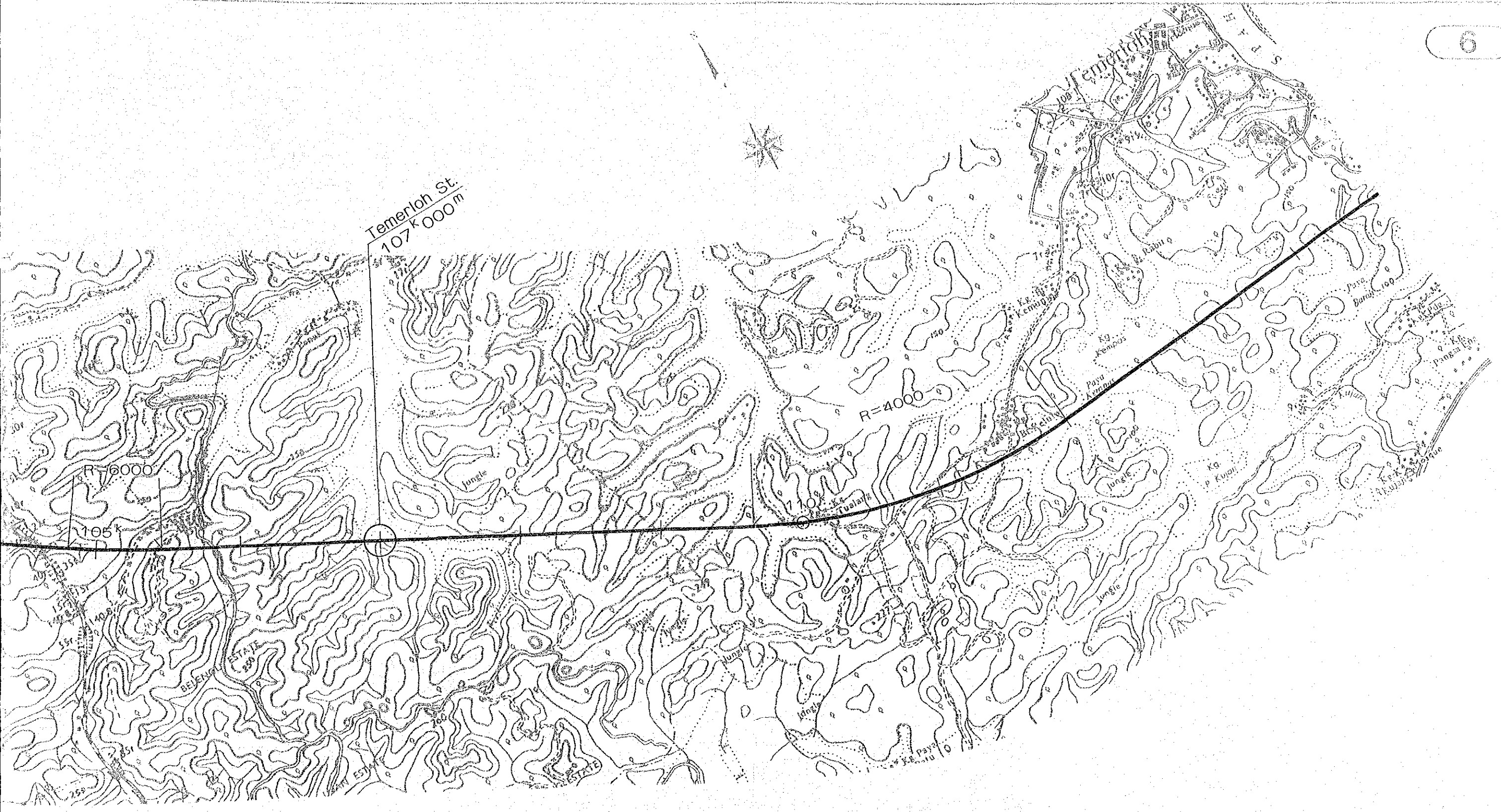
THE NEW EAST-WEST RAILWAY MAIN LINE (Sheet 6 of 28) Scale 1 : 25,000
