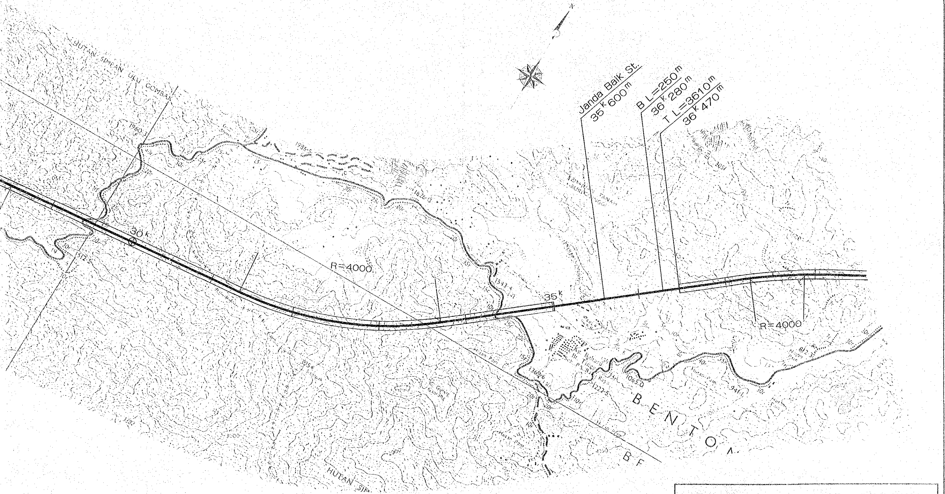
THE NEW EAST-WEST RAILWAY MAIN LINE (Sheet 2 of 28) Scale 1 : 25,000
