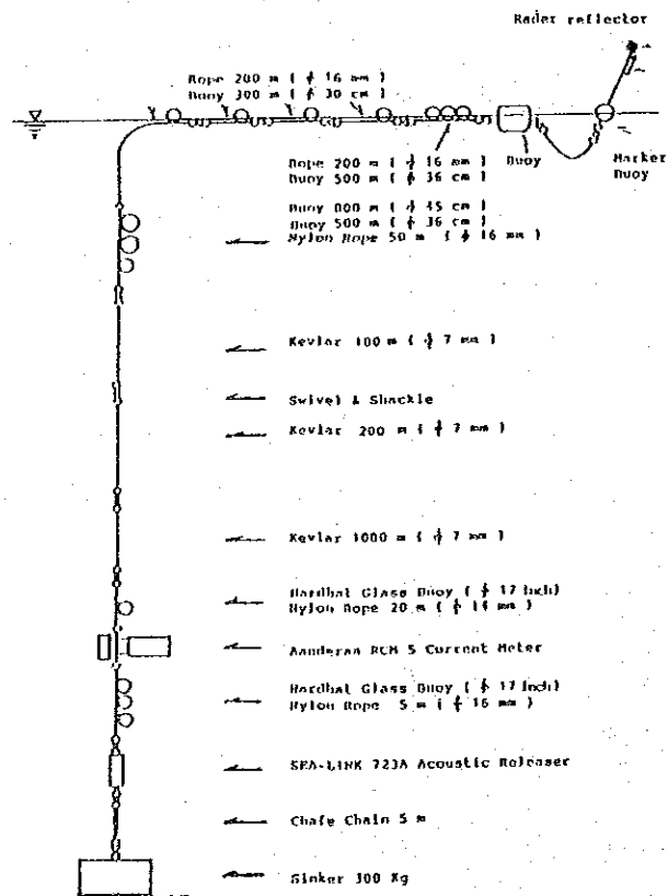
Fig. A-10-2 (2/2) Mooring Configuration for Ocean Area
