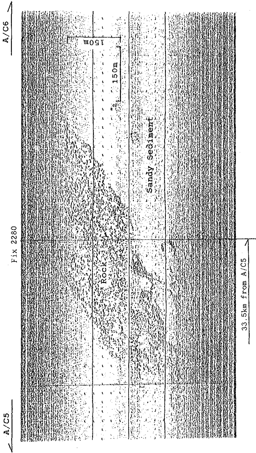
Fig. A-11-3 (3/4) Record of Side Scan Sonar (Pipeline)
