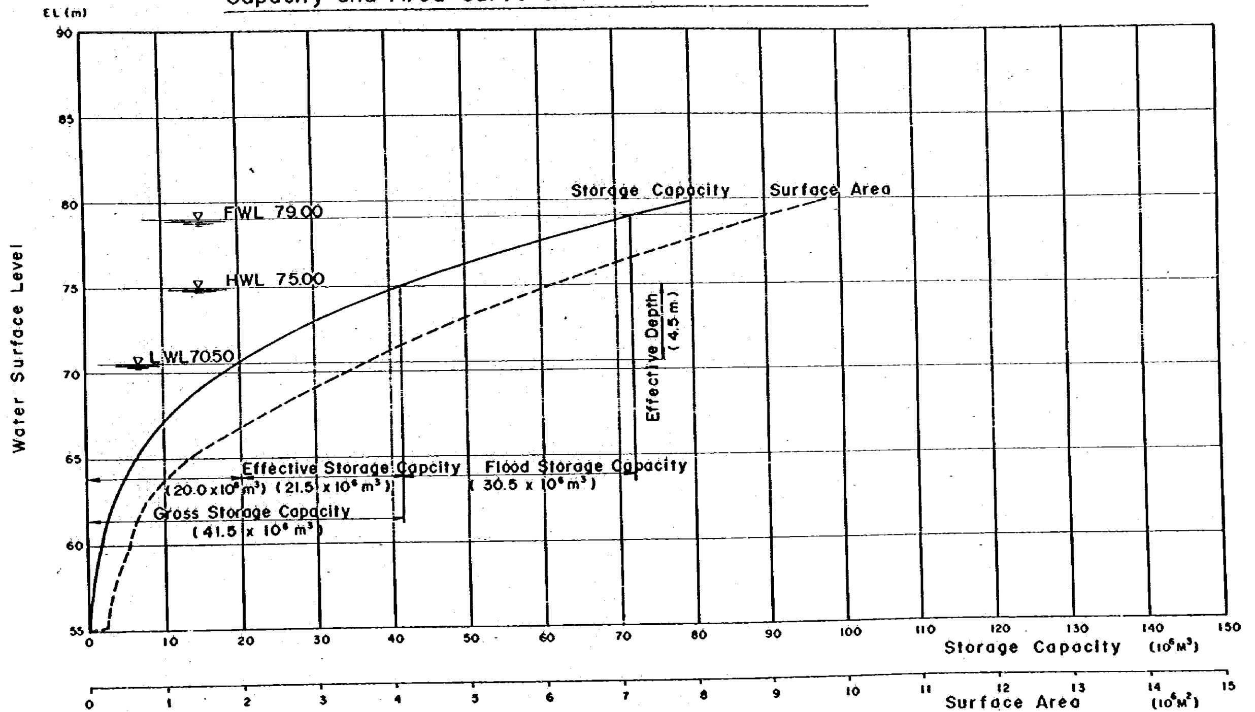
Capacity and Area Curve of Lower Tekai Reservoir
