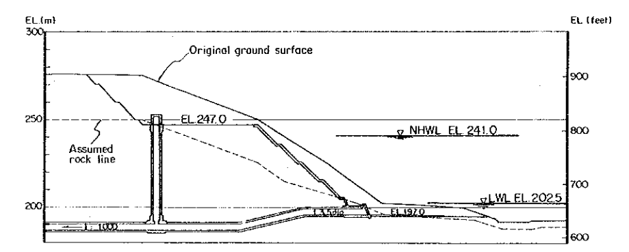
PROFILE OF INTAKE SCALE B
