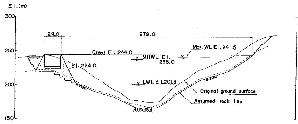
UPSTREAM ELEVATION DAM SCALE A
