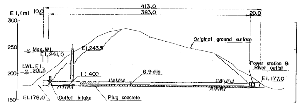
PROFILE OF DIVERSION TUNNEL NO. 2 SCALE B
