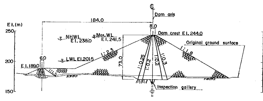
MAXIMUM SECTION SCALE A
