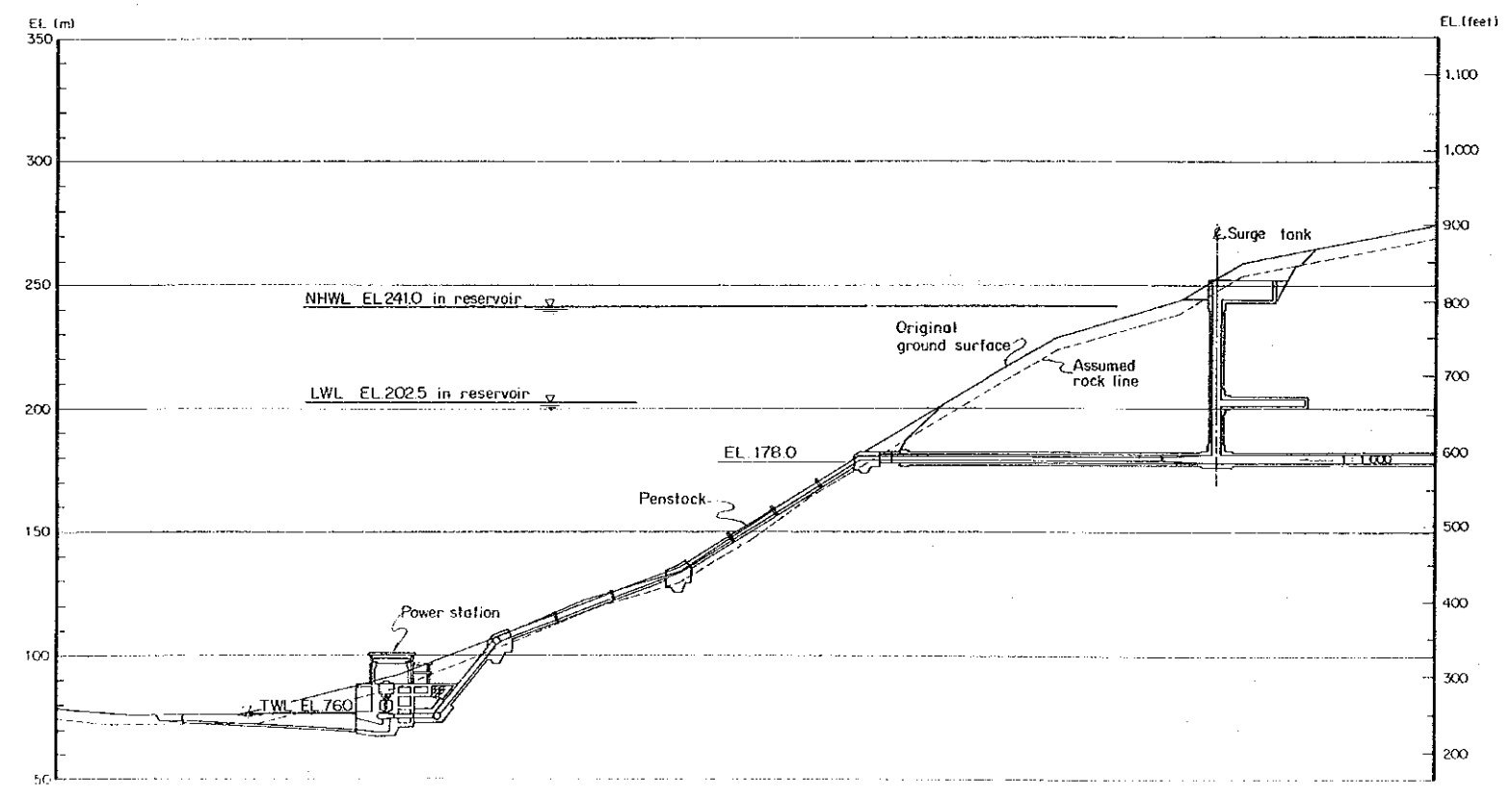
PROFILE OF OUTLET PORTION SCALE B
