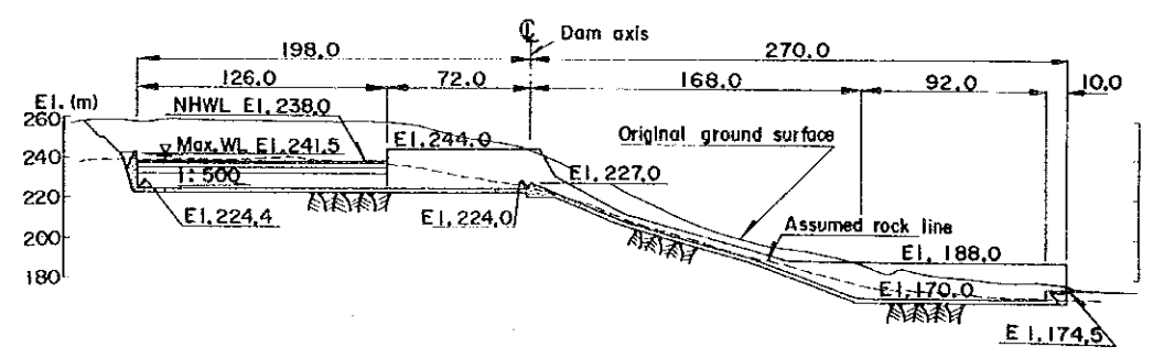
PROFILE OF SPILLWAY SCALE B
