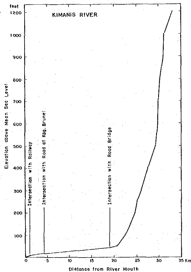
Fig. 6 River Profile (3/4)
