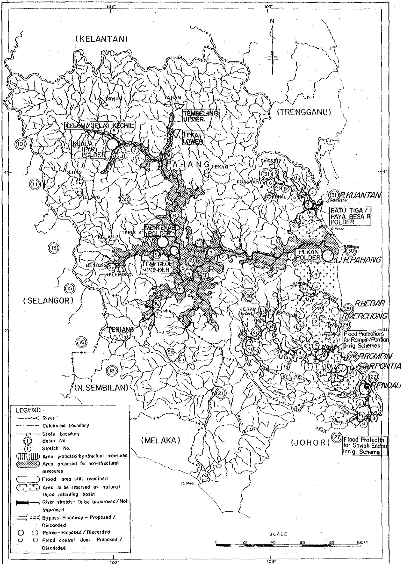
Fig. 9 Flood Mitigation Alternatives, Alternative F2
