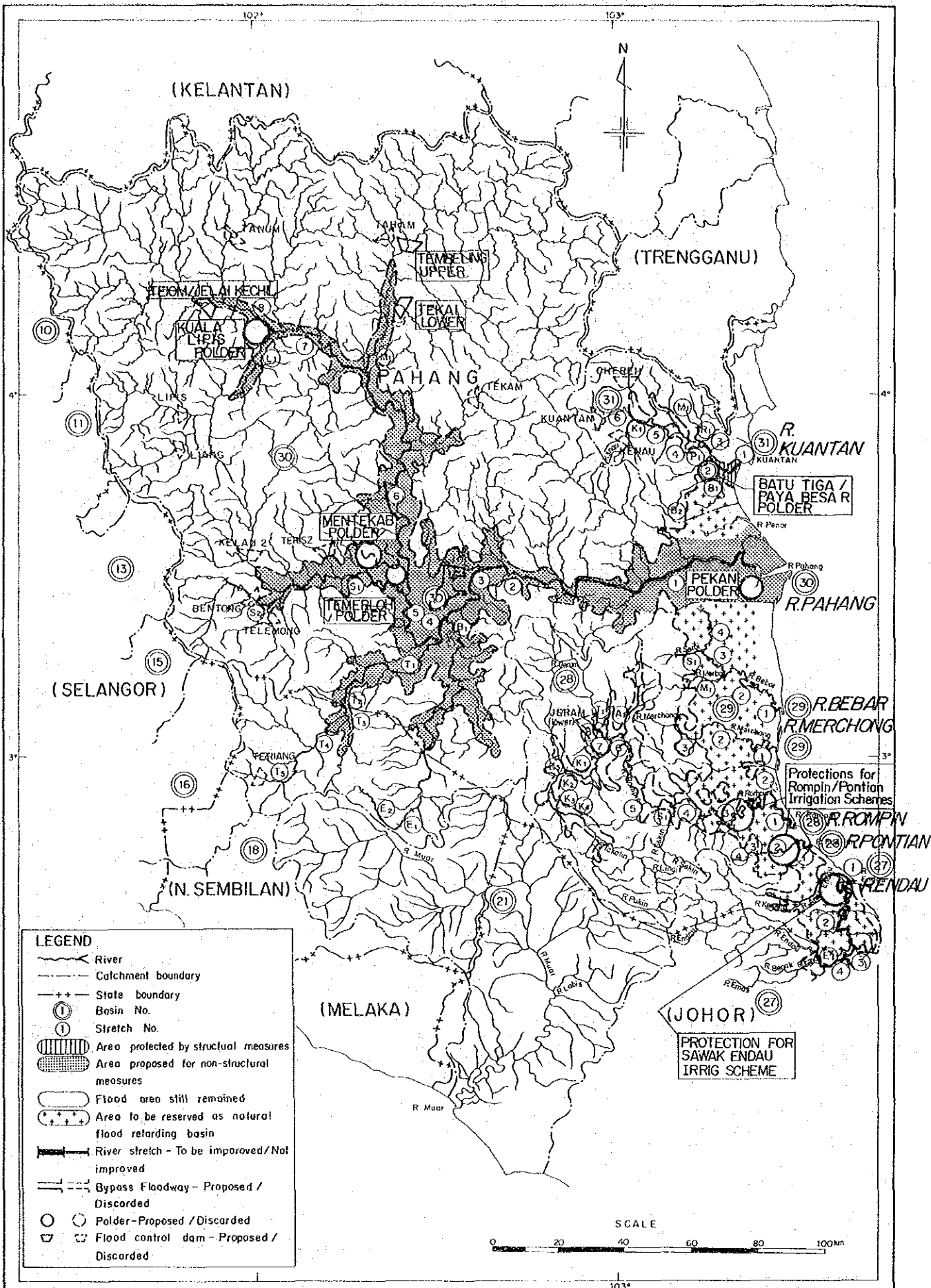
Fig.10 Flood Mitigation Alternatives, Alternative F 3
