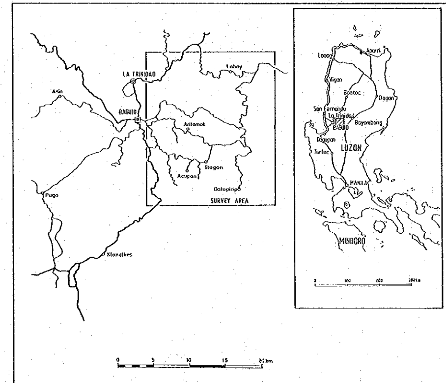
Fig.II-3-2 Route Map of Leveling Survey
