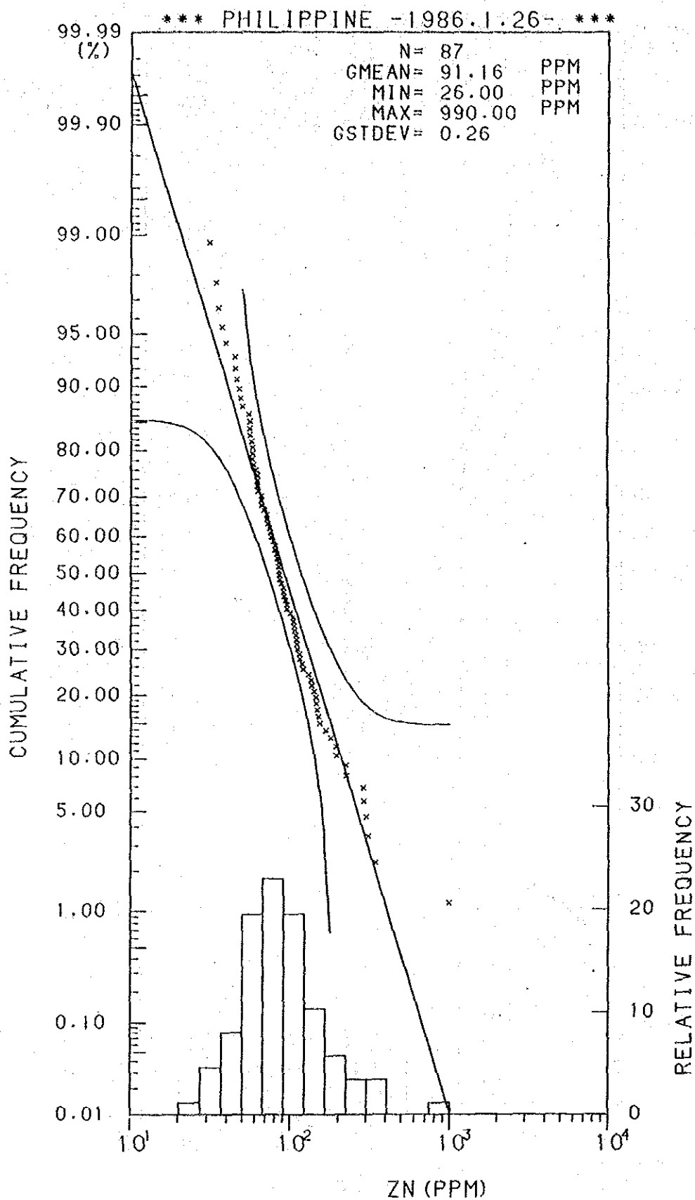
Histogram and Cumulative Frequency Curve of Zn content in Lithological Code; 0.5.
