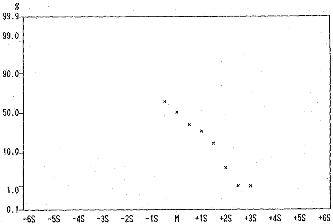
Cumulative Frequency Curve of As contents in Lithological Code; INR
