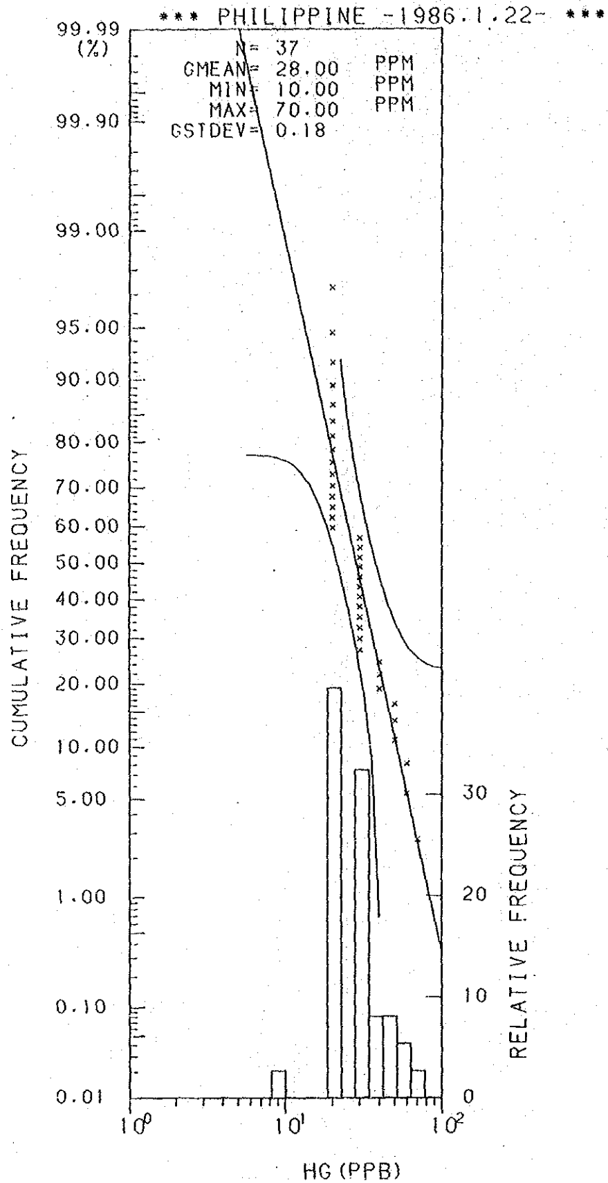
Histogram and Cumulative Frequency Curve of Hg Content in Lithological Code; 0.7.
