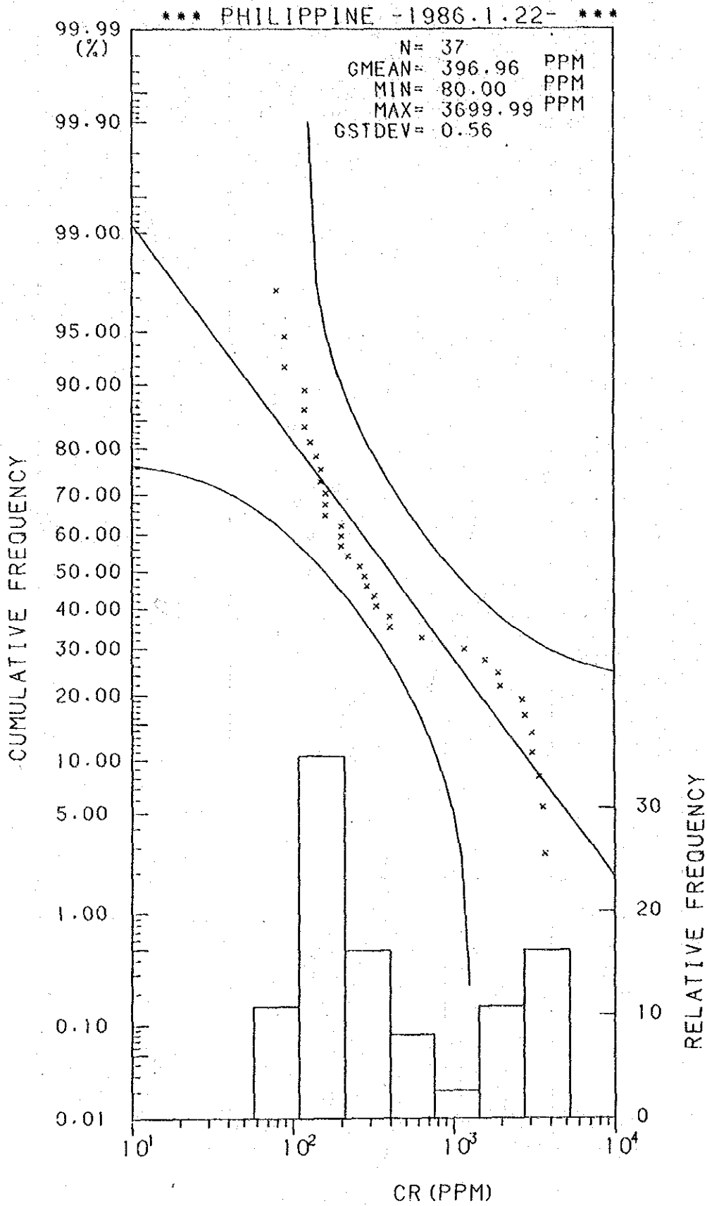
Histogram and Cumulative Frequency Curve of Cr Content in Lithological Code; 0.7.
