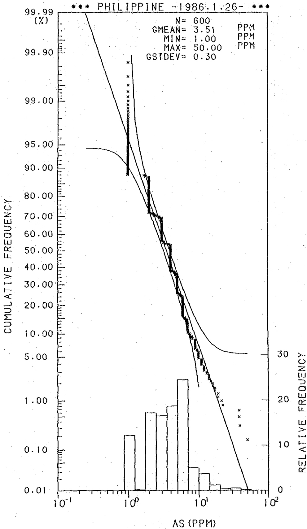
Histogram and Cumulative Frequency Curve of As content in Lithological Code; 0.2.
