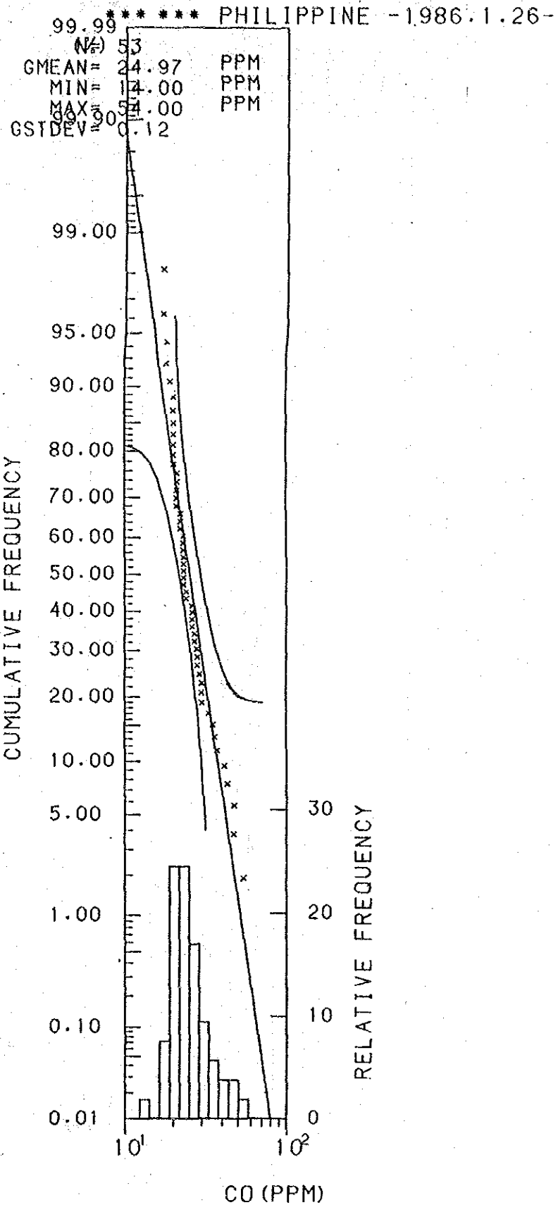
Histogram and Cumulative Frequency Curve of Co content in Lithological Code; 0.9.
