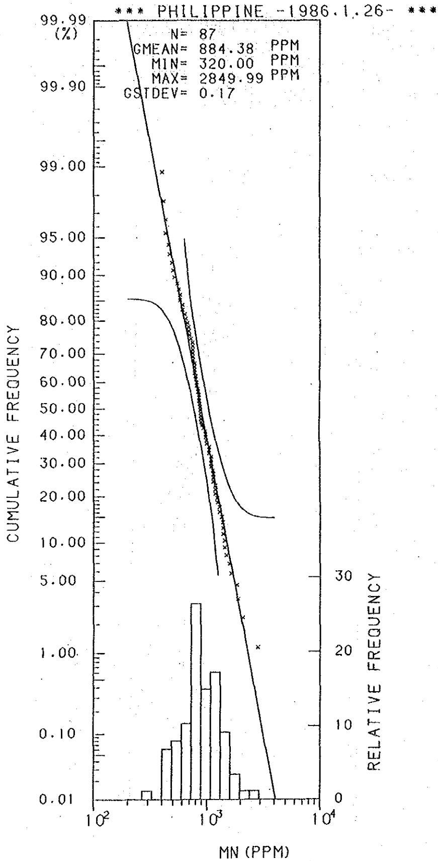
Histogram and Cumulative Frequency Curve of Mn content in Lithological Code; 0.5.
