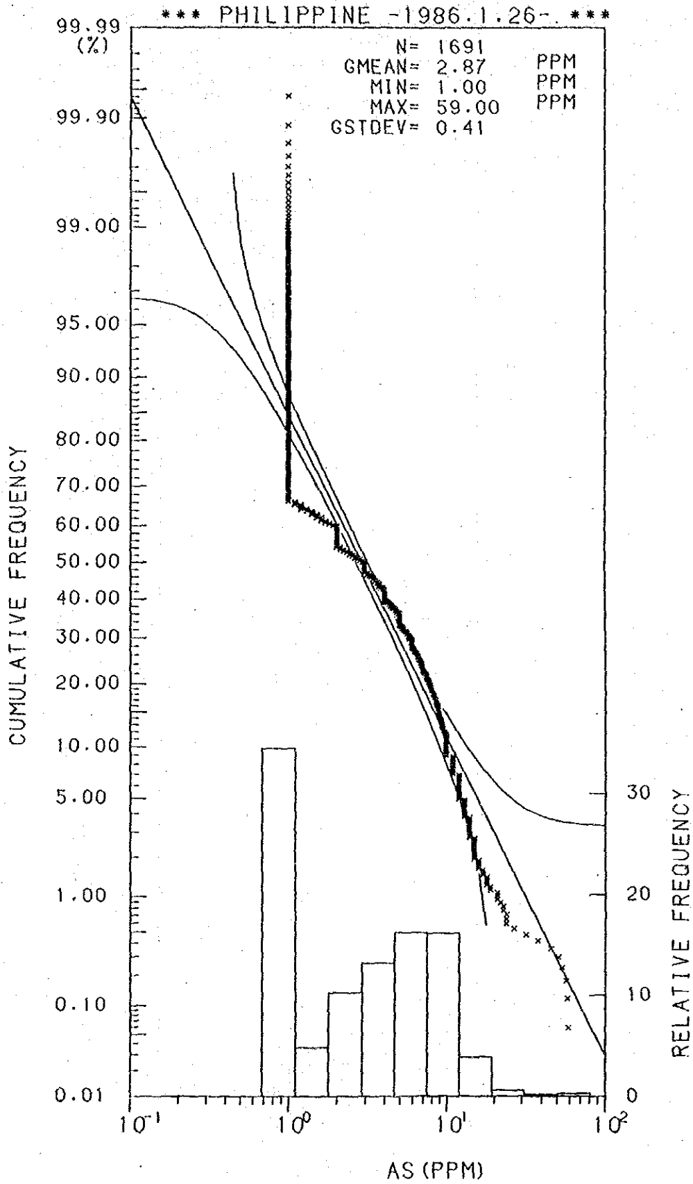
Histogram and Cumulative Frequency Curve of As content in Lithological Code; 0.3.
