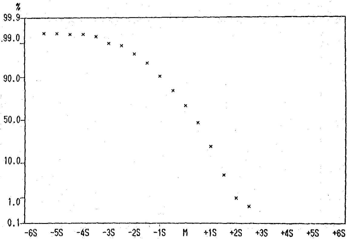
Cumulative Frequency Curve of Mn content in all Samples.
