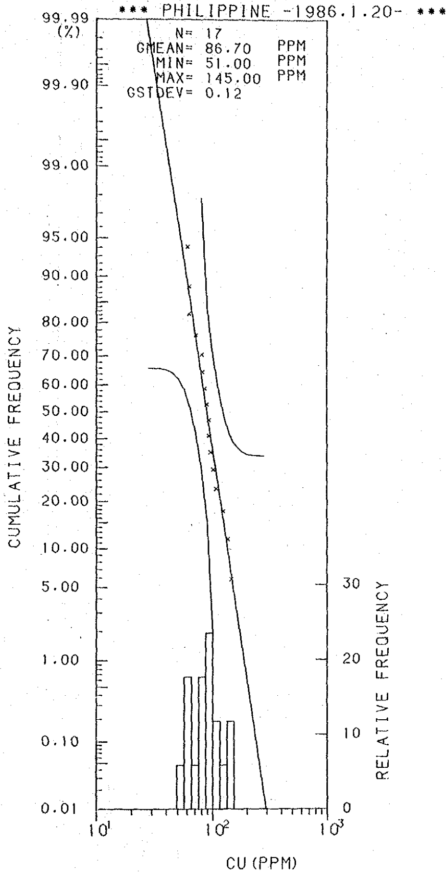
Histogram and Cumulative Frequency Curve of Cu Content in Lithological Code; 0.4.
