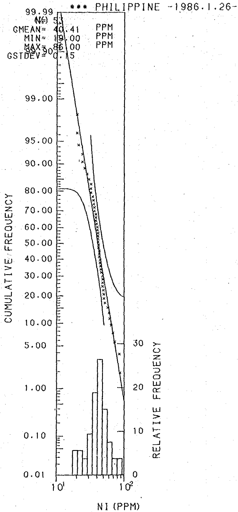
Histogram and Cumulative Frequency Curve of Ni content in Lithological Code; 0.9.
