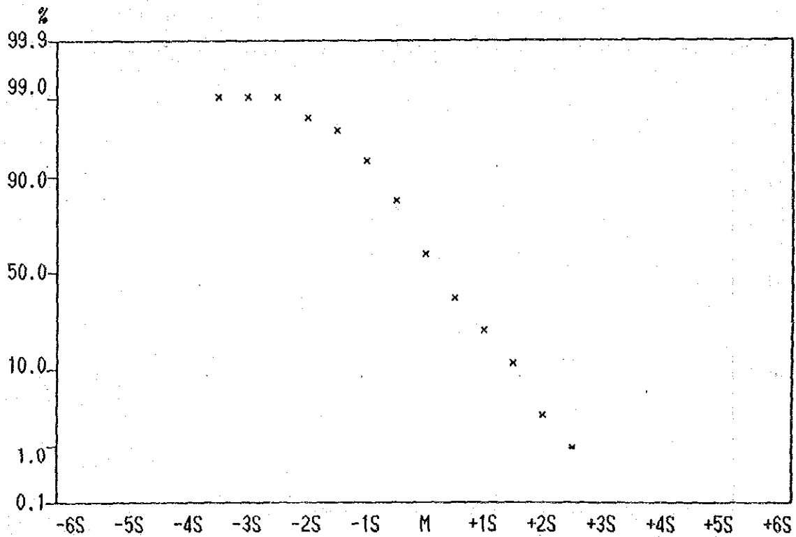
Cumulative Frequency Curve of Mn contents in Lithological Code; INR
