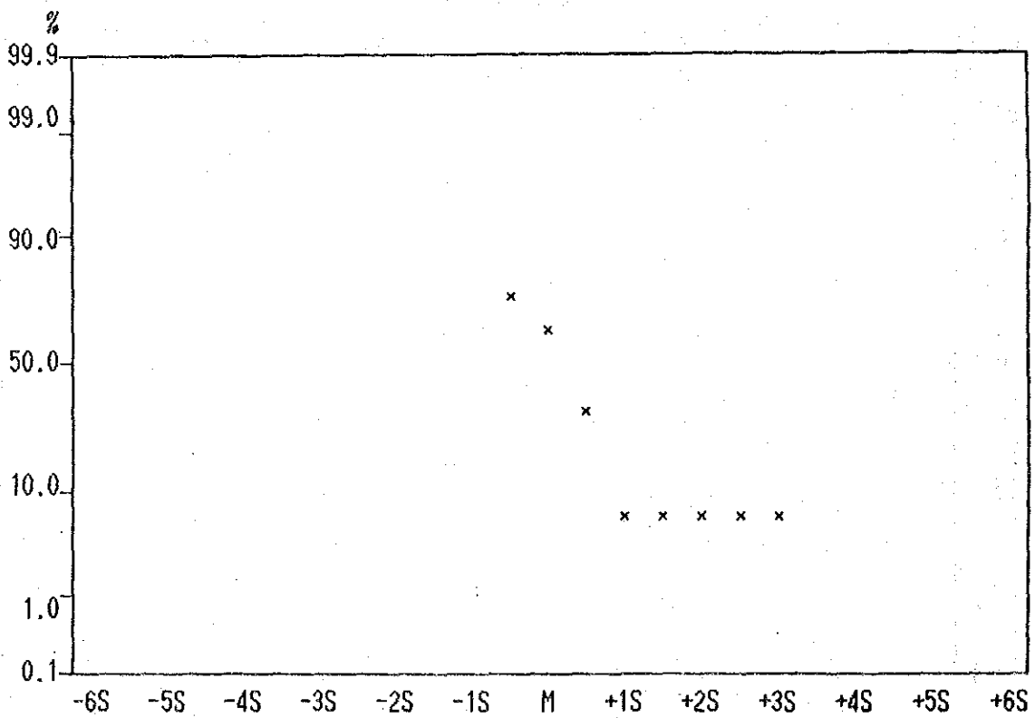
Cumulative Frequency Curve of Ni contents in Lithological Code; KPL
