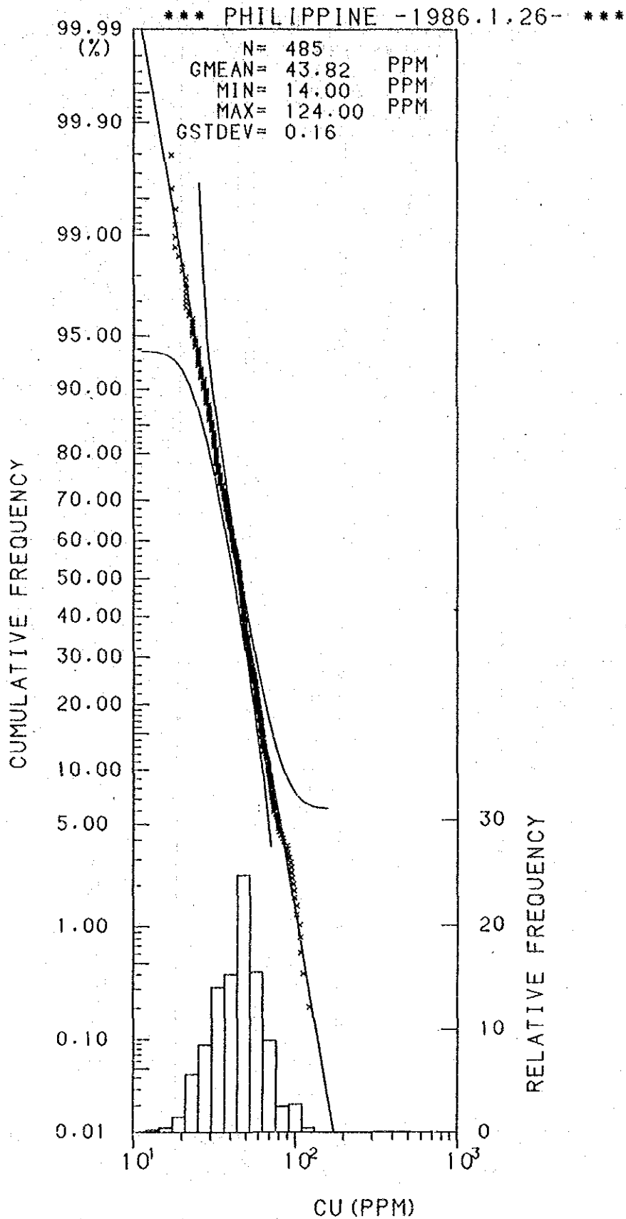
Histogram and Cumulative Frequency Curve of Cu content in Lithological Code; 0.1.
