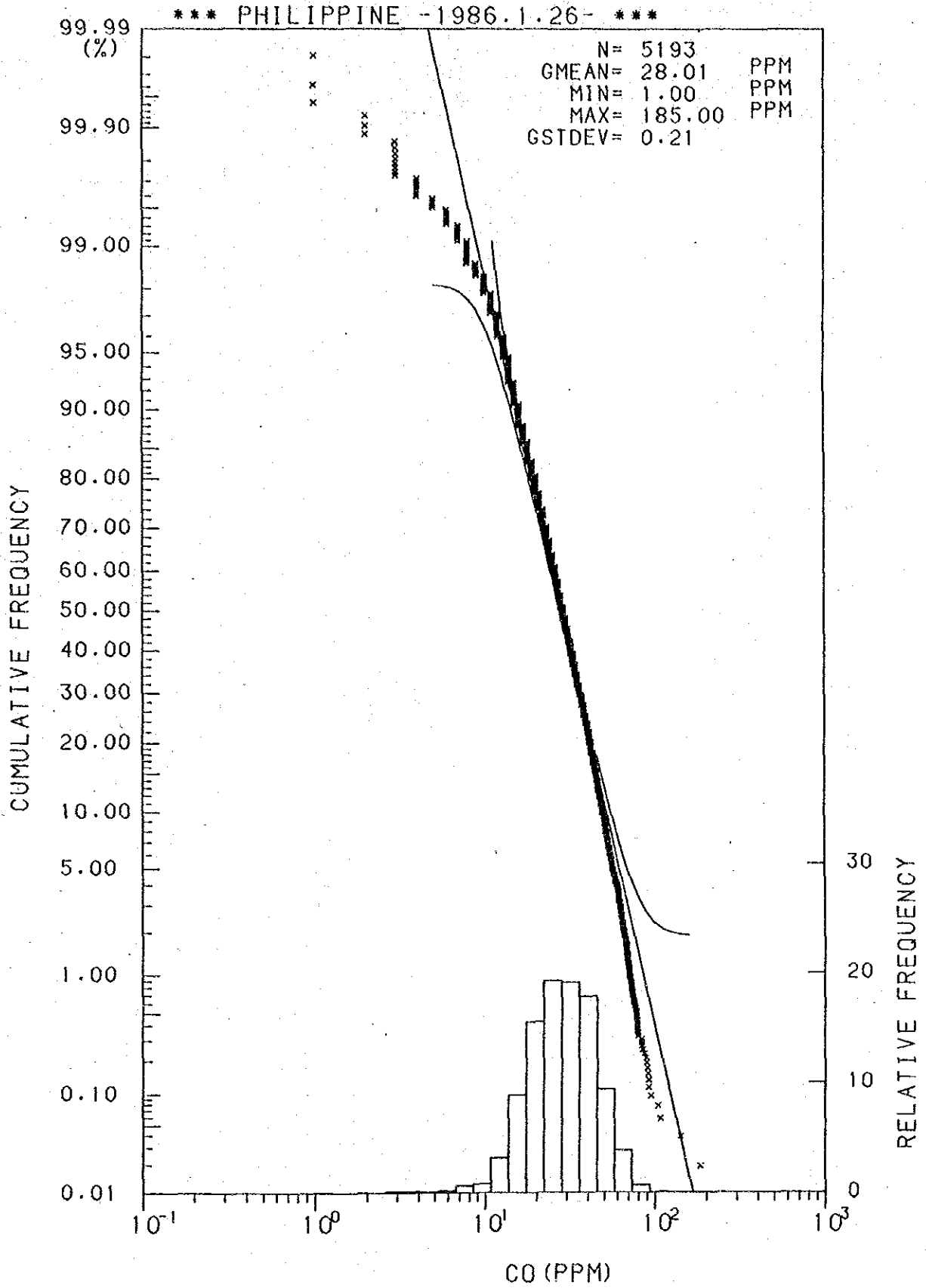
Histogram and Cumulative Frequency Curve of Co content in All Samples.
