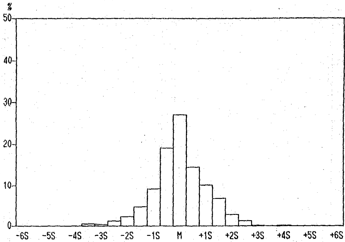
Histograms of Ni content in all Samples.
