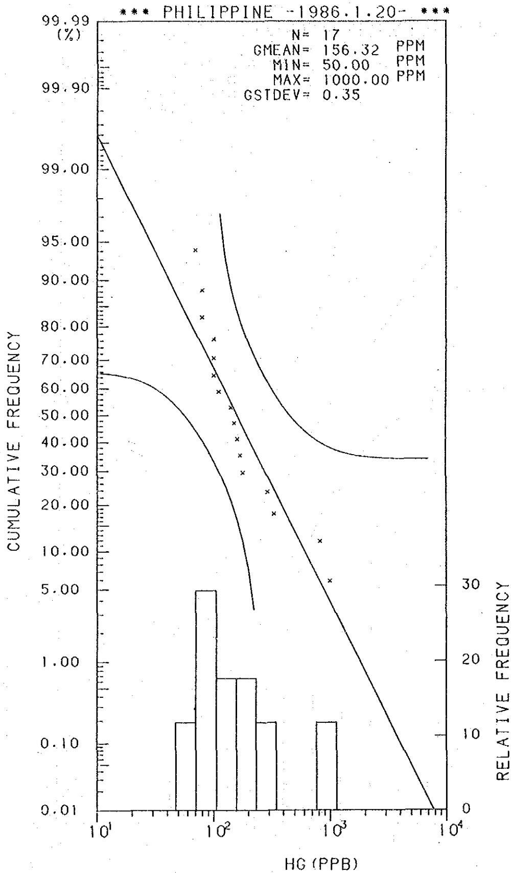
Histogram and Cumulative Frequency Curve of Hg Content in Lithological Code; 0.4.
