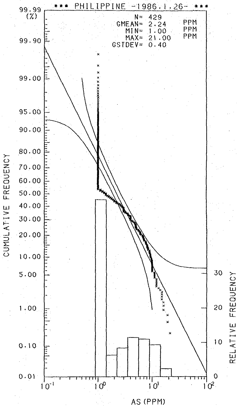
Histogram and Cumulative Frequency Curve of As content in Lithological Code; 0.8.
