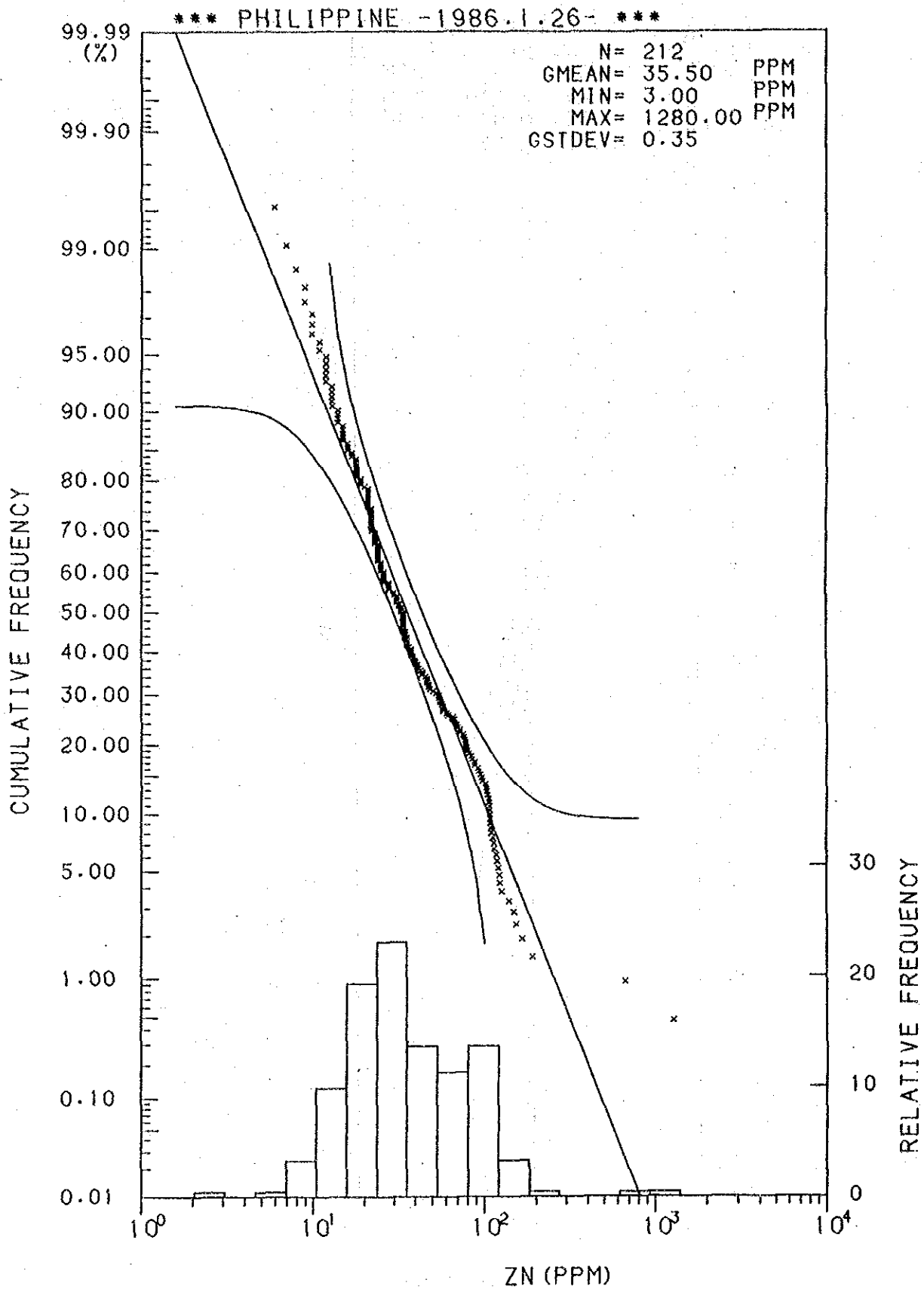
Histogram and Cumulative Frequency Curve of Zn content in Lithological Code; 0.7.
