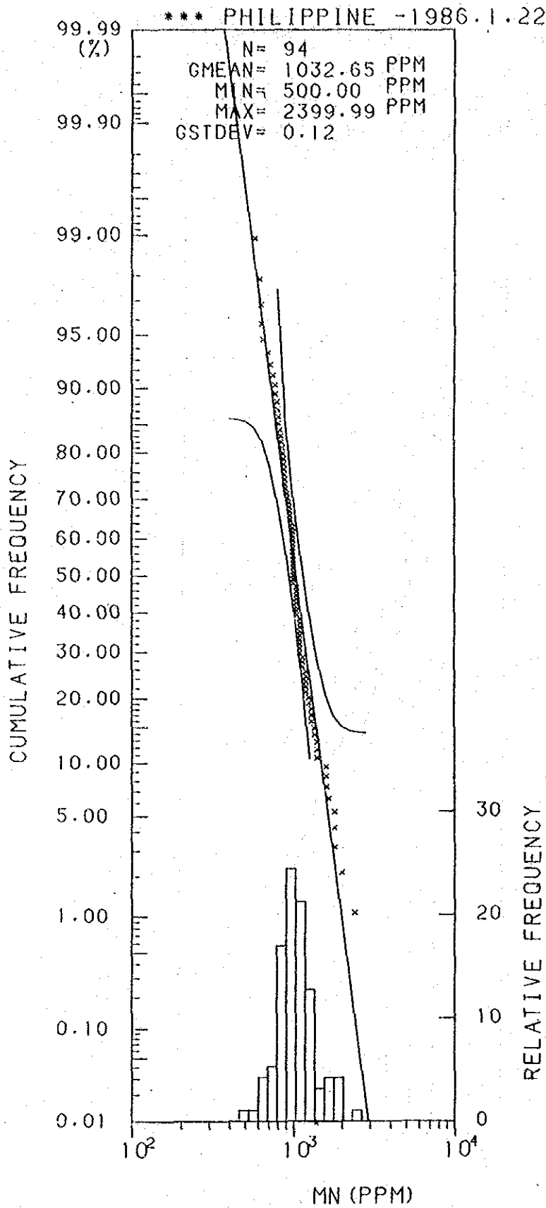
Histogram and Cumulative Frequency Curve of Mn Content in Lithological Code; 0.5.
