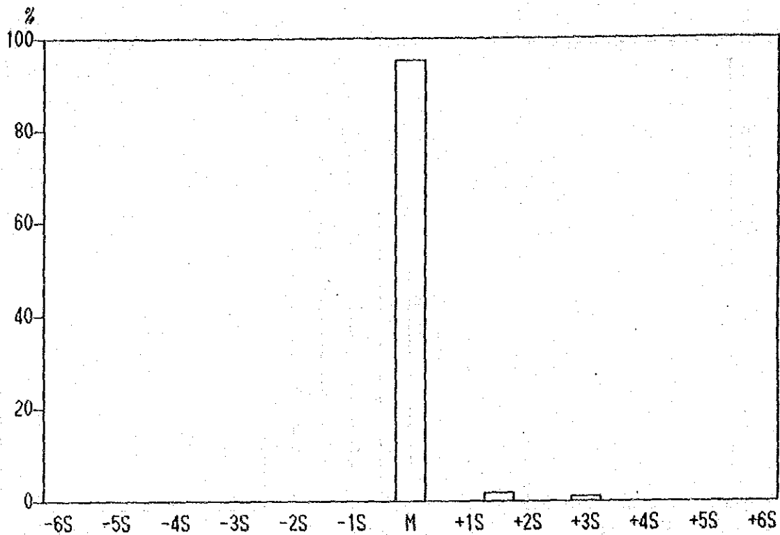
Histogram of Mo contents in Lithological Code; INR
