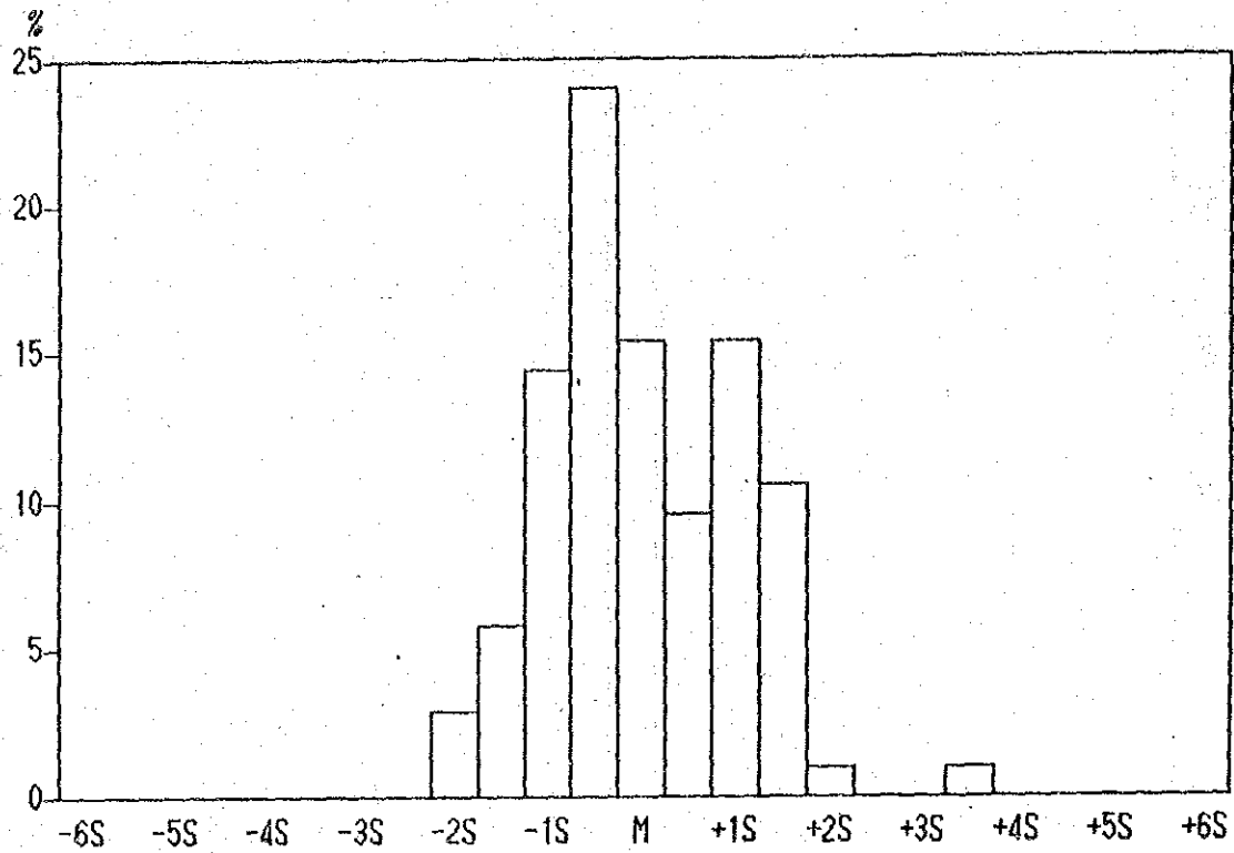
Histogram of Zn contents in Lithological Code; INR
