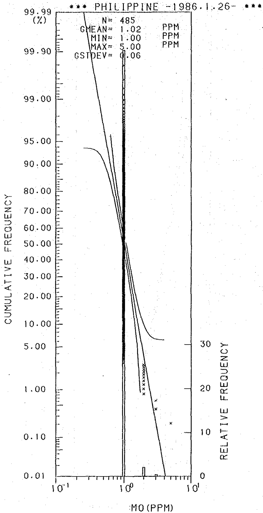
Histogram and Cumulative Frequency Curve of Mo content in Lithological Code; 0.1.
