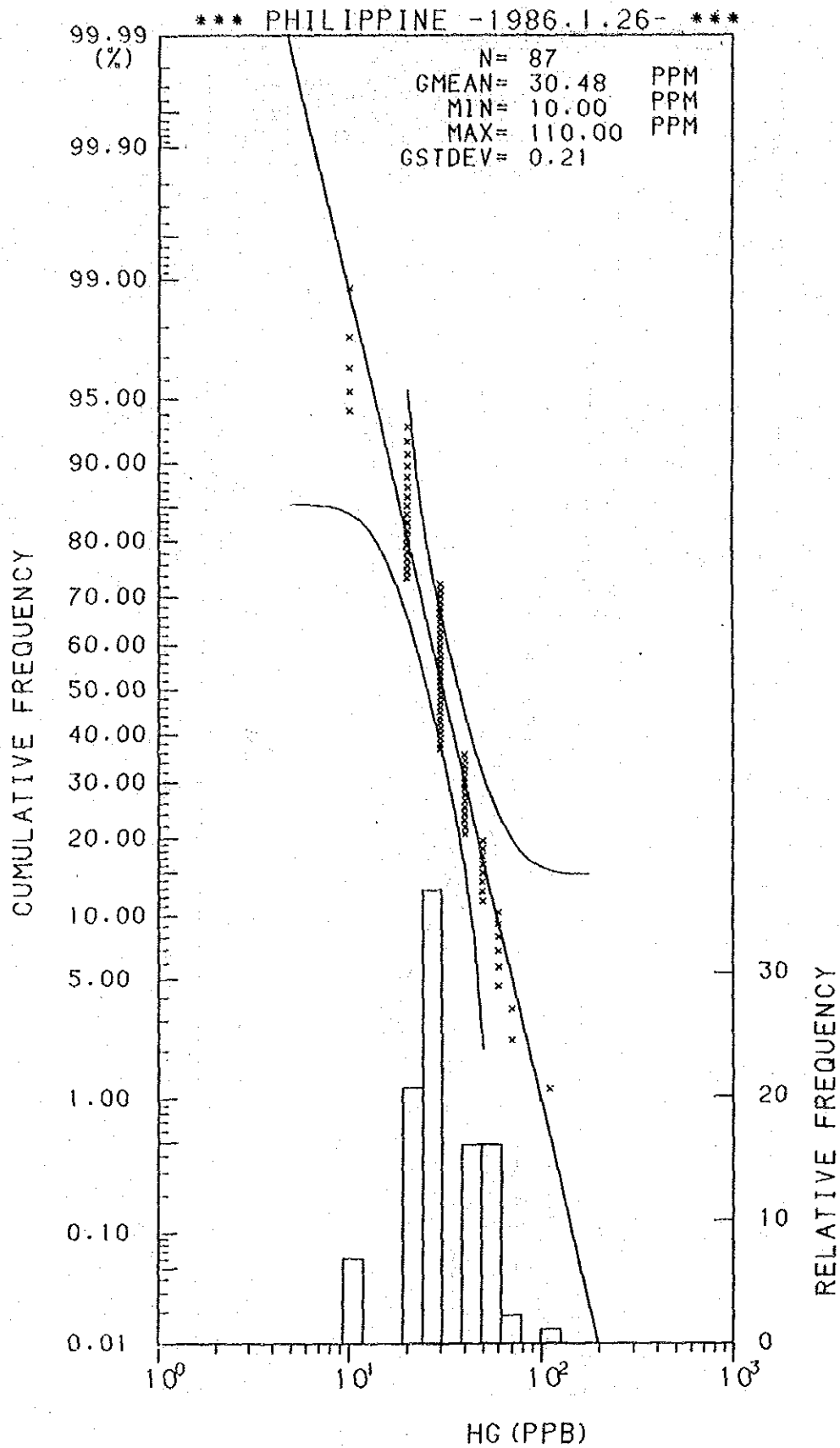
Histogram and Cumulative Frequency Curve of Hg content in Lithological Code; 0.5.
