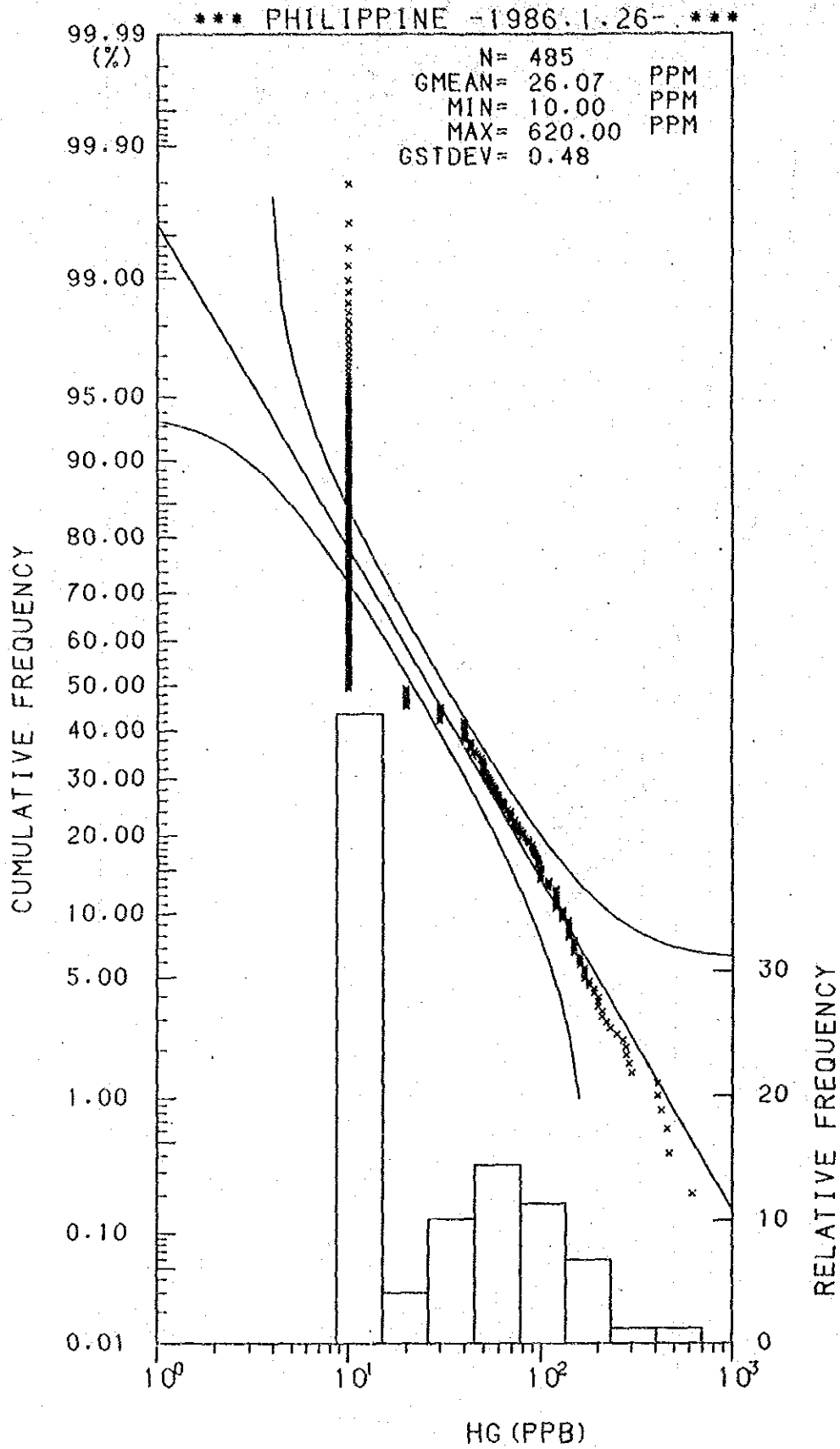
Histogram and Cumulative Frequency Curve of Hg content in Lithological Code; 0.1.
