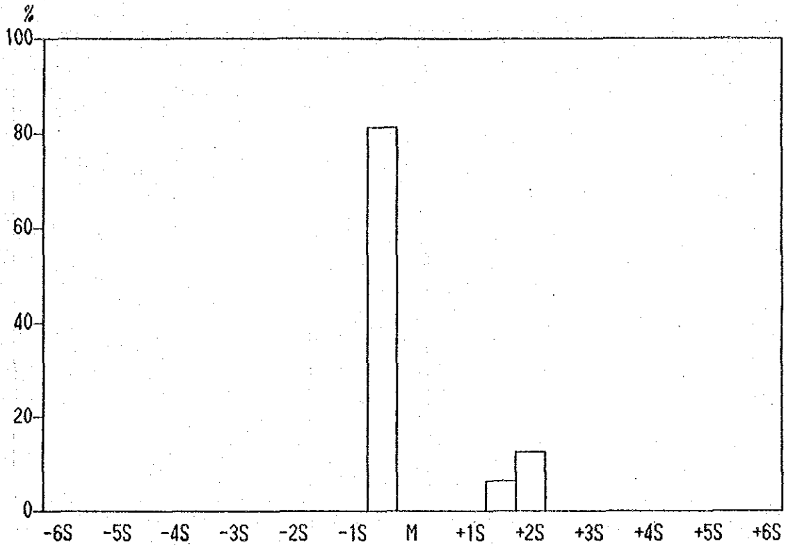
Histogram of Pb contents in Lithological Code; KPL
