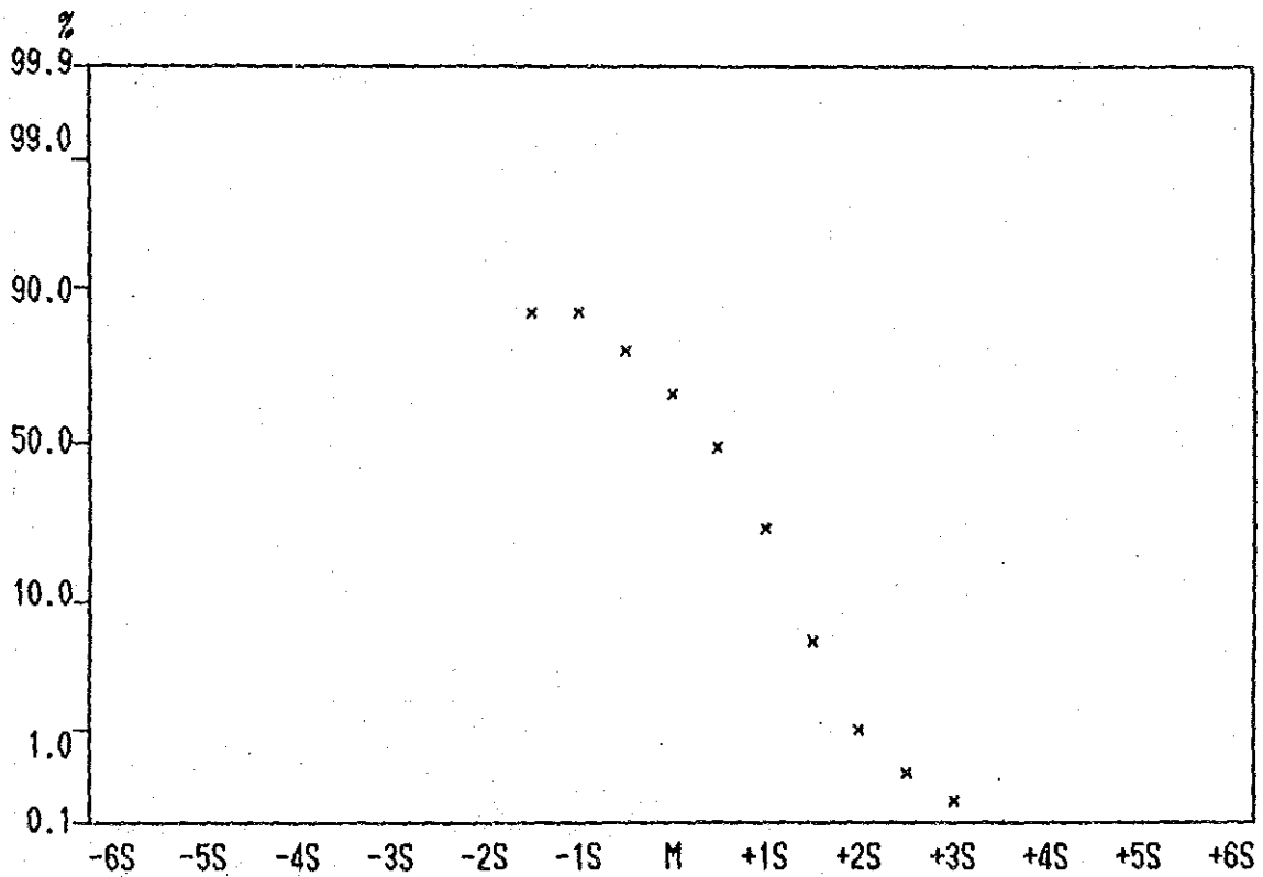
Cumulative Frequency Curve of As content in all Samples.
