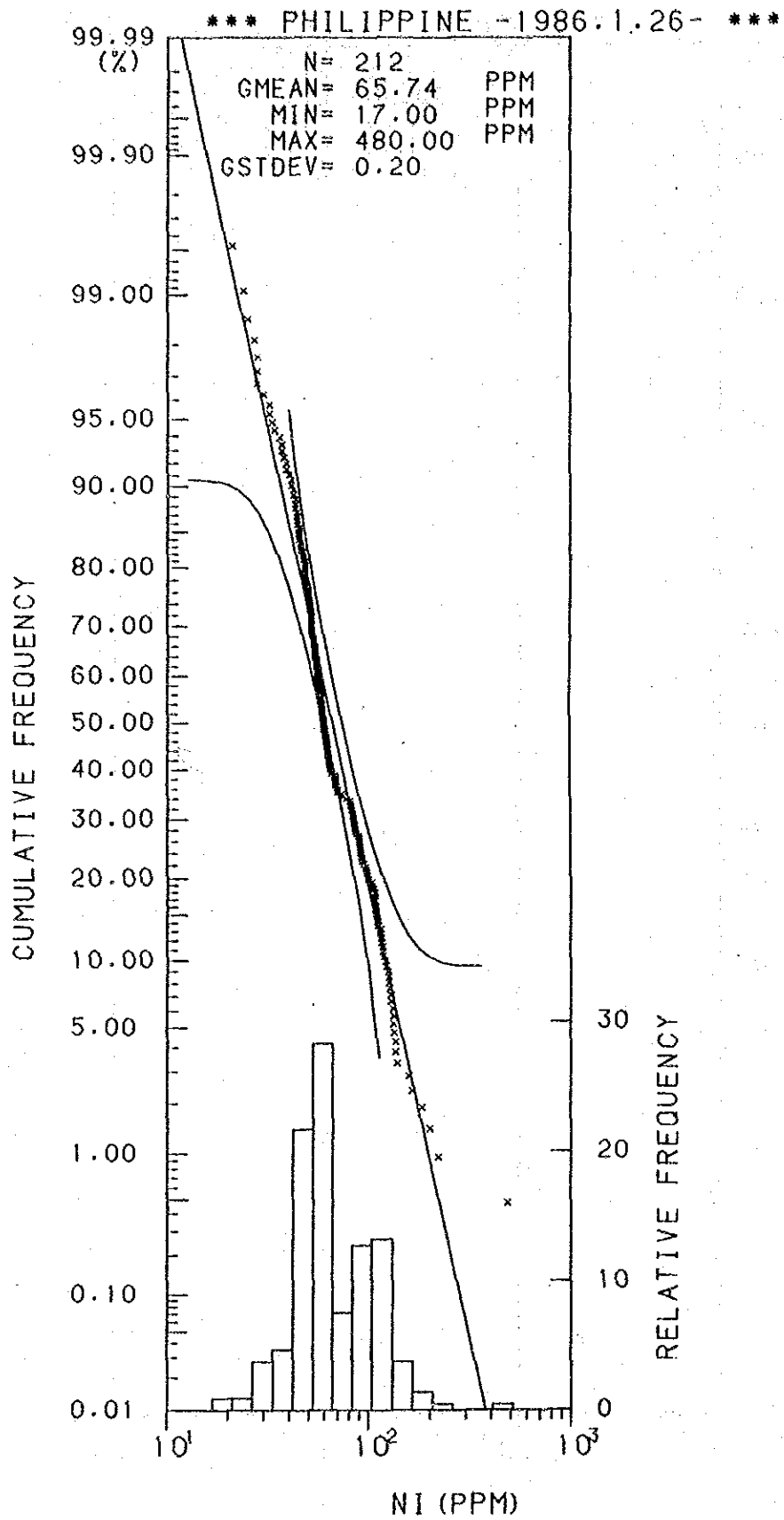
Histogram and Cumulative Frequency Curve of Ni content in Lithological Code; 0.7.
