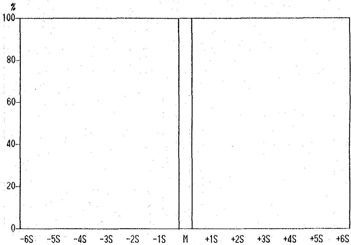
Histogram of Ag contents in Lithological Code; KPL
