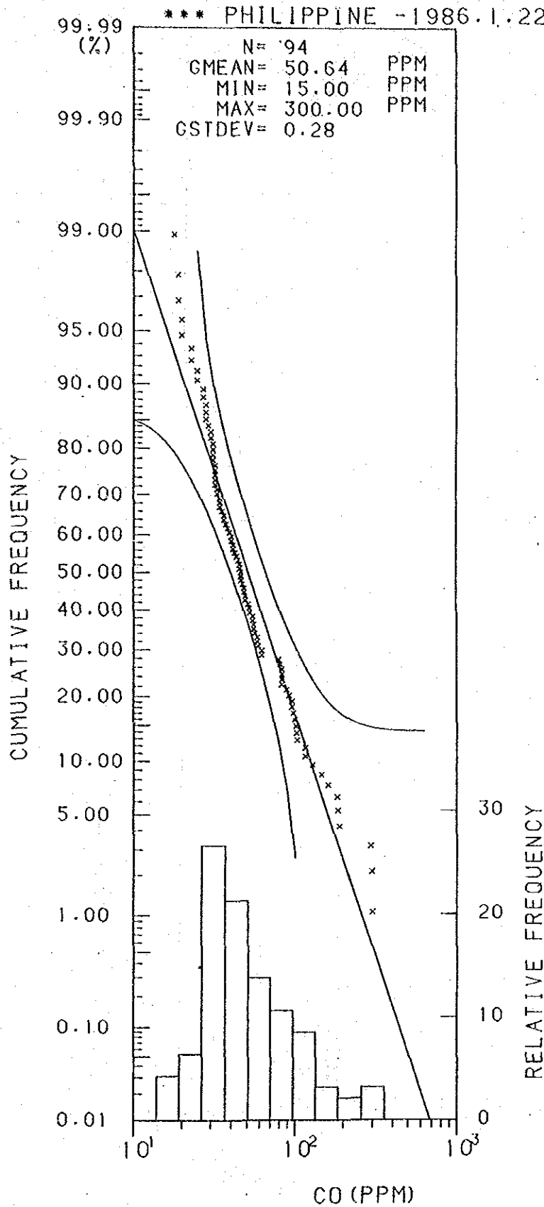
Histogram and Cumulative Frequency Curve of Co Content in Lithological Code; 0.5.
