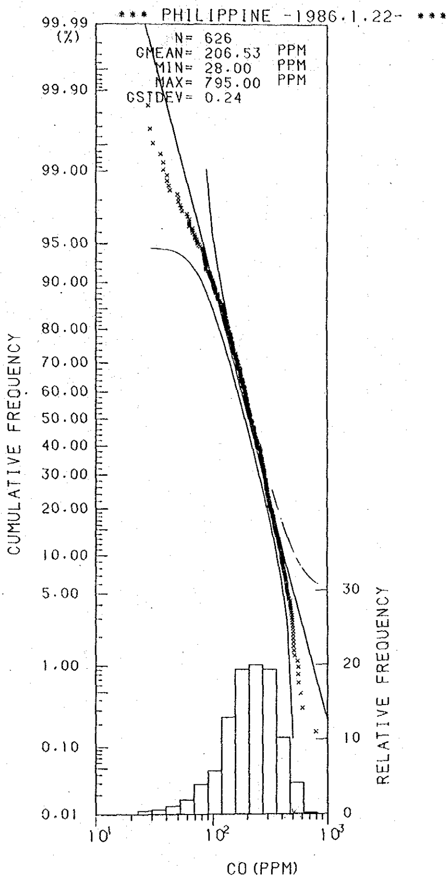
Histogram and Cumulative Frequency Curve of Co Content in Lithological Code; 0.6.
