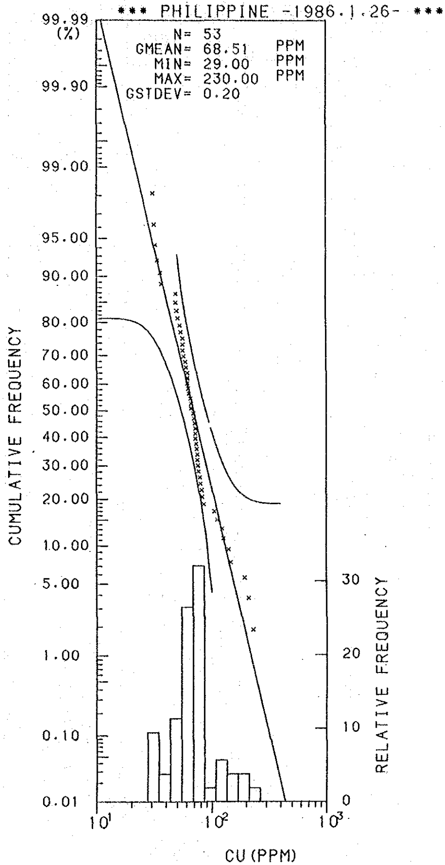
Histogram and Cumulative Frequency Curve of Cu content in Lithological Code; 0.9.
