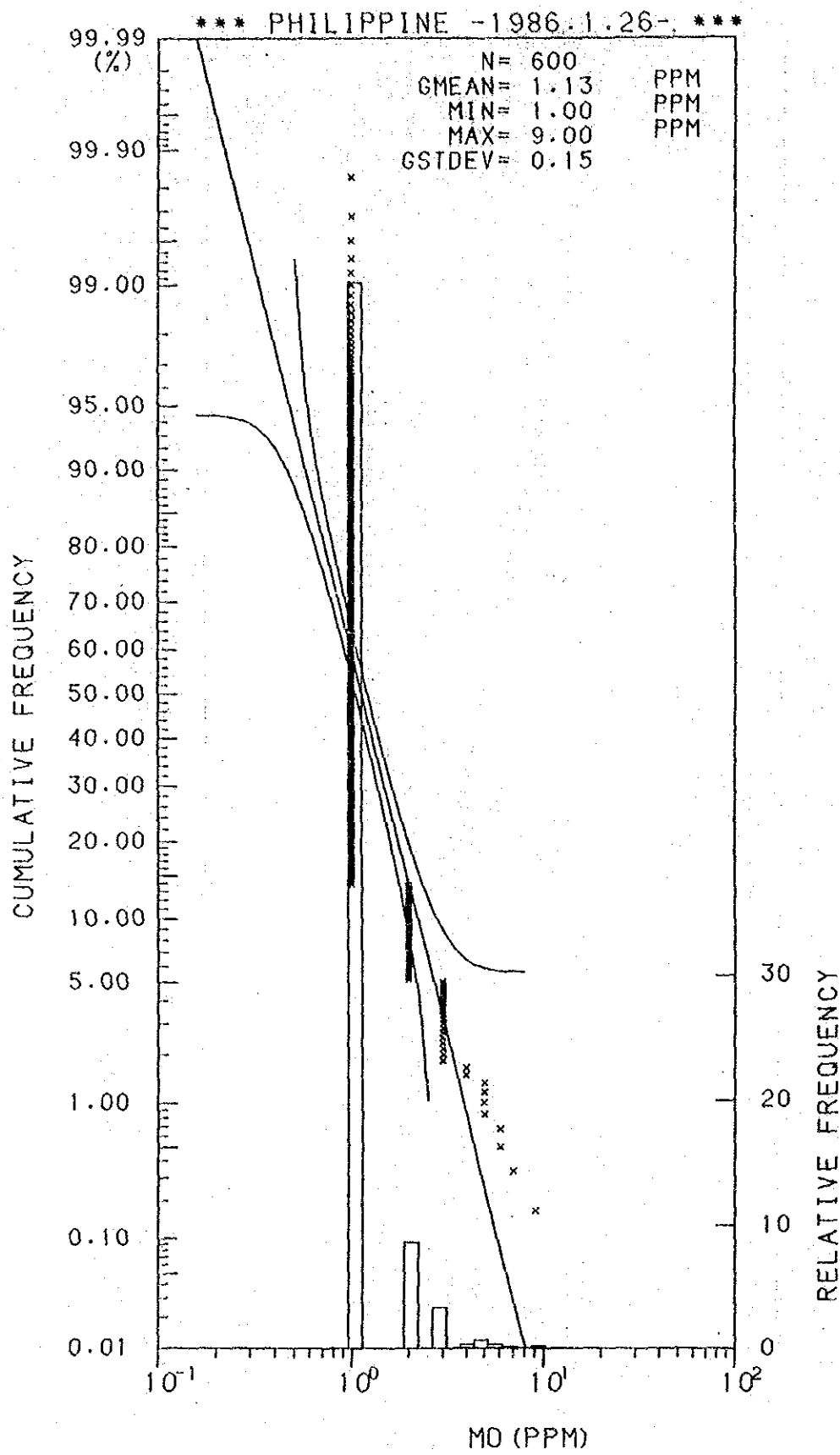
Histogram and Cumulative Frequency Curve of Mo content in Lithological Code; 0.2.
