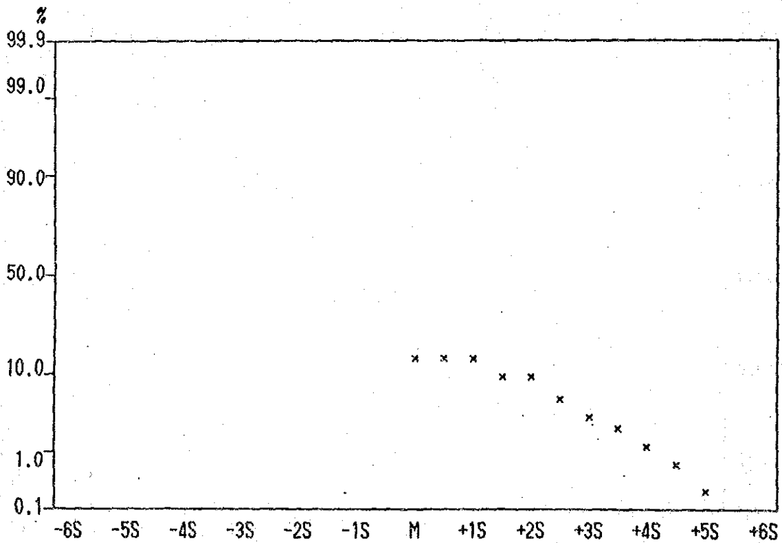
Cumulative Frequency Curve of Mo content in all Samples.
