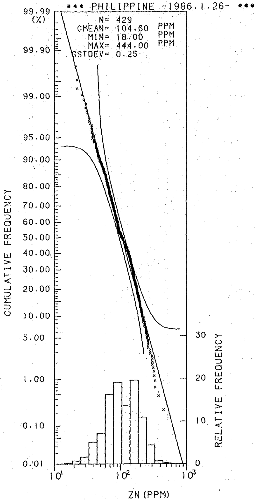
Histogram and Cumulative Frequency Curve of Zn content in Lithological Code; 0.8.
