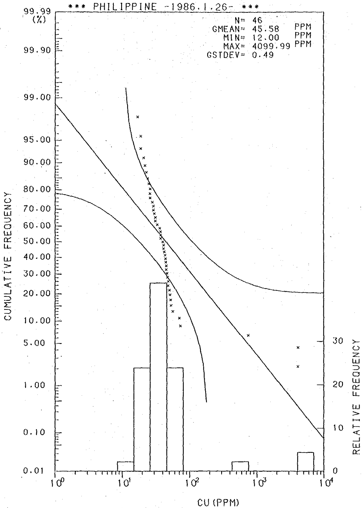
Histogram and Cumulative Frequency Curve of Cu content in Lithological Code; 0.6.
