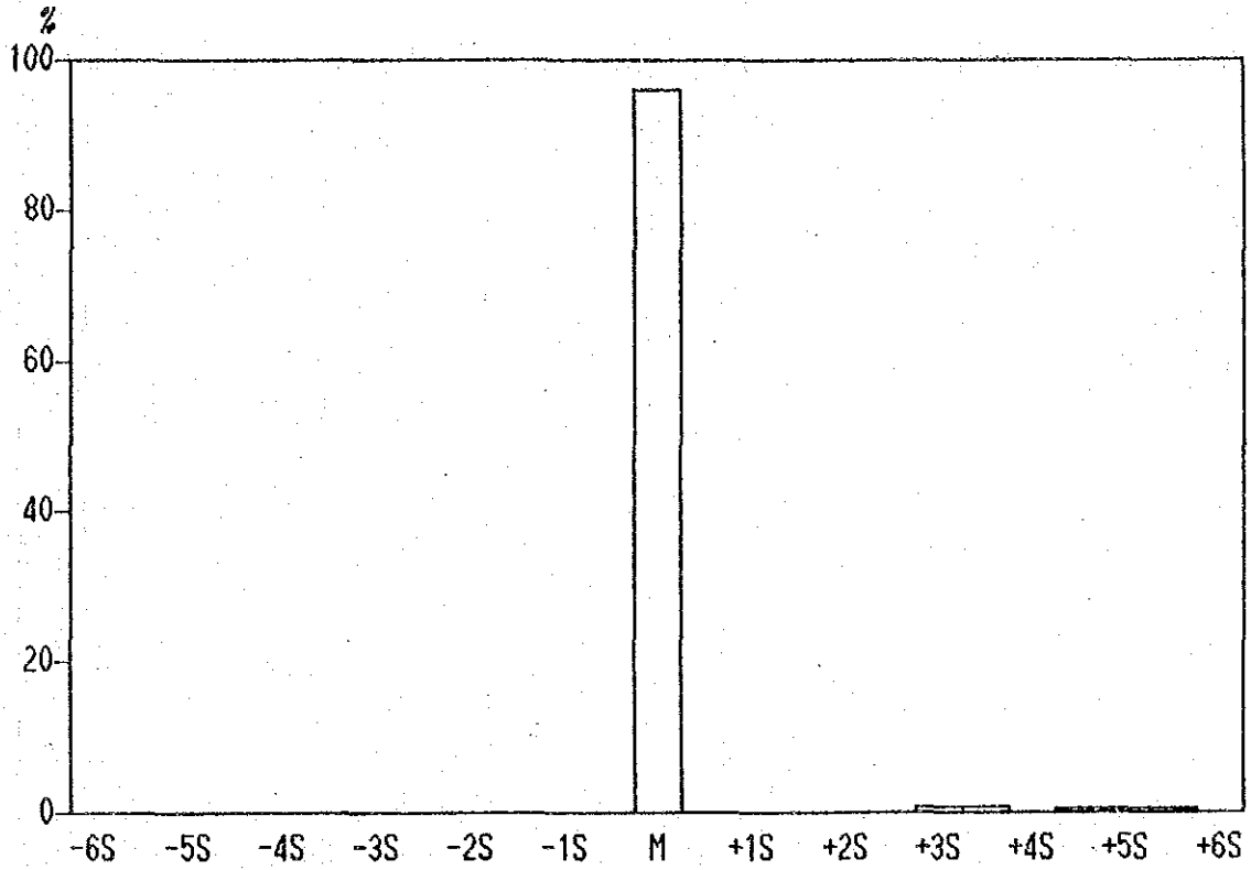
Histogram of Pb contents in Lithological Code; KPS
