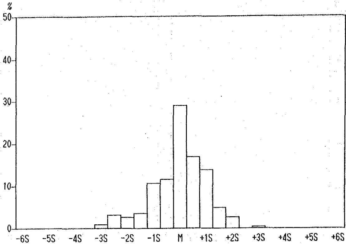
Histogram of Ni contents in Lithological Code; KPS
