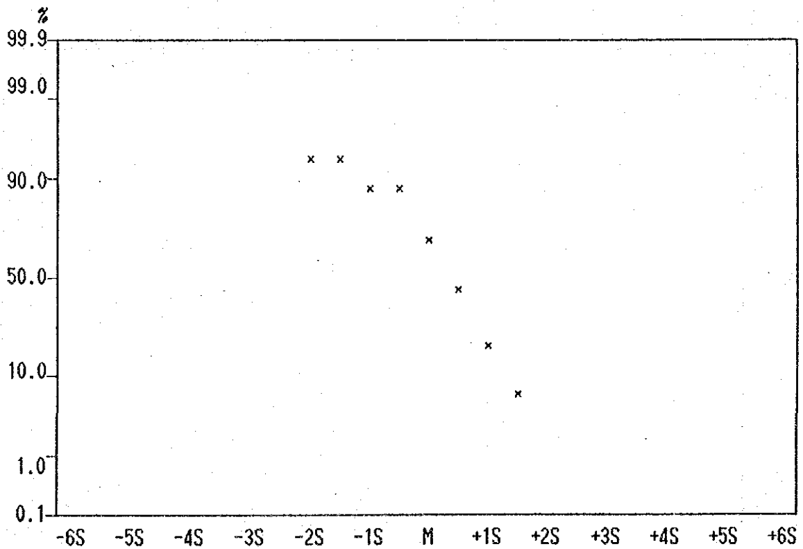
Cumulative Frequency Curve of Cu contents in Lithological Code; KPL
