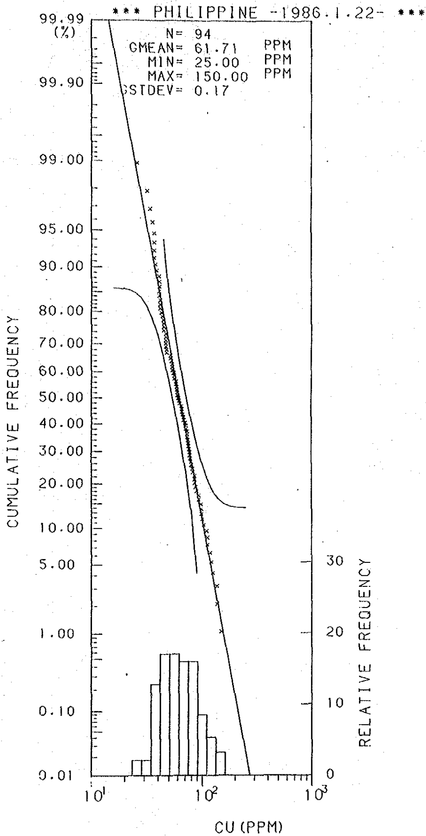
Histogram and Cumulative Frequency Curve of Cu Content in Lithological Code; 0.5.
