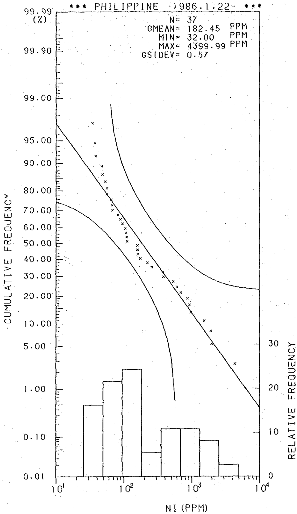
Histogram and Cumulative Frequency Curve of Ni Content in Lithological Code; 0.7.
