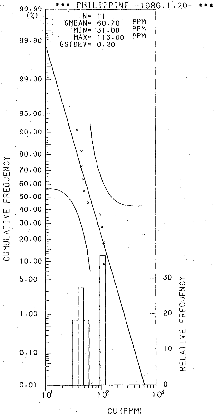
Histogram and Cumulative Frequency Curve of Cu Content in Lithological Code; 0.2.
