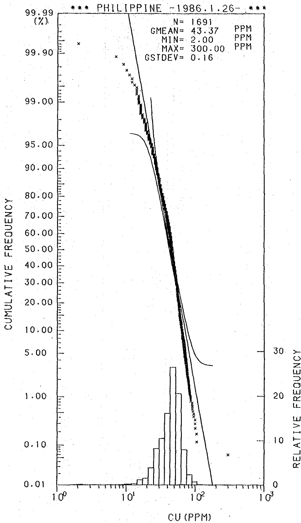
Histogram and Cumulative Frequency Curve of Cu content in Lithological Code; 0.3.
