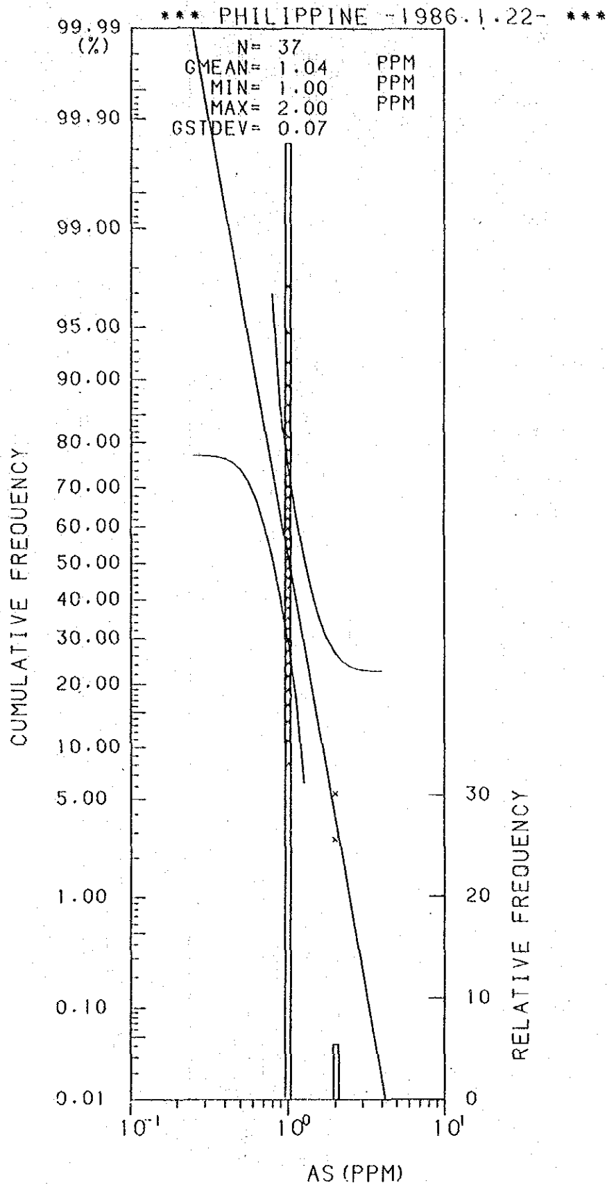
Histogram and Cumulative Frequency Curve of As Content in Lithological Code; 0.7.
