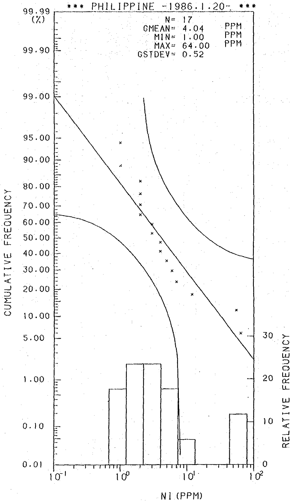
Histogram and Cumulative Frequency Curve of Ni Content in Lithological Code; 0.4.
