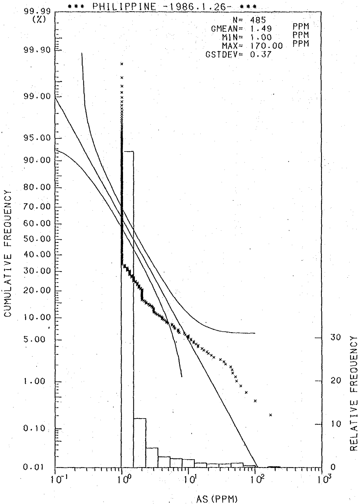
Histogram and Cumulative Frequency Curve of As content in Lithological Code; 0.1.
