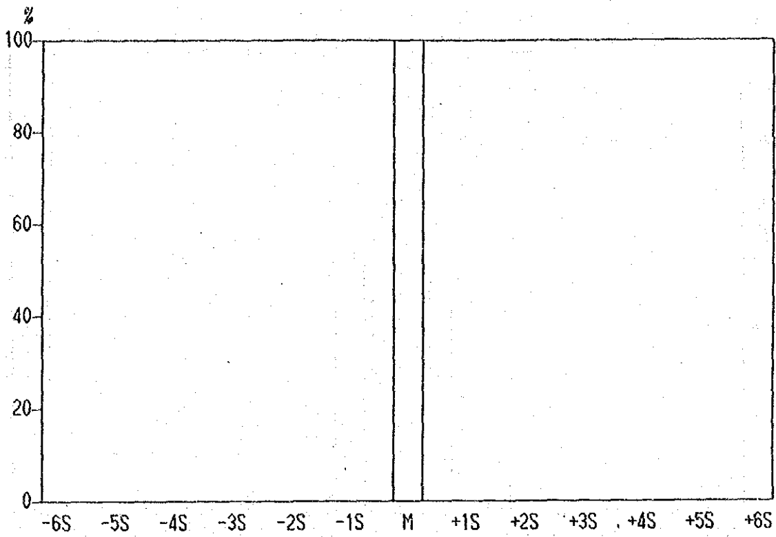
Histogram of Ag contents in Lithological Code; INR
