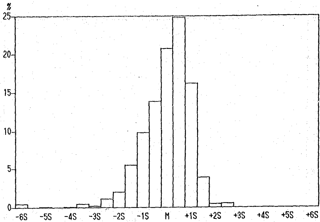
Histograms of Mn content in all Samples.
