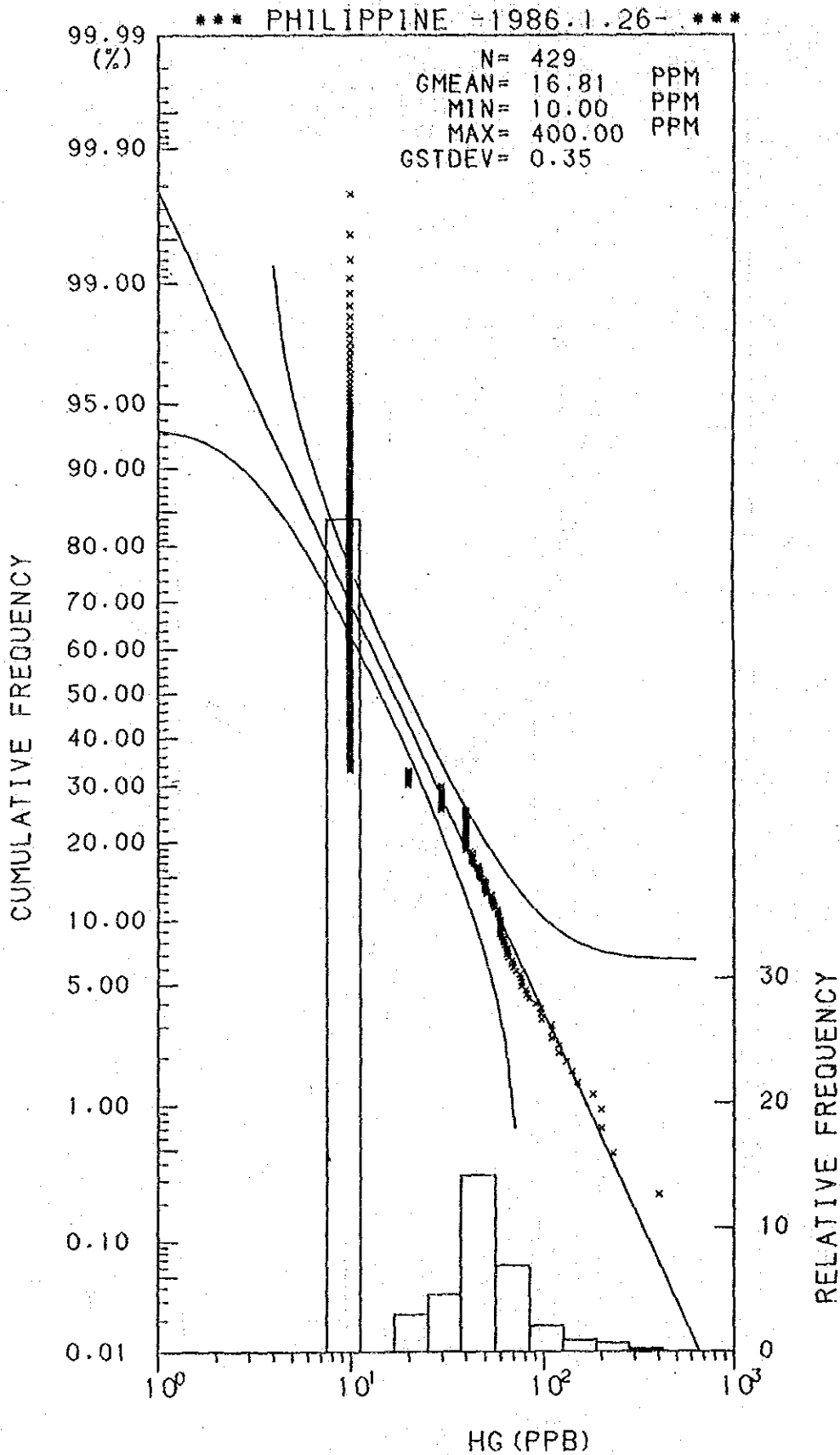
Histogram and Cumulative Frequency Curve of Hg content in Lithological Code; 0.8.
