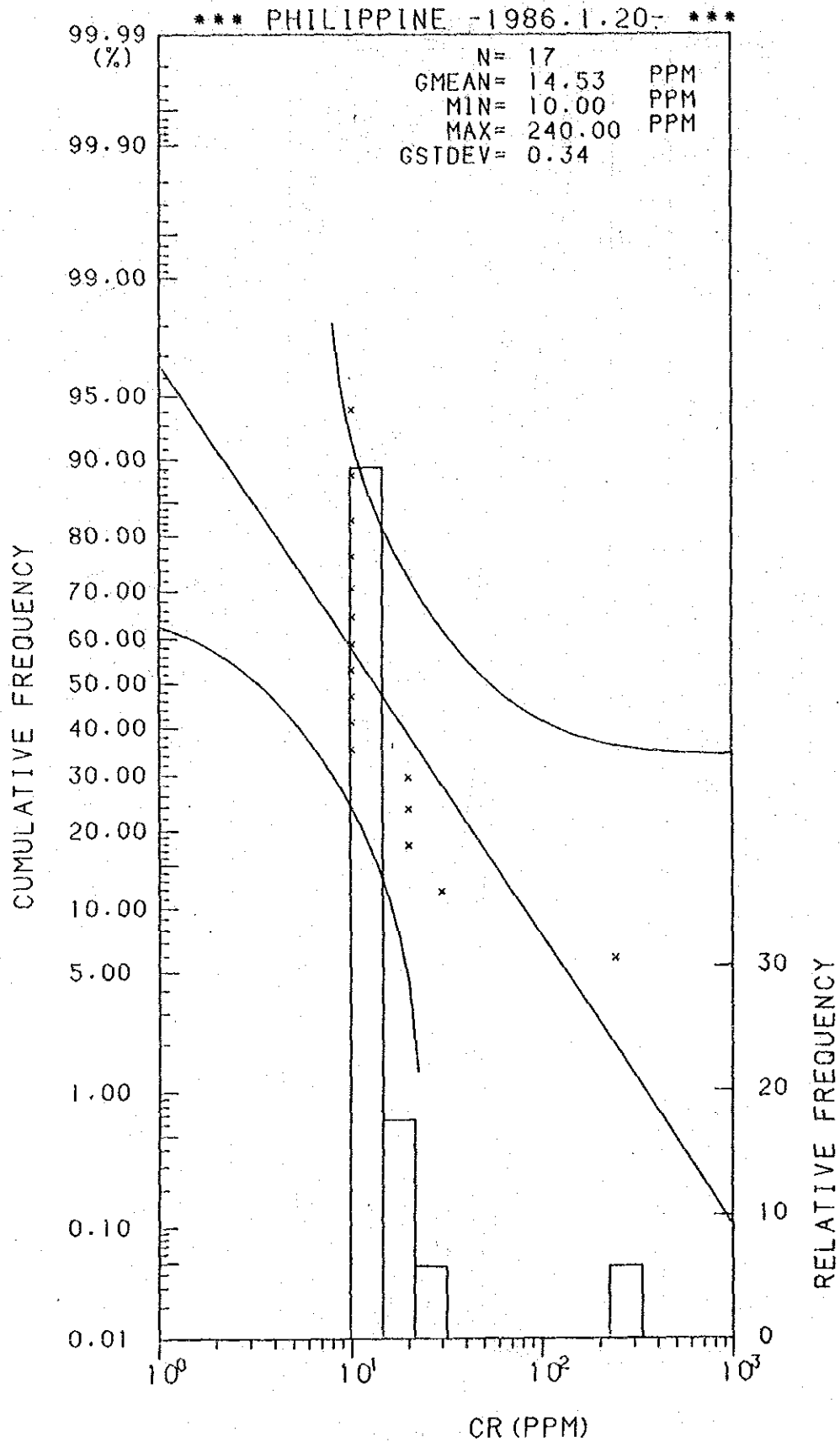
Histogram and Cumulative Frequency Curve of Cr Content in Lithological Code; 0.4.
