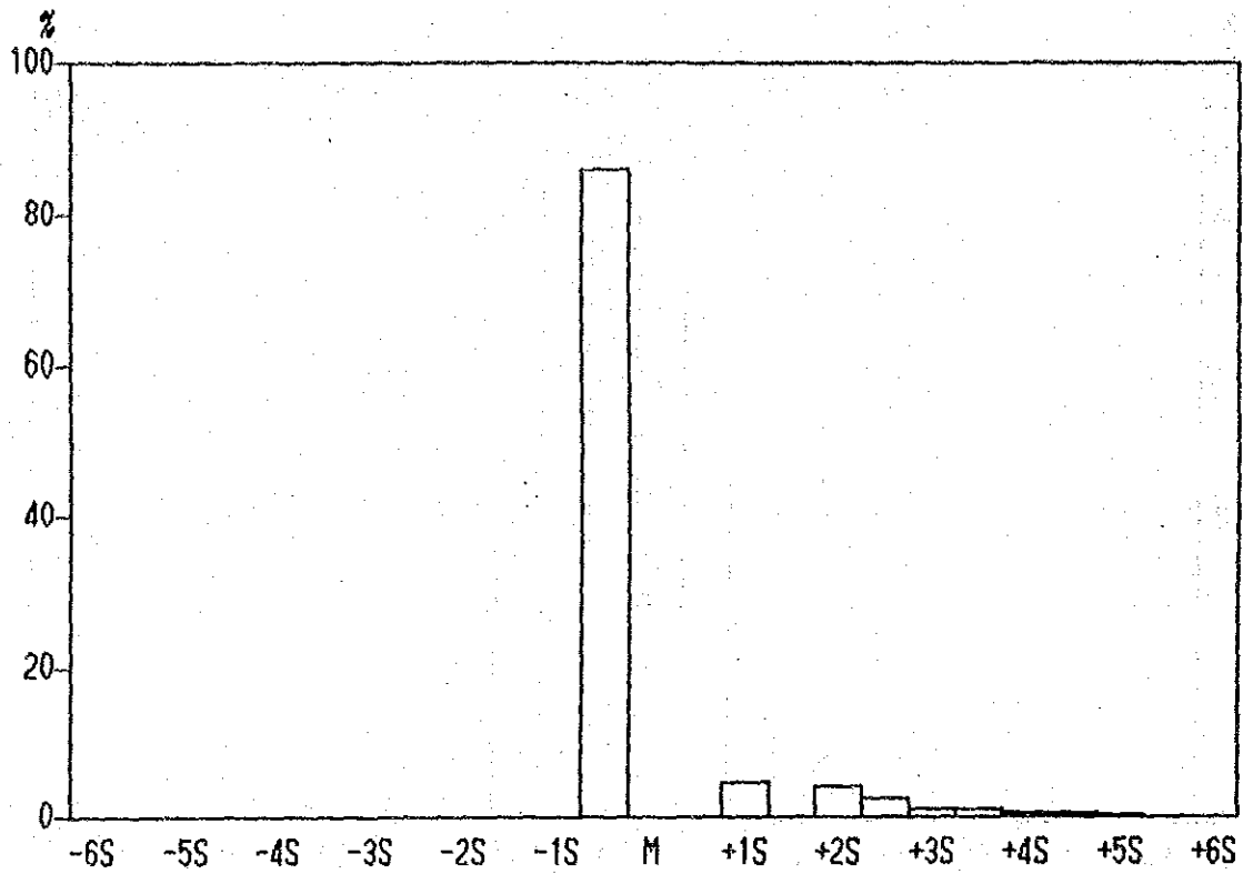
Histograms of Mo content in all Samples.
