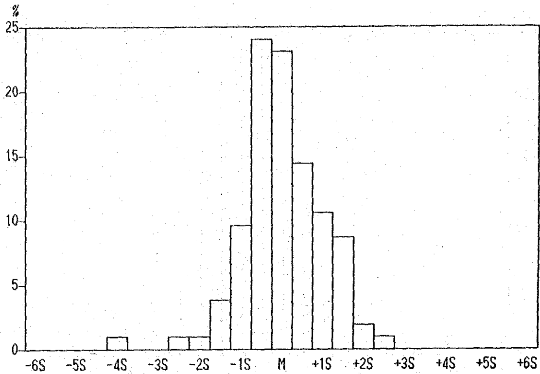
Histogram of Mn contents in Lithological Code; INR
