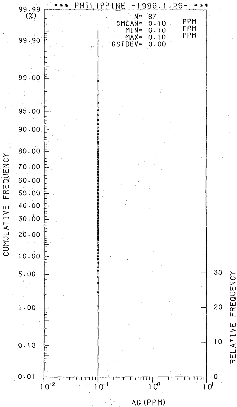
Histogram and Cumulative Frequency Curve of AG content in Lithological Code; 0.5.
