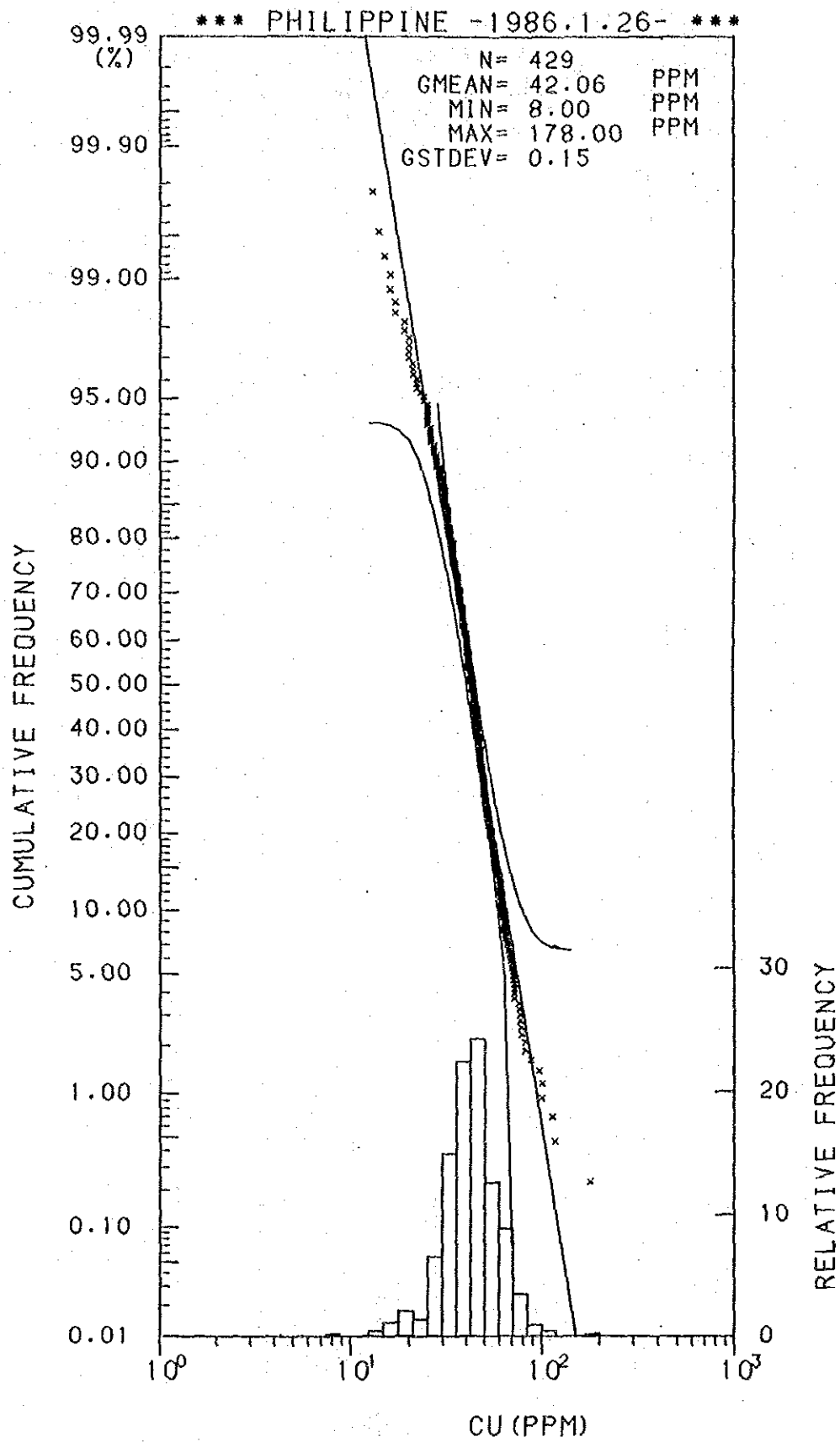
Histogram and Cumulative Frequency Curve of Cu content in Lithological Code; 0.8.
