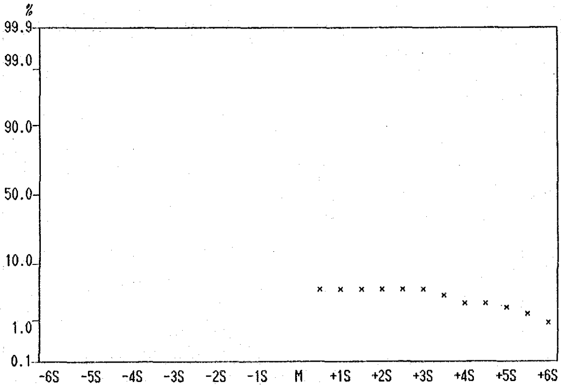
Cumulative Frequency Curve of Pb contents in Lithological Code; KPS
