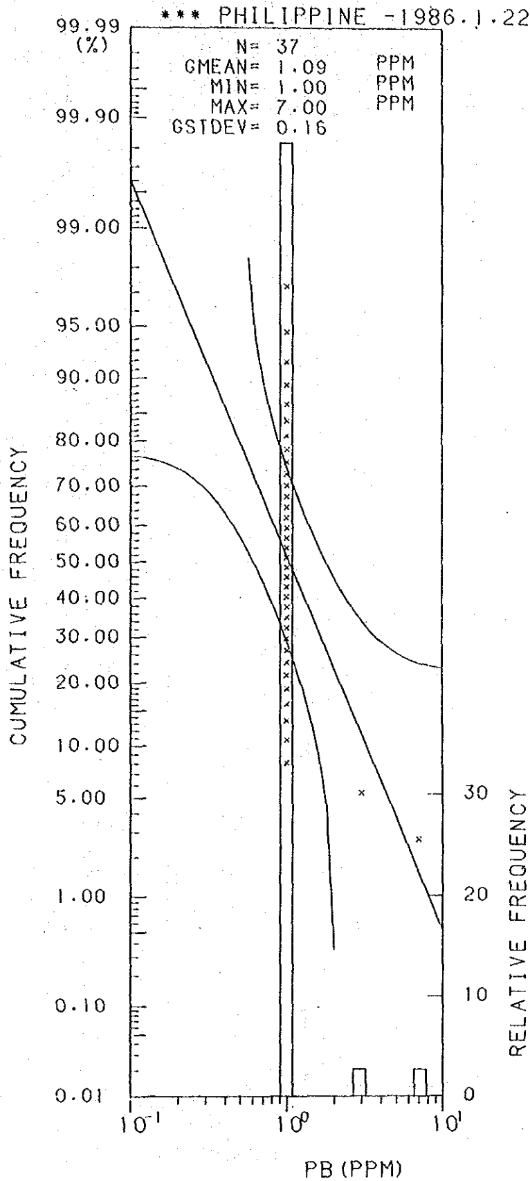
Histogram and Cumulative Frequency Curve of Pb Content in Lithological Code; 0.7.
