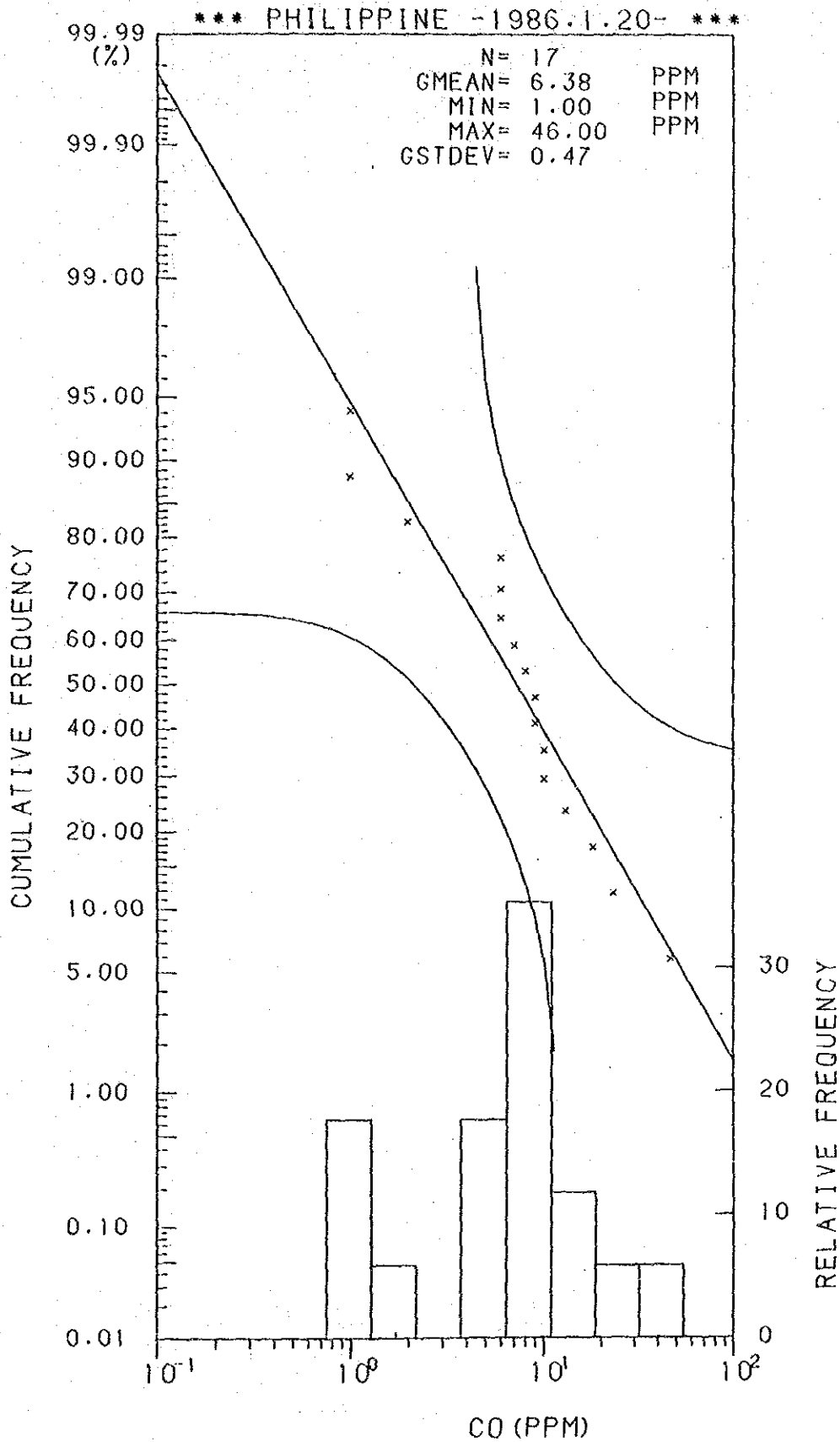
Histogram and Cumulative Frequency Curve of Co Content in Lithological Code; 0.4.
