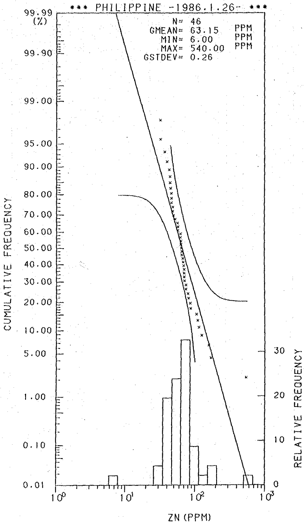
Histogram and Cumulative Frequency Curve of Zn content in Lithological Code; 0.6.
