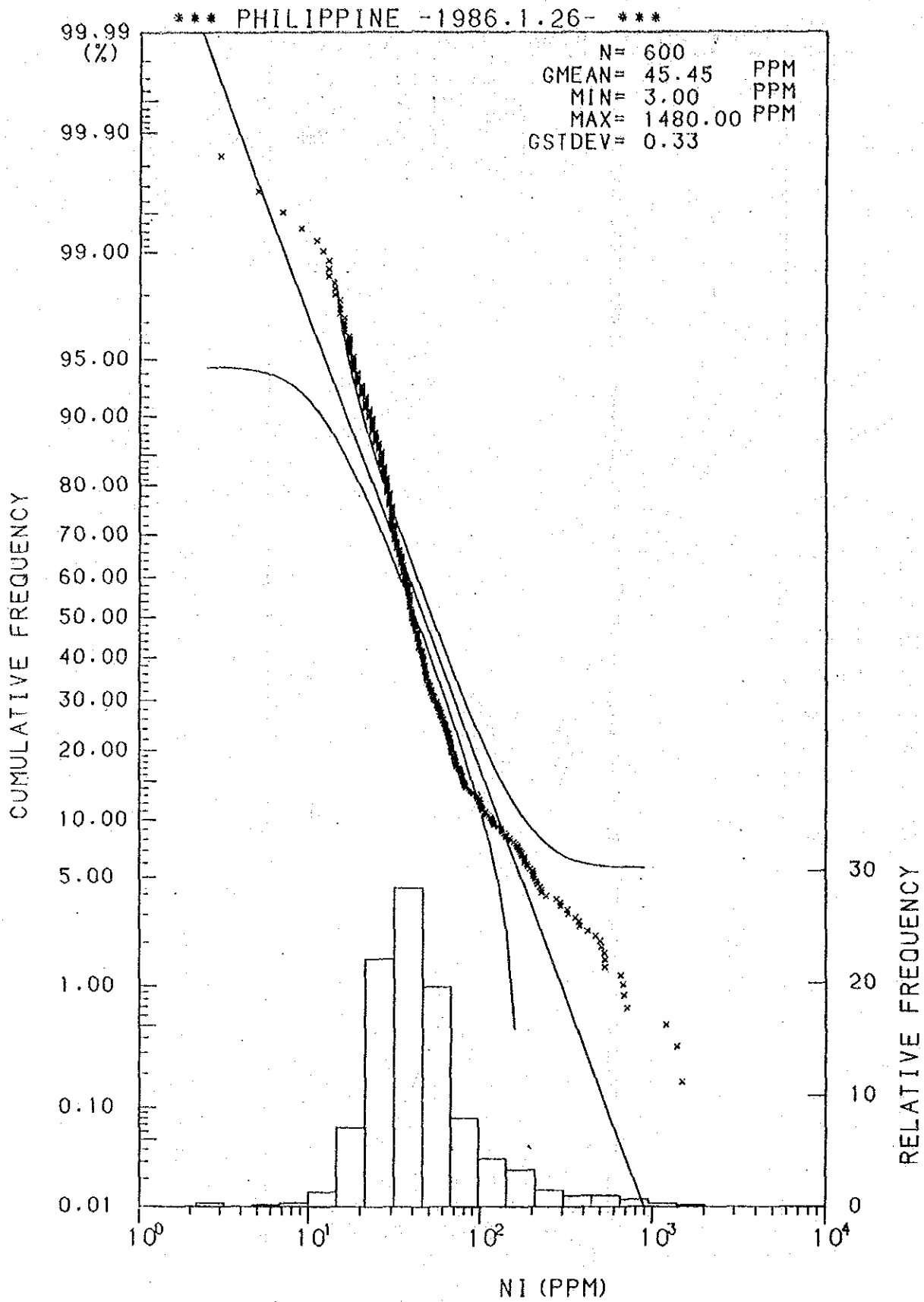
Histogram and Cumulative Frequency Curve of Ni content in Lithological Code; 0.2.
