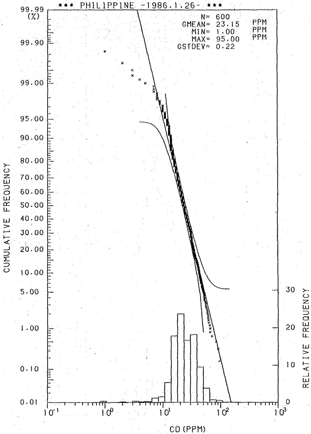
Histogram and Cumulative Frequency Curve of Co content in Lithological Code; 0.2.
