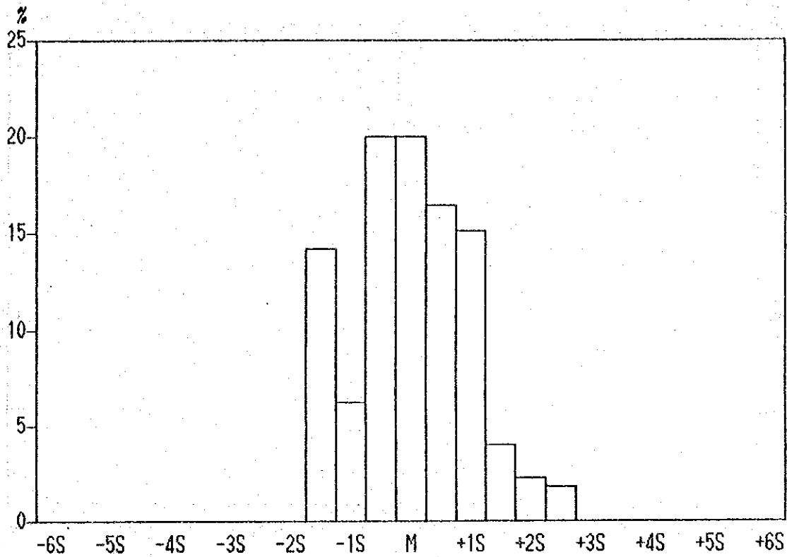
Histogram of As contents in Lithological Code; KPS
