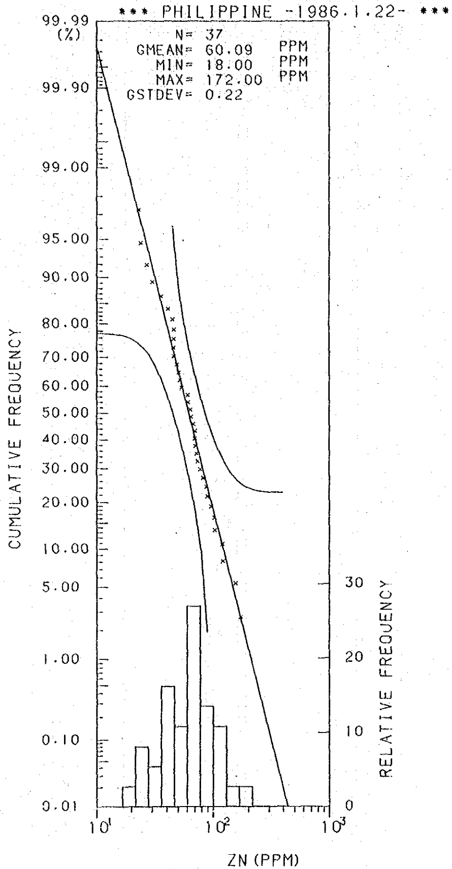
Histogram and Cumulative Frequency Curve of Zn Content in Lithological Code; 0.7.
