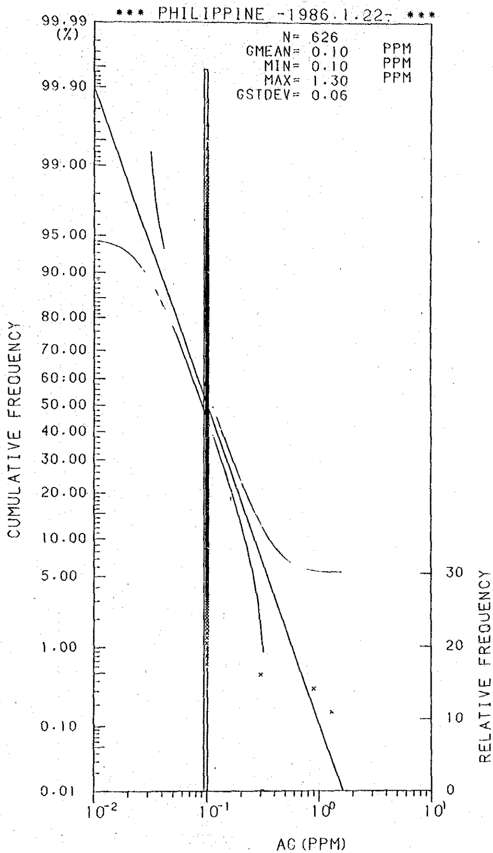
Histogram and Cumulative Frequency Curve of Ag Content in Lithological Code; 0.6.
