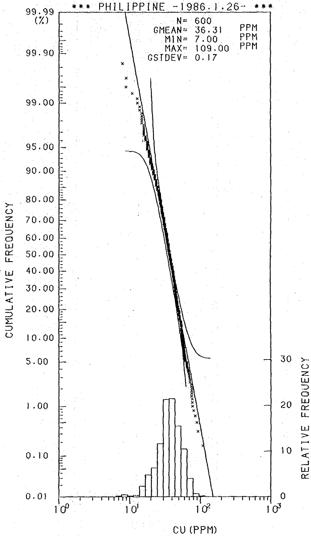
Histogram and Cumulative Frequency Curve of Cu content in Lithological Code; 0.2.
