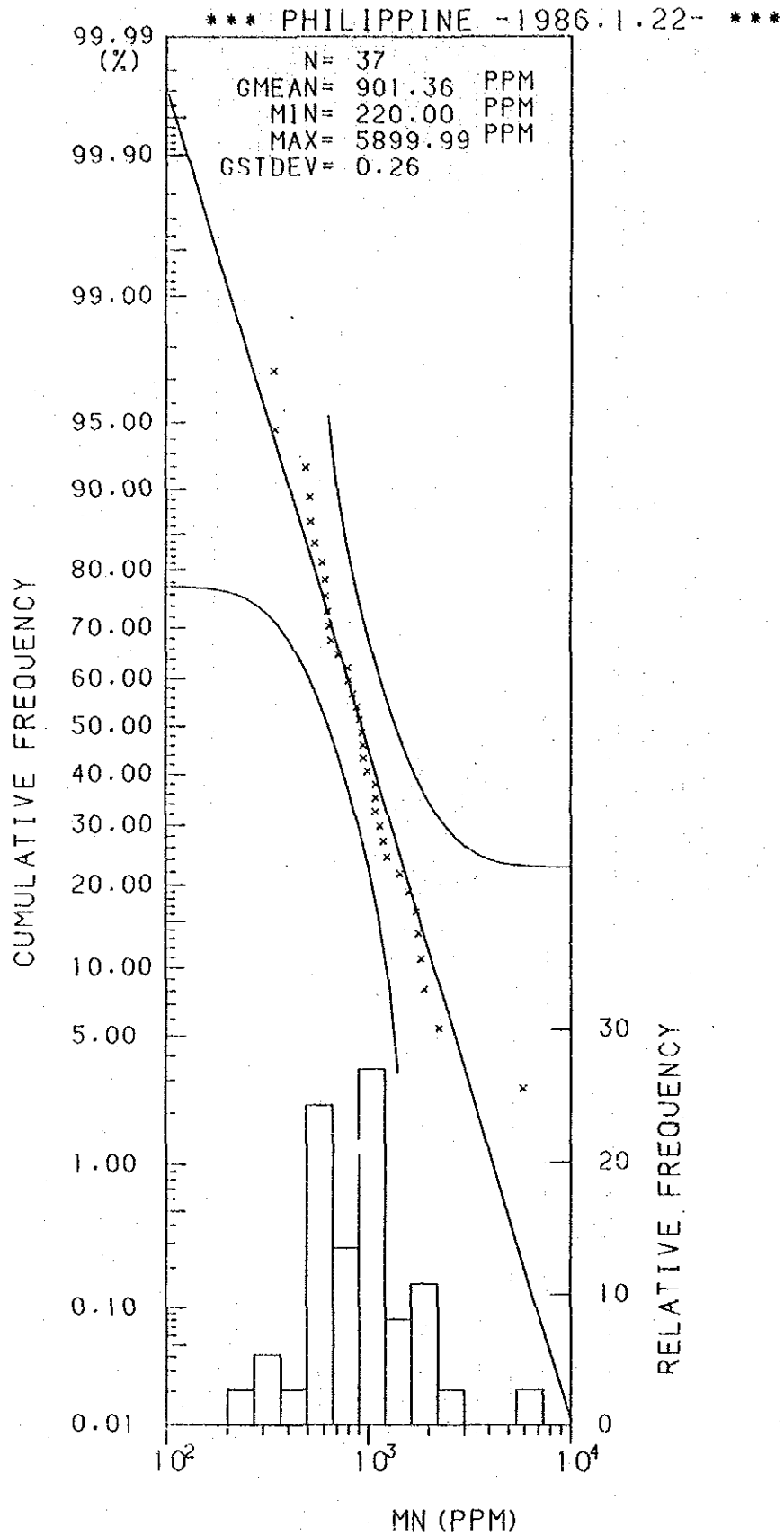
Histogram and Cumulative Frequency Curve of Mn Content in Lithological Code; 0.7.
