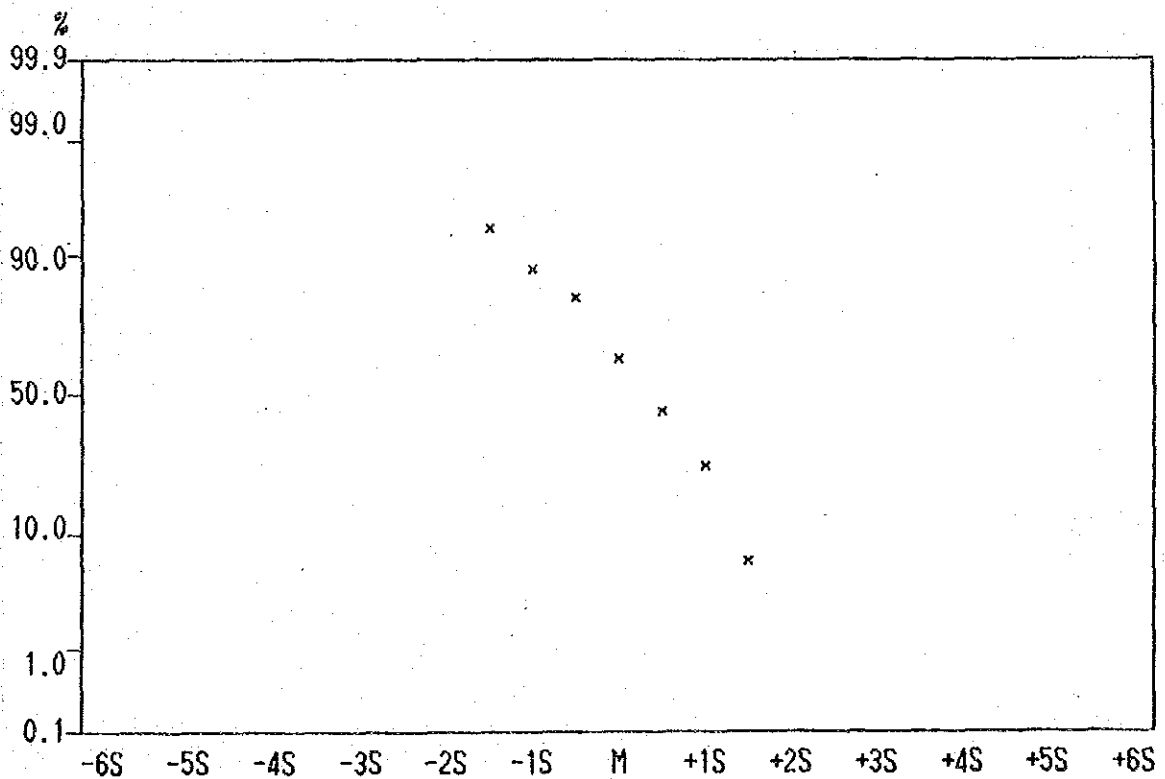
Cumulative Frequency Curve of As contents in Lithological Code; KPL
