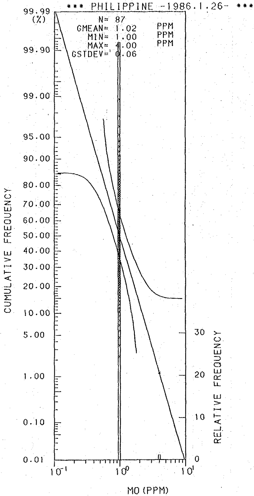
Histogram and Cumulative Frequency Curve of Mo content in Lithological Code; 0.5.
