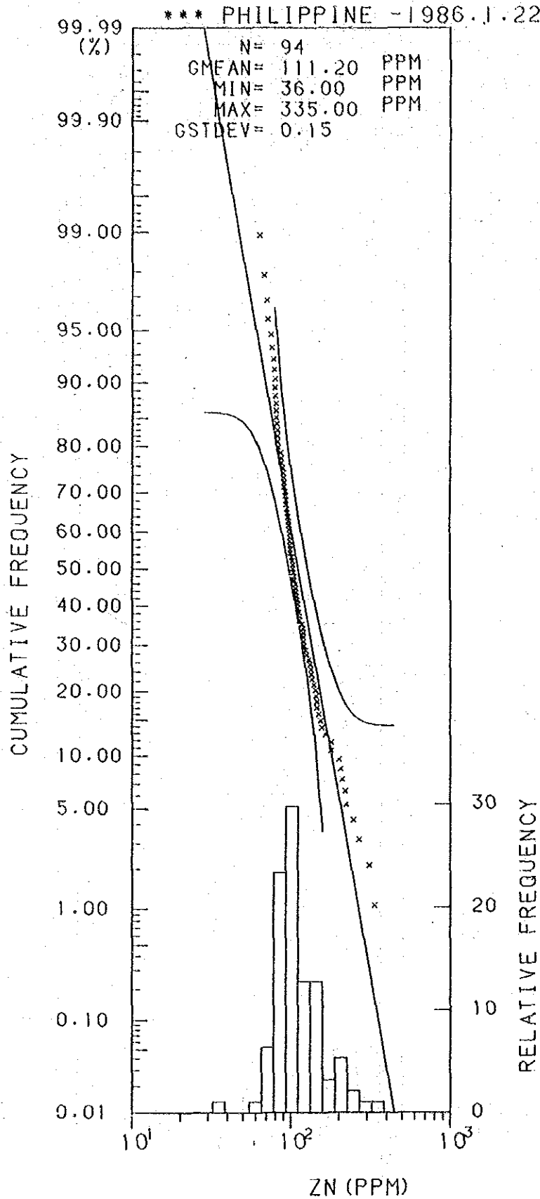
Histogram and Cumulative Frequency Curve of Zn Content in Lithological Code; 0.5.
