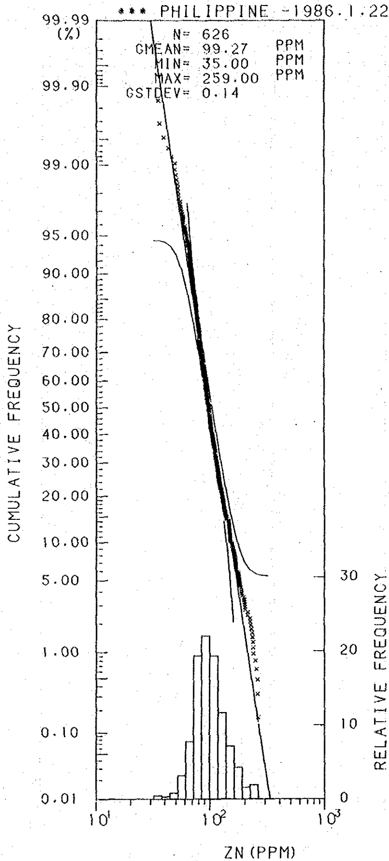
Histogram and Cumulative Frequency Curve of Zn Content in Lithological Code; 0.6.
