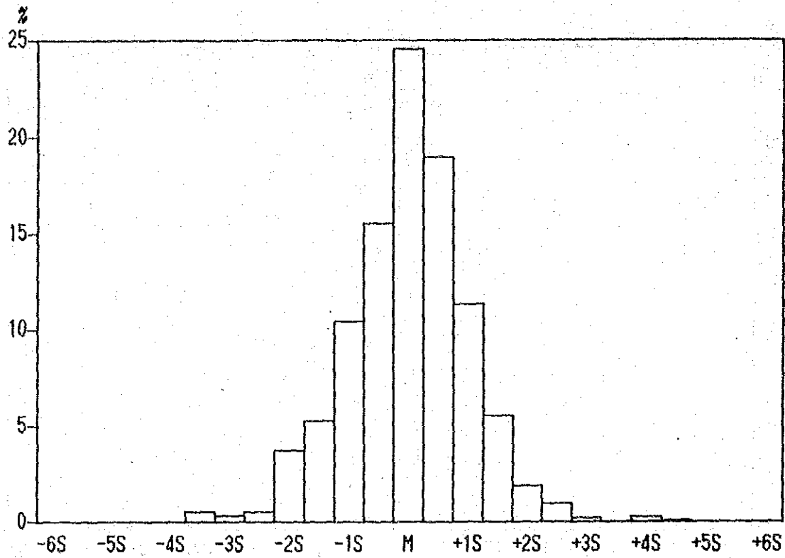
Histograms of Zn content in all Samples.
