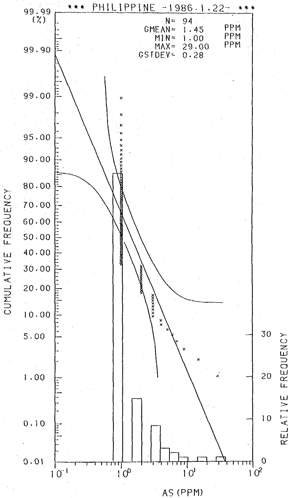
Histogram and Cumulative Frequency Curve of As Content in Lithological Code; 0.5.
