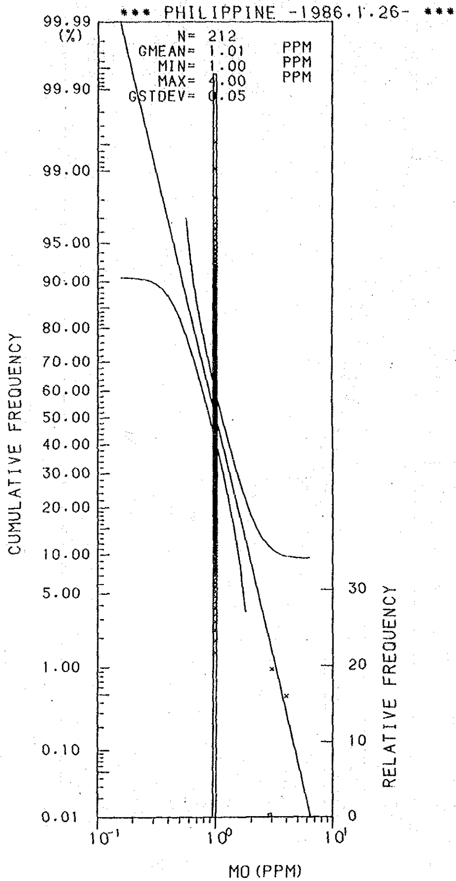
Histogram and Cumulative Frequency Curve of Mo content in Lithological Code; 0.7.
