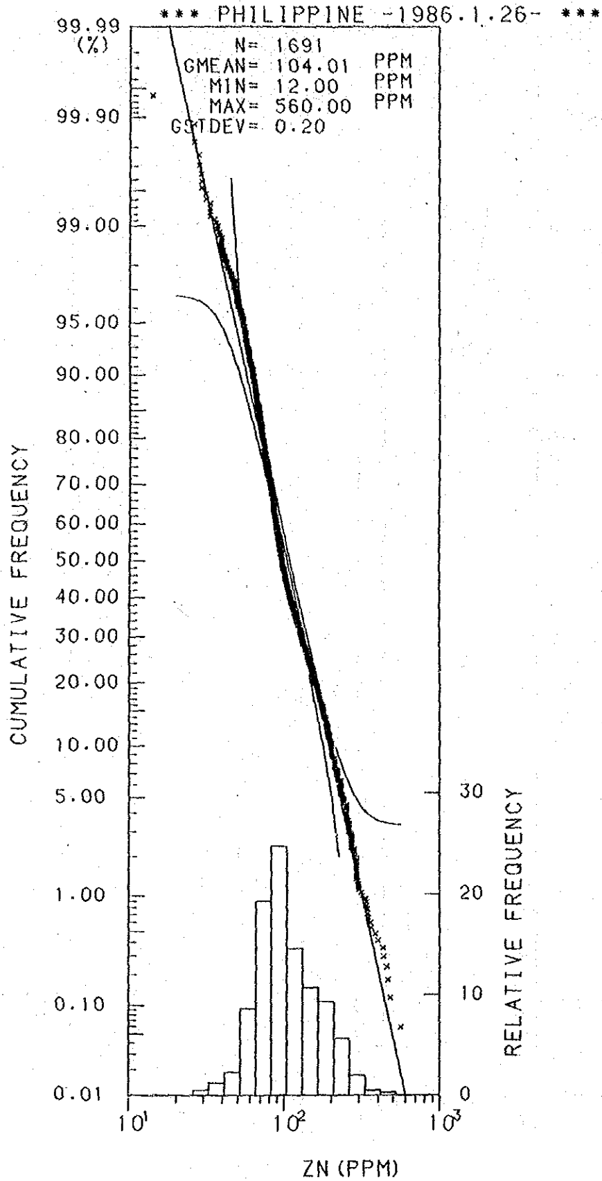
Histogram and Cumulative Frequency Curve of Zn content in Lithological Code; 0.3.
