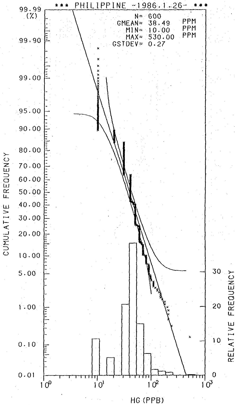
Histogram and Cumulative Frequency Curve of Hg content in Lithological Code; 0.2.
