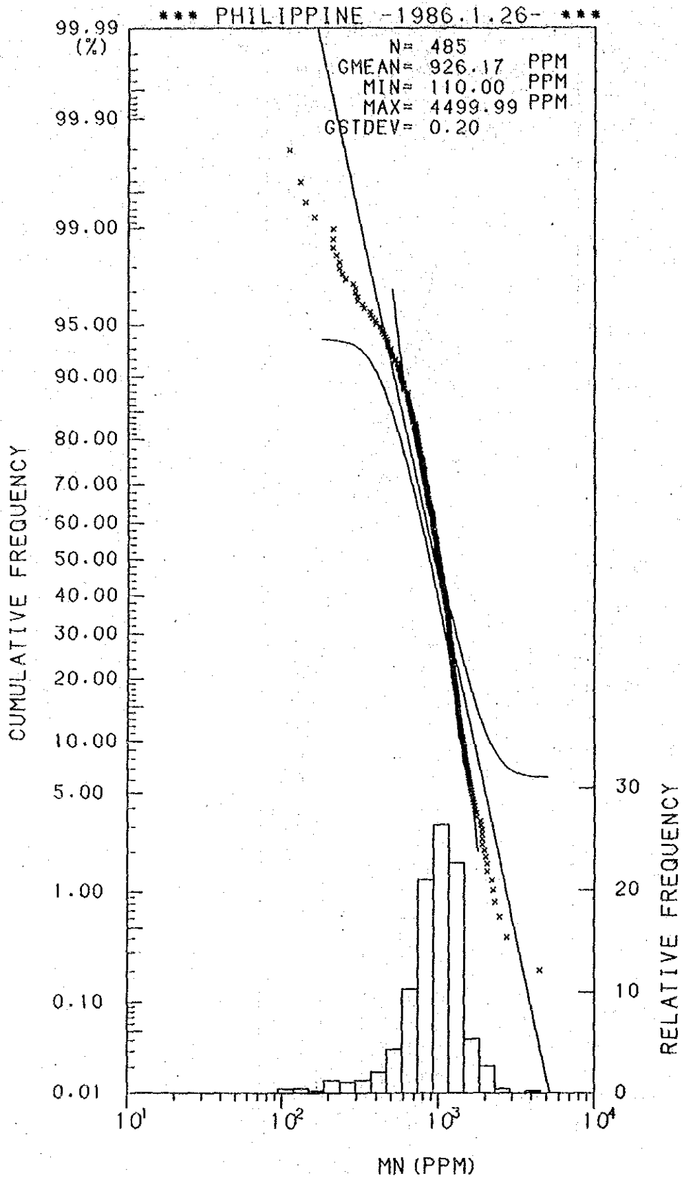
Histogram and Cumulative Frequency Curve of Mn content in Lithological Code; 0.1.
