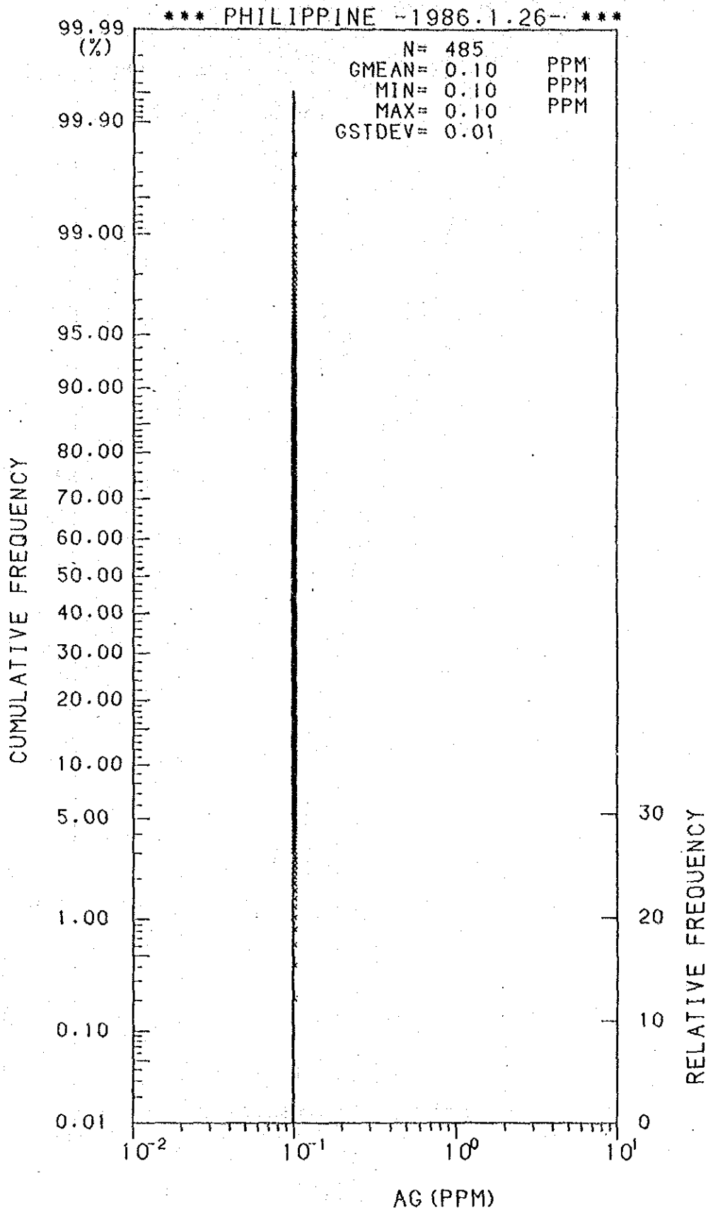
Histogram and Cumulative Frequency Curve of AG content in Lithological Code; 0.1.
