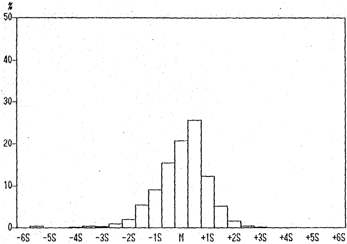
Higtograms of Co content in all Samples.
