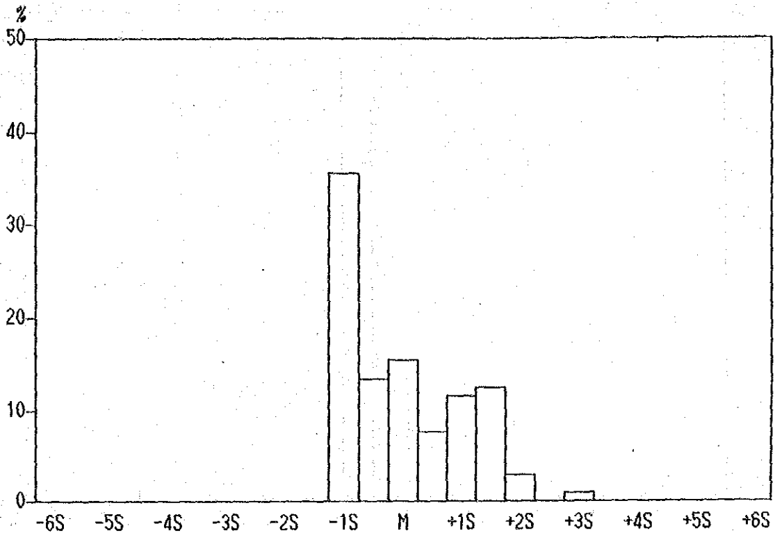
Histogram of As contents in Lithological Code; INR
