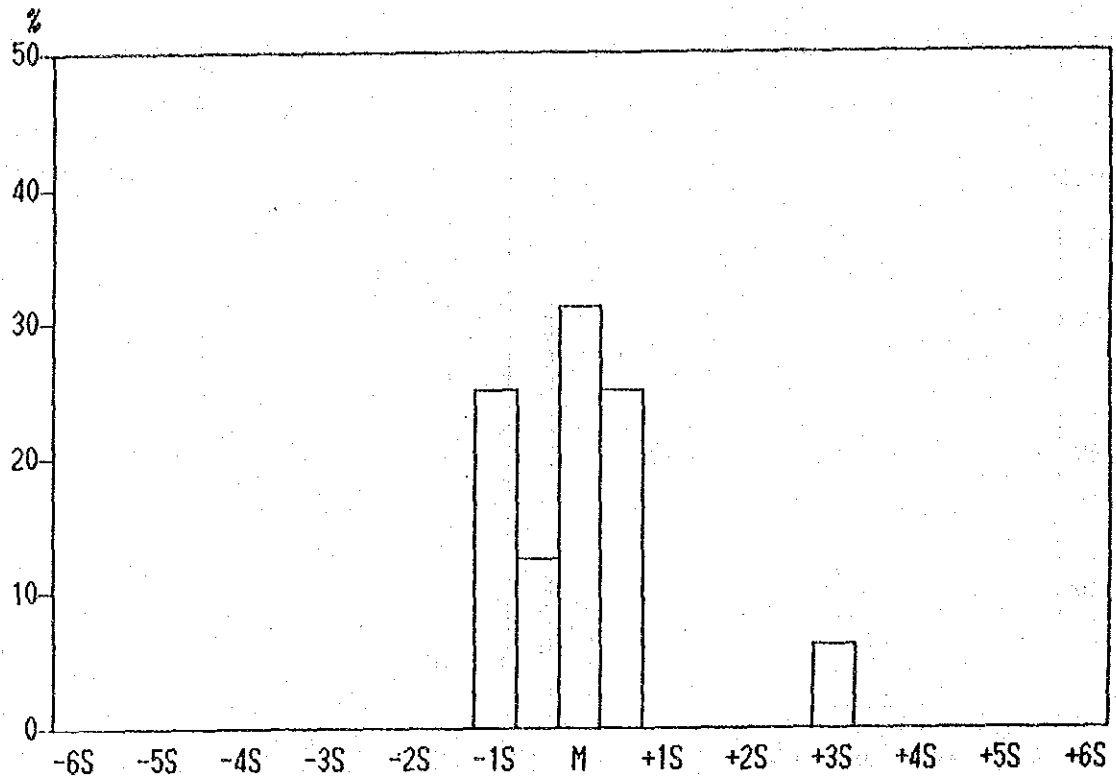
Histogram of Ni contents in Lithological Code; KPL
