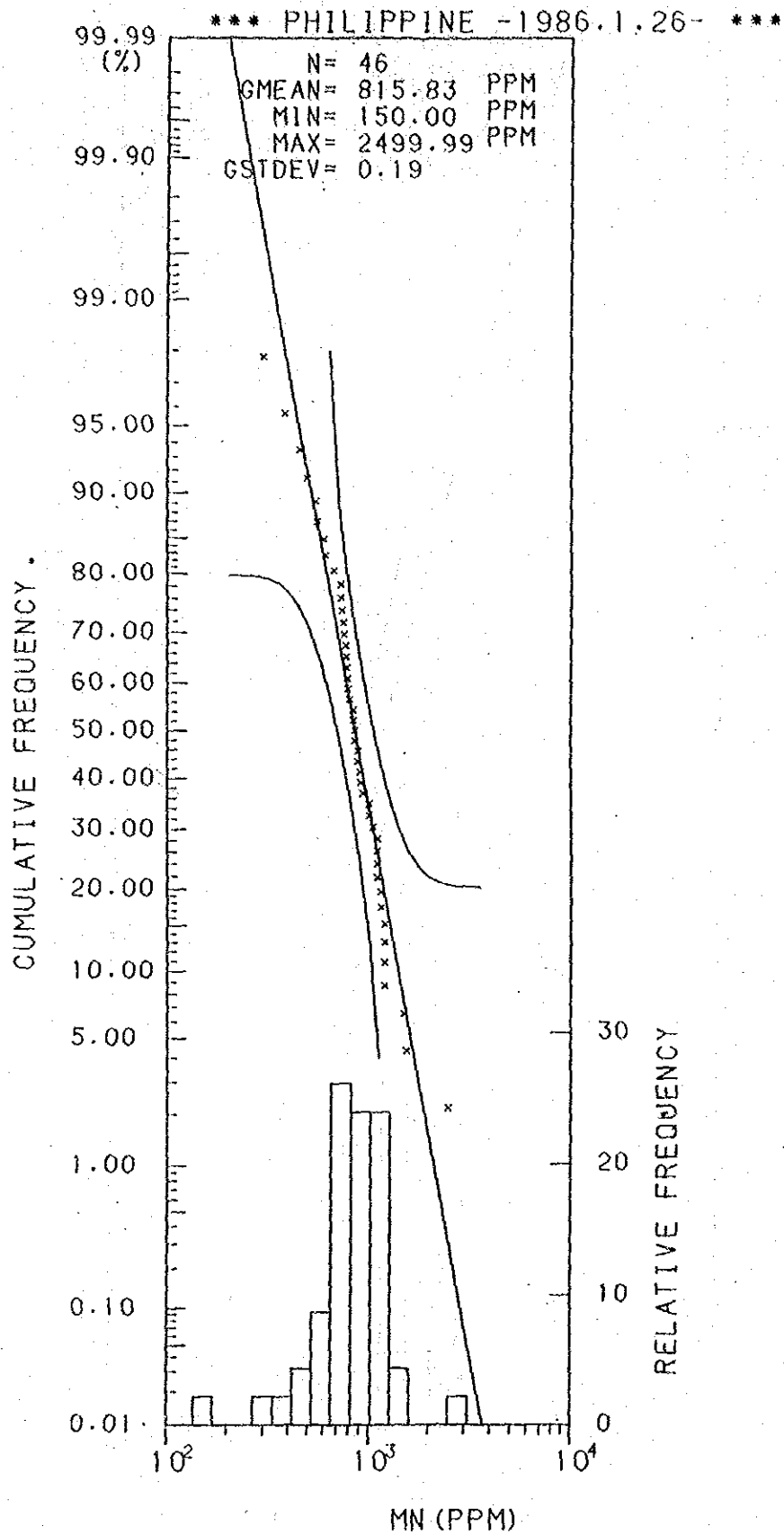
Histogram and Cumulative Frequency Curve of Mn content in Lithological Code; 0.6.
