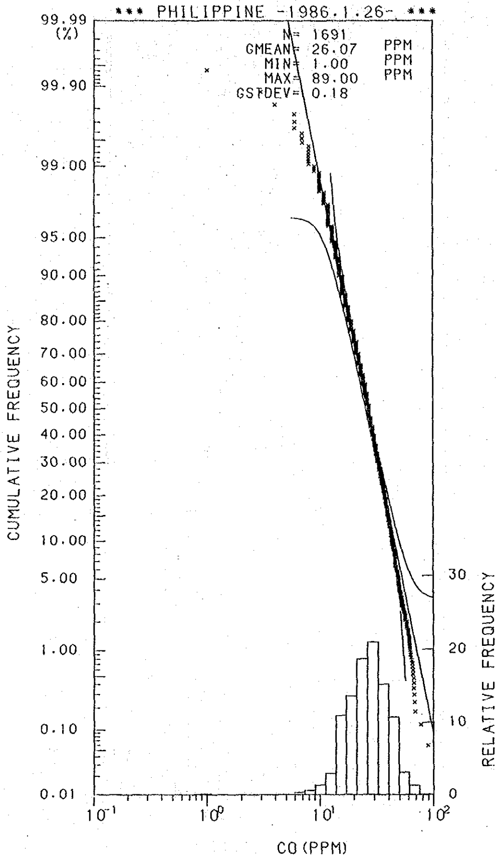
Histogram and Cumulative Frequency Curve of Co content in Lithological Code; 0.3.
