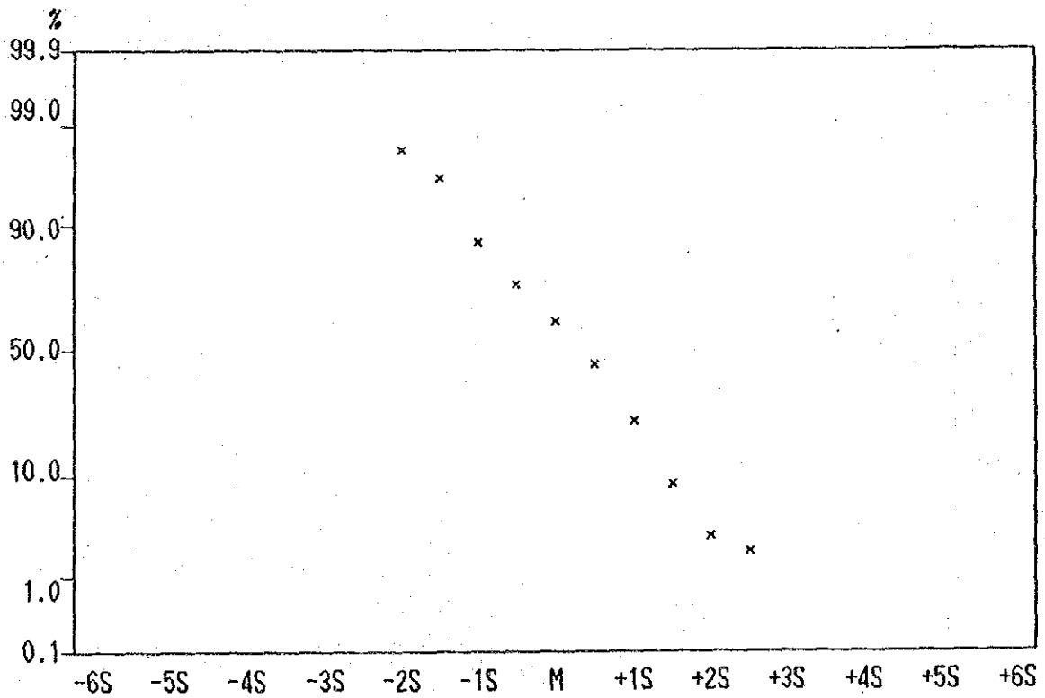
Cumulative Frequency Curve of Cu contents in Lithological Code; INR
