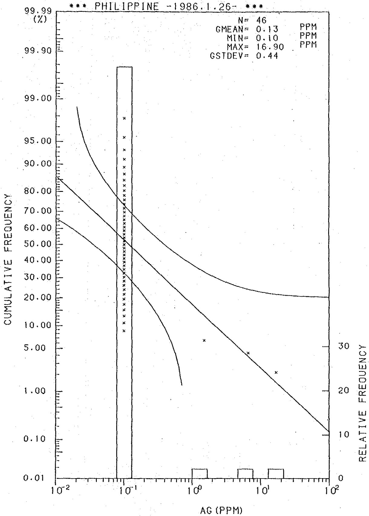
Histogram and Cumulative Frequency Curve of AG content in Lithological Code; 0.6.
