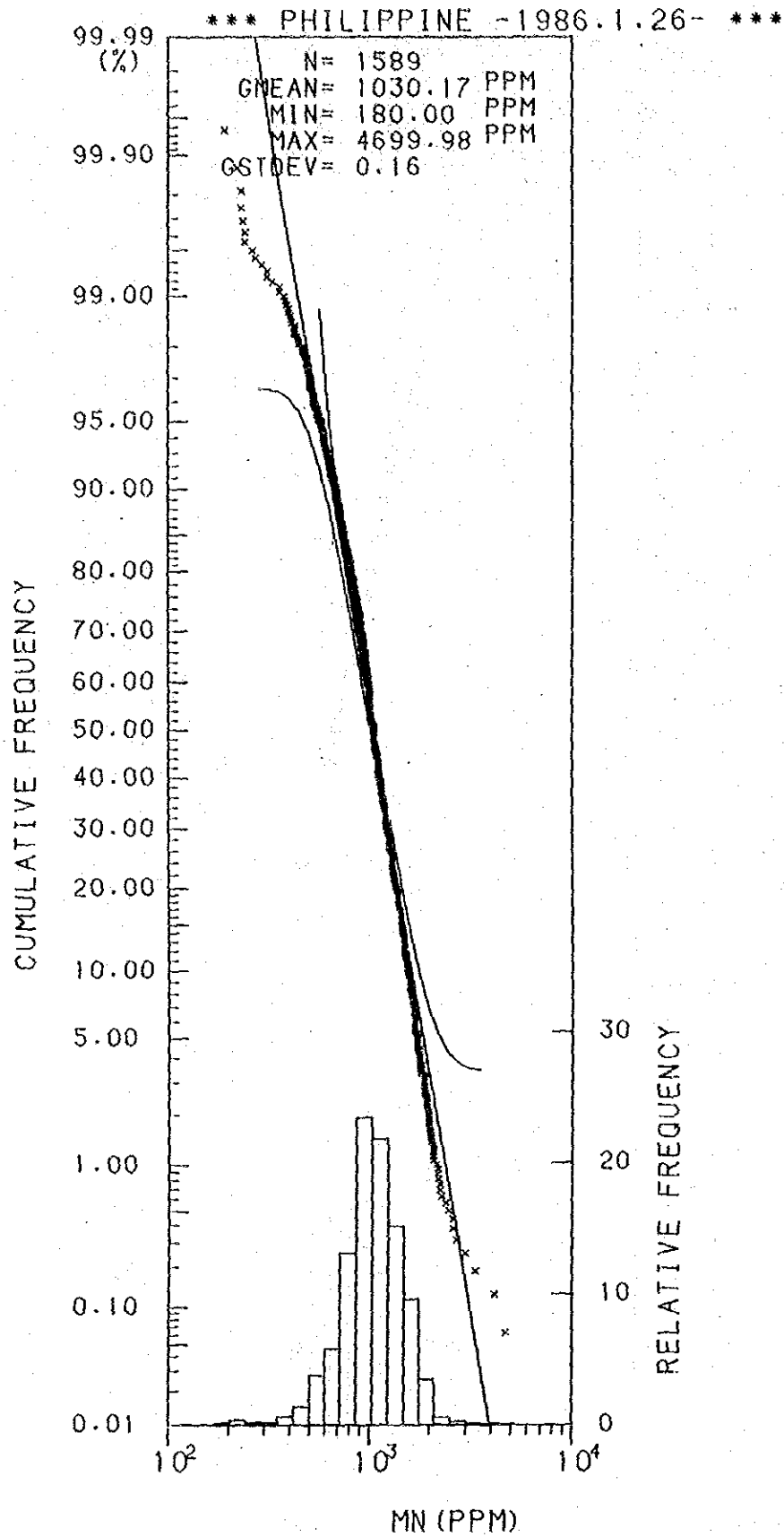
Histogram and Cumulative Frequency Curve of Mn content in Lithological Code; 0.4.
