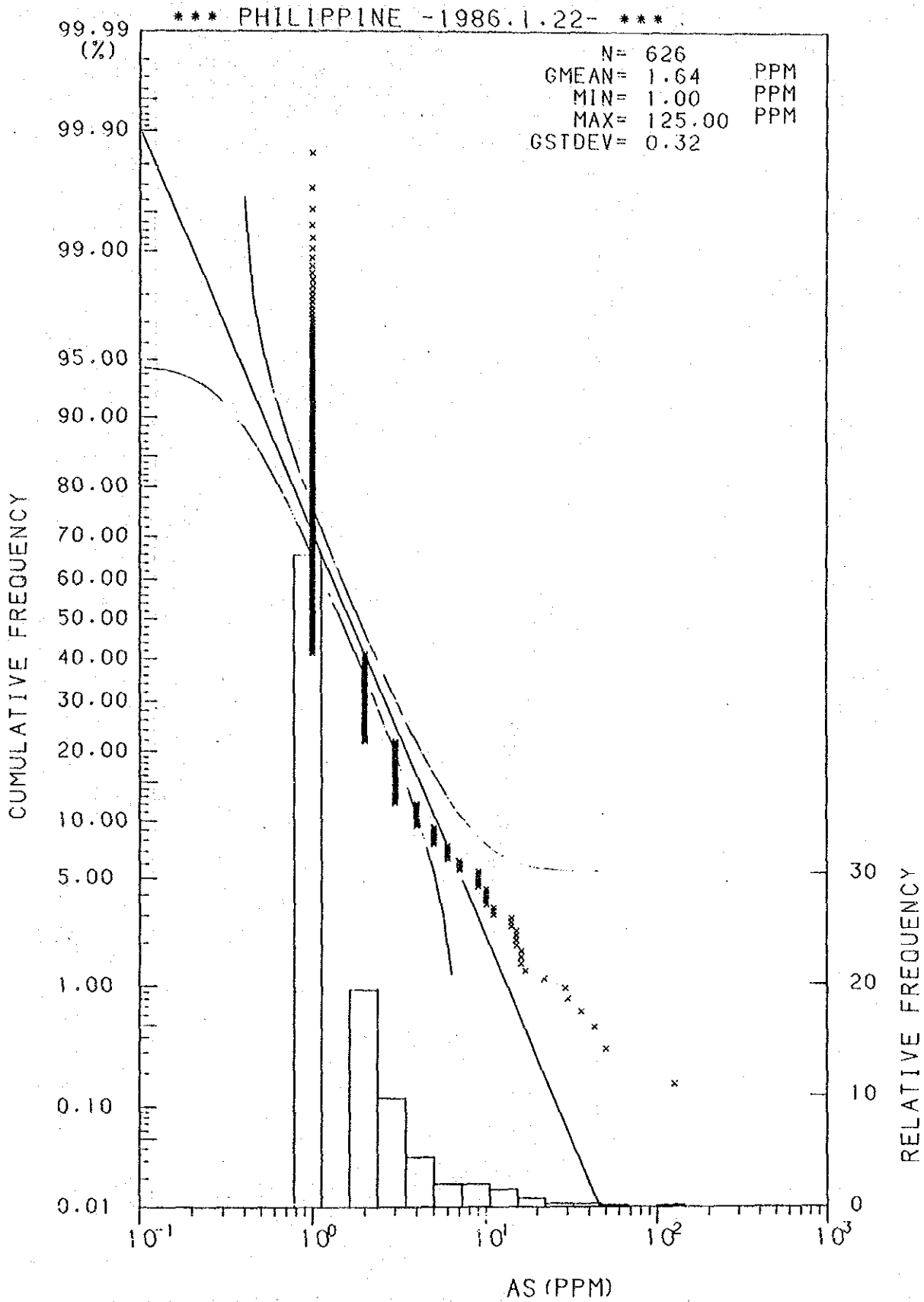
Histogram and Cumulative Frequency Curve of As Content in Lithological Code; 0.6.
