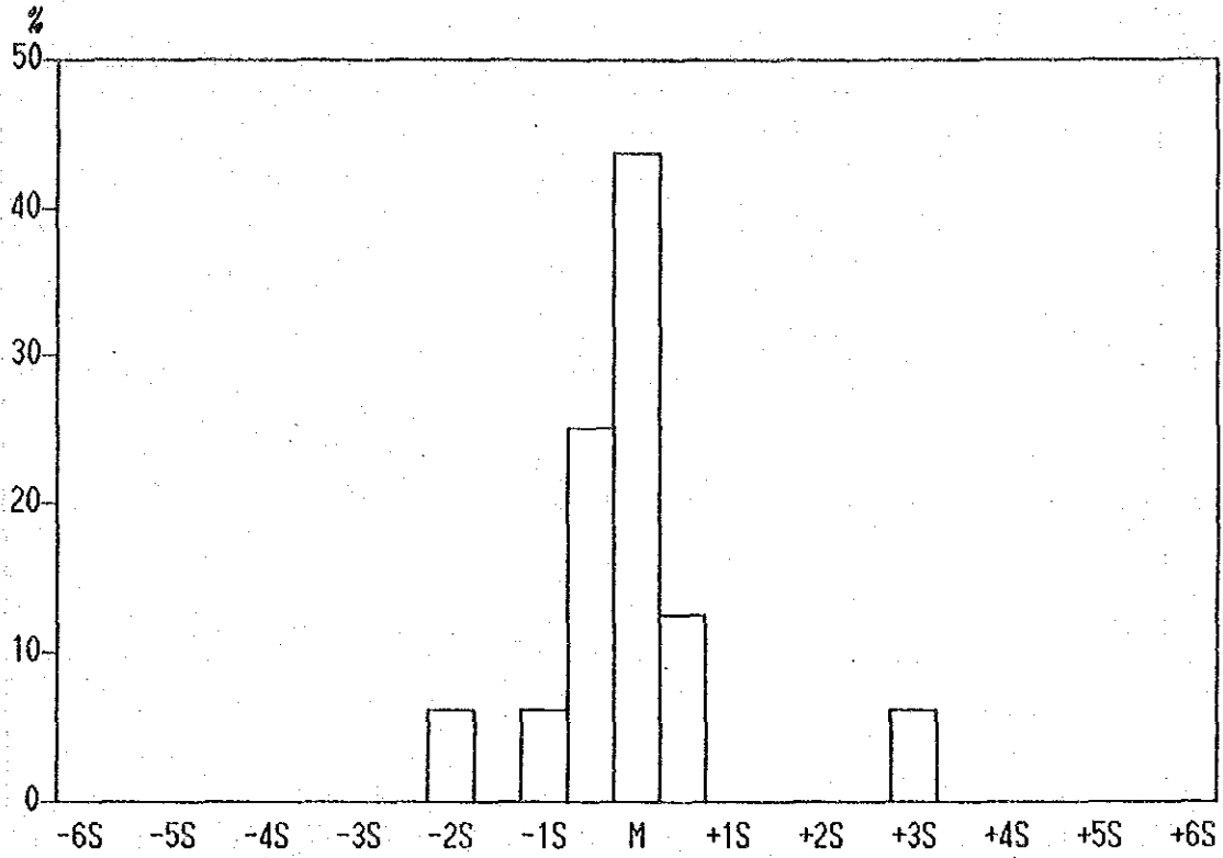
Histogram of Co contents in Lithological Code; KPL
