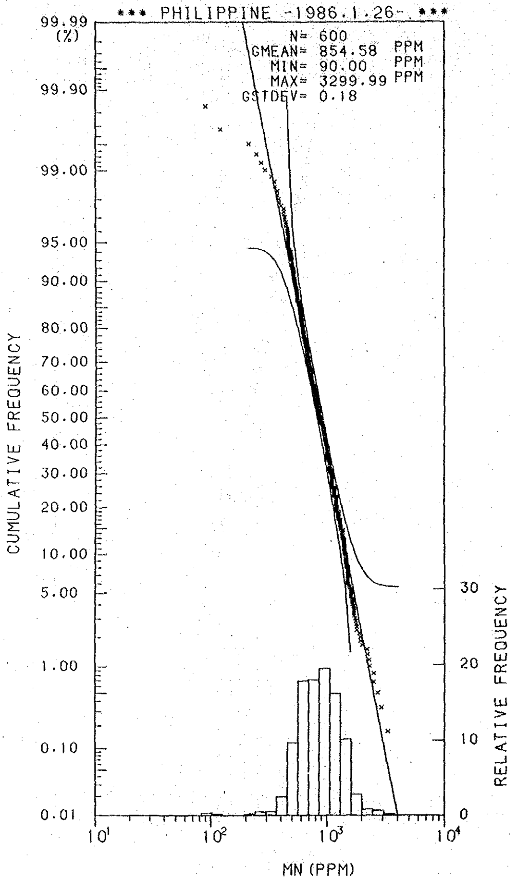
Histogram and Cumulative Frequency Curve of Mn content in Lithological Code; 0.2.
