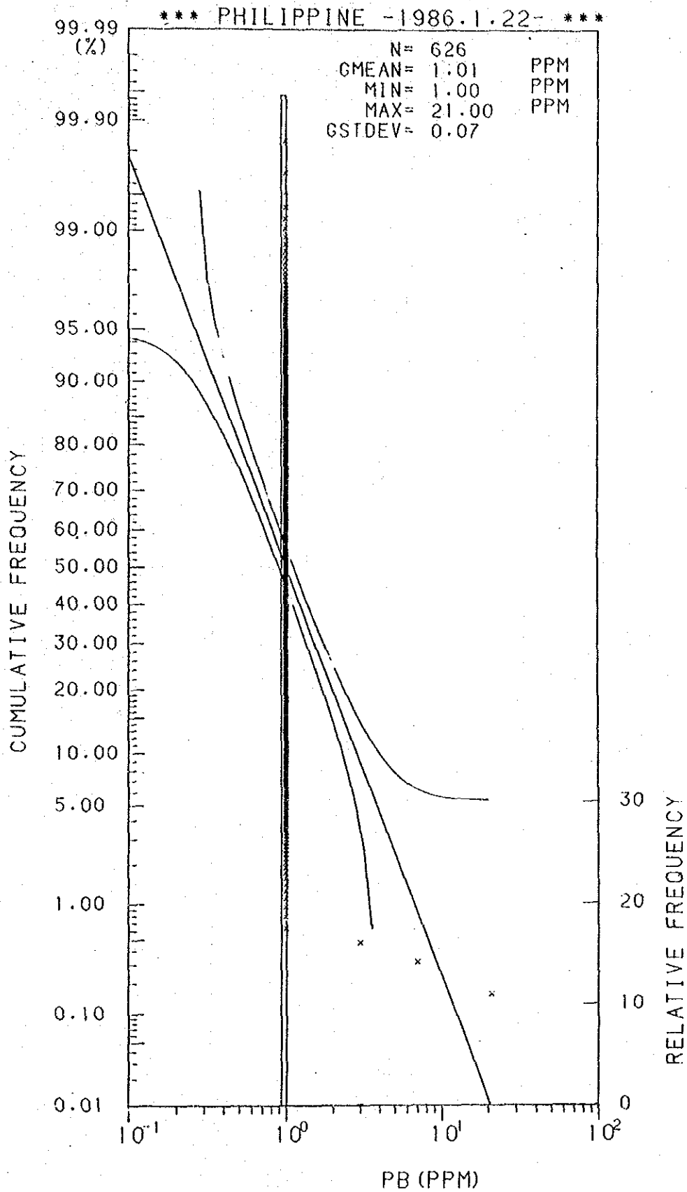
Histogram and Cumulative Frequency Curve of Pb Content in Lithological Code; 0.6.
