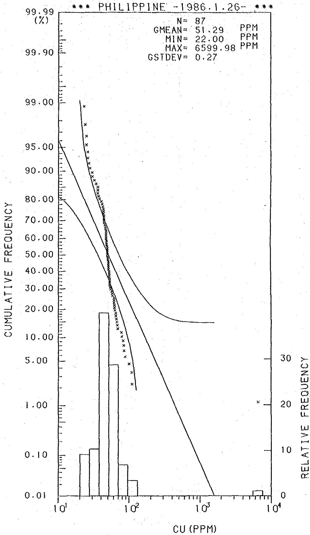
Histogram and Cumulative Frequency Curve of Cu content in Lithological Code; 0.5.
