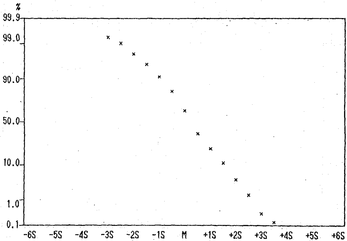
Cumulative Frequency Curve of Ni content in all Samples.
