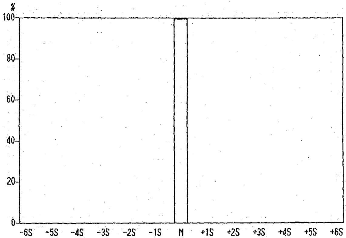
Higtograms of Ag content in all Samples.
