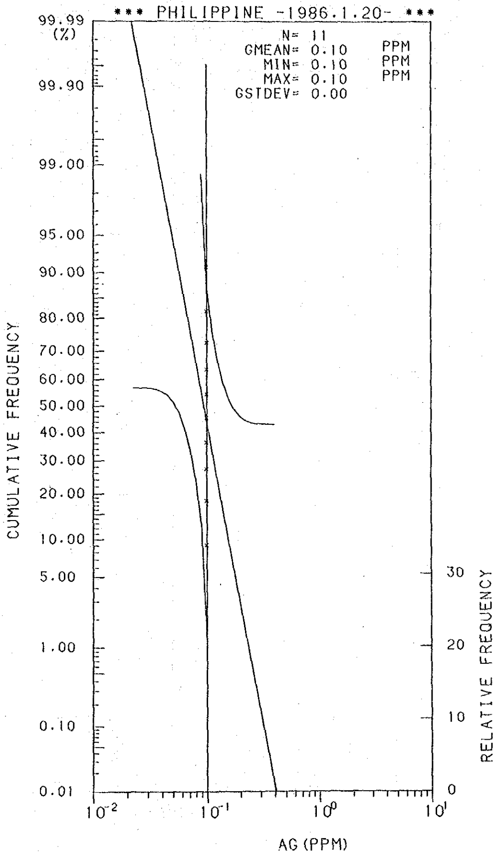
Histogram and Cumulative Frequency Curve of Ag Content in Lithological Code; 0.2.
