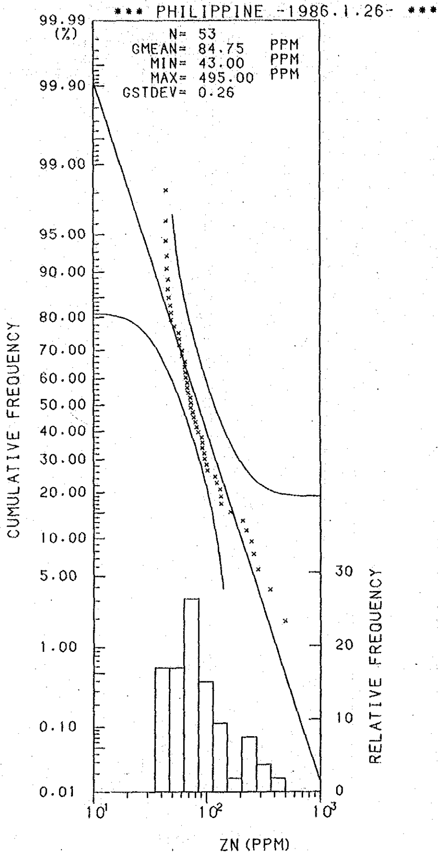
Histogram and Cumulative Frequency Curve of Zn content in Lithological Code; 0.9.
