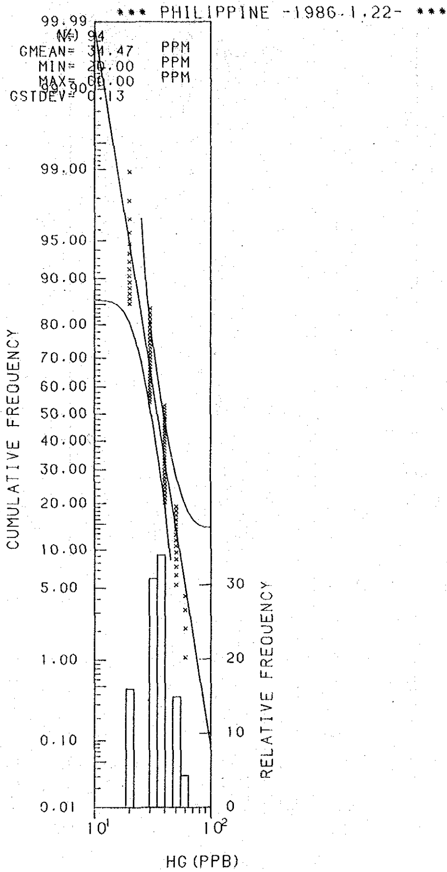
Histogram and Cumulative Frequency Curve of Hg Content in Lithological Code; 0.5.
