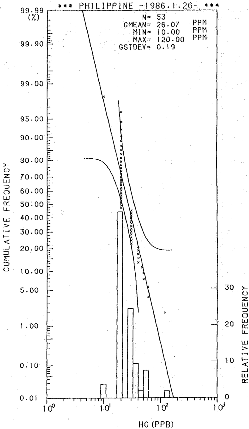
Histogram and Cumulative Frequency Curve of Hg content in Lithological Code; 0.9.
