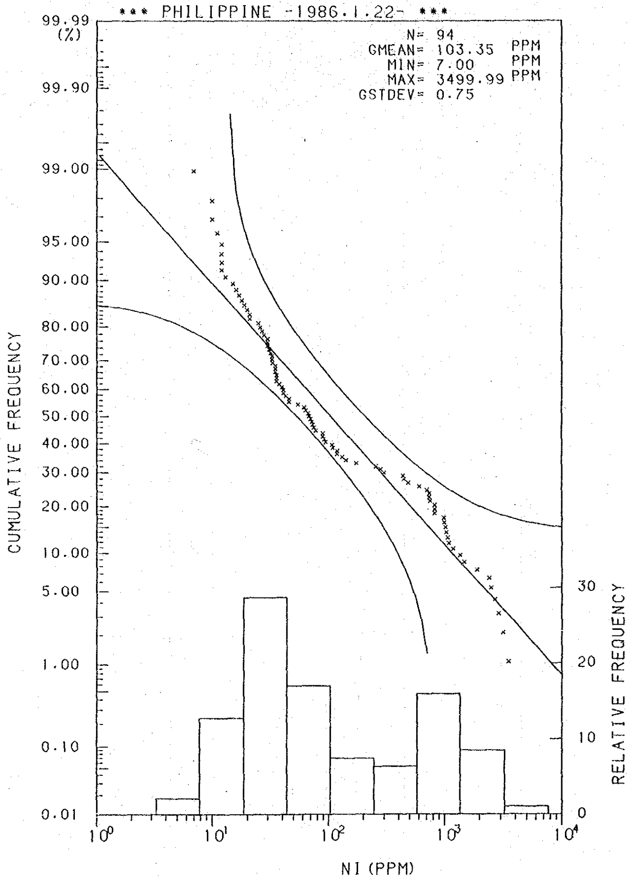
Histogram and Cumulative Frequency Curve of Ni Content in Lithological Code; 0.5.
