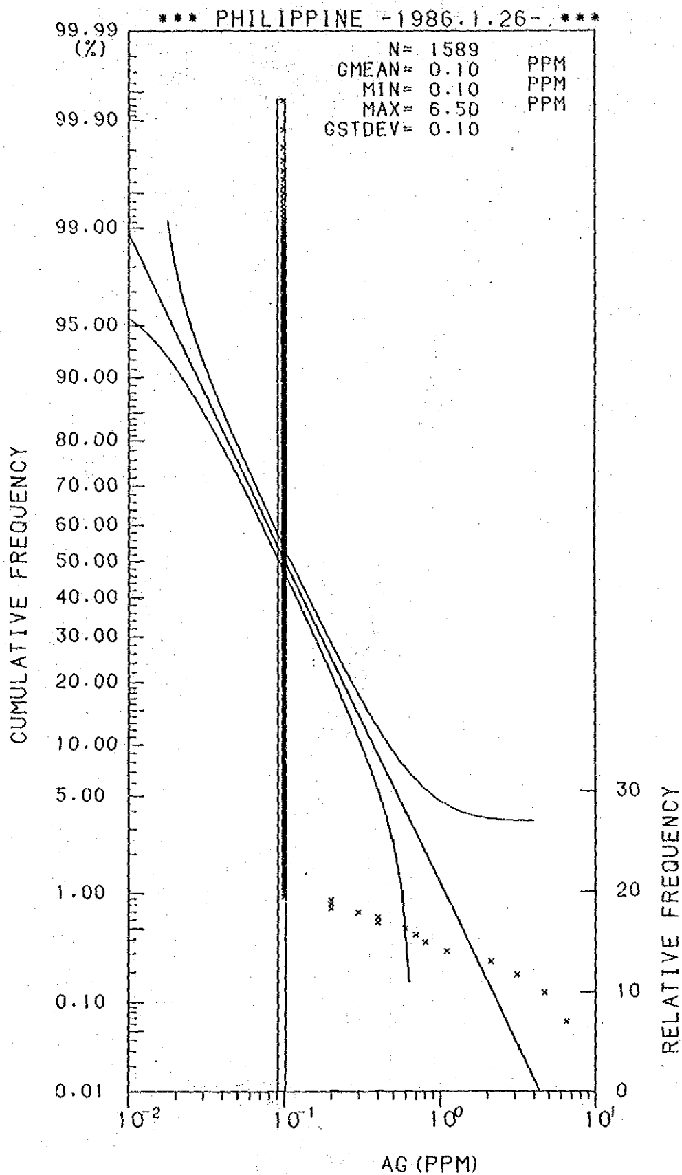
Histogram and Cumulative Frequency Curve of AG content in Lithological Code; 0.4.
