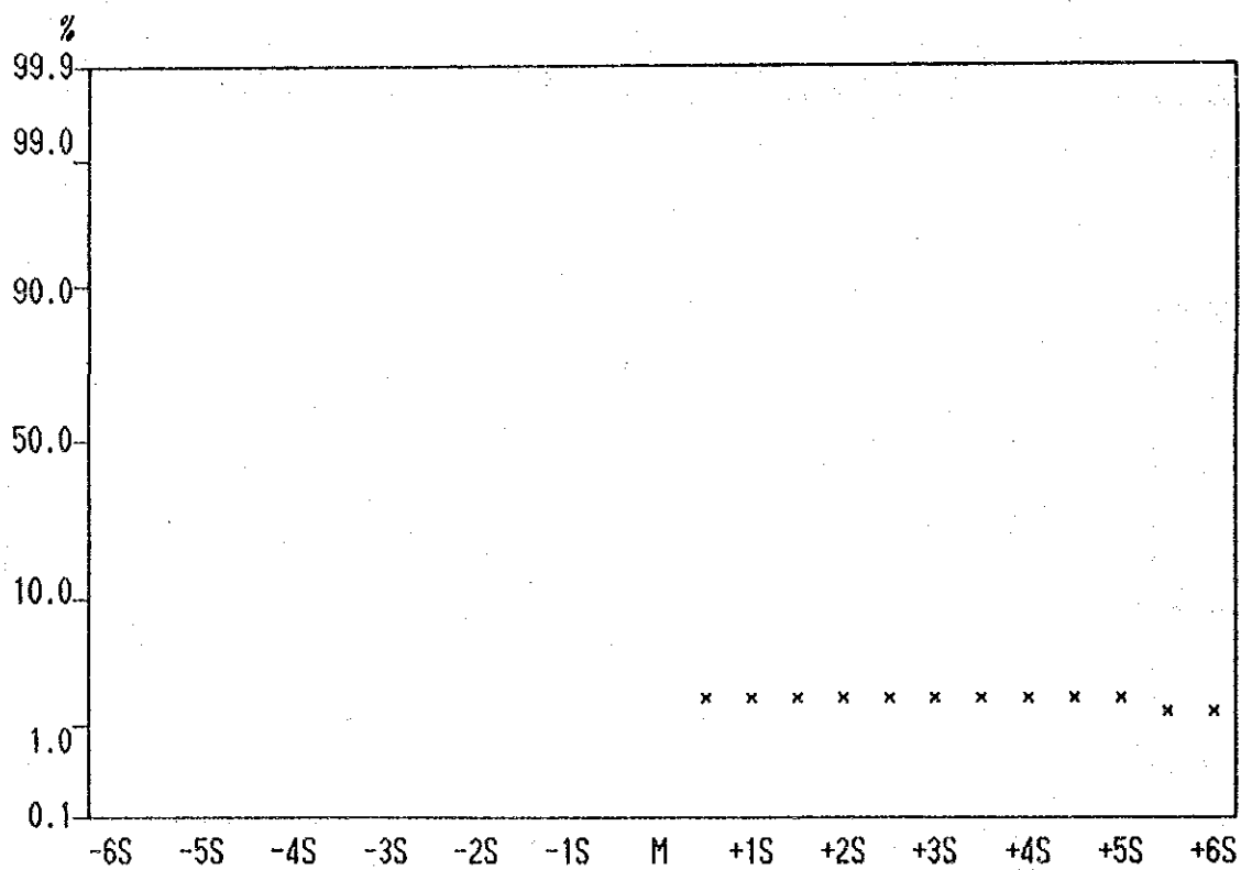
Cumulative Frequency Curve of Hg contents in Lithological Code; KPS
