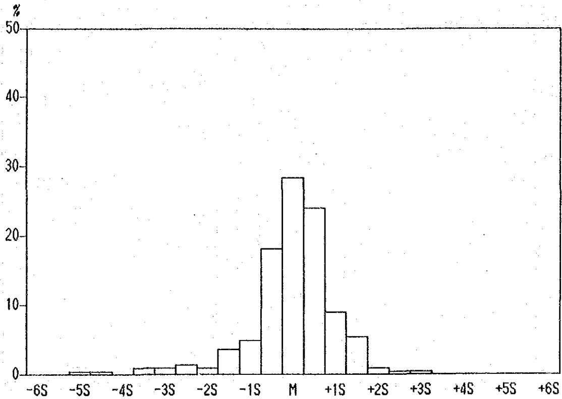
Histogram of Co contents in Lithological Code; KPS
