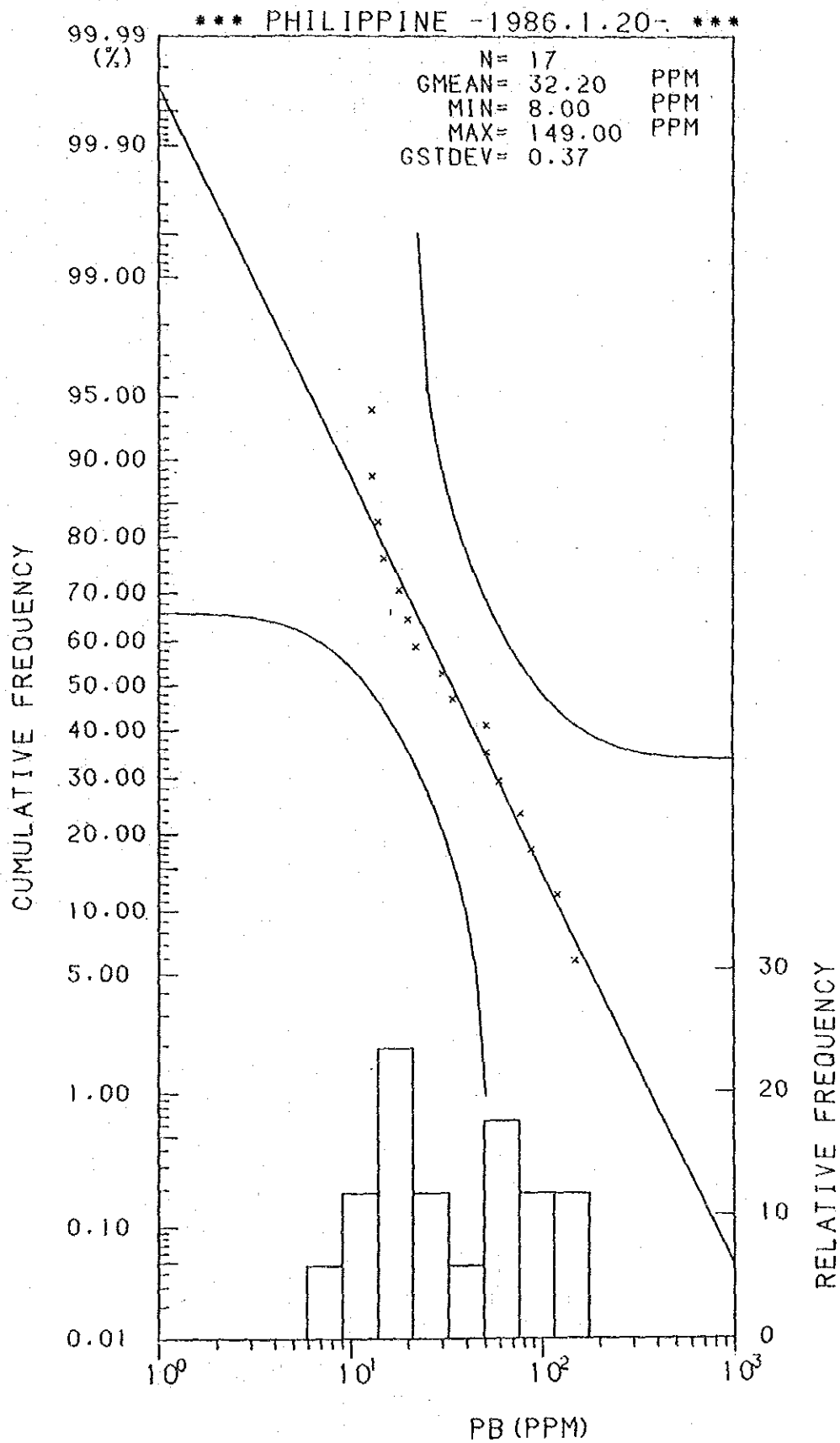
Histogram and Cumulative Frequency Curve of Pb Content in Lithological Code; 0.4.
