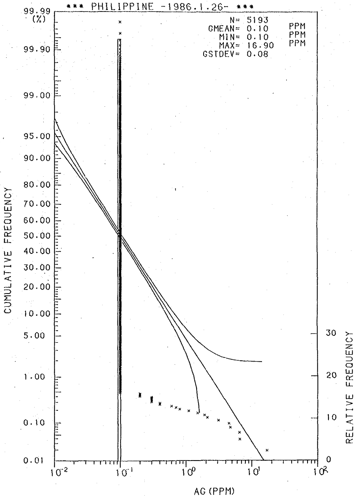
Histogram and Cumulative Frequency Curve of AG content in All Samples.
