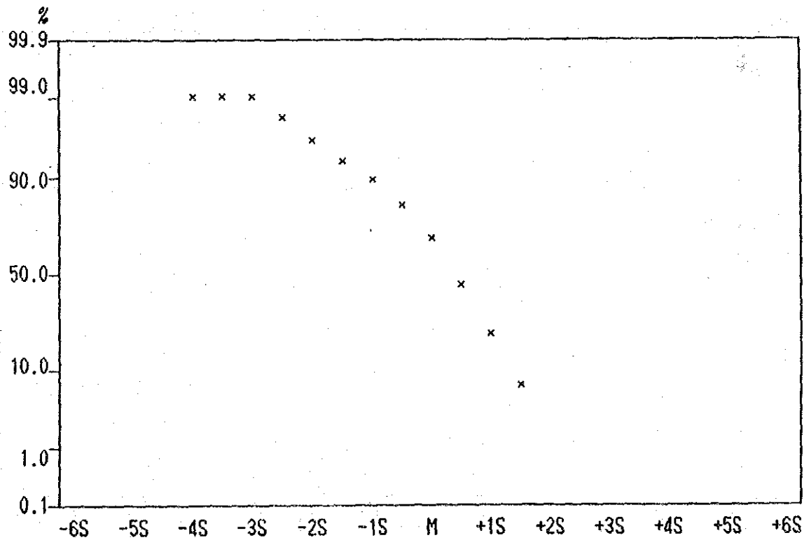
Cumulative Frequency Curve of Co contents in Lithological Code; INR
