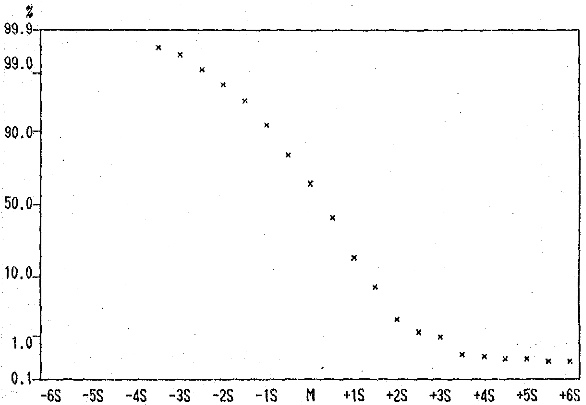
Cumulative Frequency Curve of Cu content in all Samples.
