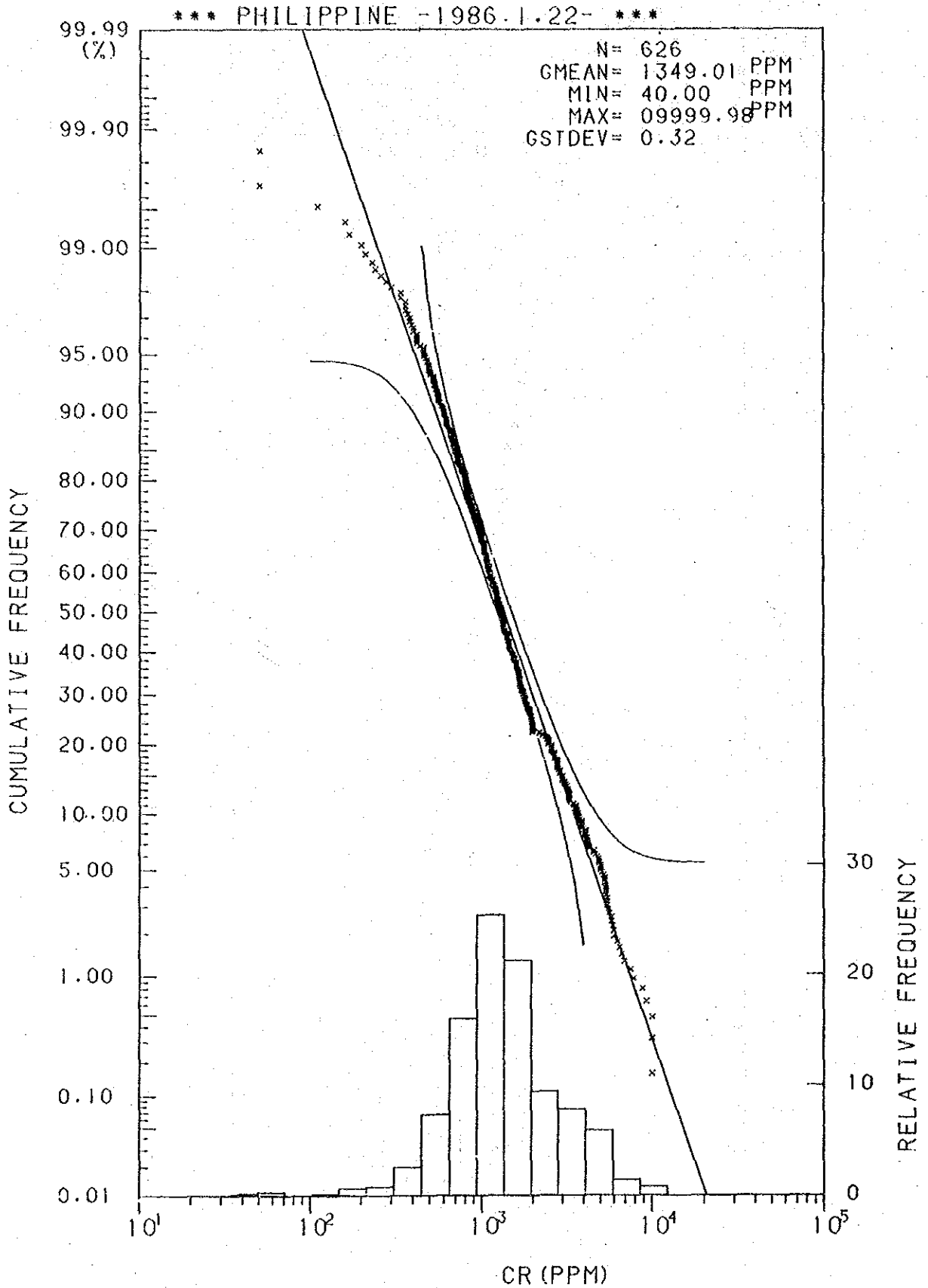
Histogram and Cumulative Frequency Curve of Cr Content in Lithological Code; 0.6.
