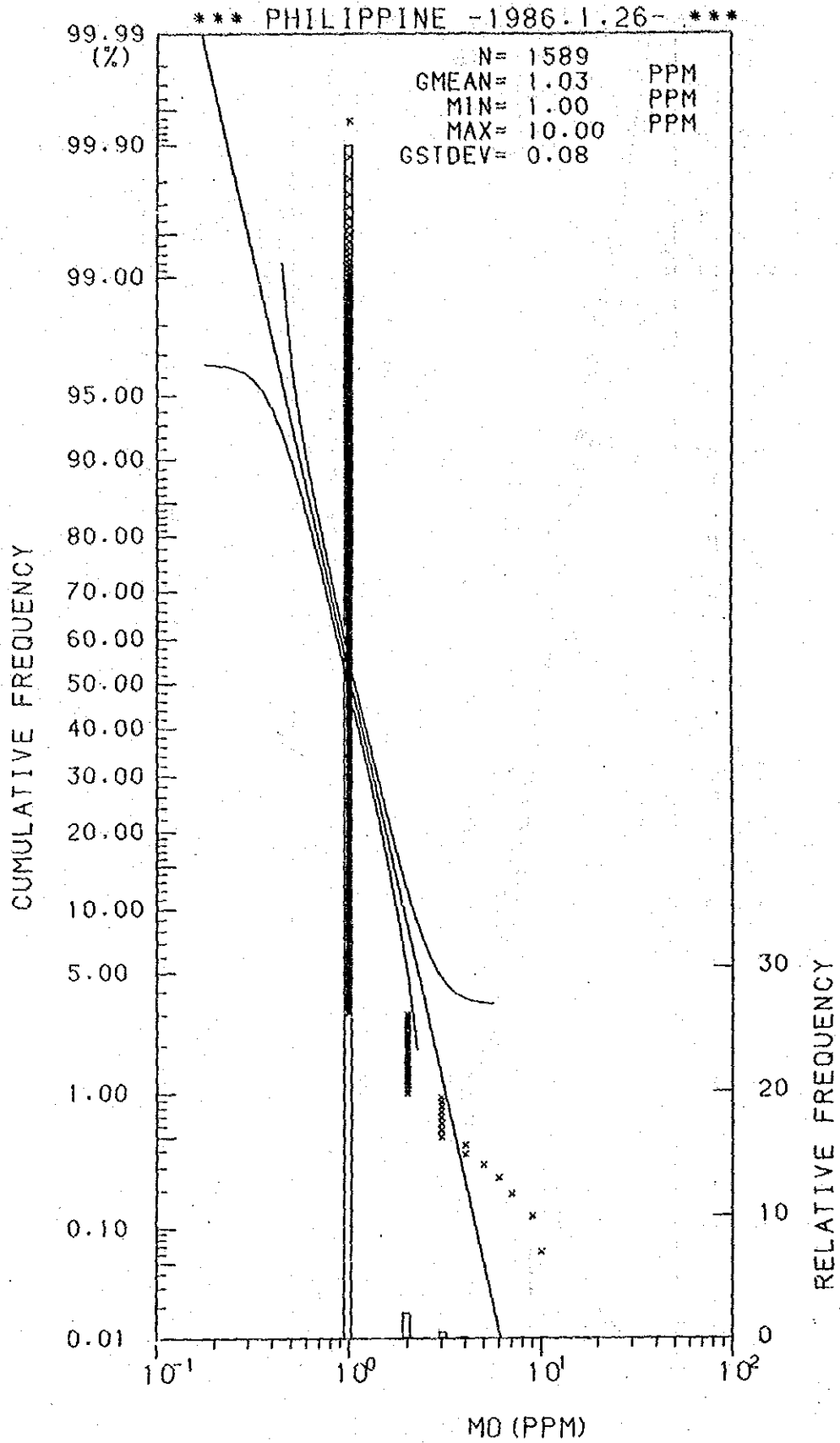
Histogram and Cumulative Frequency Curve of Mo content in Lithological Code; 0.4.
