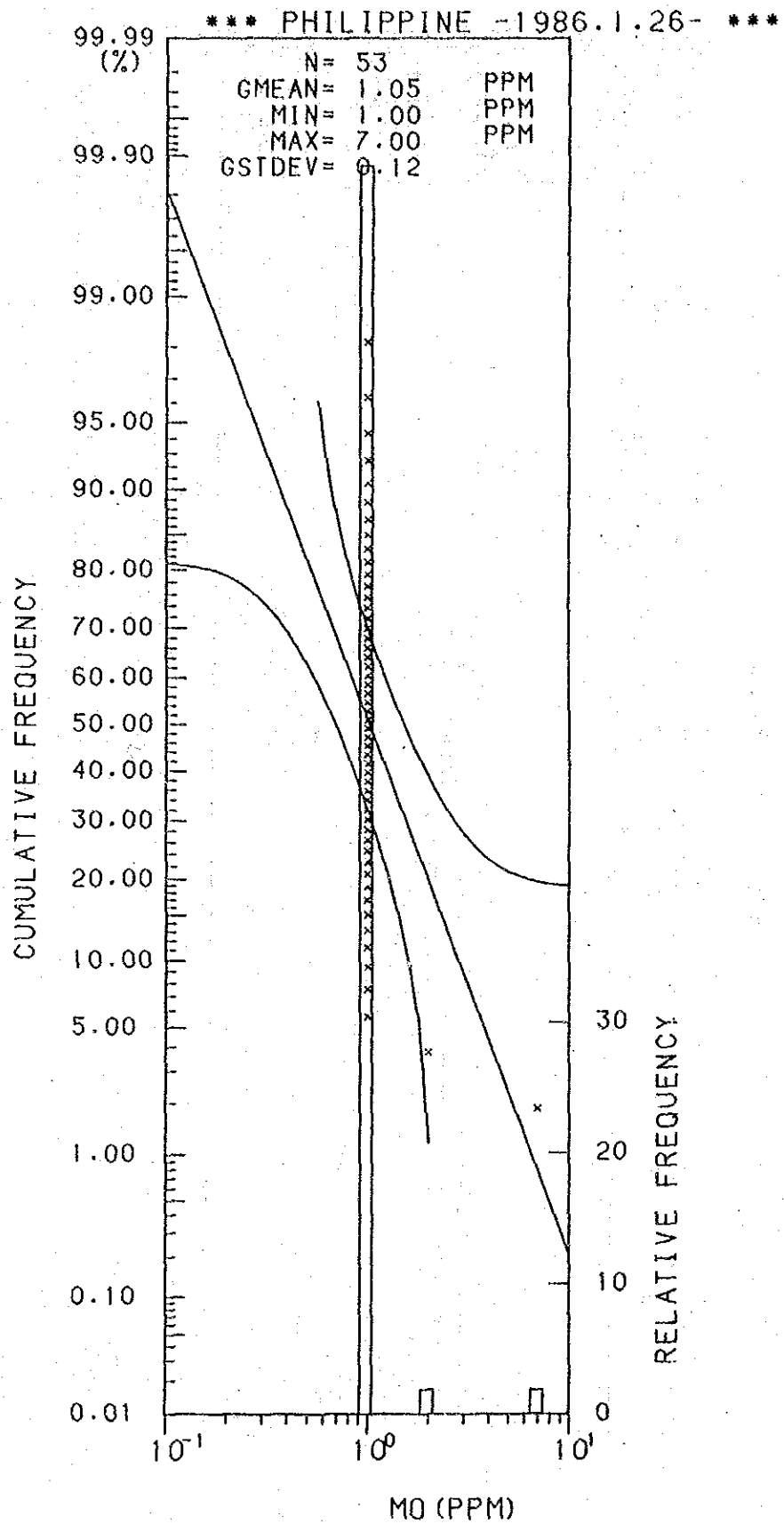
Histogram and Cumulative Frequency Curve of Mo content in Lithological Code; 0.9.
