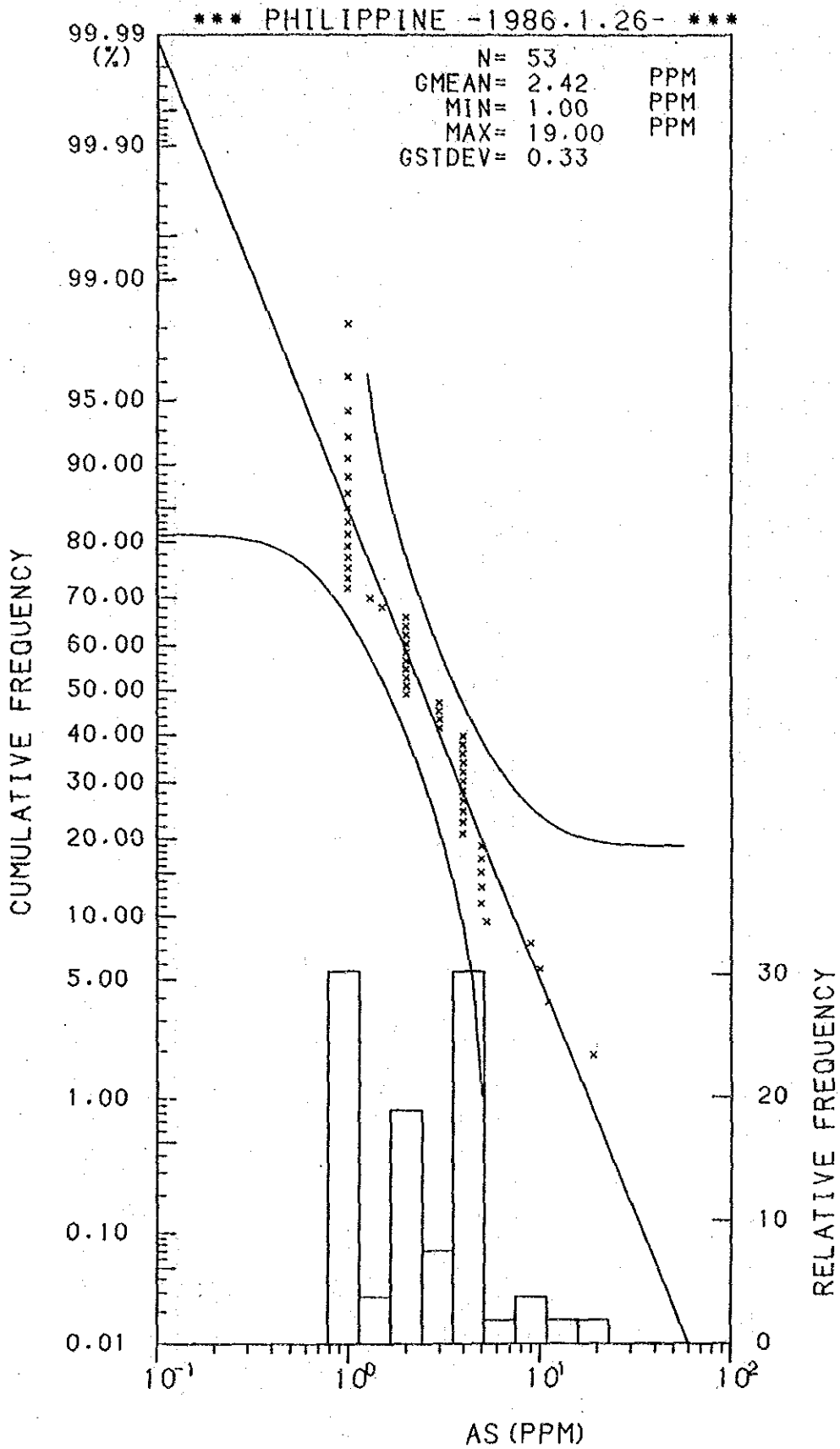
Histogram and Cumulative Frequency Curve of As content in Lithological Code; 0.9.
