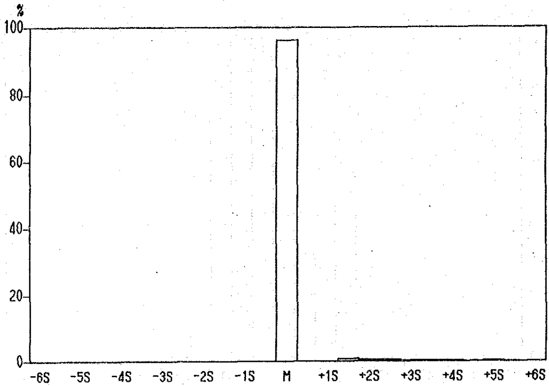
Higtograms of Hg content in all Samples.
