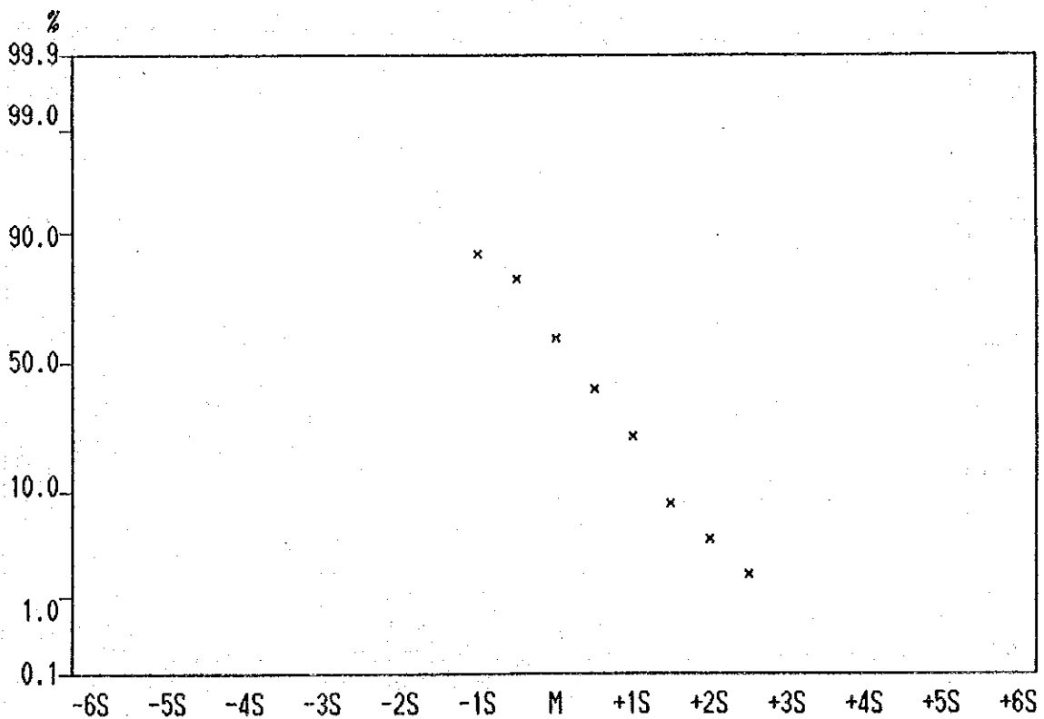
Cumulative Frequency Curve of As contents in Lithological Code; KPS
