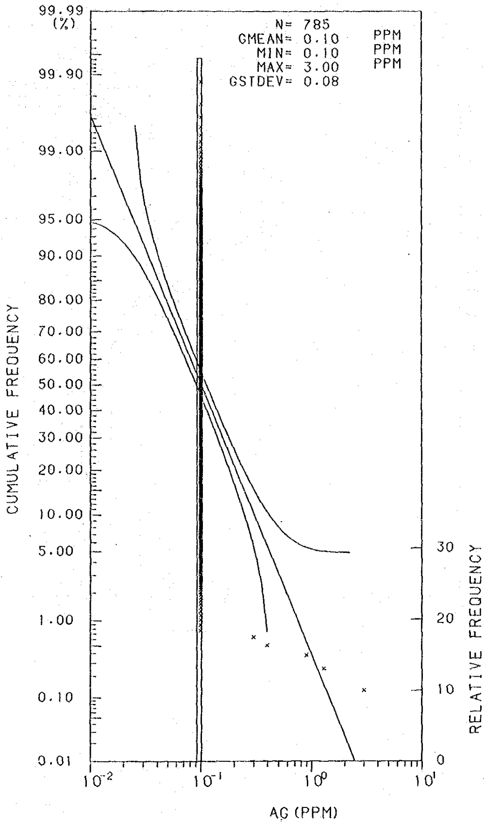
Histogram and Cumulative Frequency Curve of Ag Content in All Samples.
