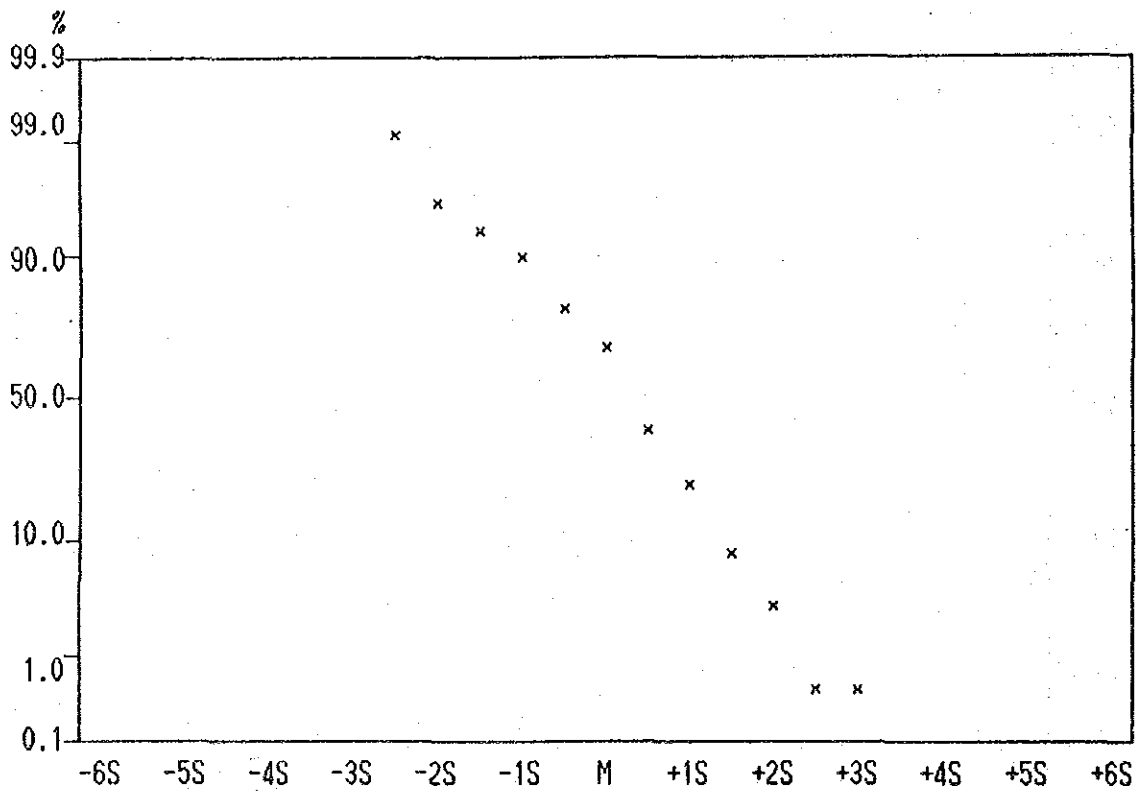
Cumulative Frequency Curve of Ni contents in Lithological Code; KPS
