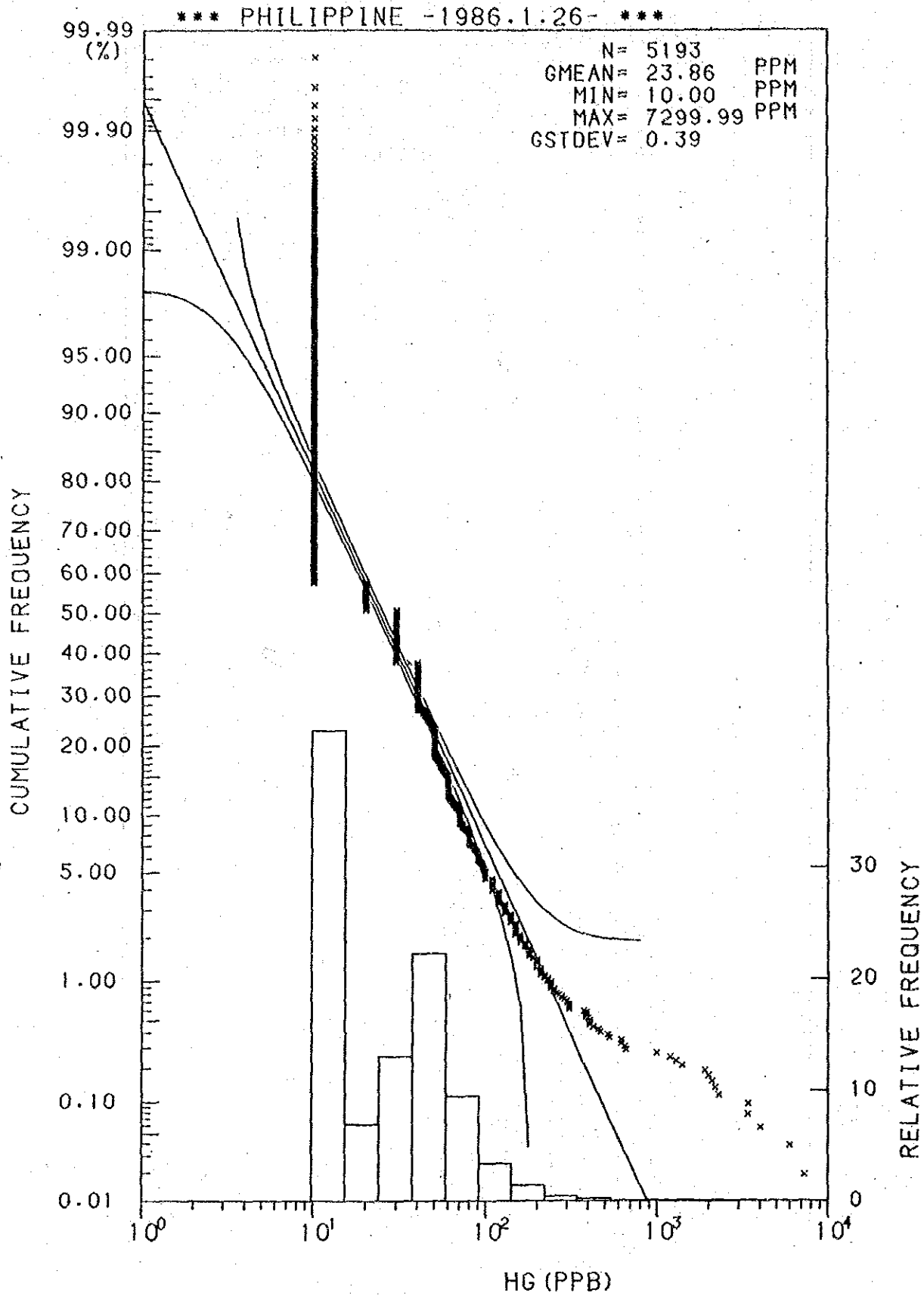
Histogram and Cumulative Frequency Curve of Hg content in All Samples.
