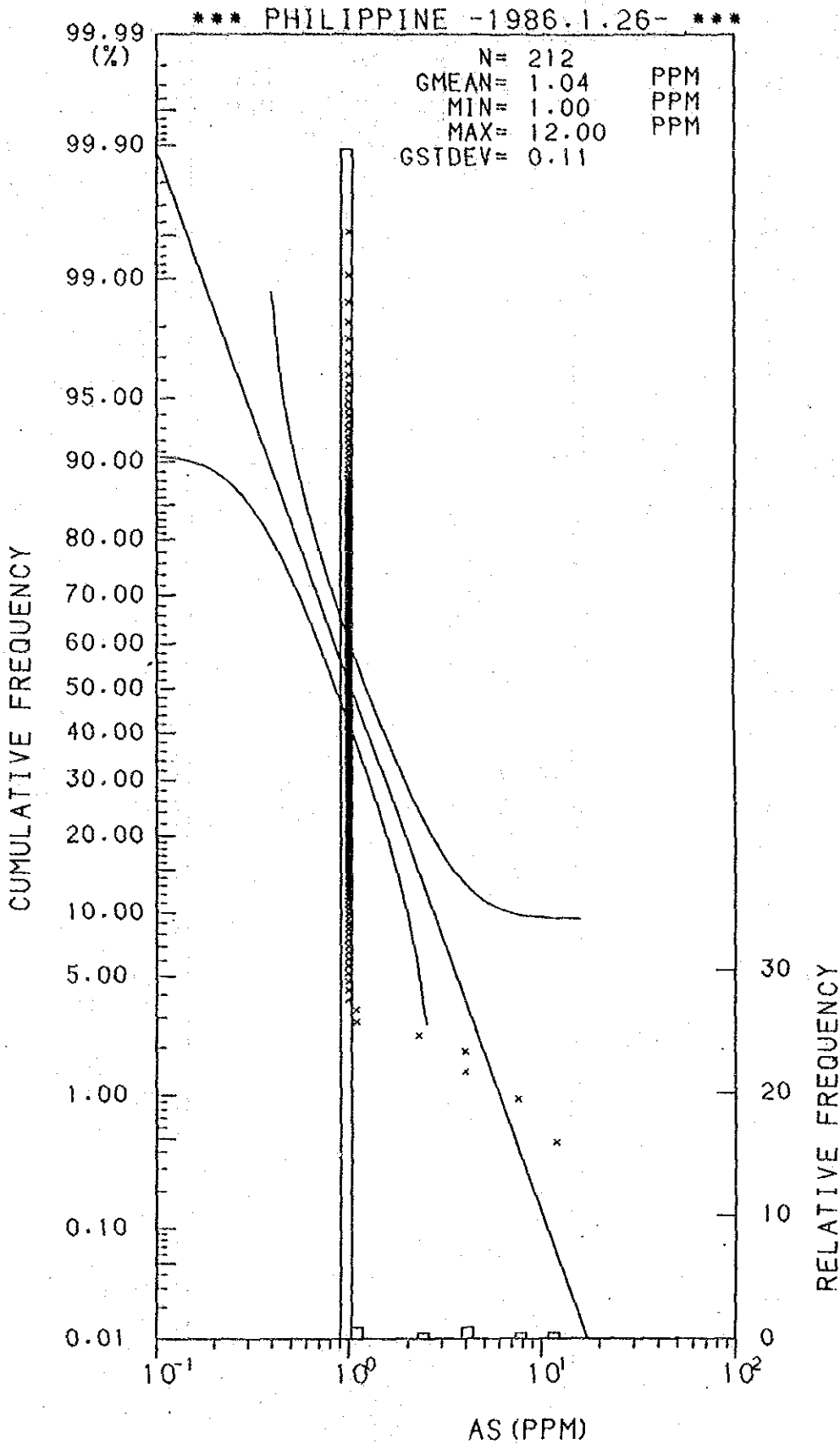
Histogram and Cumulative Frequency Curve of As content in Lithological Code; 0.7.
