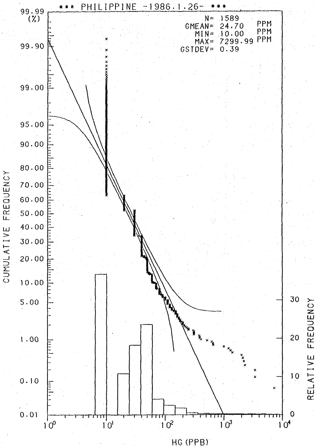
Histogram and Cumulative Frequency Curve of Hg content in Lithological Code; 0.4.
