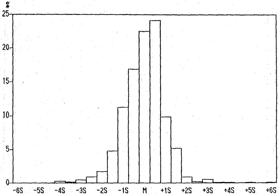
Histograms of Cu content in all Samples.
