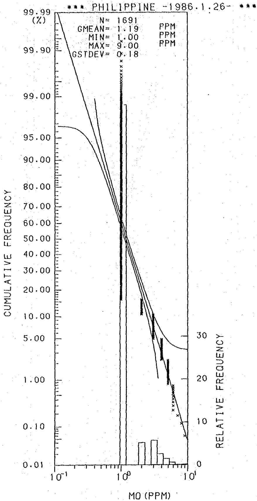
Histogram and Cumulative Frequency Curve of Mo content in Lithological Code; 0.3.
