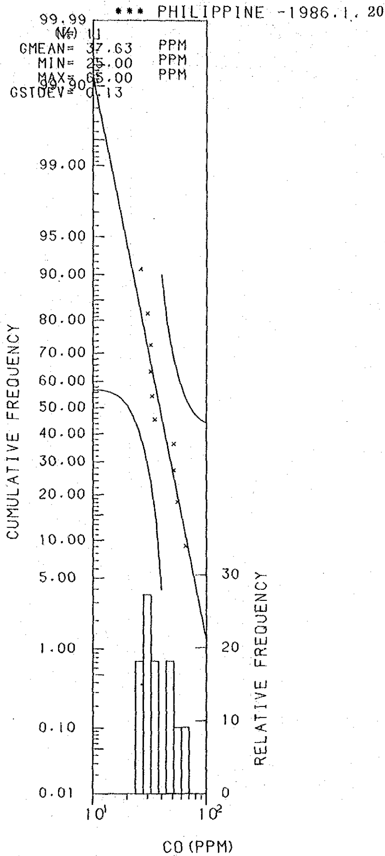
Histogram and Cumulative Frequency Curve of Co Content in Lithological Code; 0.2.
