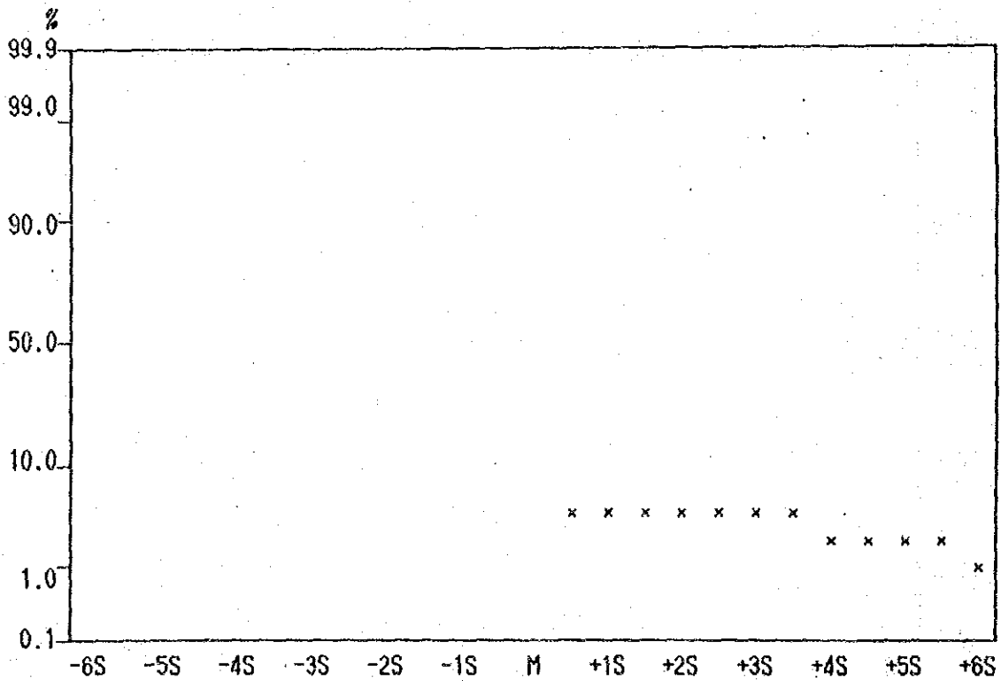
Cumulative Frequency Curve of Hg contents in Lithological Code; INR
