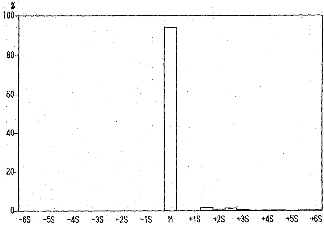
Histograms of Pb content in all Samples.
