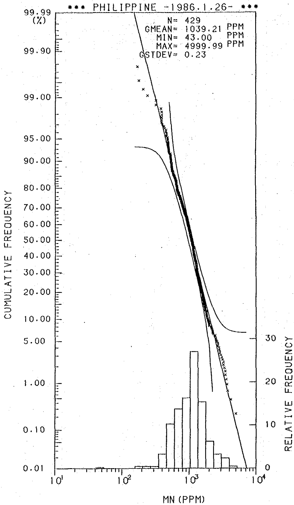
Histogram and Cumulative Frequency Curve of Mn content in Lithological Code; 0.8.
