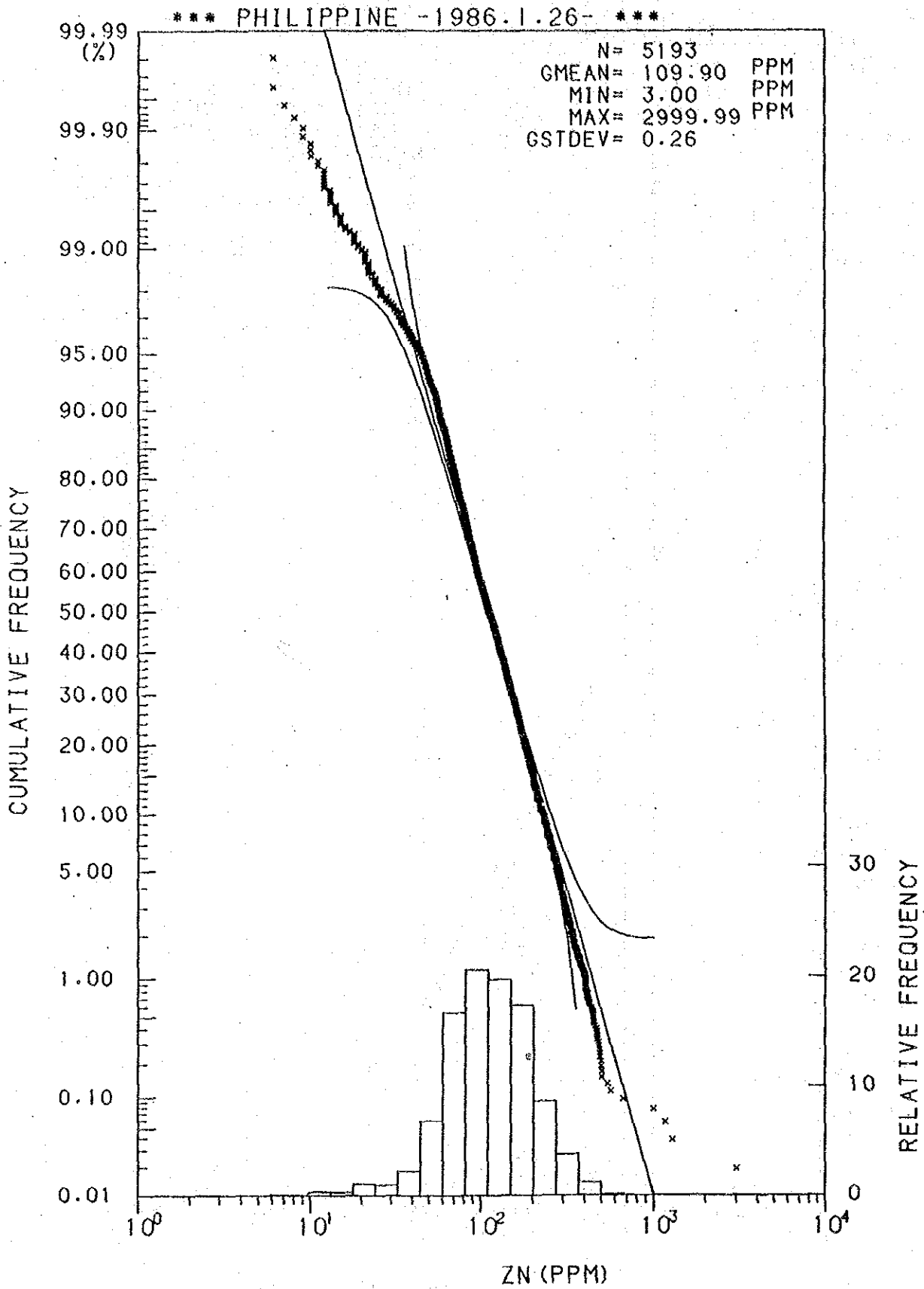
Histogram and Cumulative Frequency Curve of Zn content in All Samples.
