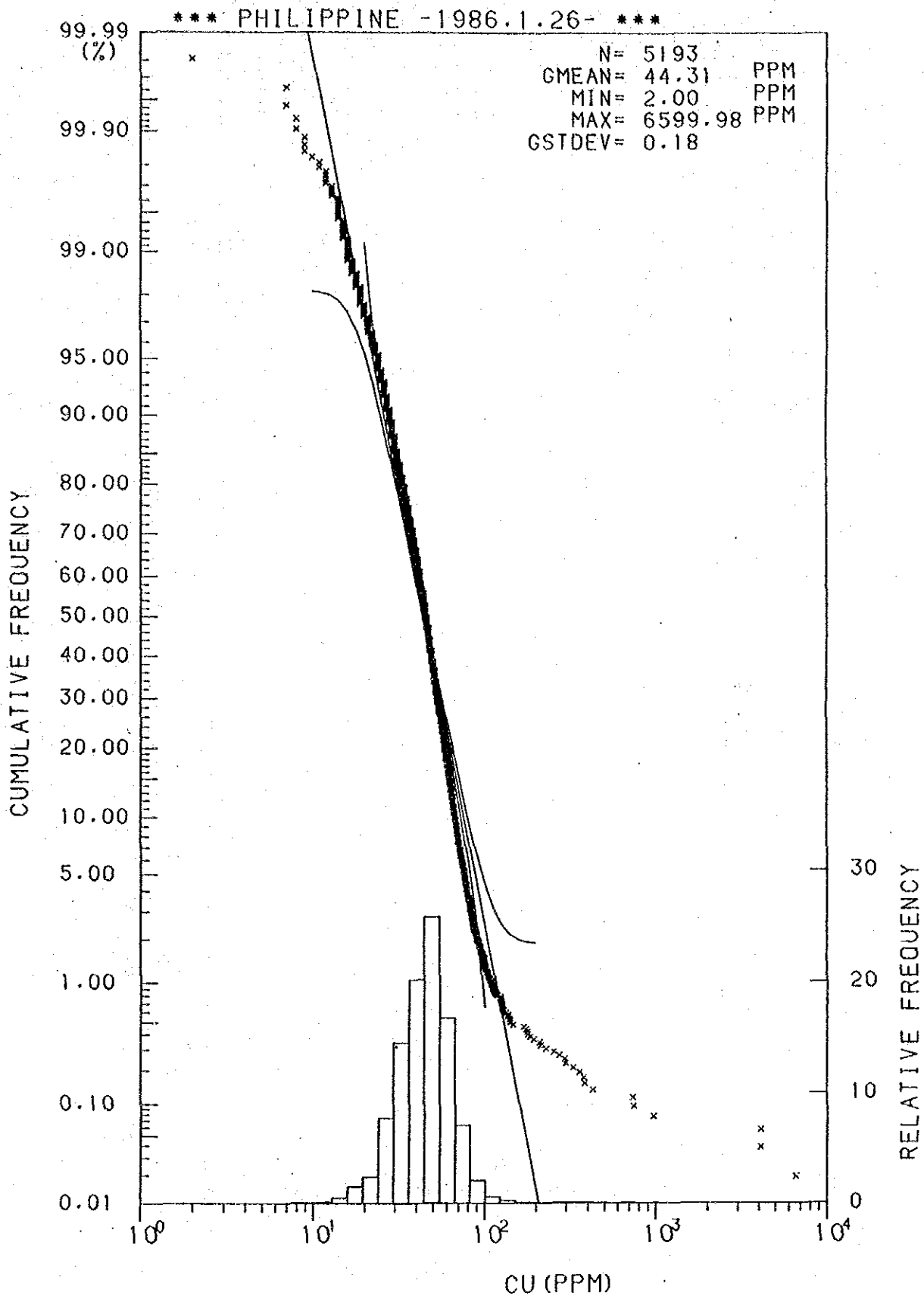
Histogram and Cumulative Frequency Curve of Cu content in All Samples.
