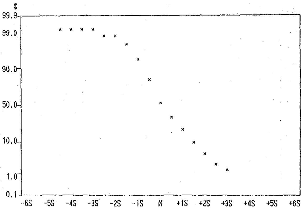
Cumulative Frequency Curve of Zn contents in Lithological Code; KPS
