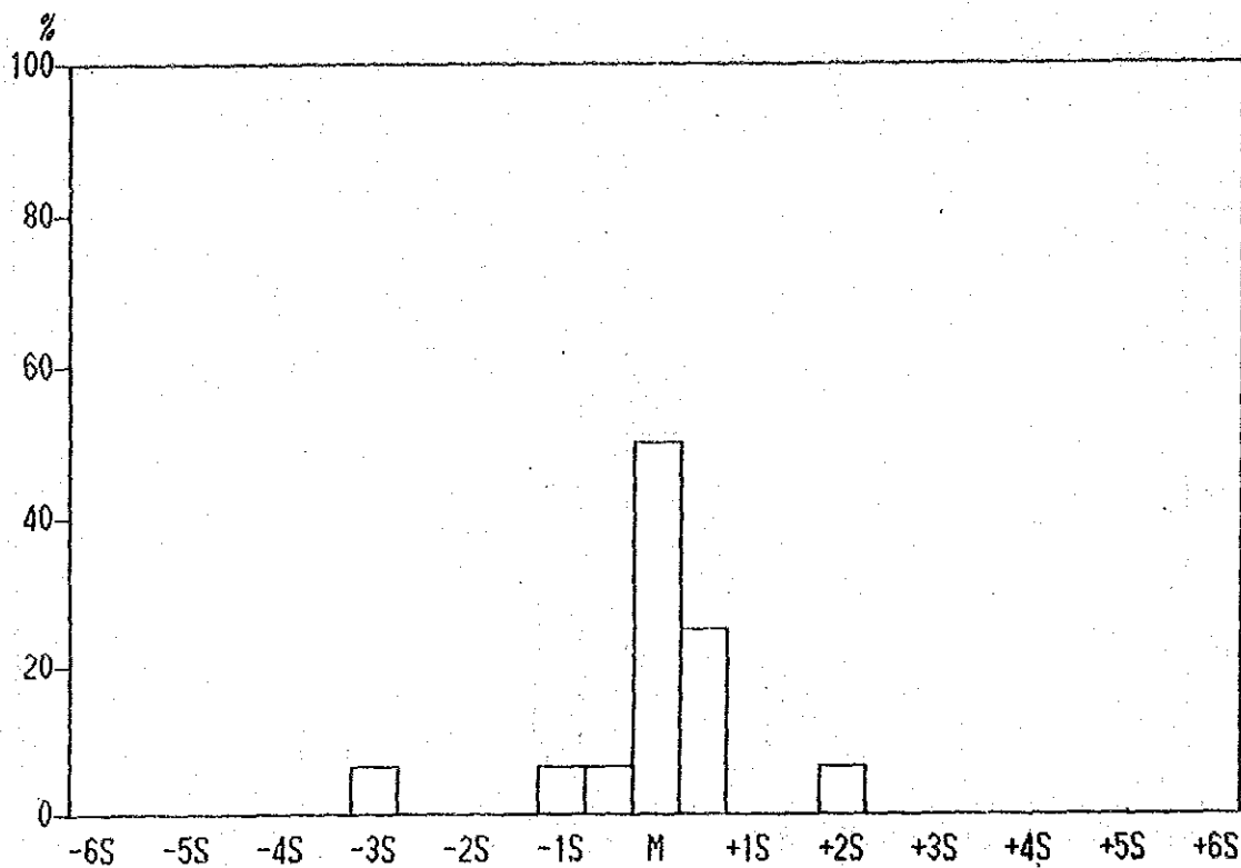
Histogram of Mn contents in Lithological Code; KPL
