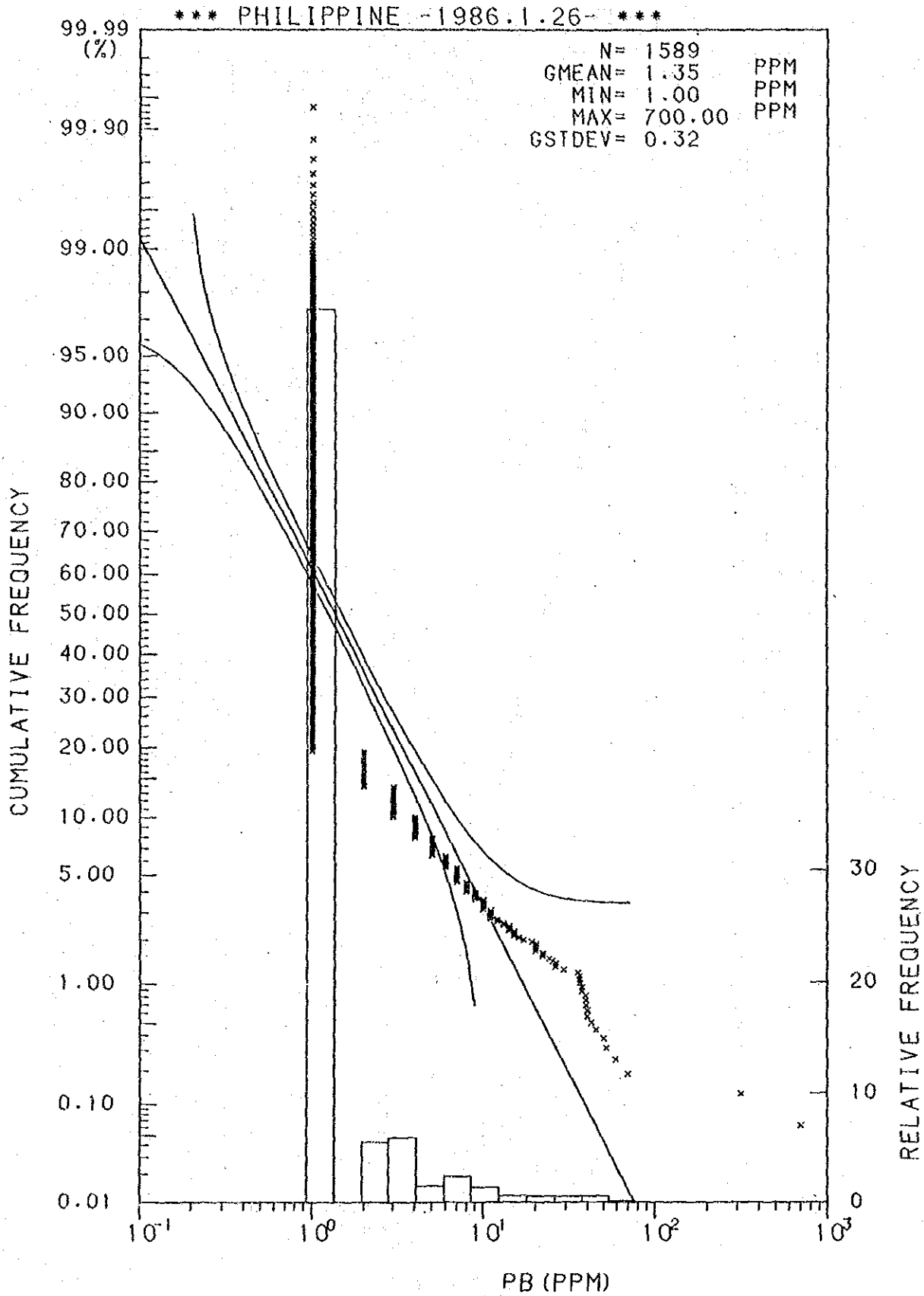
Histogram and Cumulative Frequency Curve of Pb content in Lithological Code; 0.4.
