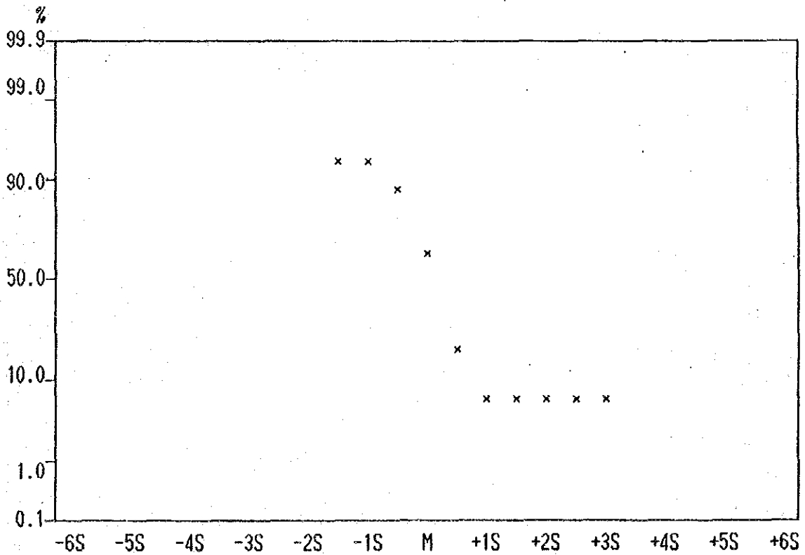
Cumulative Frequency Curve of Co contents in Lithological Code; KPL
