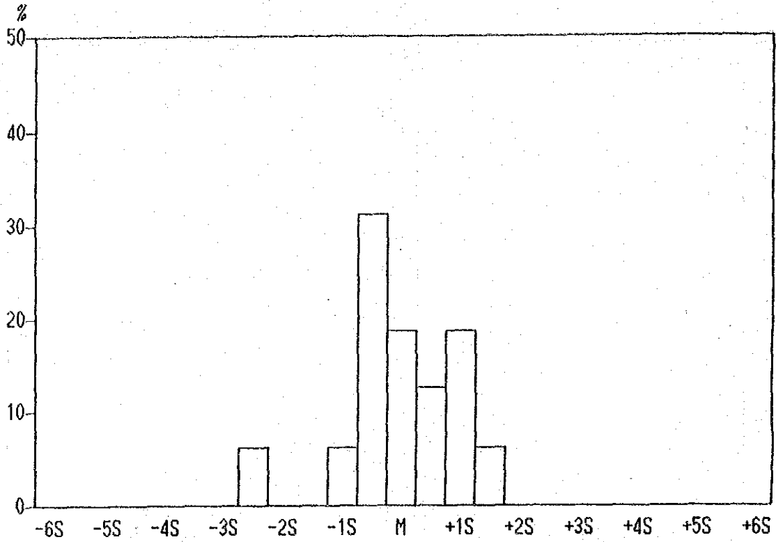
Histogram of Zn contents in Lithological Code; KPL
