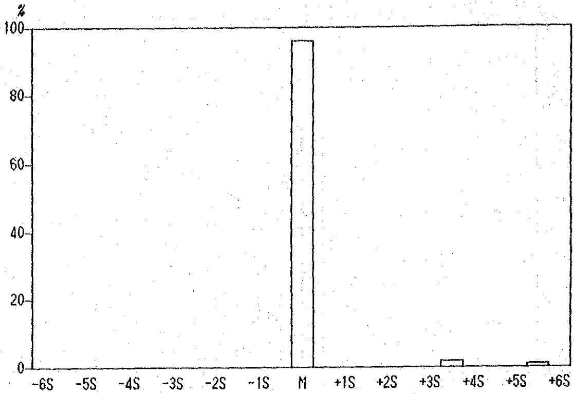
Histogram of Hg contents in Lithological Code; INR
