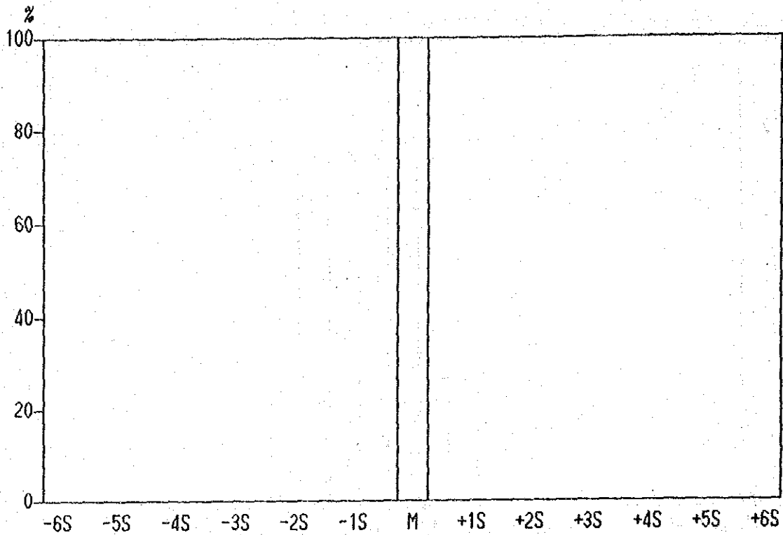
Histogram of Hg contents in Lithological Code; KPL
