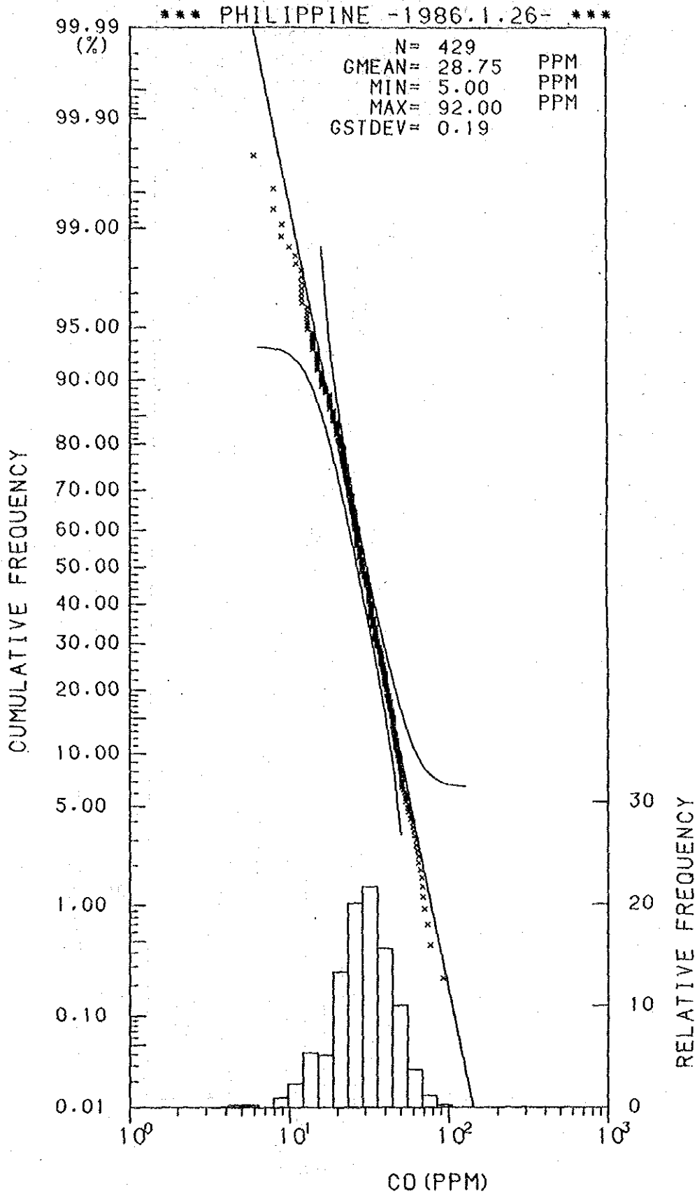
Histogram and Cumulative Frequency Curve of Co content in Lithological Code; 0.8.
