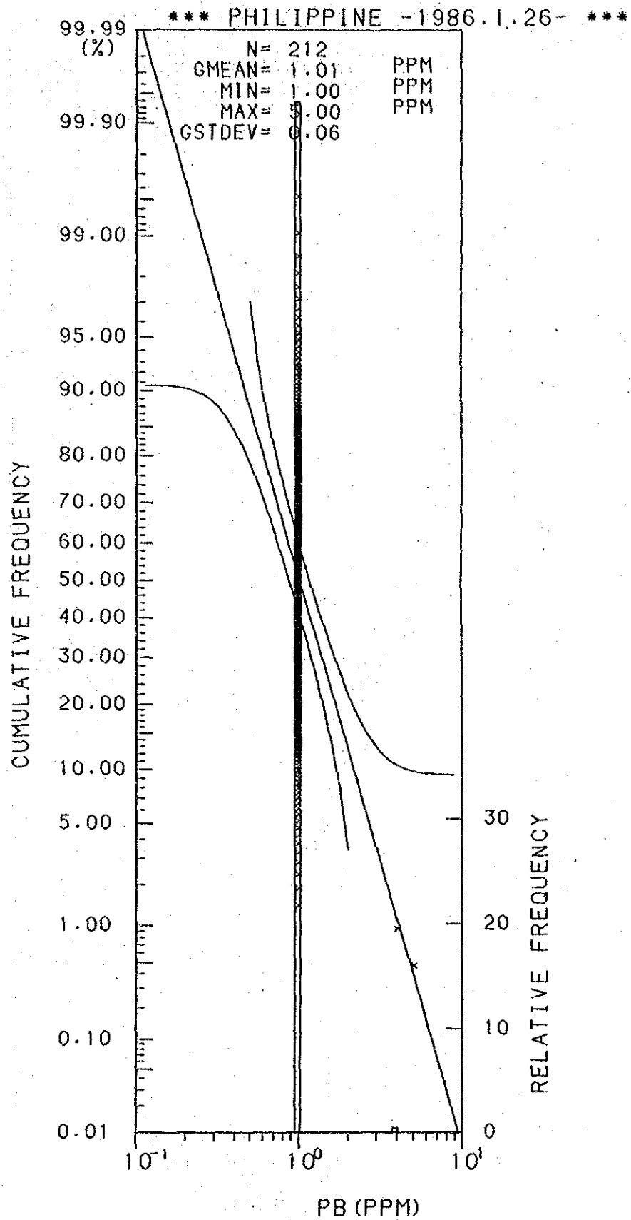
Histogram and Cumulative Frequency Curve of Pb content in Lithological Code; 0.7.
