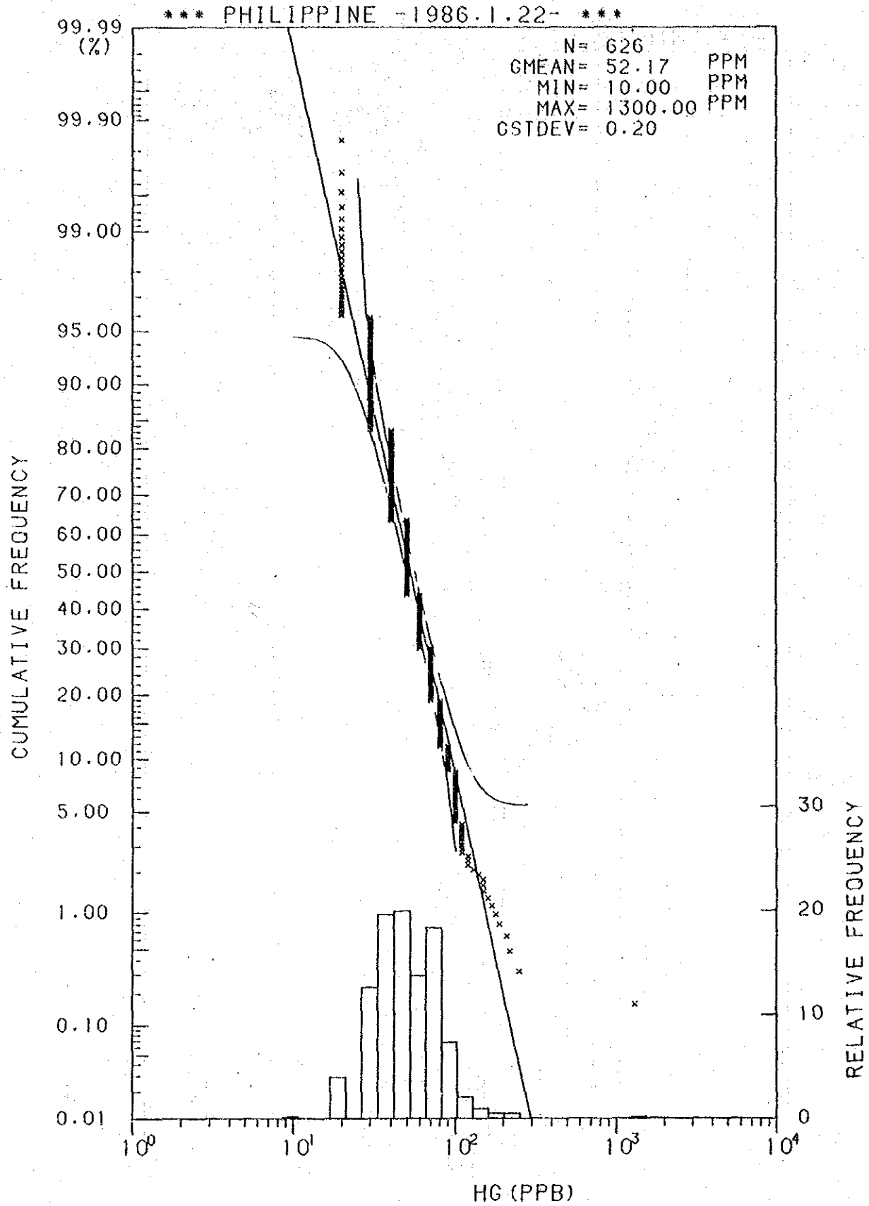
Histogram and Cumulative Frequency Curve of Hg Content in Lithological Code; 0.6.
