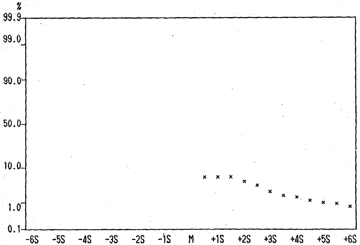
Cumulative Frequency Curve of Pb content in all Samples.
