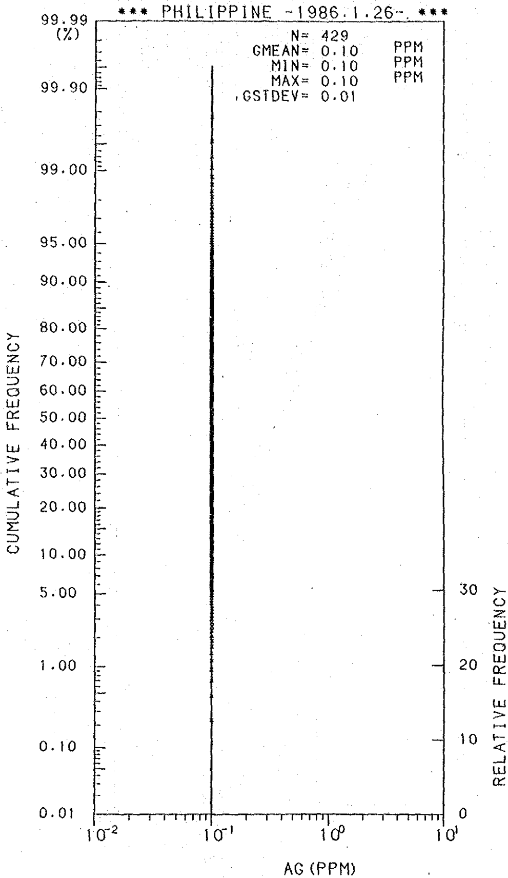
Histogram and Cumulative Frequency Curve of AG content in Lithological Code; 0.8.
