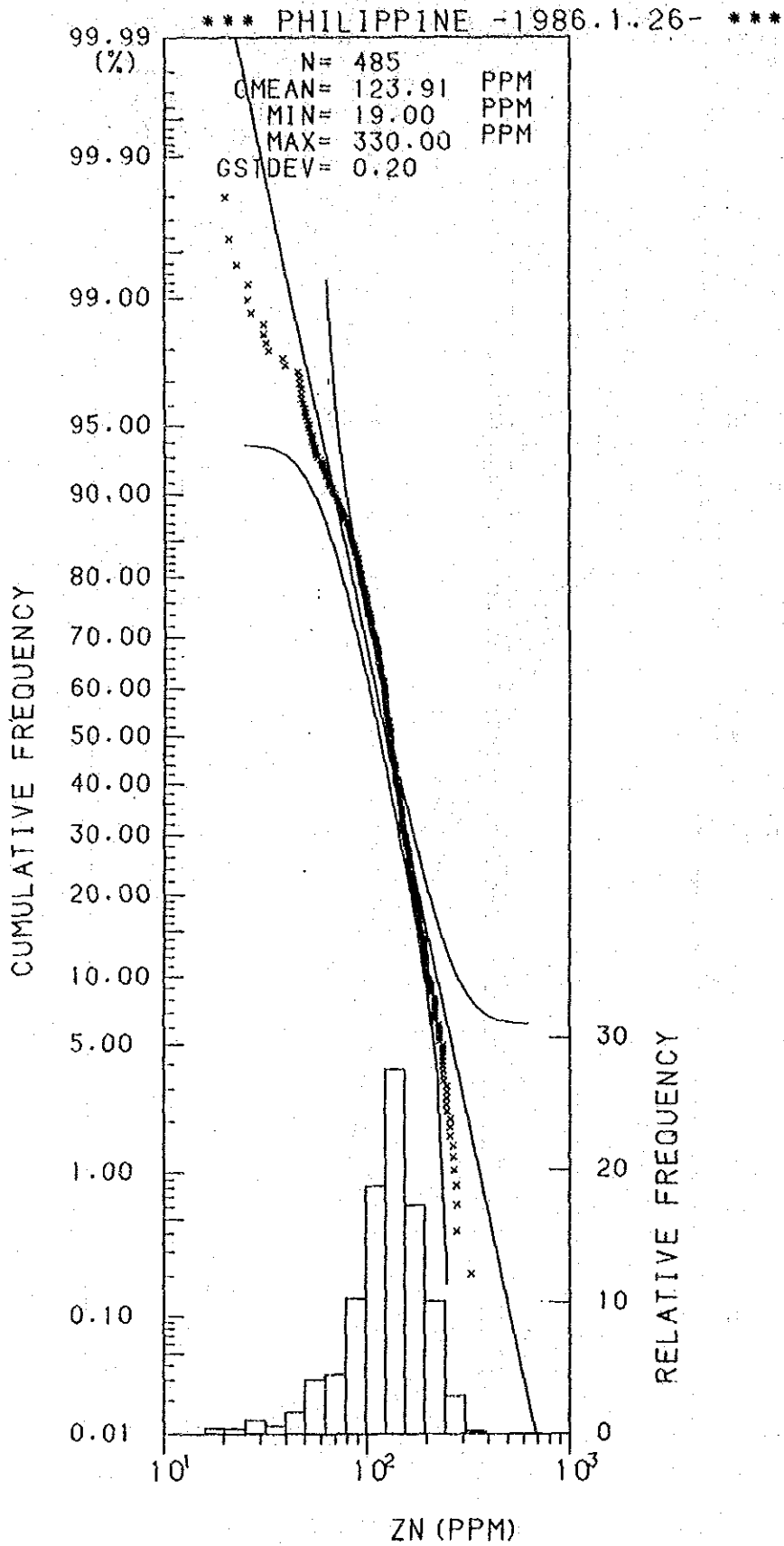
Histogram and Cumulative Frequency Curve of Zn content in Lithological Code; 0.1.
