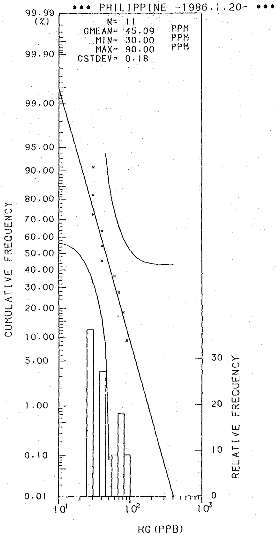
Histogram and Cumulative Frequency Curve of Hg Content in Lithological Code; 0.2.
