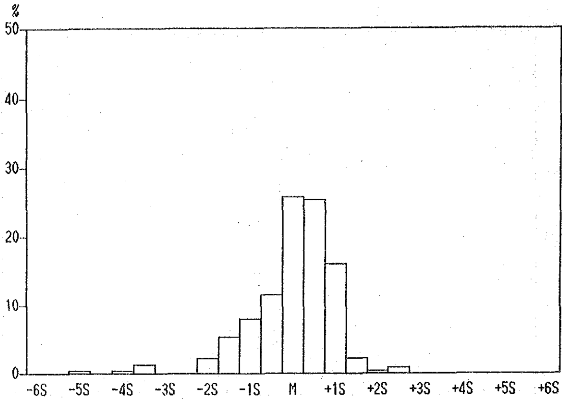
Histogram of Mn contents in Lithological Code; KPS
