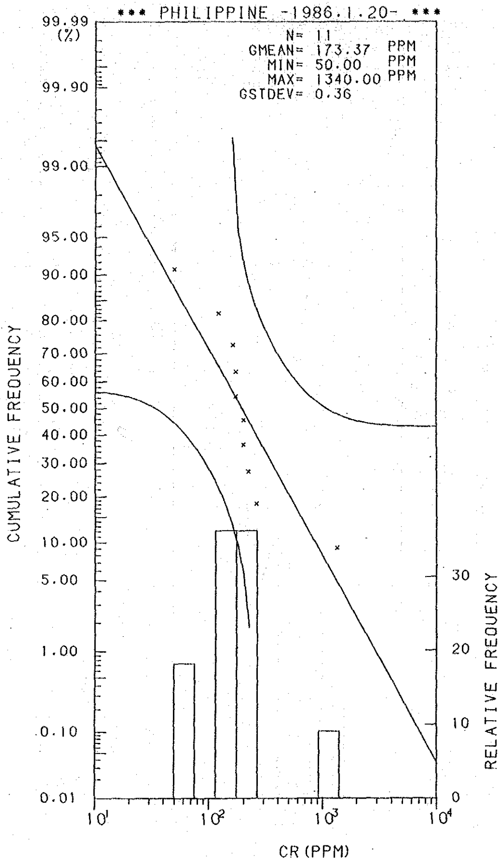
Histogram and Cumulative Frequency Curve of Cr Content in Lithological Code; 0.2.
