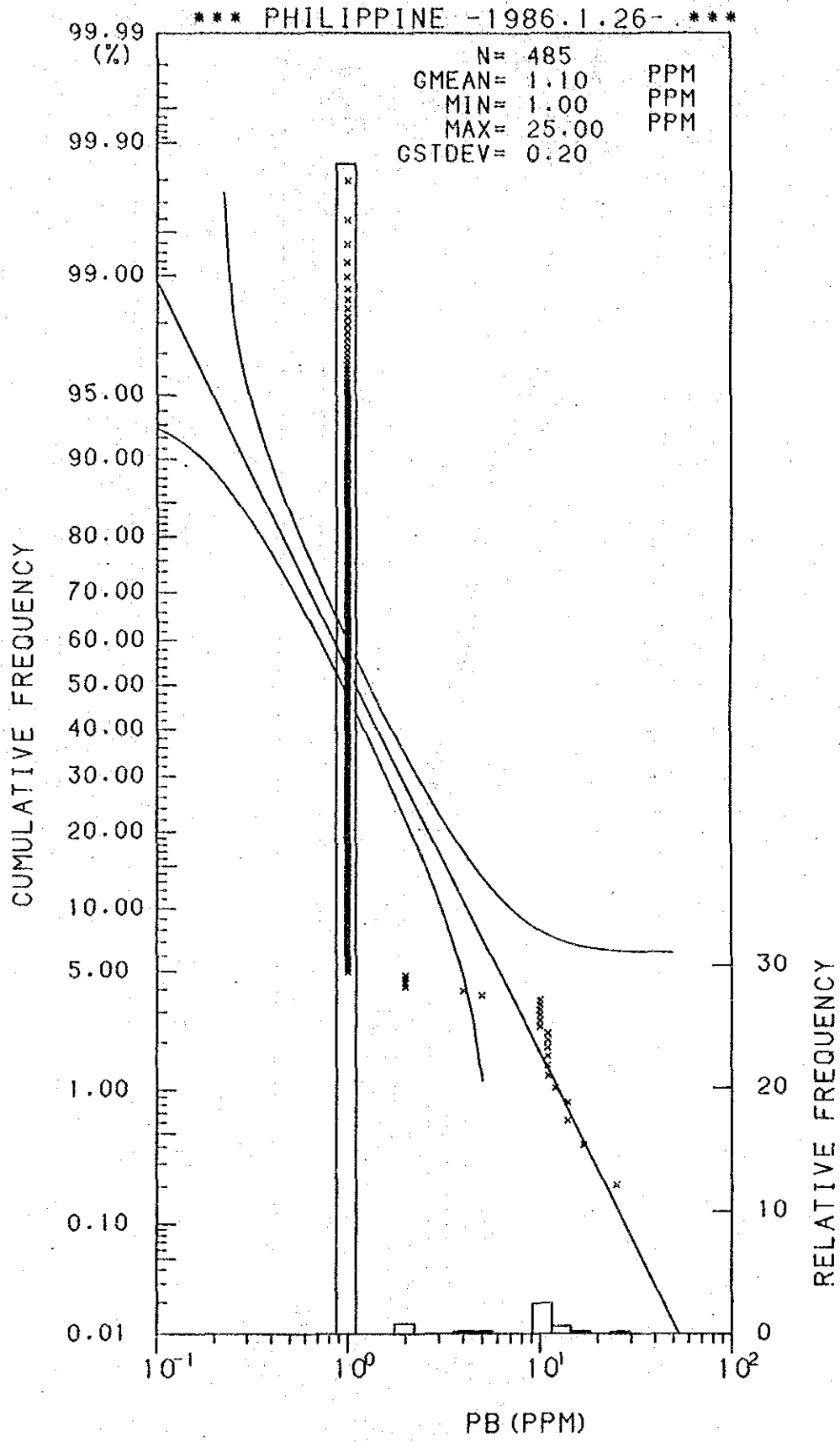
Histogram and Cumulative Frequency Curve of Pb content in Lithological Code; 0.1.
