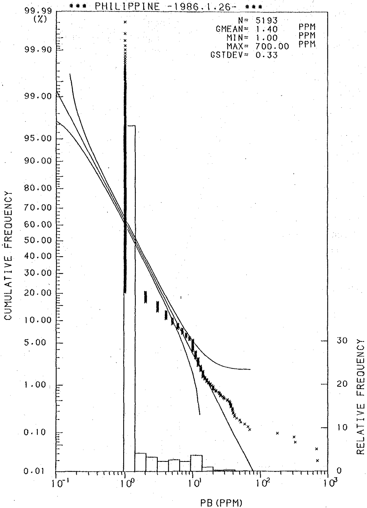
Histogram and Cumulative Frequency Curve of Pb content in All Samples.
