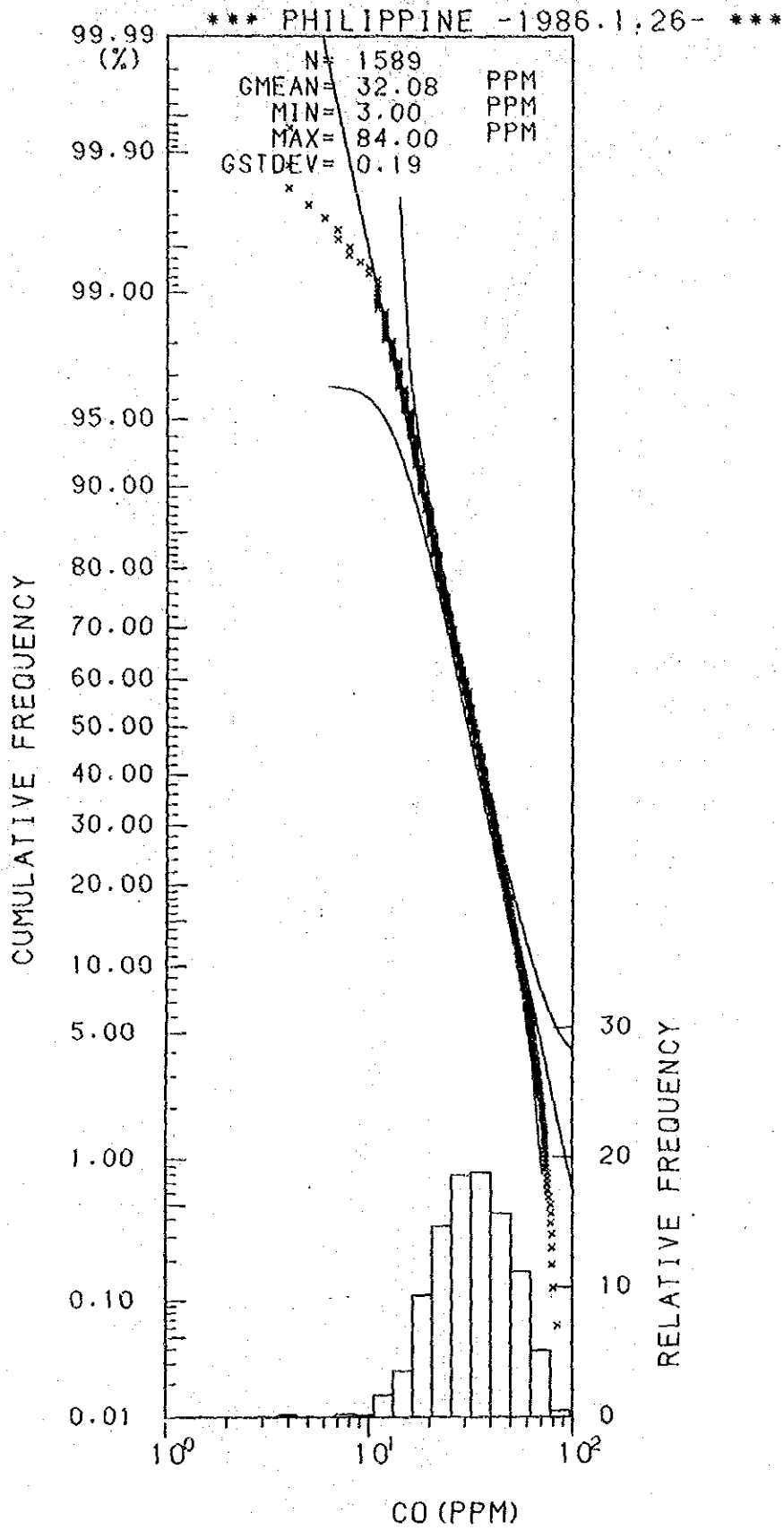
Histogram and Cumulative Frequency Curve of Co content in Lithological Code; 0.4.
