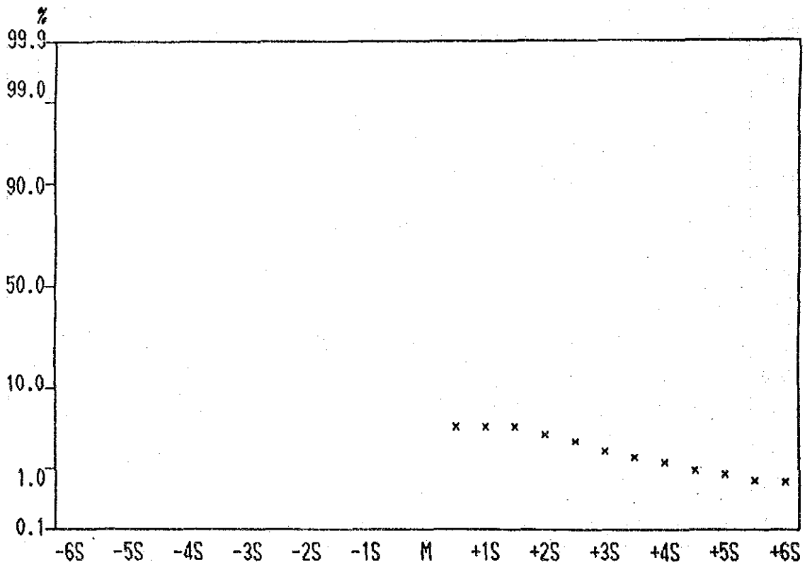
Cumulative Frequency Curve of Hg content in all Samples.
