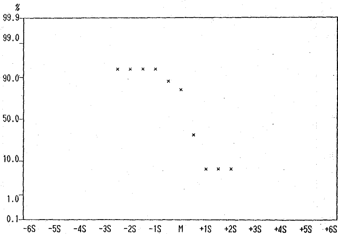
Cumulative Frequency Curve of Mn contents in Lithological Code; KPL
