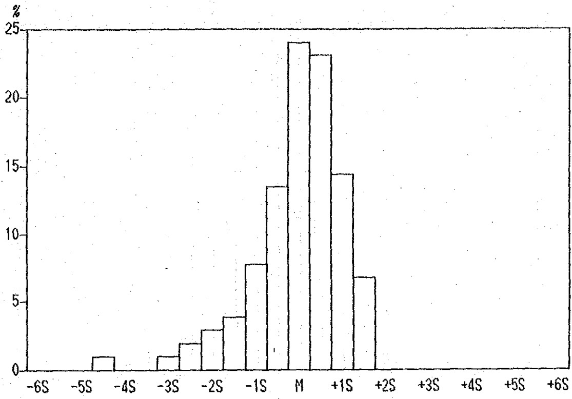
Histogram of Co contents in Lithological Code; INR
