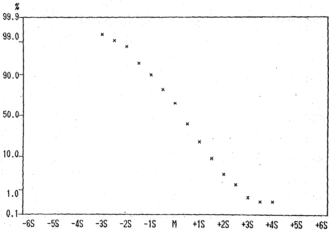
Cumulative Frequency Curve of Zn content in all Samples.
