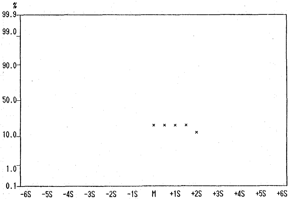
Cumulative Frequency Curve of Pb contents in Lithological Code; KPL
