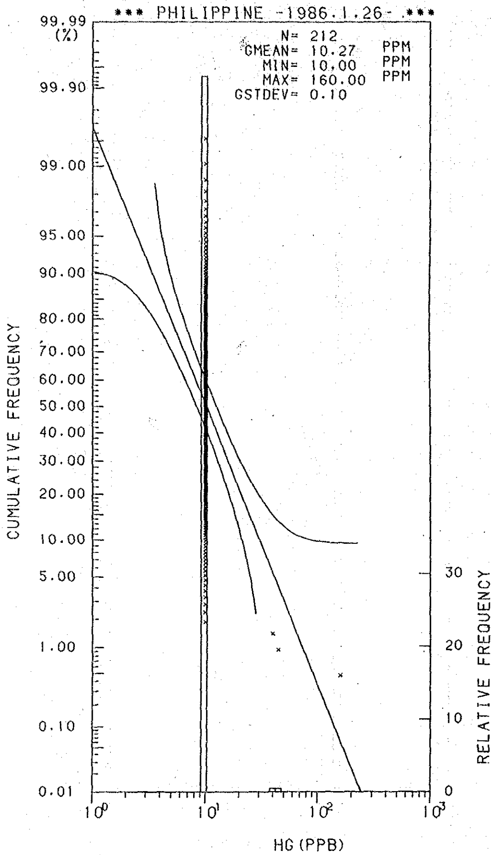
Histogram and Cumulative Frequency Curve of Hg content in Lithological Code; 0.7.
