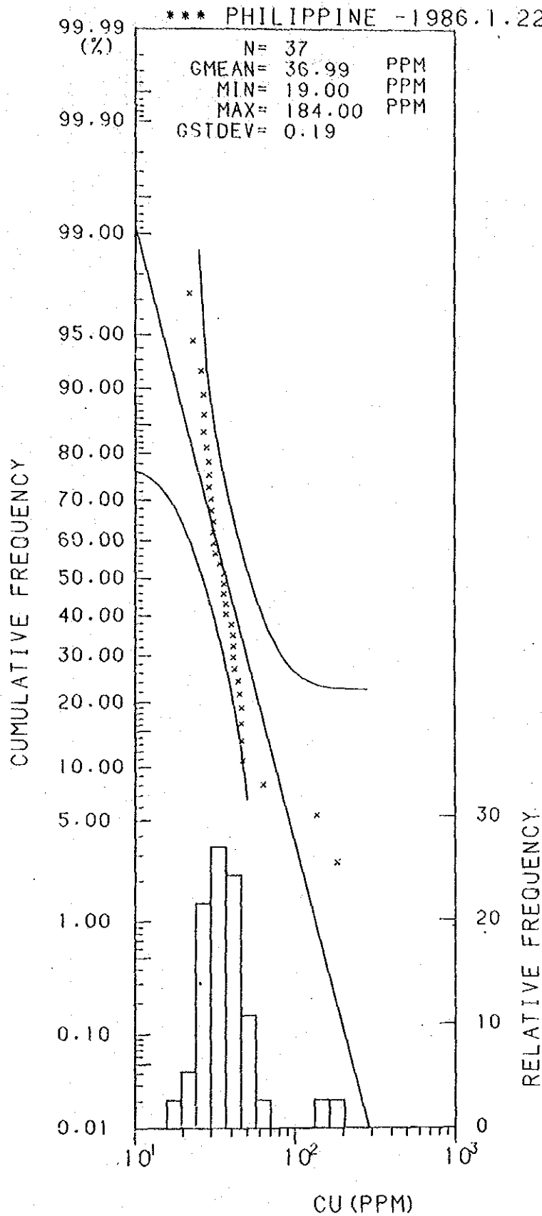
Histogram and Cumulative Frequency Curve of Cu Content in Lithological Code; 0.7.
