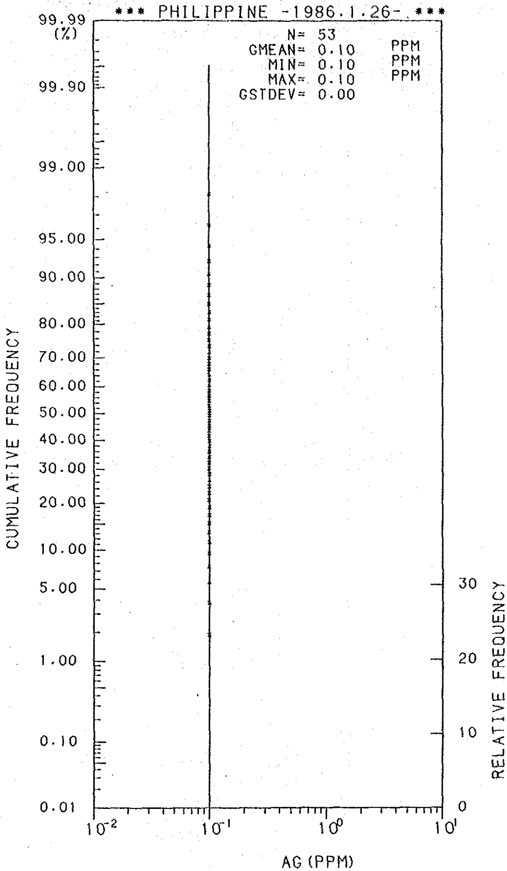
Histogram and Cumulative Frequency Curve of AG content in Lithological Code; 0.9.
