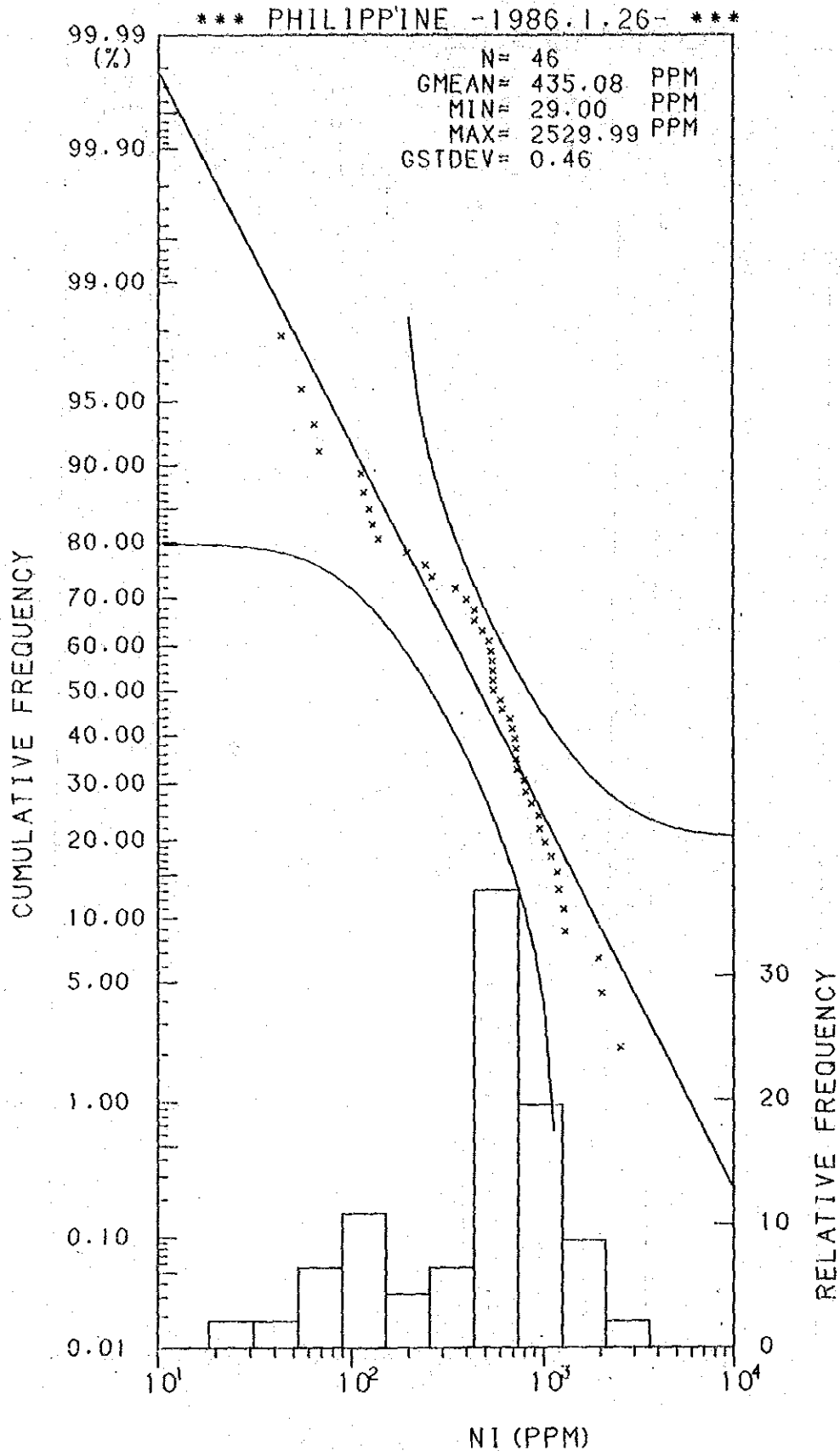
Histogram and Cumulative Frequency Curve of Ni content in Lithological Code; 0.6.
