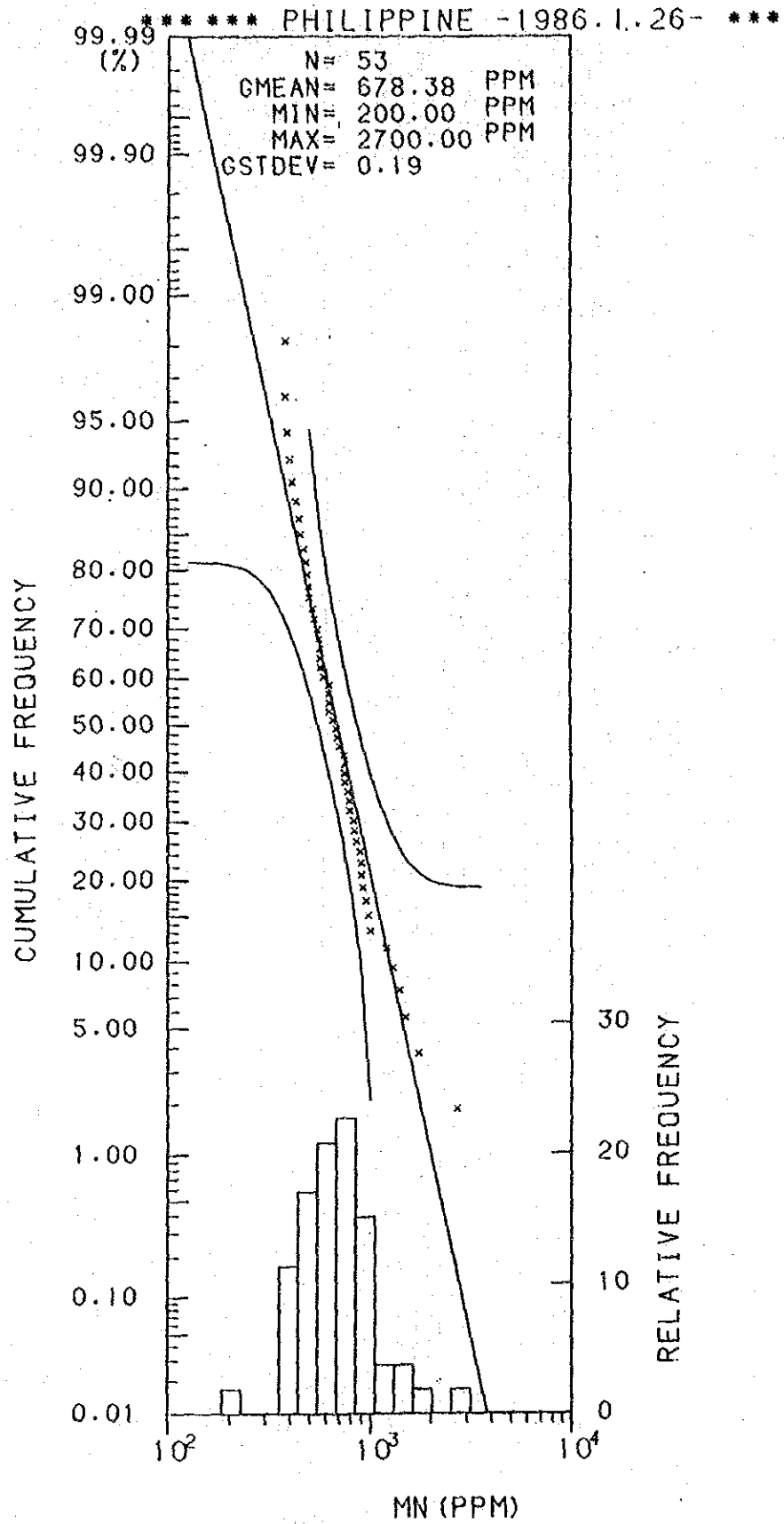
Histogram and Cumulative Frequency Curve of Mn content in Lithological Code; 0.9.
