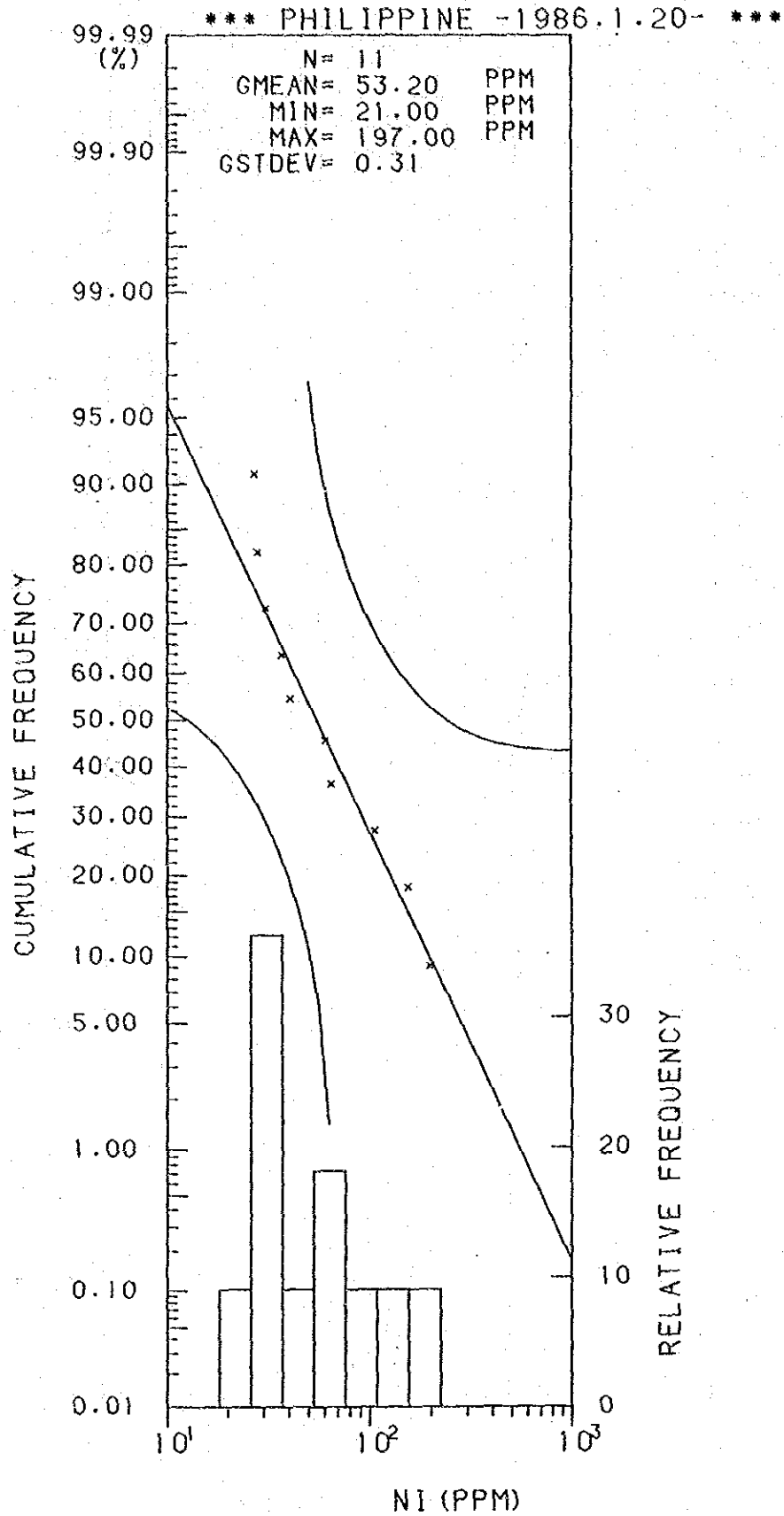
Histogram and Cumulative Frequency Curve of Ni Content in Lithological Code; 0.2.
