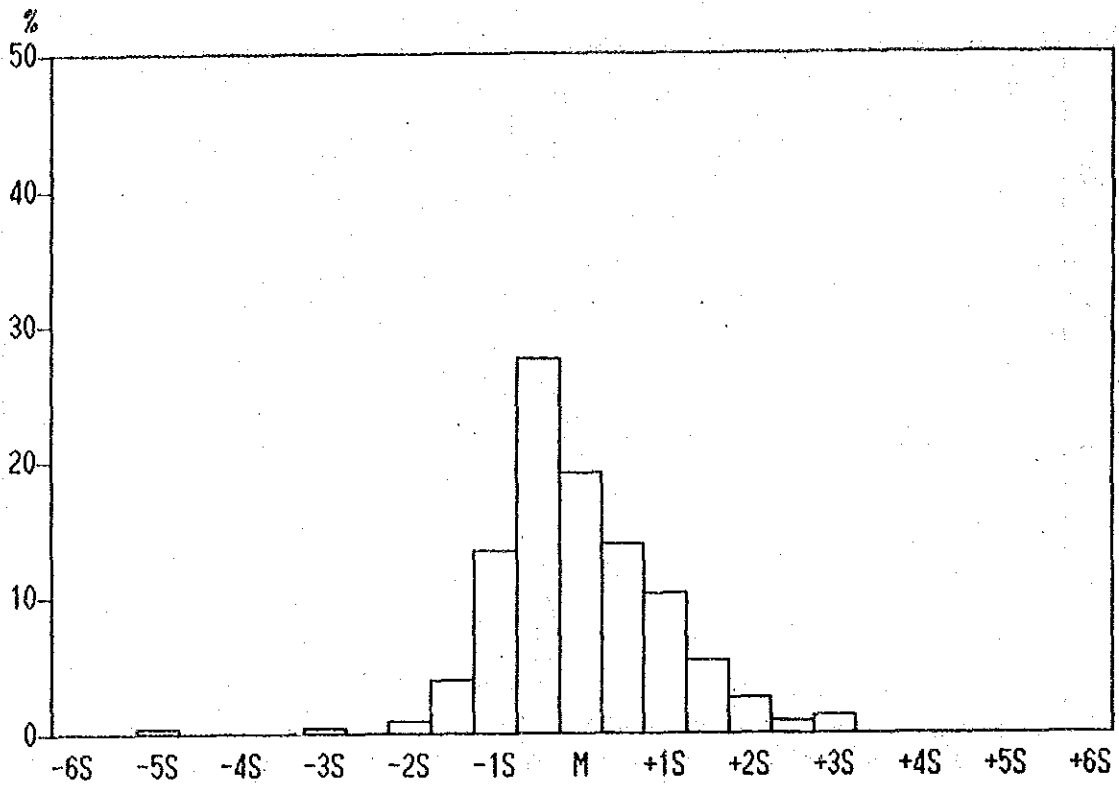
Histogram of Zn contents in Lithological Code; KPS
