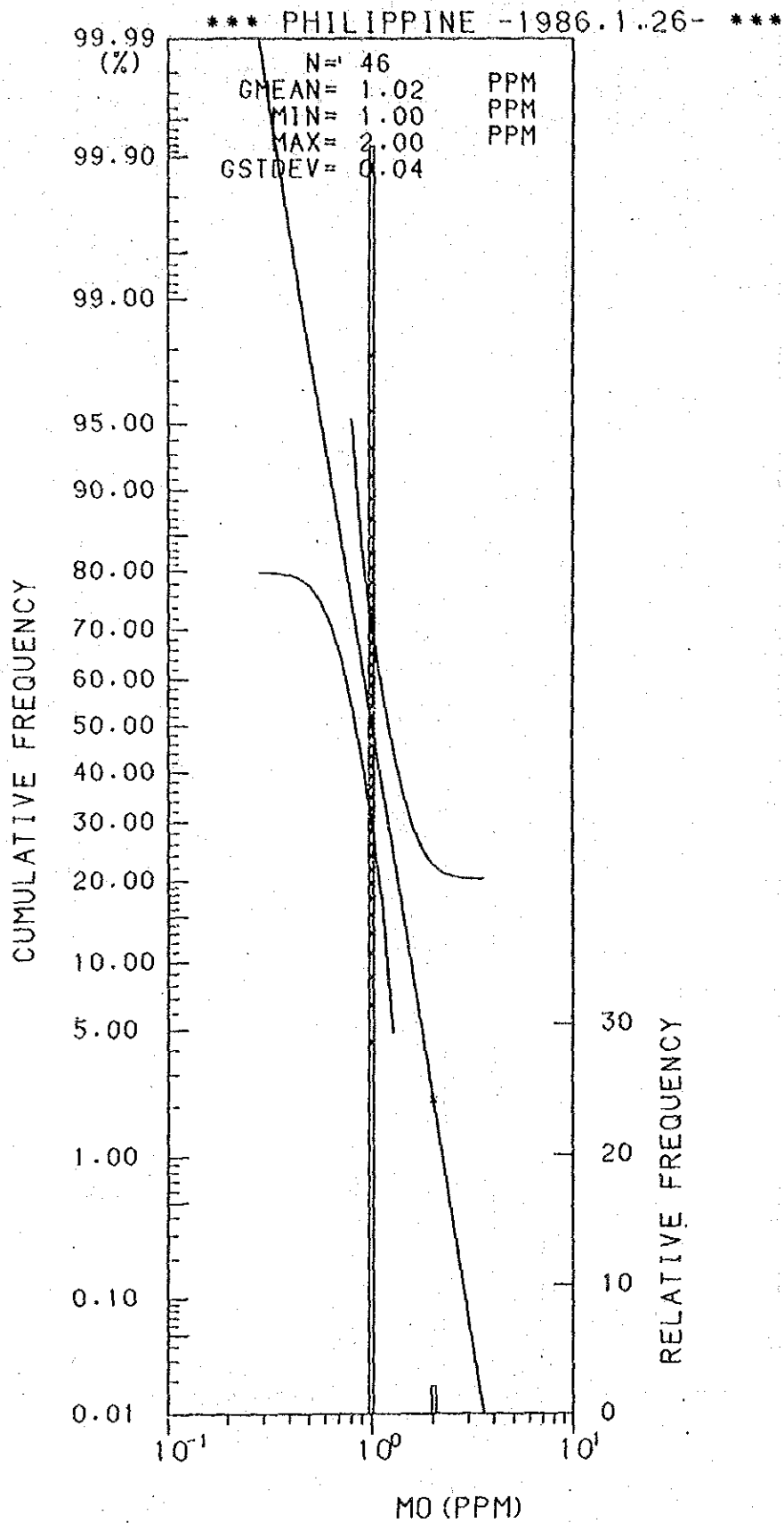
Histogram and Cumulative Frequency Curve of Mo content in Lithological Code; 0.6.
