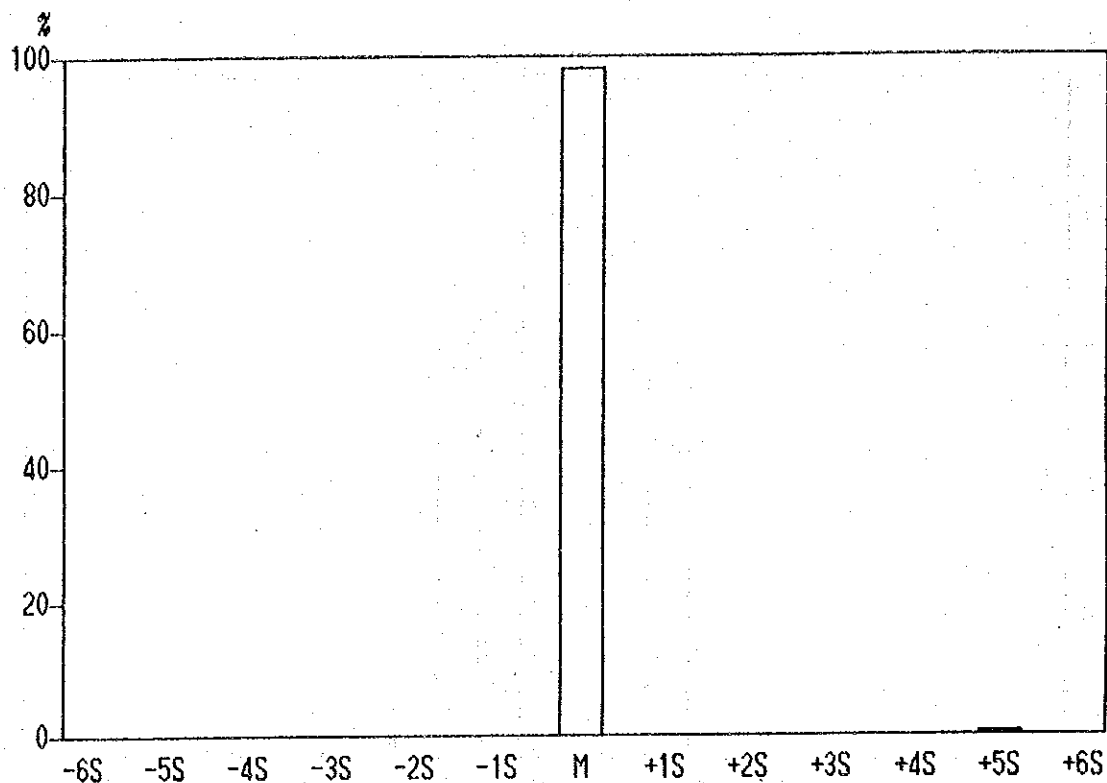
Histogram of Hg contents in Lithological Code; KPS
