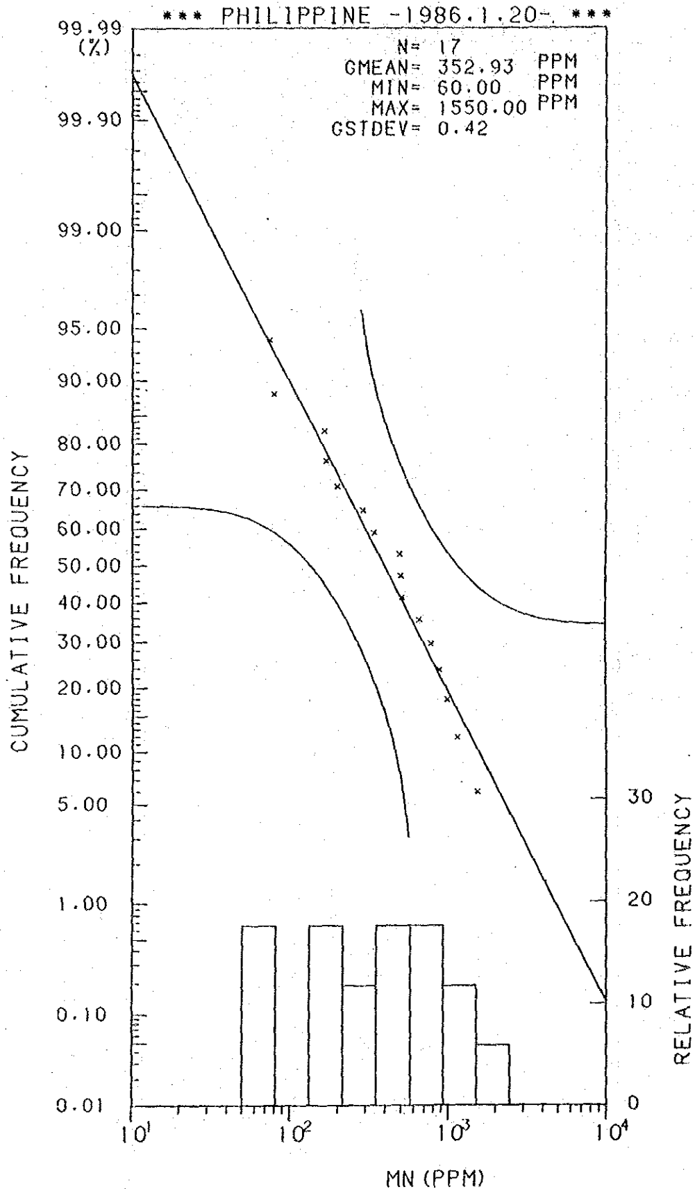
Histogram and Cumulative Frequency Curve of Mn Content in Lithological Code; 0.4.
