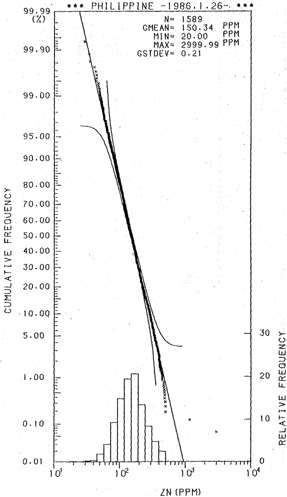
Histogram and Cumulative Frequency Curve of Zn content in Lithological Code; 0.4.
