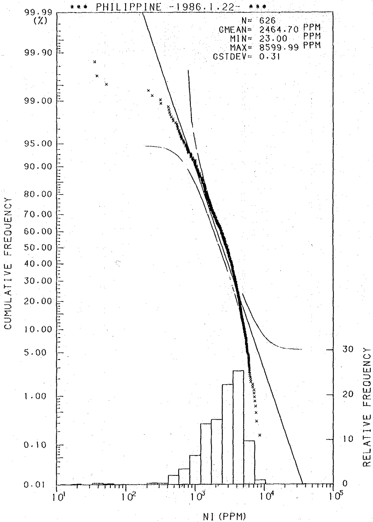
Histogram and Cumulative Frequency Curve of Ni Content in Lithological Code; 0.6.
