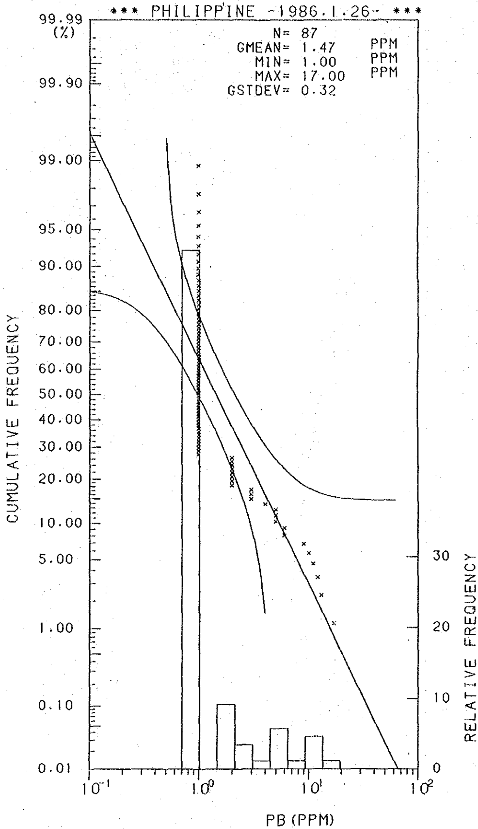
Histogram and Cumulative Frequency Curve of Pb content in Lithological Code; 0.5.
