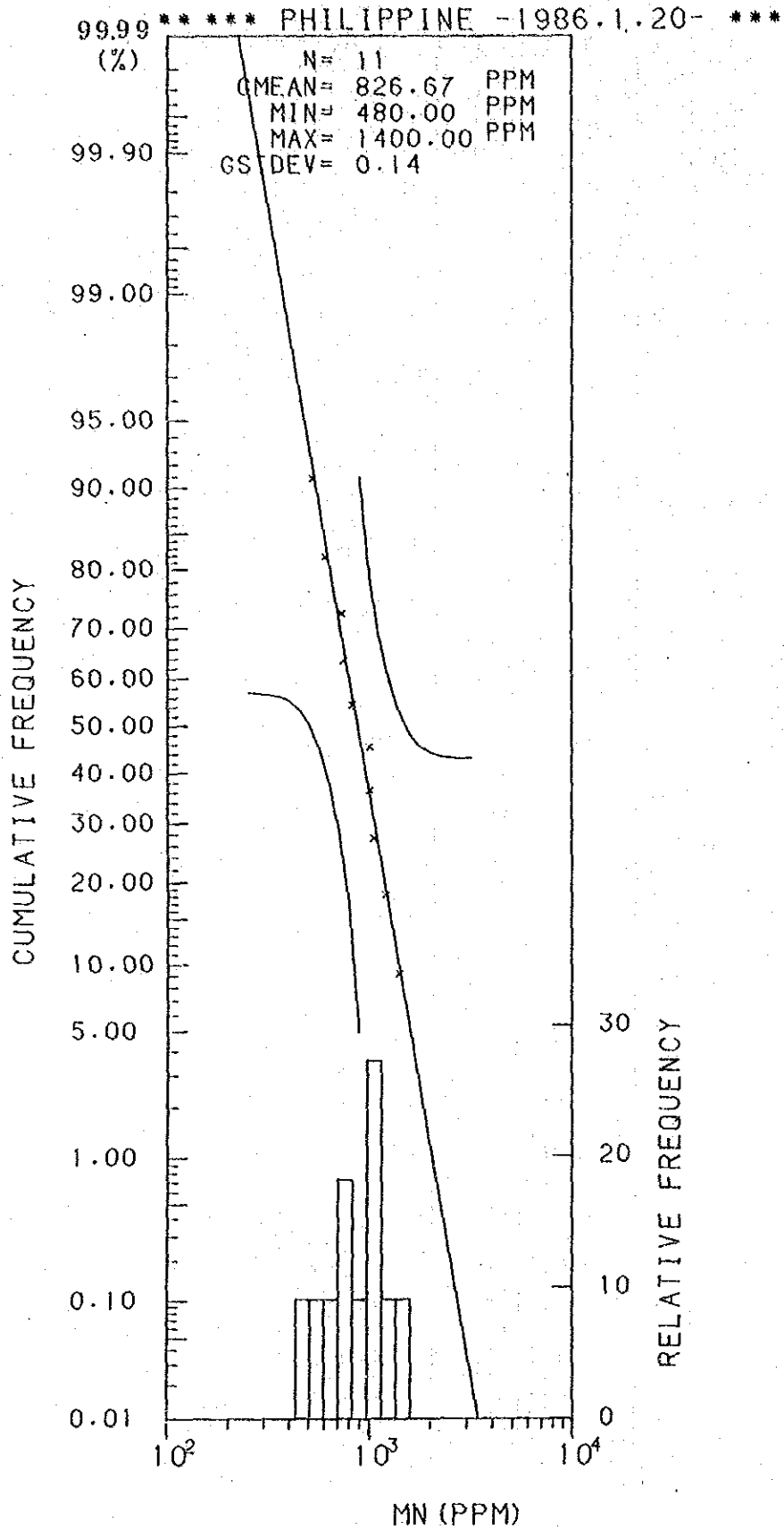
Histogram and Cumulative Frequency Curve of Mn Content in Lithological Code; 0.2.
