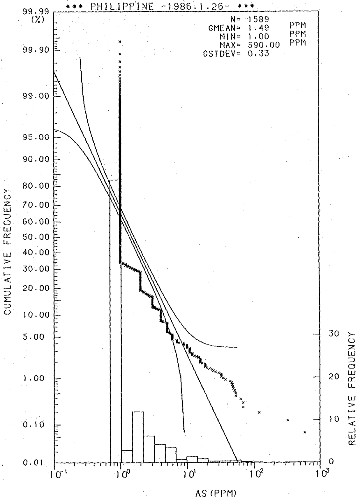
Histogram and Cumulative Frequency Curve of As content in Lithological Code; 0.4.
