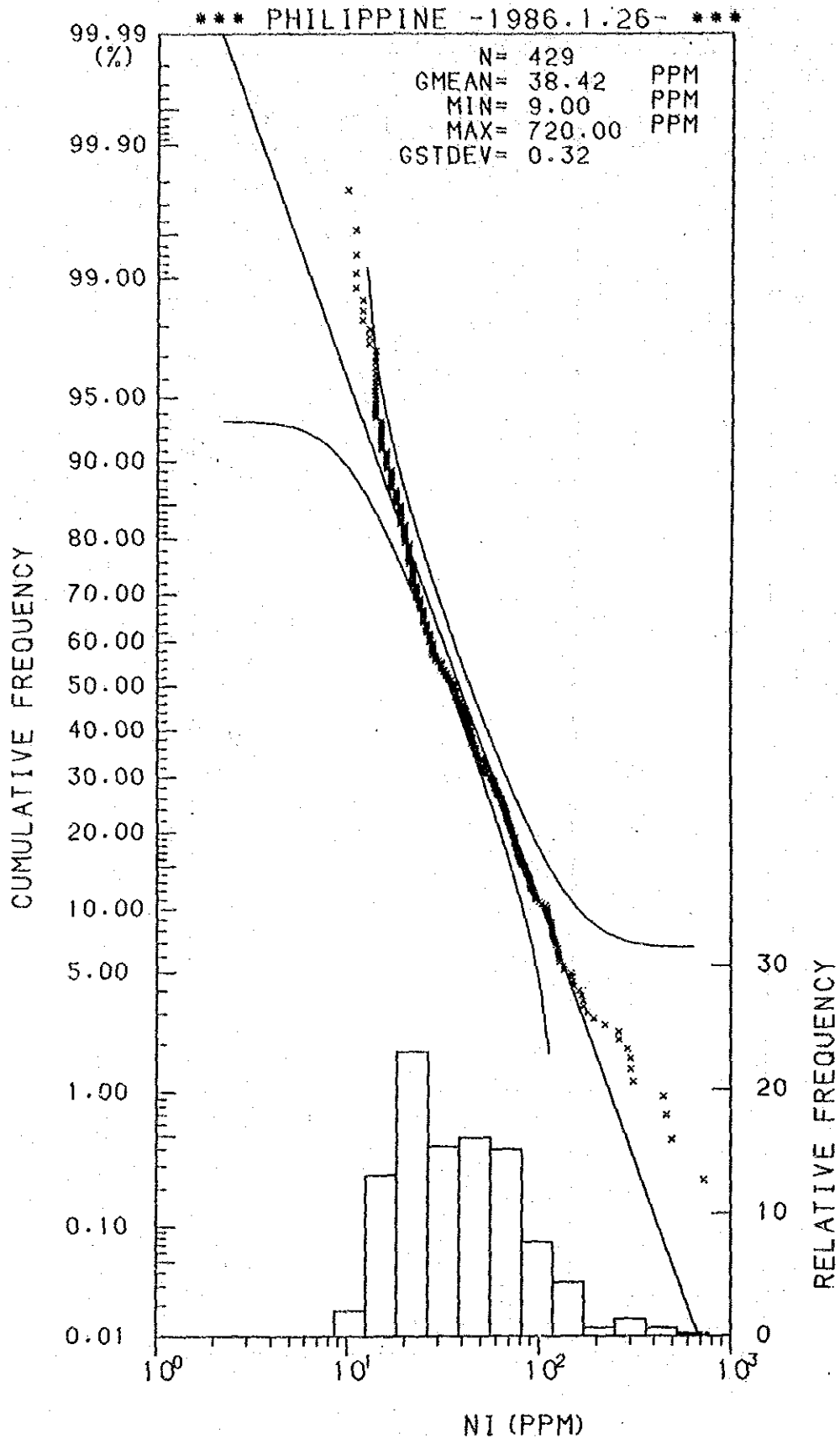
Histogram and Cumulative Frequency Curve of Ni content in Lithological Code; 0.8.
