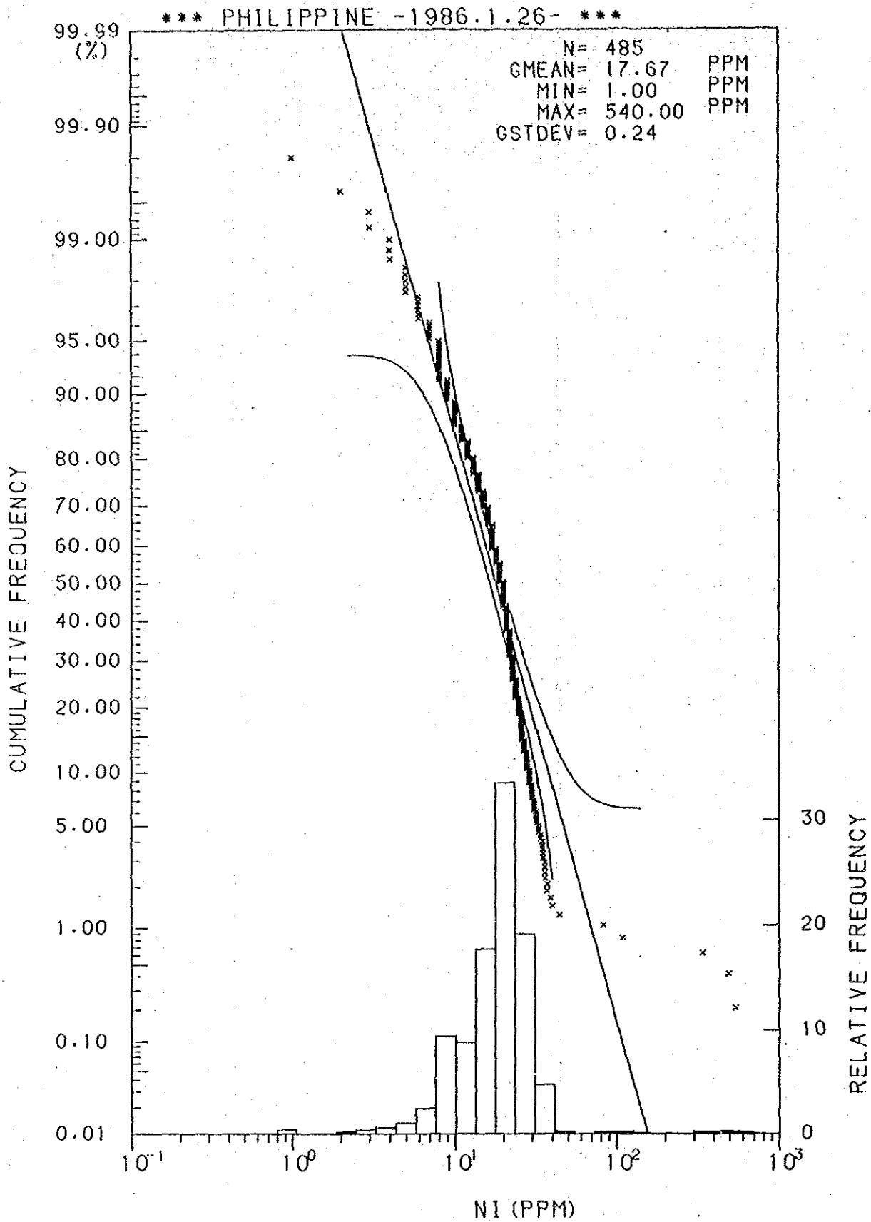
Histogram and Cumulative Frequency Curve of Ni content in Lithological Code; 0.1.
