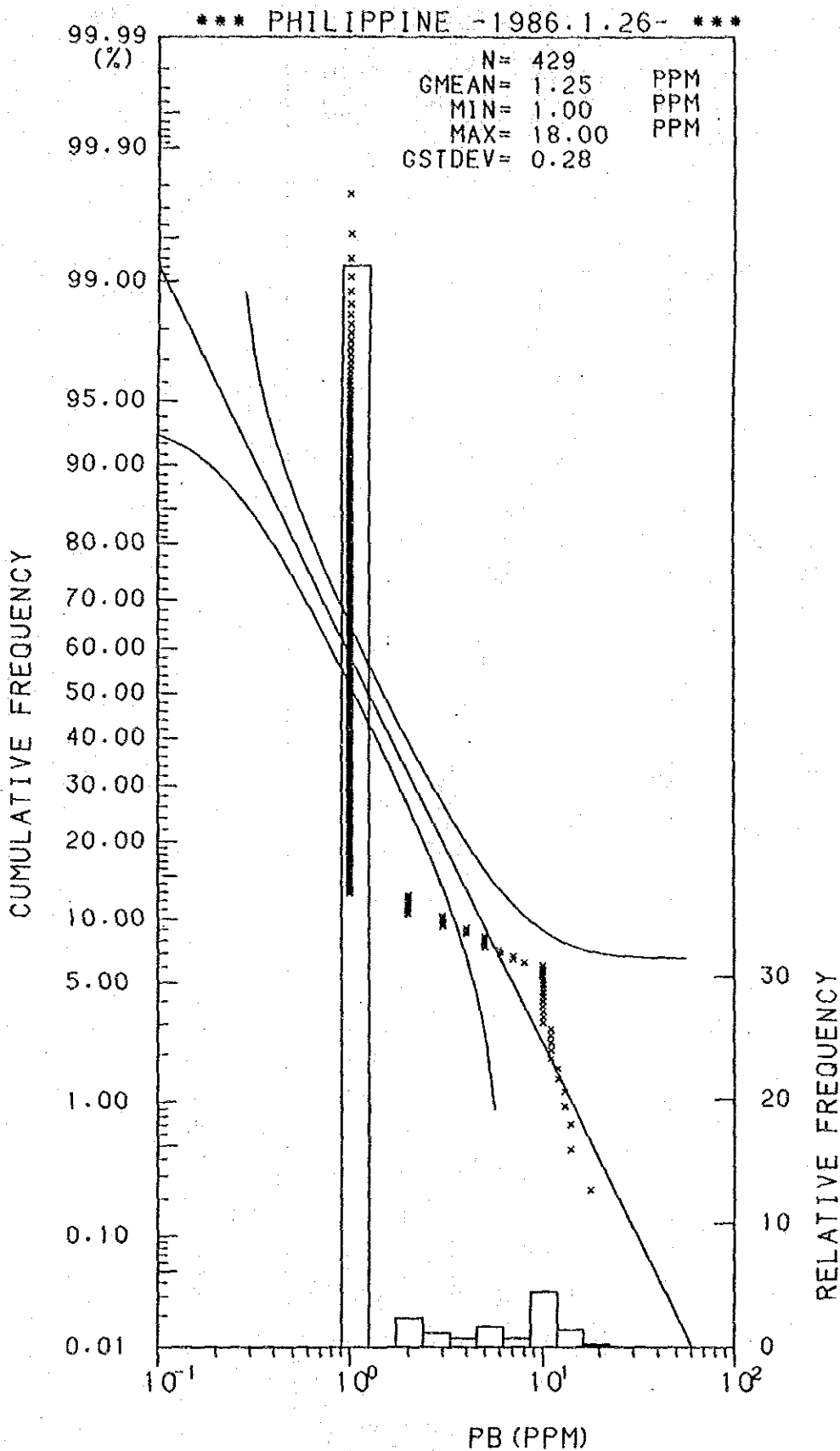
Histogram and Cumulative Frequency Curve of Pb content in Lithological Code; 0.8.
