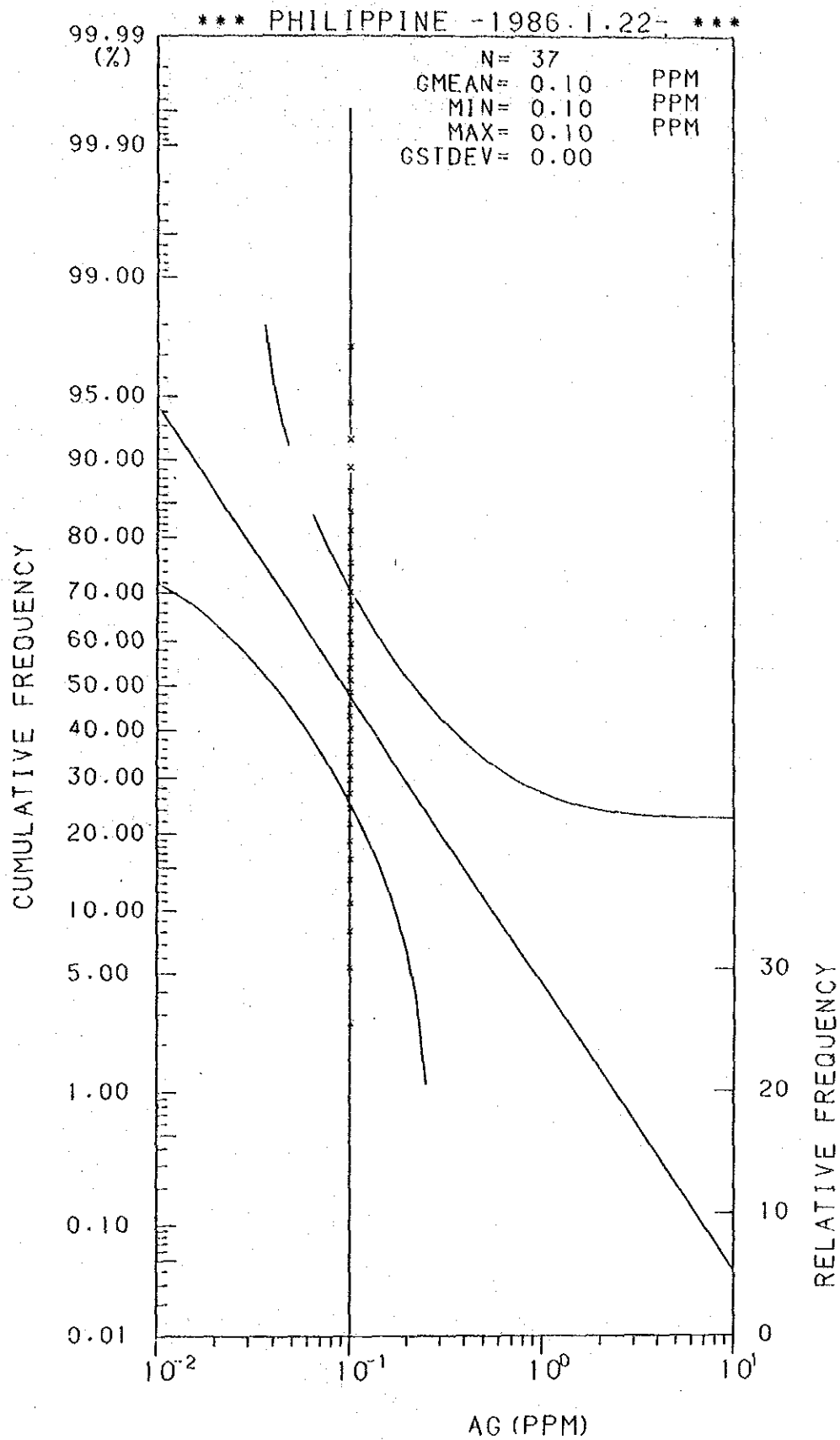
Histogram and Cumulative Frequency Curve of Ag Content in Lithological Code; 0.7.
