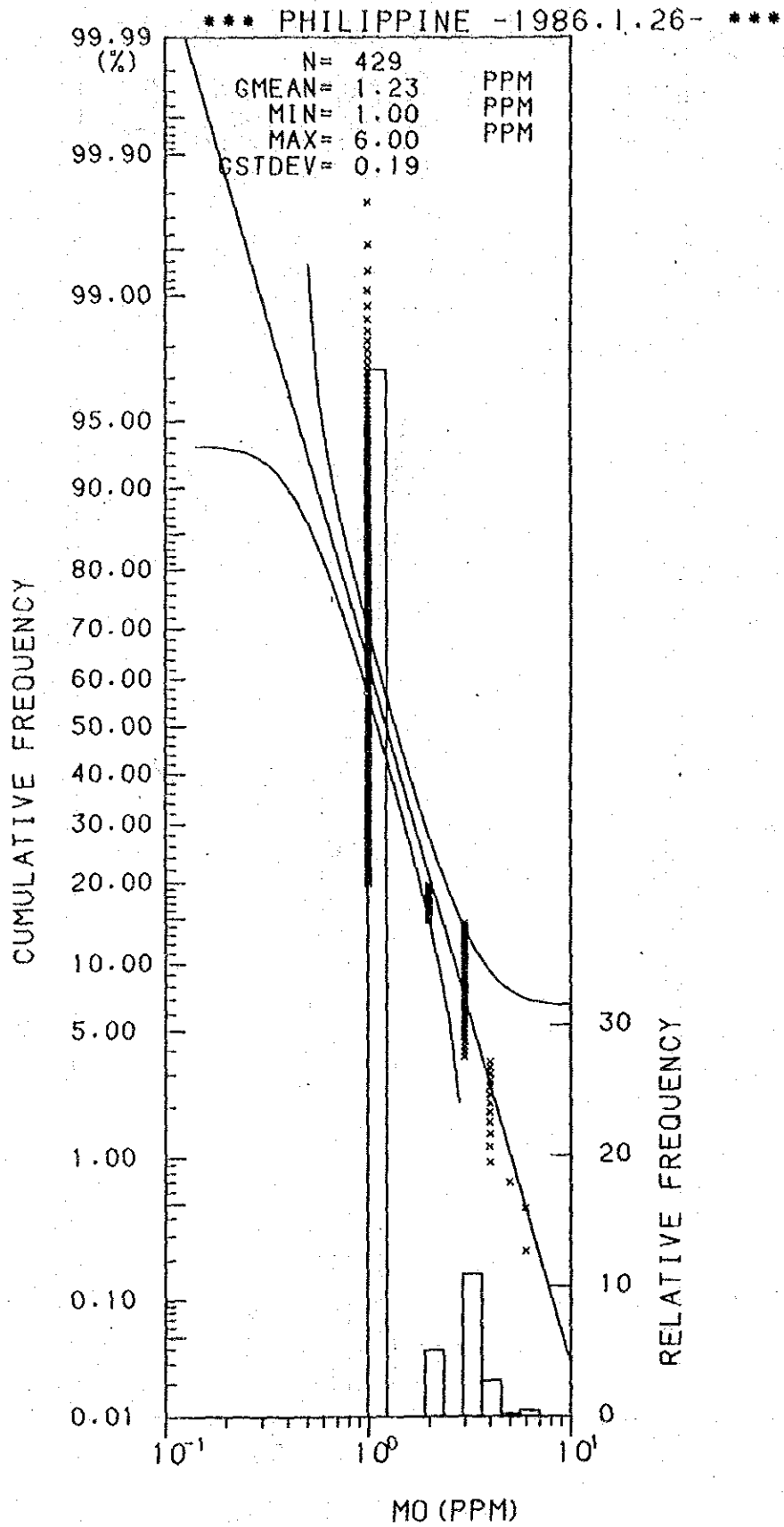
Histogram and Cumulative Frequency Curve of Mo content in Lithological Code; 0.8.
