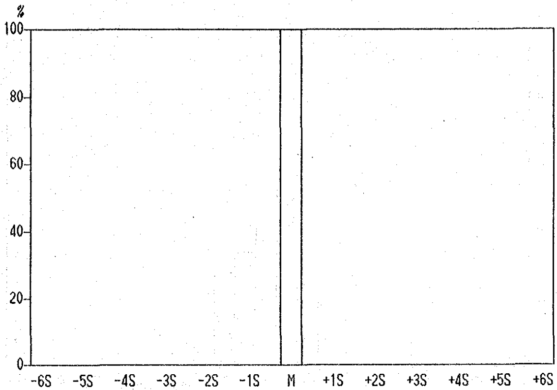
Histogram of Ag contents in Lithological Code; KPS
