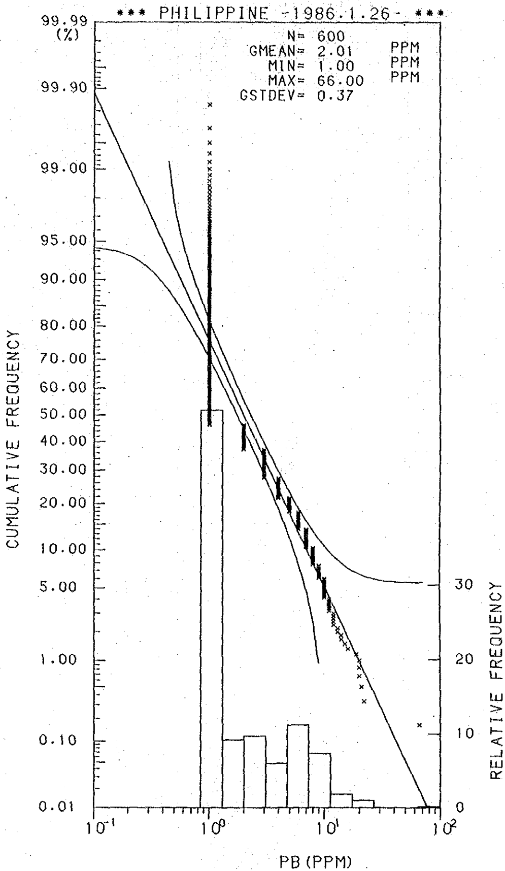
Histogram and Cumulative Frequency Curve of Pb content in Lithological Code; 0.2.
