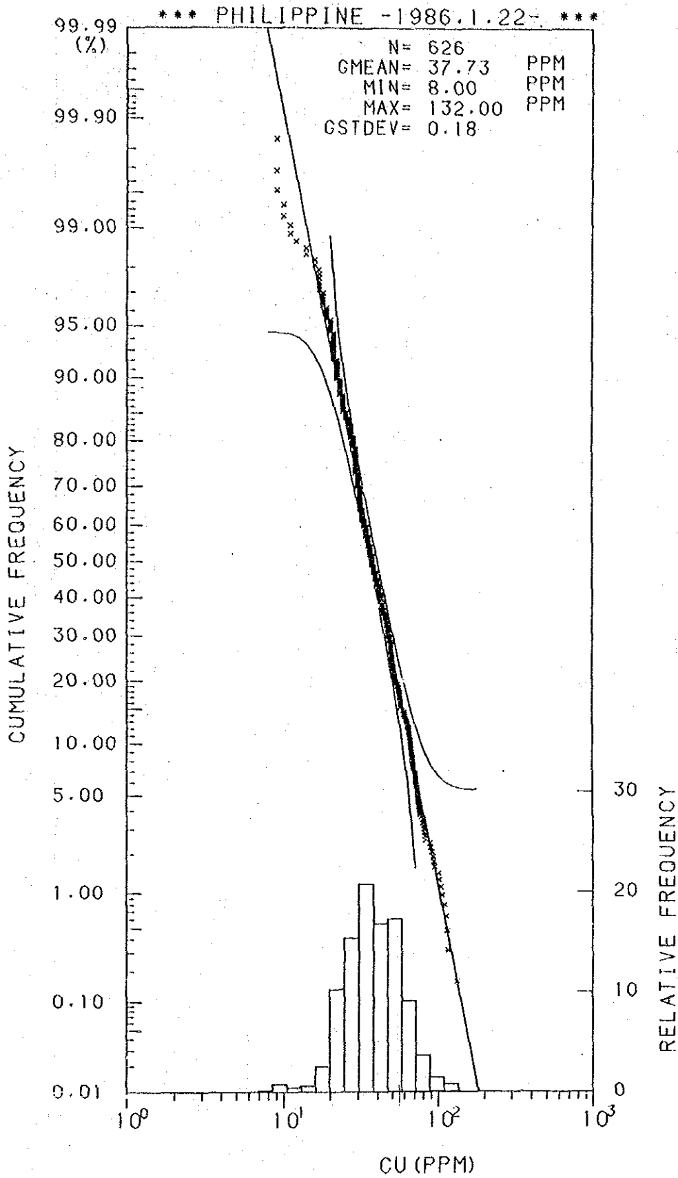
Histogram and Cumulative Frequency Curve of Cu Content in Lithological Code; 0.6.
