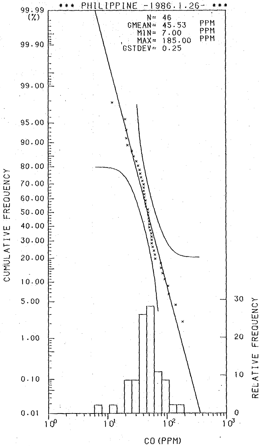
Histogram and Cumulative Frequency Curve of Co content in Lithological Code; 0.6.
