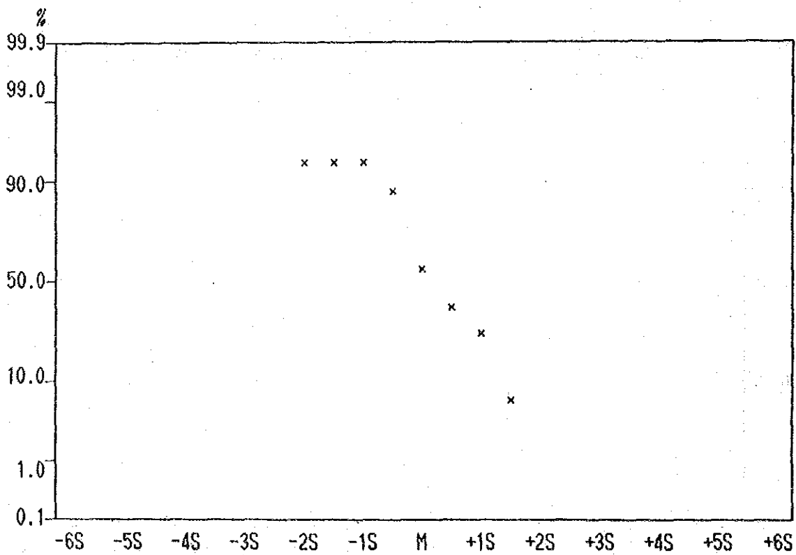
Cumulative Frequency Curve of Zn contents in Lithological Code; KPL
