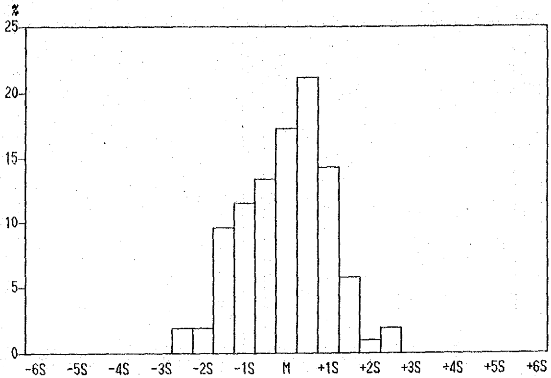
Histogram of Cu contents in Lithological Code; INR
