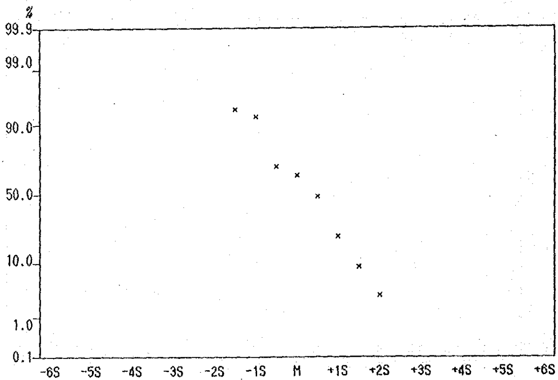
Cumulative Frequency Curve of Ni contents in Lithological Code; INR
