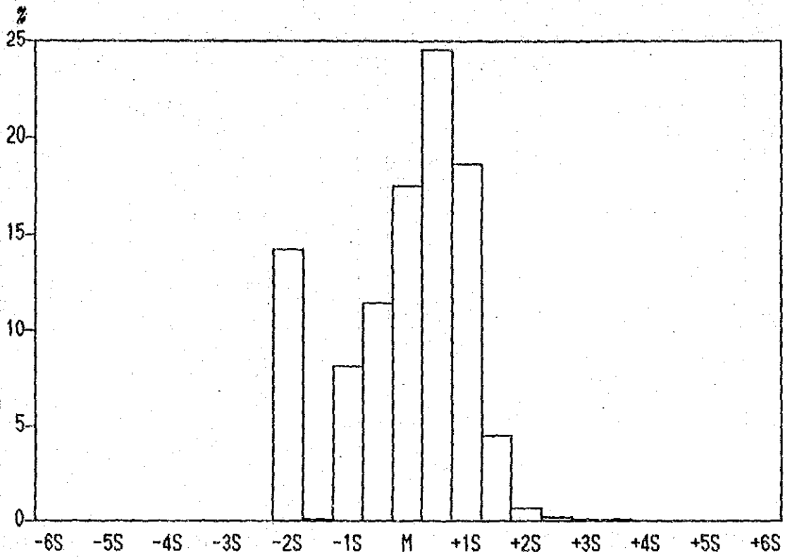
Histograms of As content in all Samples.
