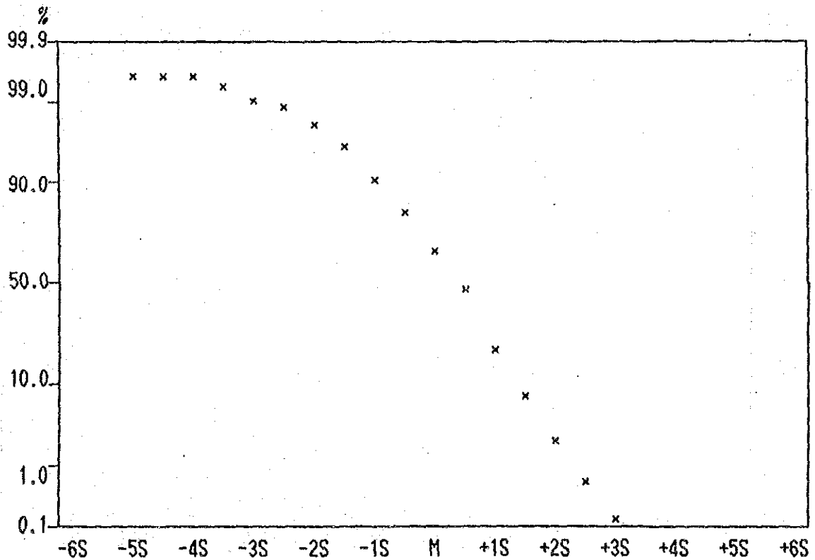
Cumulative Frequency Curve of Co content in all Samples.
