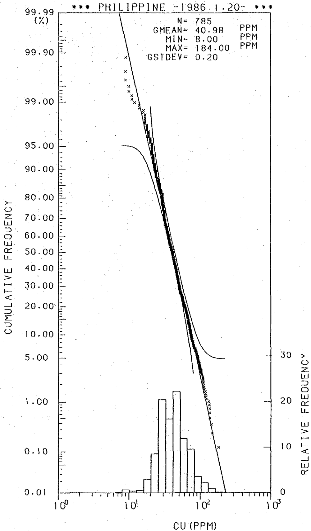
Histogram and Cumulative Frequency Curve of Cu Content in All Samples.
