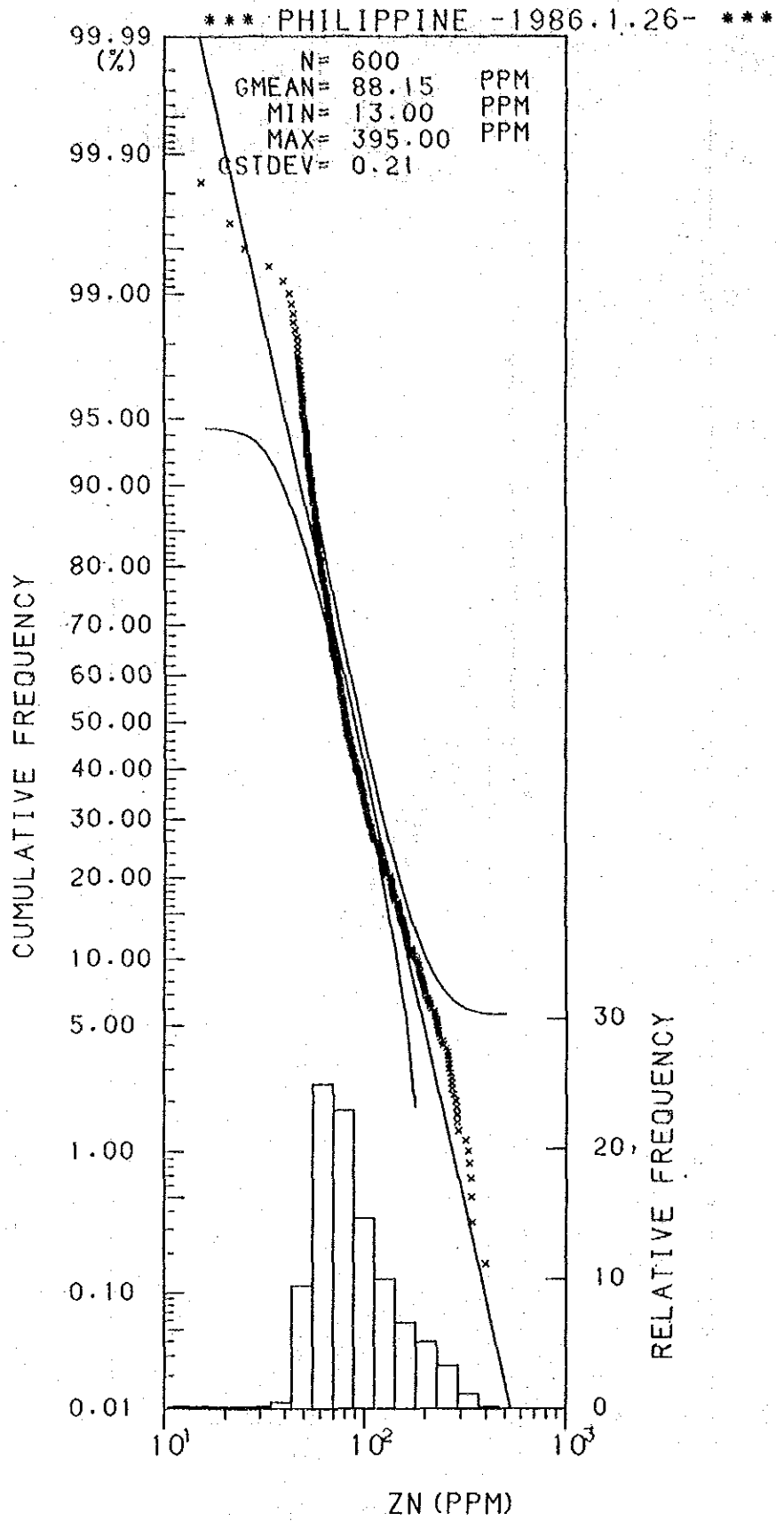
Histogram and Cumulative Frequency Curve of Zn content in Lithological Code; 0.2.
