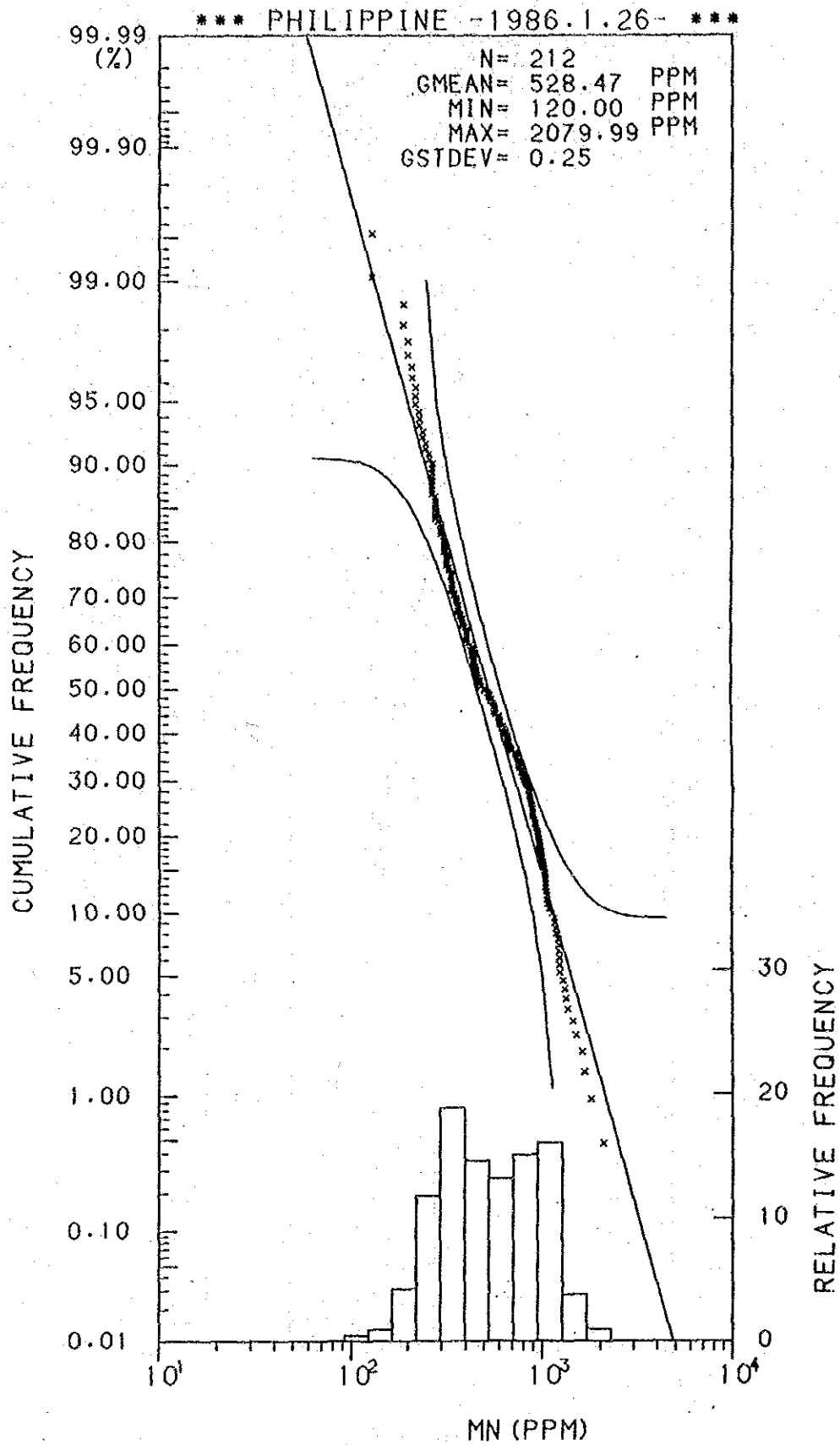
Histogram and Cumulative Frequency Curve of Mn content in Lithological Code; 0.7.
