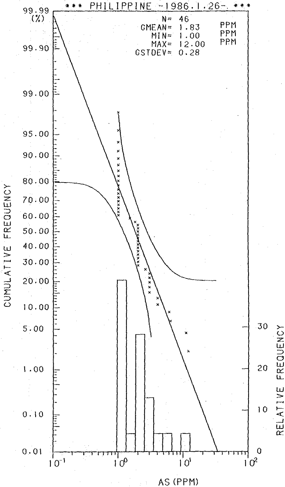
Histogram and Cumulative Frequency Curve of As content in Lithological Code; 0.6.
