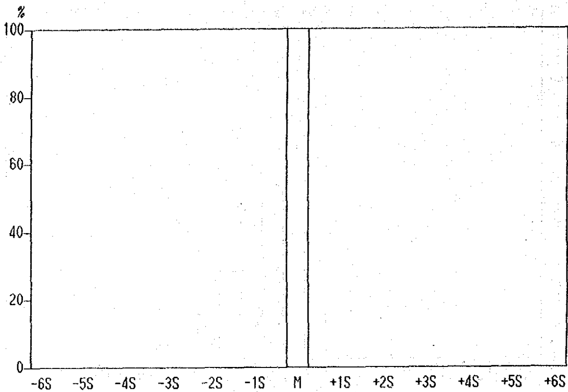
Histogram of Mo contents in Lithological Code; KPL
