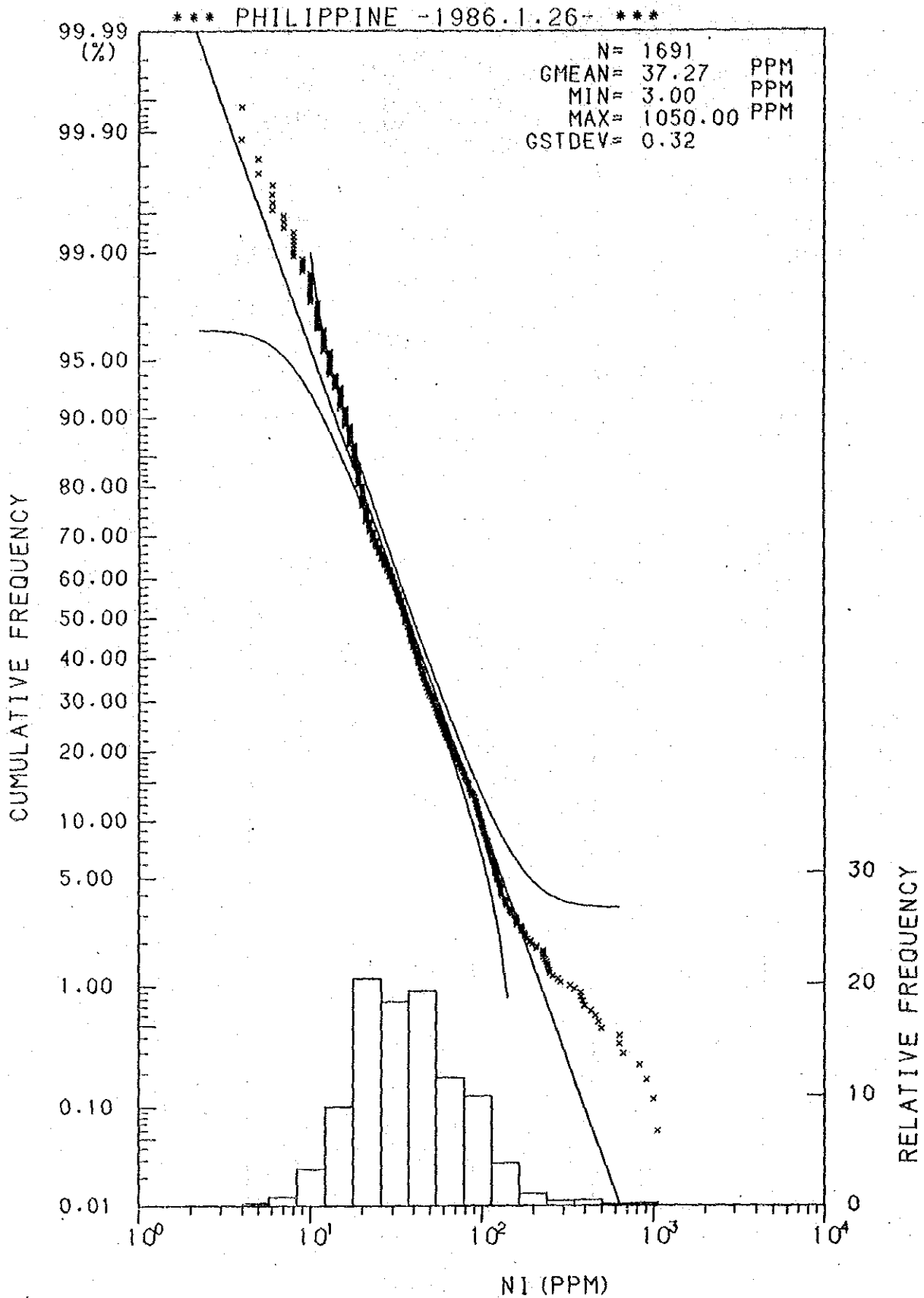
Histogram and Cumulative Frequency Curve of Ni content in Lithological Code; 0.3.
