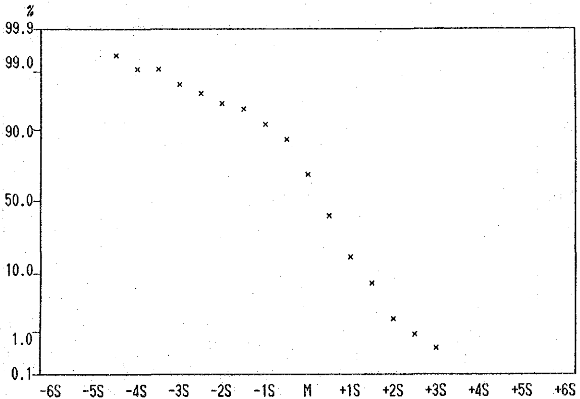
Cumulative Frequency Curve of Co contents in Lithological Code; KPS
