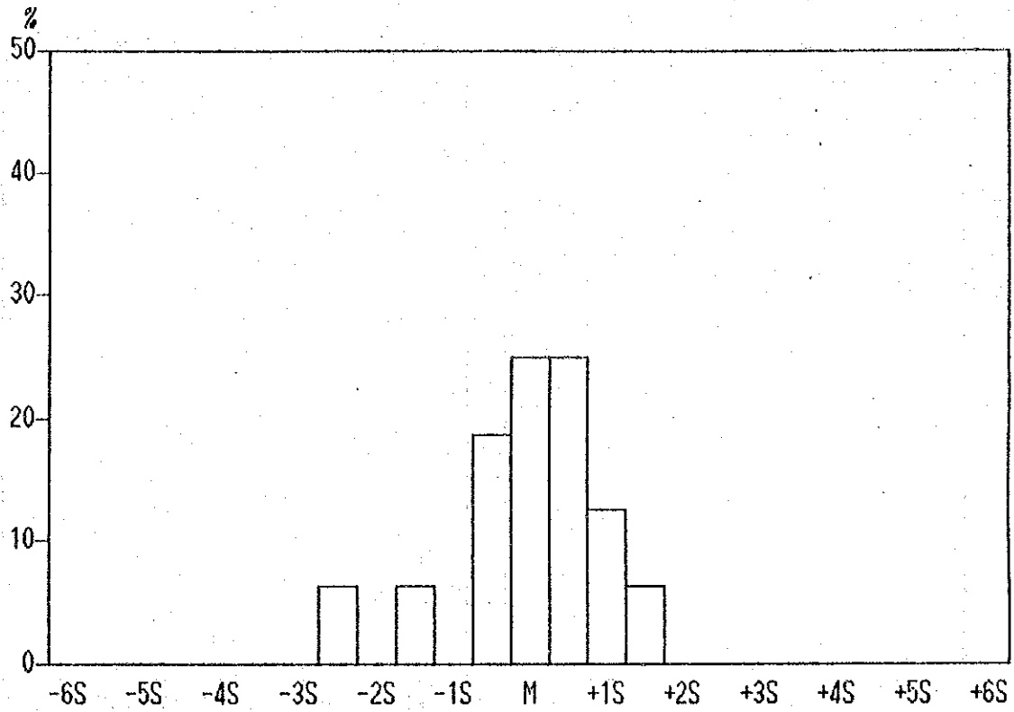
Histogram of Cu contents in Lithological Code; KPL
