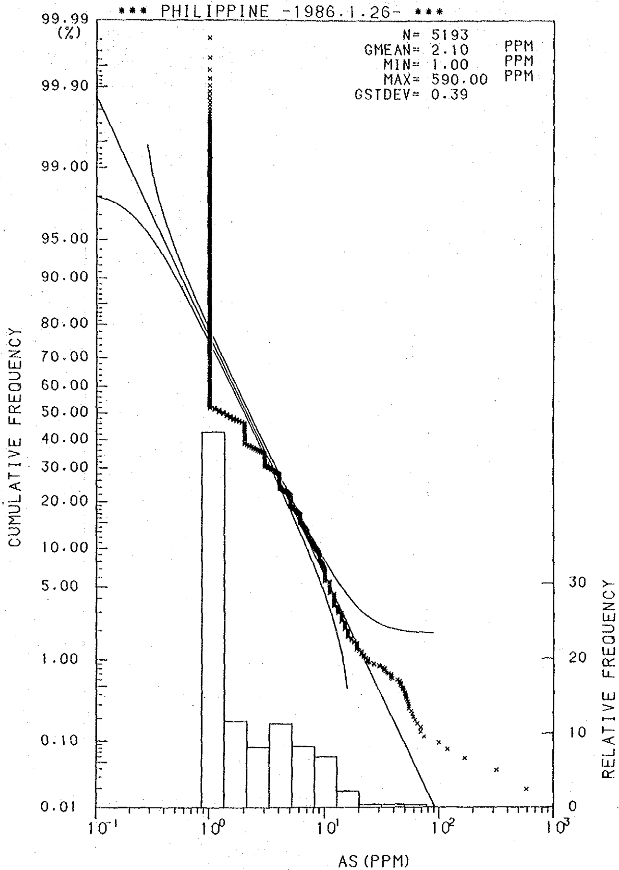
Histogram and Cumulative Frequency Curve of As content in All Samples.
