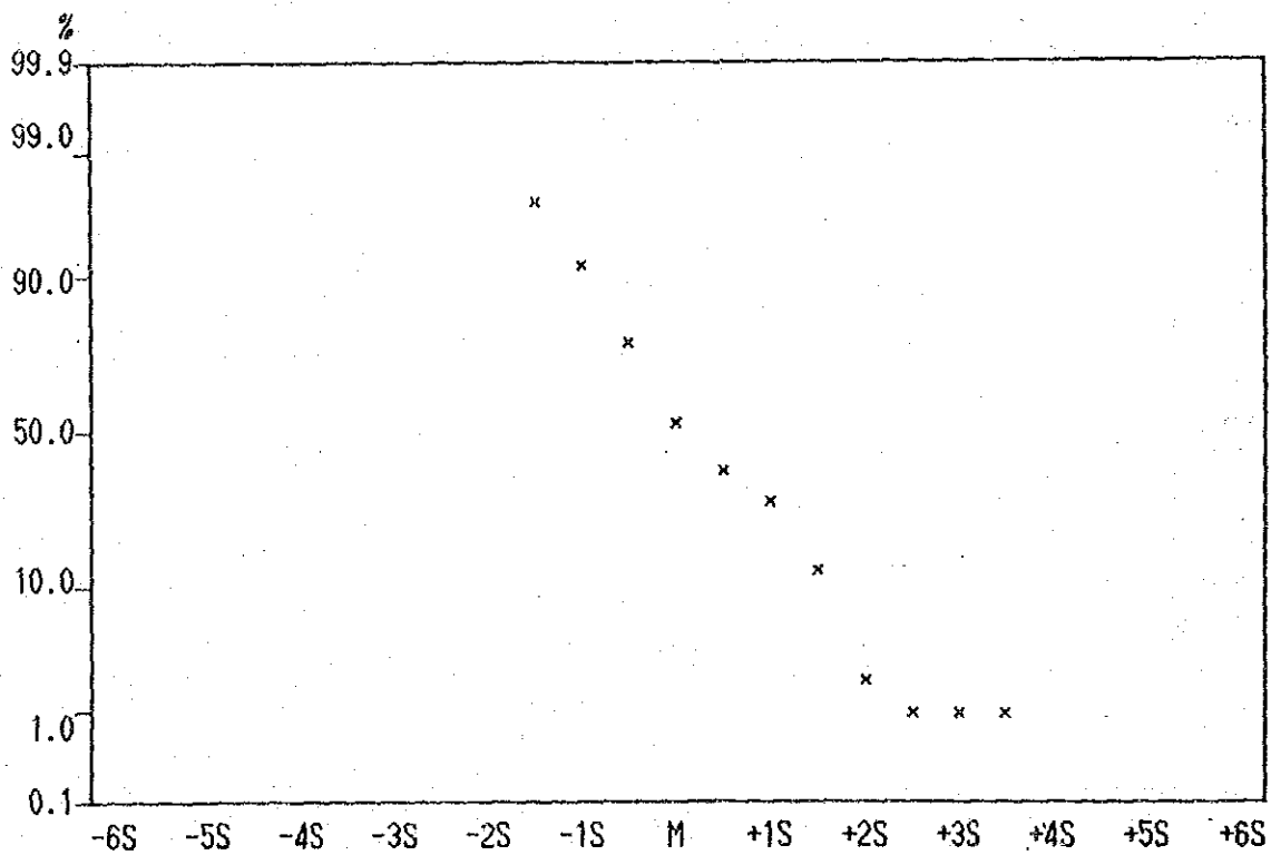
Cumulative Frequency Curve of Zn contents in Lithological Code; INR
