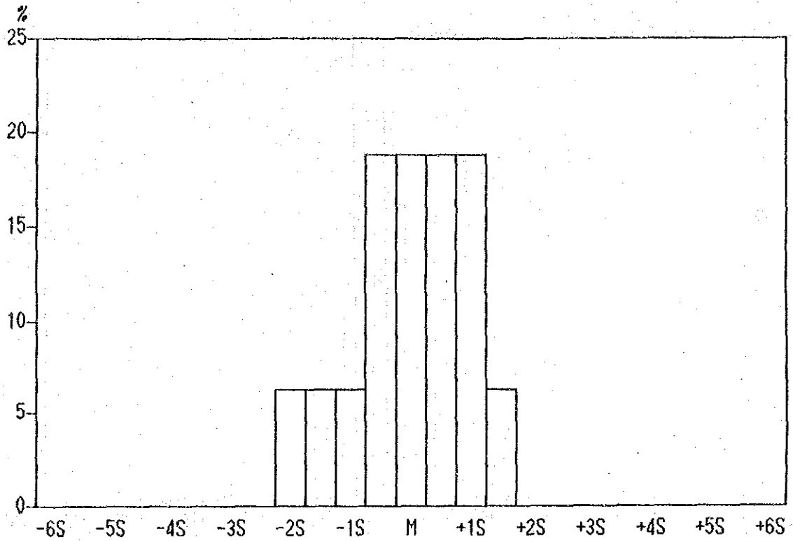
Histogram of As contents in Lithological Code; KPL
