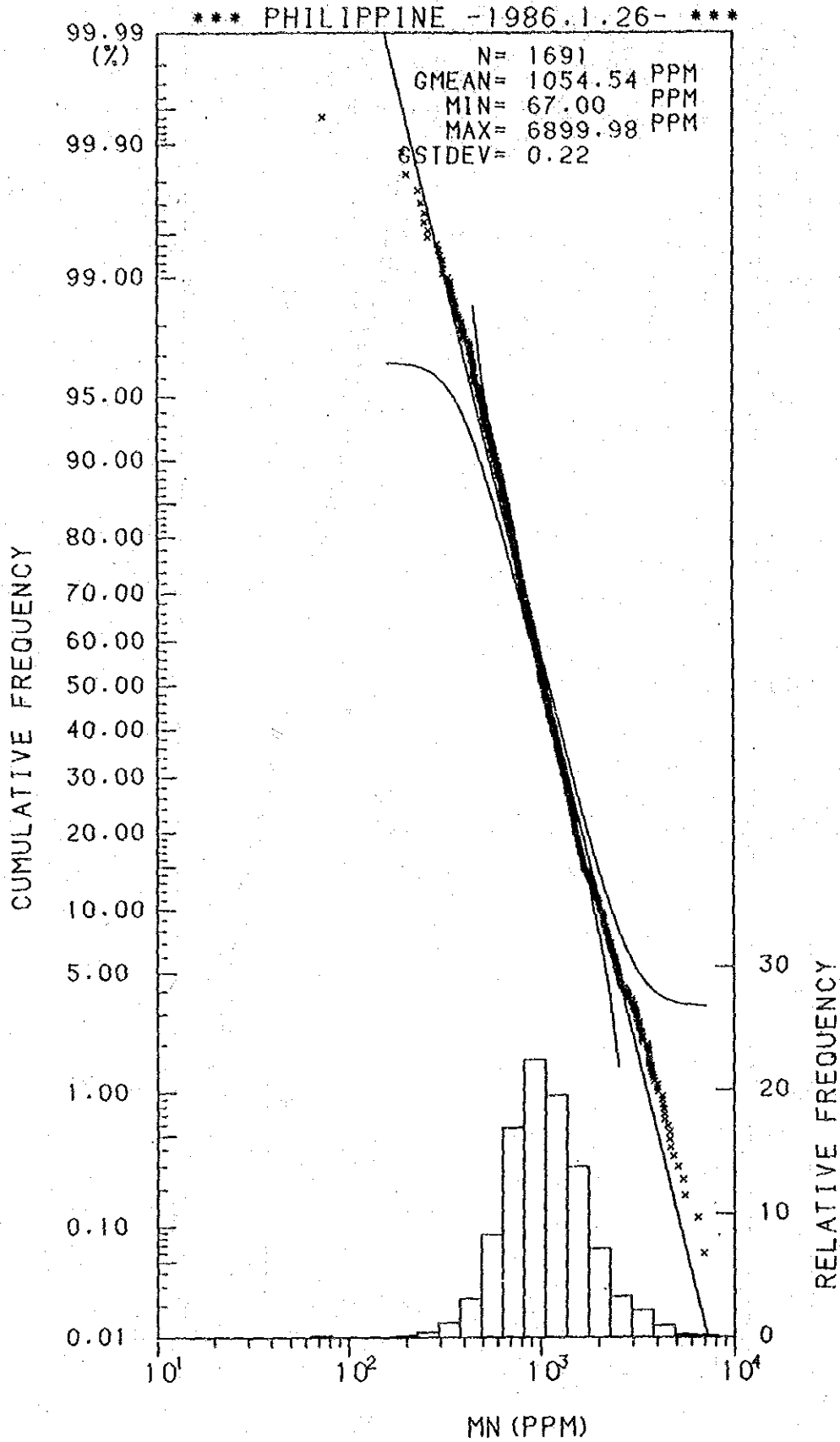
Histogram and Cumulative Frequency Curve of Mn content in Lithological Code; 0.3.
