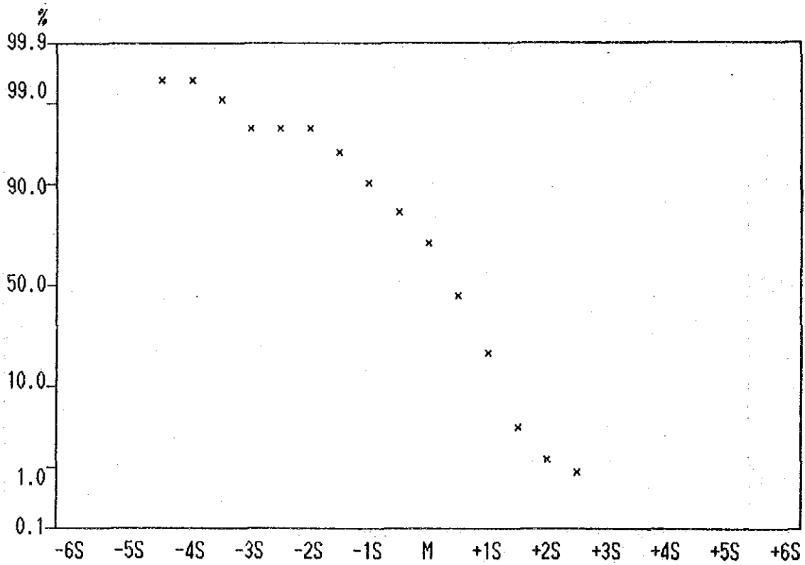
Cumulative Frequency Curve of Mn contents in Lithological Code; KPS
