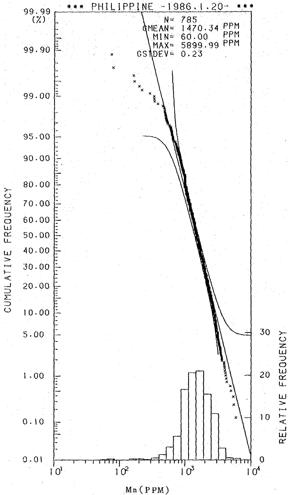
Histogram and Cumulative Frequency Curve of Mn Content in All Samples.
