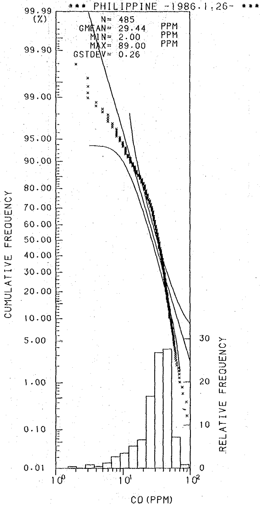
Histogram and Cumulative Frequency Curve of Co content in Lithological Code; 0.1.
