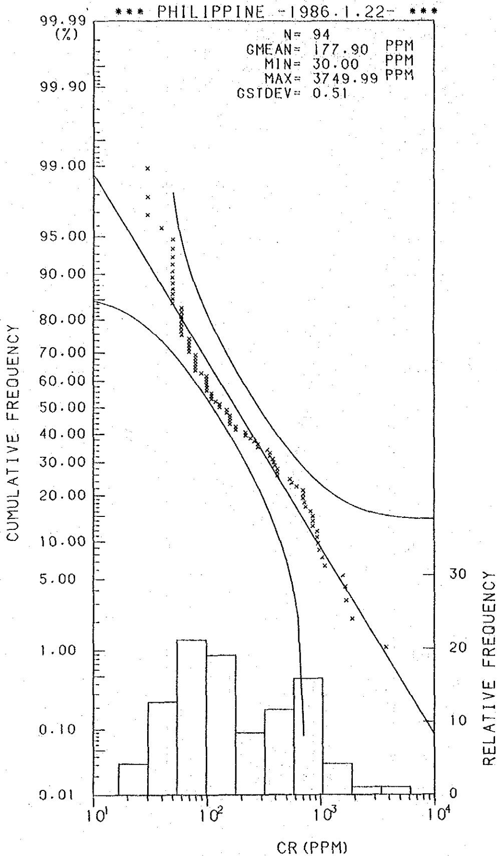
Histogram and Cumulative Frequency Curve of Cr Content in Lithological Code; 0.5.
