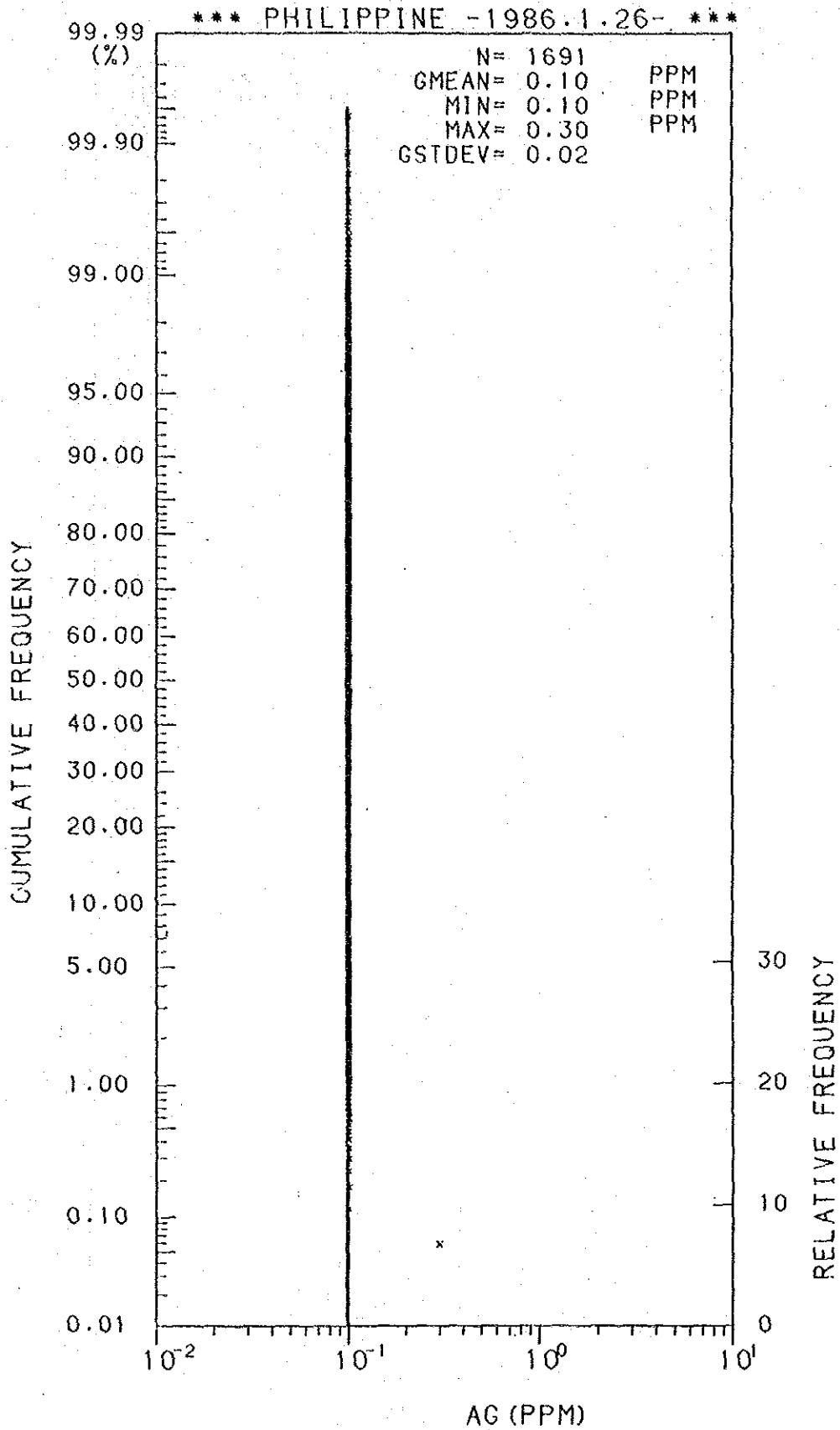
Histogram and Cumulative Frequency Curve of AG content in Lithological Code; 0.3.
