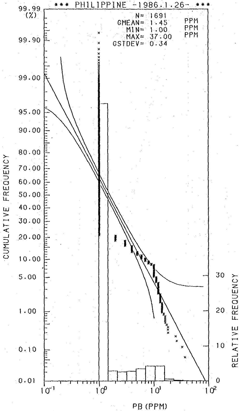
Histogram and Cumulative Frequency Curve of Pb content in Lithological Code; 0.3.
