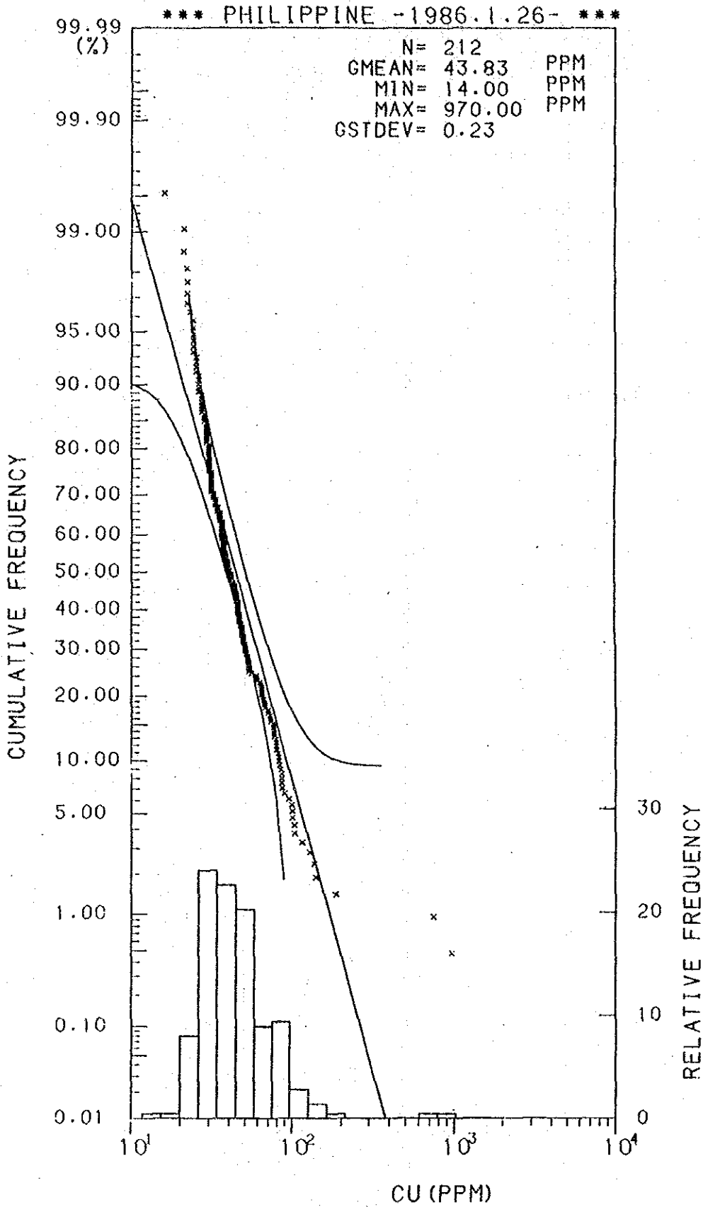
Histogram and Cumulative Frequency Curve of Cu content in Lithological Code; 0.7.
