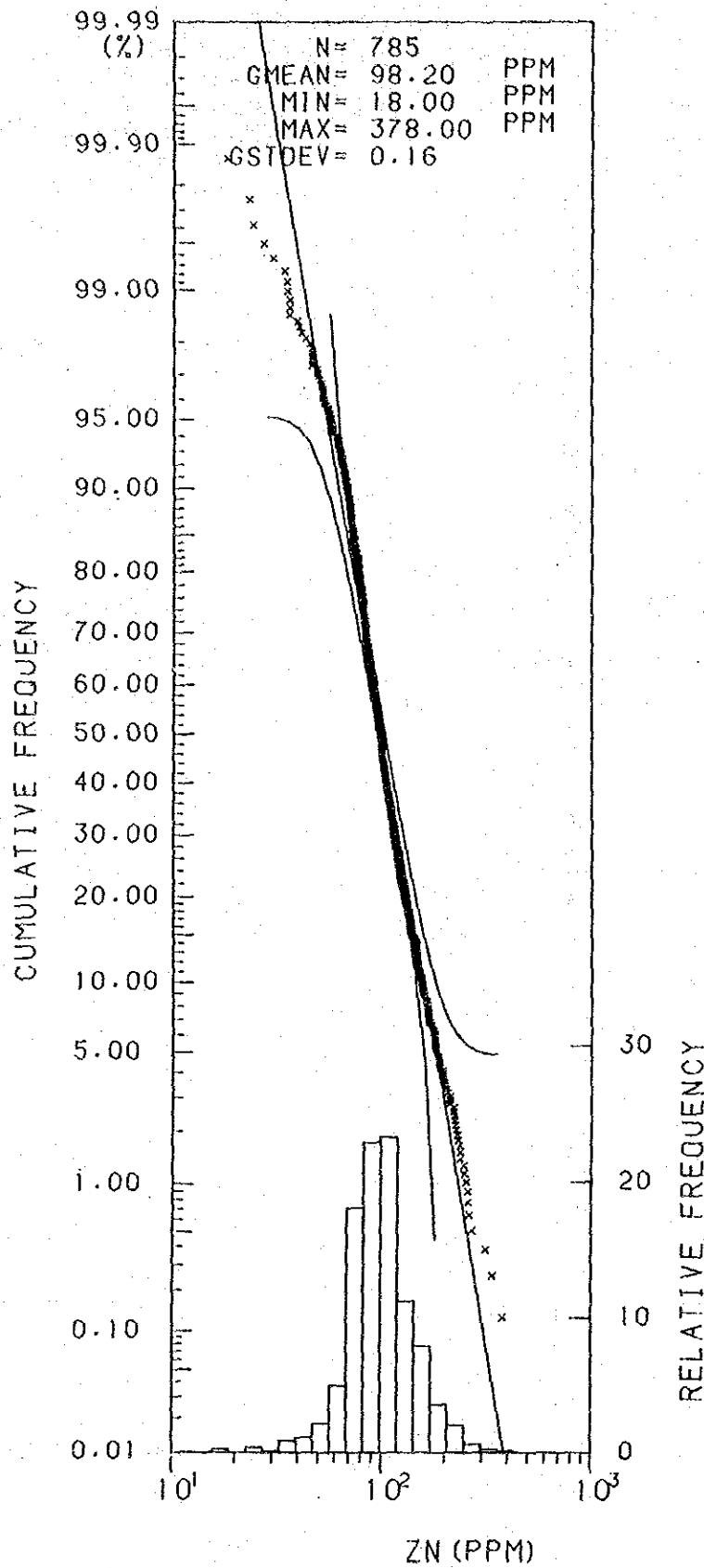
Histogram and Cumulative Frequency Curve of Zn Content in All Samples.
