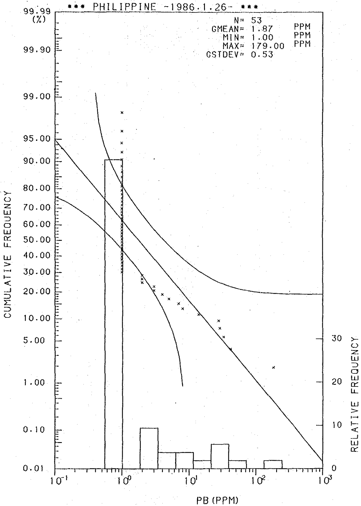
Histogram and Cumulative Frequency Curve of Pb content in Lithological Code; 0.9.
