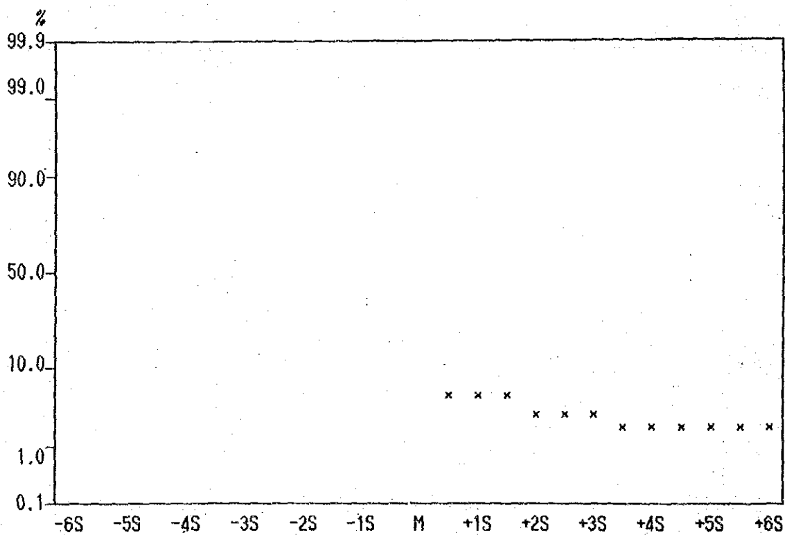
Cumulative Frequency Curve of Mo contents in Lithological Code; INR
