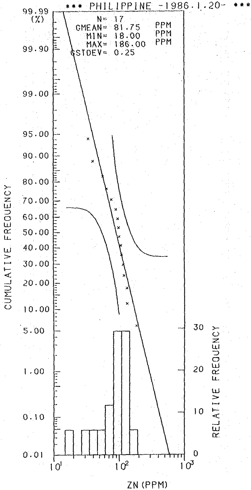
Histogram and Cumulative Frequency Curve of Zn Content in Lithological Code; 0.4.
