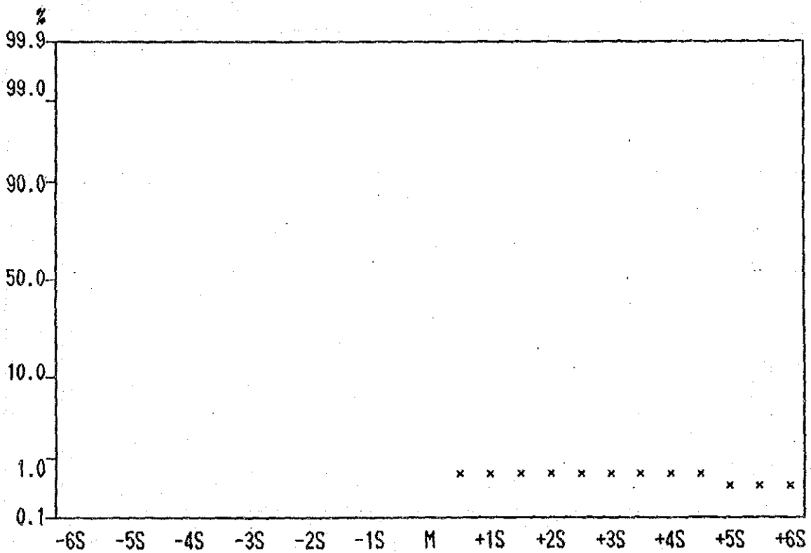
Cumulative Frequency Curve of Ag content in all Samples.
