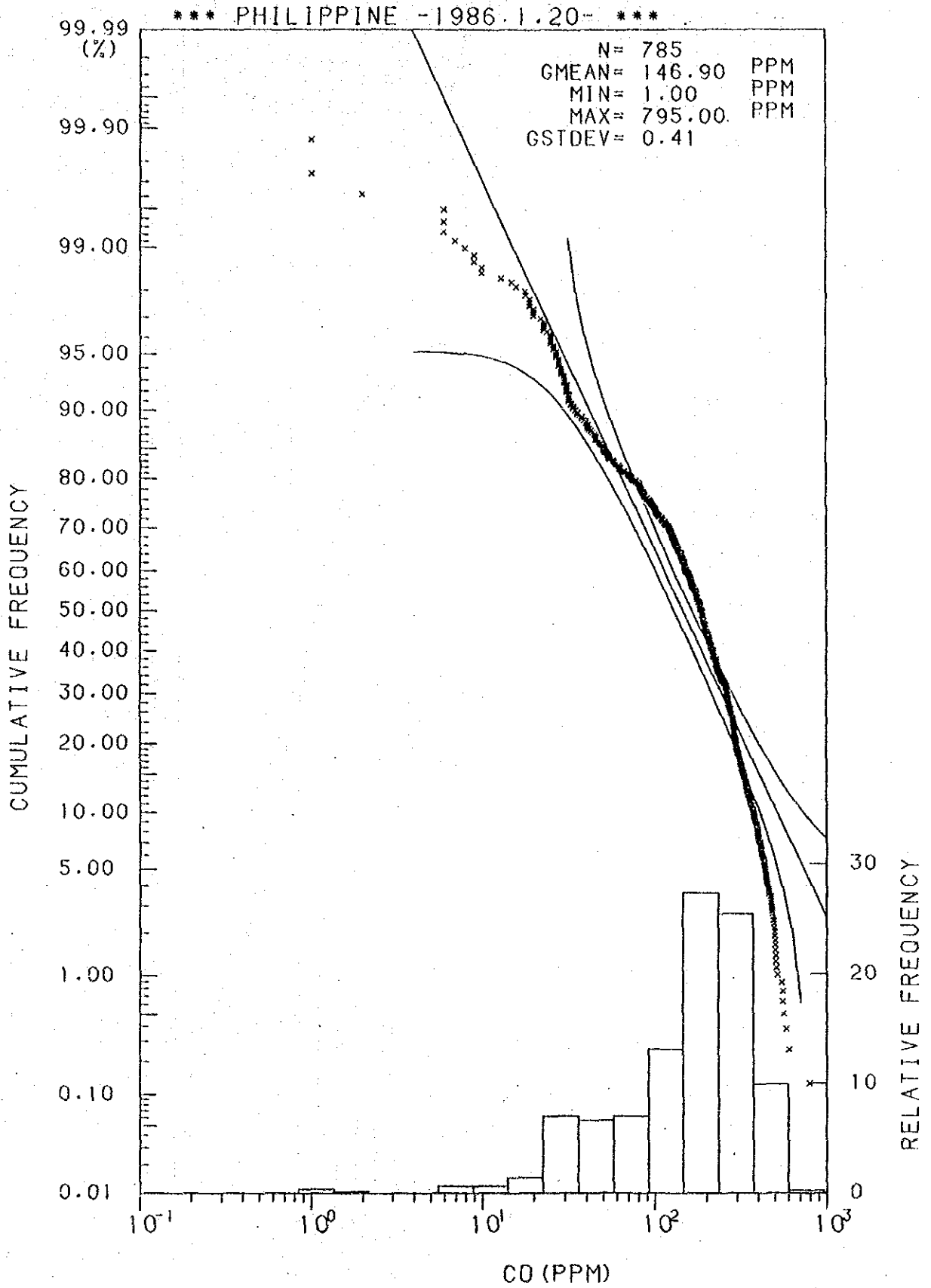
Histogram and Cumulative Frequency Curve of Co Content in All Samples.
