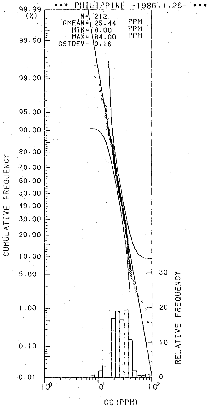
Histogram and Cumulative Frequency Curve of Co content in Lithological Code; 0.7.
