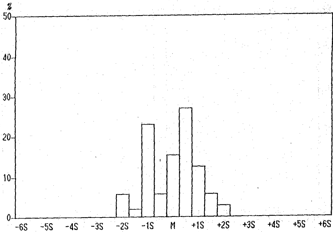
Histogram of Ni contents in Lithological Code; INR
