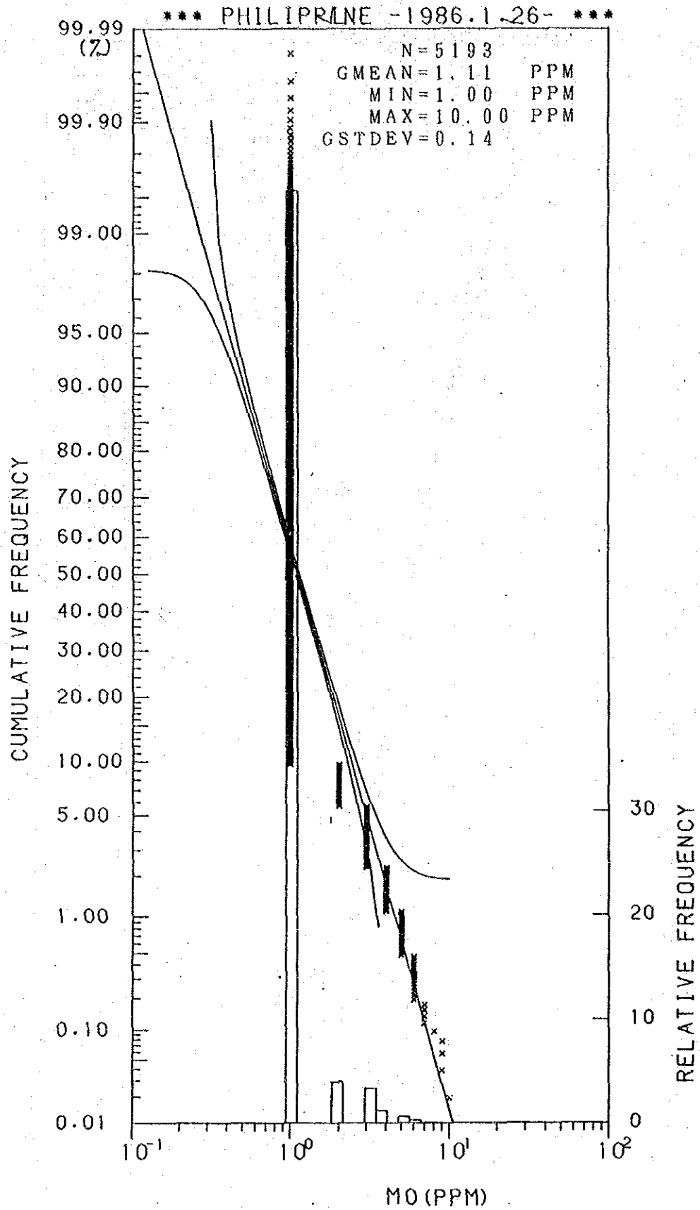
Histogram and Cumulative Frequency Curve of Mo content in All Samples.
