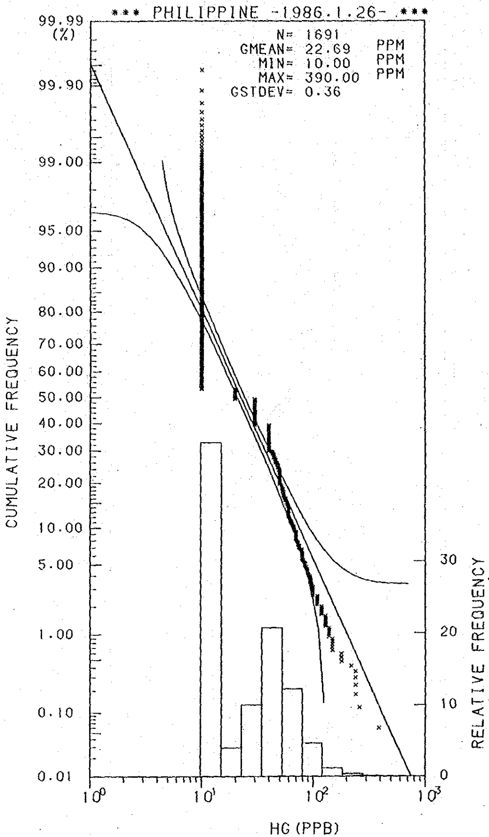
Histogram and Cumulative Frequency Curve of Hg content in Lithological Code; 0.3.
