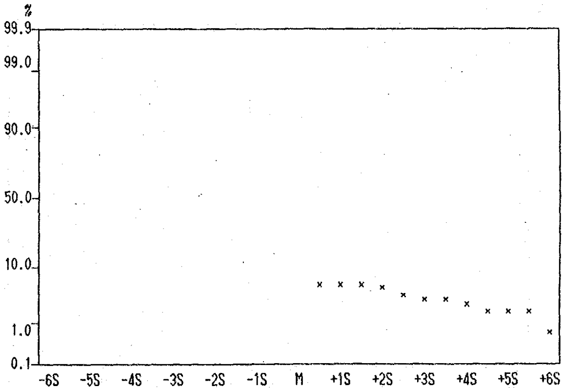
Cumulative Frequency Curve of Pb contents in Lithological Code; N2L
