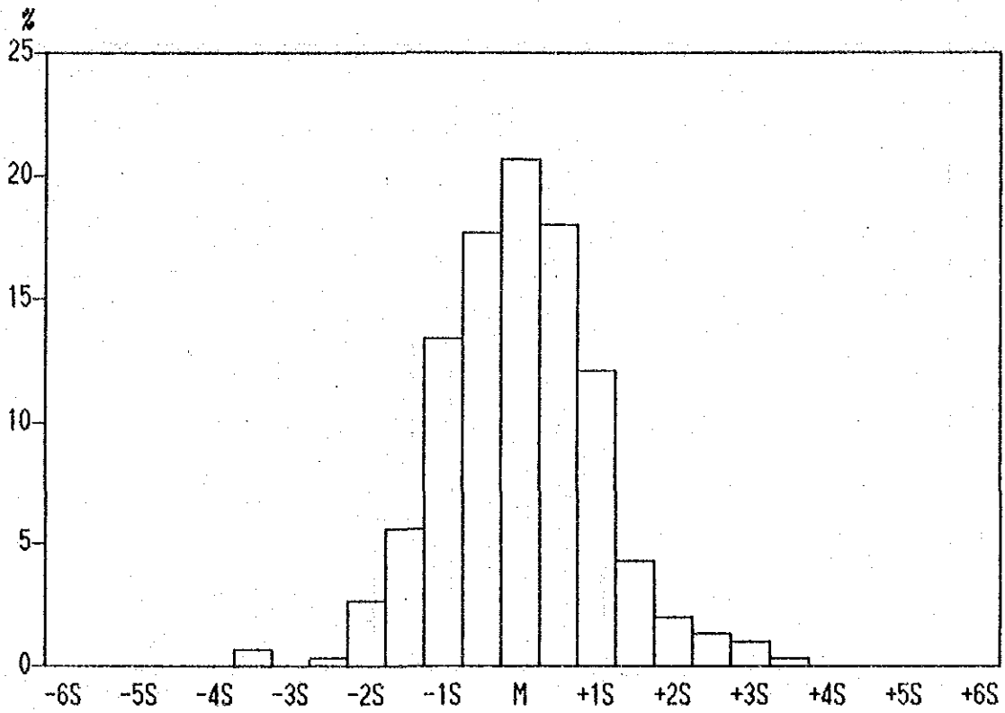
Histogram of Co contents in Lithological Code; KPB
