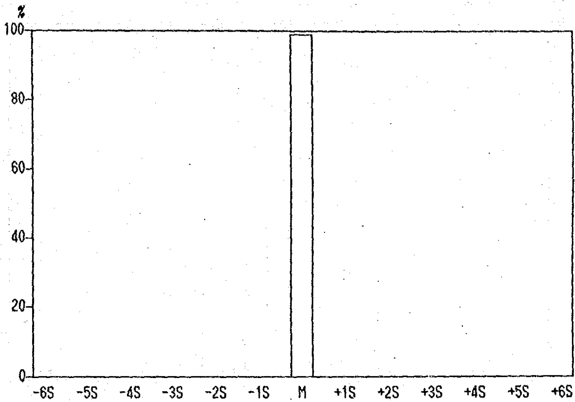
Histogram of Ag contents in Lithological Code; N1S
