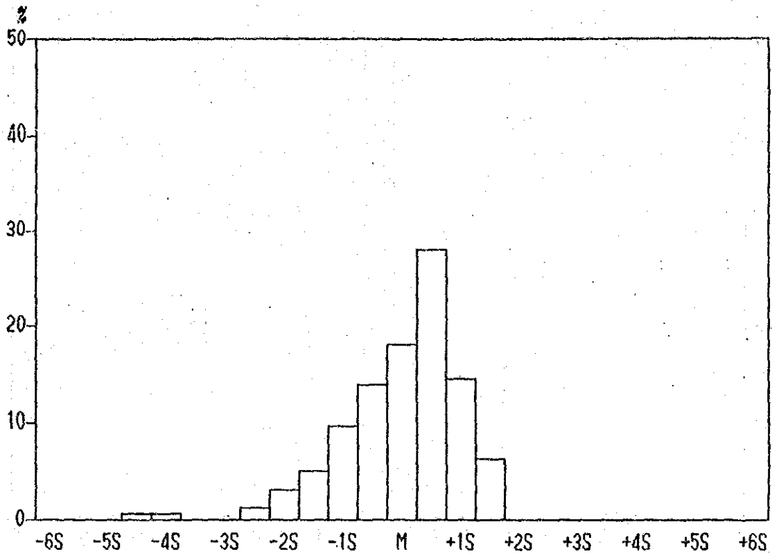
Histogram of As contents in Lithological Code; N2L
