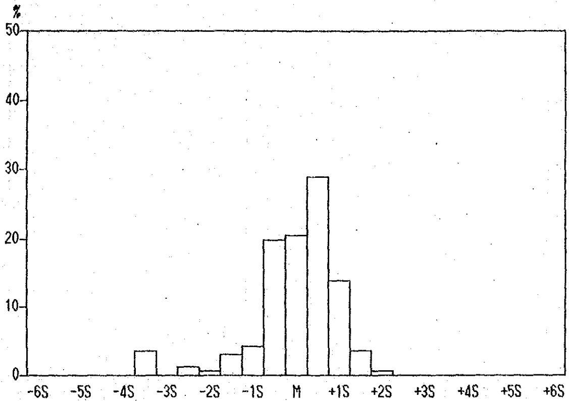
Histogram of Co contents in Lithological Code; N2L
