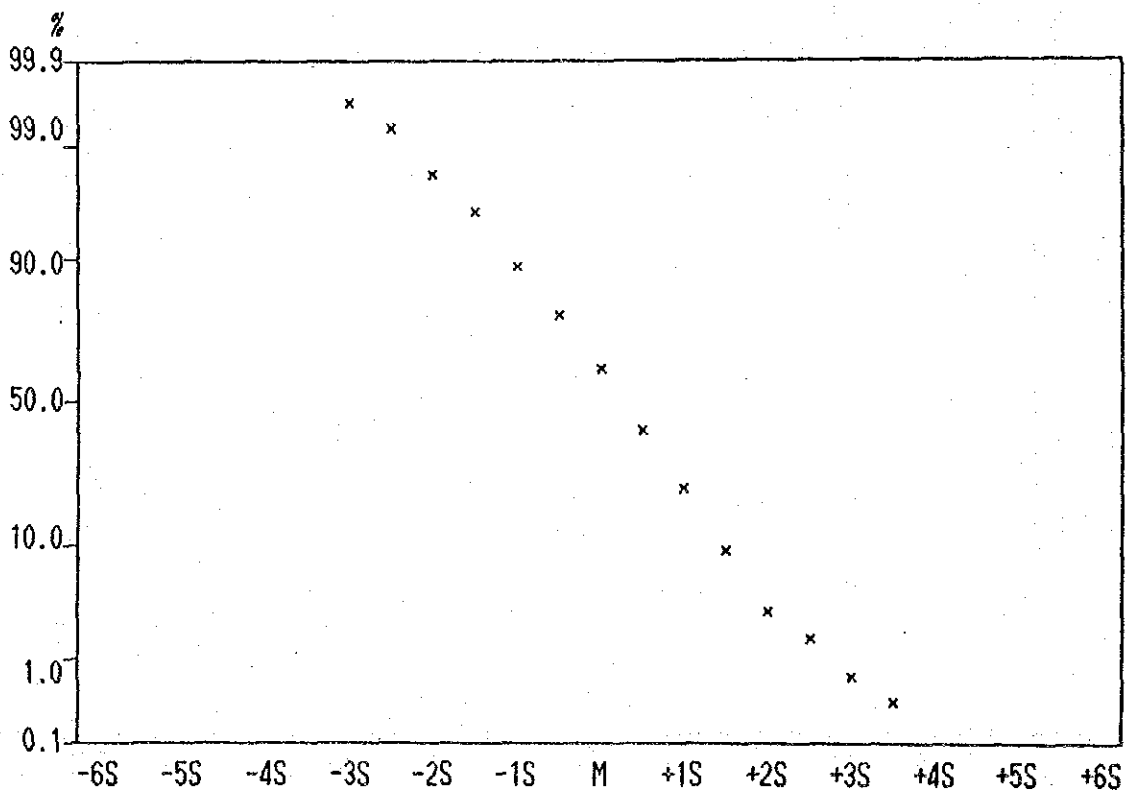
Cumulative Frequency Curve of Ni contents in Lithological Code; KPB
