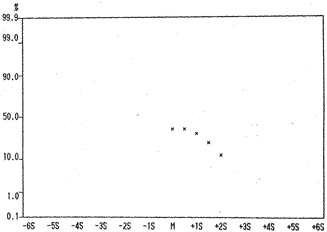
Cumulative Frequency Curve of Mo contents in Lithological Code; N2L
