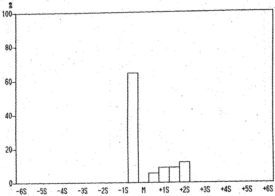
Histogram of Mo contents in Lithological Code; N2L
