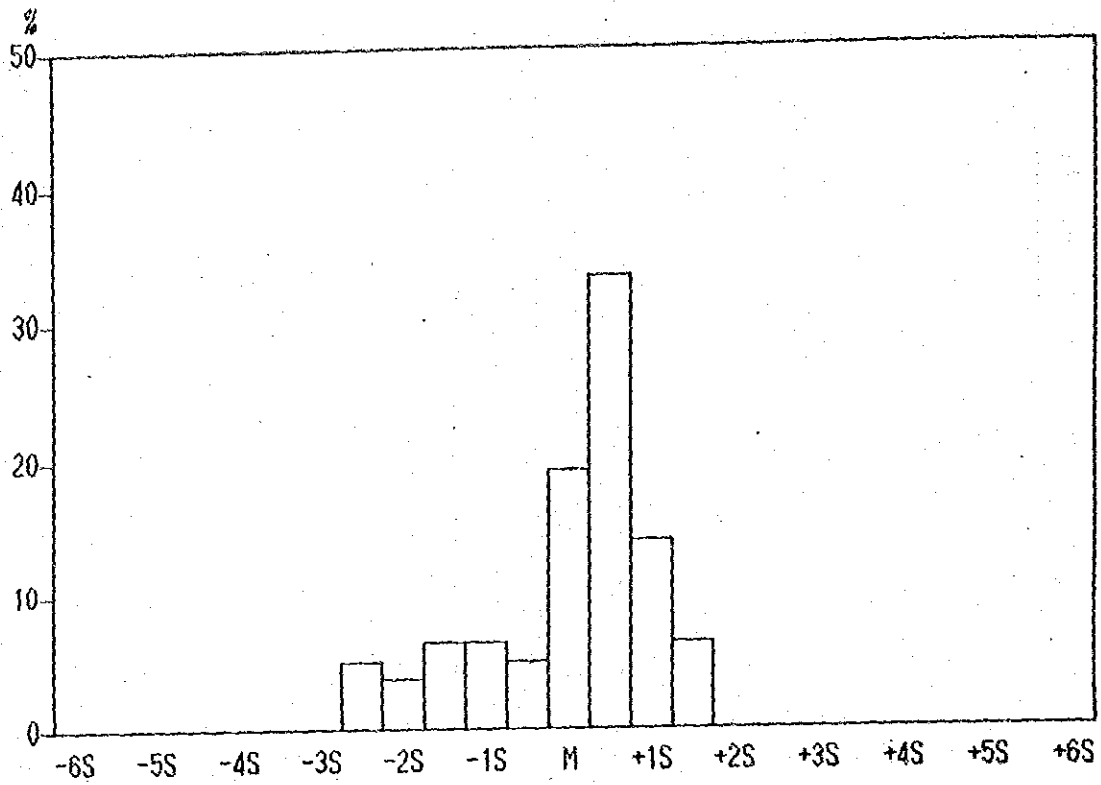
Histogram of Mn contents in Lithological Code; N2A
