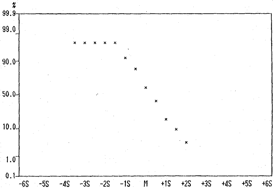
Cumulative Frequency Curve of Cu contents in Lithological Code; NQL
