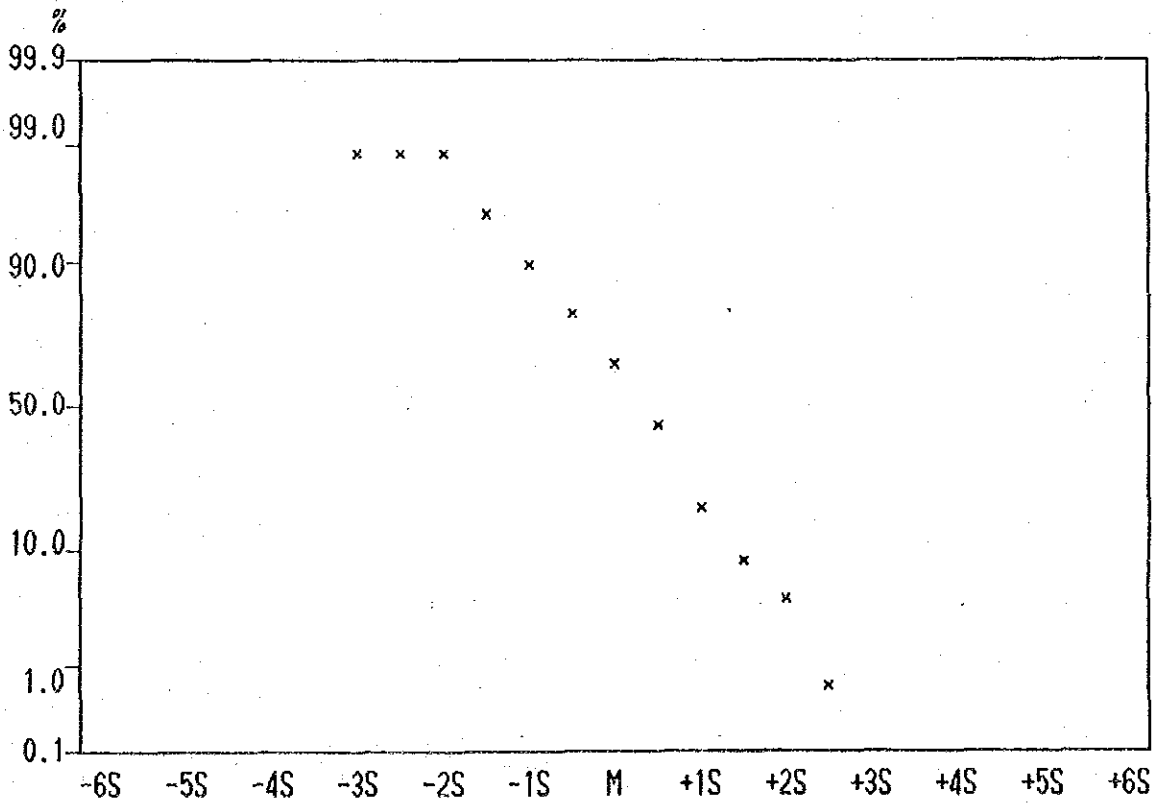
Cumulative Frequency Curve of Co contents in Lithological Code; R
