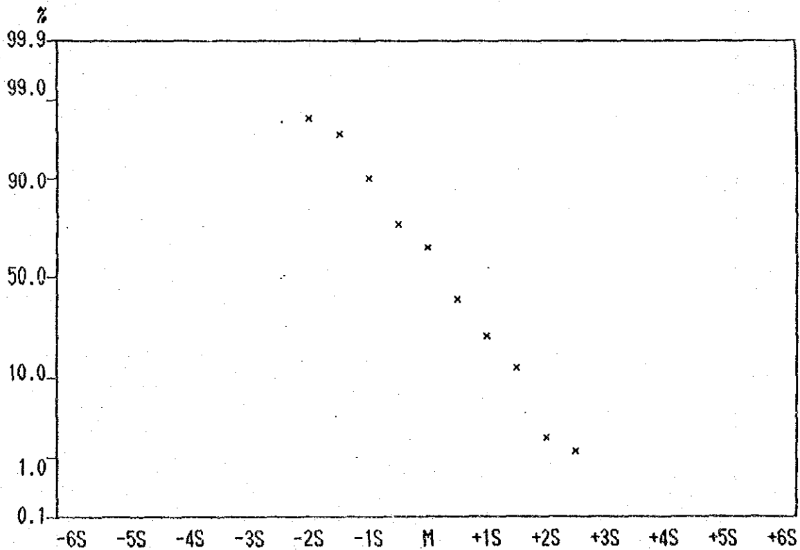
Cumulative Frequency Curve of Co contents in Lithological Code; NQS
