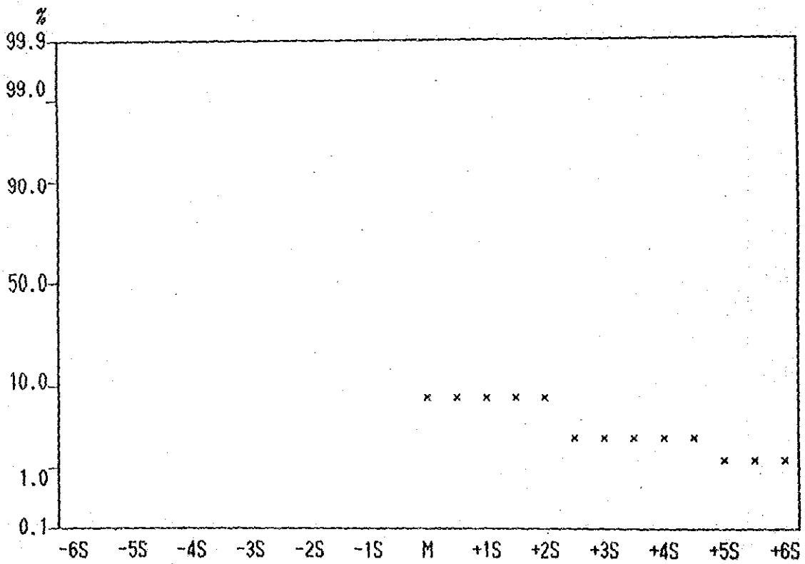
Cumulative Frequency Curve of Hg contents in Lithological Code; NZA
