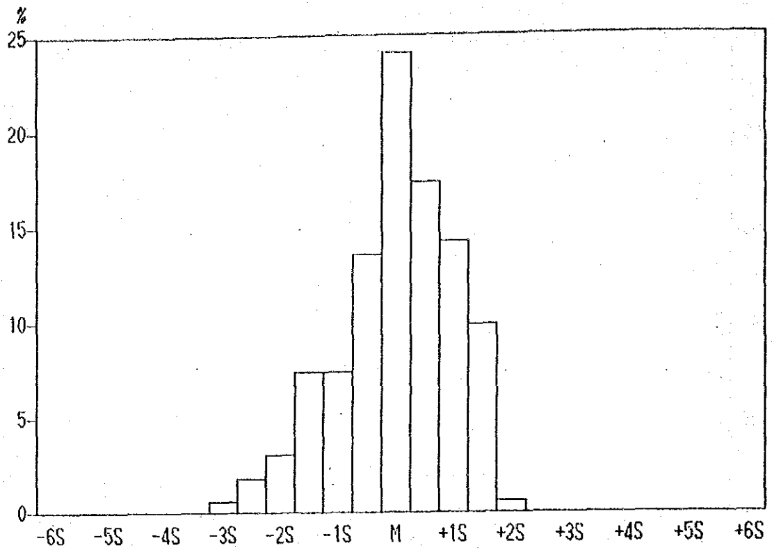
Histogram of Zn contents in Lithological Code; NQS
