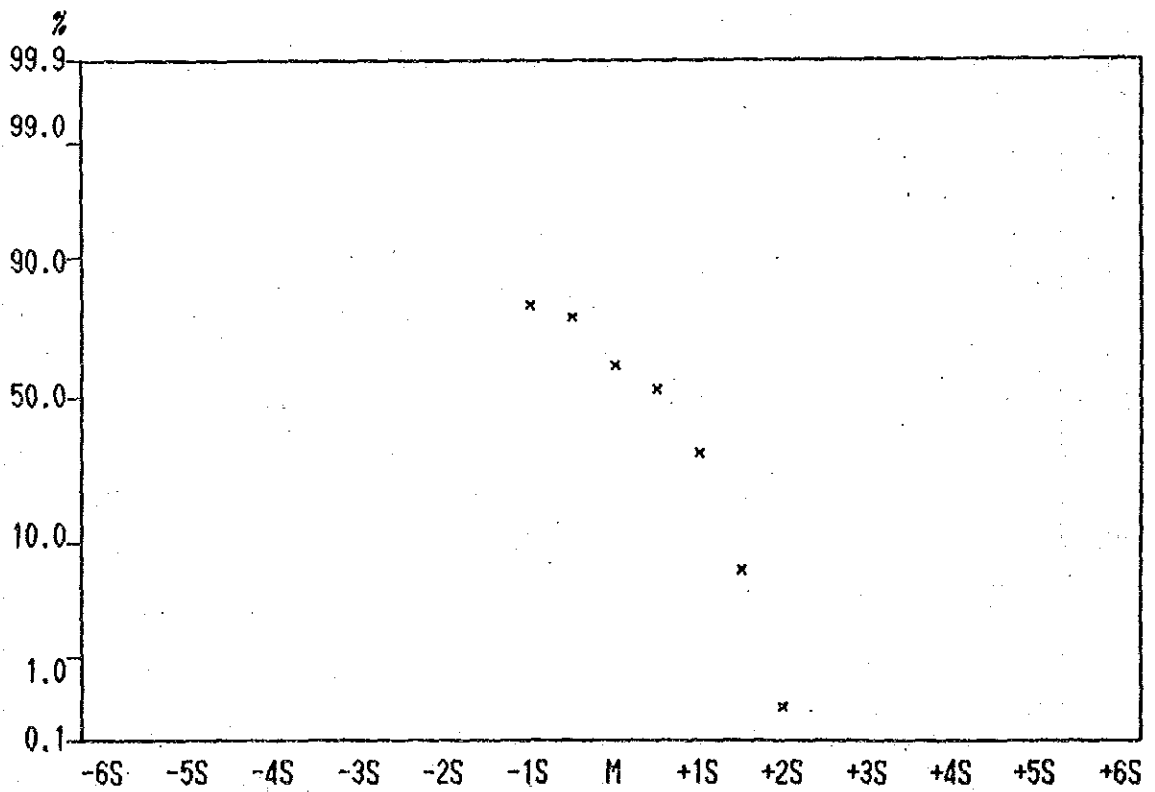
Cumulative Frequency Curve of As contents in Lithological Code; N2S
