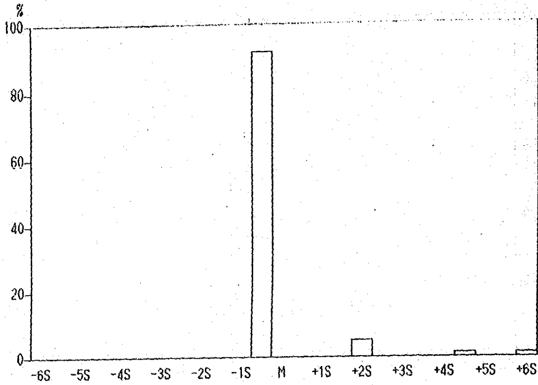
Histogram of Hg contents in Lithological Code; NZA
