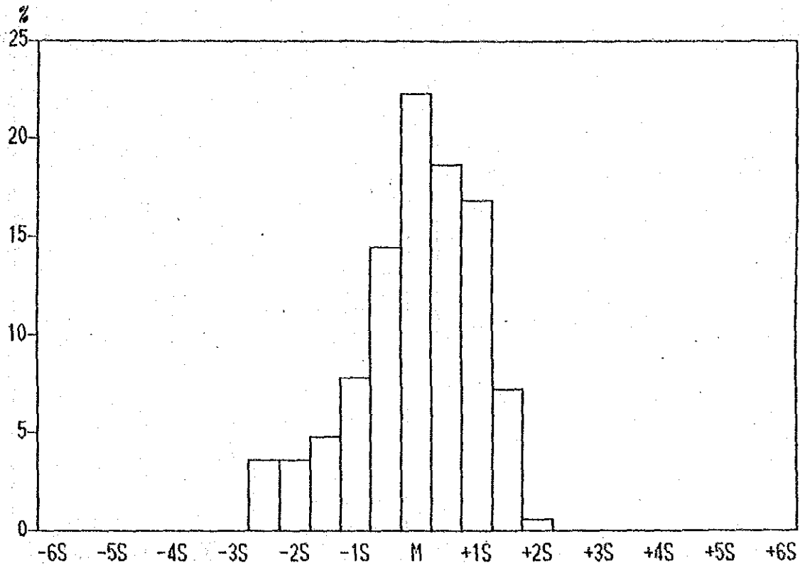
Histogram of Cu contents in Lithological Code; N2L
