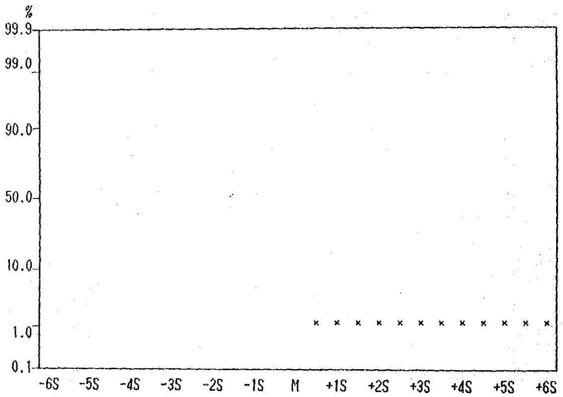
Cumulative Frequency Curve of Hg contents in Lithological Code; NQS
