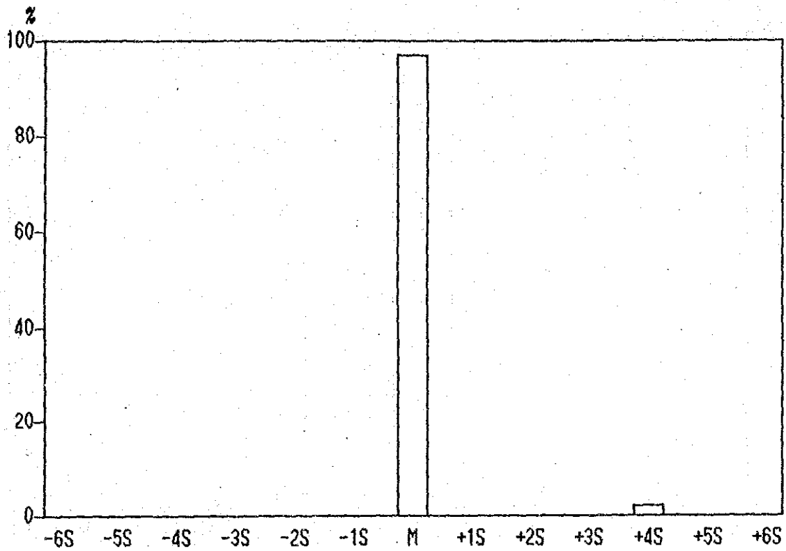
Histogram of Pb contents in Lithological Code; N1S
