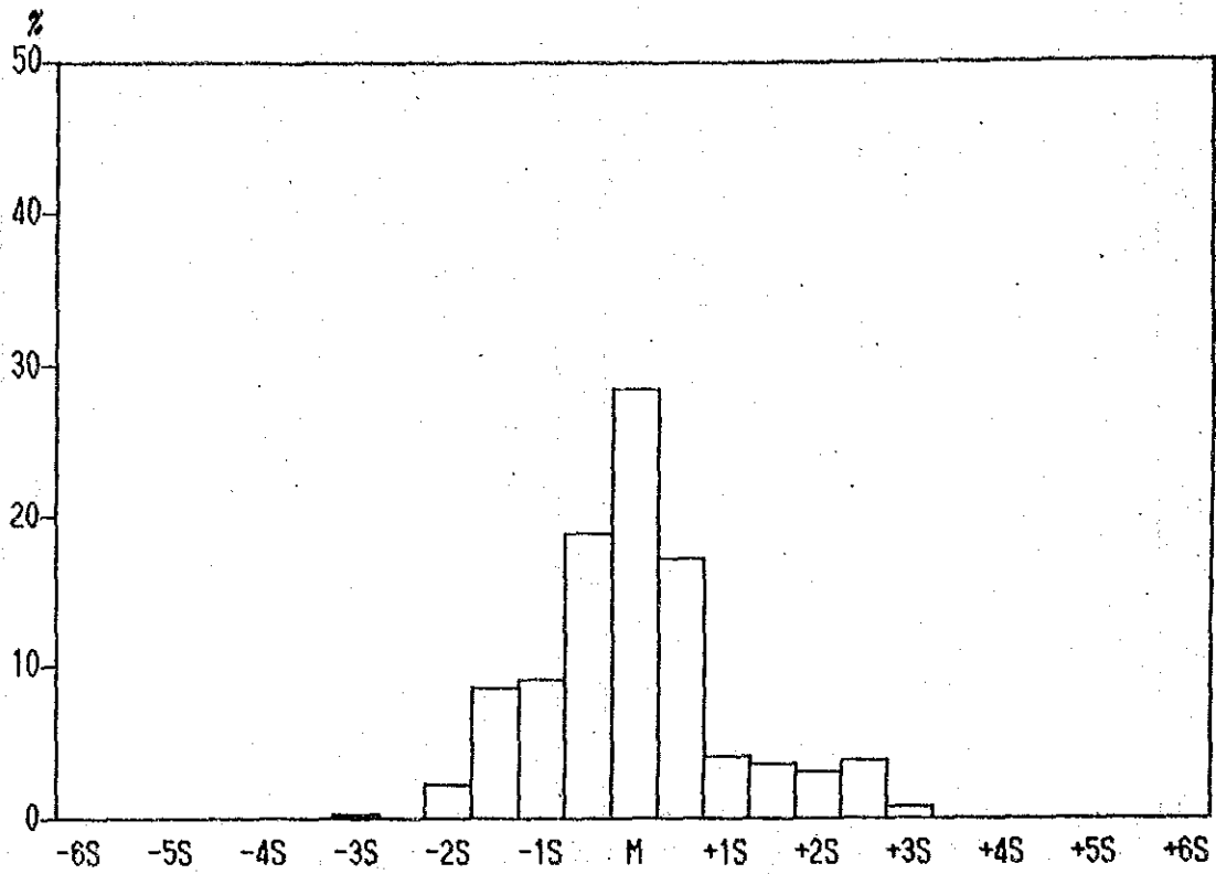
Histogram of Ni contents in Lithological Code; N2S
