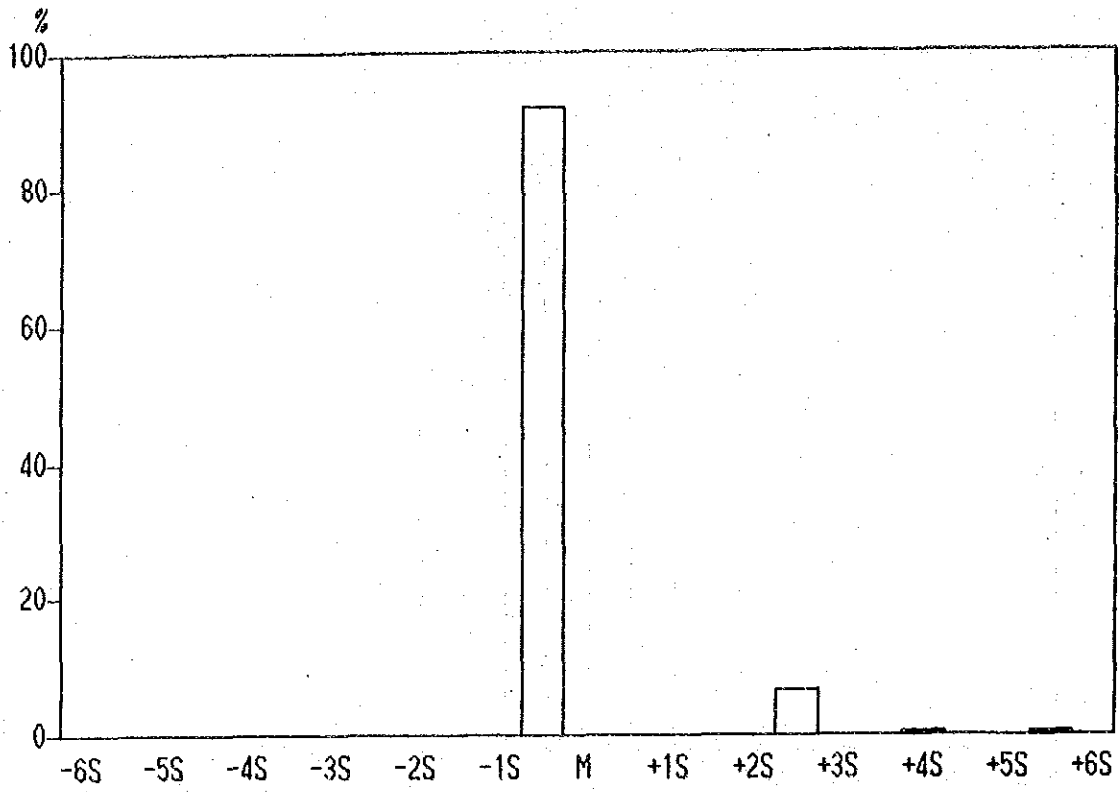
Histogram of Mo contents in Lithological Code; KPB
