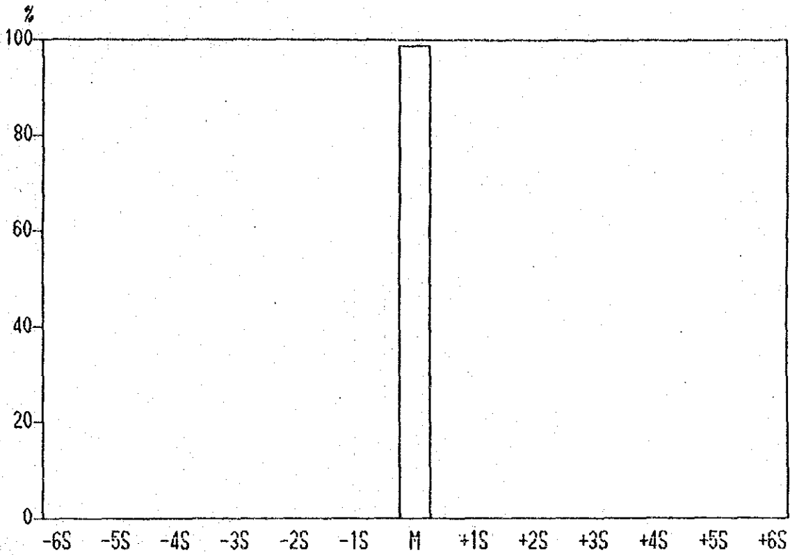
Histogram of Pb contents in Lithological Code; N2A
