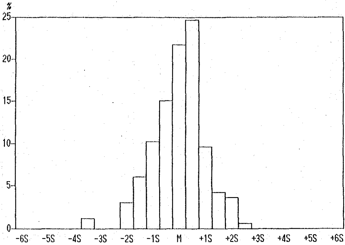
Histogram of Co contents in Lithological Code; R
