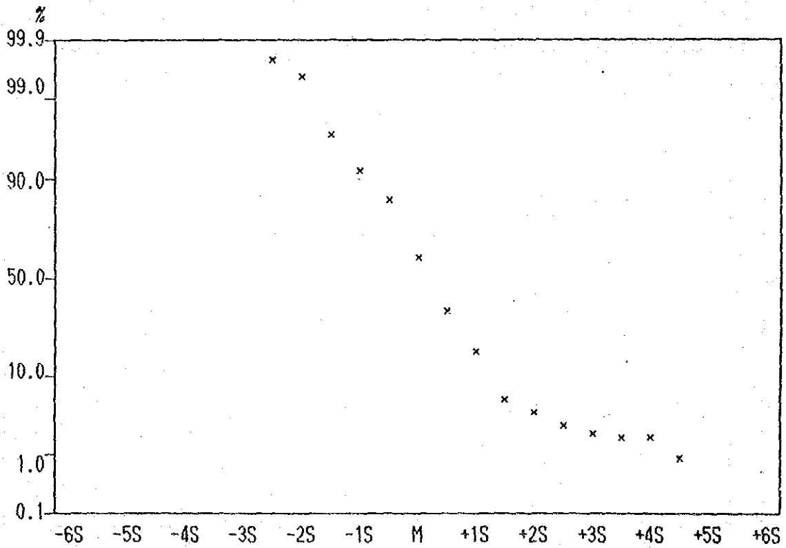
Cumulative Frequency Curve of Zn contents in Lithological Code; KPA
