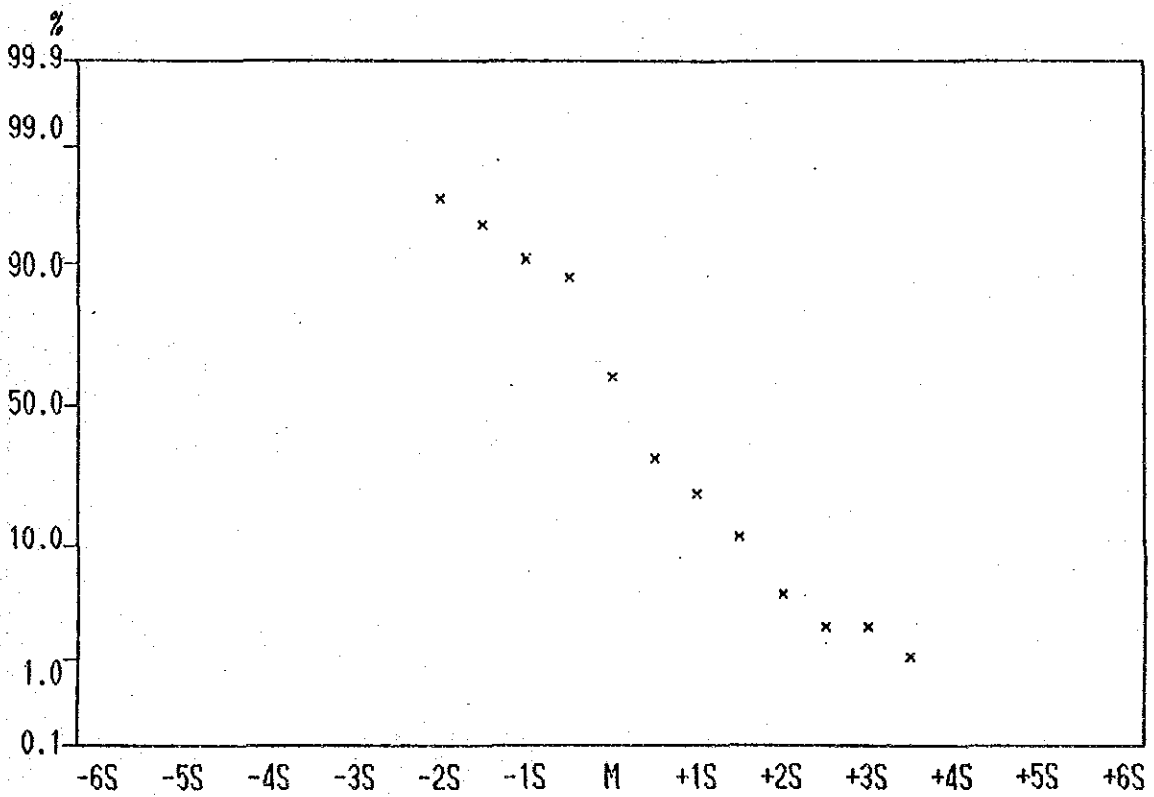
Cumulative Frequency Curve of Co contents in Lithological Code; N1S
