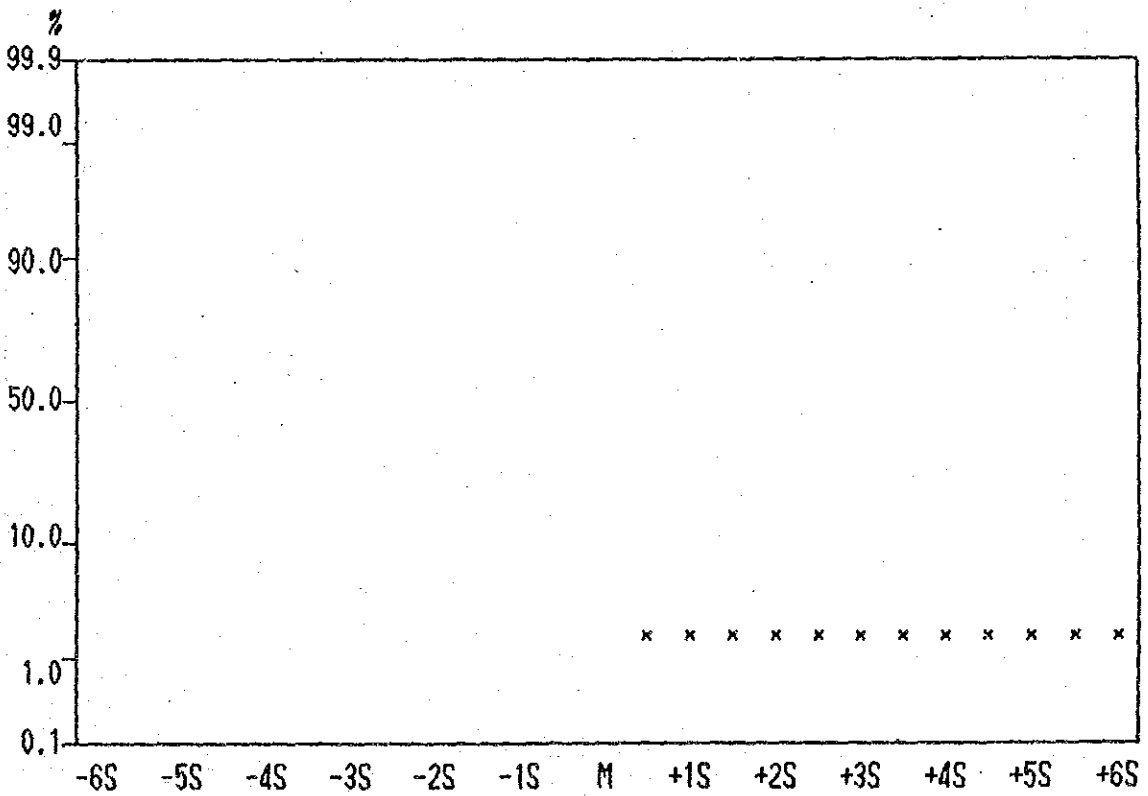
Cumulative Frequency Curve of Pb contents in Lithological Code; N2S
