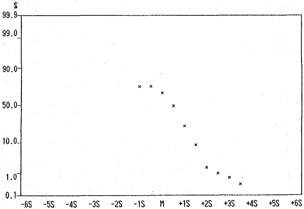
Cumulative Frequency Curve of As contents in Lithological Code; KPB
