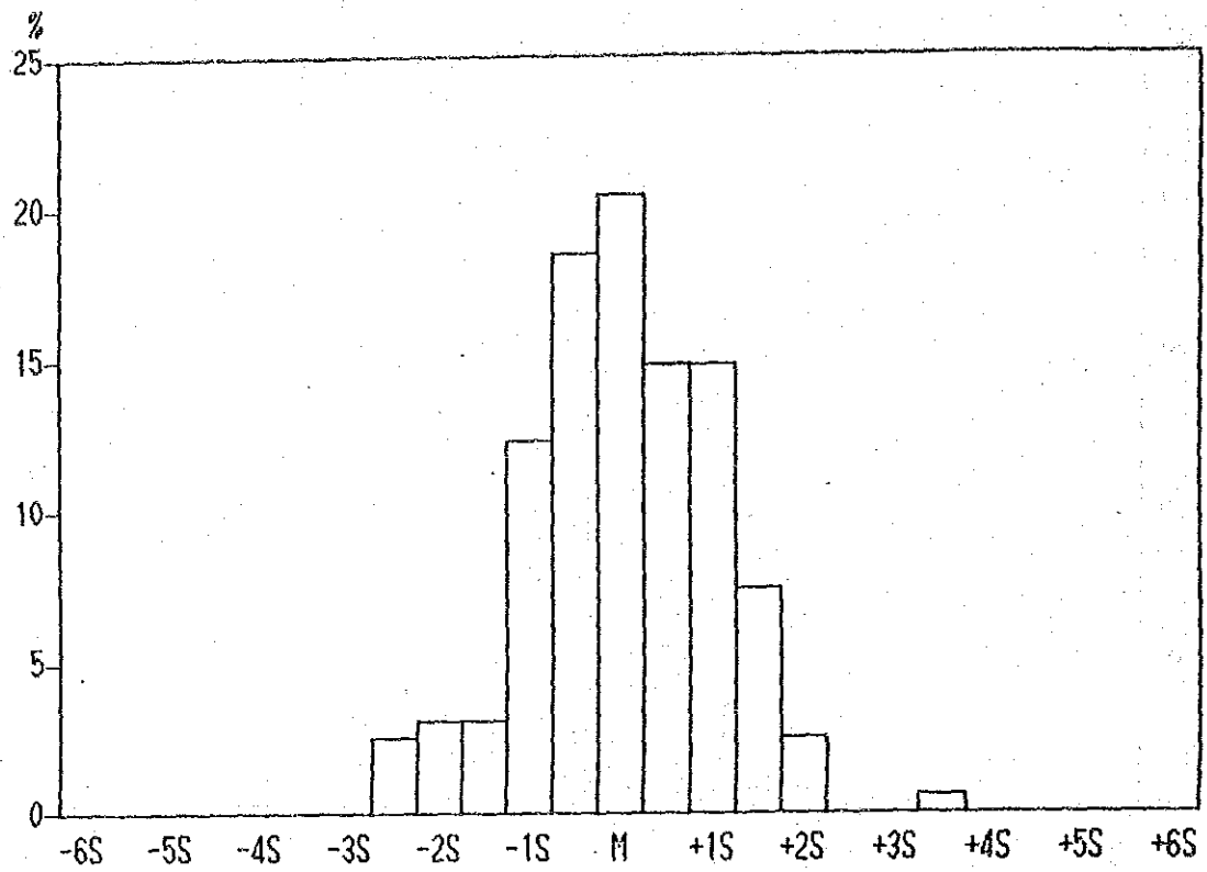
Histogram of Mn contents in Lithological Code; NQS
