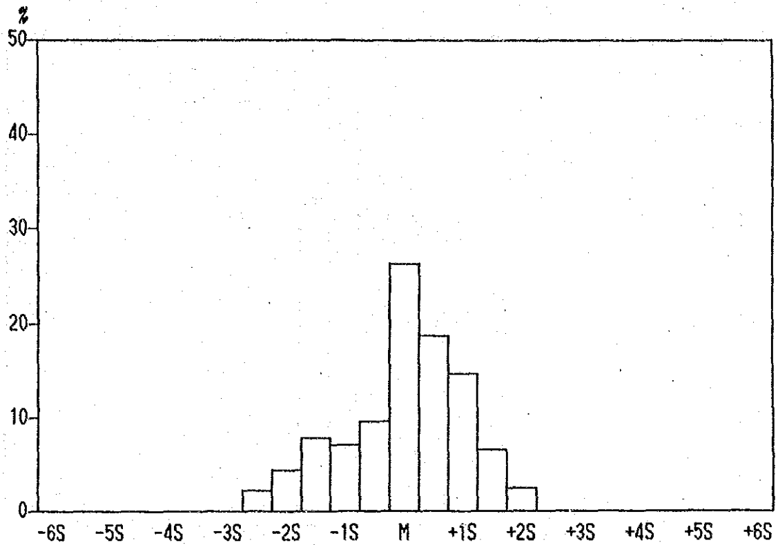
Histogram of Co contents in Lithological Code; N2S
