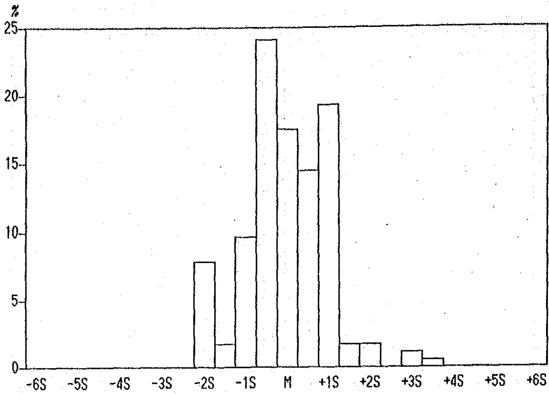
Histogram of Zn contents in Lithological Code; N2L
