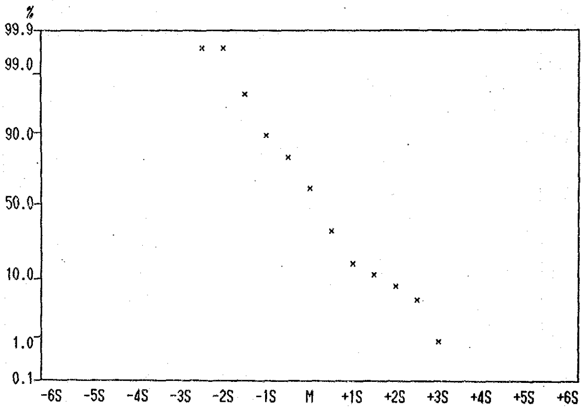
Cumulative Frequency Curve of Ni contents in Lithological Code; N2S
