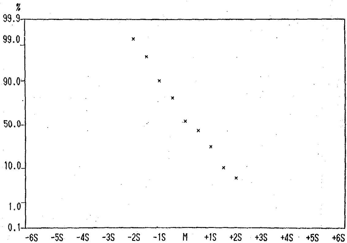
Cumulative Frequency Curve of Ni contents in Lithological Code; N2L
