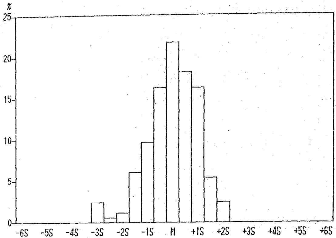
Histogram of Ni contents in Lithological Code; R
