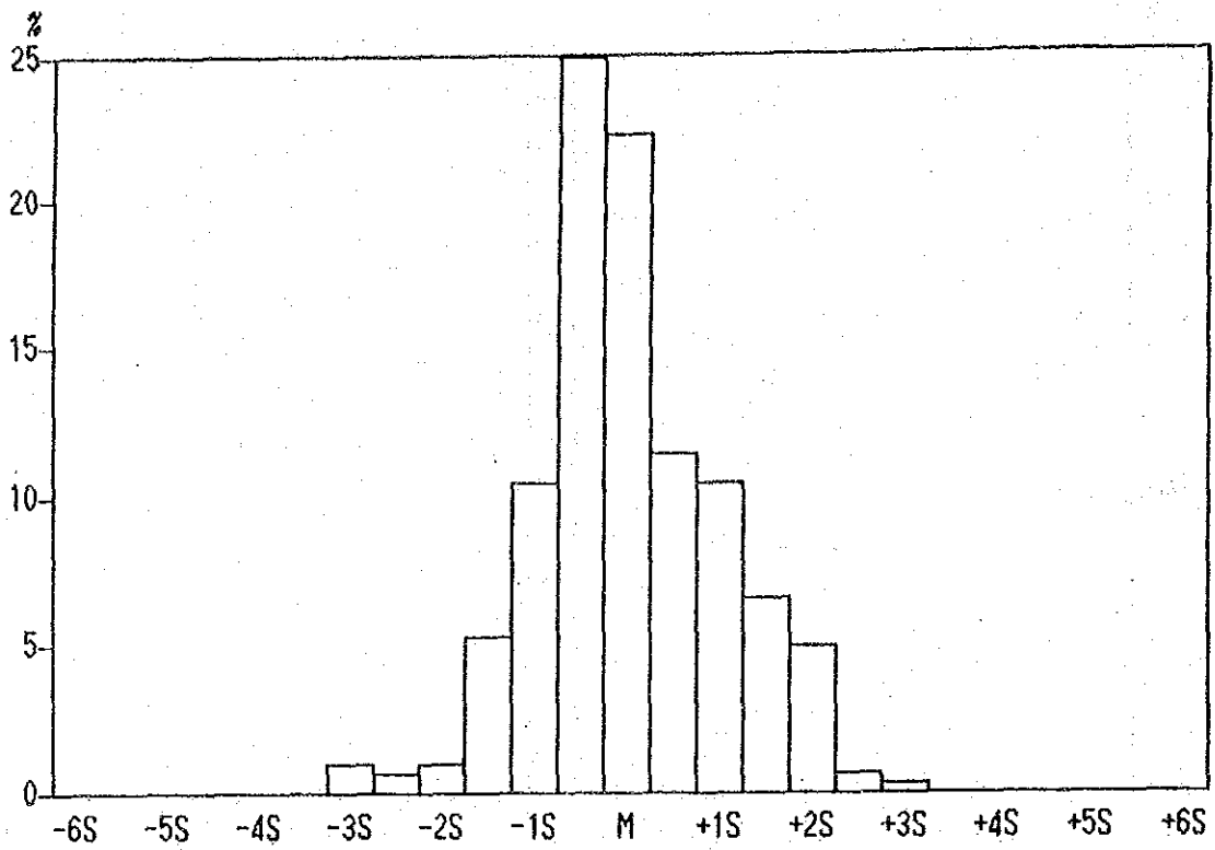
Histogram of Zn contents in Lithological Code; KPB
