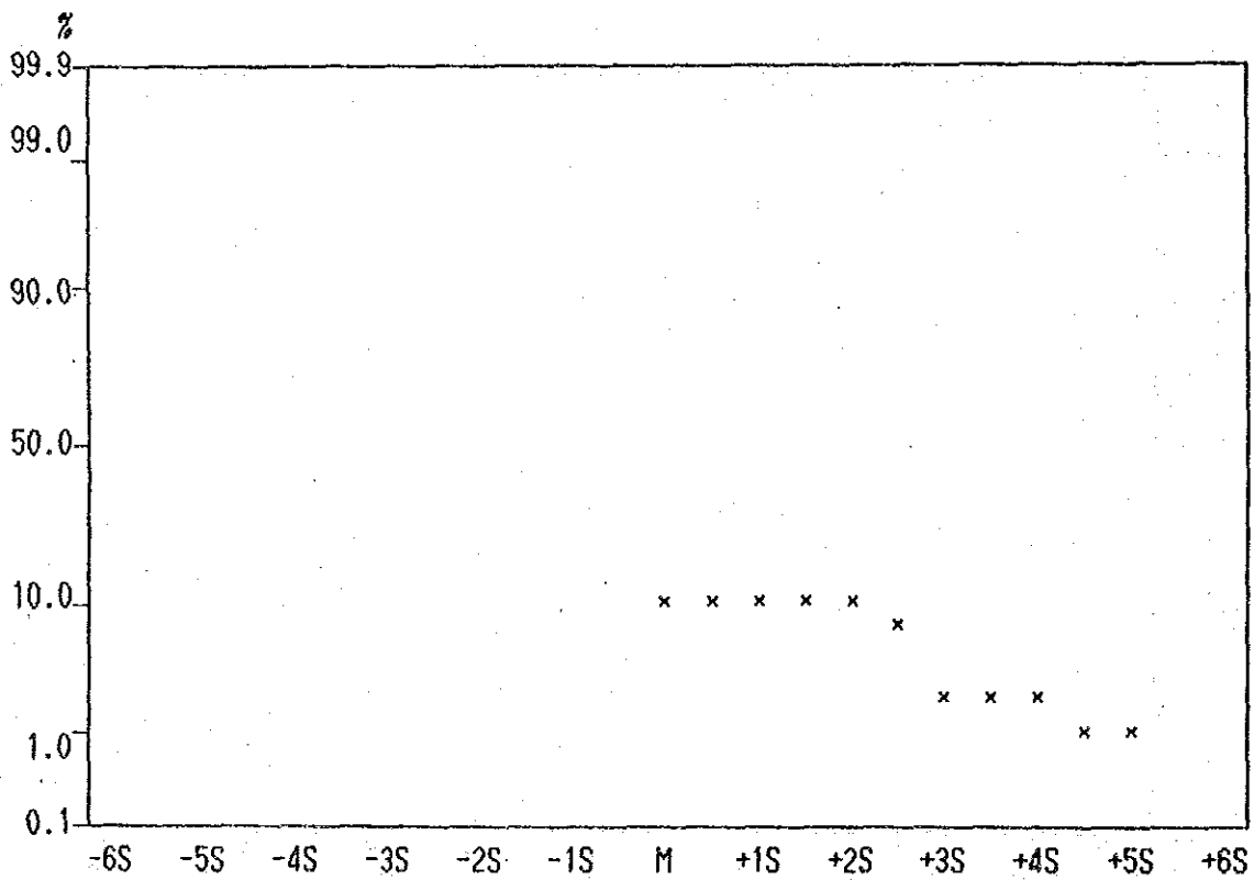
Cumulative Frequency Curve of Hg contents in Lithological Code; N1S
