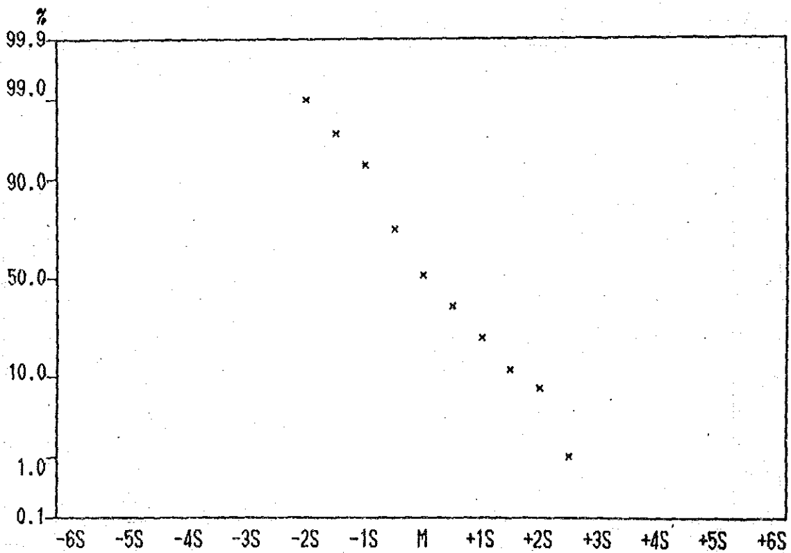
Cumulative Frequency Curve of Zn contents in Lithological Code; N1S
