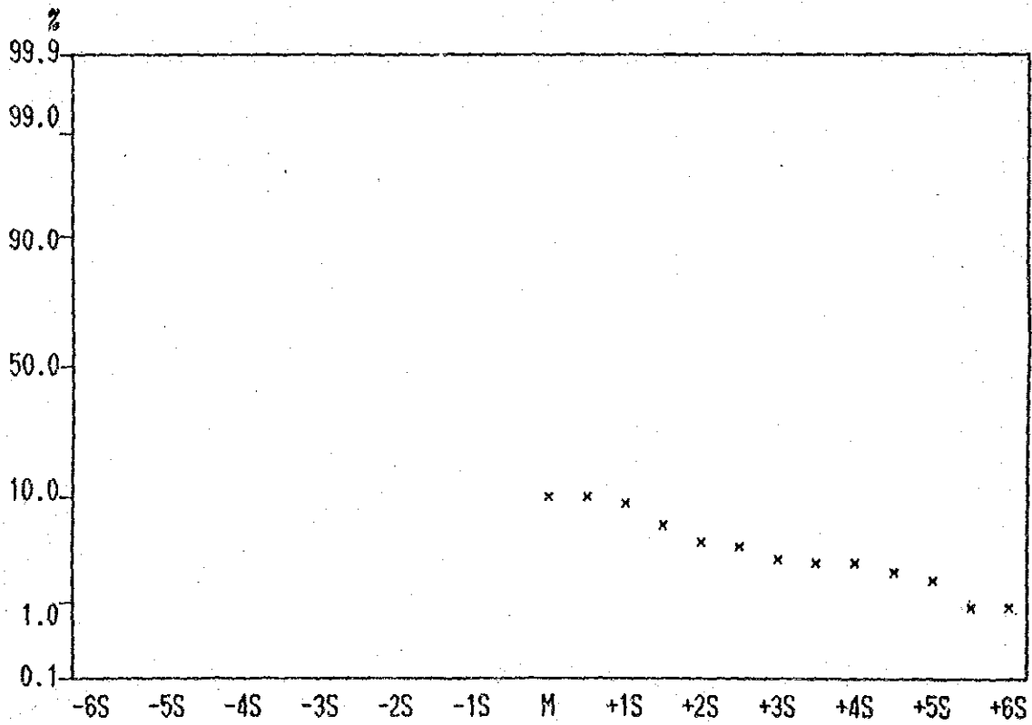
Cumulative Frequency Curve of Hg contents in Lithological Code; KPA
