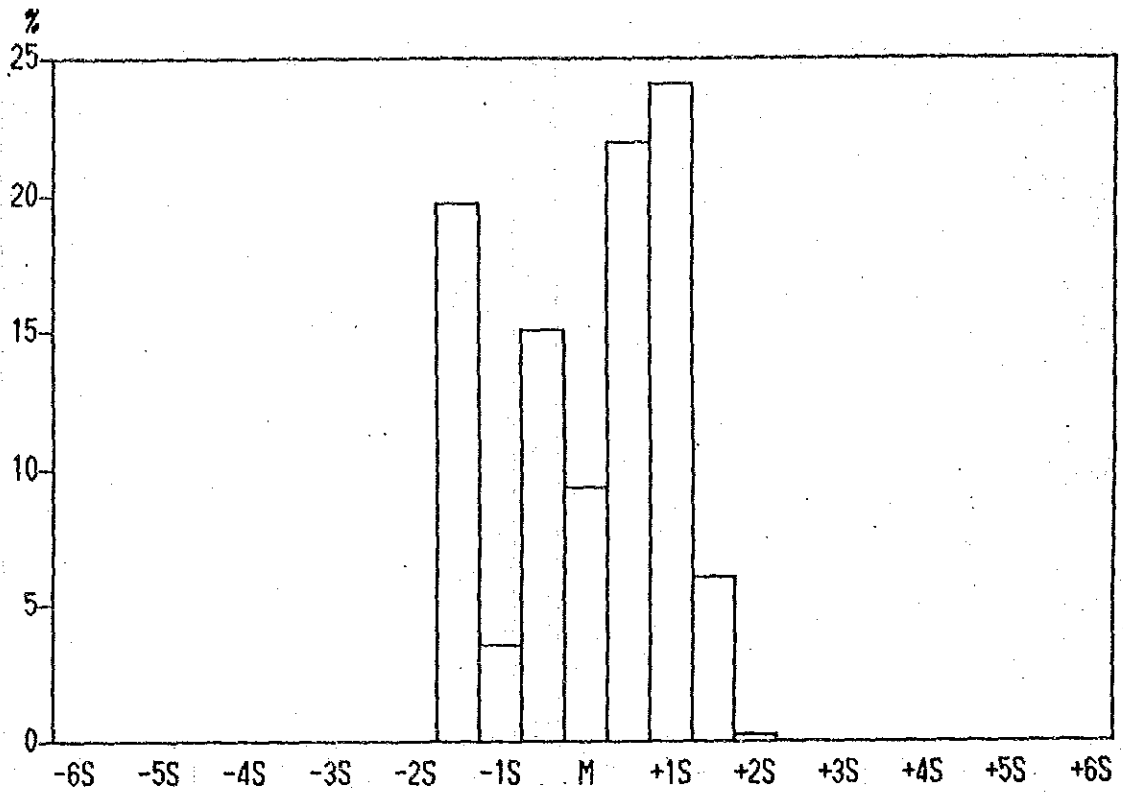
Histogram of As contents in Lithological Code; N2S
