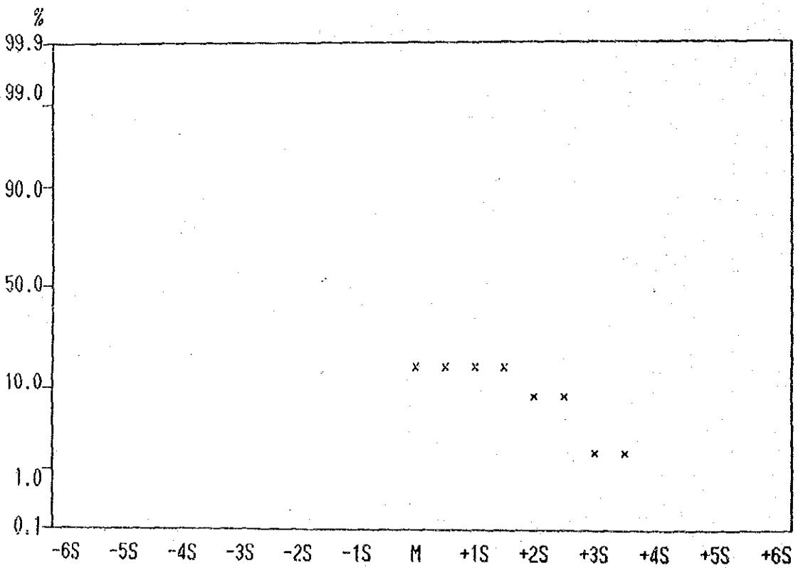
Cumulative Frequency Curve of Mo contents in Lithological Code; R
