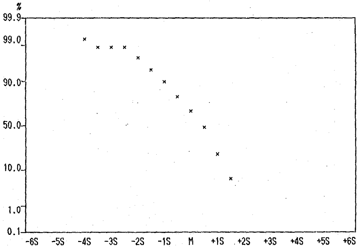
Cumulative Frequency Curve of As contents in Lithological Code; N2L
