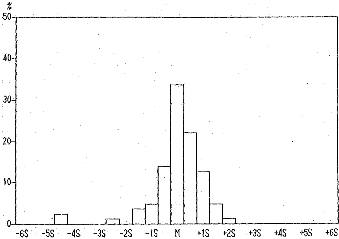
Histogram of Co contents in Lithological Code; NQL
