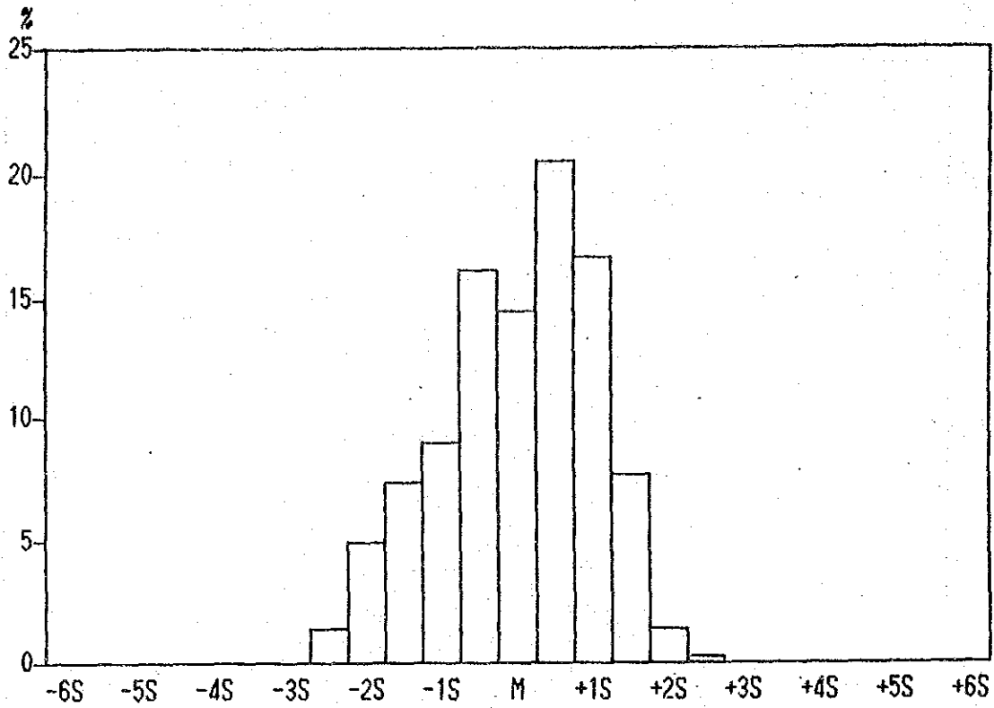
Histogram of Mn contents in Lithological Code; N2S
