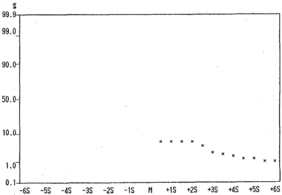
Cumulative Frequency Curve of Pb contents in Lithological Code; KPB
