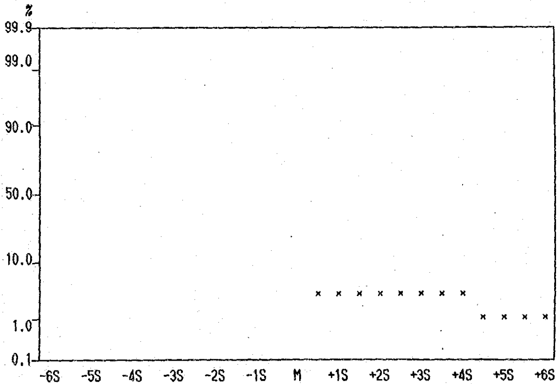
Cumulative Frequency Curve of Pb contents in Lithological Code; N1S
