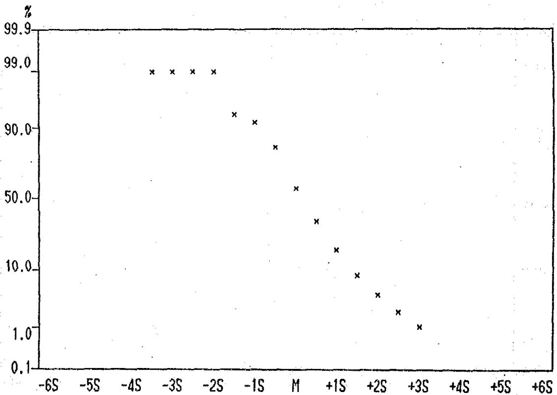
Cumulative Frequency Curve of Ni contents in Lithological Code; N1S
