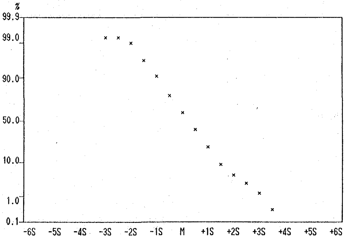
Cumulative Frequency Curve of Co contents in Lithological Code; KPB
