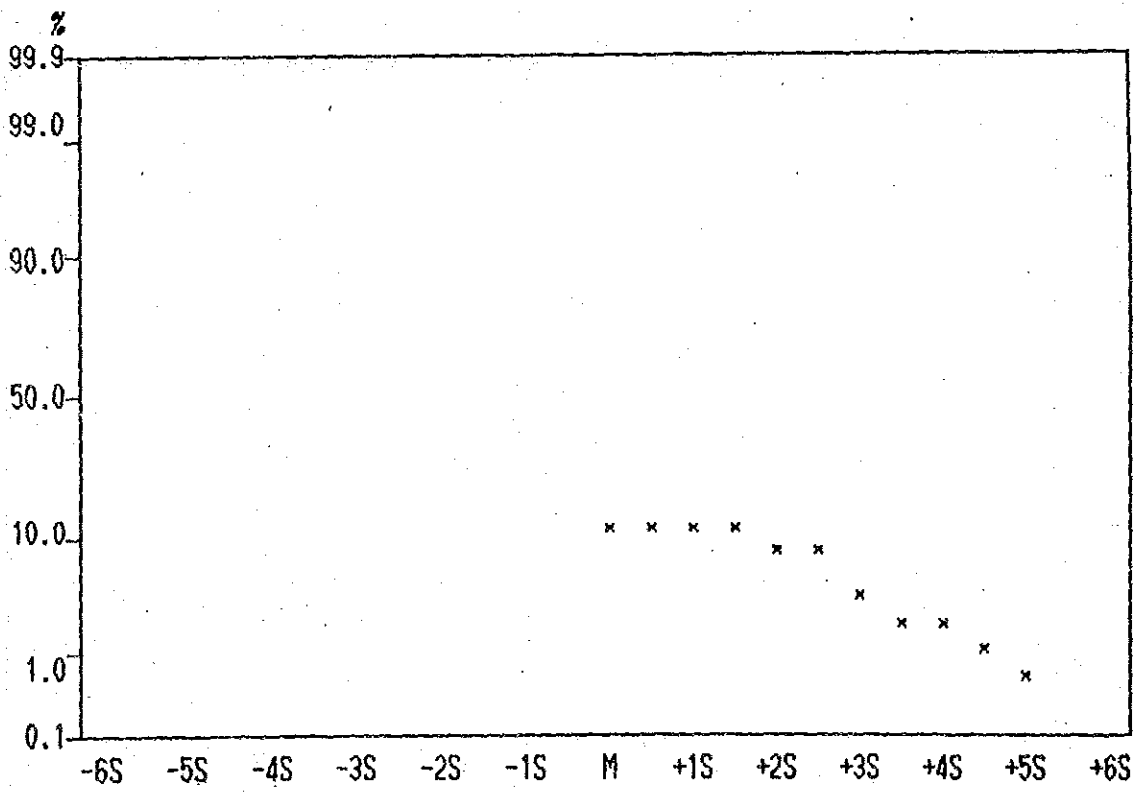
Cumulative Frequency Curve of Mo contents in Lithological Code; N2S
