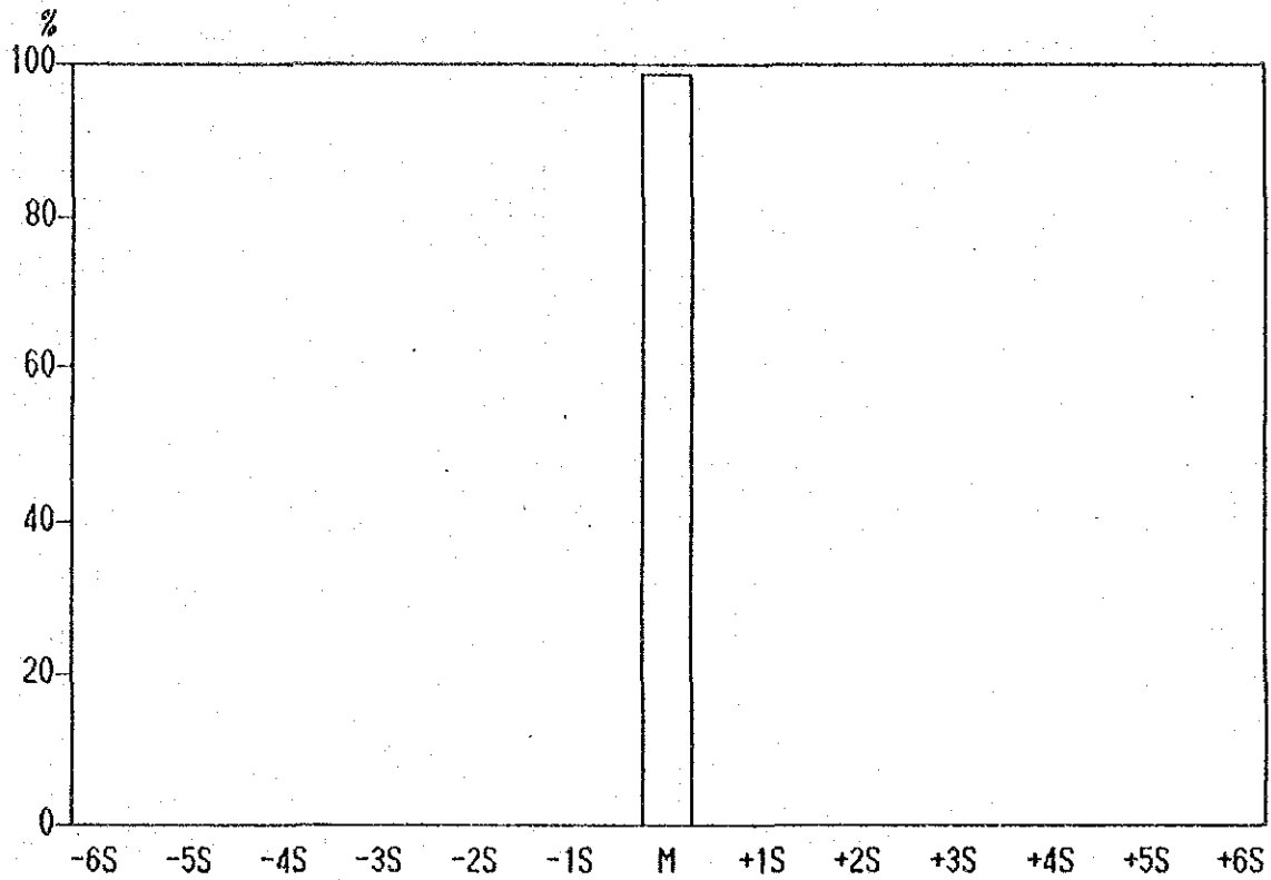
Histogram of Pb contents in Lithological Code; R
