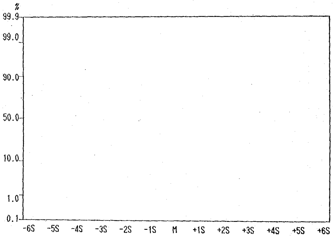
Cumulative Frequency Curve of Hg contents in Lithological Code; R
