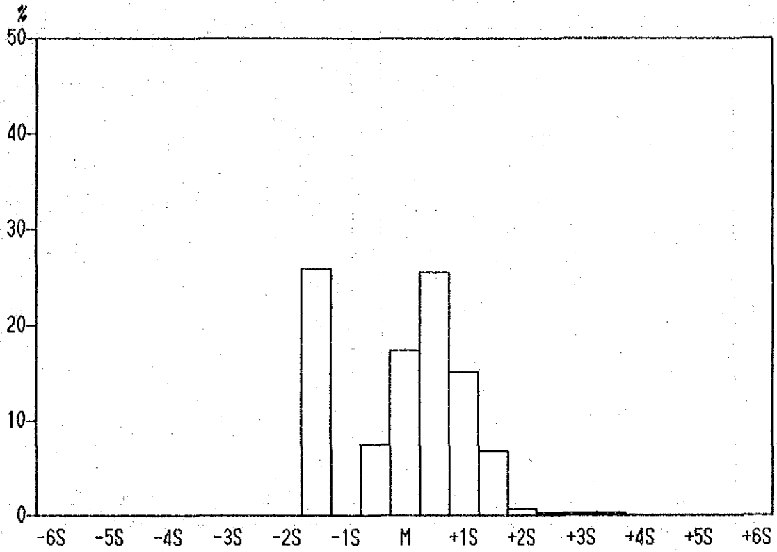
Histogram of As contents in Lithological Code; KPB
