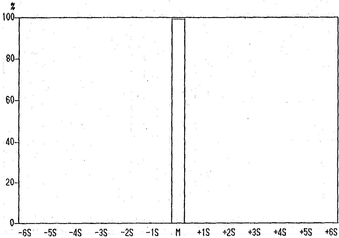
Histogram of Hg contents in Lithological Code; N2S
