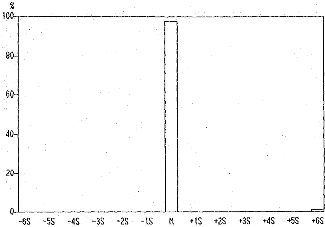
Histogram of Pb contents in Lithological Code; NQL
