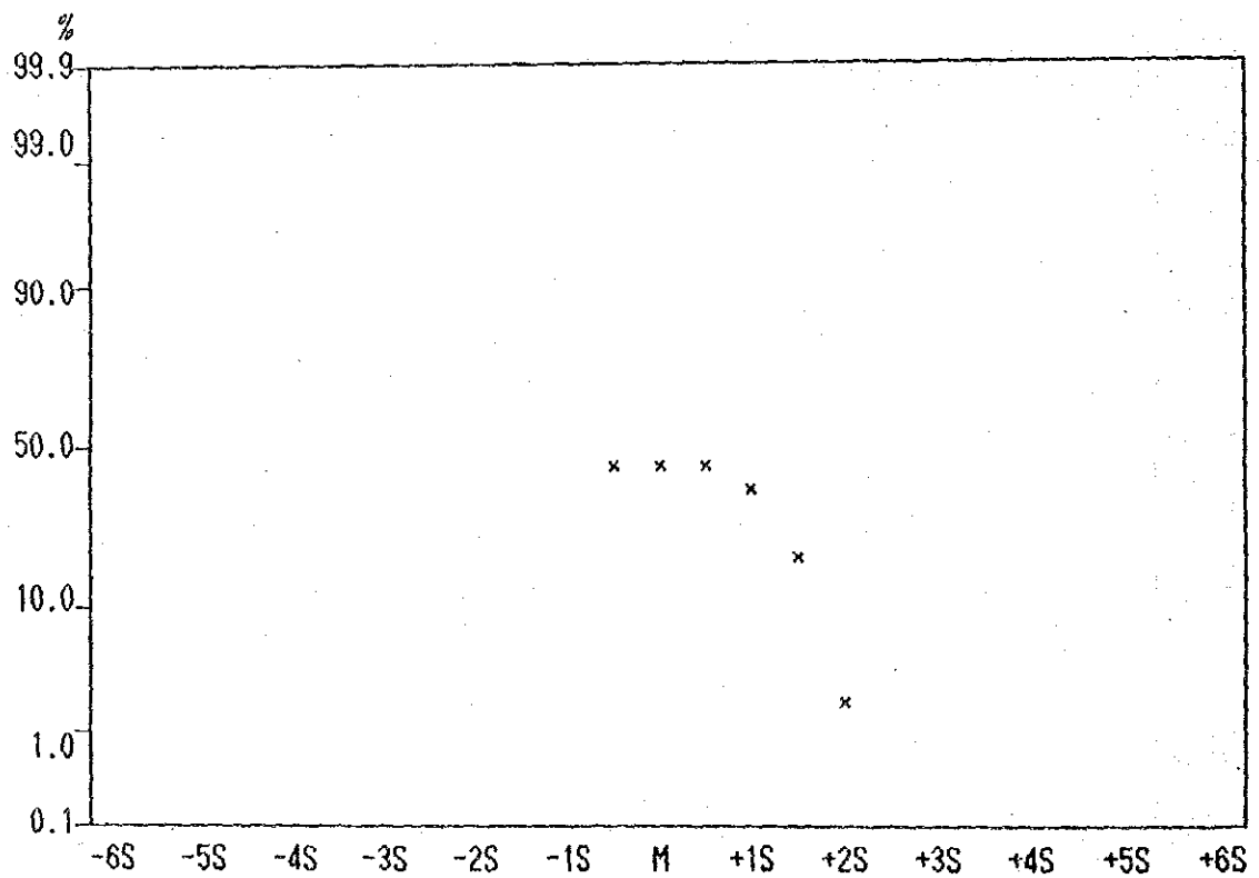
Cumulative Frequency Curve of Mo contents in Lithological Code; NQS
