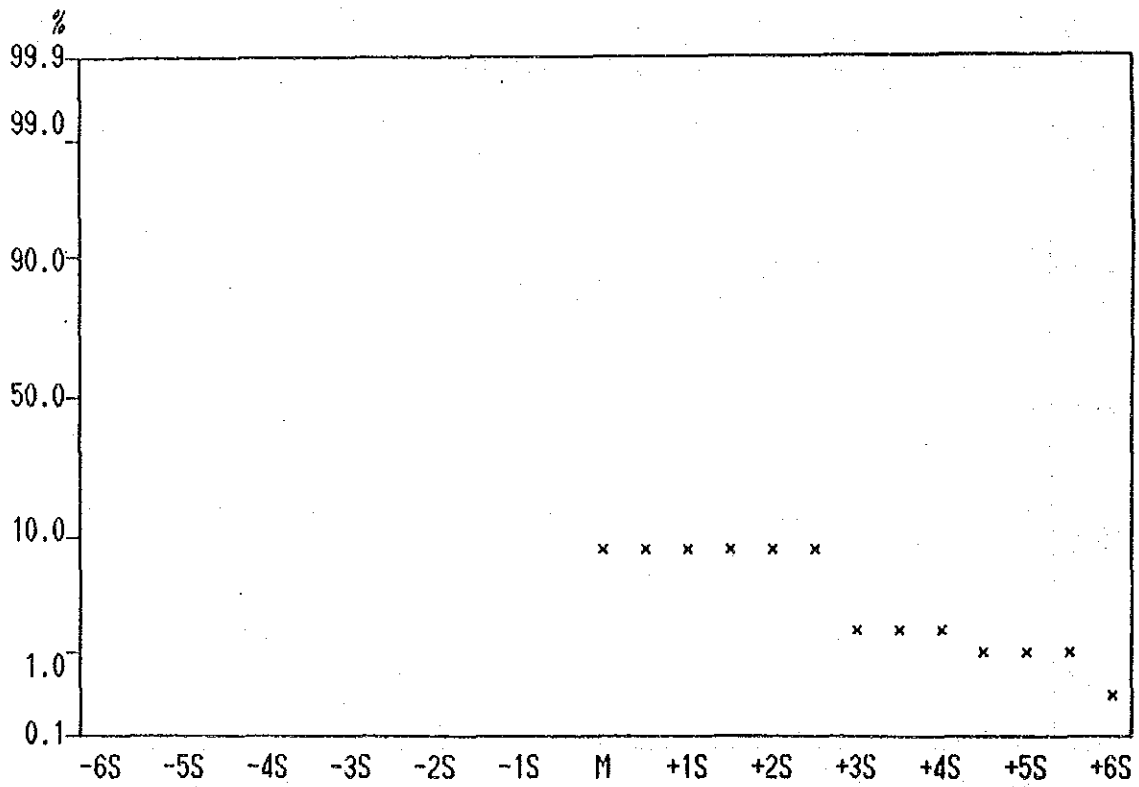
Cumulative Frequency Curve of Mo contents in Lithological Code; KPB
