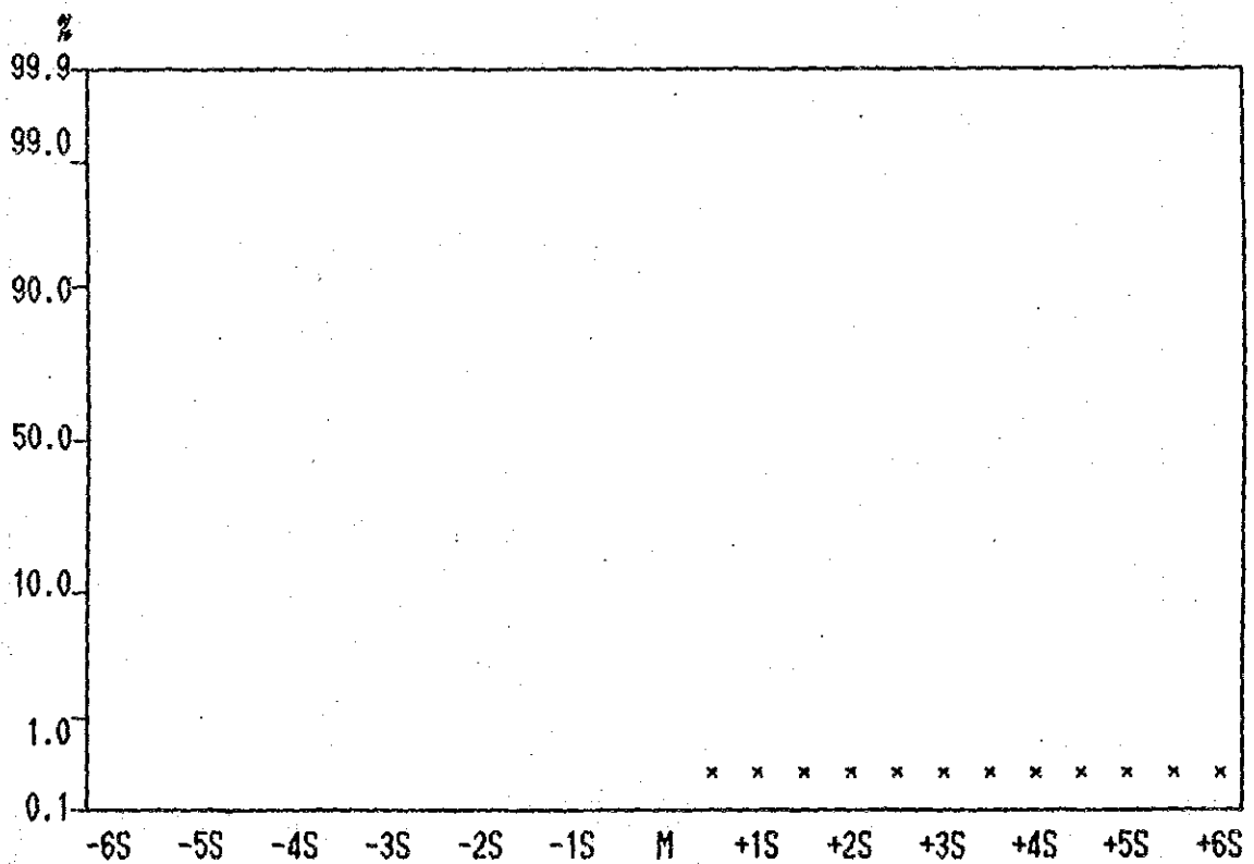
Cumulative Frequency Curve of Ag contents in Lithological Code; N2S
