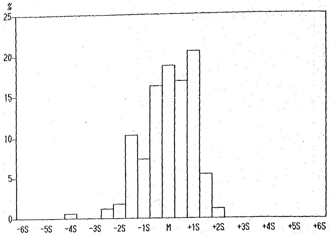
Histogram of Mn contents in Lithological Code; R
