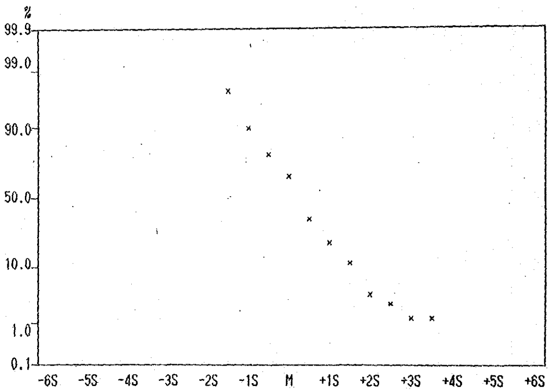
Cumulative Frequency Curve of Ni contents in Lithological Code; N2A
