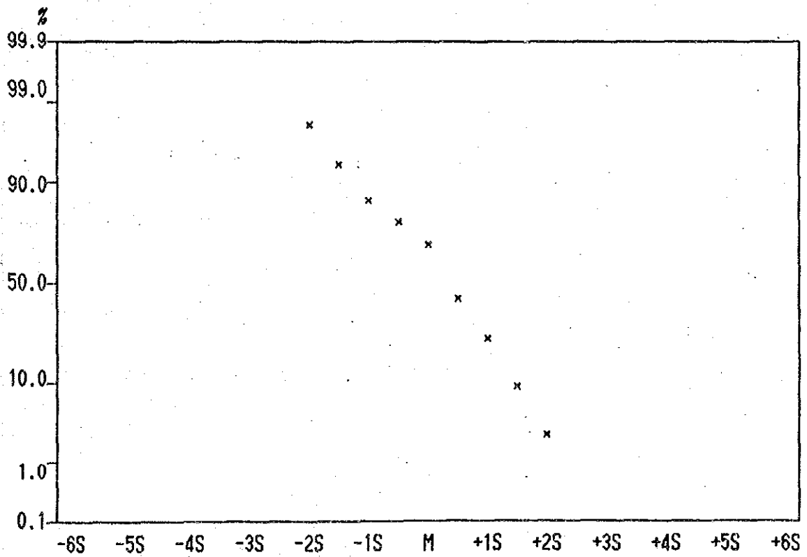
Cumulative Frequency Curve of Co contents in Lithological Code; N2S
