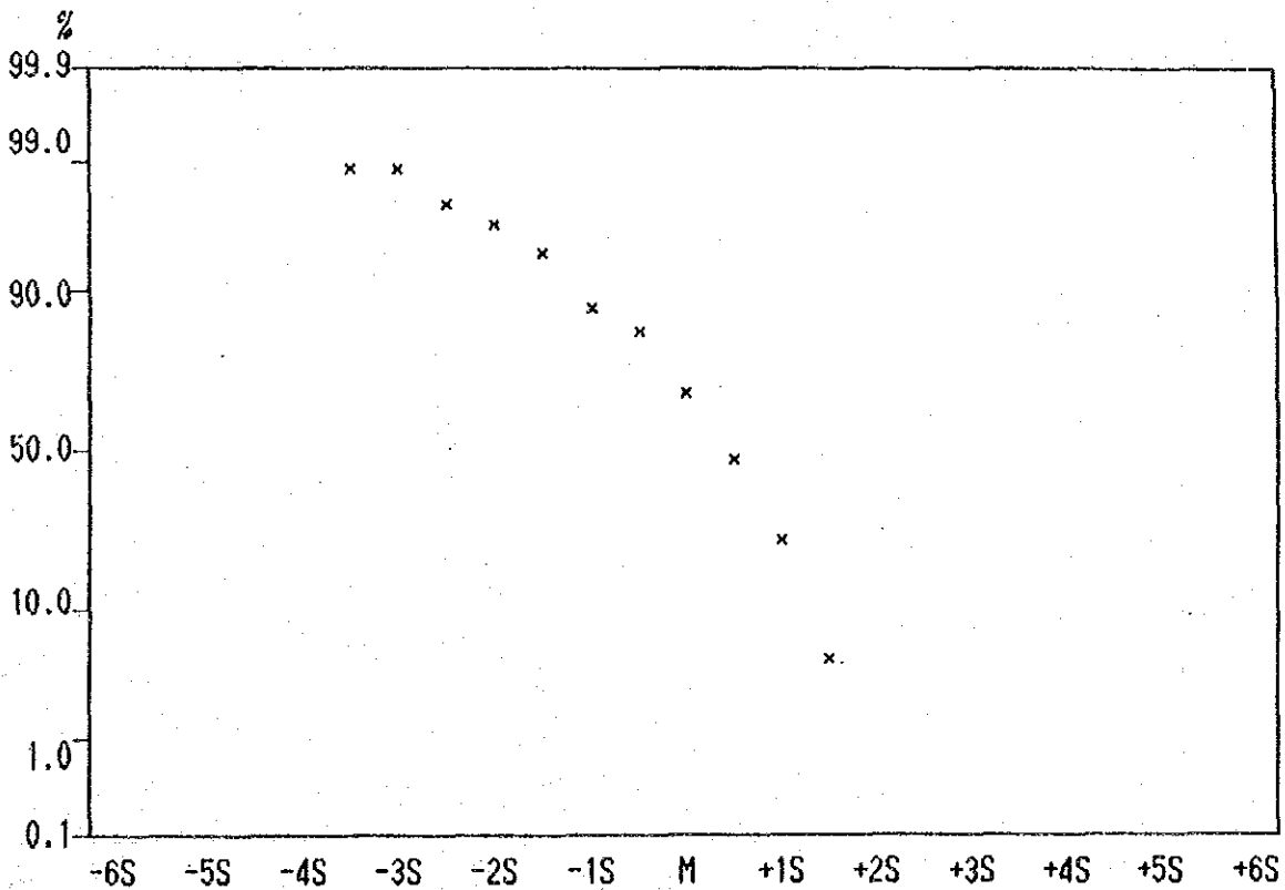
Cumulative Frequency Curve of As contents in Lithological Code; NQL
