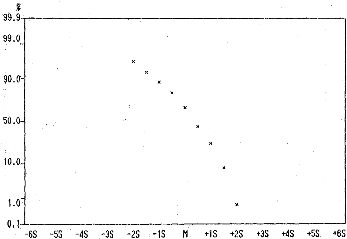
Cumulative Frequency Curve of Cu contents in Lithological Code; N2L
