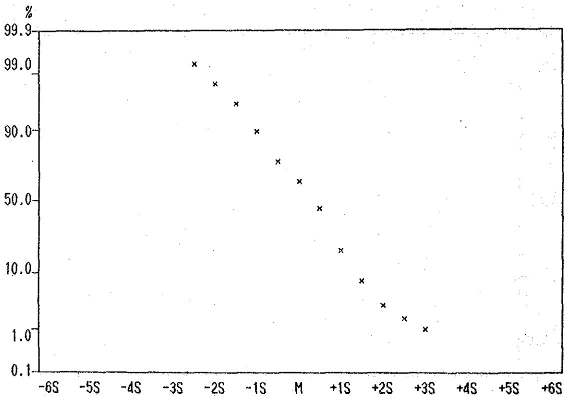
Cumulative Frequency Curve of Mn contents in Lithological Code; KPB
