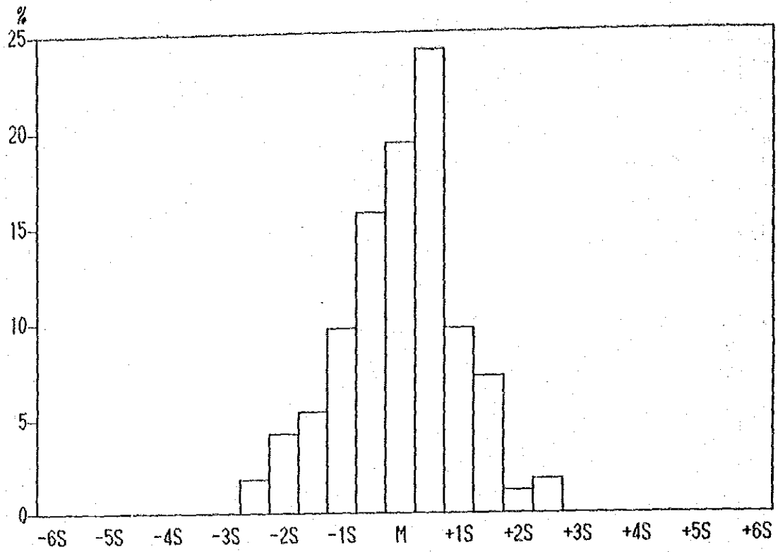
Histogram of Zn contents in Lithological Code; R
