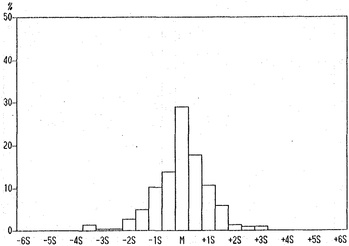
Histogram of Cu contents in Lithological Code; KPS
