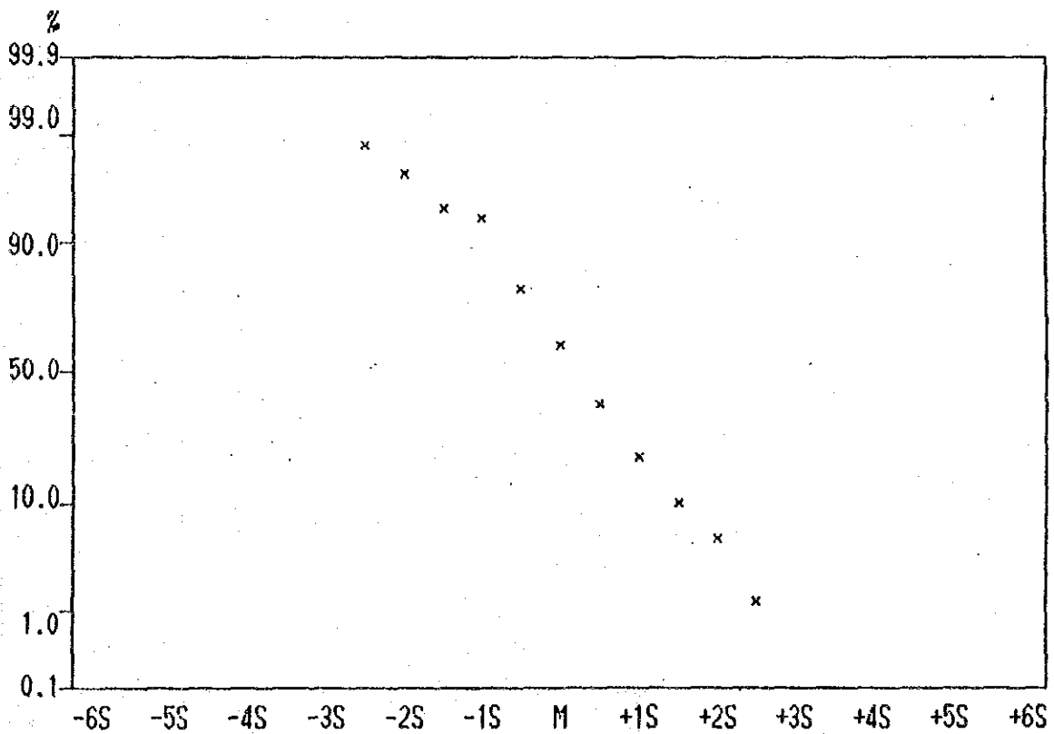
Cumulative Frequency Curve of Co contents in Lithological Code; N2A
