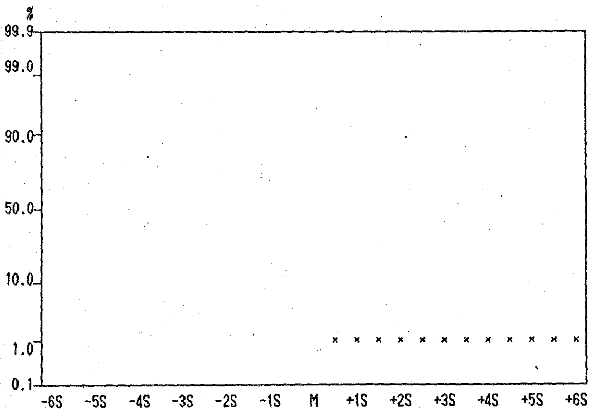
Cumulative Frequency Curve of Ag contents in Lithological Code; N1S
