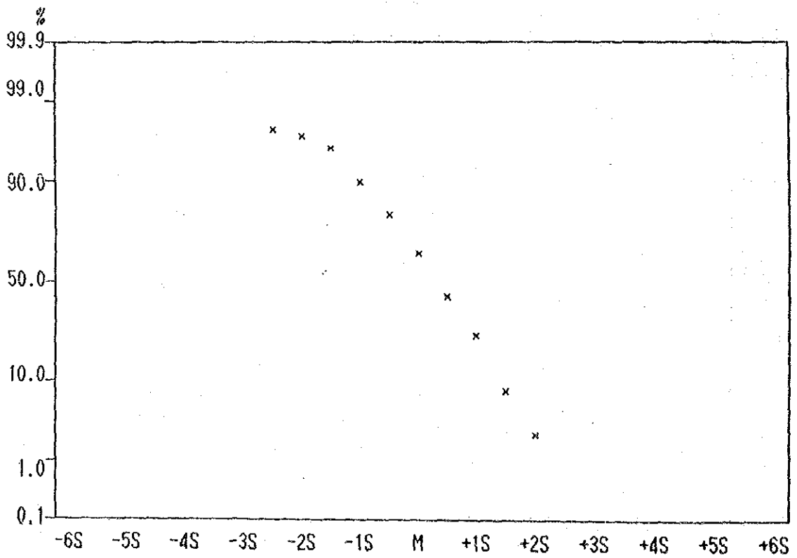
Cumulative Frequency Curve of Ni contents in Lithological Code; R
