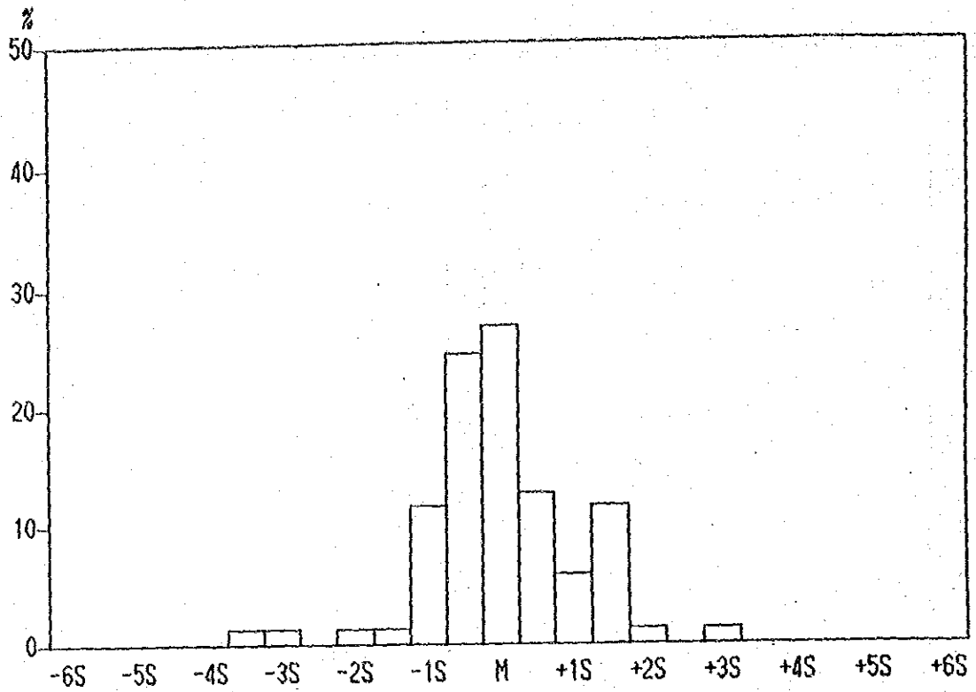
Histogram of Zn contents in Lithological Code; NQL
