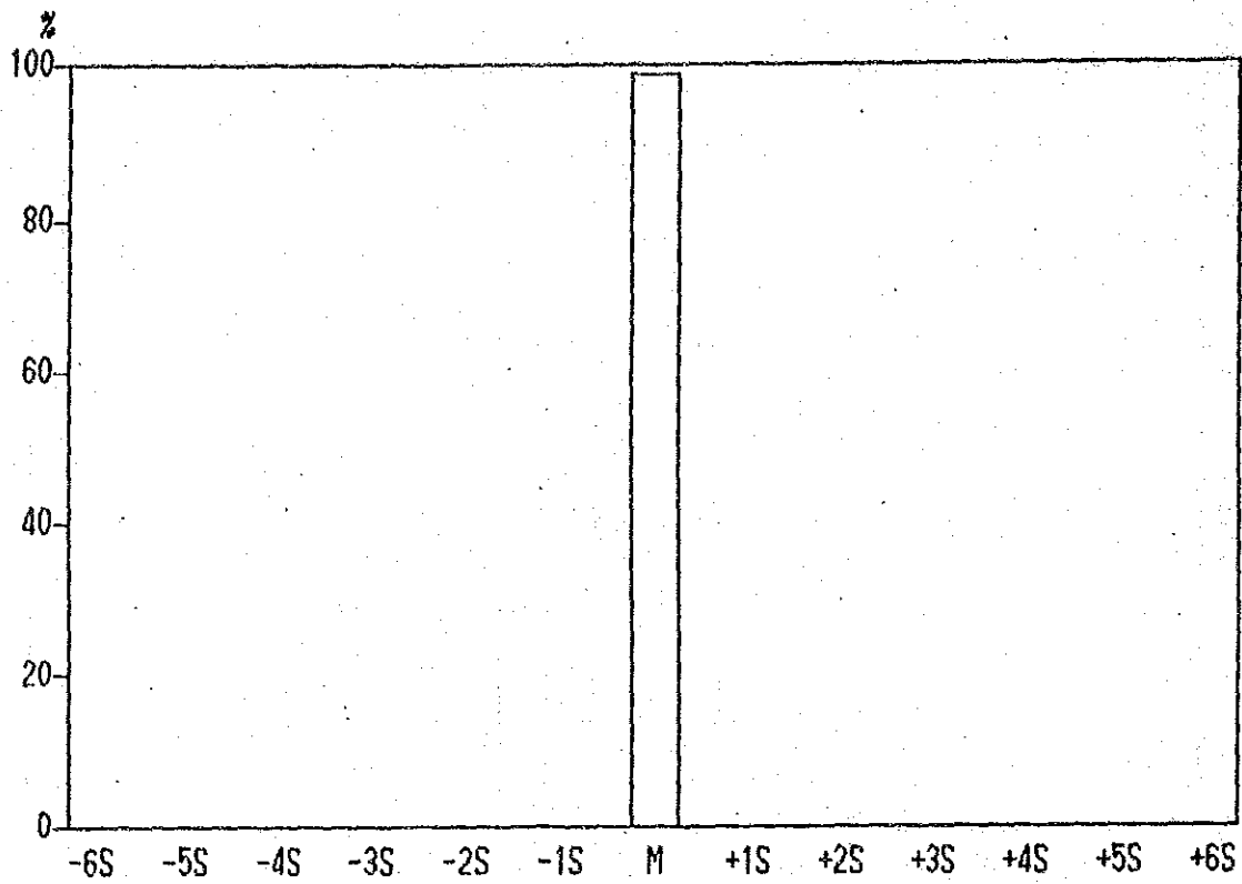
Histogram of Hg contents in Lithological Code; N2L
