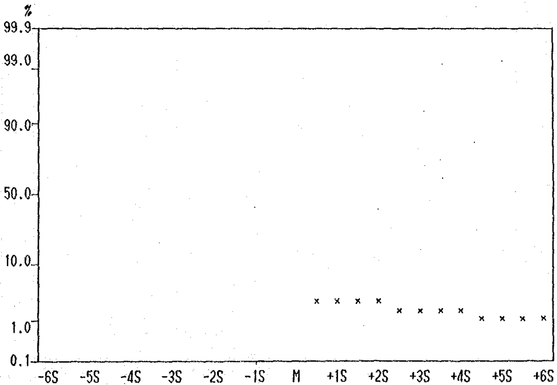
Cumulative Frequency Curve of Ag contents in Lithological Code; KPA
