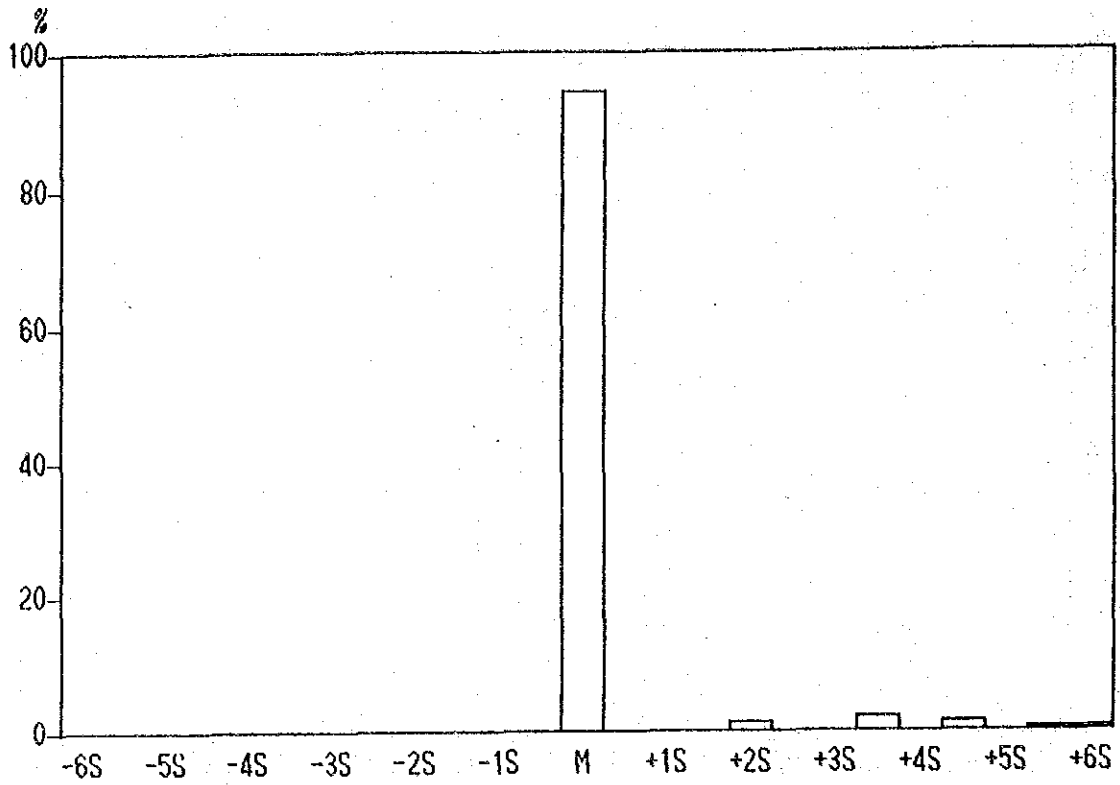
Histogram of Mo contents in Lithological Code; KPS
