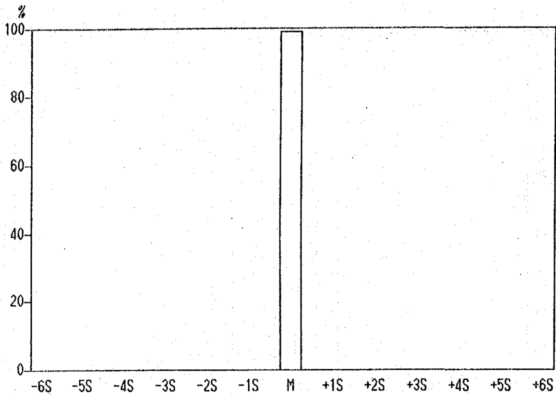
Histogram of Hg contents in Lithological Code; KPB
