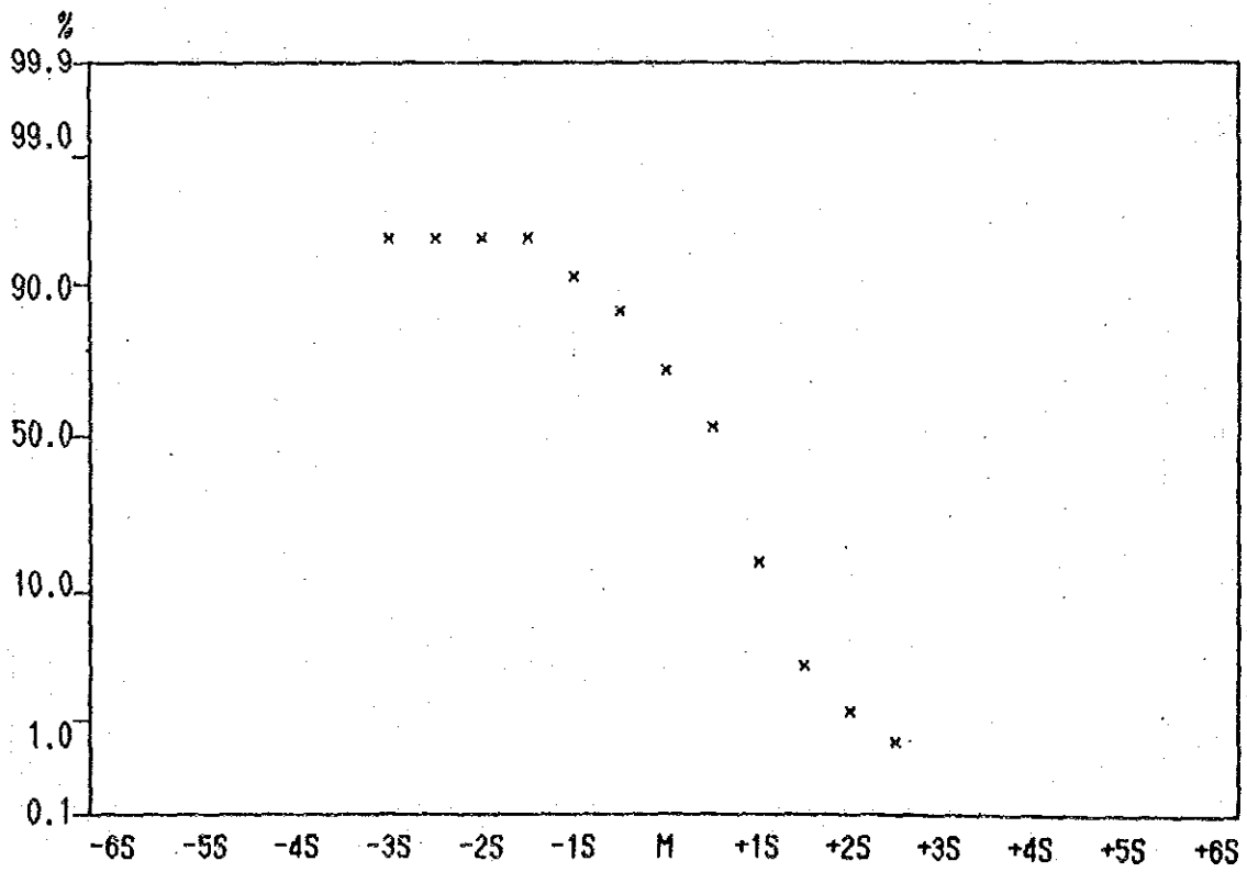
Cumulative Frequency Curve of Mn contents in Lithological Code; N2L
