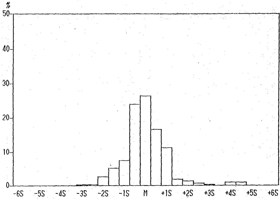
Histogram of Zn contents in Lithological Code; KPA
