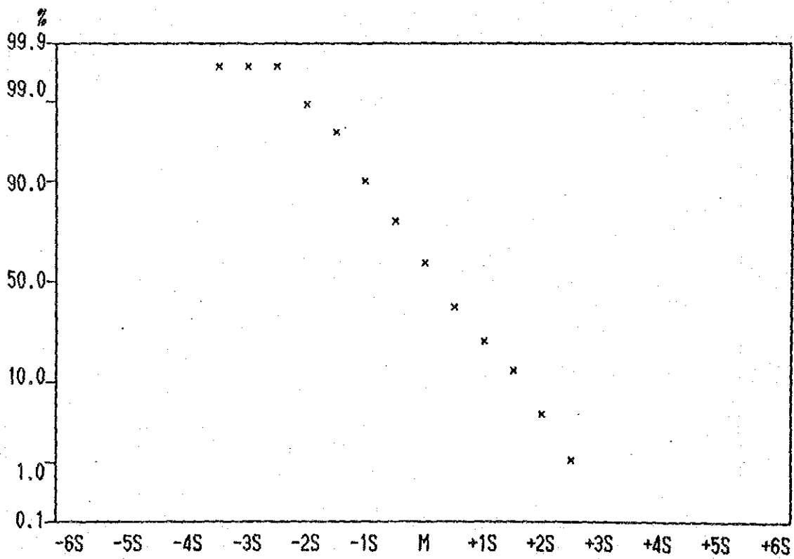
Cumulative Frequency Curve of Zn contents in Lithological Code; N2S
