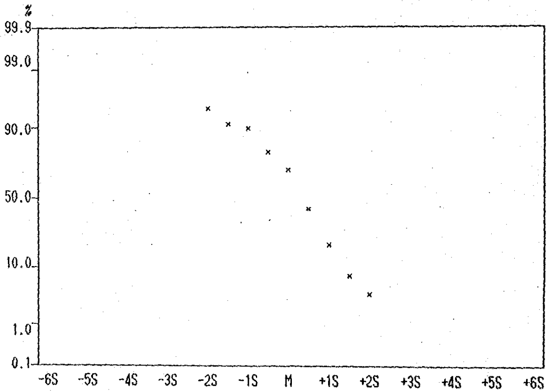
Cumulative Frequency Curve of Zn contents in Lithological Code; N2A
