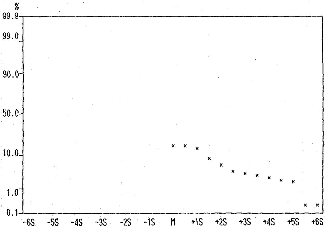
Cumulative Frequency Curve of Pb contents in Lithological Code; KPA
