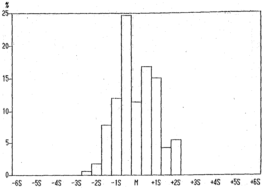
Histogram of Ni contents in Lithological Code; N2L
