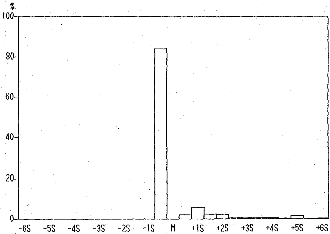
Histogram of Pb contents in Lithological Code; KPA
