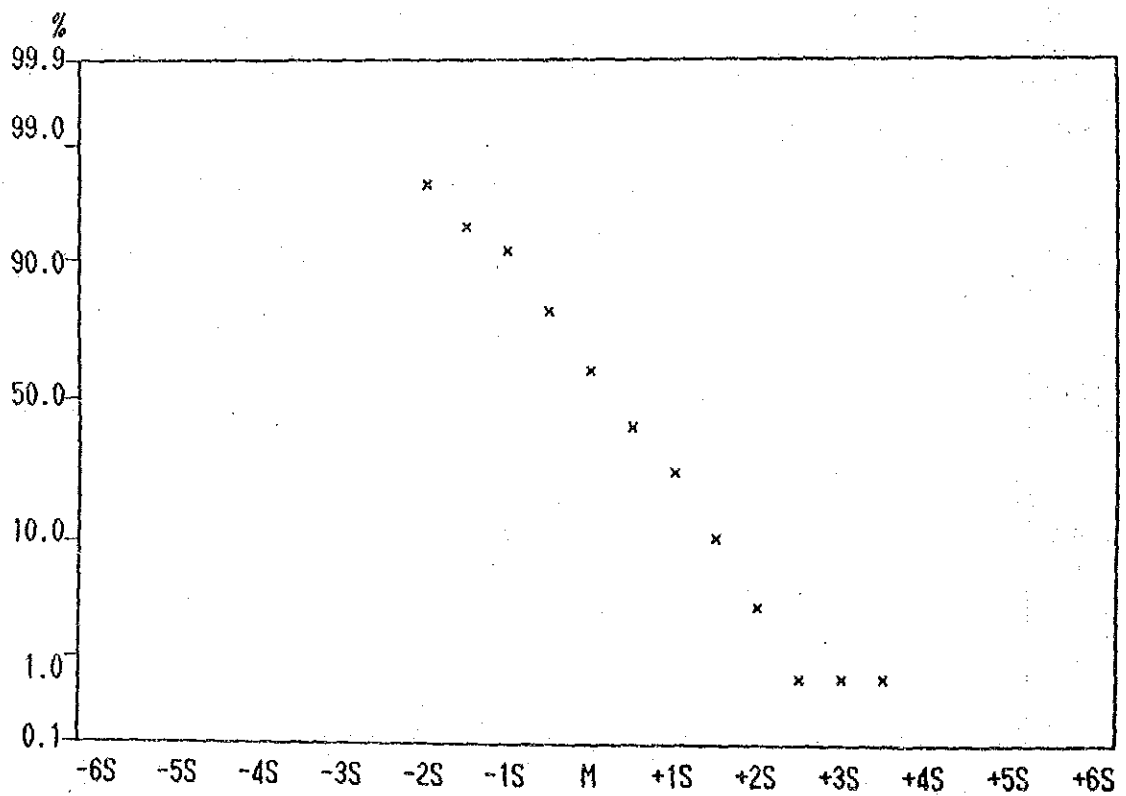
Cumulative Frequency Curve of Mn contents in Lithological Code; NQS
