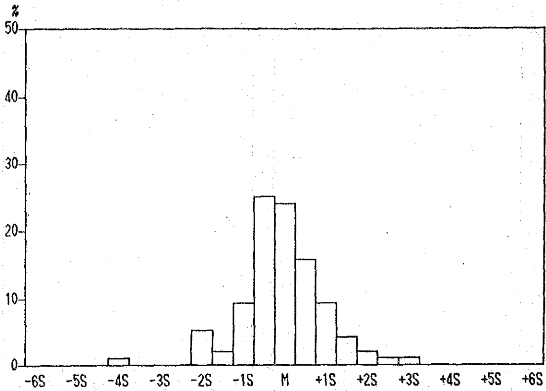
Histogram of Ni contents in Lithological Code; N1S
