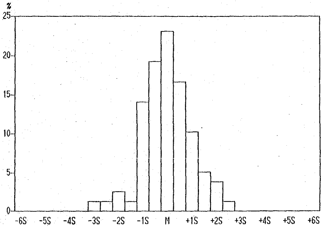
Histogram of Co contents in Lithological Code; N2A
