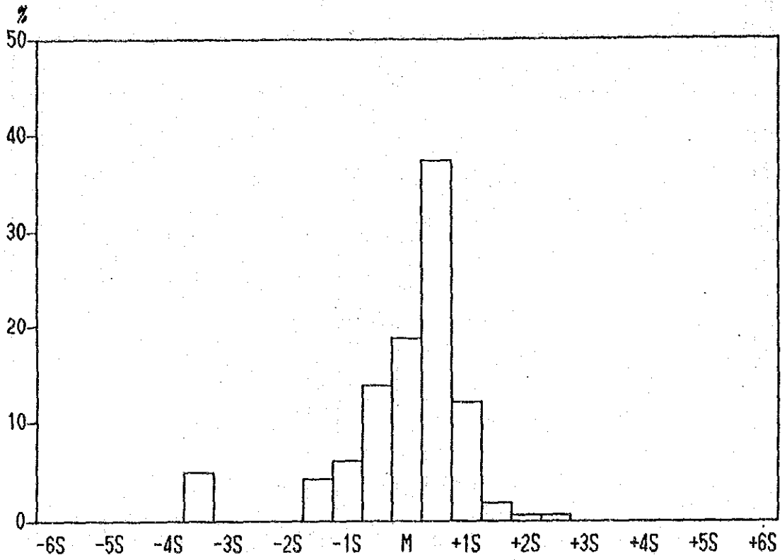
Histogram of Mn contents in Lithological Code; N2L
