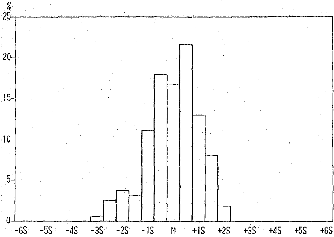
Histogram of Cu contents in Lithological Code; NQS
