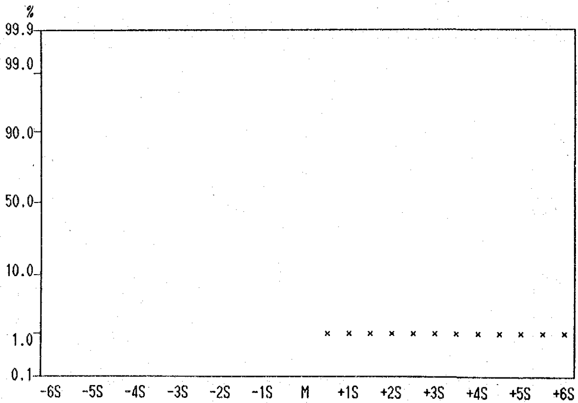
Cumulative Frequency Curve of Hg contents in Lithological Code; KPB
