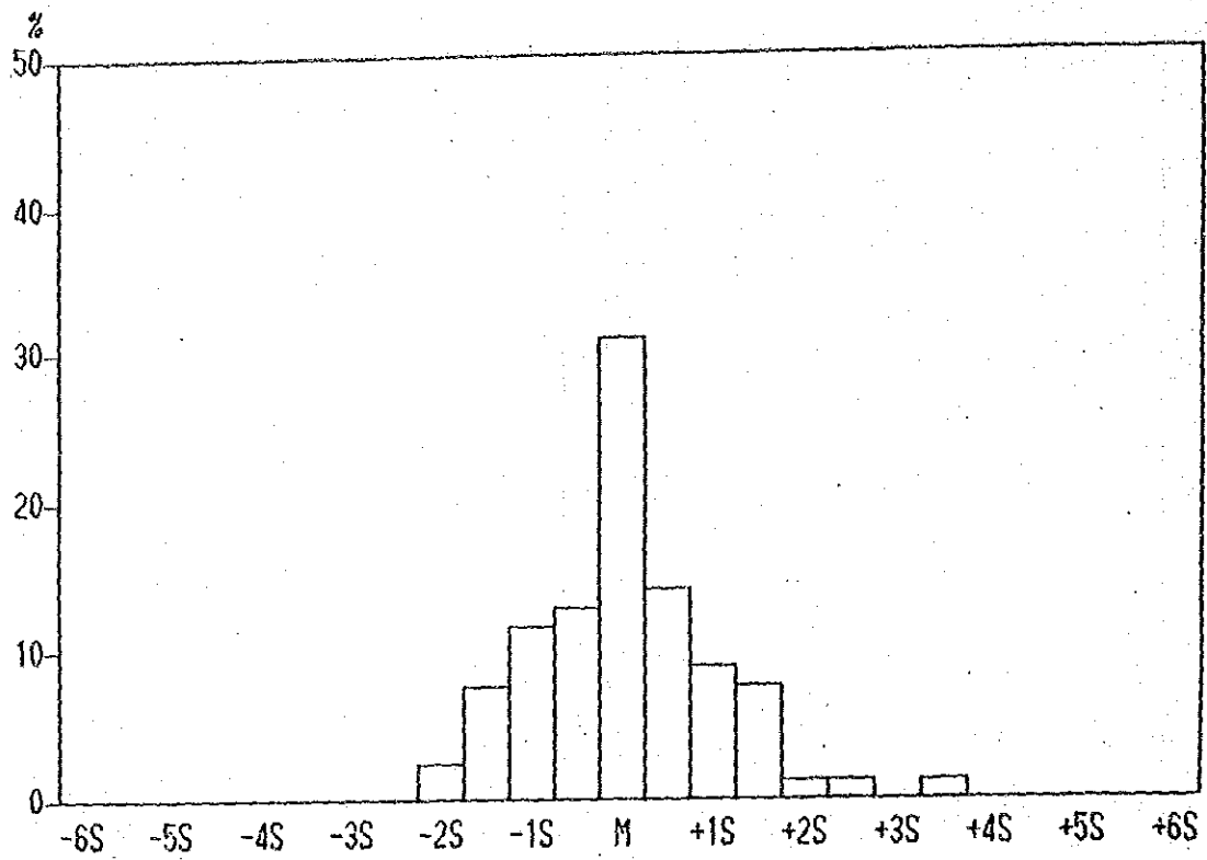
Histogram of Ni contents in Lithological Code; N2A
