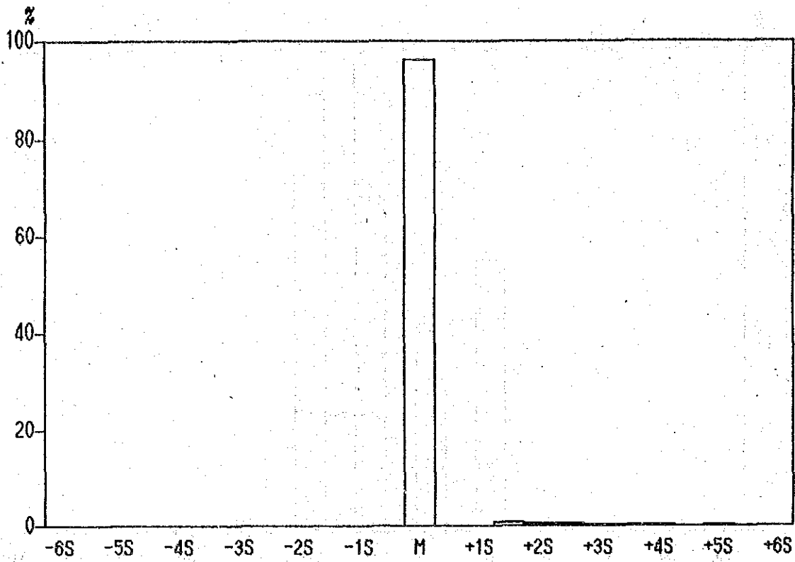
Histograms of Hg content in all Samples.
