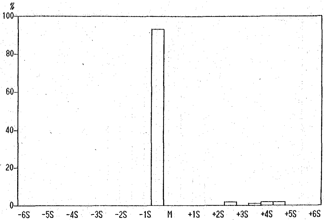
Histogram of Pb contents in Lithological Code; INR
