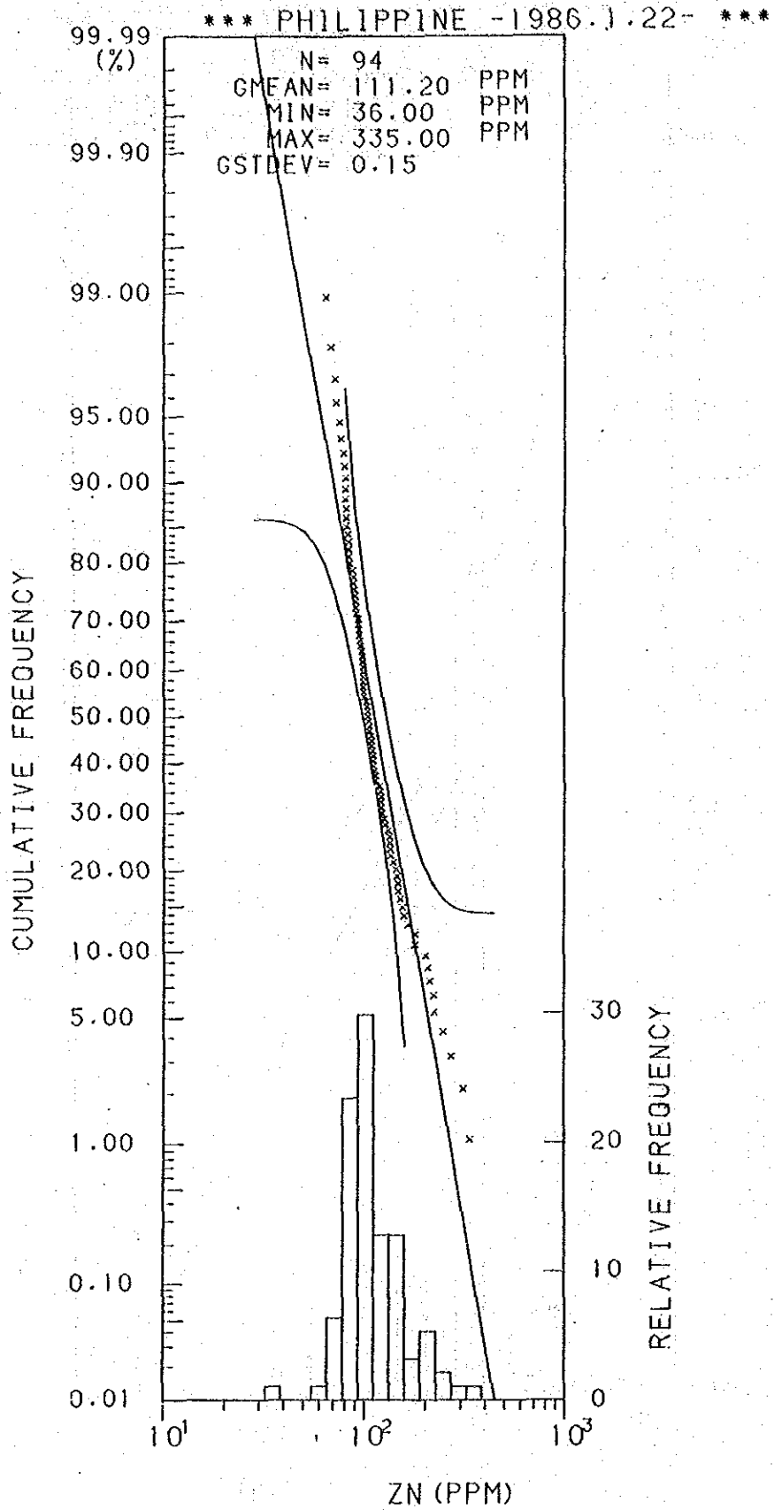
Histogram and Cumulative Frequency Curve of Zn Content in Lithological Code; 0.5.
