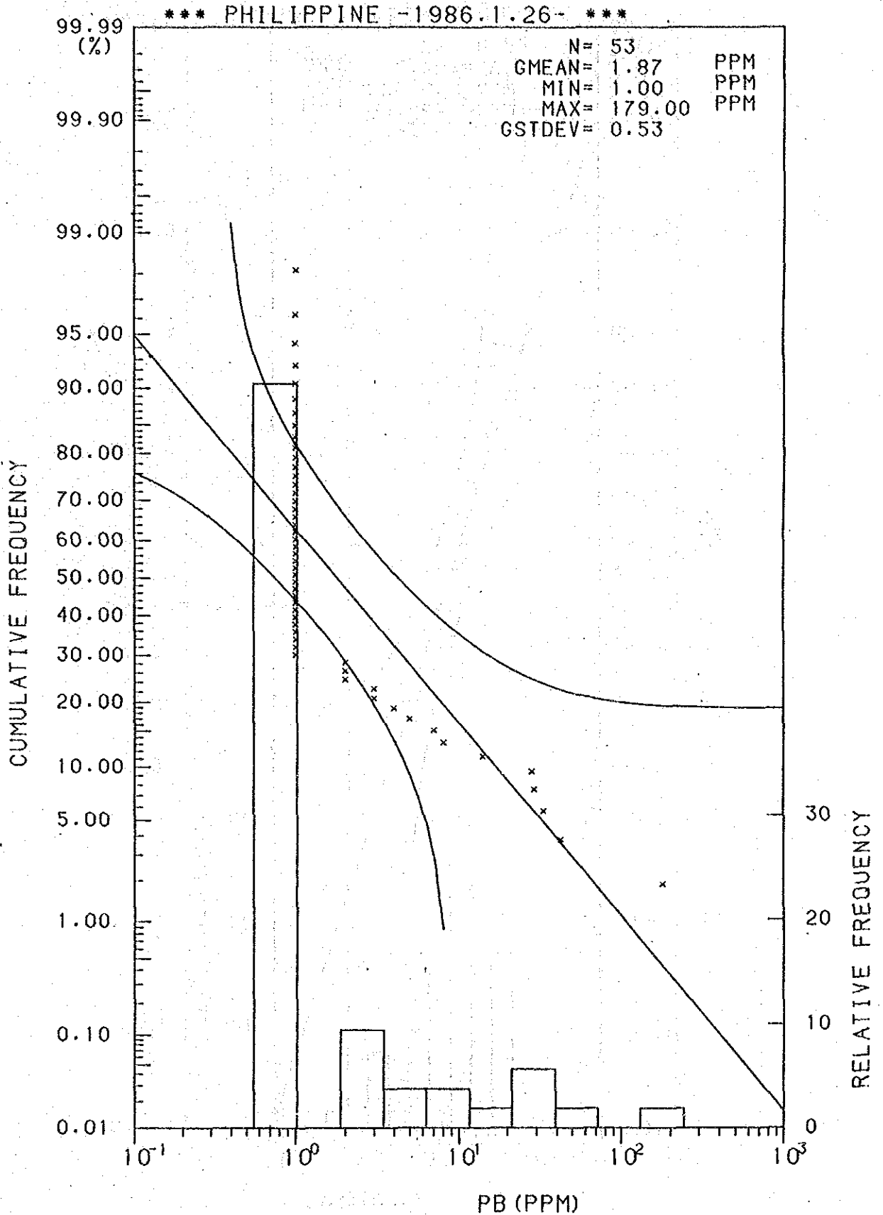
Histogram and Cumulative Frequency Curve of Pb content in Lithological Code; 0.9.
