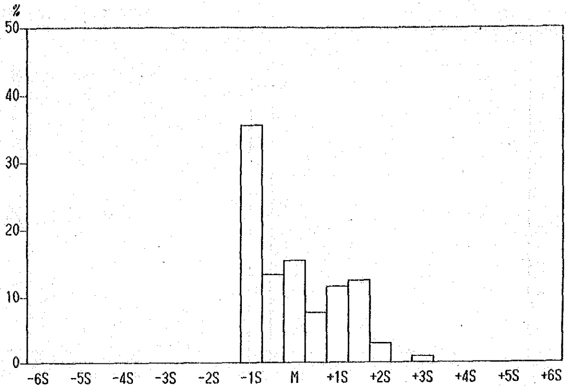
Histogram of As contents in Lithological Code; INR
