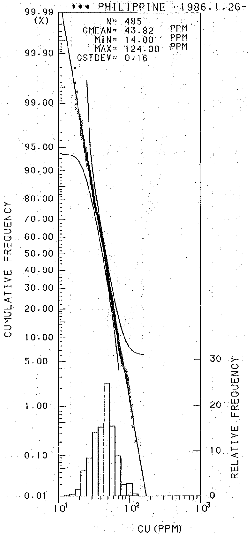
Histogram and Cumulative Frequency Curve of Cu content in Lithological Code; 0.1.
