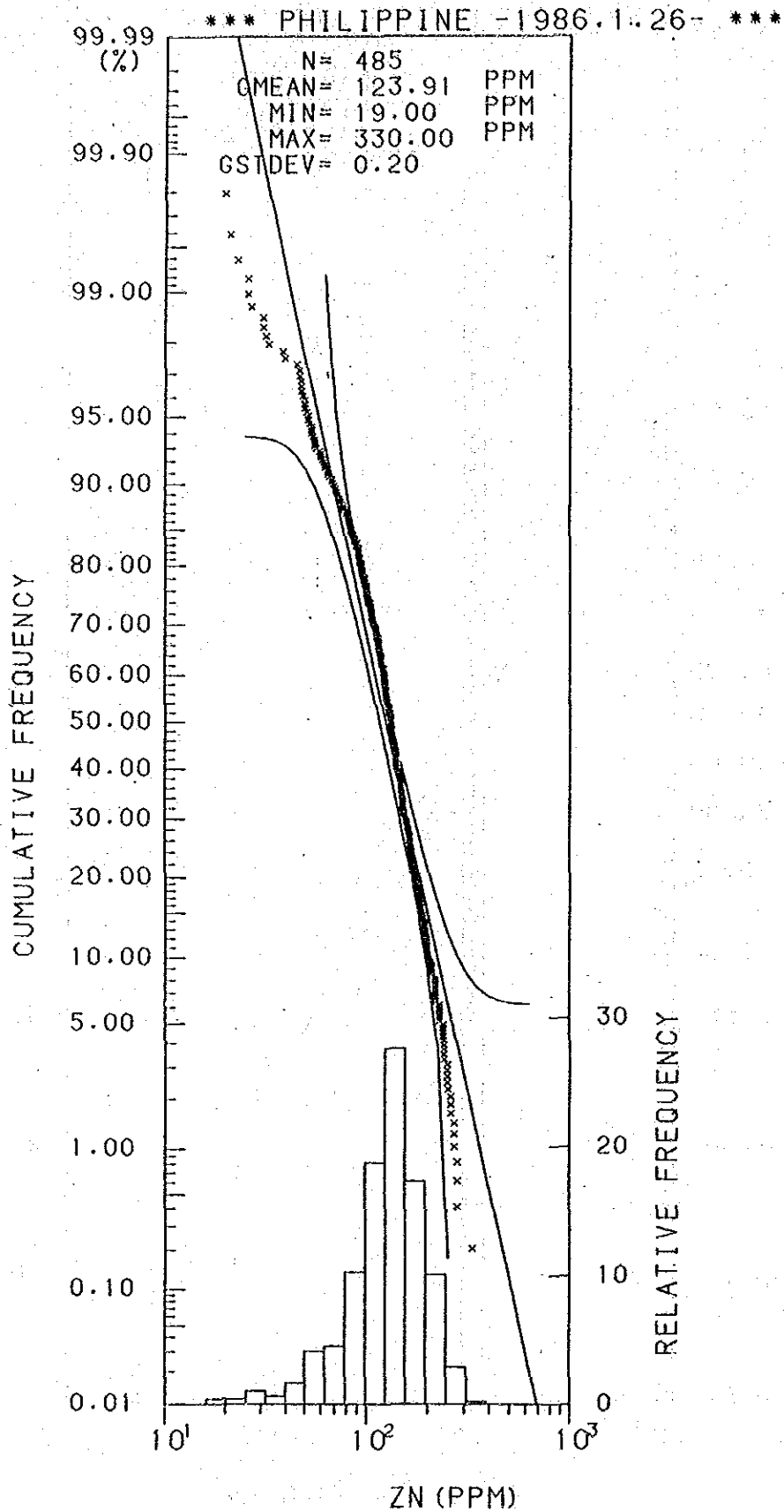
Histogram and Cumulative Frequency Curve of Zn content in Lithological Code; 0.1.
