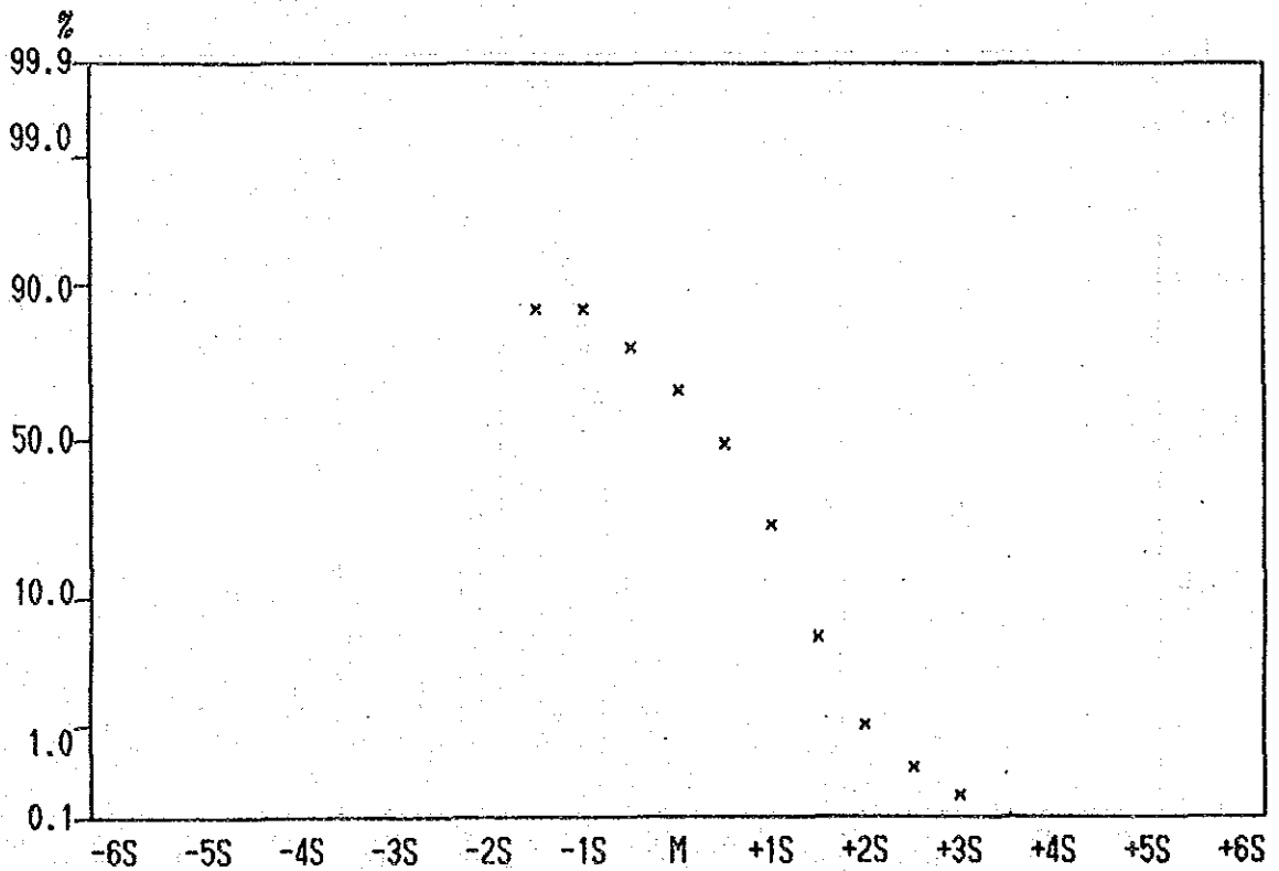
Cumulative Frequency Curve of As content in all Samples.
