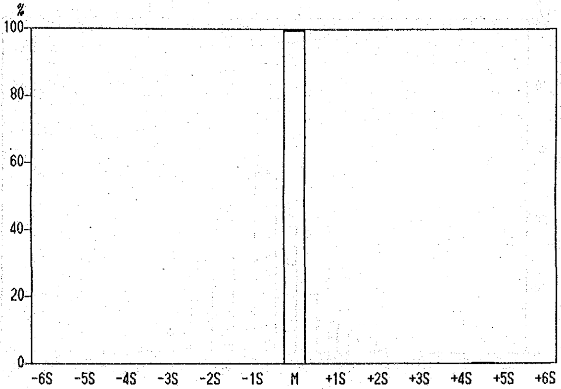
Histograms of Ag content in all Samples.
