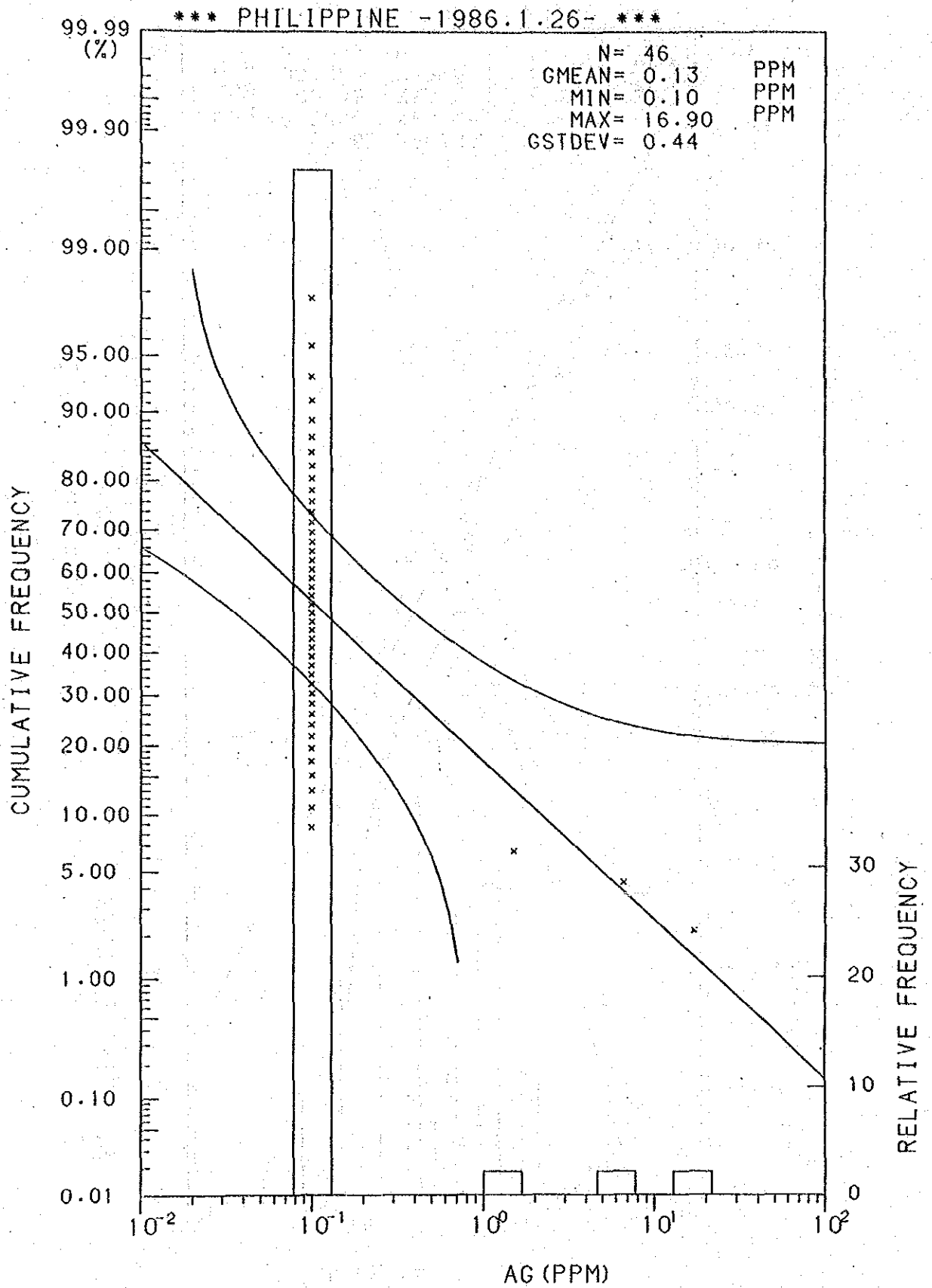
Histogram and Cumulative Frequency Curve of AG content in Lithological Code; 0.6.
