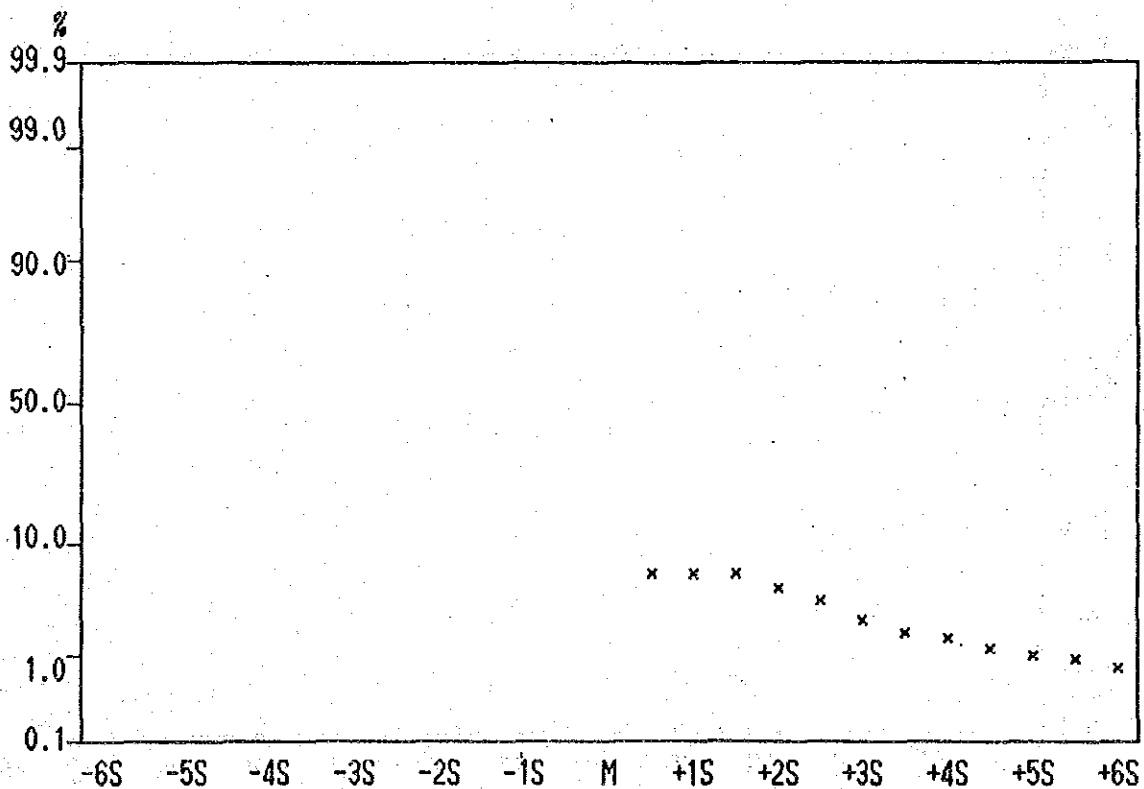
Cumulative Frequency Curve of Pb content in all Samples.
