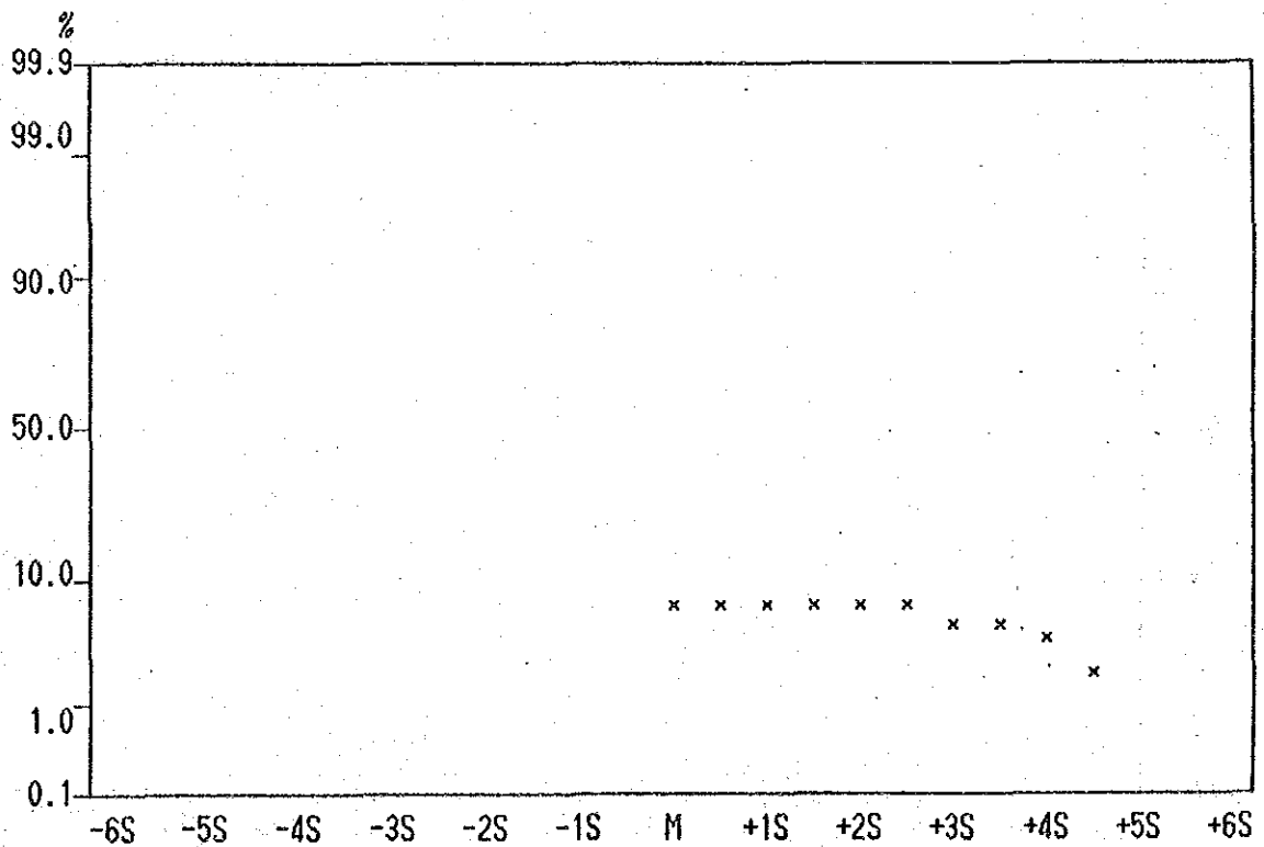
Cumulative Frequency Curve of Pb contents in Lithological Code; INR
