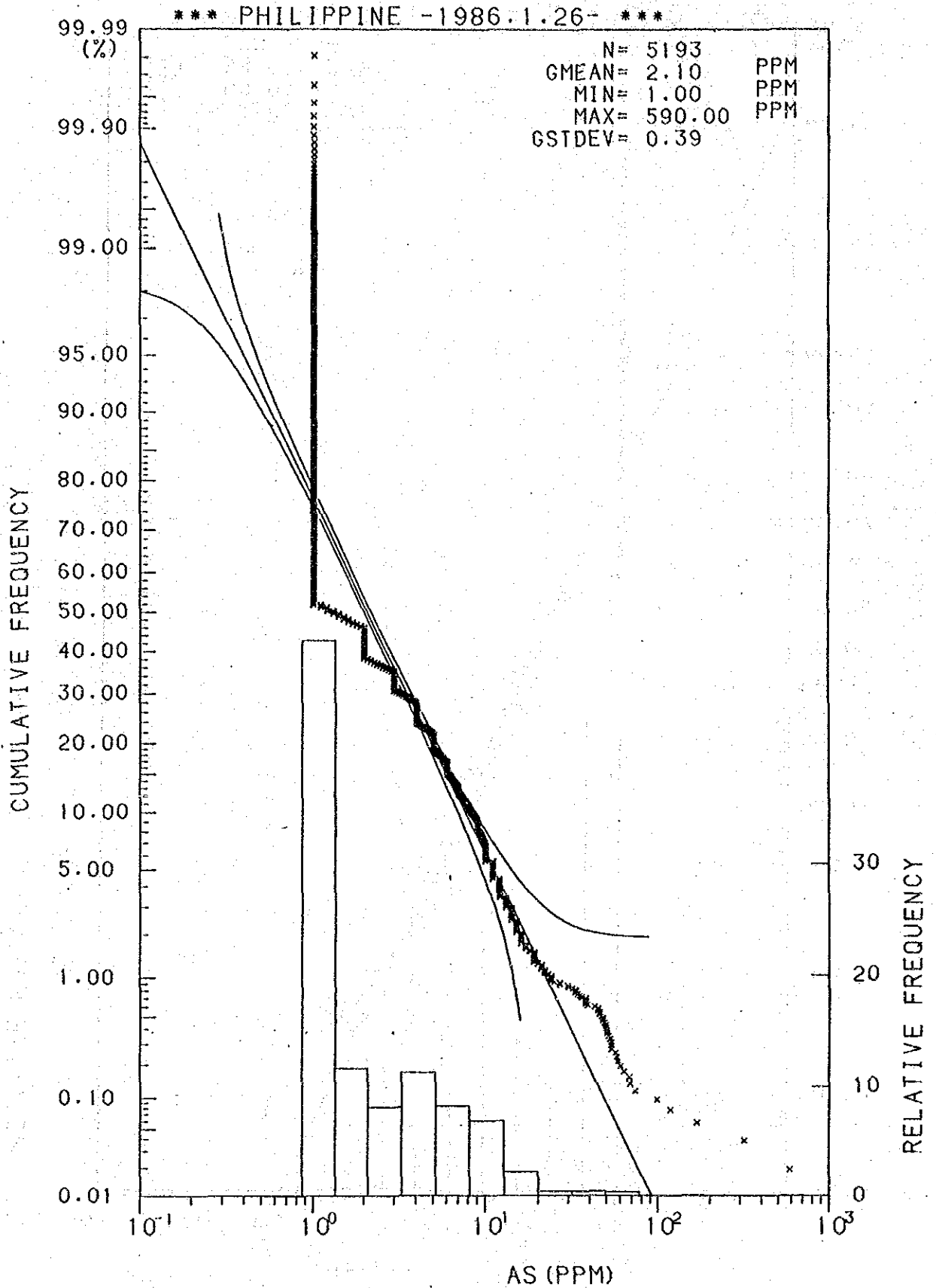
Histogram and Cumulative Frequency Curve of As content in All Samples.
