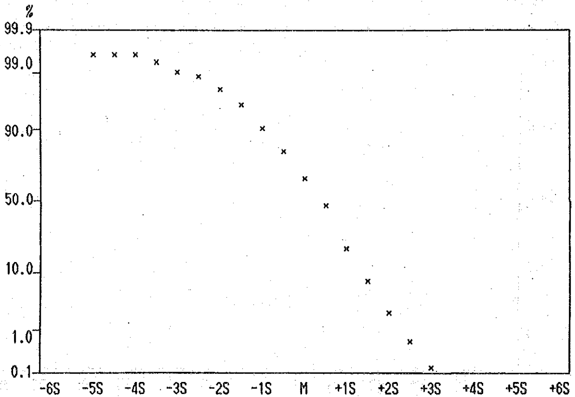
Cumulative Frequency Curve of Co content in all Samples.
