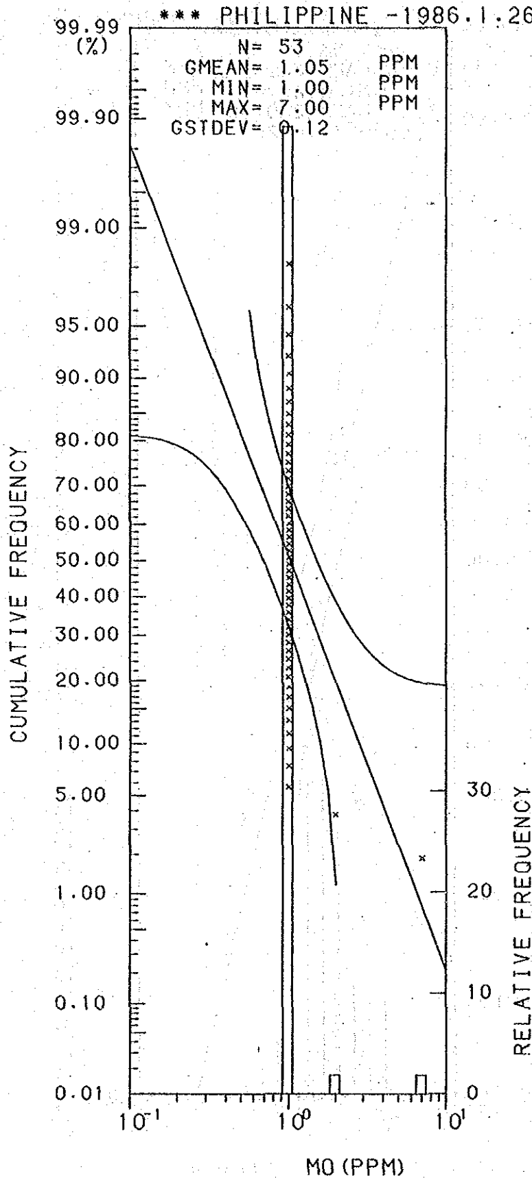
Histogram and Cumulative Frequency Curve of Mo content in Lithological Code; 0.9.
