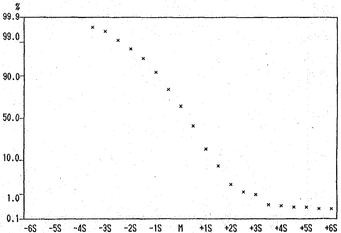
Cumulative Frequency Curve of Cu content in all Samples.
