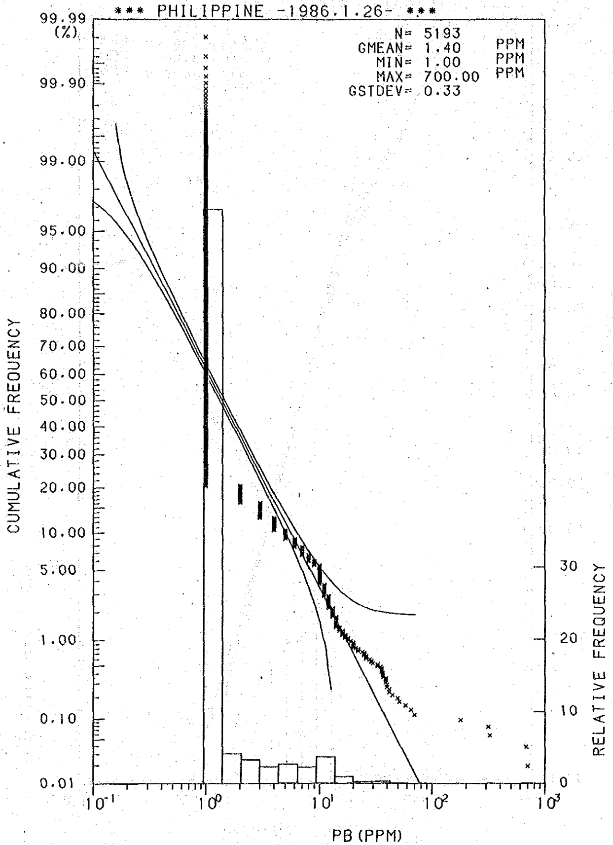
Histogram and Cumulative Frequency Curve of Pb content in All Samples.
