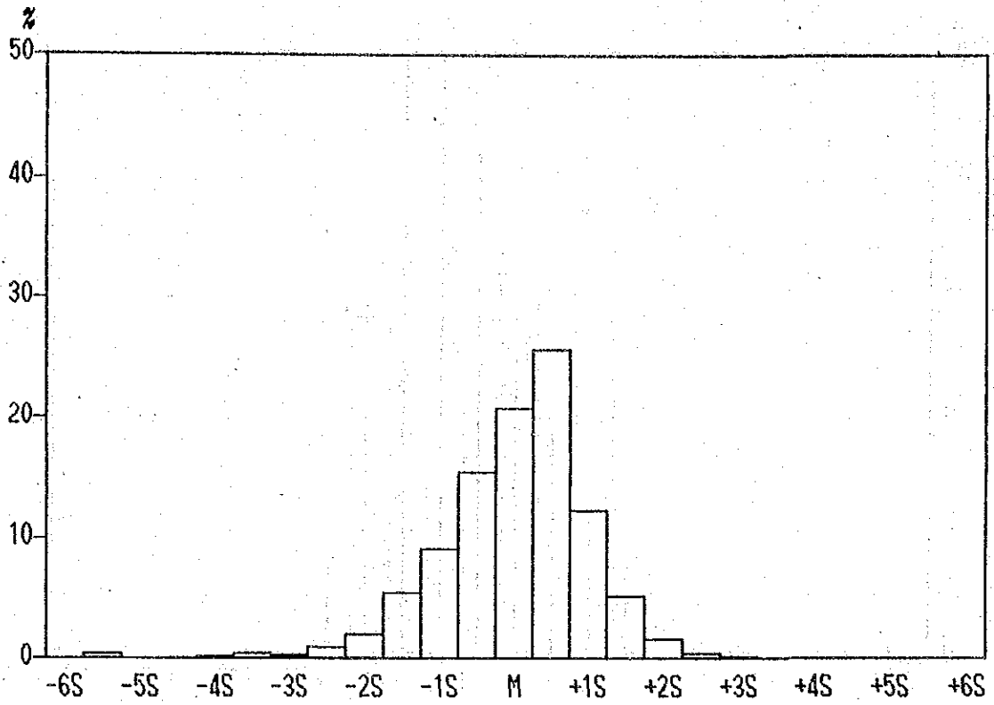
Histograms of Co content in all Samples.
