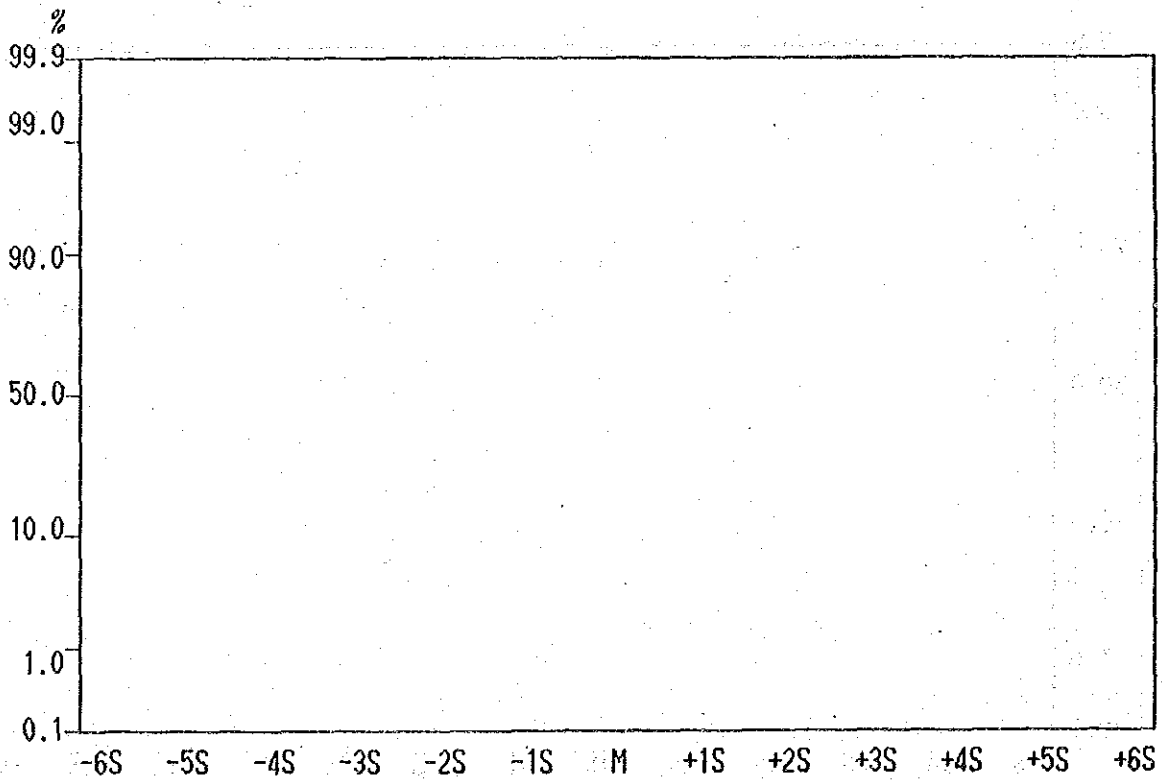
Cumulative Frequency Curve of Mo contents in Lithological Code; KPL
