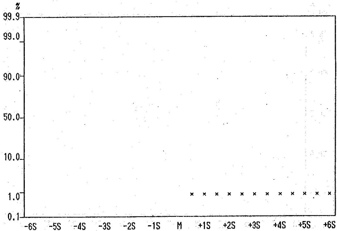
Cumulative Frequency Curve of Hg contents in Lithological Code; N2S
