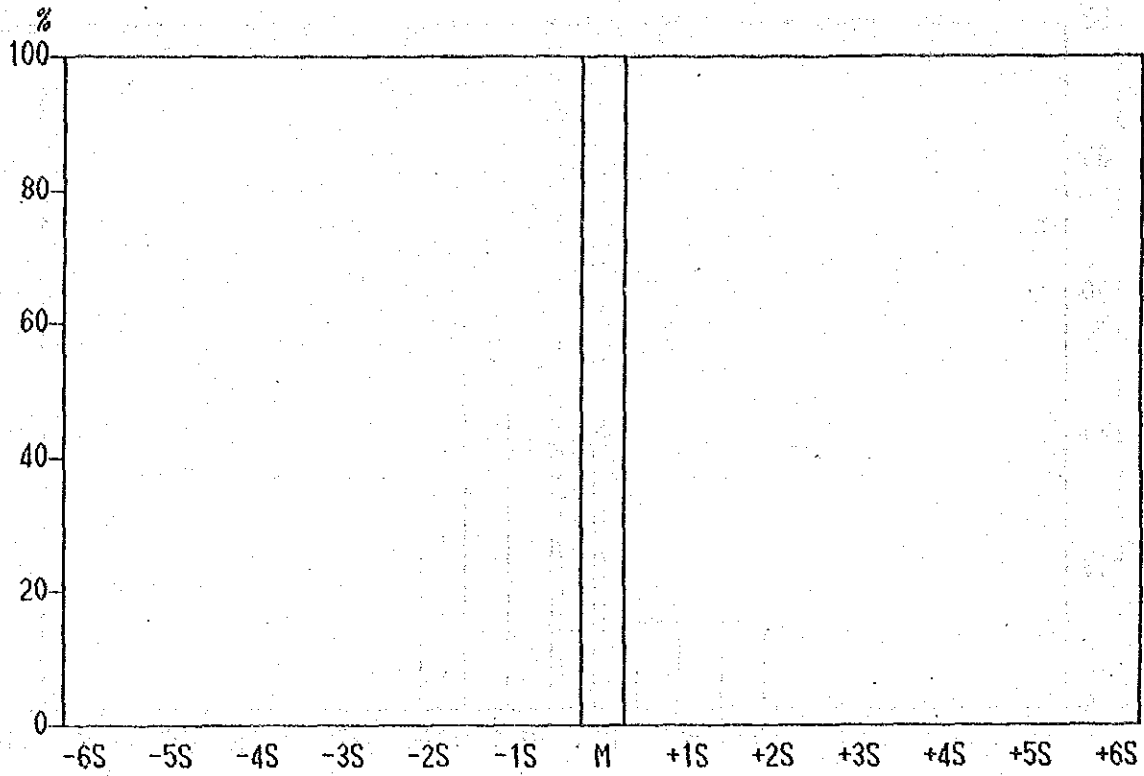
Histogram of Mo contents in Lithological Code; KPL
