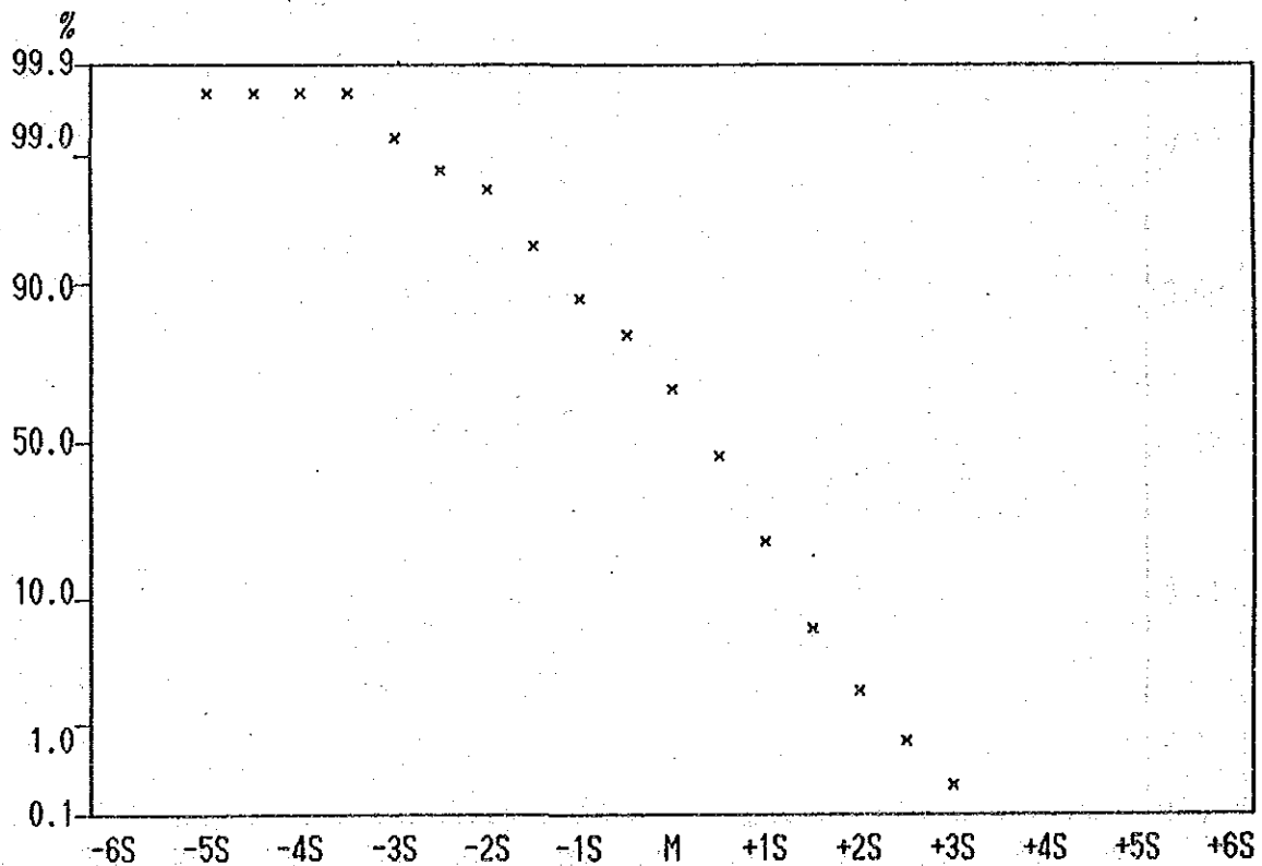
Cumulative Frequency Curve of Mn contents in Lithological Code; KPA
