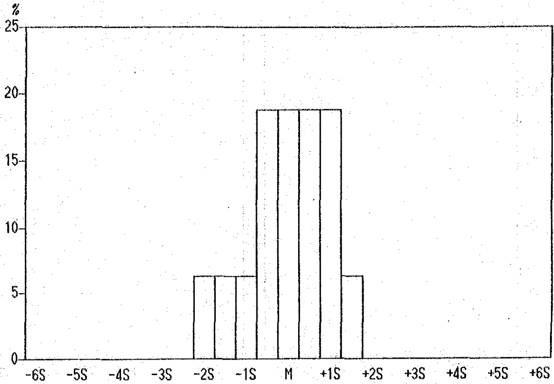
Histogram of As contents in Lithological Code; KPL
