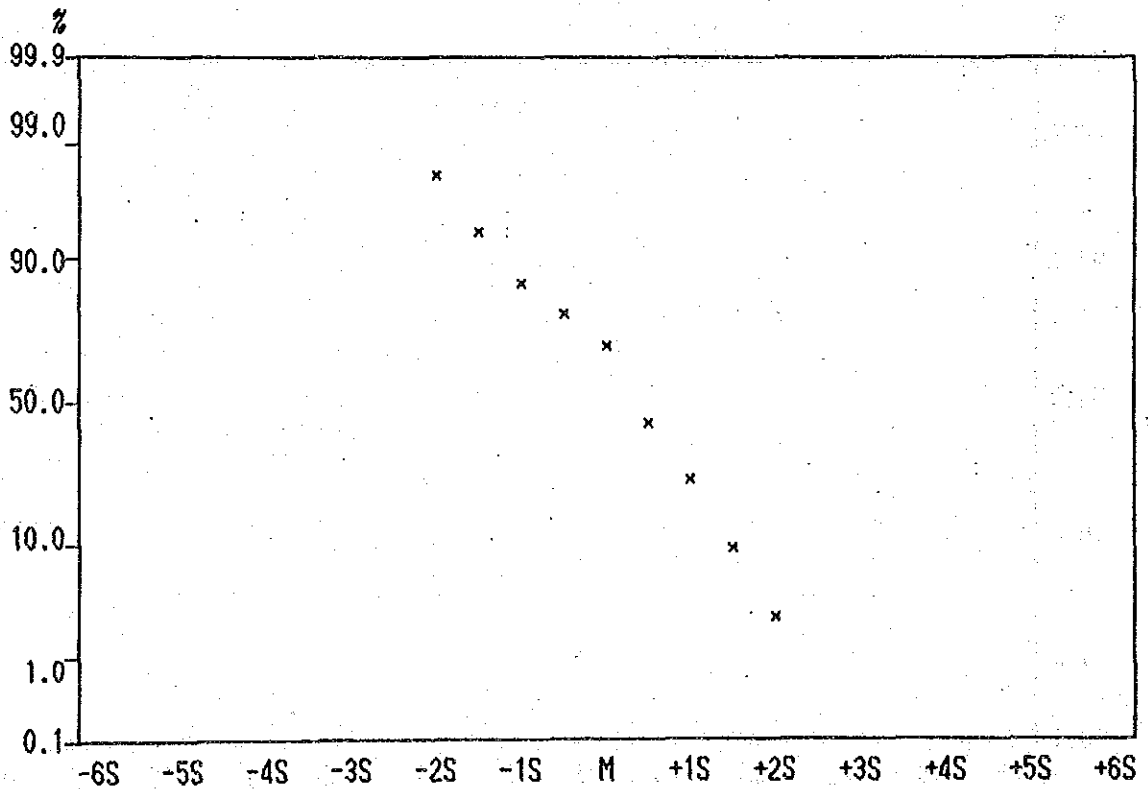
Cumulative Frequency Curve of Co contents in Lithological Code; N2S
