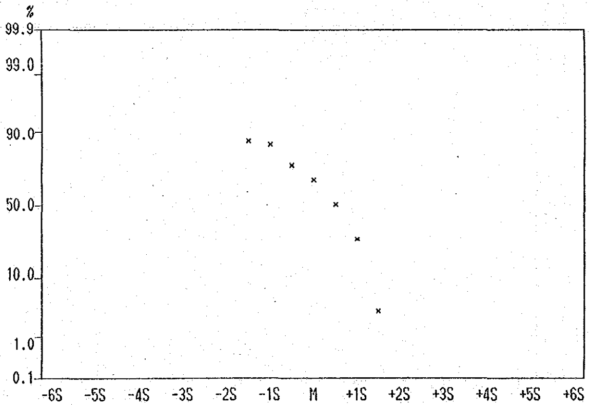
Cumulative Frequency Curve of As contents in Lithological Code; R
