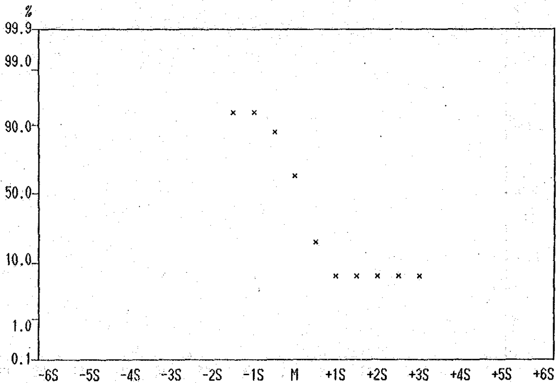
Cumulative Frequency Curve of Co contents in Lithological Code; KPL
