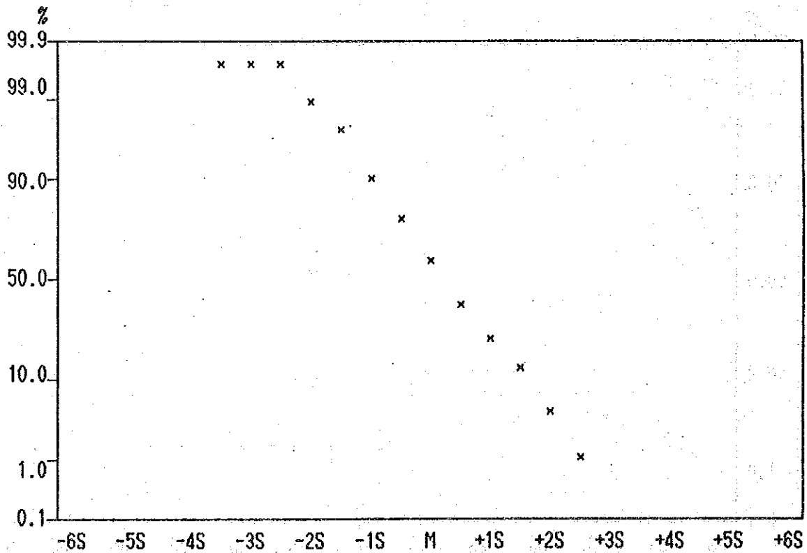
Cumulative Frequency Curve of Zn contents in Lithological Code; N2S
