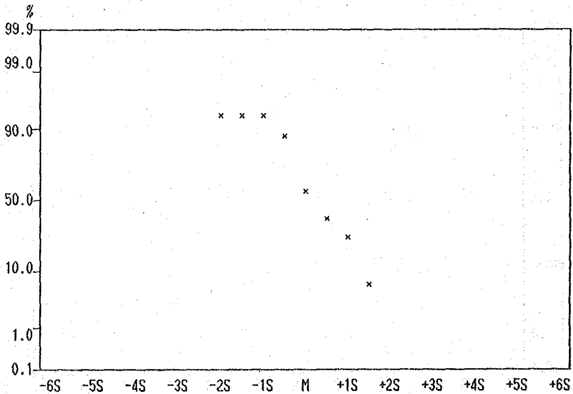
Cumulative Frequency Curve of Zn contents in Lithological Code; KPL
