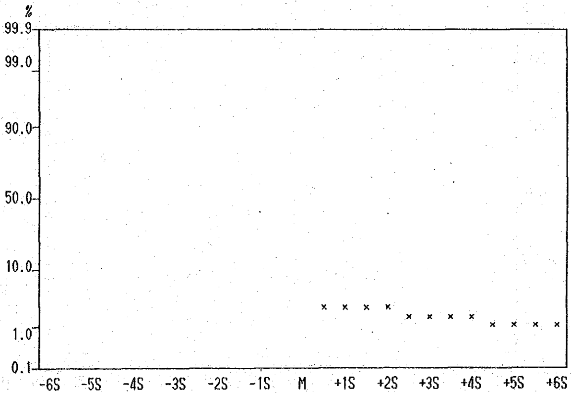
Cumulative Frequency Curve of Ag contents in Lithological Code; KPA
