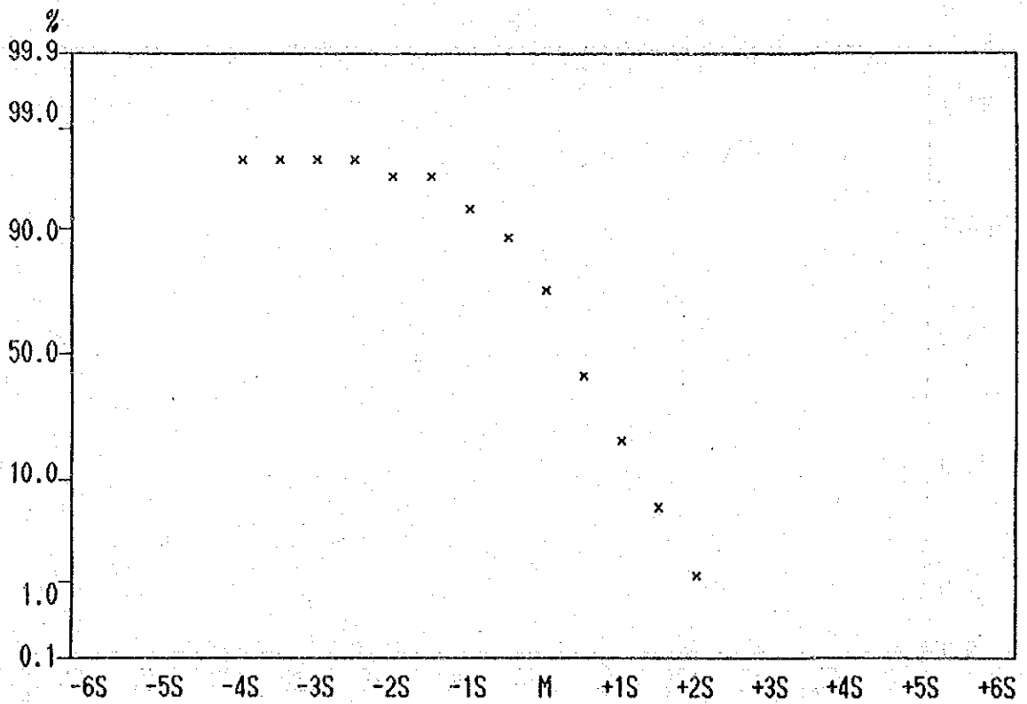
Cumulative Frequency Curve of Co contents in Lithological Code; NQL
