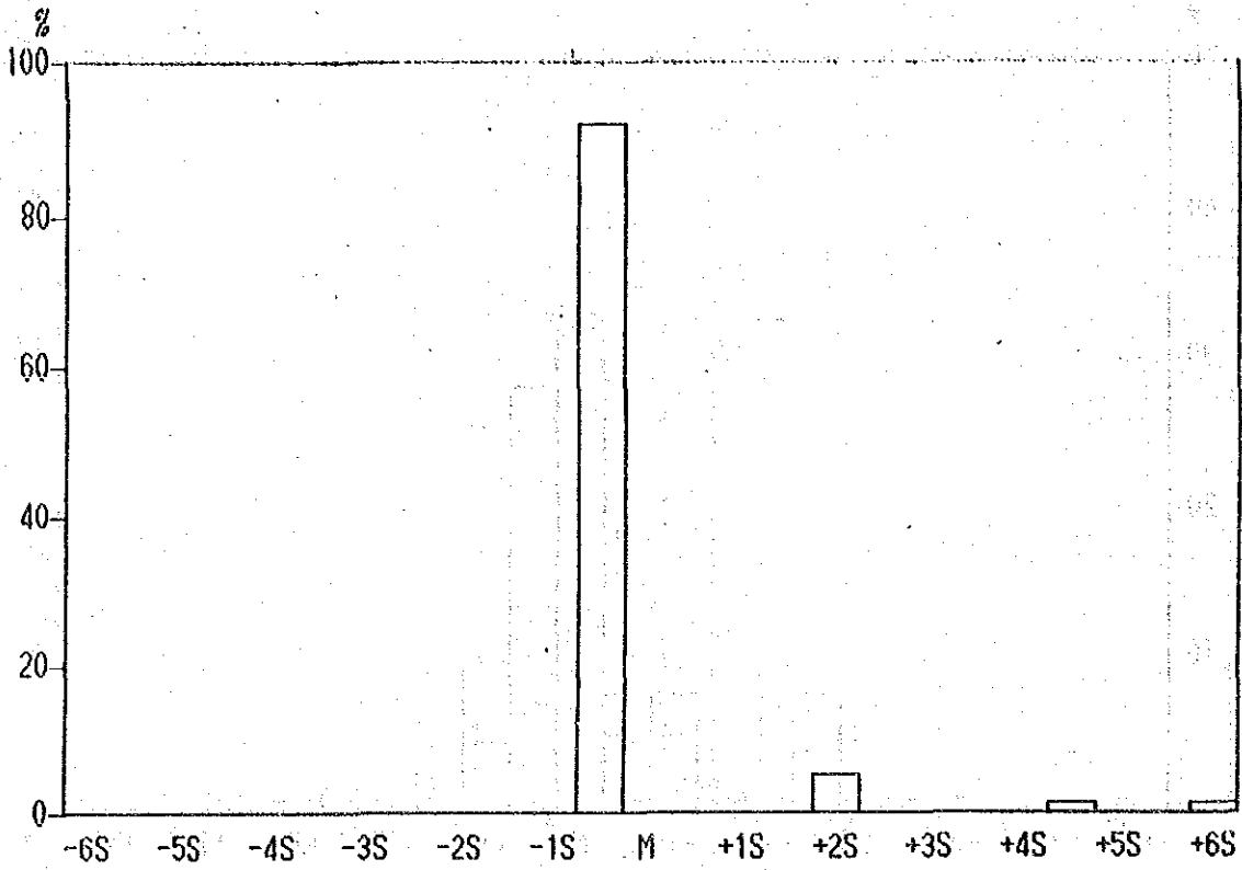
Histogram of Hg contents in Lithological Code; N2A
