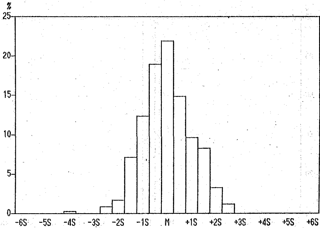
Histogram of Zn contents in Lithological Code; N2S
