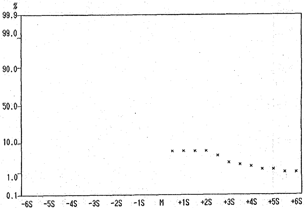
Cumulative Frequency Curve of Pb contents in Lithological Code; KPB
