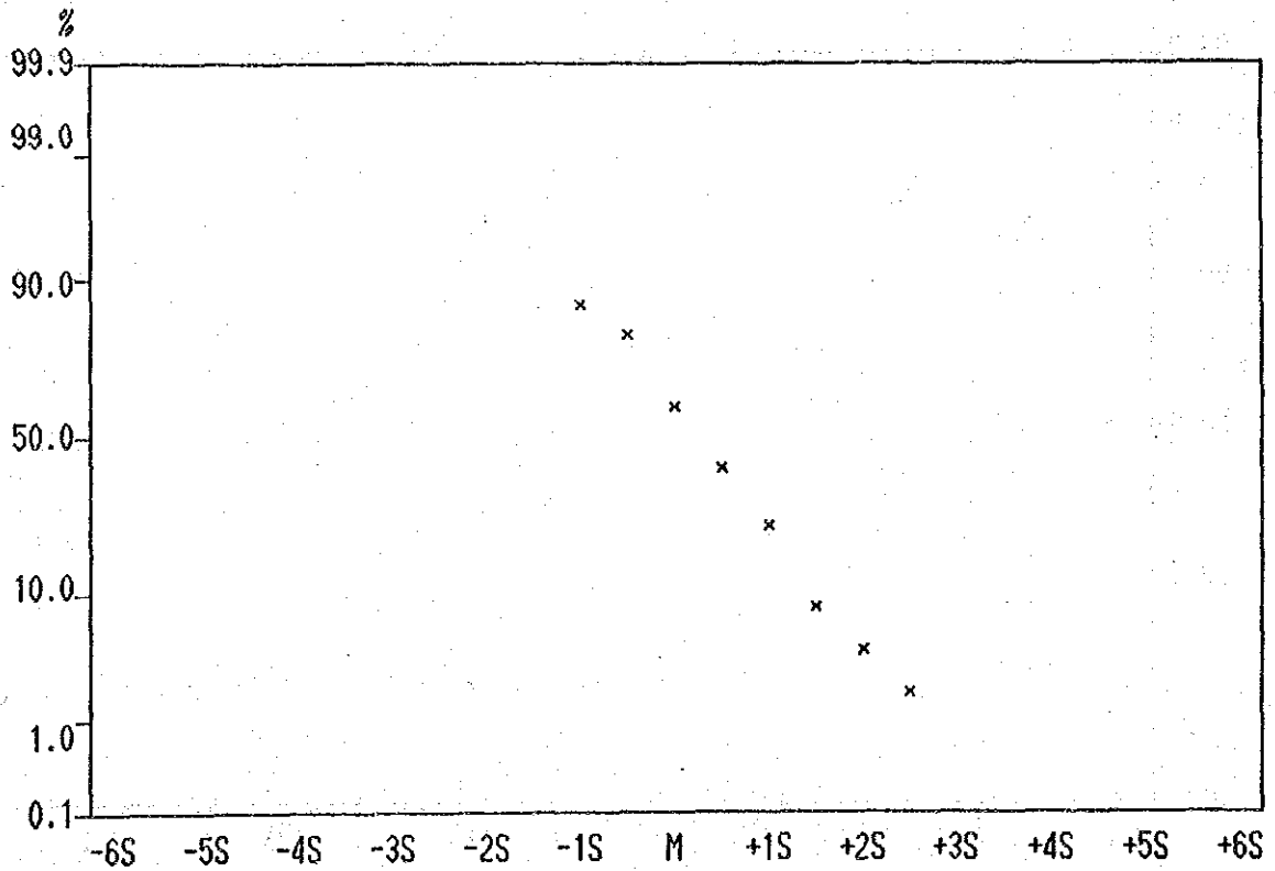
Cumulative Frequency Curve of As contents in Lithological Code; KPS
