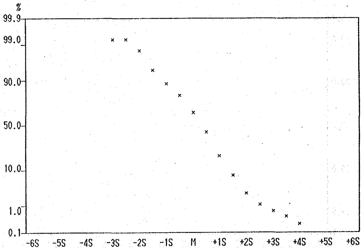
Cumulative Frequency Curve of Ni contents in Lithological Code; KPA
