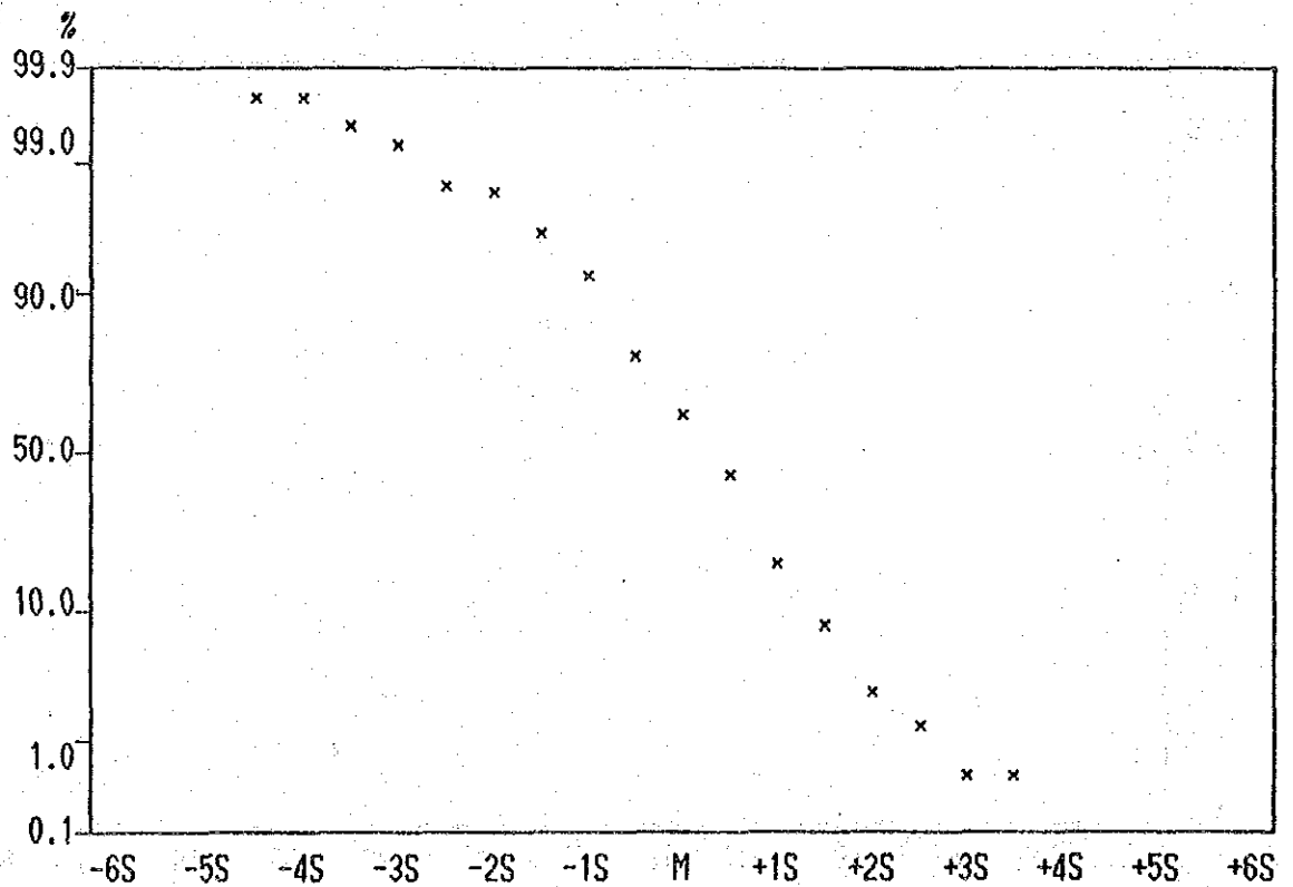
Cumulative Frequency Curve of Co contents in Lithological Code; KPA
