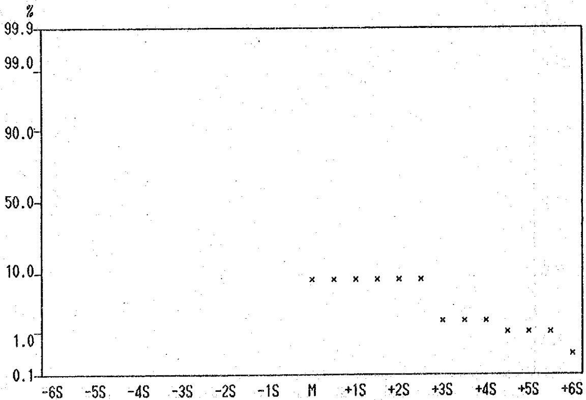
Cumulative Frequency Curve of Mo contents in Lithological Code; KPB
