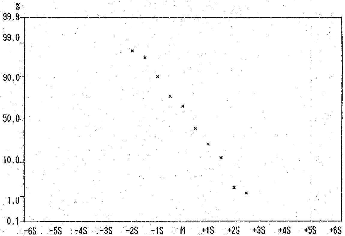
Cumulative Frequency Curve of Co contents in Lithological Code; NQS
