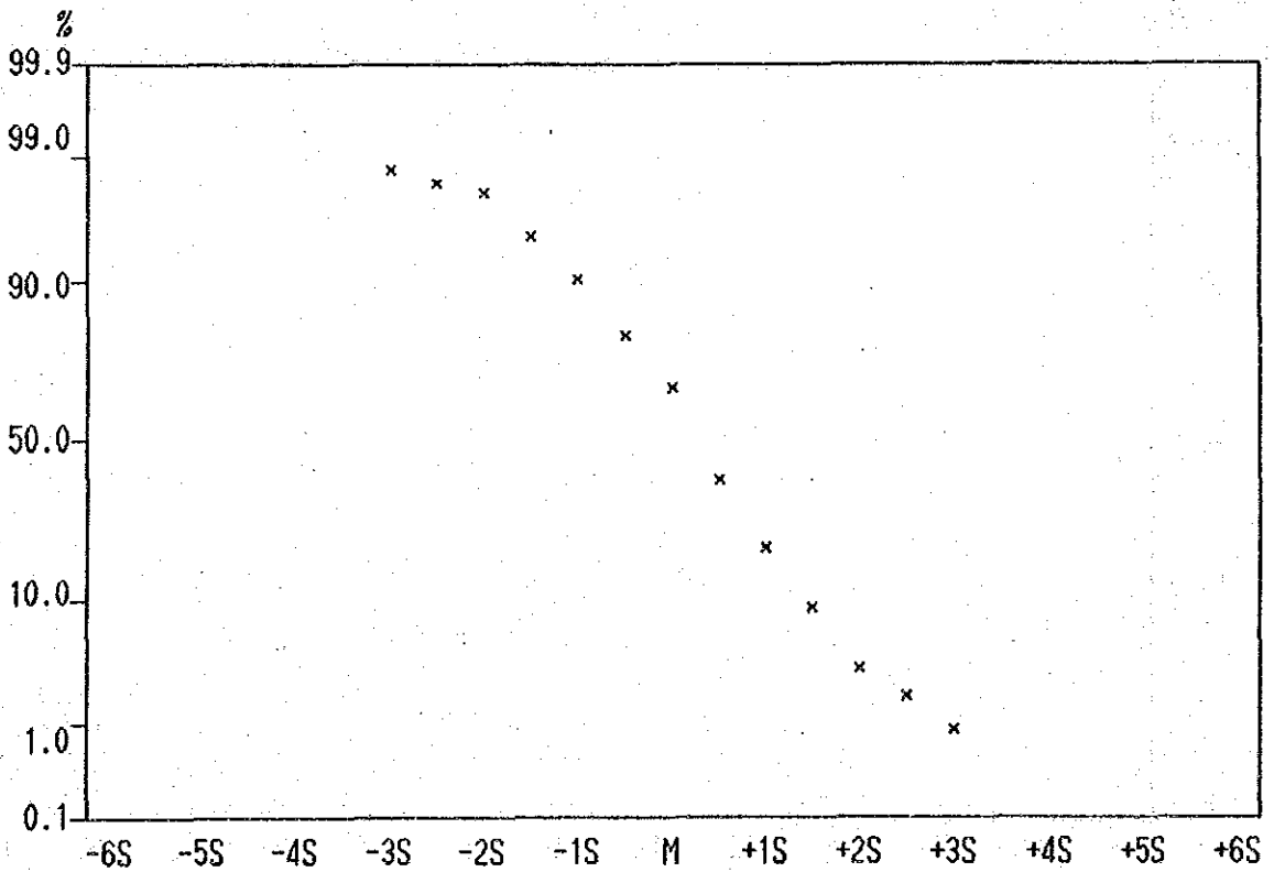
Cumulative Frequency Curve of Cu contents in Lithological Code; KPS
