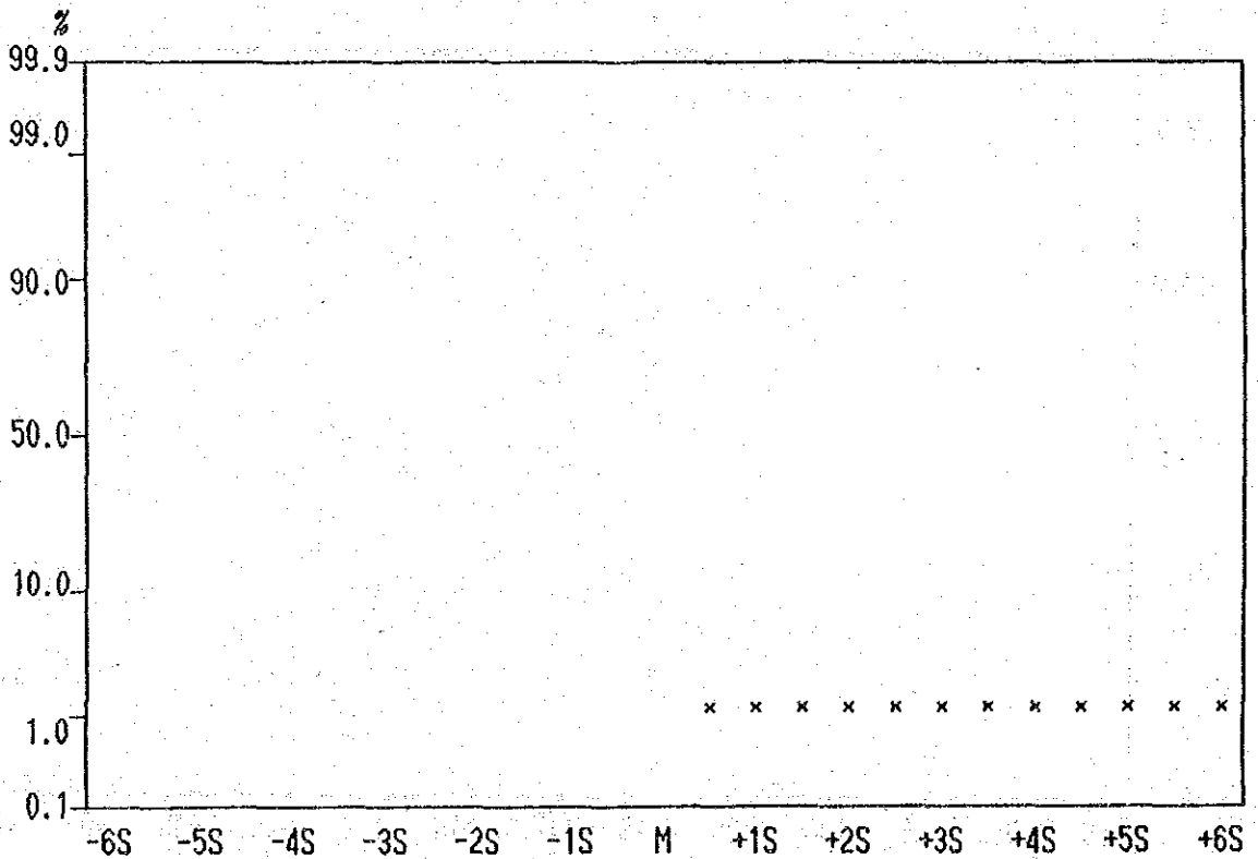
Cumulative Frequency Curve of Pb contents in Lithological Code; R
