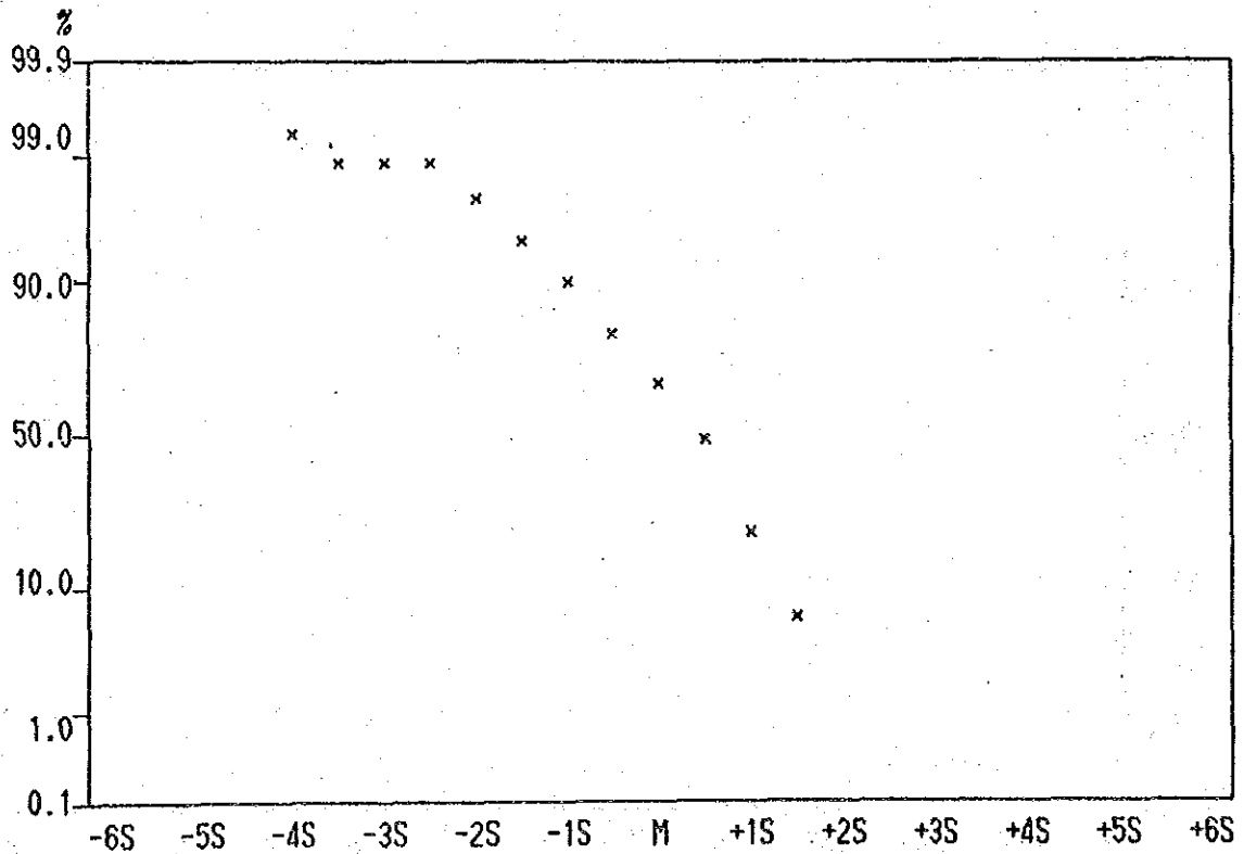
Cumulative Frequency Curve of As contents in Lithological Code; N2L
