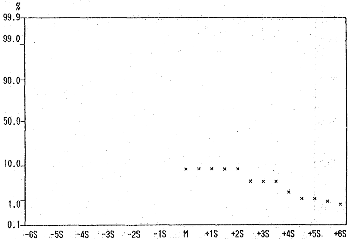
Cumulative Frequency Curve of Mo contents in Lithological Code; KPA
