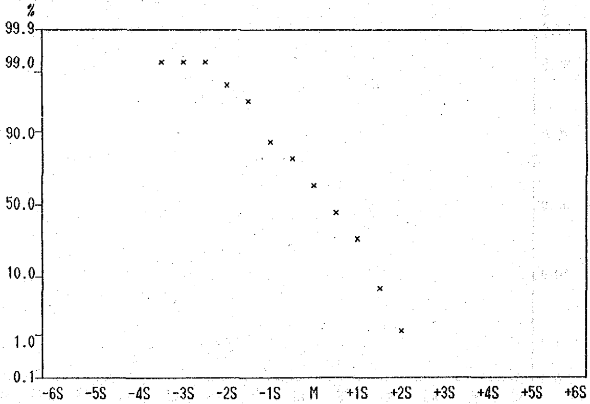
Cumulative Frequency Curve of Mn contents in Lithological Code; R
