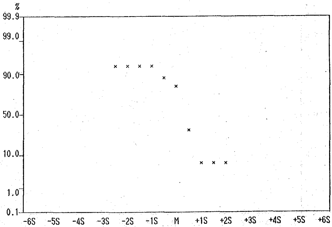
Cumulative Frequency Curve of Mn contents in Lithological Code; KPL
