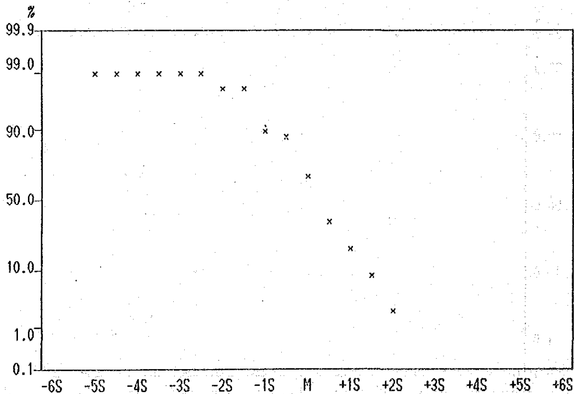
Cumulative Frequency Curve of Mn contents in Lithological Code; N1S
