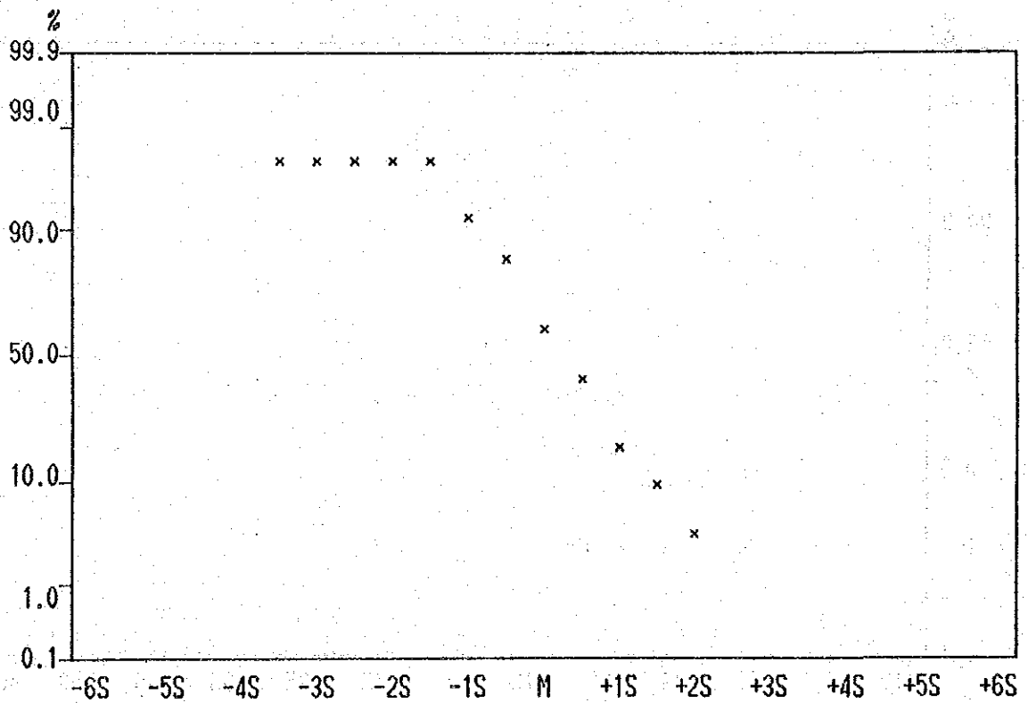
Cumulative Frequency Curve of Cu contents in Lithological Code; NQL
