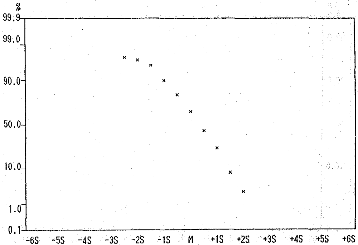
Cumulative Frequency Curve of Ni contents in Lithological Code; R
