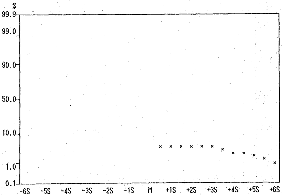
Cumulative Frequency Curve of Pb contents in Lithological Code; KPS
