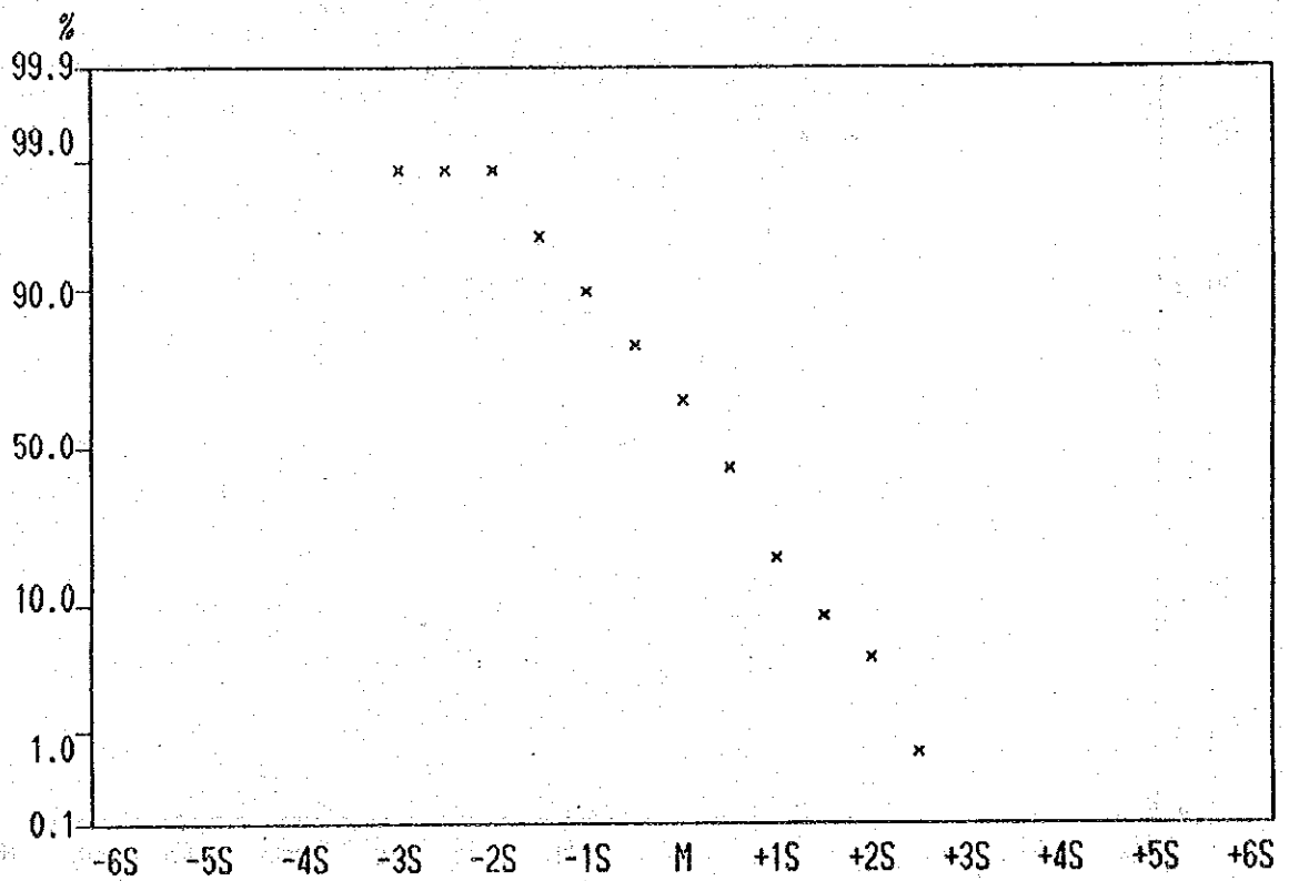
Cumulative Frequency Curve of Co contents in Lithological Code; R
