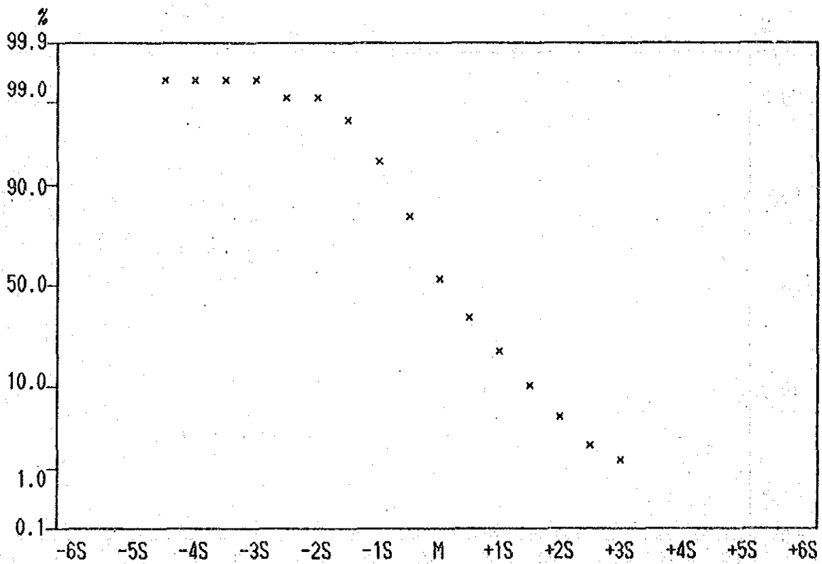
Cumulative Frequency Curve of Zn contents in Lithological Code; KPS
