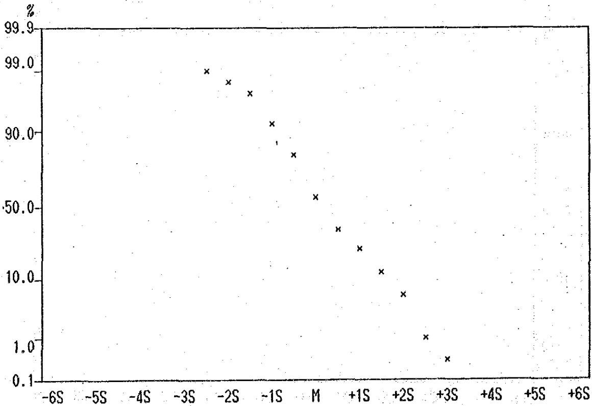
Cumulative Frequency Curve of Zn contents in Lithological Code; KPB
