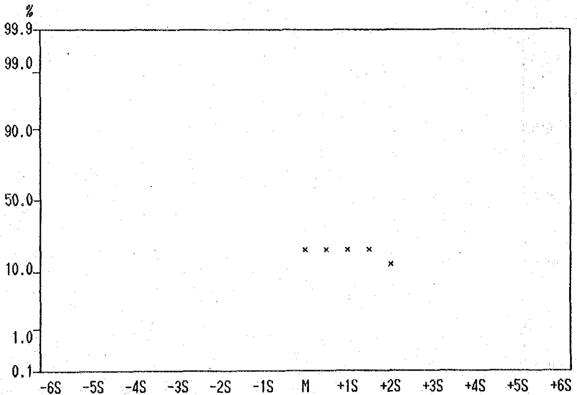
Cumulative Frequency Curve of Pb contents in Lithological Code; KPL
