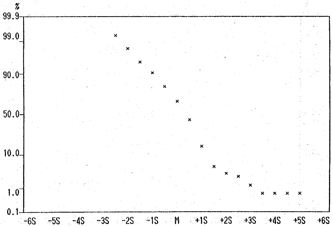
Cumulative Frequency Curve of As contents in Lithological Code; NQS
