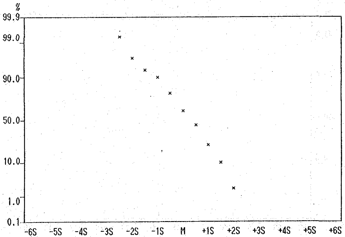
Cumulative Frequency Curve of Cu contents in Lithological Code; NQS
