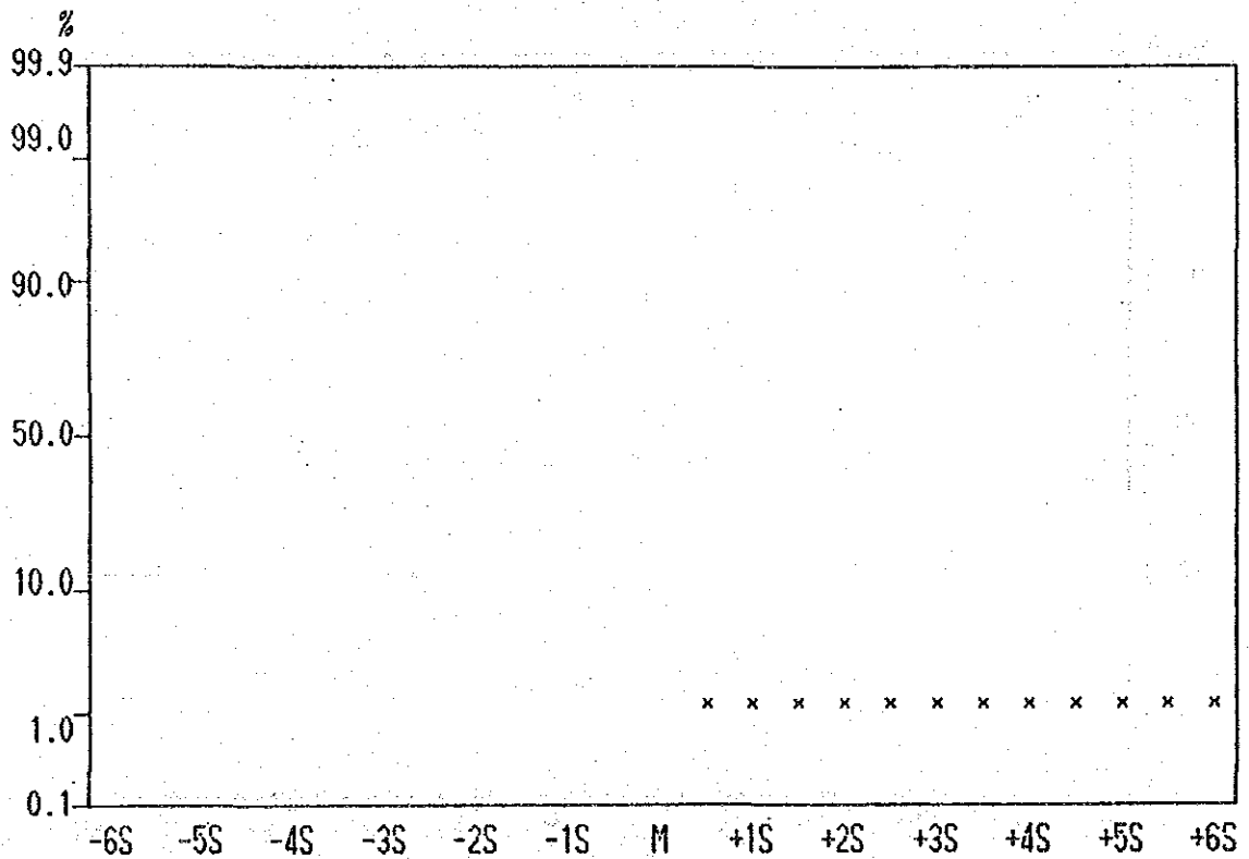
Cumulative Frequency Curve of Pb contents in Lithological Code; NQS
