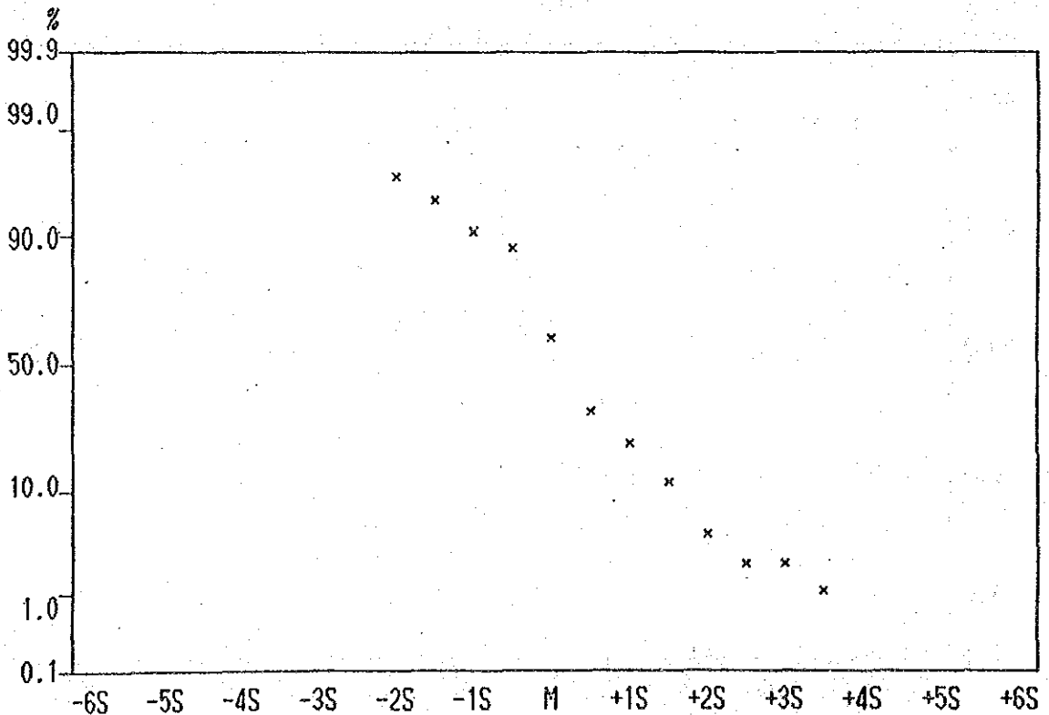
Cumulative Frequency Curve of Co contents in Lithological Code; N1S
