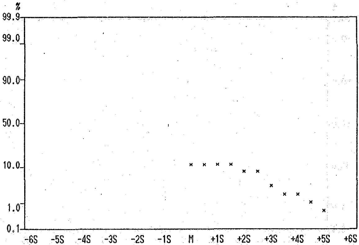
Cumulative Frequency Curve of Mo contents in Lithological Code; N2S
