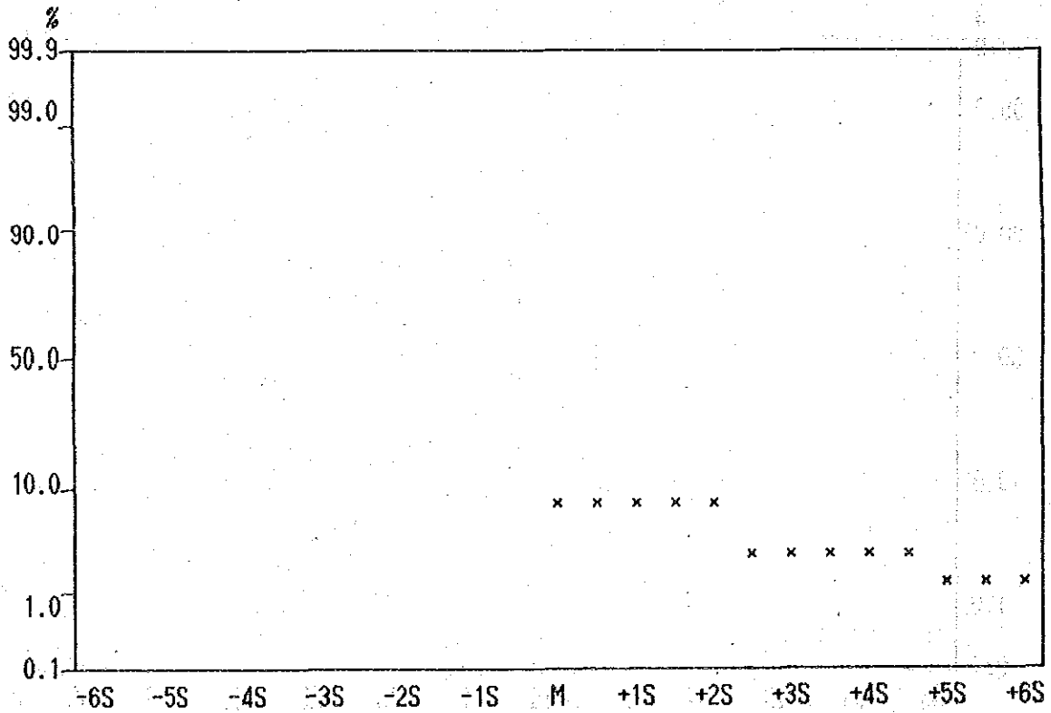
Cumulative Frequency Curve of Hg contents in Lithological Code; N2A
