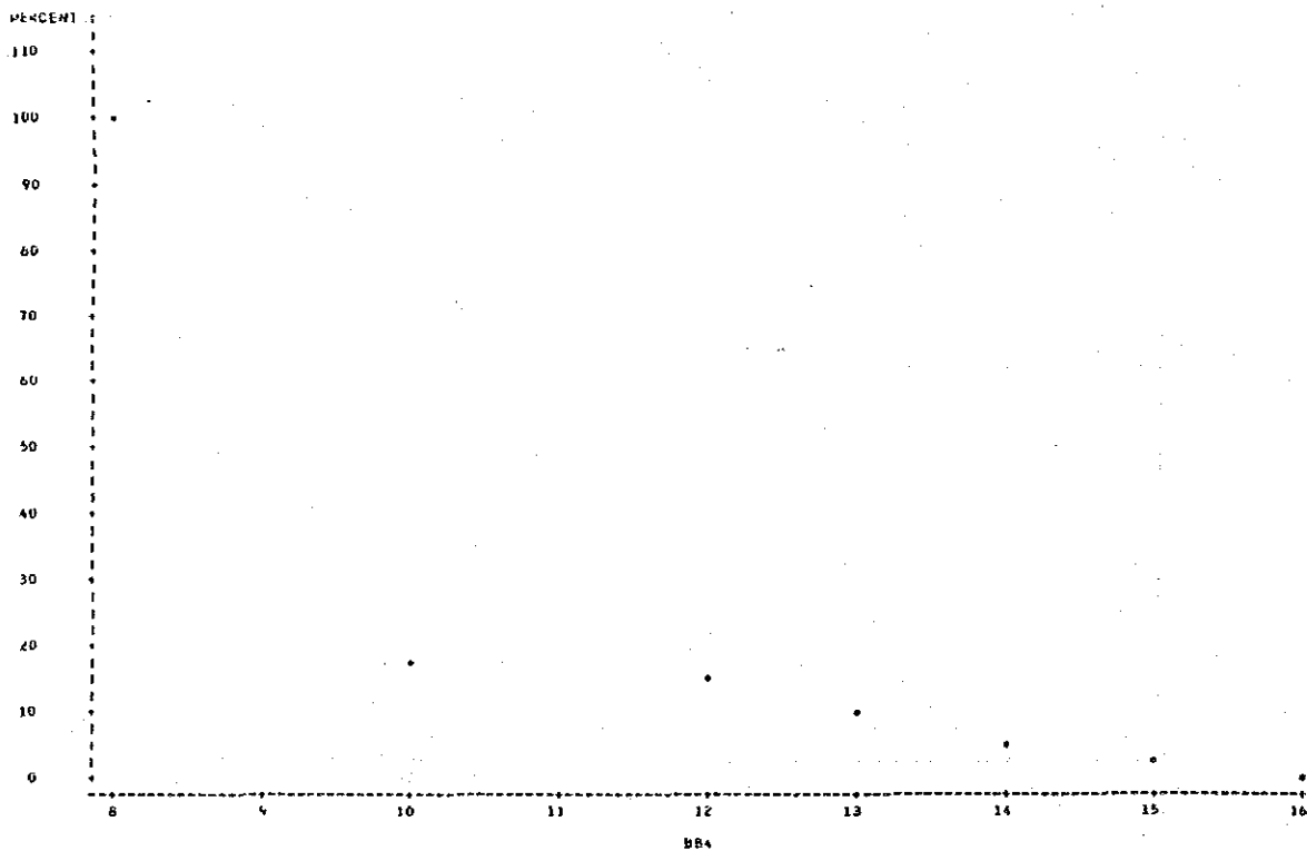
Cumulative Frequency Curve of Ag Contents Distribution in Lithological Code I
