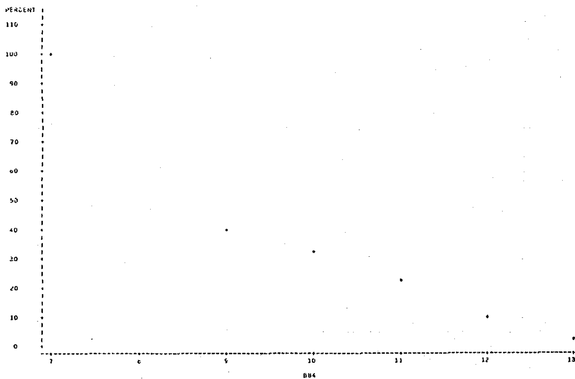
Cumulative Frequency Curve of Ag Contents Distribution in Lithological Code IV
