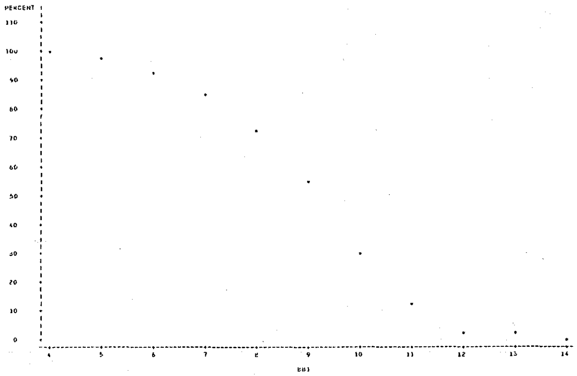
Cumulative Frequency Curve of Cu Contents Distribution in Lithological Code II-III
