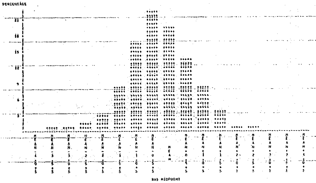
Histogram of N_i Contents Distribution in Lithological Code I
