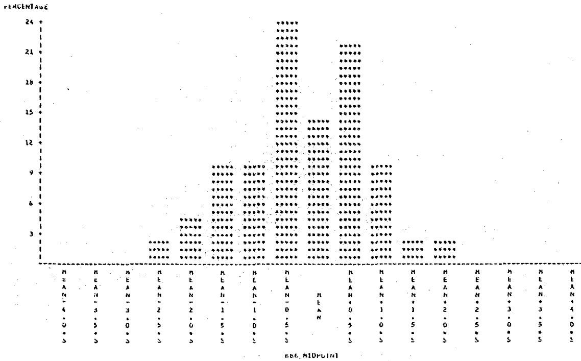
Histogram of Co Contents Distribution in Lithological Code II
