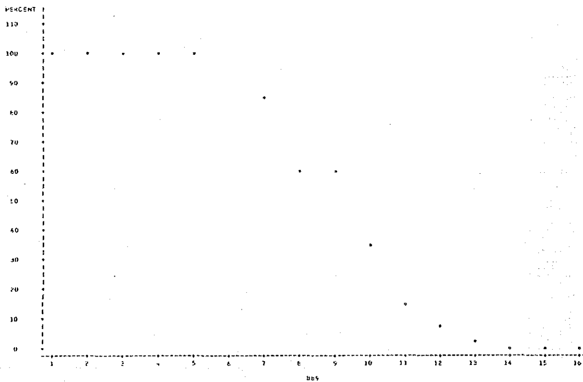
Cumulative Frequency Curve of Hg Contents Distribution in Lithological Code I
