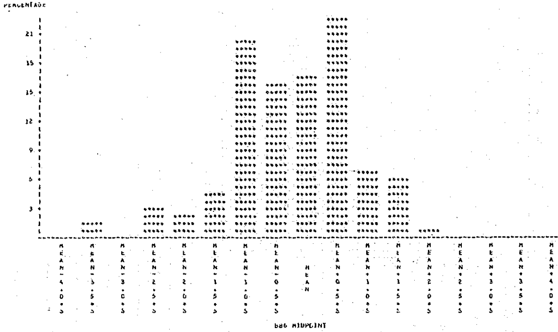
Histogram of Co Contents Distribution in Lithological Code III
