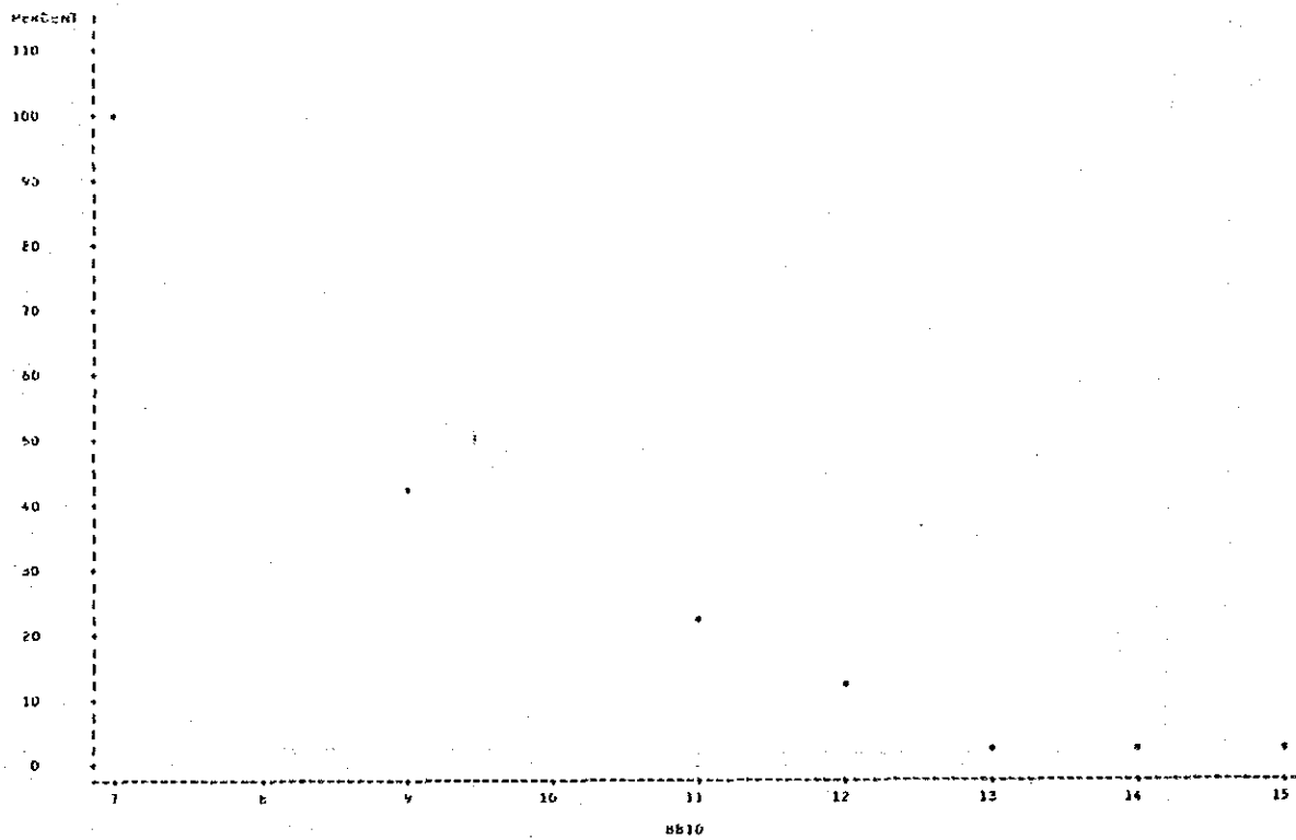
Cumulative Frequency Curve of Mo Contents Distribution in Lithological Code I-VI
