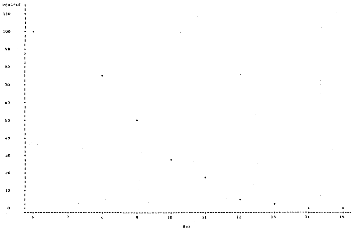
Cumulative Frequency Curve of Pb Contents Distribution in Lithological Code III
