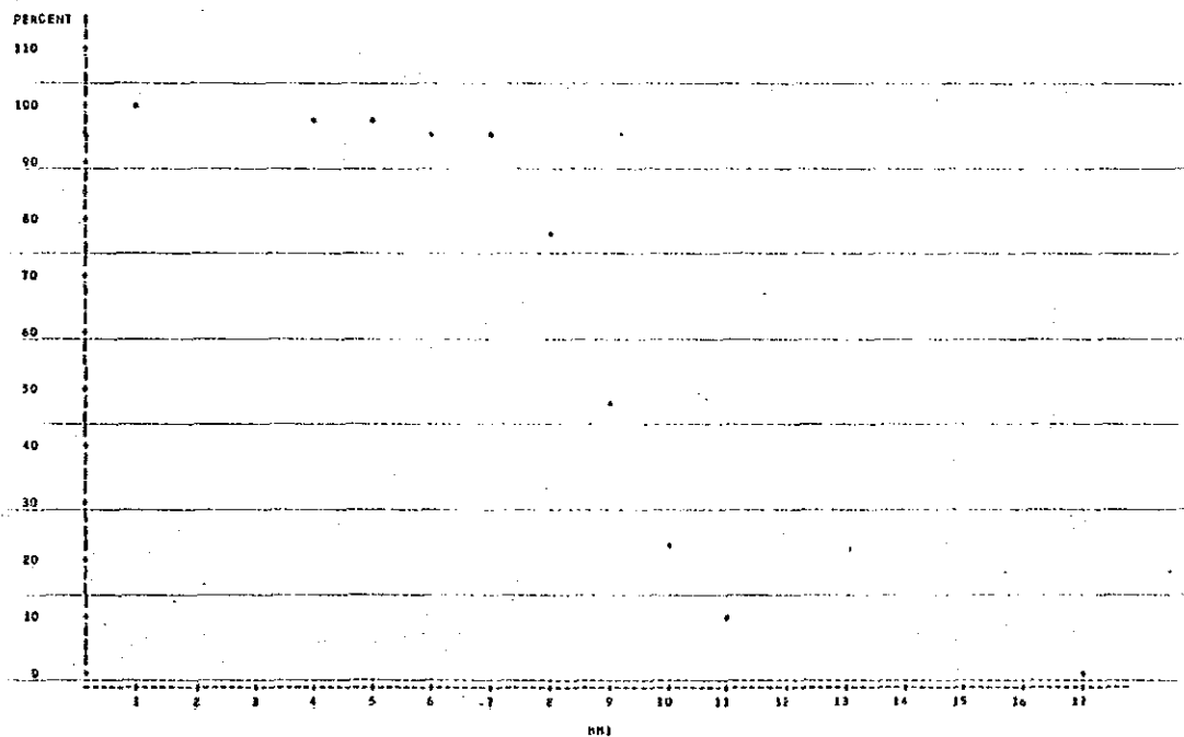
Cumulative Frequency Curve of Cu Contents Distribution in Lithological Code IV
