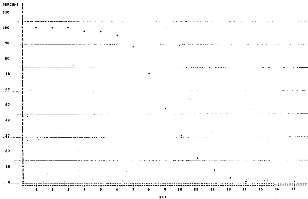
Cumulative Frequency Curve of Zn Contents Distribution in Lithological Code III + IV
