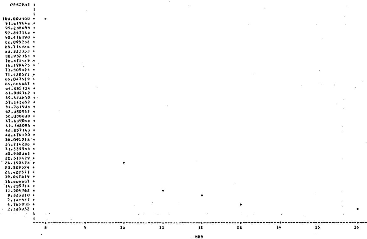
Cumulative Frequency Curve of Hg Contents Distribution in Lithological Code II
