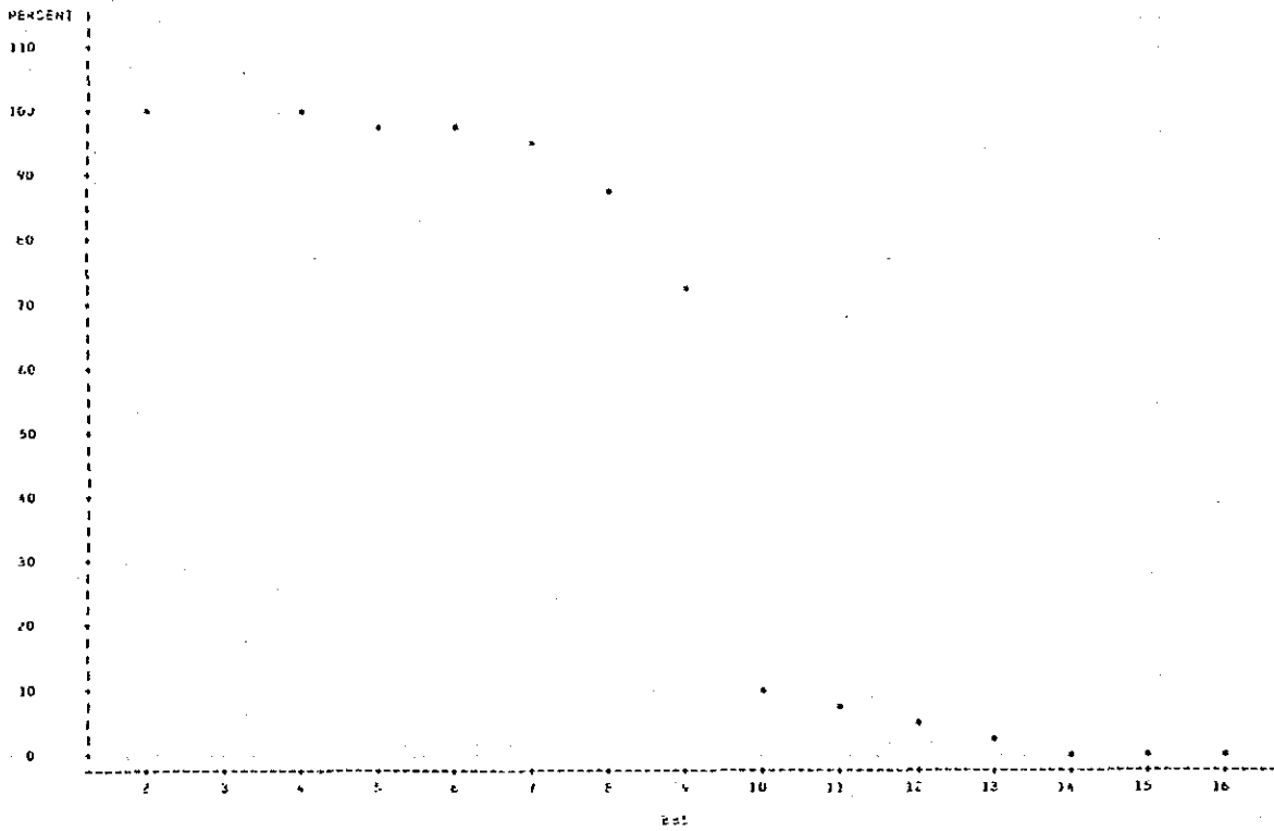
Cumulative Frequency Curve of Ni Contents Distribution in Lithological Code I
