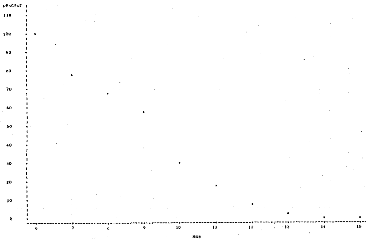
Cumulative Frequency Curve of As Contents Distribution in Lithological Code I
