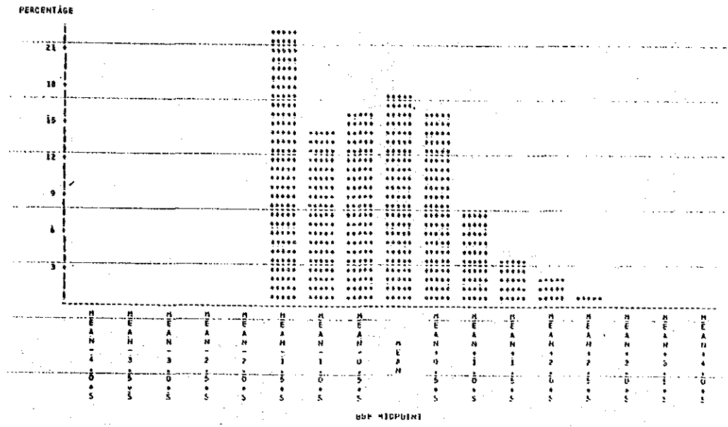
Histogram of As Contents Distribution in Lithological Code III-IV
