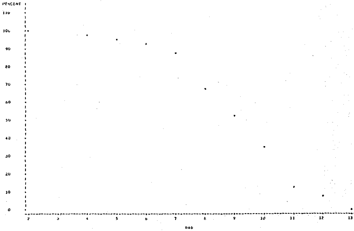
Cumulative Frequency Curve of Co Contents Distribution in Lithological Code III
