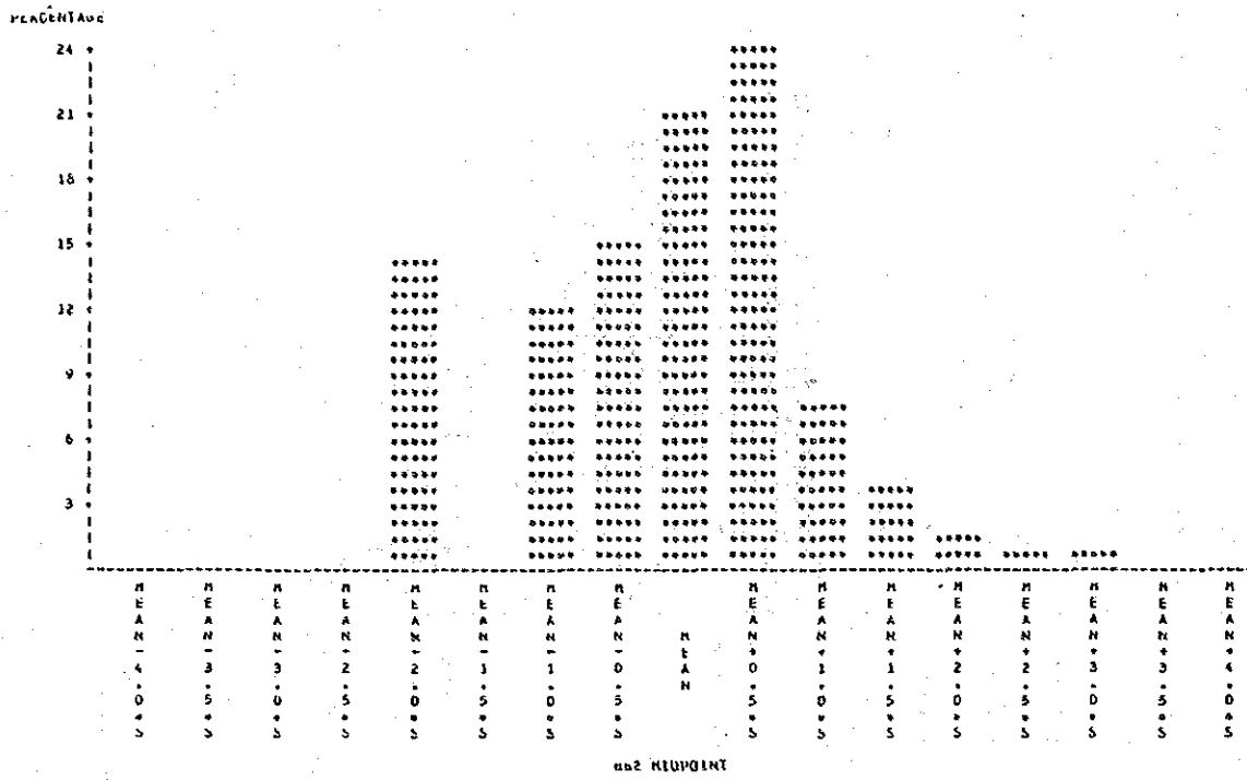
Histogram of Pb Contents Distribution in Lithological Code IV
