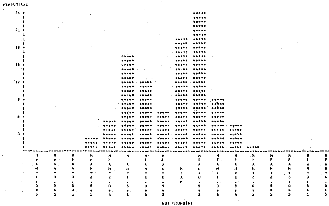
Histogram of Cu Contents Distribution in Lithological Code IV
