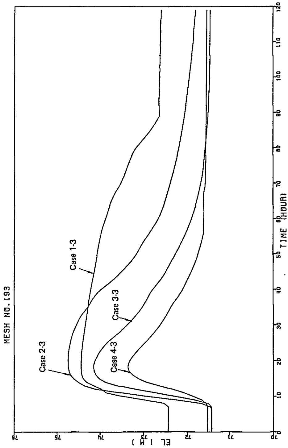
Fig. 5-39 Curves of the Water Level
