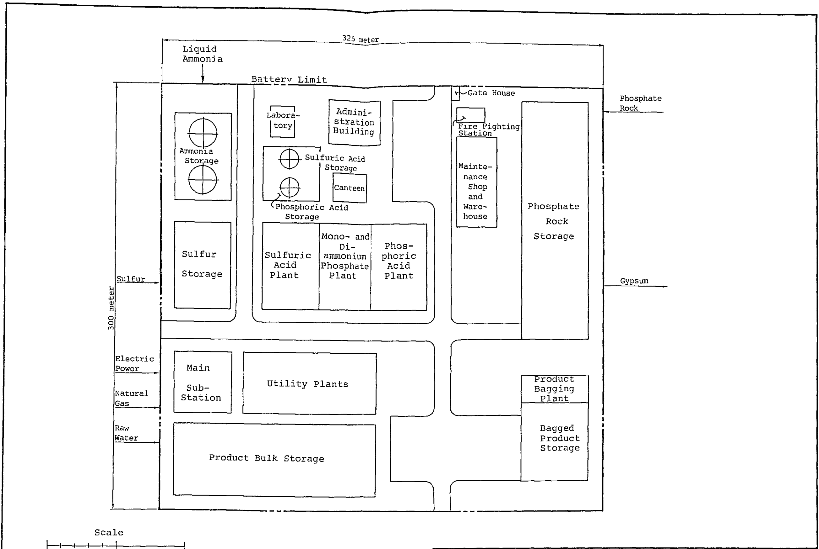
Figure AV-6-2 GENERAL PLOT PLAN FOR PHOSPHATE FERTILIZER PLANT Project: Monoammonium and Diammonium Phosphate Fertilizer Plant ... PF-5 Feasibility Study: The Establishment of a Phosphate Fertilizer Plant in the Argentine Republic. Japan International Cooperation Agency. April, 1984
