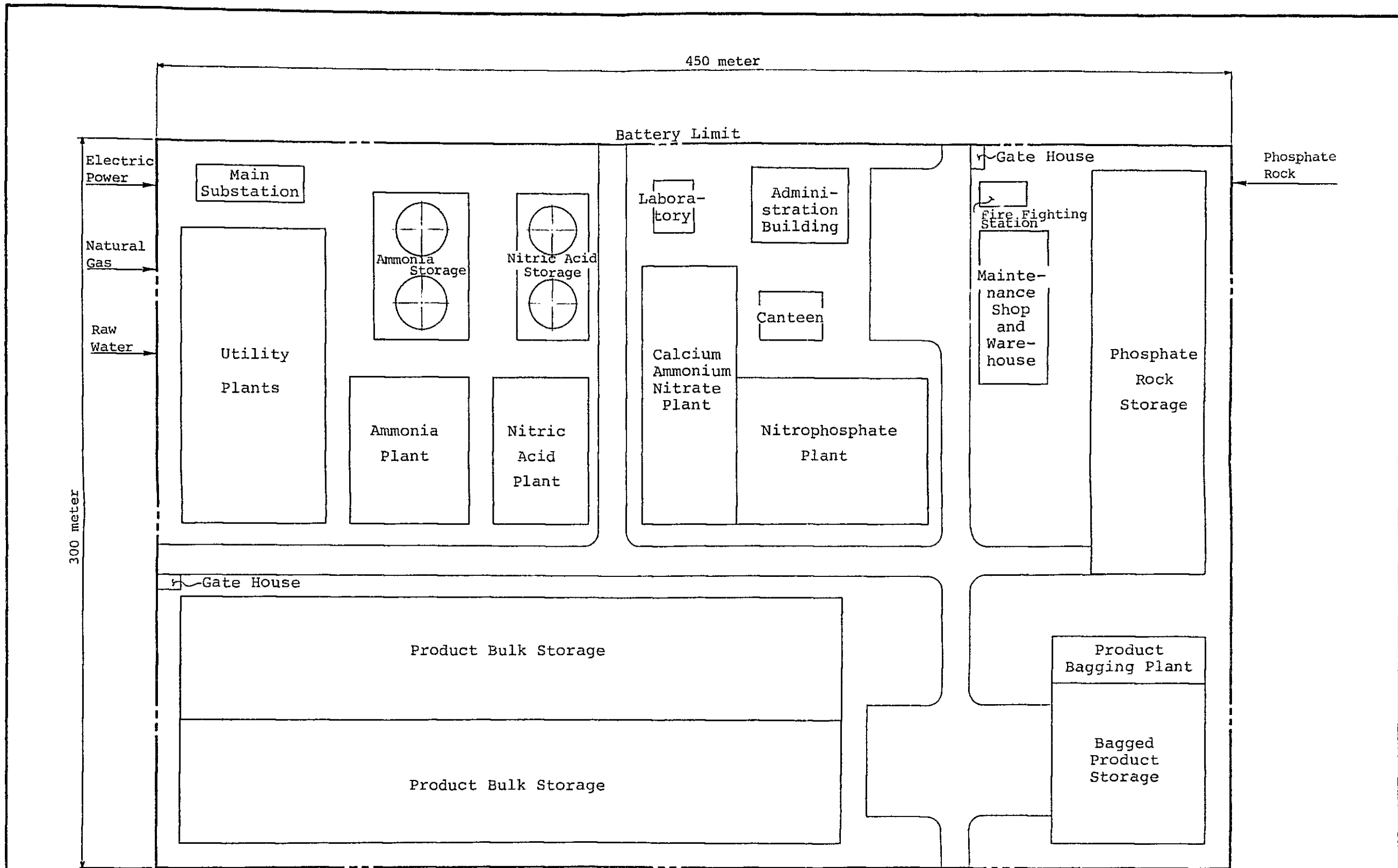
Figure AV-8-2 GENERAL PLOT PLAN FOR PHOSPHATE FERTILIZER PLANT ... PF-7 Project: Nitrophosphate and Calcium Ammonium Nitrate Fertilizer Plan Feasibility Study: The Establishment of a Phosphate Fertilizer Plant in the Argentine Republic. Japan International Cooperation Agency. April, 1984
