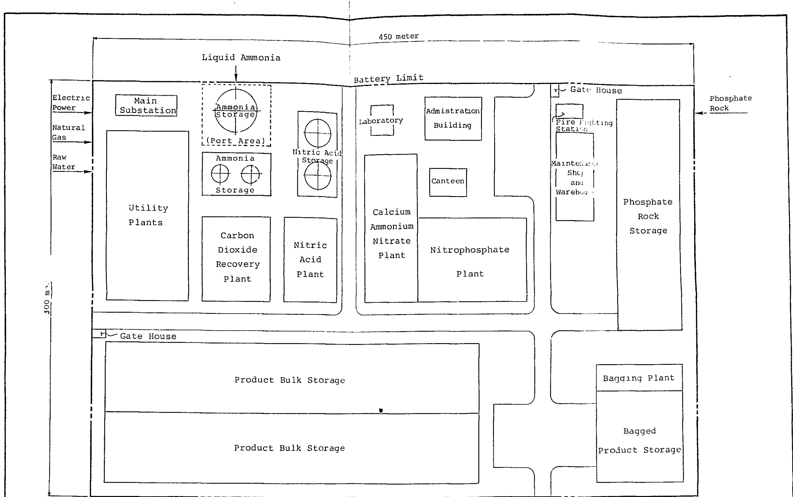
Figure AV-7-2 GENERAL PLOT PLAN FOR PHOSPHATE FERTILIZER PLANT ... PF-6 Project: Nitrophosphate and Calcium Ammonium Nitrate Fertilizer Plan Feasibility Study: The Establishment of a Phosphate Fertilizer Plant in the Argentine Republic. Japan International Cooperation Agency. April, 1984
