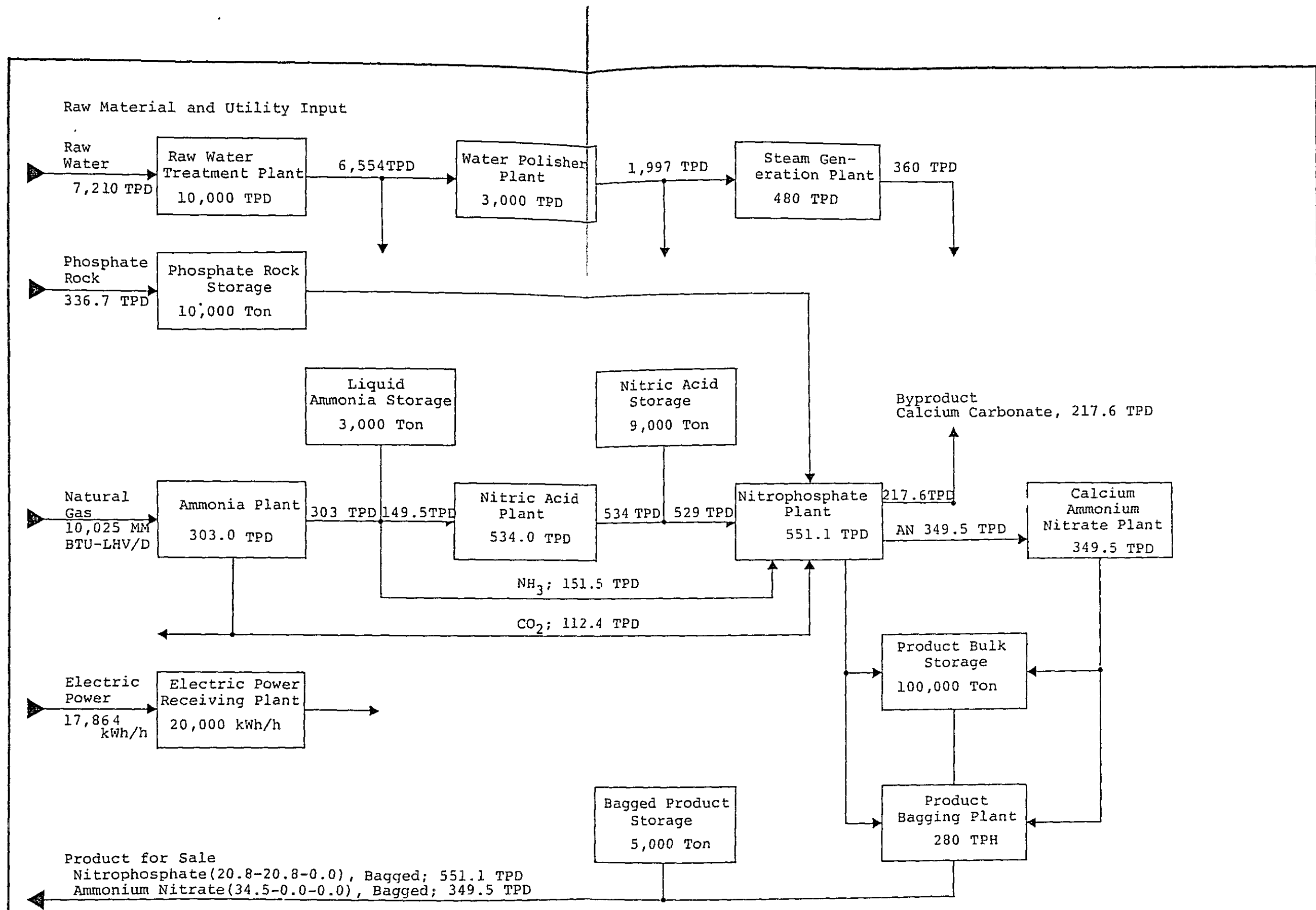
Figure AV-8-1(B) BLOCK FLOW DIAGRAM FOR PHOSPHATE FERTILIZER PLANT Project: Nitrophosphate and Ammonium Nitrate Fertilizer Plant...PF-7 Feasibility Study: The Establishment of a Phosphate Fertilizer Plant in the Argentine Republic. Japan International Cooperation Agency. April, 1984
