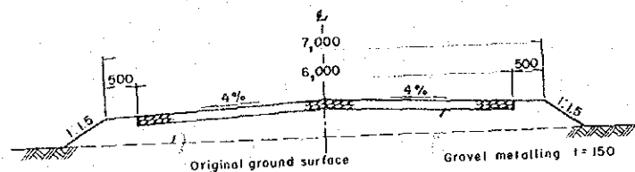
MAIN FARM ROAD & LINKED ROAD
