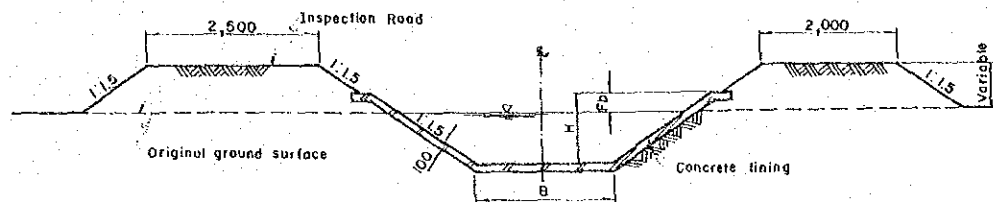
MAIN CANAL & BRANCH CANAL
