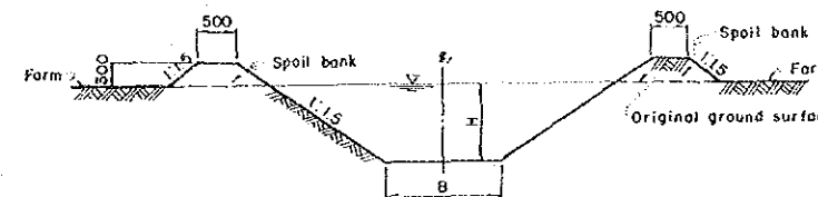
MAIN DRAIN & SECONDARY DRAIN
