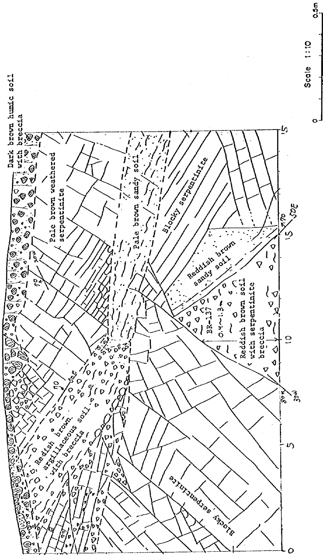
Fig. A-20 Geological Sketch of V-19 Pit
