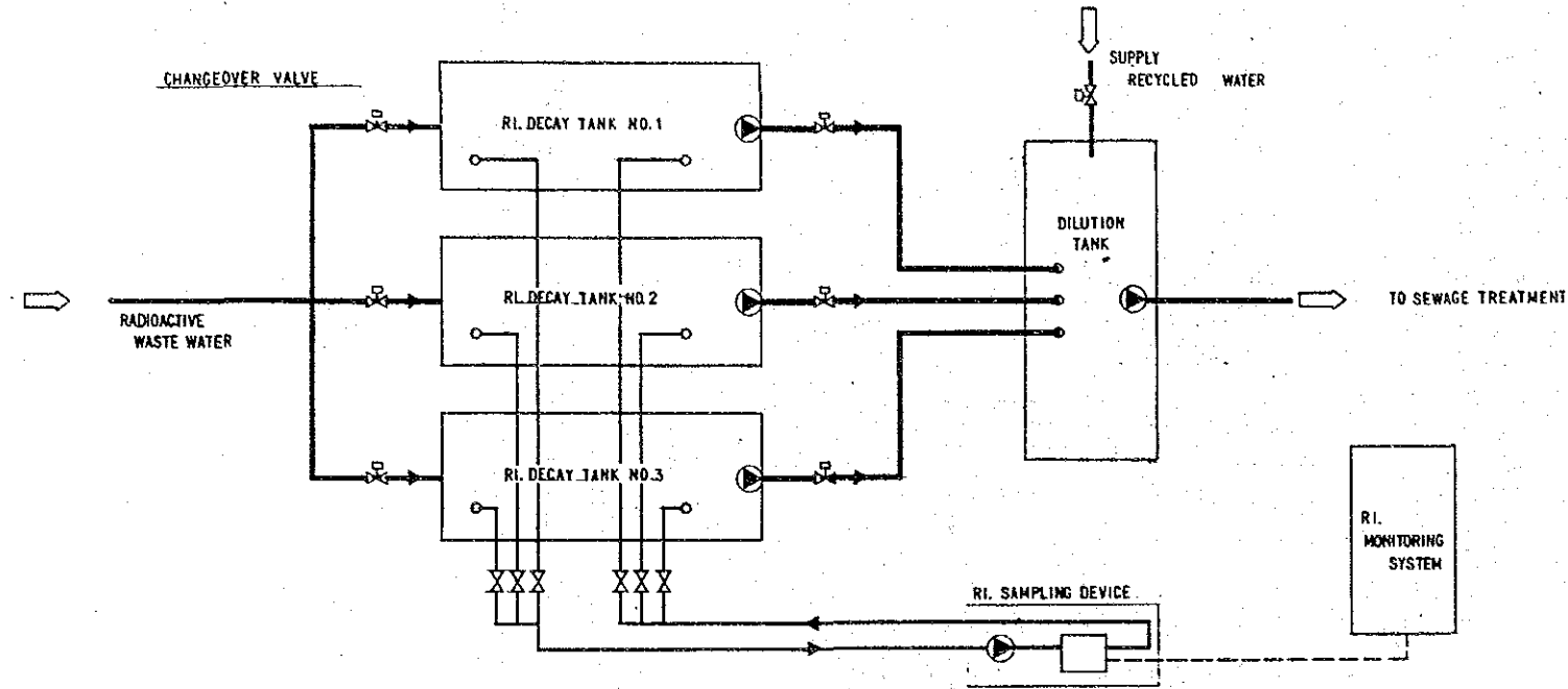
RADIOACTIVE WASTE WATER TREATMENT DIAGRAM
