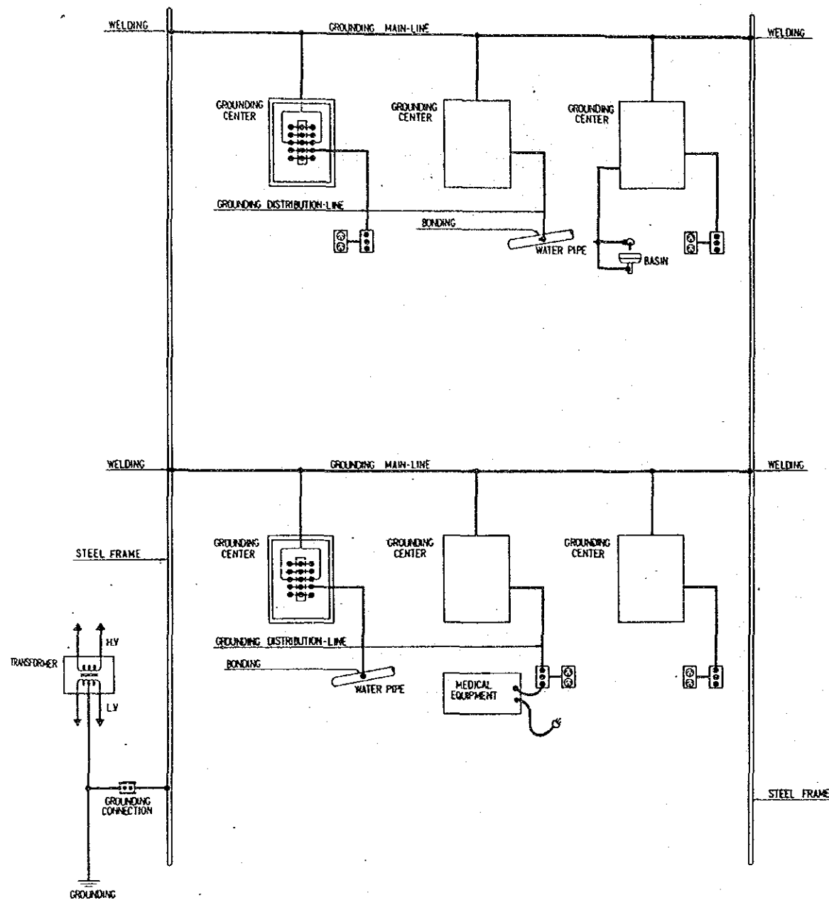
CONCEPT OF GROUNDING SYSTEM
