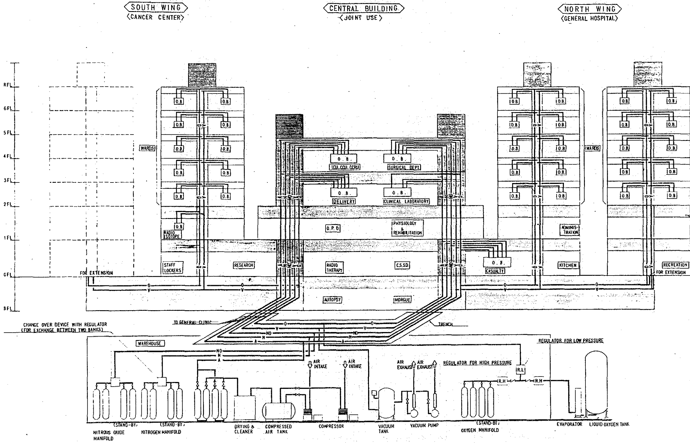
MEDICAL GAS SUPPLY SYSTEM DIAGRAM
