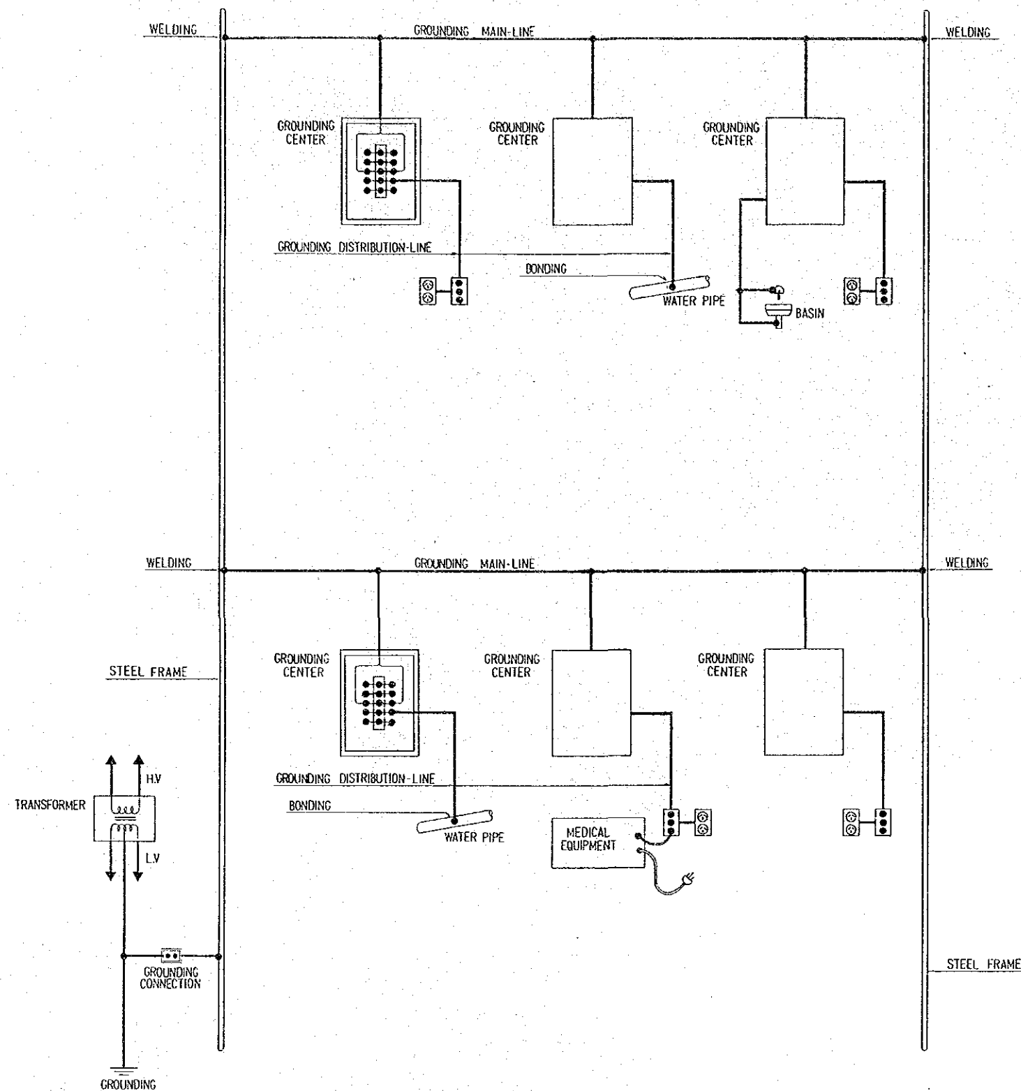
CONCEPT OF GROUNDING SYSTEM
