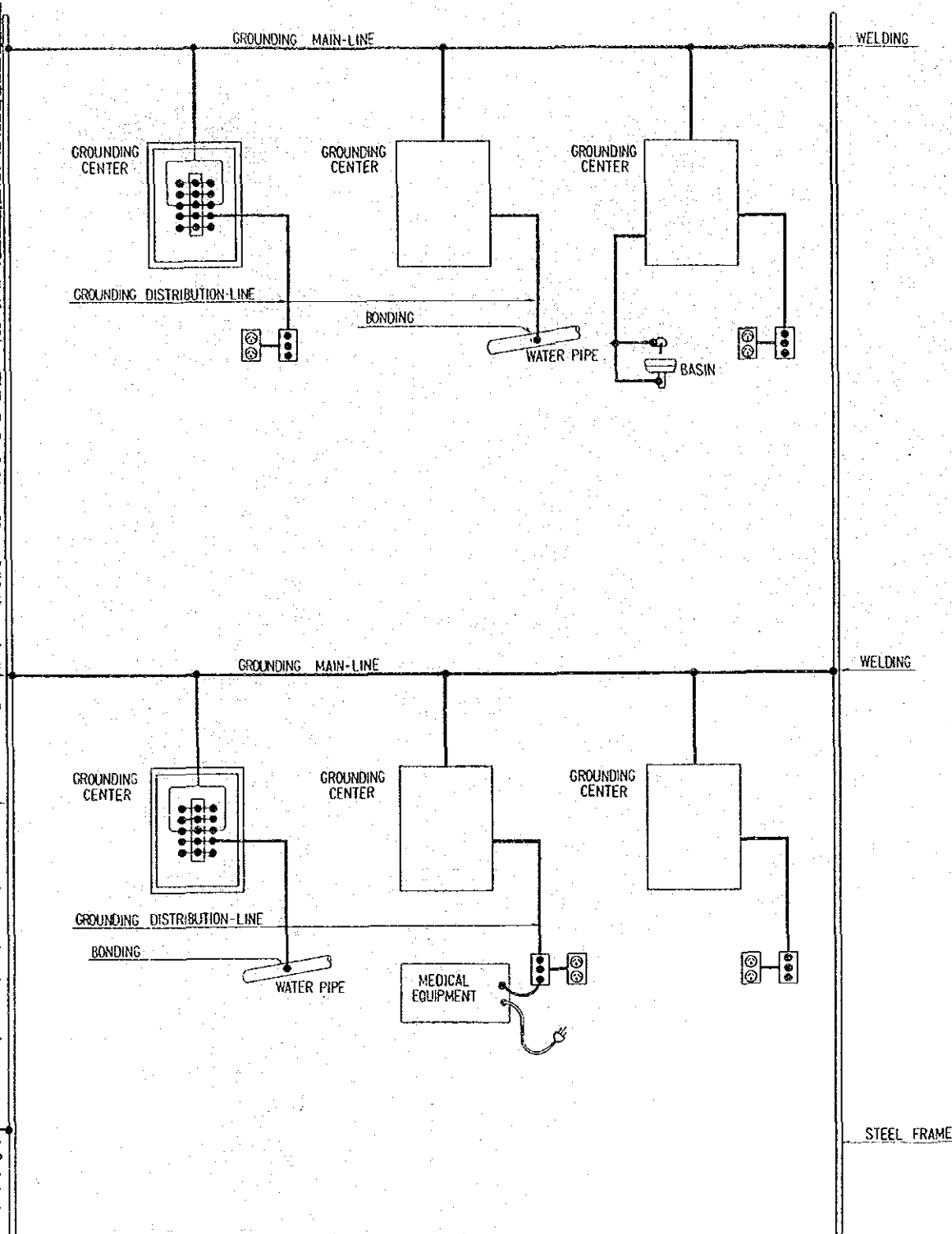
CONCEPT OF GROUNDING SYSTEM
